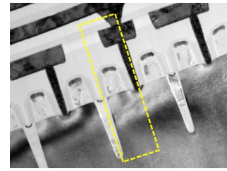
Fig.1. eSTM cell Transmission Electron Microscopy (TEM) cross section. Doted line highlight one bitcell.
