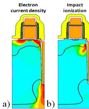
Fig. 3. TCAD simulations of (a) electron current density and (b) impact ionization during programming operation.
