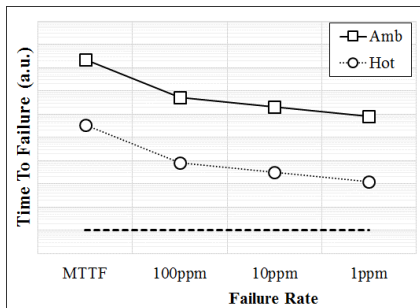
Fig. 13: Select transistor gate oxide lifetime extrapolation at ambient( 25^\circ C ) and hot temperature ( 125^\circ C ) showing high margin versus specification.
