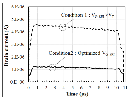
Fig. 17. Dynamic drain current measured during programming step: current consumption peak is in the range of 1\mu A .
