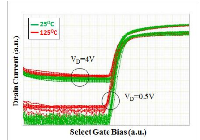
Fig. 12. Select transistor I_d(V_g) curves for both read ( V_d=0.5V ) and write ( V_d=4V ) conditions at ambient ( 25^\circ C ) and hot temperature ( 125^\circ C ).
