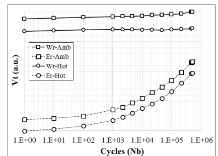
Fig.18. eSTM single cell erase and program threshold evolution during cycling at ambient ( 25^\circ C ) and hot temperature ( 125^\circ C ).
