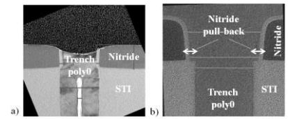
Fig.10. TEM cross-section (a) without and (b) with nitride pull-back process.
