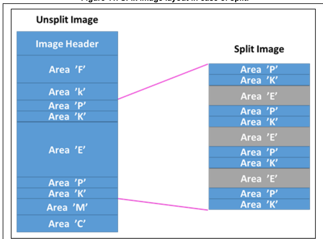
Figure 11. SFIx image layout in case of split.
