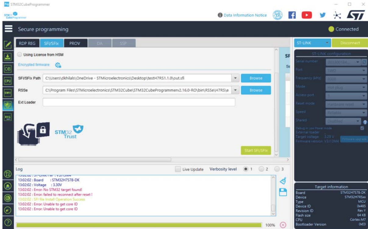
Figure 61. STM32H7Rx/7Sx SFI successful programming via GUI
