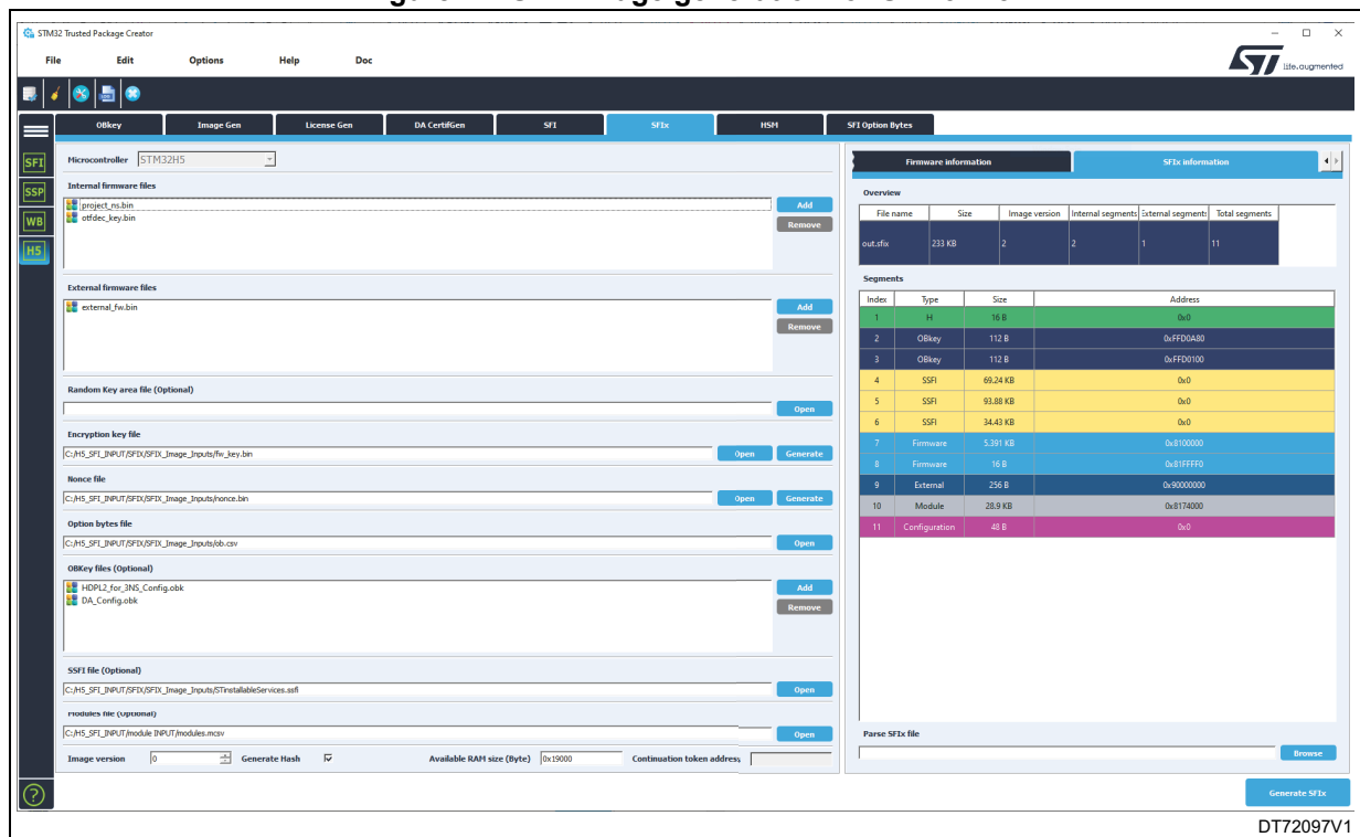
Figure 77. SFlx image generation for STM32H5
