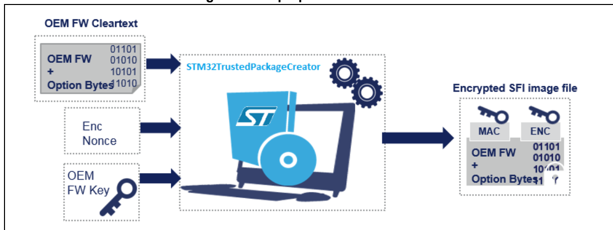
Figure 1. SFI preparation mechanism
