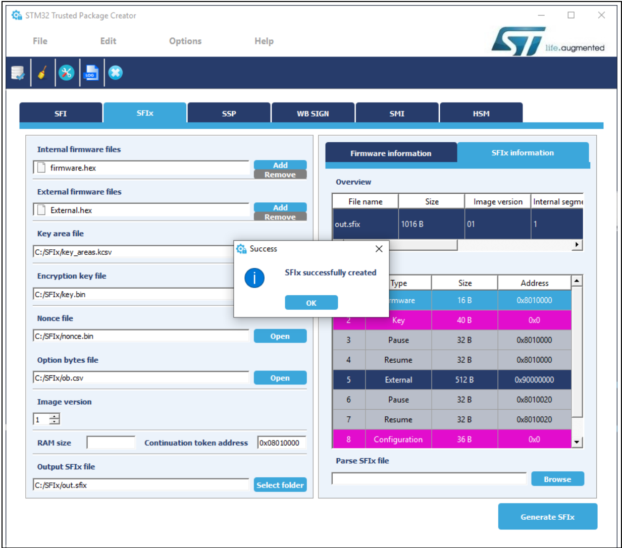
Figure 62. Successful SFIx generation
