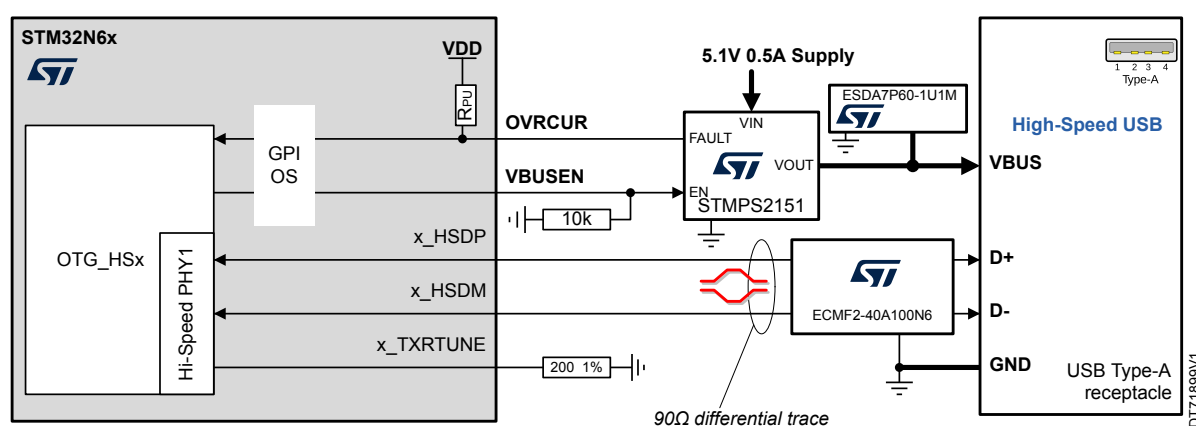
Figure 14. USB hi-speed host example
