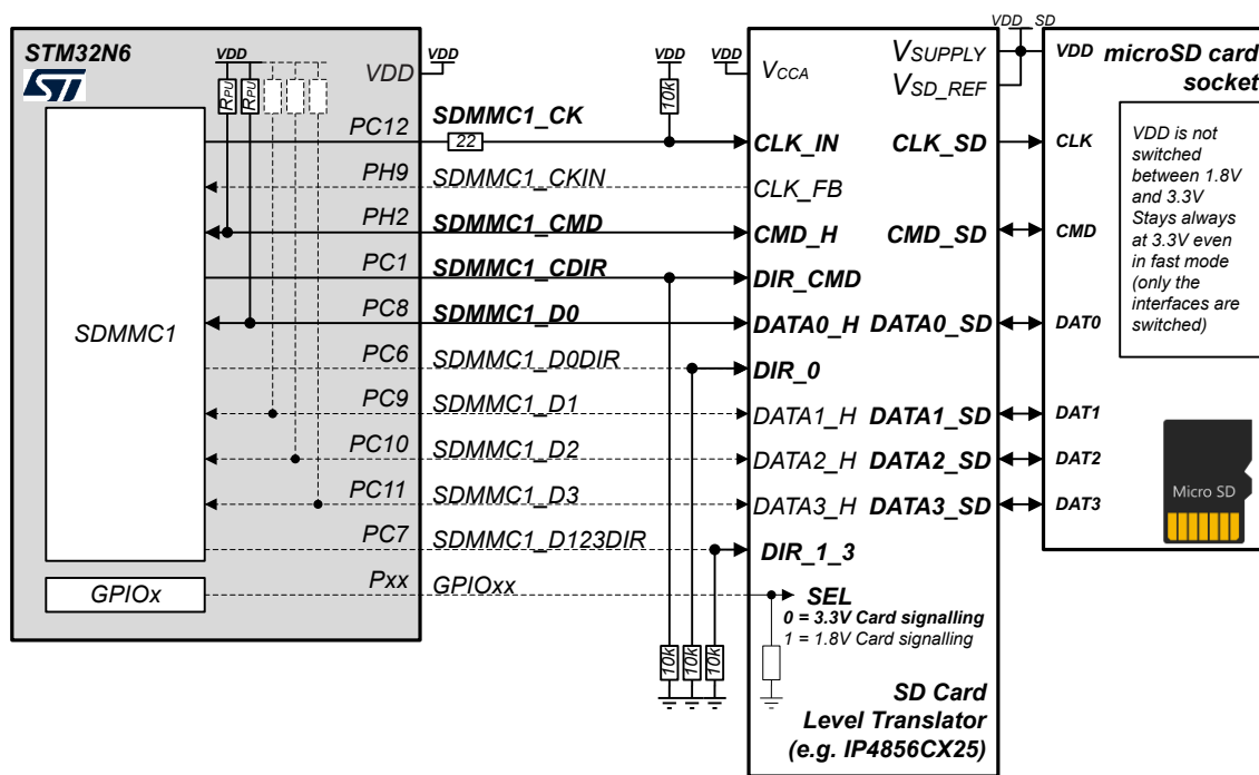
Figure 26. SD card interconnection example
