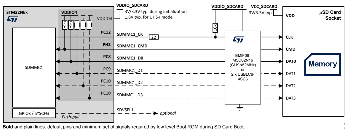
Figure 13. SD-Card with embedded level shifter connection
