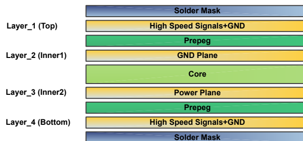
Figure 21. Layer PCB stack-up
