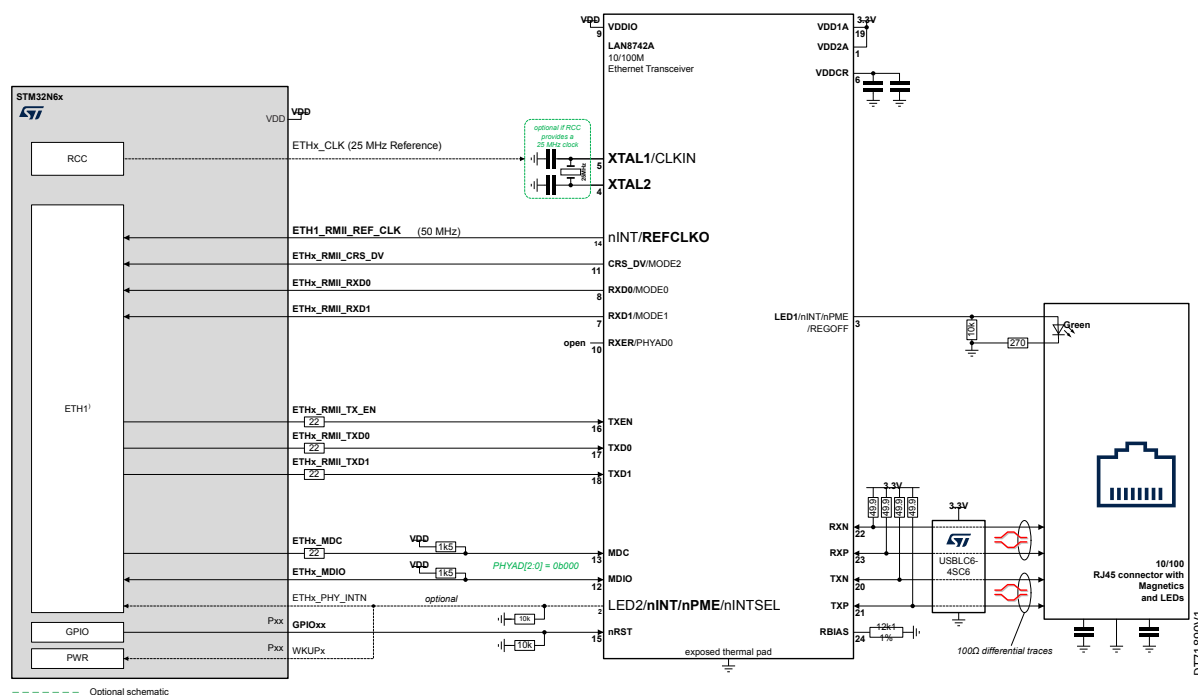
Figure 15. 10/100M Ethernet PHY connection example
