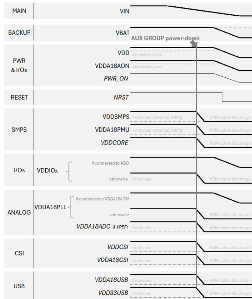
Figure 4. Power-off sequence with V_{DD} = 1.8\text{ V}
