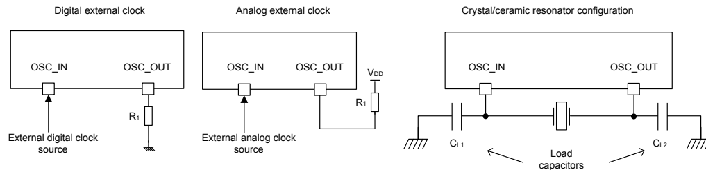
Figure 10. HSE source clock
