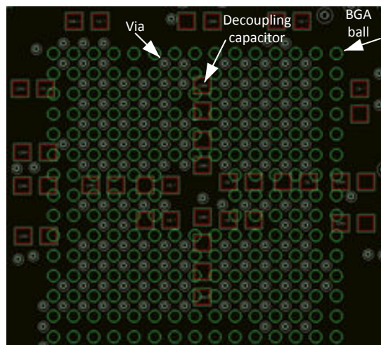
Figure 24. Example of decoupling capacitor placed underneath
