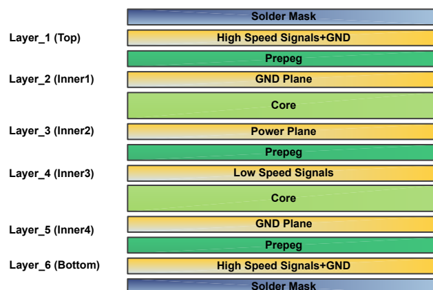
Figure 22. Six layer PCB stack-up example
