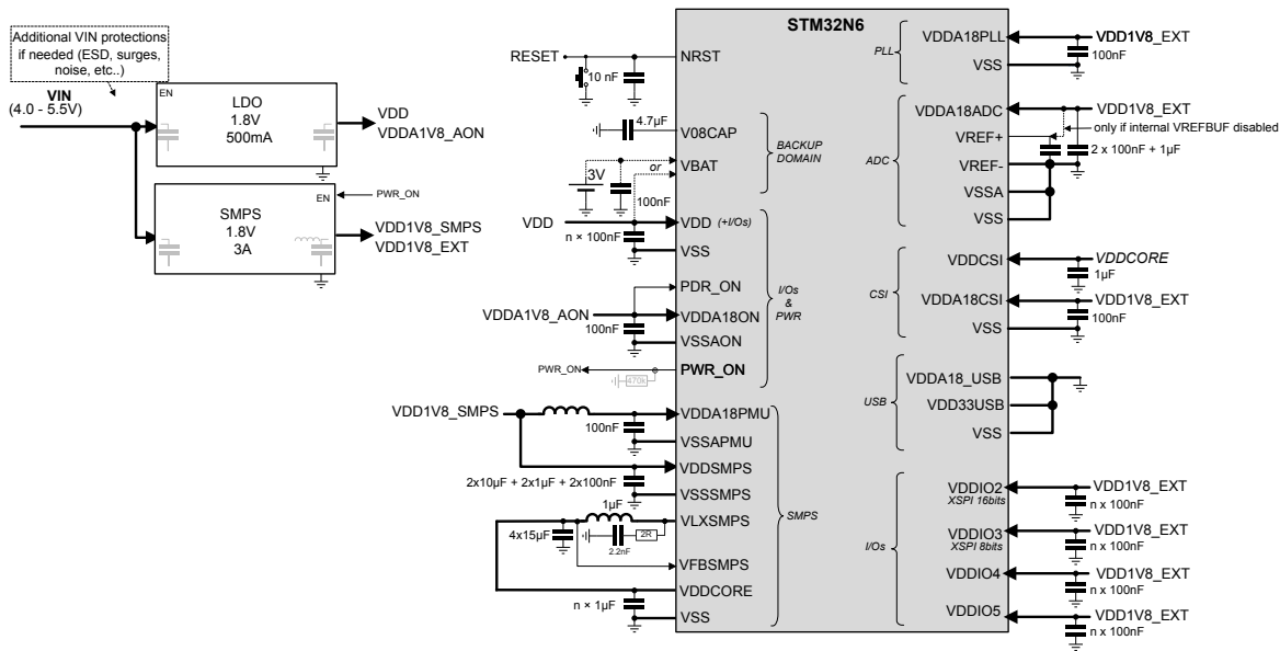
Figure 6. STM32N6 - V_{DD} = 1.8\text{ V} - Internal SMPS – no USB application example
