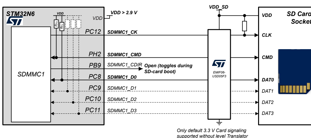
Figure 26. SD card interconnection example
