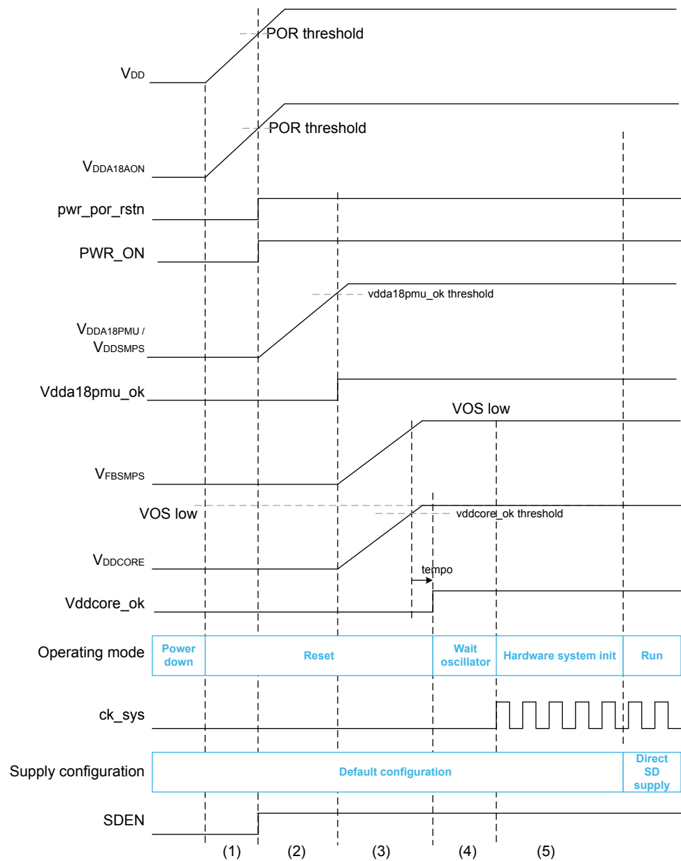
Figure 7. Device startup with V DDCORE supplied directly from SMPS step-down converter
