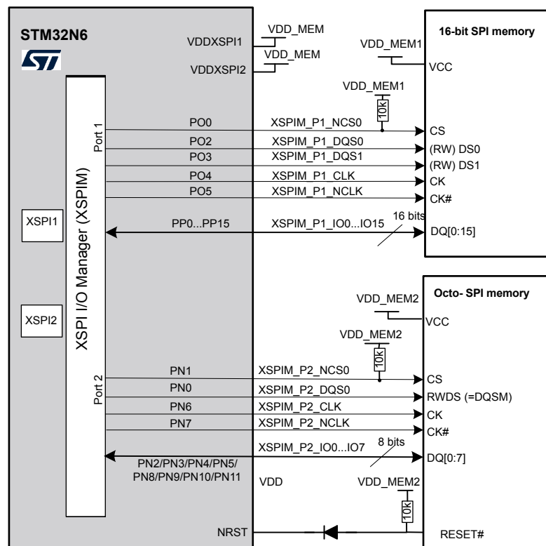
Figure 27. XSPI direct mode example
