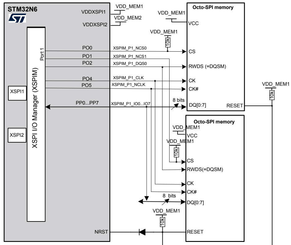
Figure 28. XSPI multiplexed interconnection example
