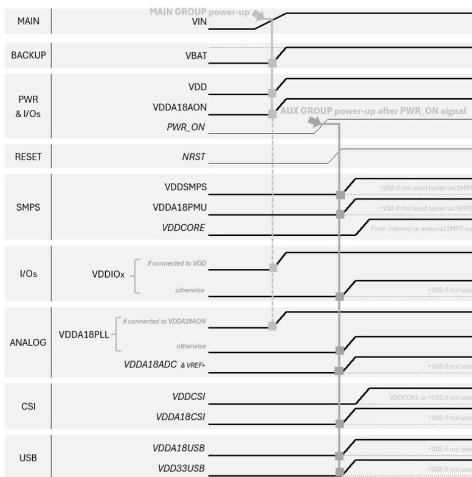
Figure 2. STM32N6 power-on sequence (two steps execution)
