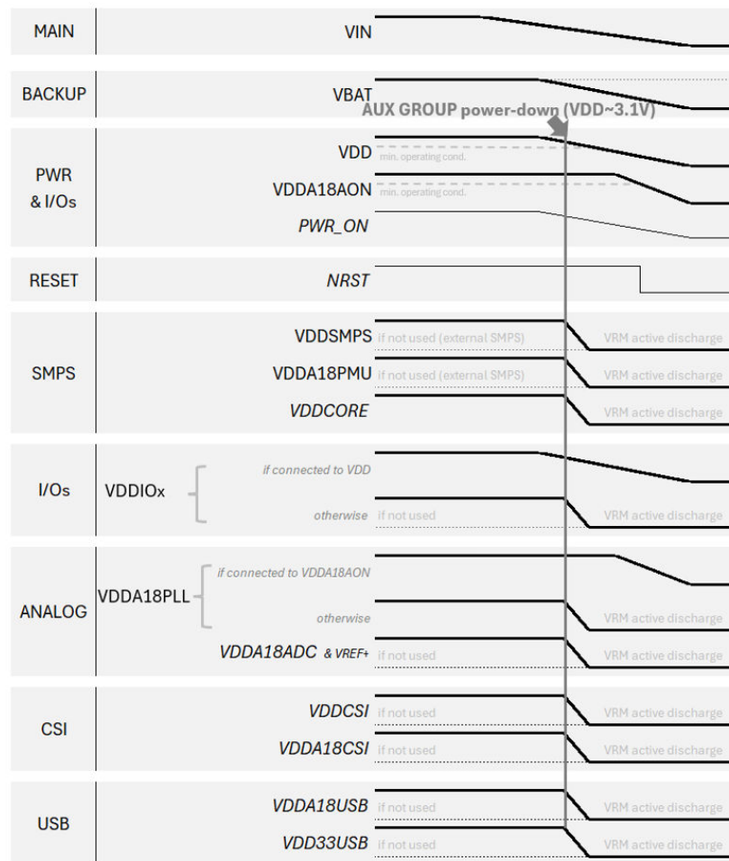
Figure 3. Power off sequence with V_{DD} = 3.3\text{ V}
