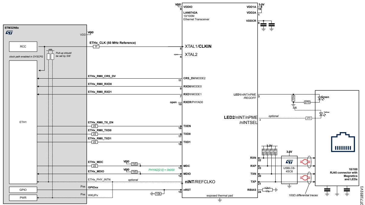
Figure 16. 10/100M Ethernet PHY connection (with REFCLK from RCC)
