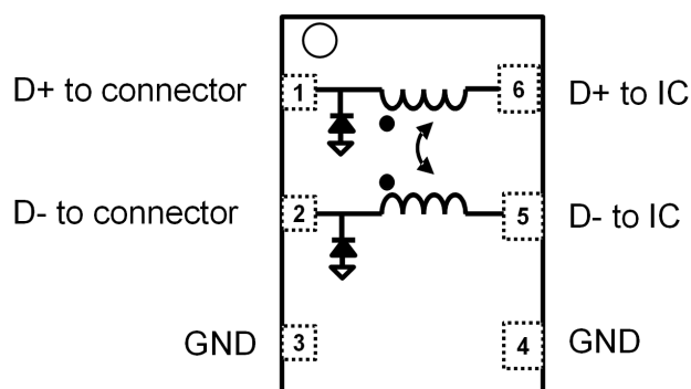
Figure 13. ECMF2-40A100M6Y functional diagrams
