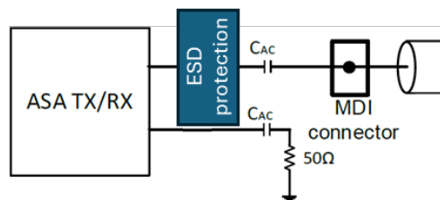
Figure 8. ESD protection implementation on a single-ended system
