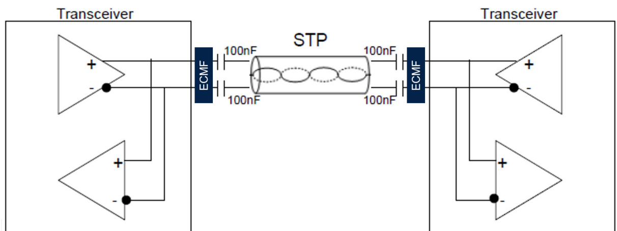
Figure 12. ECMF implementation on a differential system
