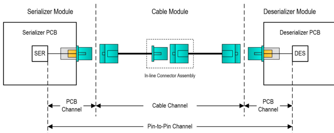
Figure 4. Channel definition
