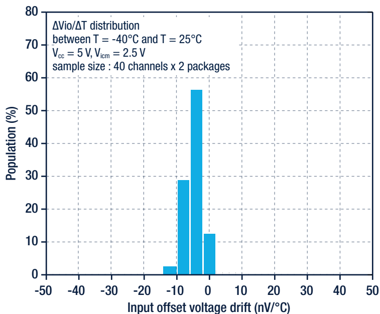
Input offset voltage temperature drift distribution at V_{cc} = 5 V (-40°C to 25°C)
