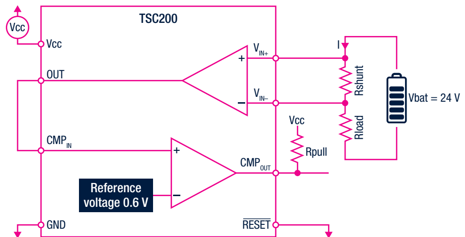
Figure 3 OCP function with dedicated device TSC200
