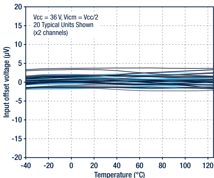
Vio vs. temperature
