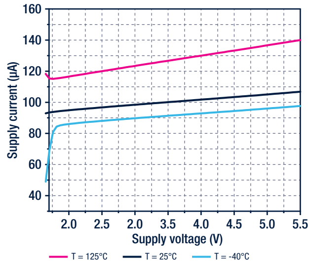
Supply current vs. supply voltage at V_{icm} = V_{CC} , output high
