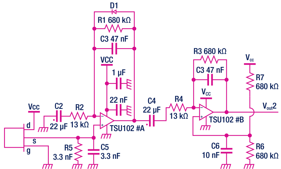
Figure 2: PIR schematics
