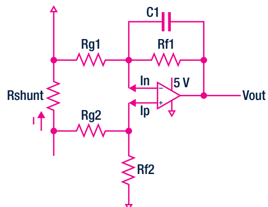
Low-side current sensing schematic
