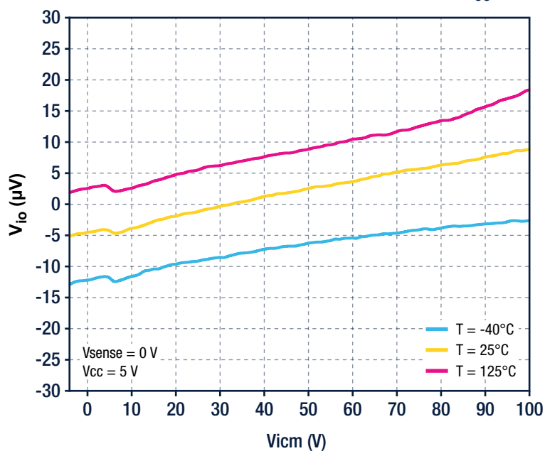
Input offset voltage vs. input common-mode with V_{CC} = 5 \text{ V}
