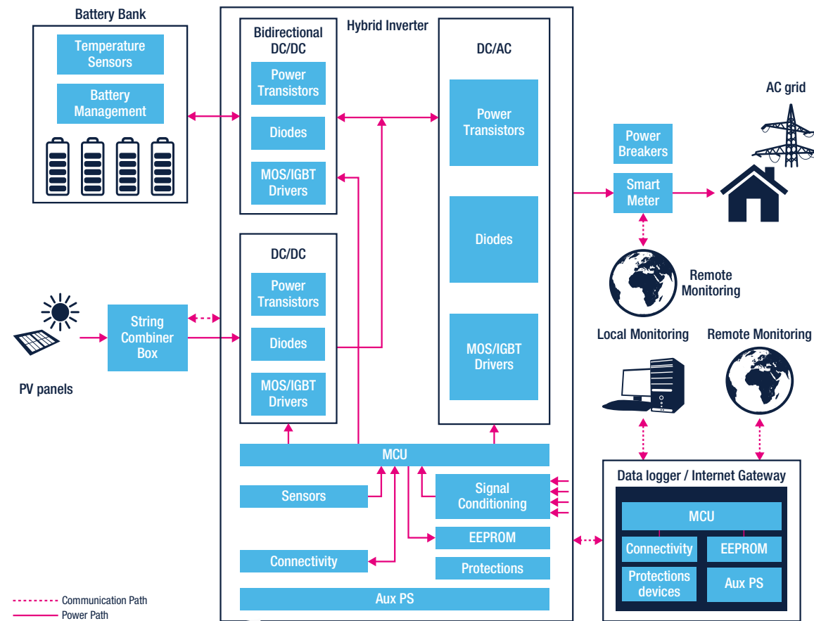
Typical block diagram - home battery storage system
