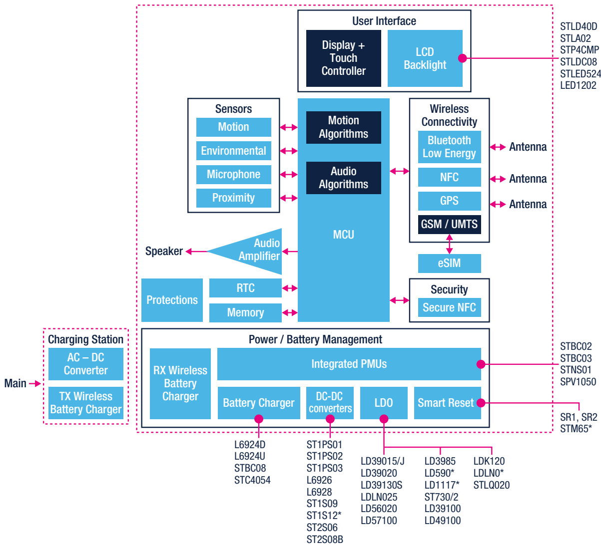
Typical block diagram of a smart watch
