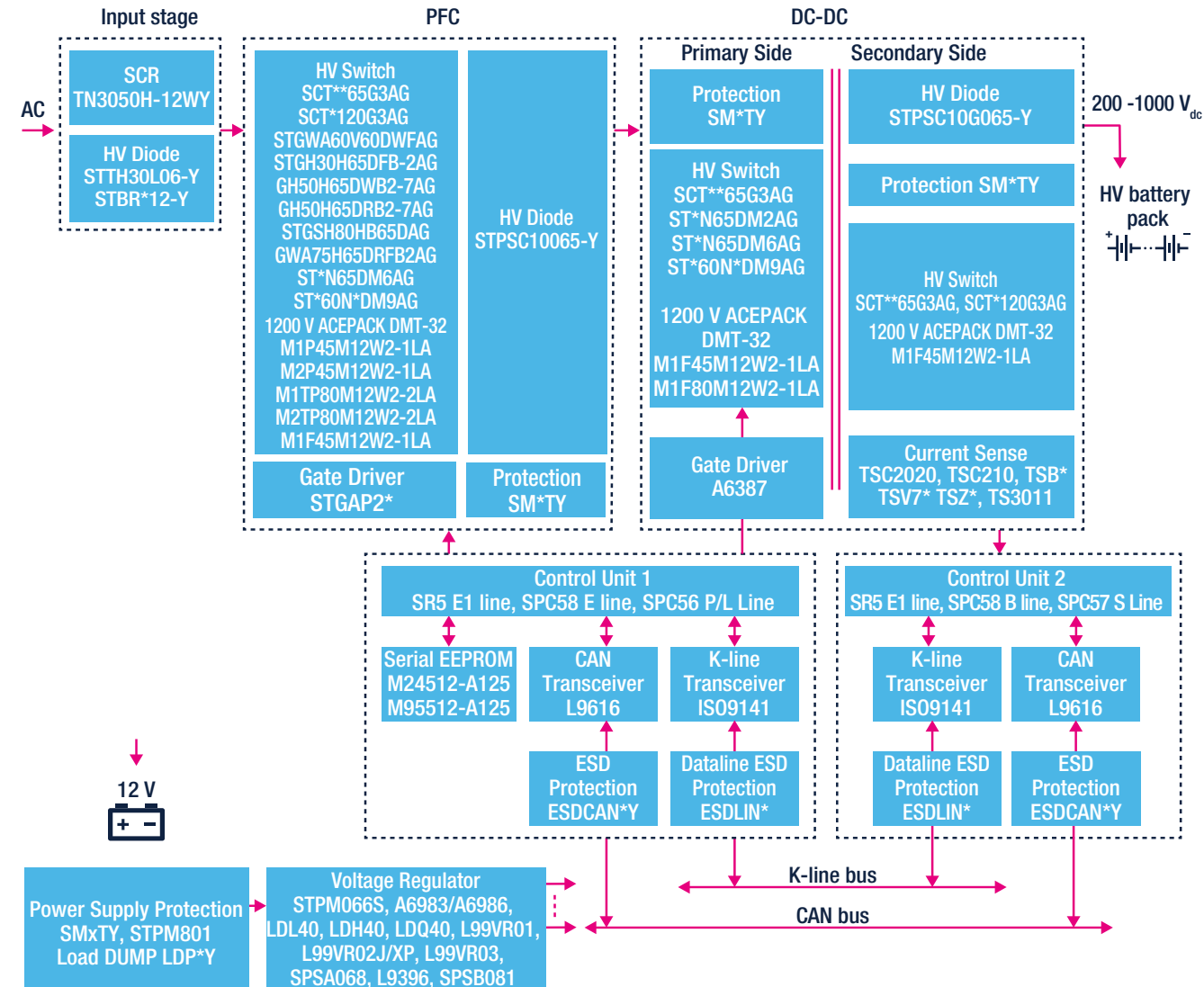
Typical block diagram - OBC
