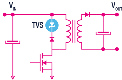
MOSFET protection with TVS
