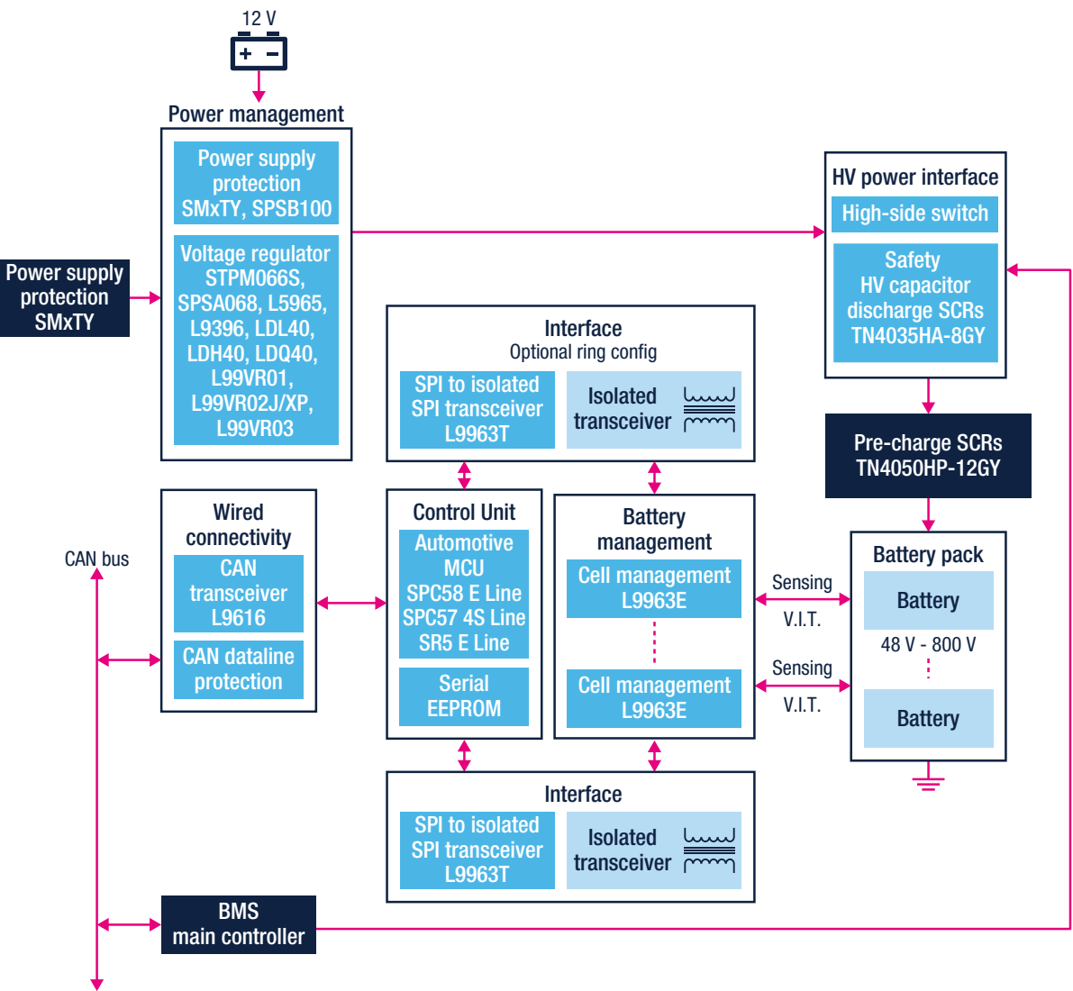
Typical block diagram - automotive battery management system (BMS)
