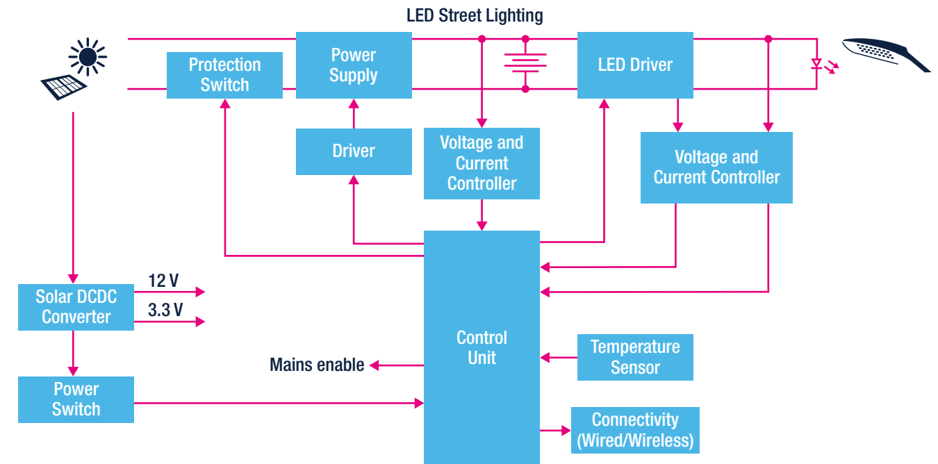
Typical block diagram
