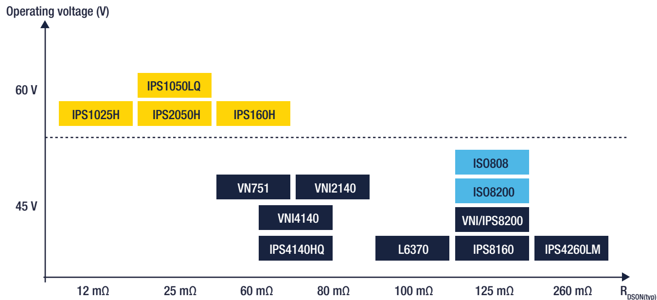
Industrial power switches—high-side and low-side Positioning by operating voltage and on-resistance
