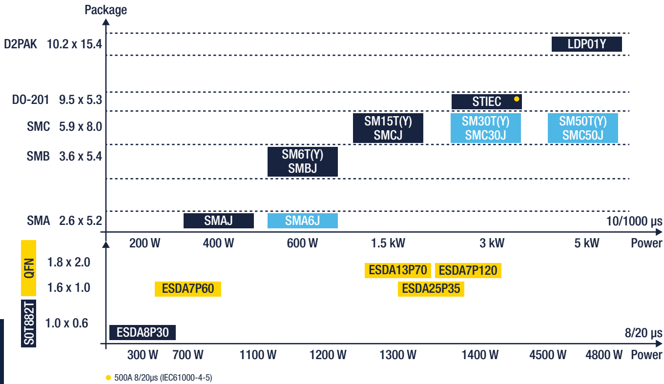
TVS Transil series against repetitive overvoltage in high temperature conditions
