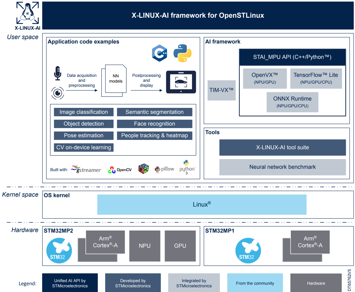
Figure 1. X-LINUX-AI architecture
