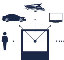
Semantic segmentation
