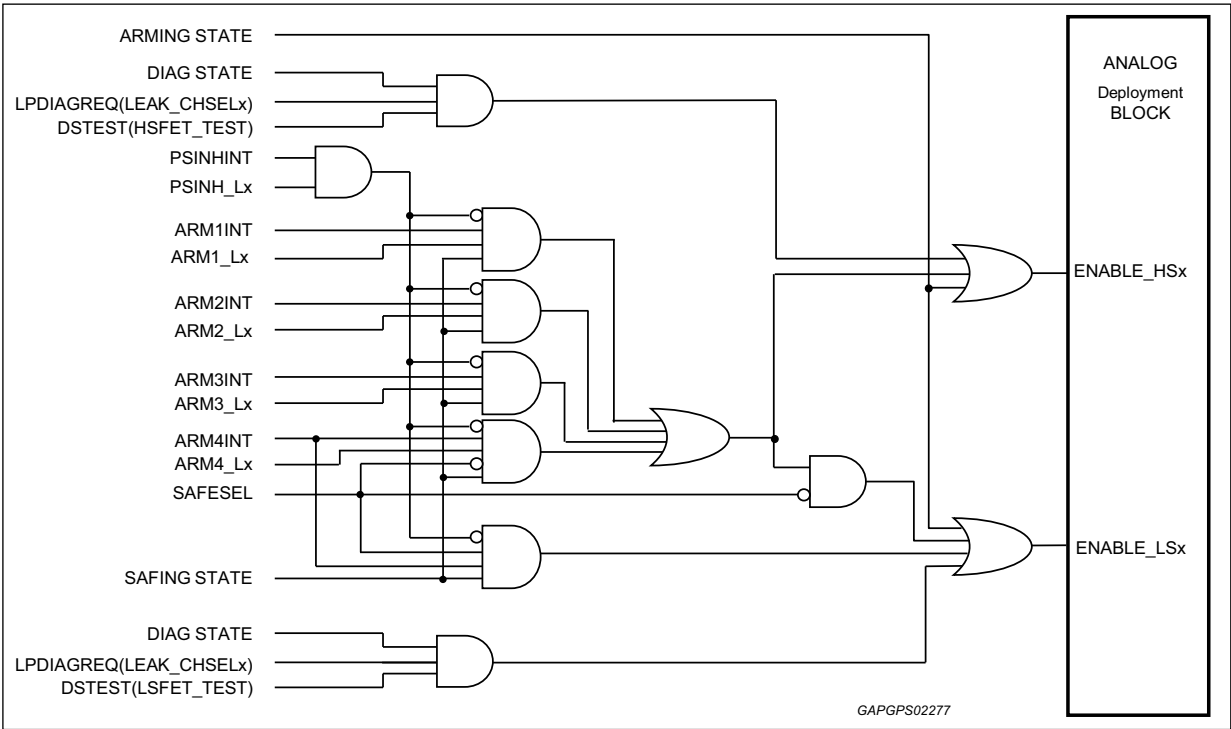
Figure 29. Deployment driver control logic - Turn-on signals
