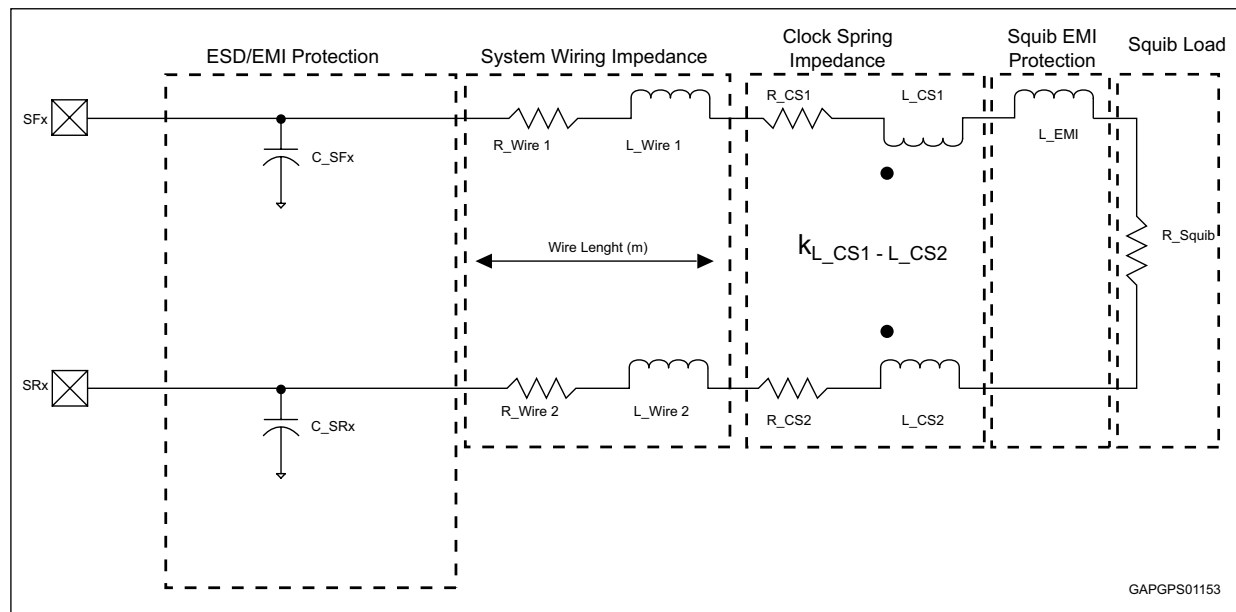
Figure 72. Deployment drivers diagram
