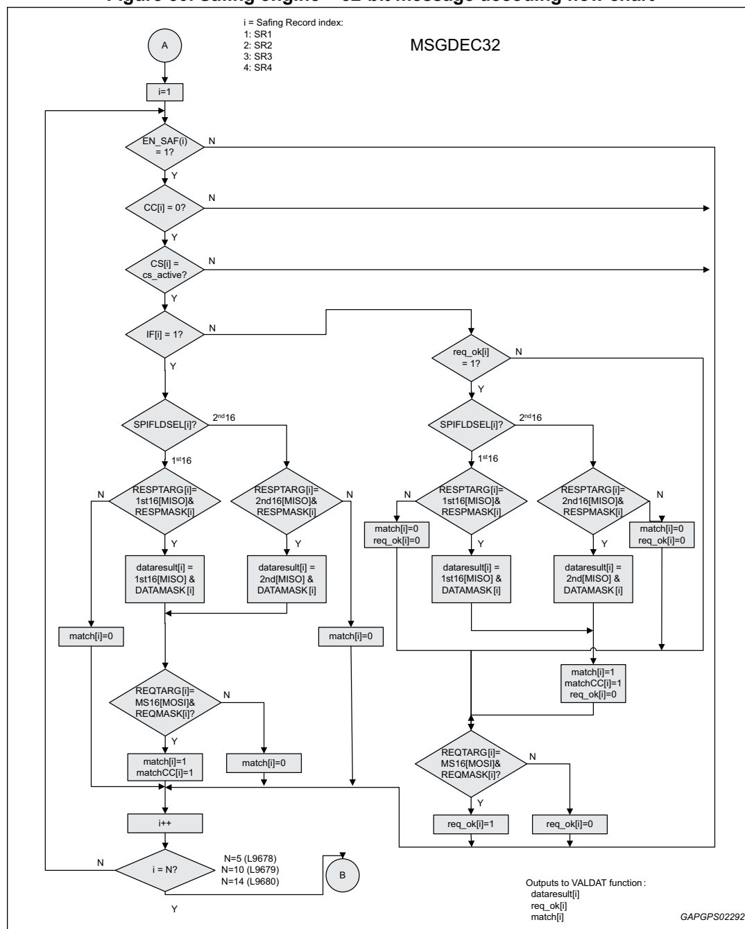
Figure 50. Safing engine – 32-bit message decoding flow chart
