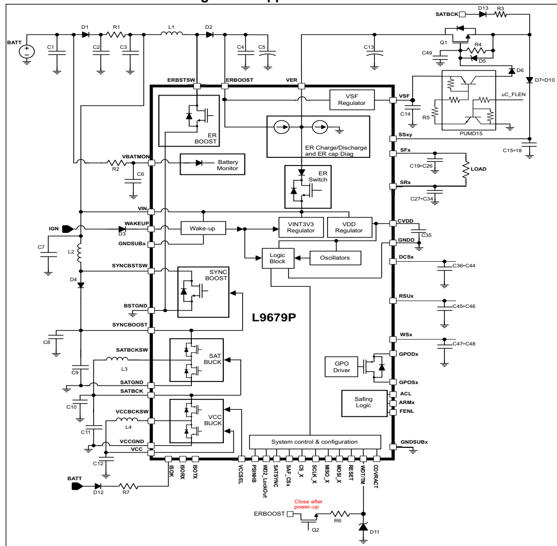
Figure 70. Application circuit
