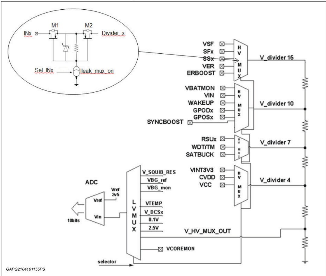
Figure 68. ADC MUX
