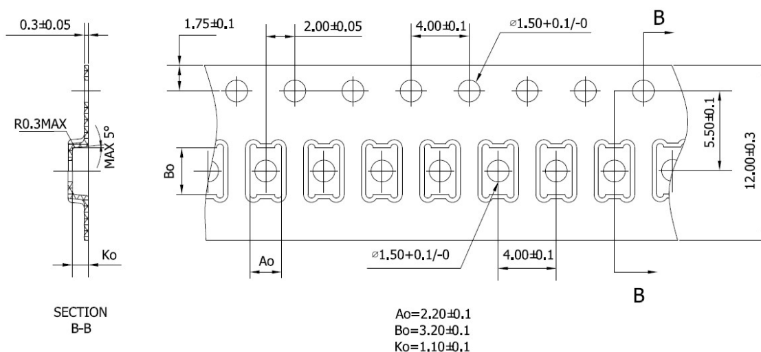
Figure 30. VFDFN8 tape and reel shipment
