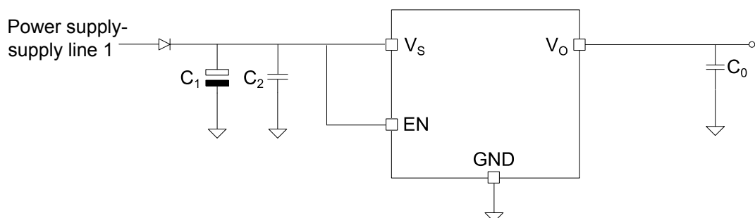
Figure 19. Typical example of enable control
