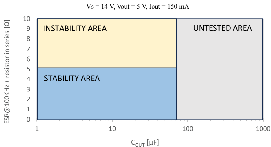
Figure 17. Stability plane
