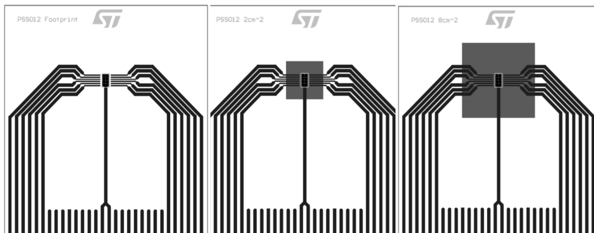
Figure 23. PWSSO12 PCB 2 layers
