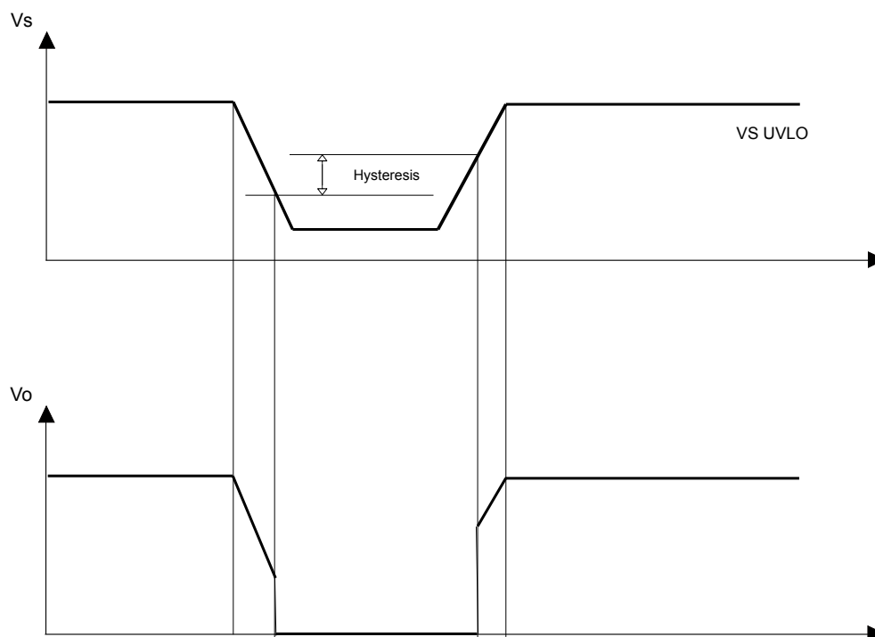
Figure 20. Undervoltage lock out on output voltage
