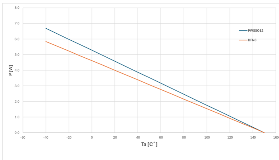
Figure 21. Derating curve
