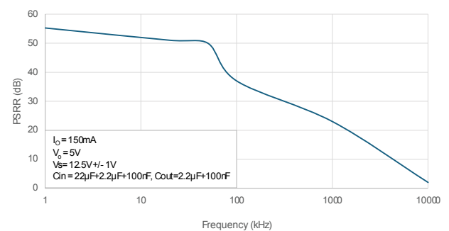
Figure 10. PSRR
