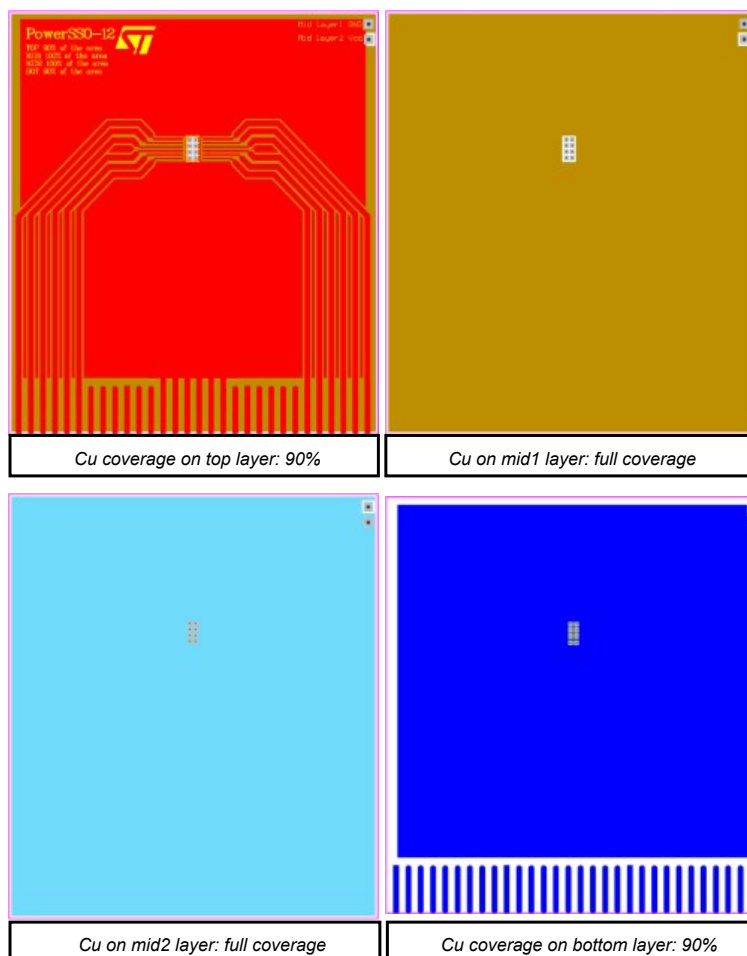
Figure 24. PWSSO12 PCB 4 layers
