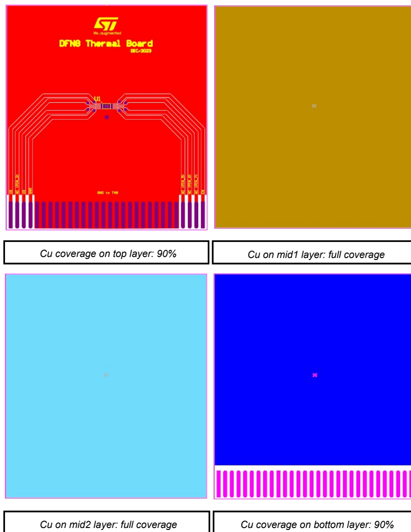
Figure 22. VFDFN8 PC board
