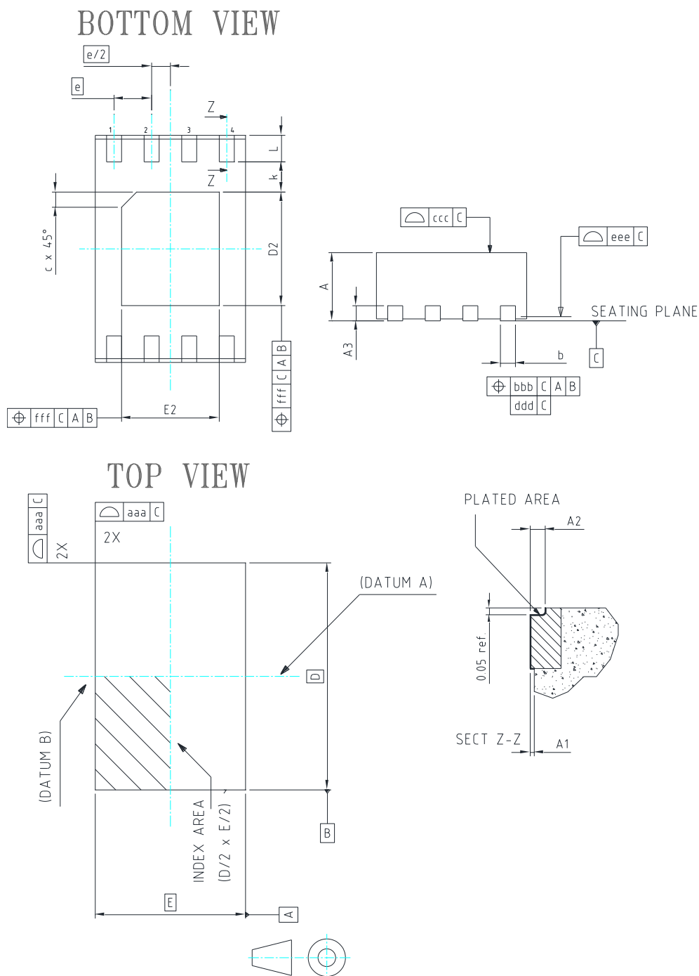
Figure 28. VFDFN8 (3x2x0.9 mm 8L wettable flanks) package outline
