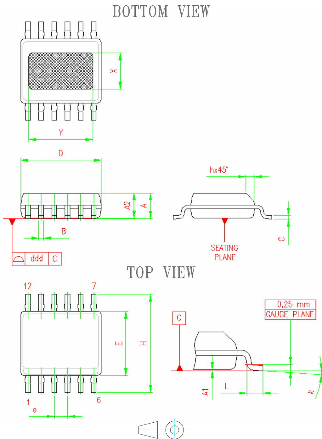
Figure 29. PWSSO12 (4.9x3.9x1.5 mm exposed pad down) package outline
