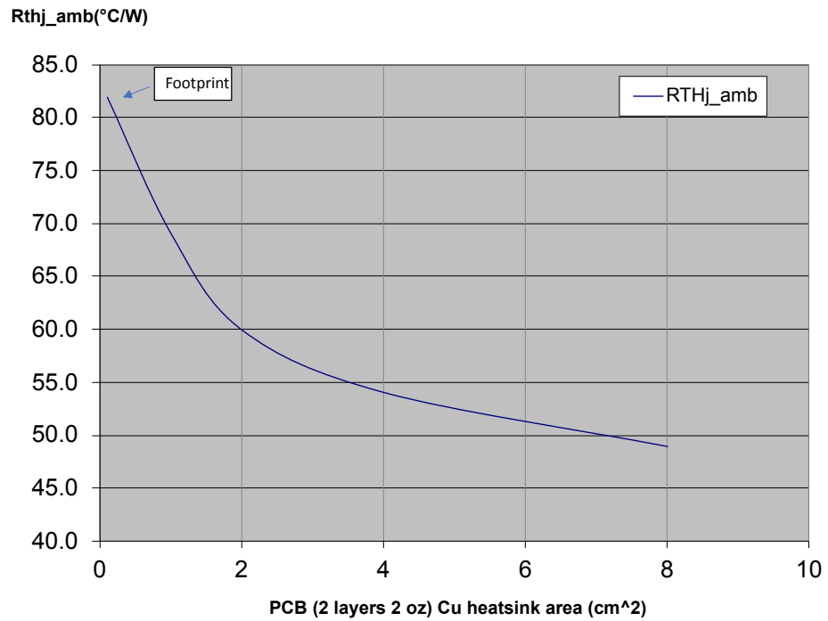
Figure 26. Thermal impedance curves junction to ambient - PWSSO12
