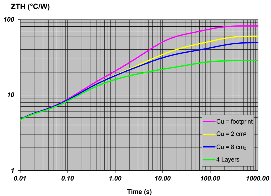
Figure 26. Thermal impedance curves junction to ambient - PWSSO12
