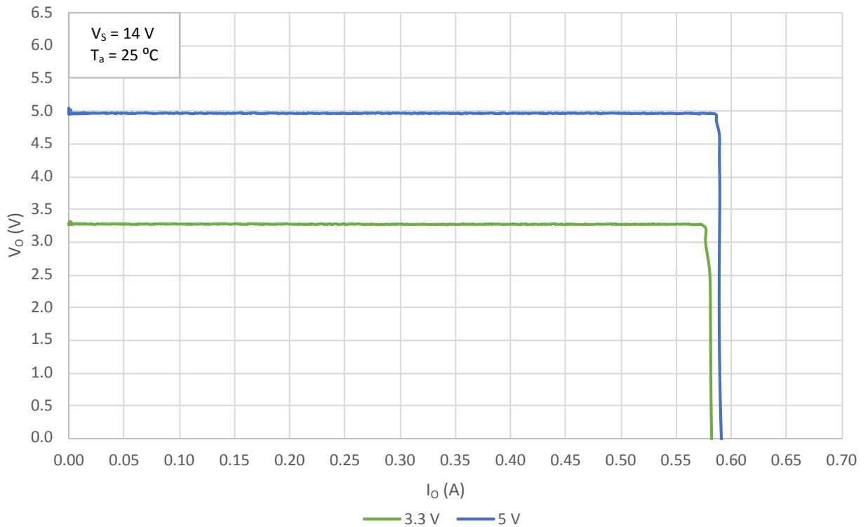
Figure 18. Behavior of output current versus regulated voltage V_O
