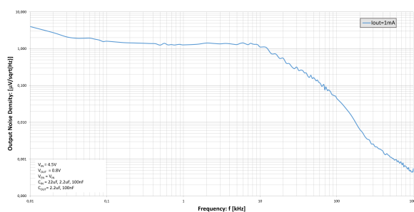
Figure 15. Output noise voltage
