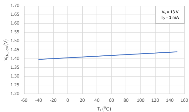
Figure 14. V_{EN\_low} vs T_J
