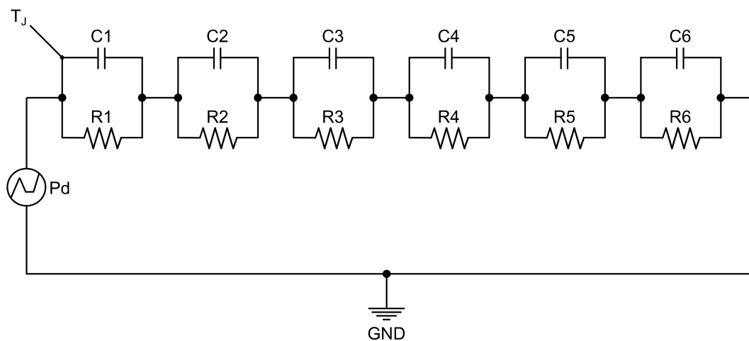
Figure 27. Thermal fitting model of a V_{reg} - PWSSO12
