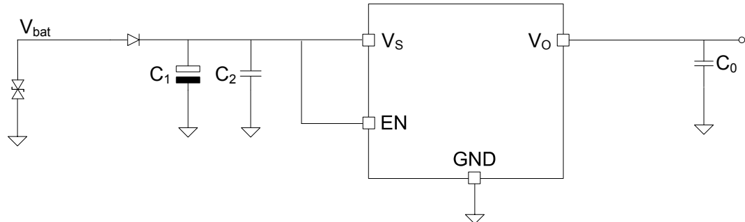
Figure 16. Application schematic
