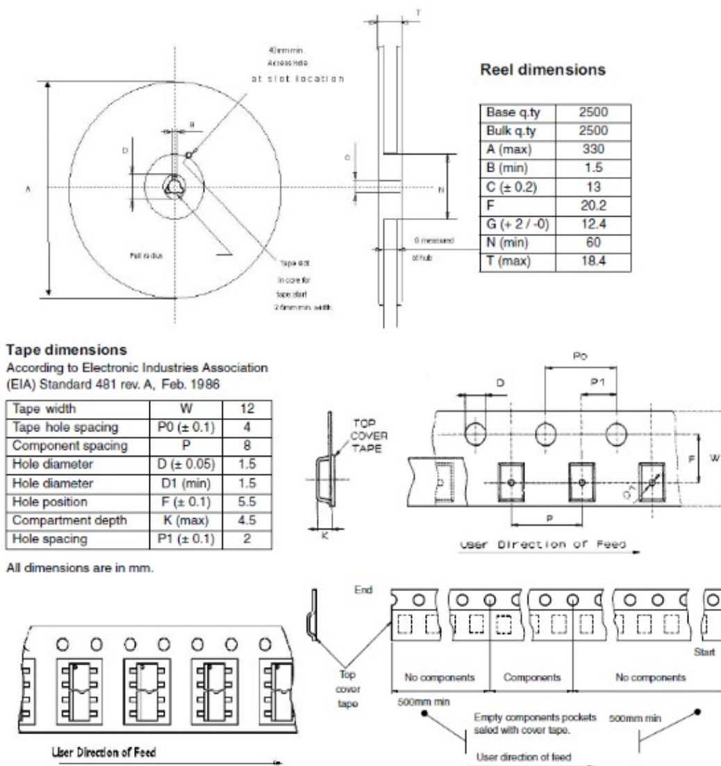
Figure 31. PWSSO12 tape and reel shipment
