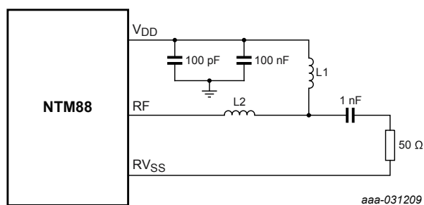
Figure 6. RF output power measurement configuration
