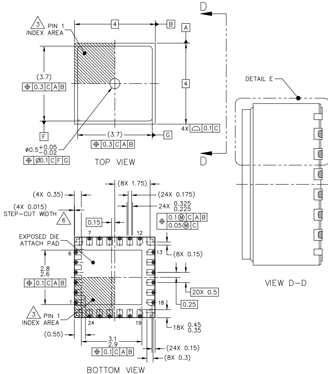
Figure 8. Package outline HQFN24 (SOT1931-1(D))
