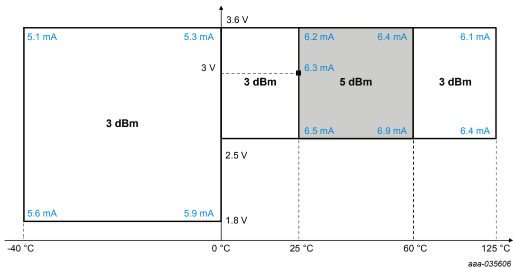
Figure 5. Dynamic power adjustment — 434 MHz
