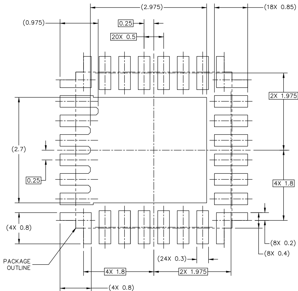
Figure 11. Reflow soldering footprint part2 for HQFN24 (SOT1931-1(D))
