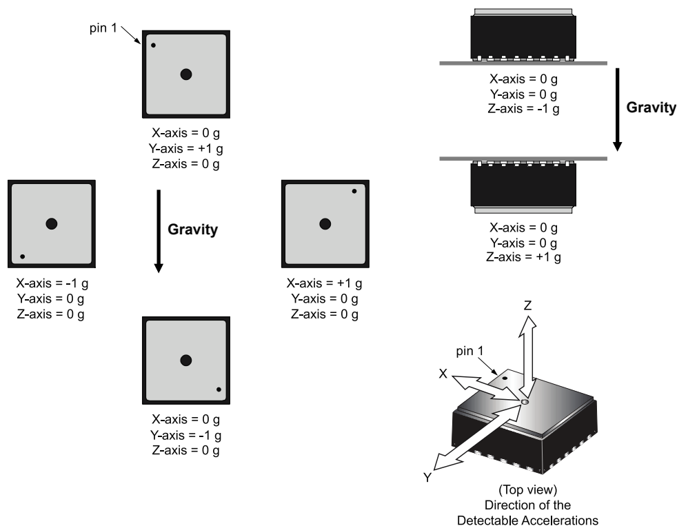
Figure 3. NTM88Jxx5S orientation at rest
