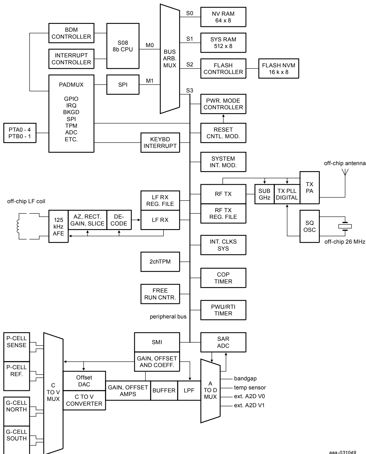
Figure 1. Block diagram
