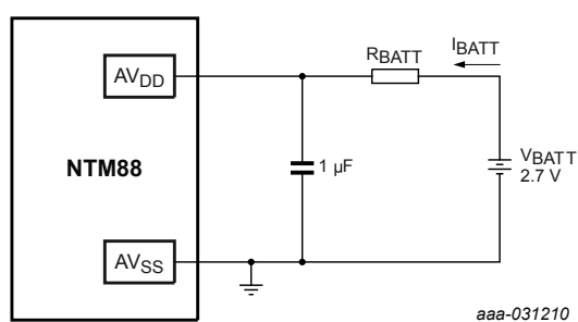
Figure 7. Battery performance test configuration
