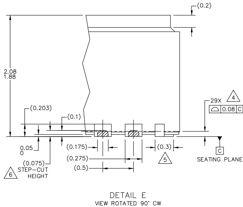
Figure 9. Package outline detail HQFN24 (SOT1931-1(D))
