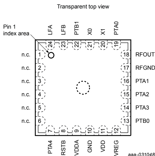
Figure 2. Pin configuration
