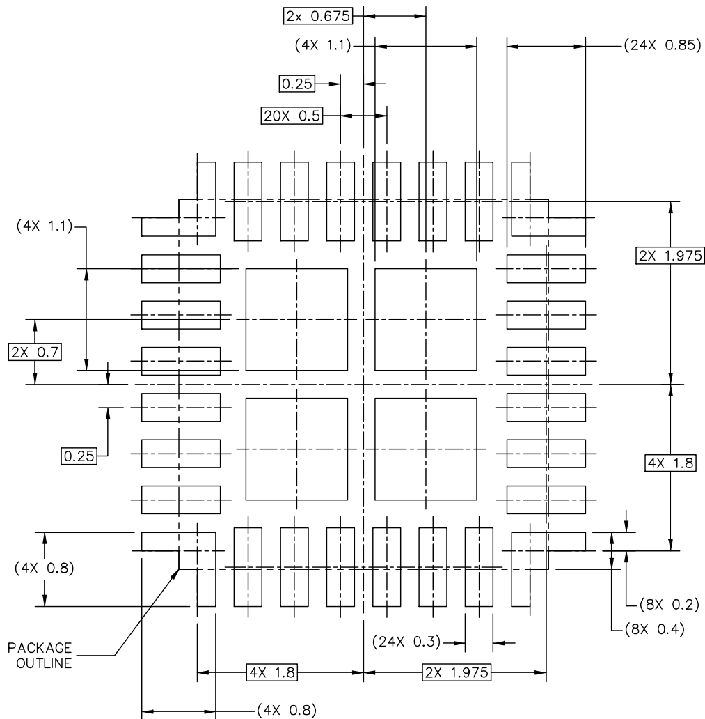
Figure 12. Reflow soldering footprint part3 for HQFN24 (SOT1931-1(D))
