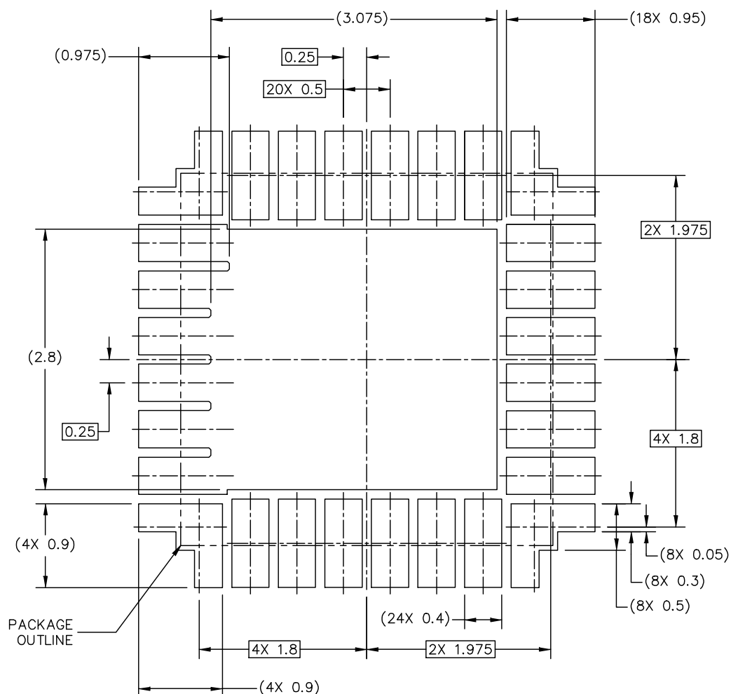
Figure 10. Reflow soldering footprint part1 for HQFN24 (SOT1931-1(D))
