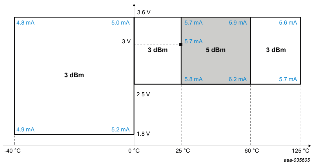
Figure 4. Dynamic power adjustment — 315 MHz
