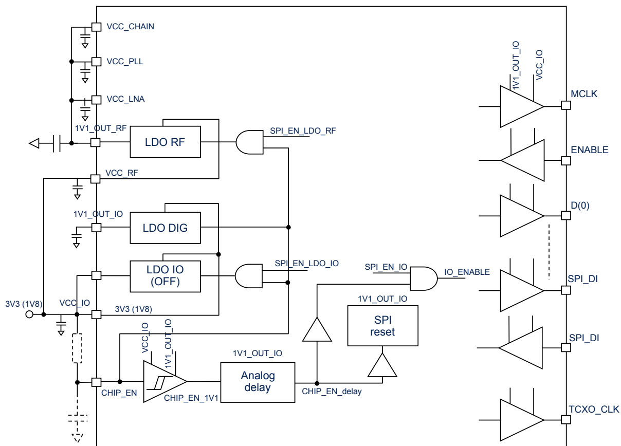
Figure 3. Power configuration
