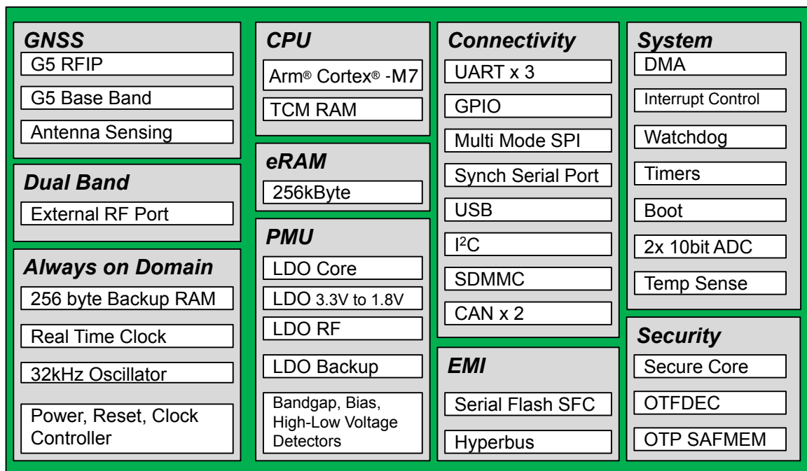
Figure 1. STA8135G block diagram
