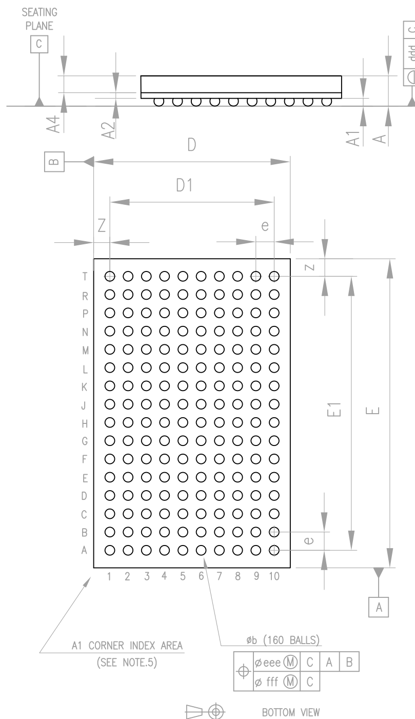
Figure 9. TFBGA160 (7x11x1.2 mm) package outline
