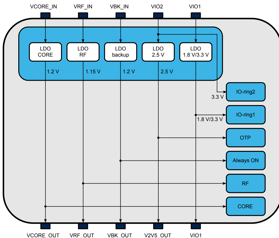
Figure 2. LDO on-chip regulators dependencies
