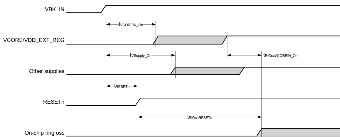
Figure 6. Power-up timing diagram
