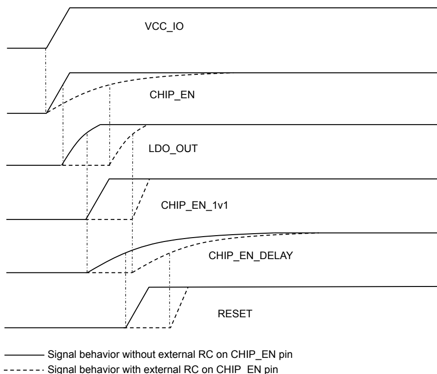
Figure 4. Power-up strategy
