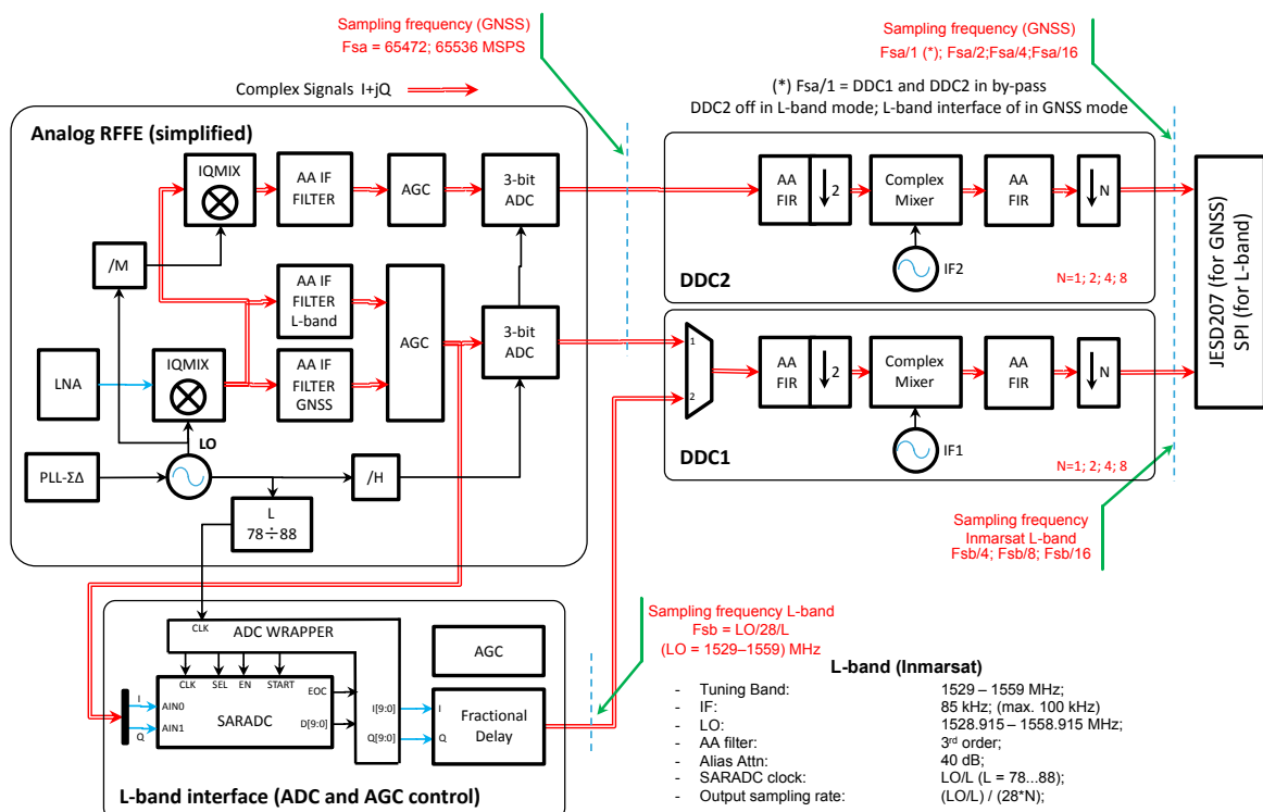
Figure 2. RF chip DDC block diagram
