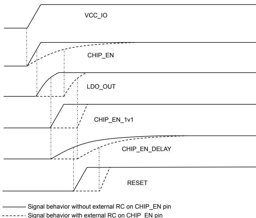
Figure 5. Power-up strategy
