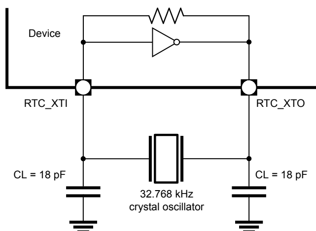
Figure 6. 32.768 kHz crystal oscillator connection
