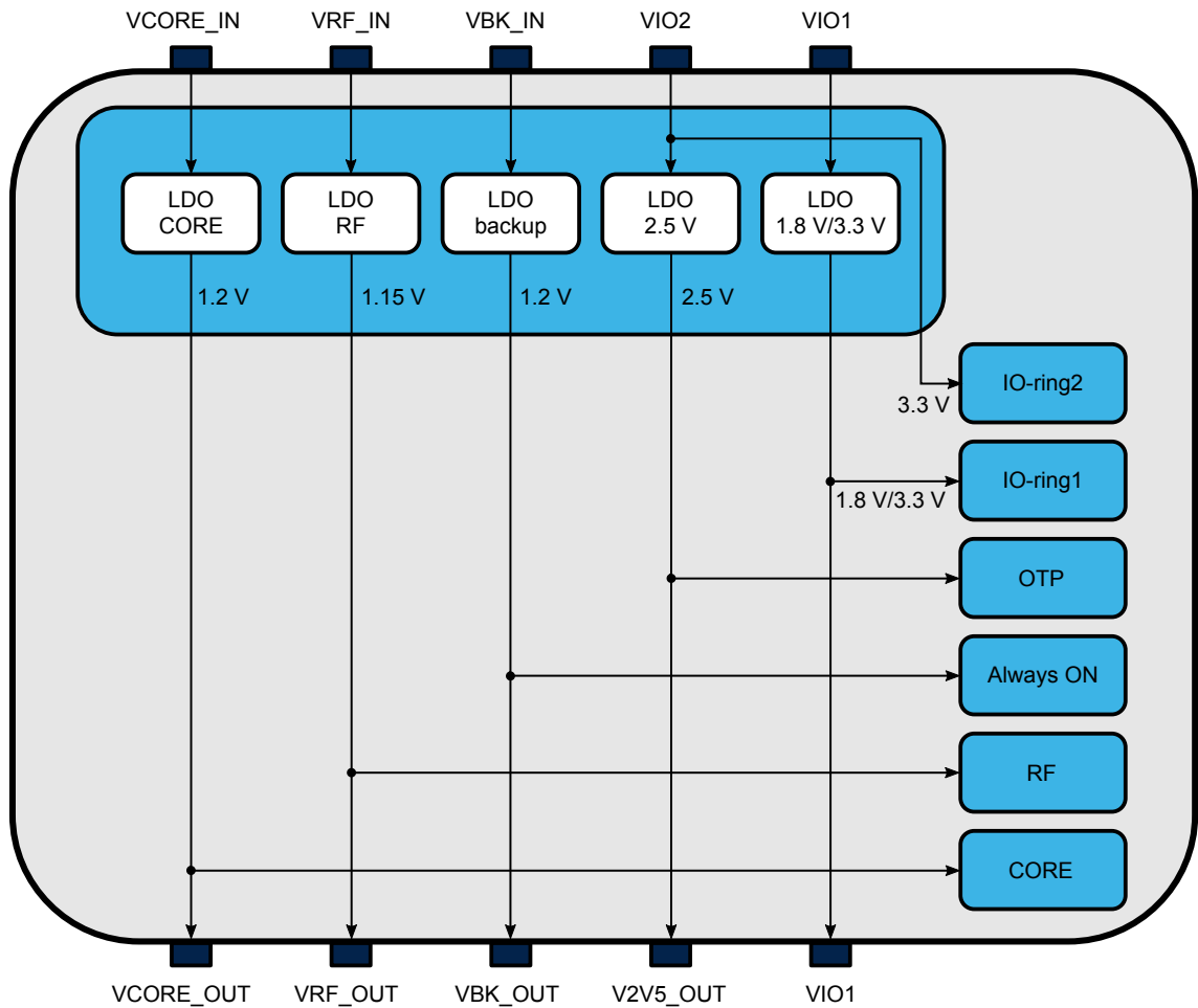
Figure 3. LDO on-chip regulators dependencies
