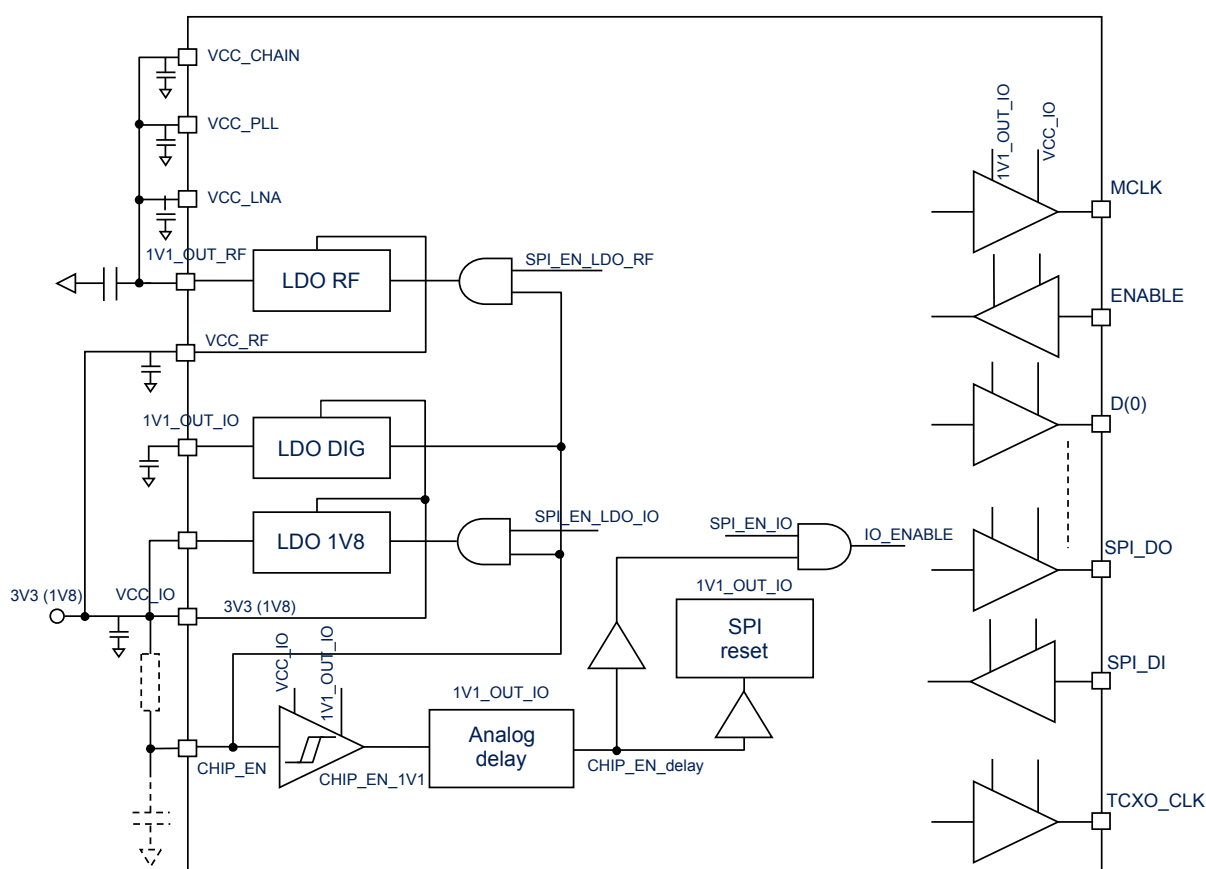
Figure 4. Power configuration
