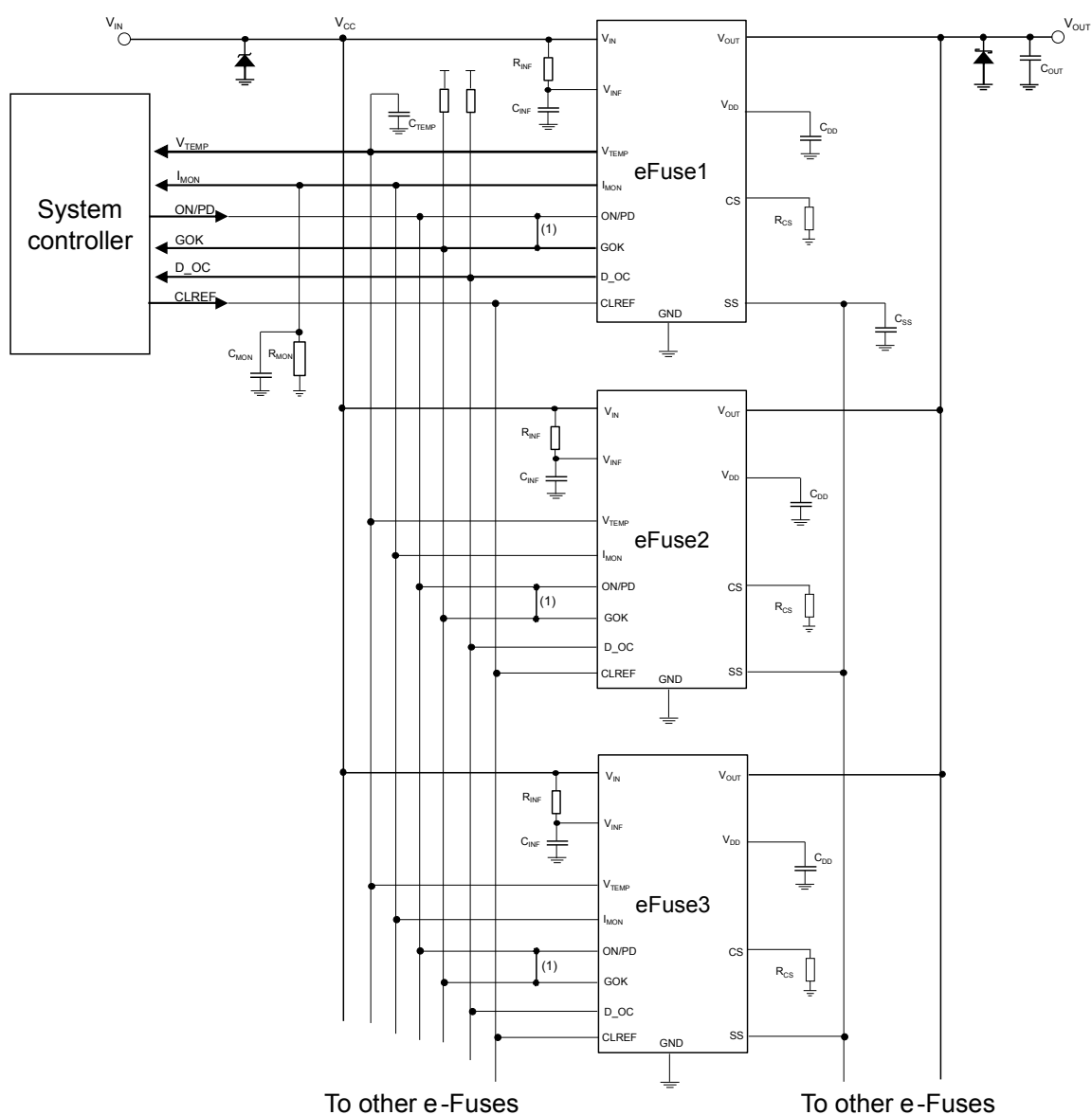
Figure 5. Typical application diagram (multiple e-Fuses in parallel)
