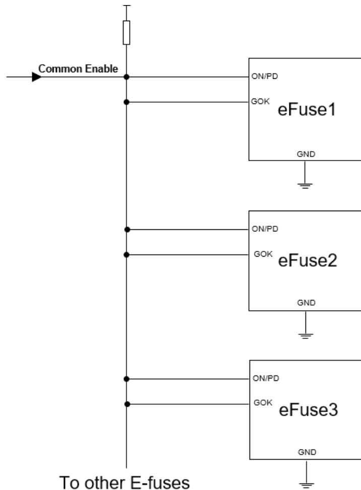
Figure 7. Additional connections for multiple STEF12H60GAPUR (autoretry version)
