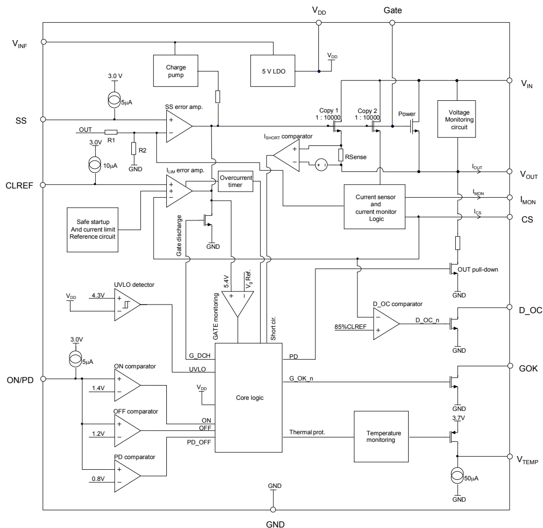
Figure 1. Block diagram
