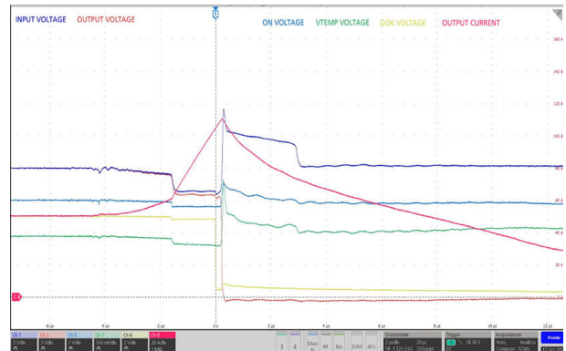
Figure 35. Device reset after fault
