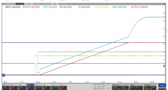
Figure 35. Device reset after fault
