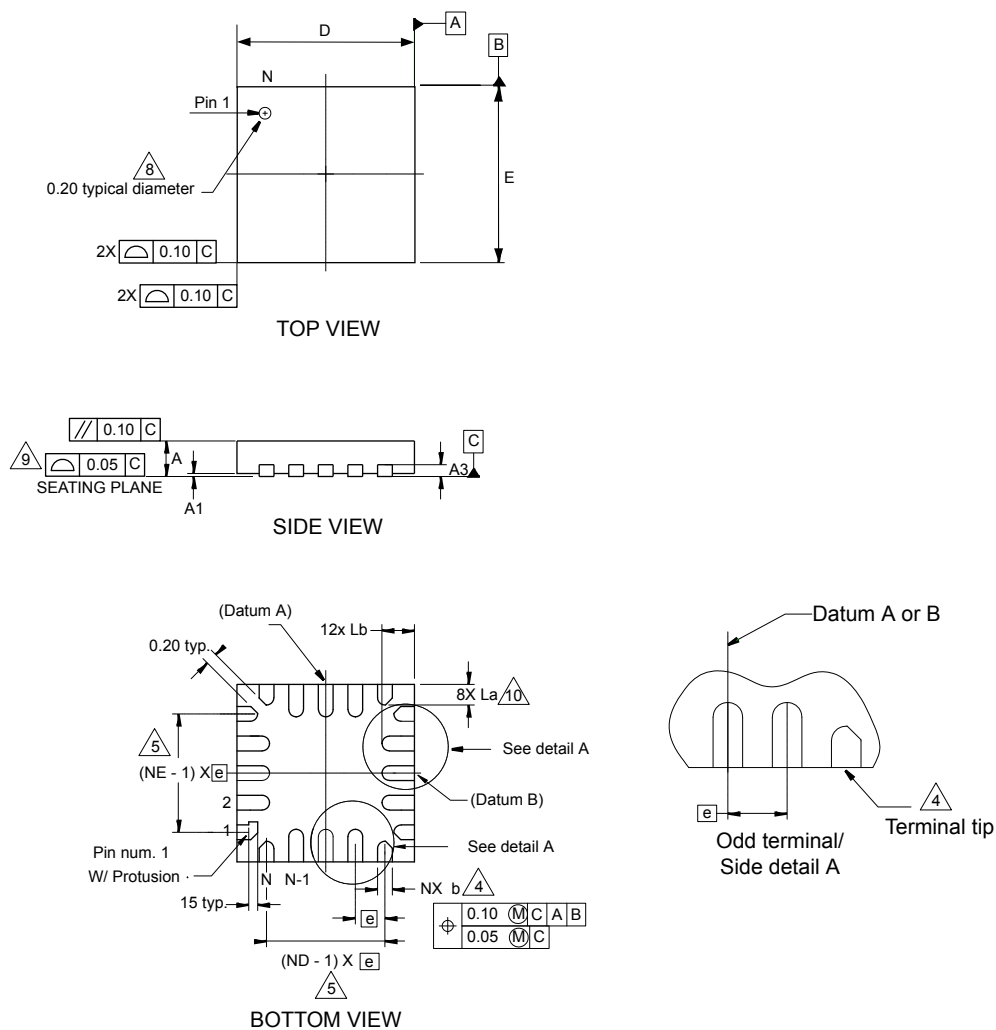
Figure 39. UFQFPN20 - Outline
