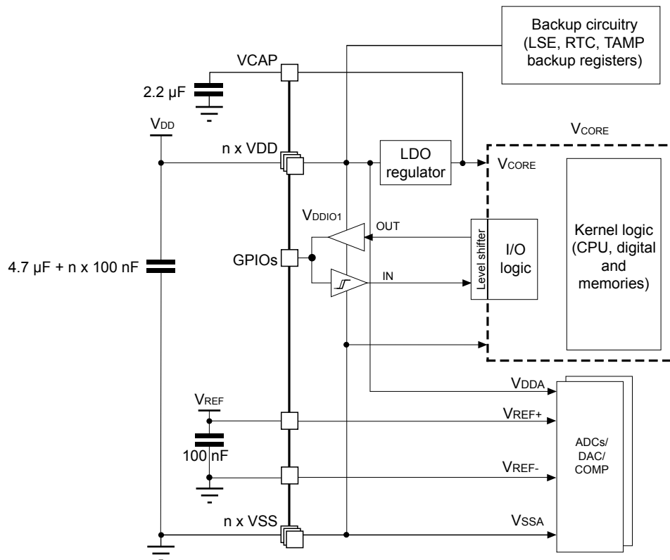
Figure 13. STM32C53xxx power supply scheme
