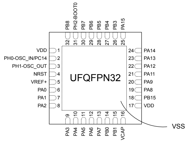
Figure 7. UFQFPN32 pinout
