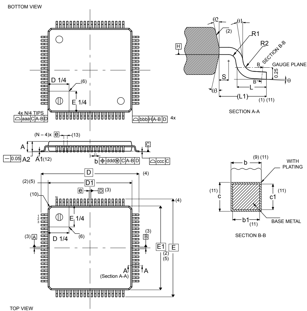
Figure 46. LQFP80 - Outline (15.)
