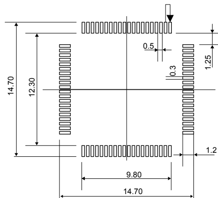
Figure 47. LQFP80 - Footprint example
