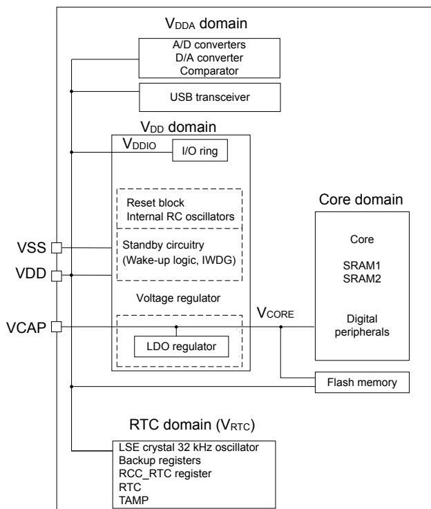
Figure 2. STM32C55xxx power supply overview
