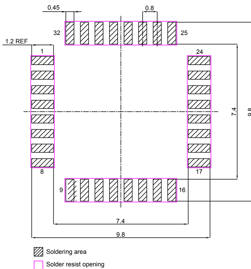
Figure 38. LQFP32 - Footprint example
