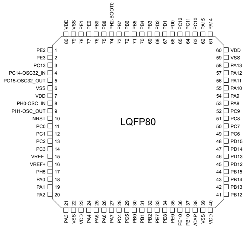
Figure 9. LQFP80 pinout
