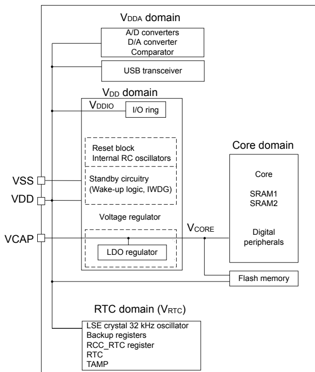
Figure 2. STM32C5A3xxx power supply overview
