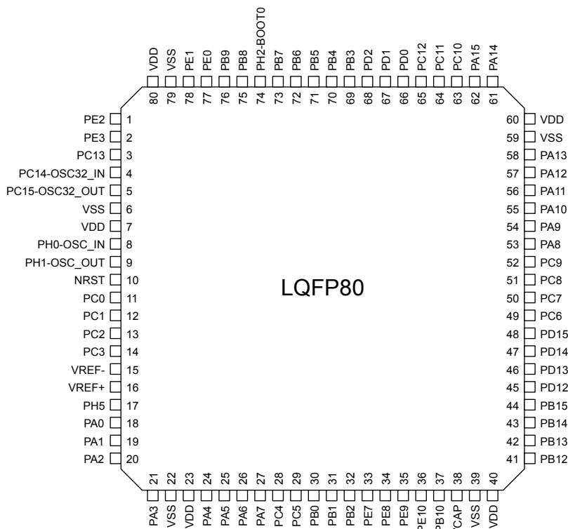
Figure 8. LQFP80 pinout
