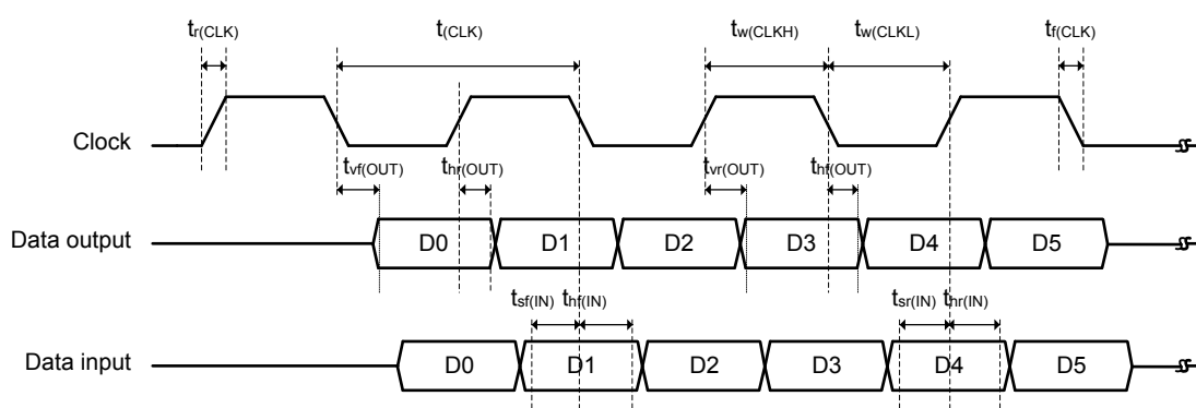
Figure 25. OCTOSPI Hyperbus clock
