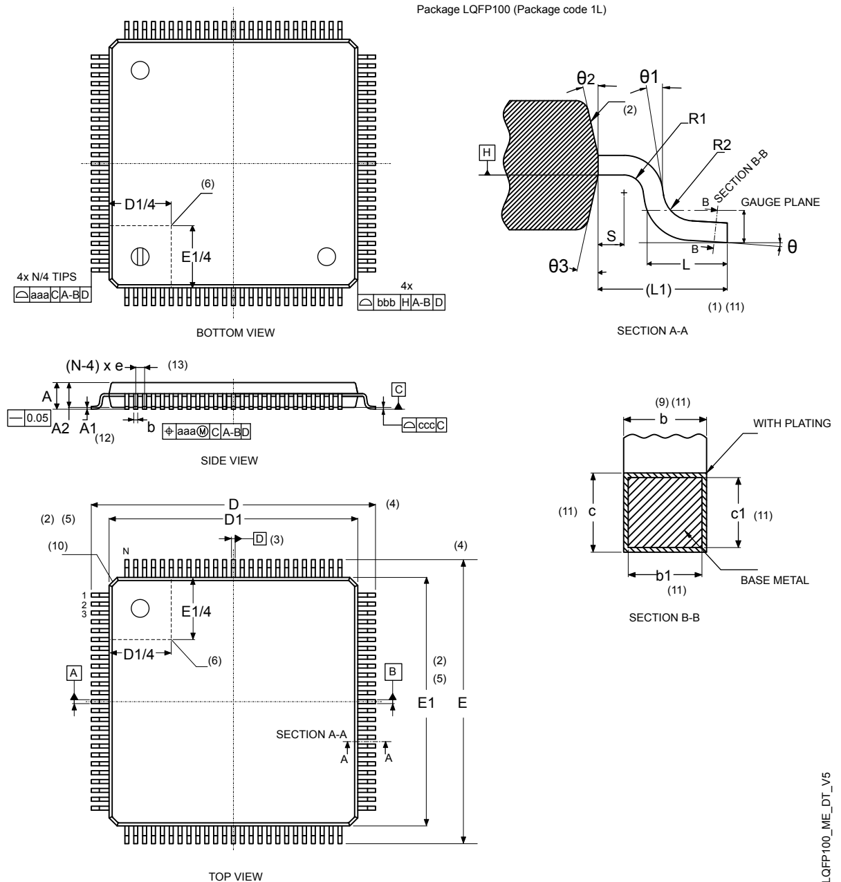
Figure 56. LQFP100 - Outline (15.)
