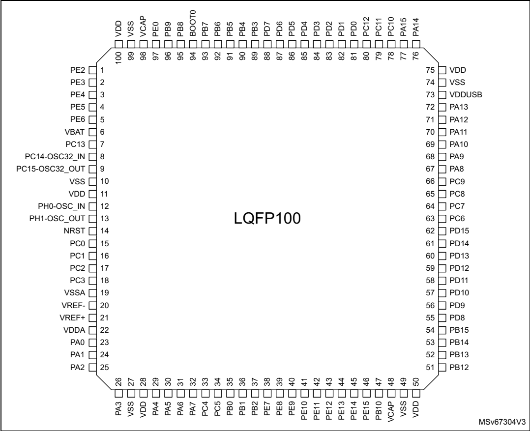
Figure 9. LQFP100 pinout
