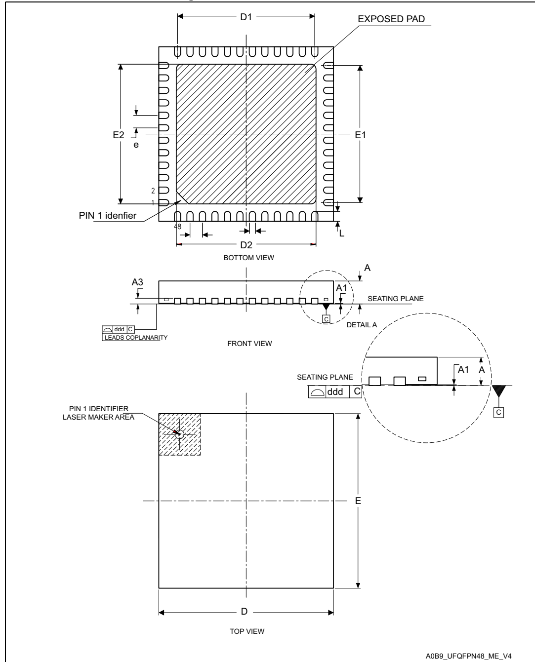
Figure 69. UFQFPN48 - Outline
