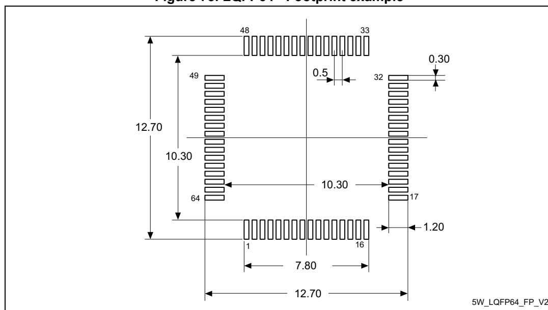
Figure 73. LQFP64 - Footprint example
