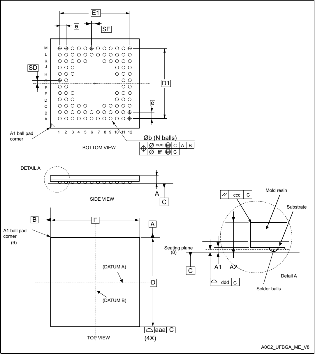
Figure 78. UFBGA100 - Outline (13)
