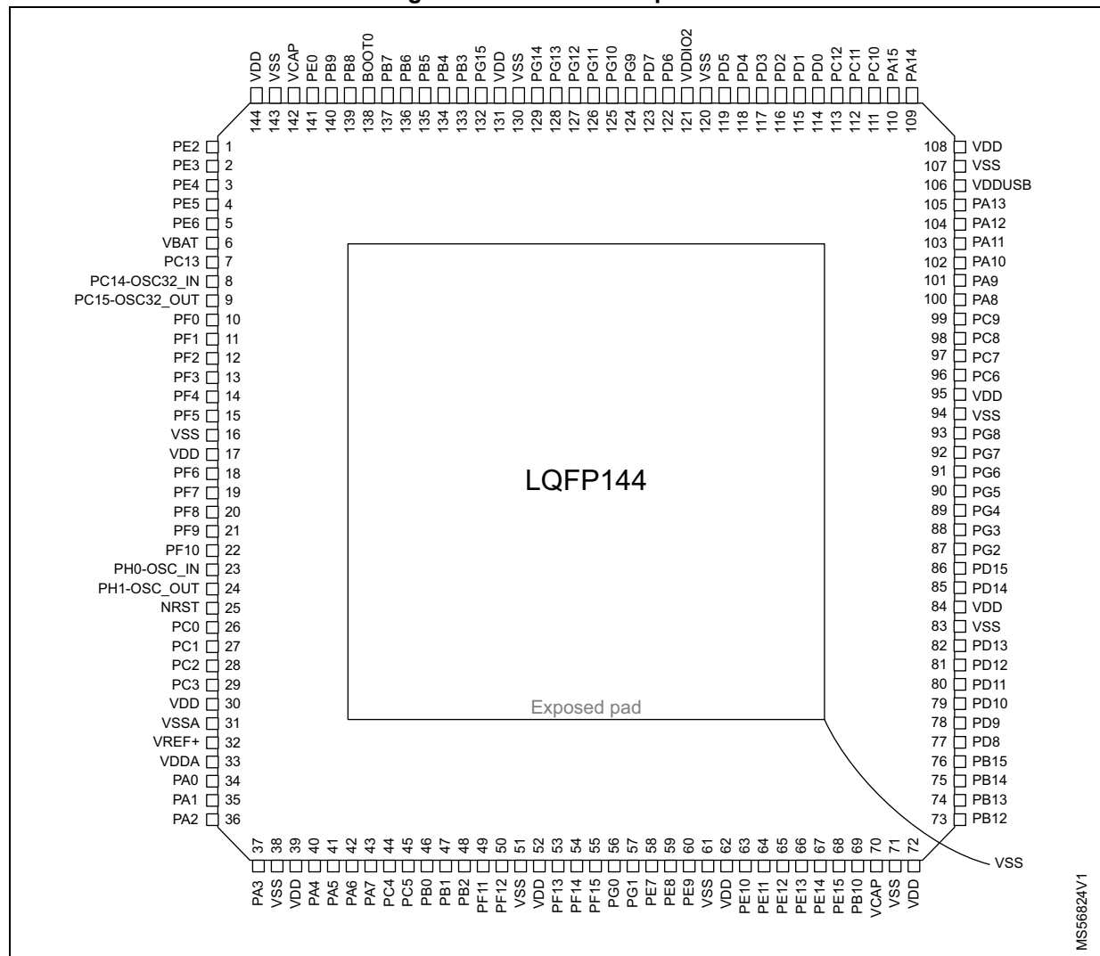
Figure 13. LQFP144-EP pinout
