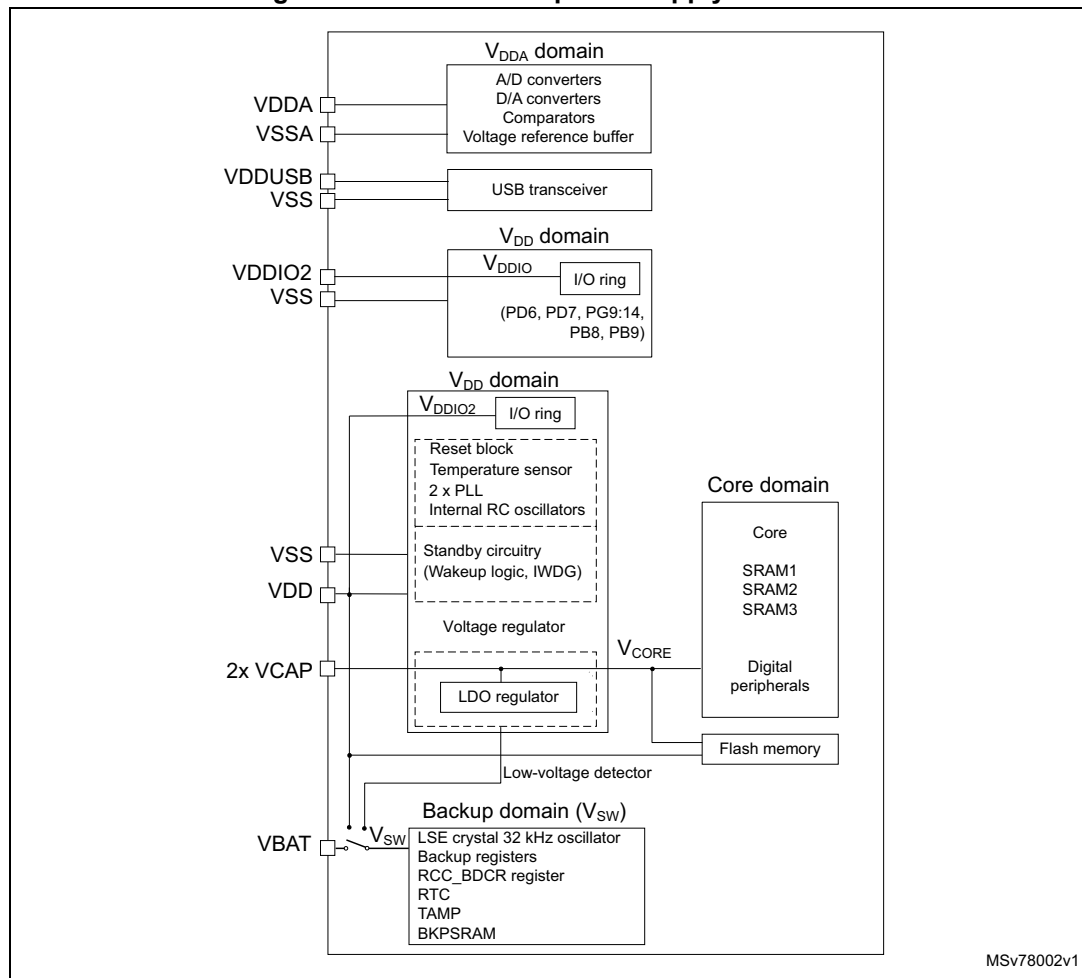
Figure 2. STM32H543xx power supply overview
