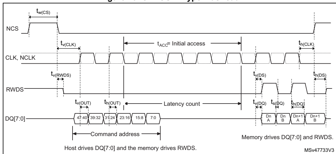
Figure 43. OCTOSPI HyperBus read
