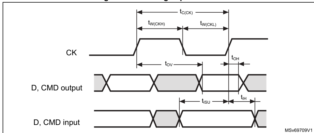
Figure 42. SDIO high-speed mode
