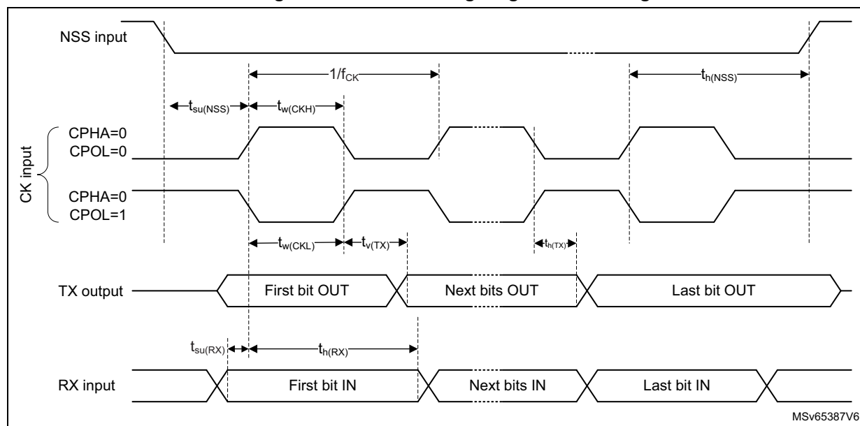
Figure 66. USART timing diagram in SPI target mode
