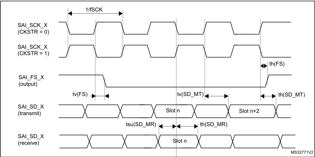
Figure 60. SAI controller timing waveforms
