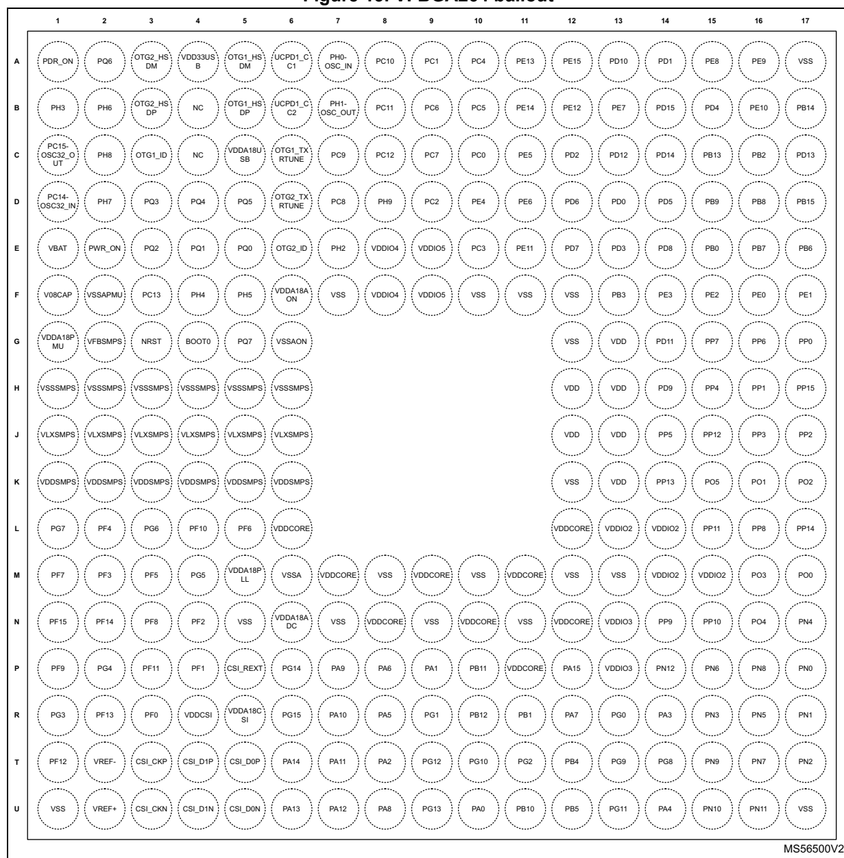
Figure 13. VFBGA264 ballout
