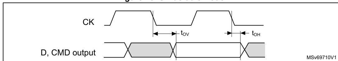
Figure 43. SD default mode
