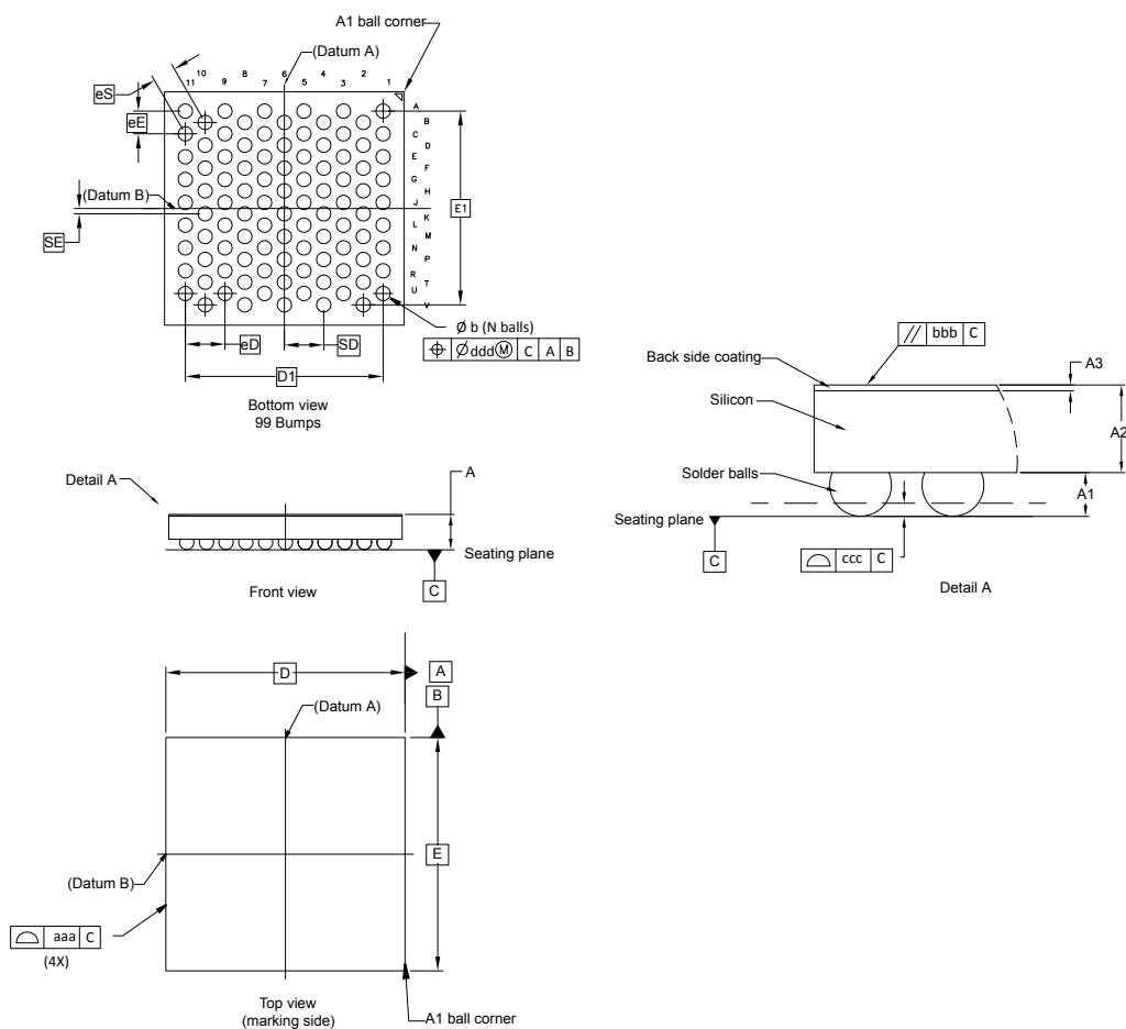
Figure 73. WLCSP99 - Outline
