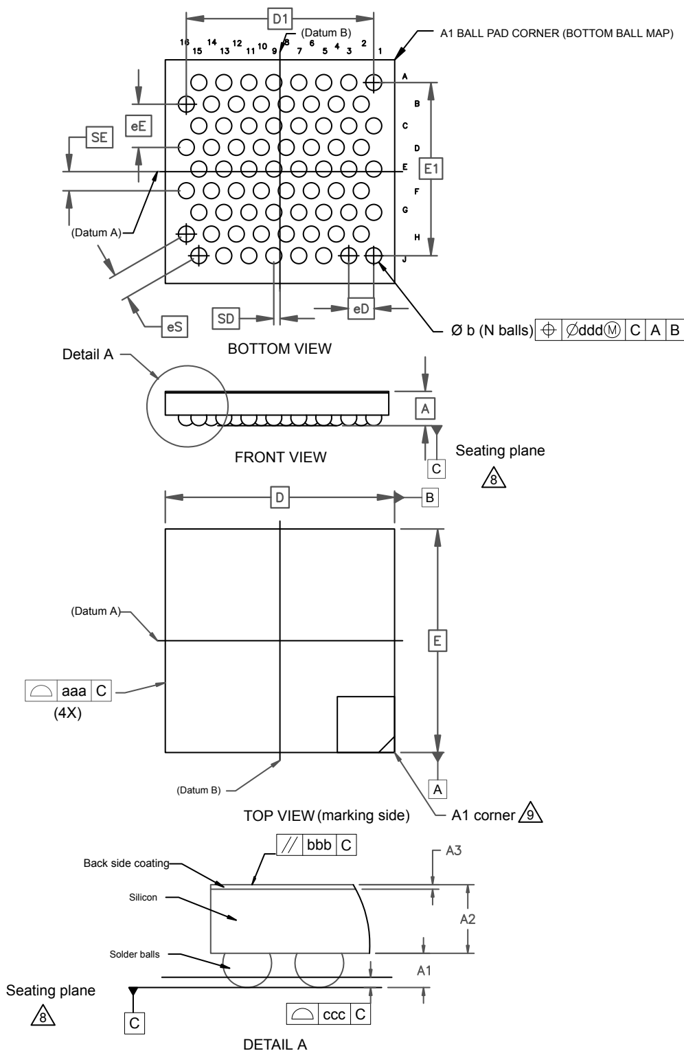
Figure 71. WLCSP72 - Outline
