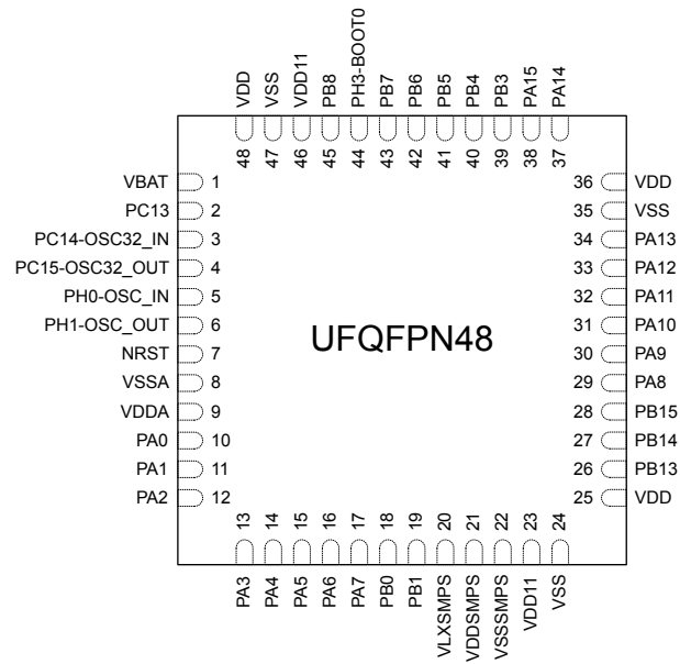
Figure 9. UFQFPN48 pinout
