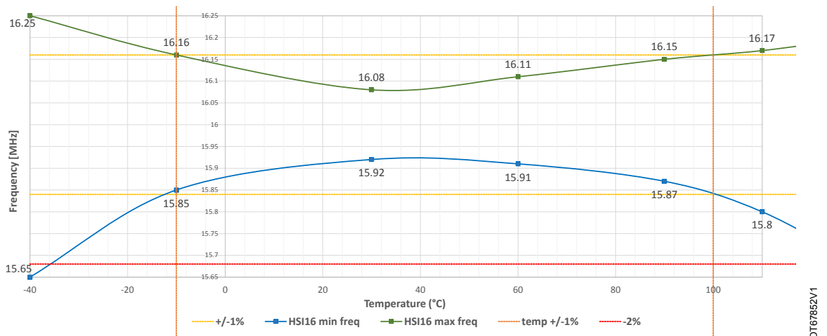
Figure 33. HSI16 frequency versus temperature and V_{\text{DD}}
