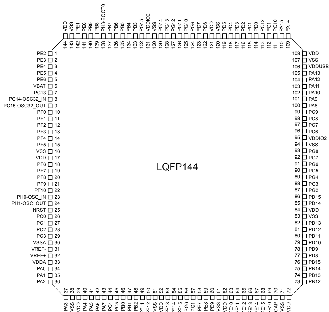
Figure 20. LQFP144 pinout
