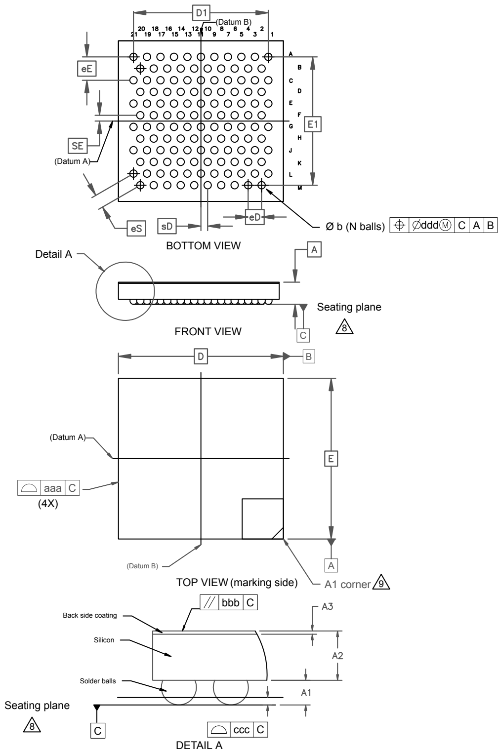
Figure 77. WLCSP126 - Outline
