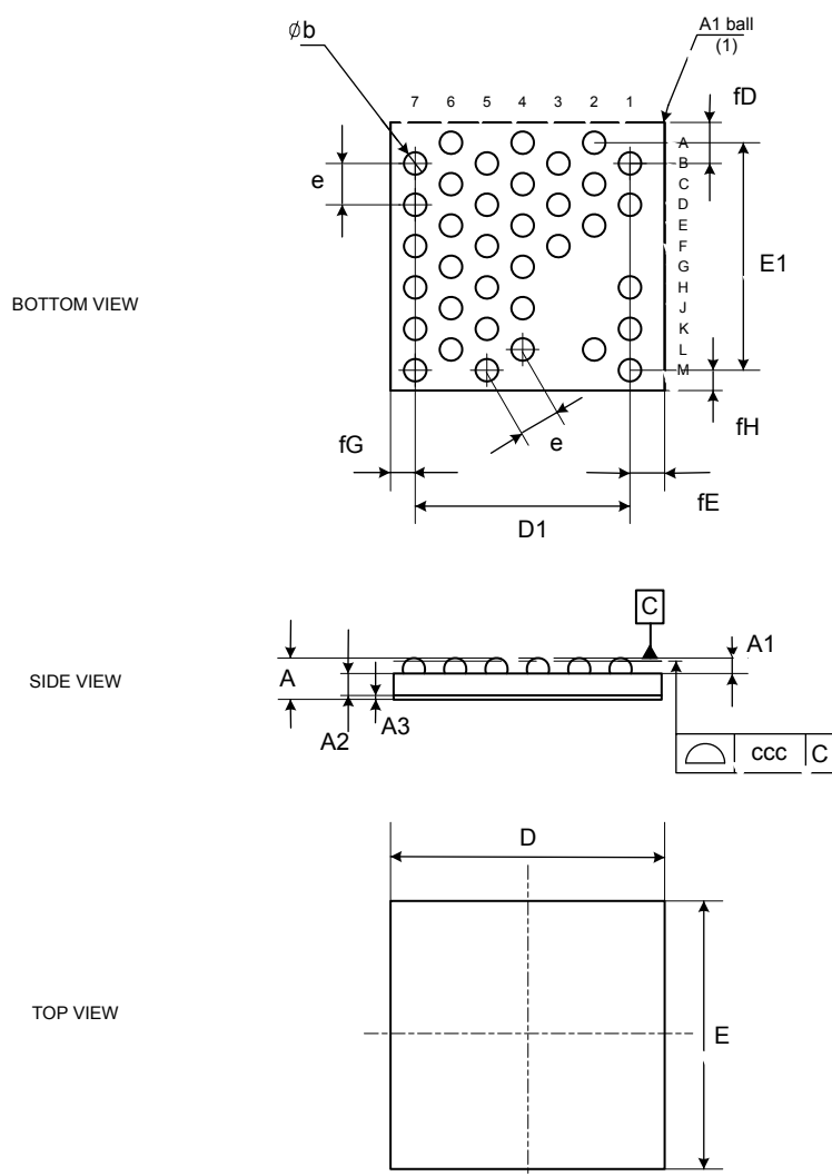
Figure 15. WLCSP36 - Outline
