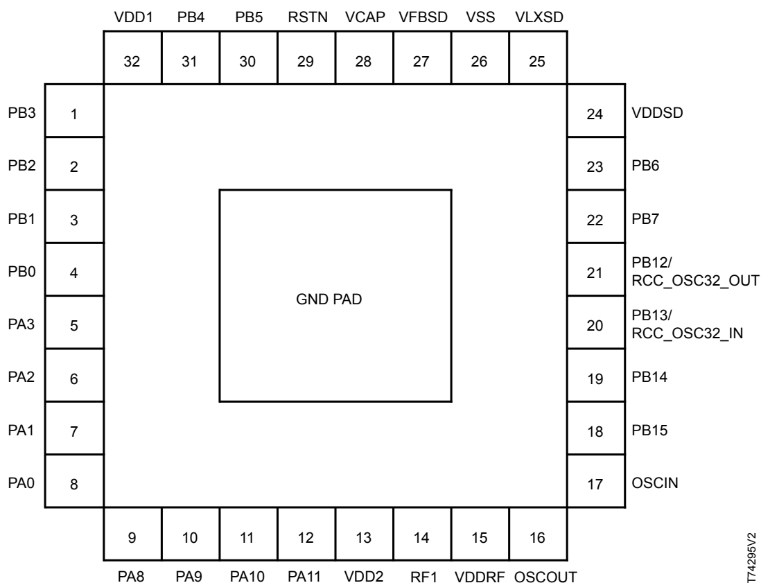
Figure 3. Pinout top view (VFQFPN32 package)
