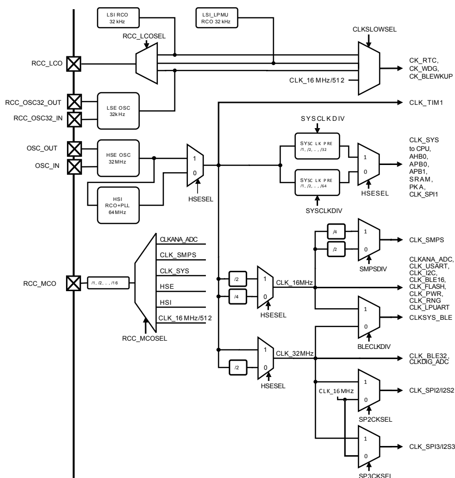
Figure 6. Clock tree
