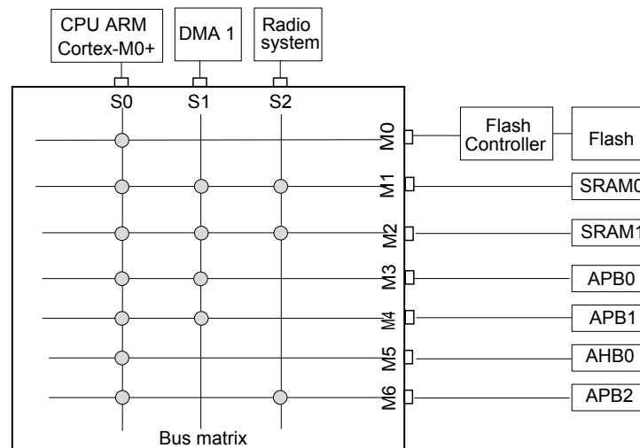
Figure 5. Bus matrix
