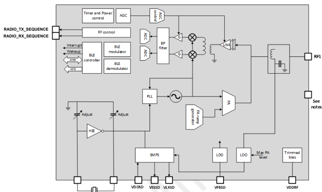
Figure 3. STM3WB09xE RF block diagram
