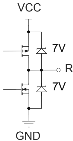
Figure 22. R output
