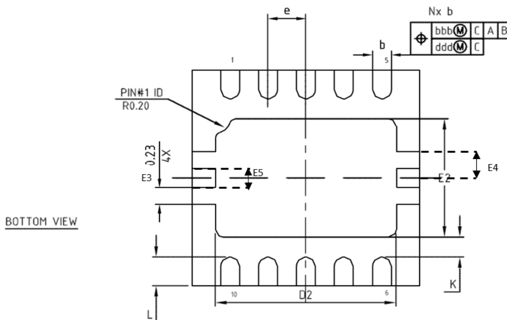
Figure 26. DFN10 package outline (bottom view)
