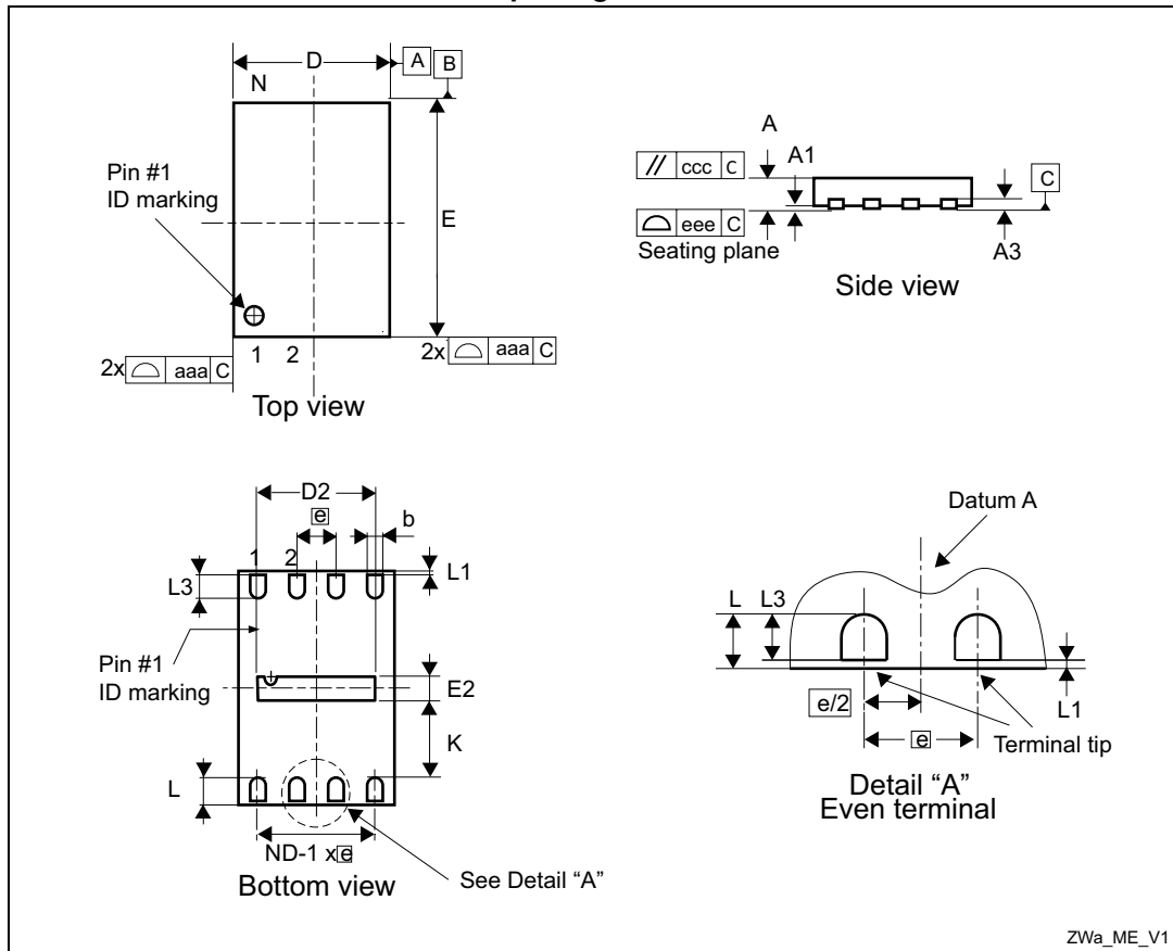
Figure 21. UDFFPN8 - 8-lead, 2 × 3 mm, 0.5 mm pitch ultra thin profile fine pitch dual flat package outline
