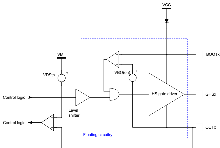
Figure 21. V_{BO} UVLO circuitry and high-side VDS monitoring
