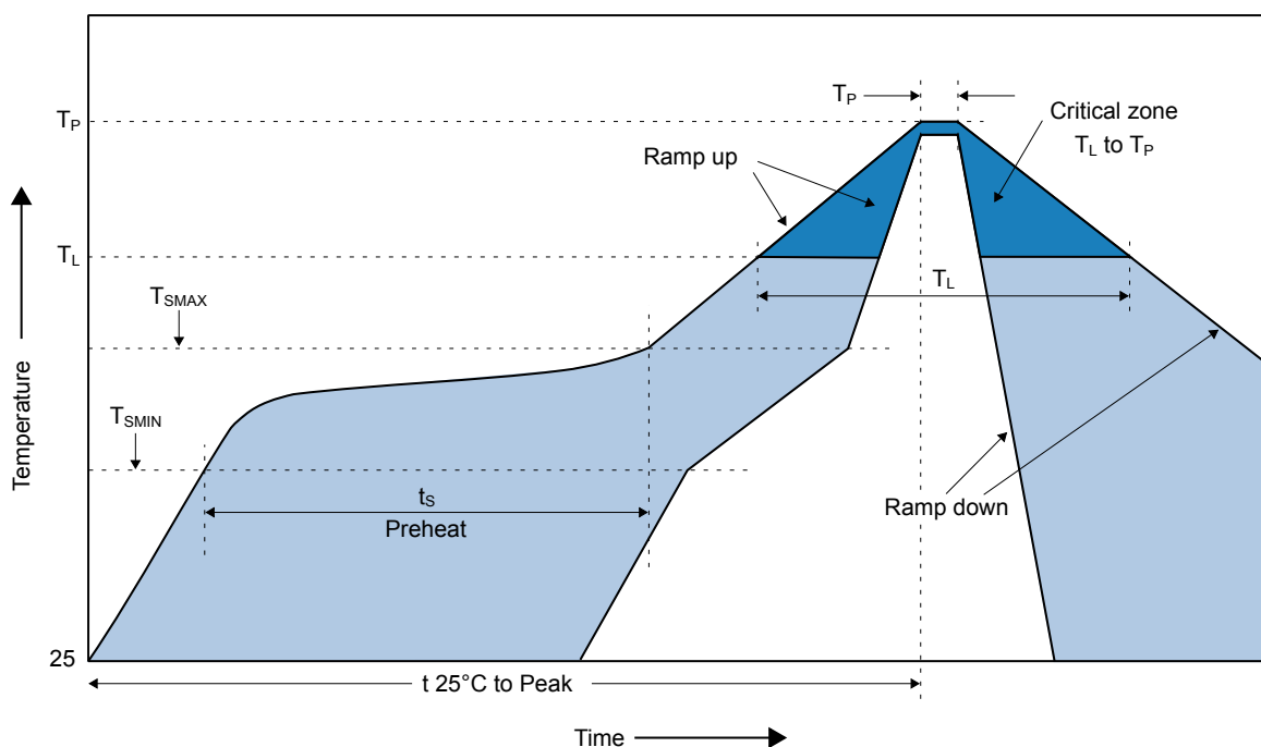
Figure 10. Soldering profile
