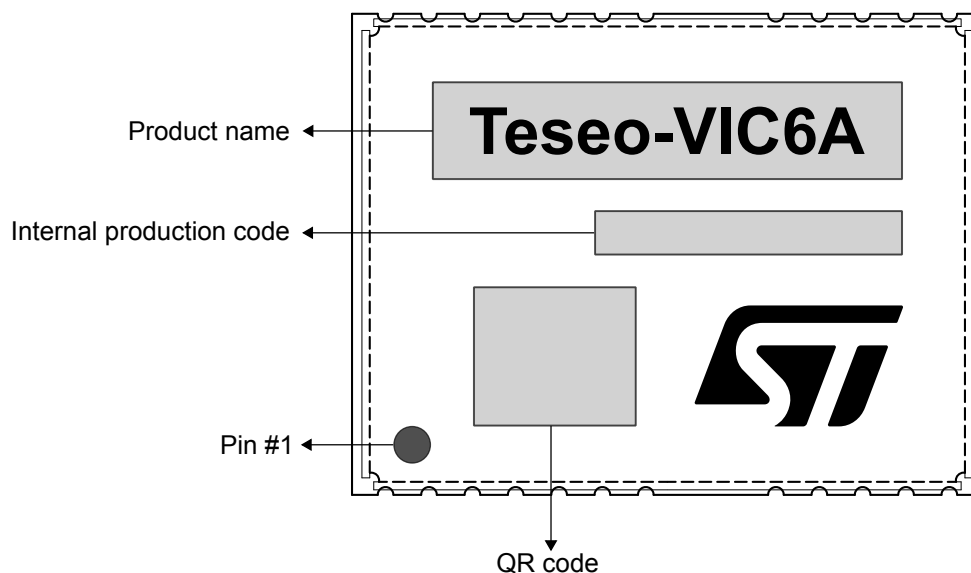
Figure 9. Labeling information
