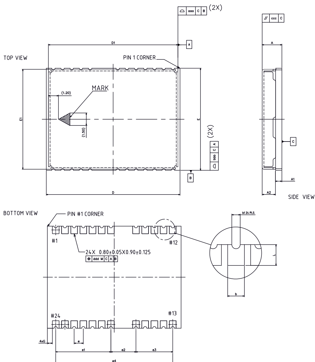
Figure 5. LCC 24 pins package outline
