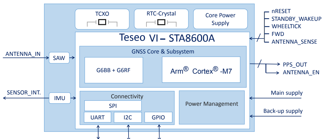
Figure 1. Block schematic
