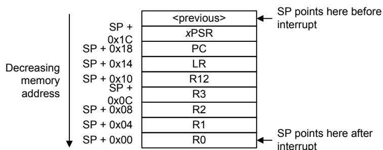
Figure 9. Stack frame
