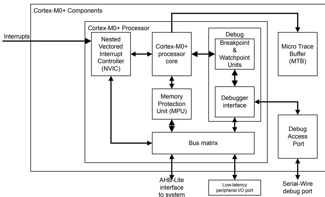
Figure 1. Cortex®-M0+ implementation
