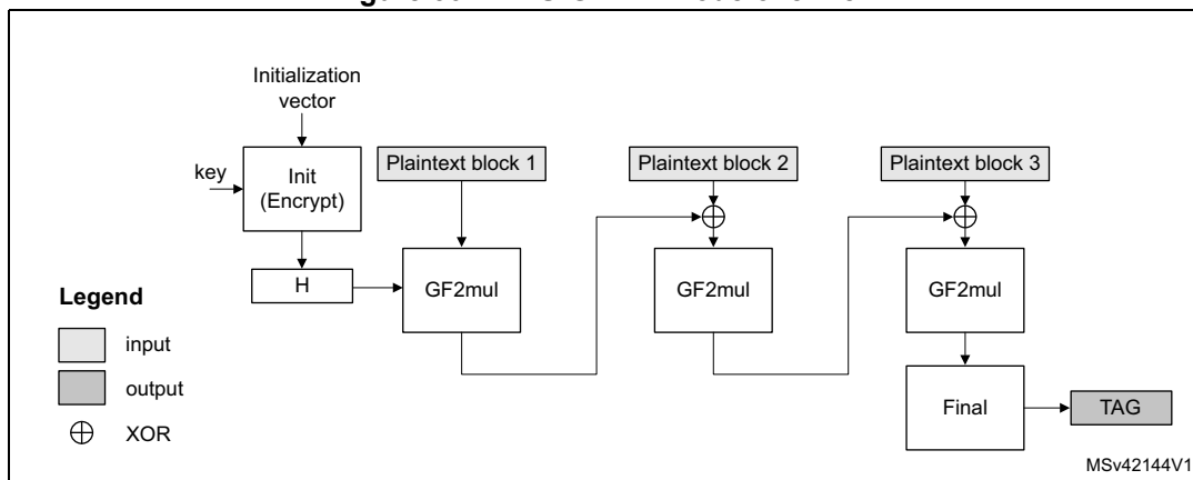
Figure 301. AES-GMAC mode overview
