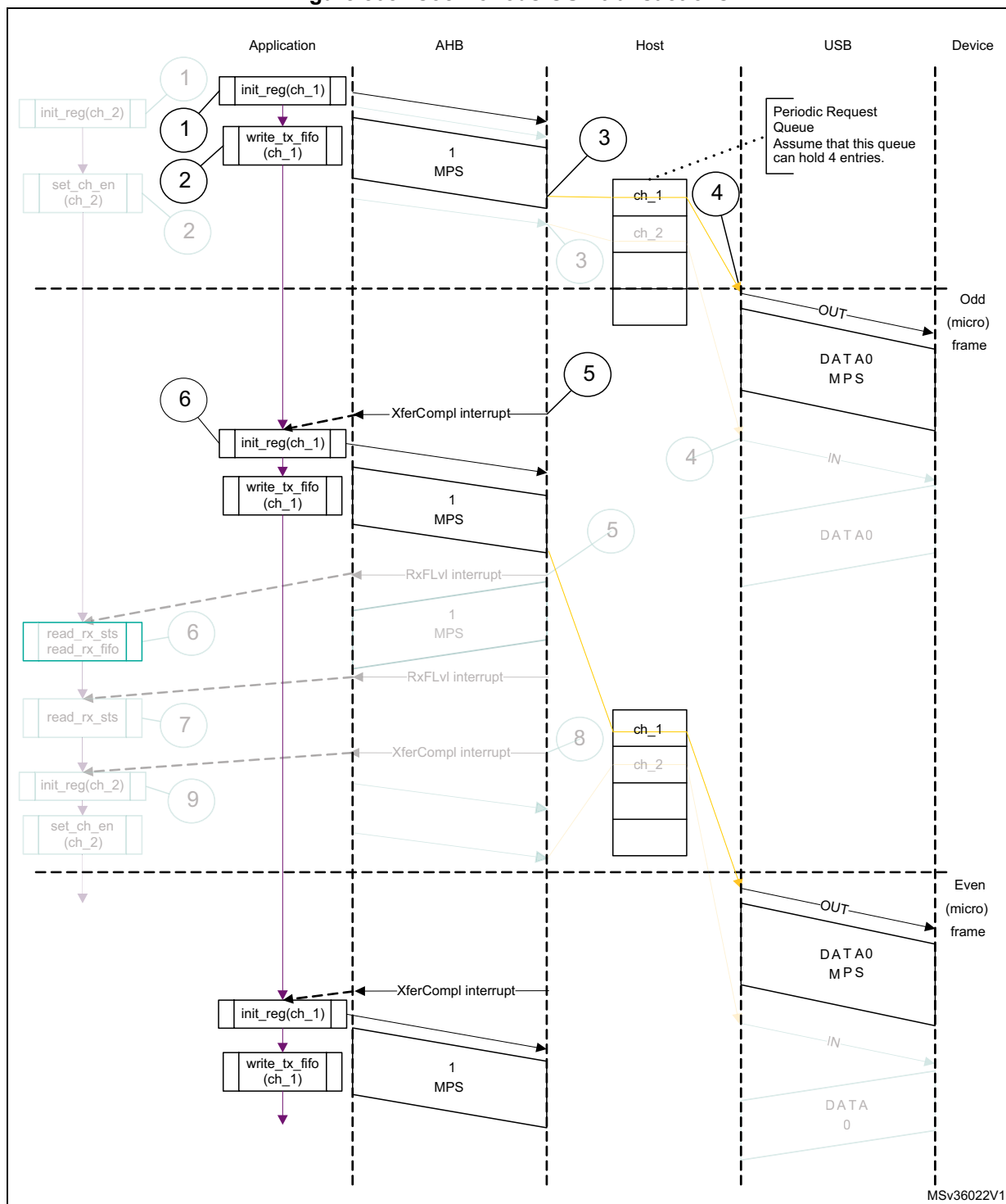
Figure 808. Isochronous OUT transactions
