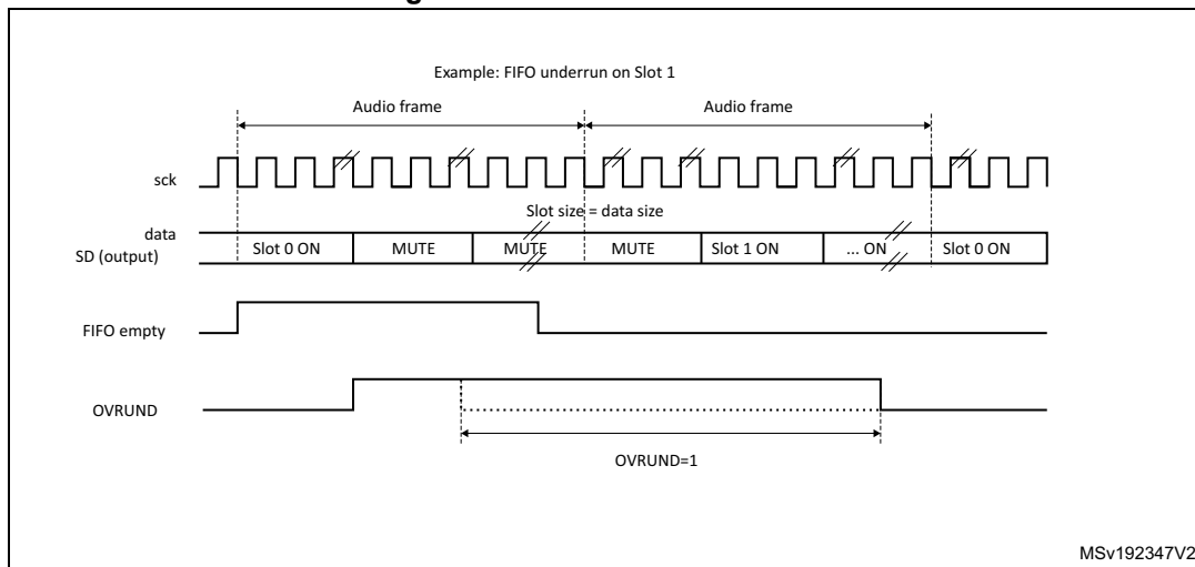
Figure 710. FIFO underrun event
