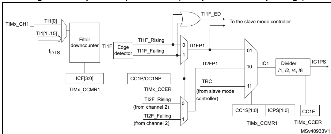
Figure 509. Capture/compare channel (example: channel 1 input stage)
