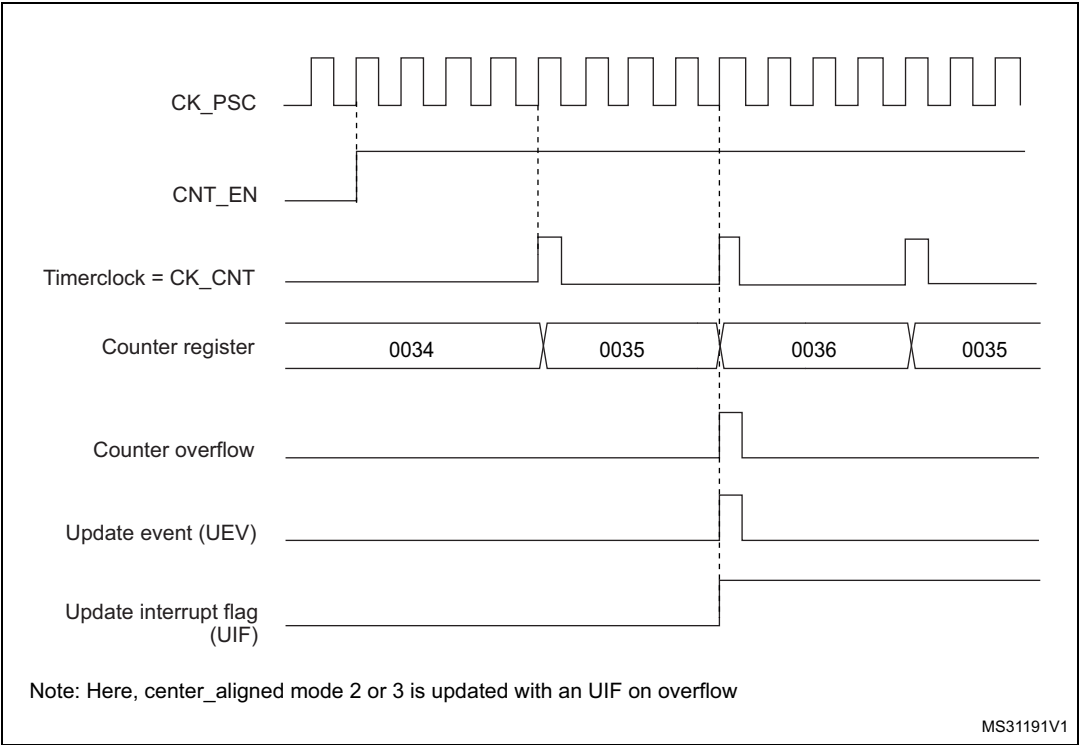
Figure 402. Counter timing diagram, internal clock divided by 4, TIMx_ARR=0x36
