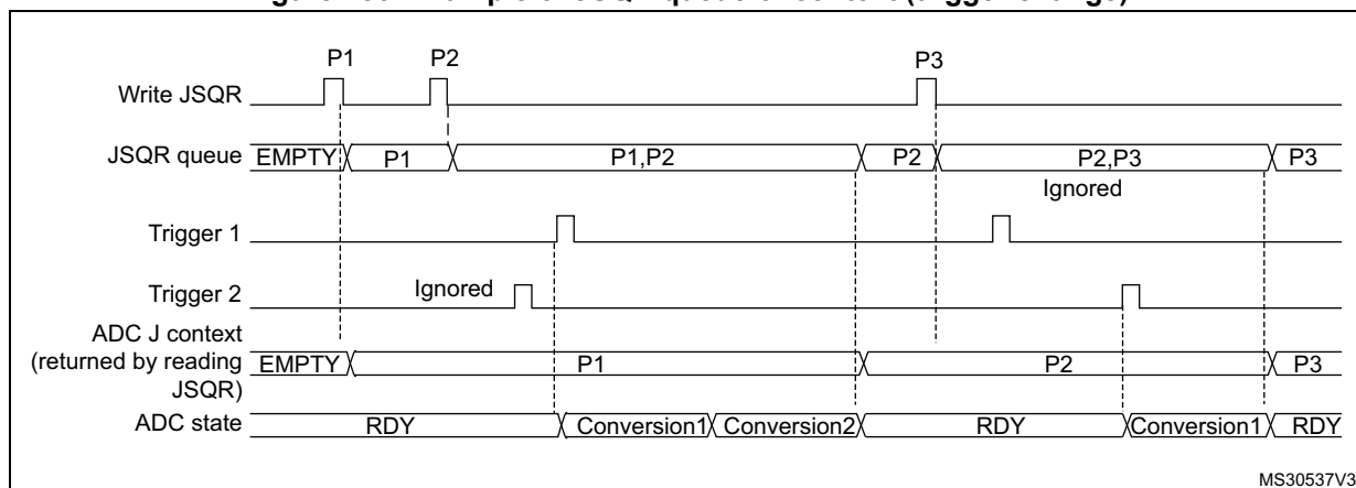
Figure 156. Example of JSQR queue of context (trigger change)
