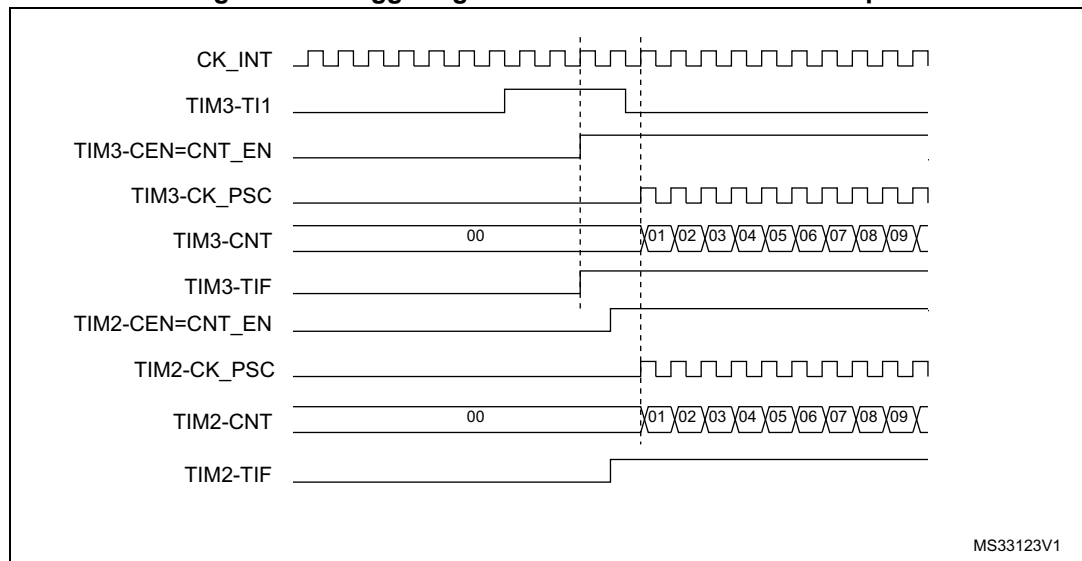
Figure 495. Triggering TIM3 and TIM2 with TIM3 TI1 input
