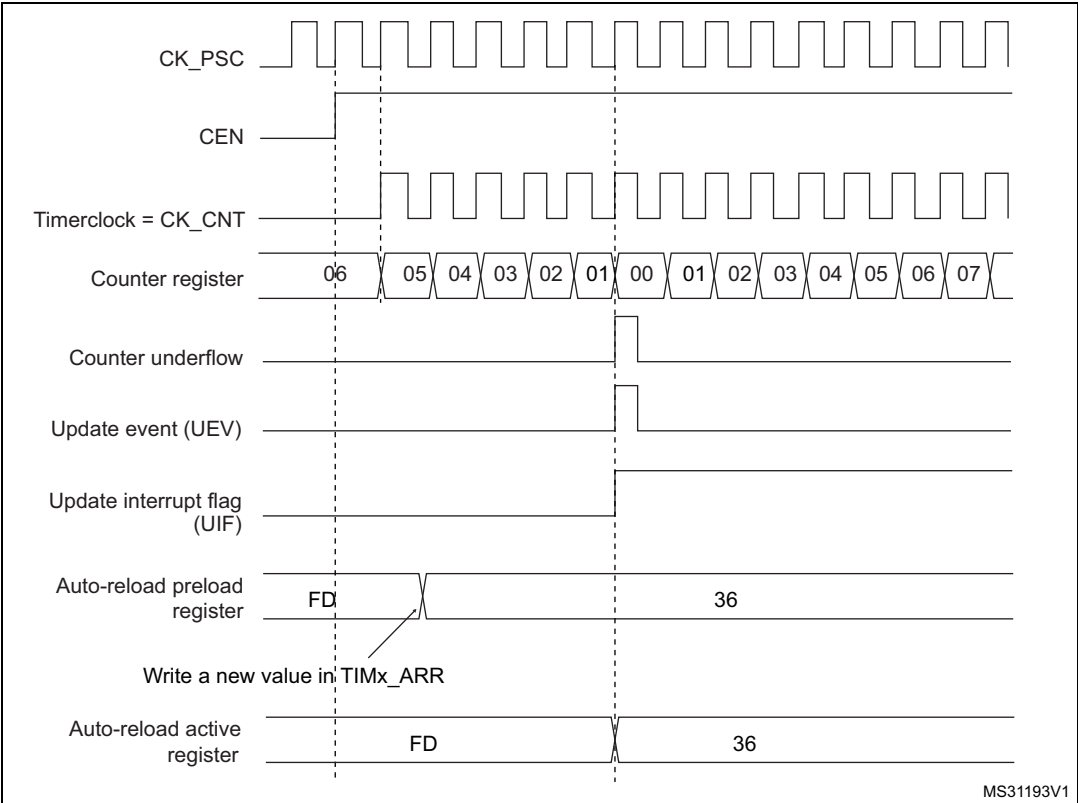
Figure 464. Counter timing diagram, Update event with ARPE=1 (counter underflow)
