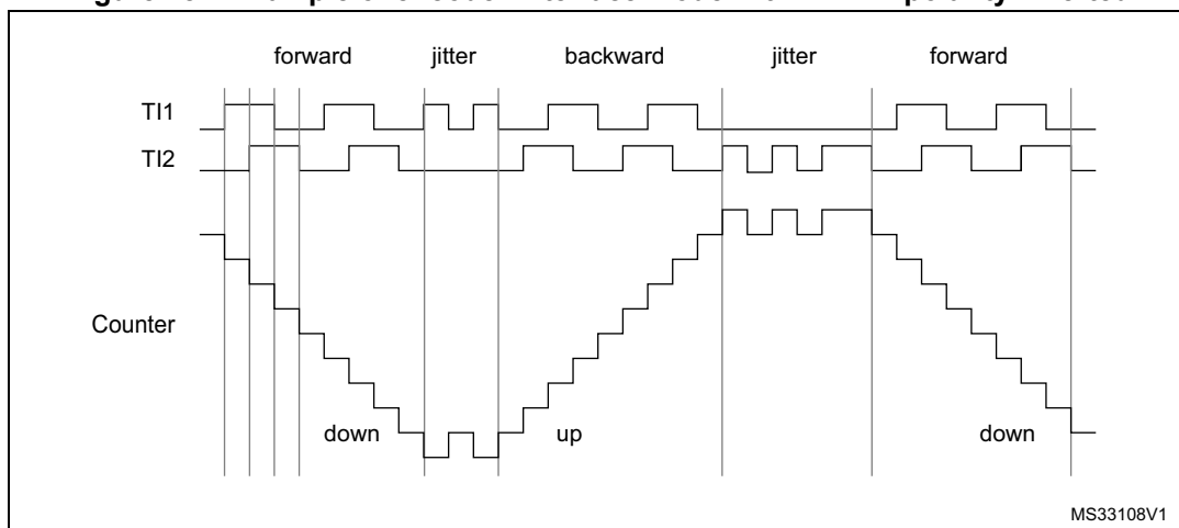
Figure 484. Example of encoder interface mode with TI1FP1 polarity inverted
