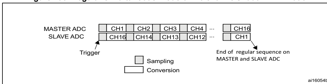
Figure 195. Regular simultaneous mode on 16 channels: dual ADC mode
