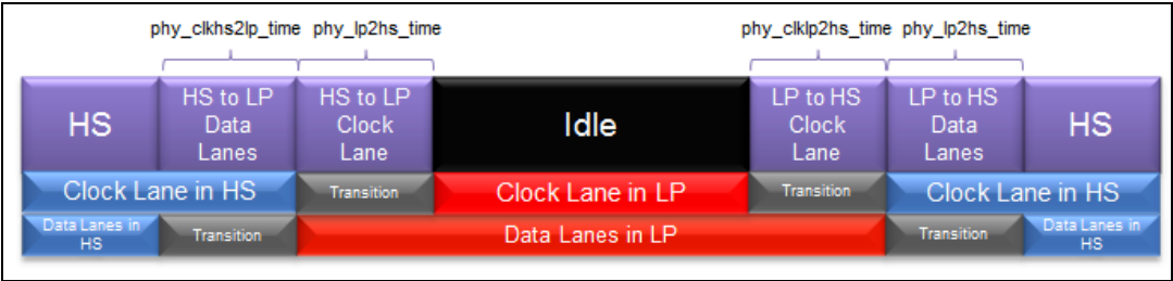
Figure 280. Clock lane and data lane in LP
