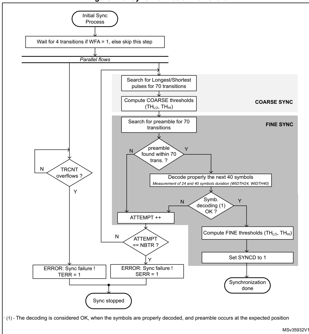
Figure 719. Synchronization flowchart
