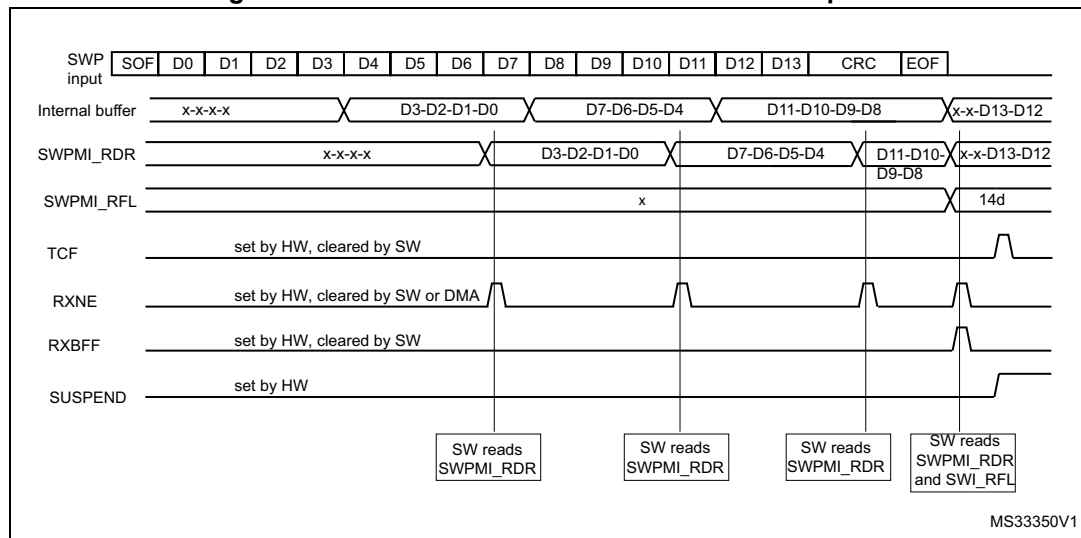
Figure 735. SWPMI No software buffer mode reception
