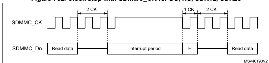
Figure 762. Clock stop with SDMMC_CK for DS, HS, SDR12, SDR25
