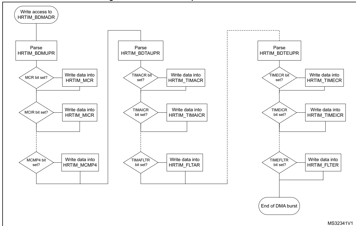
Figure 376. Burst DMA operation flowchart
