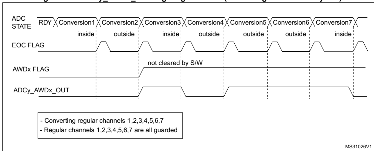
Figure 184. ADCy_AWDx_OUT signal generation (AWDx flag not cleared by SW)
