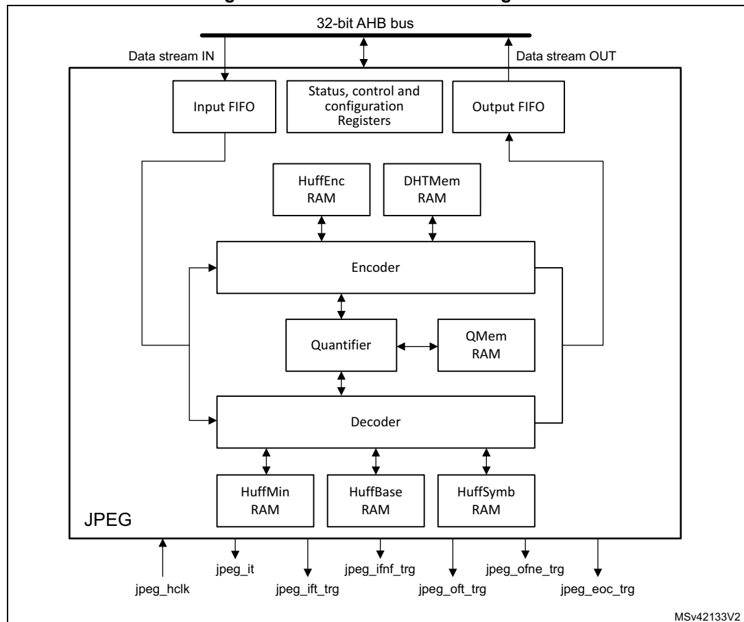
Figure 292. JPEG codec block diagram
