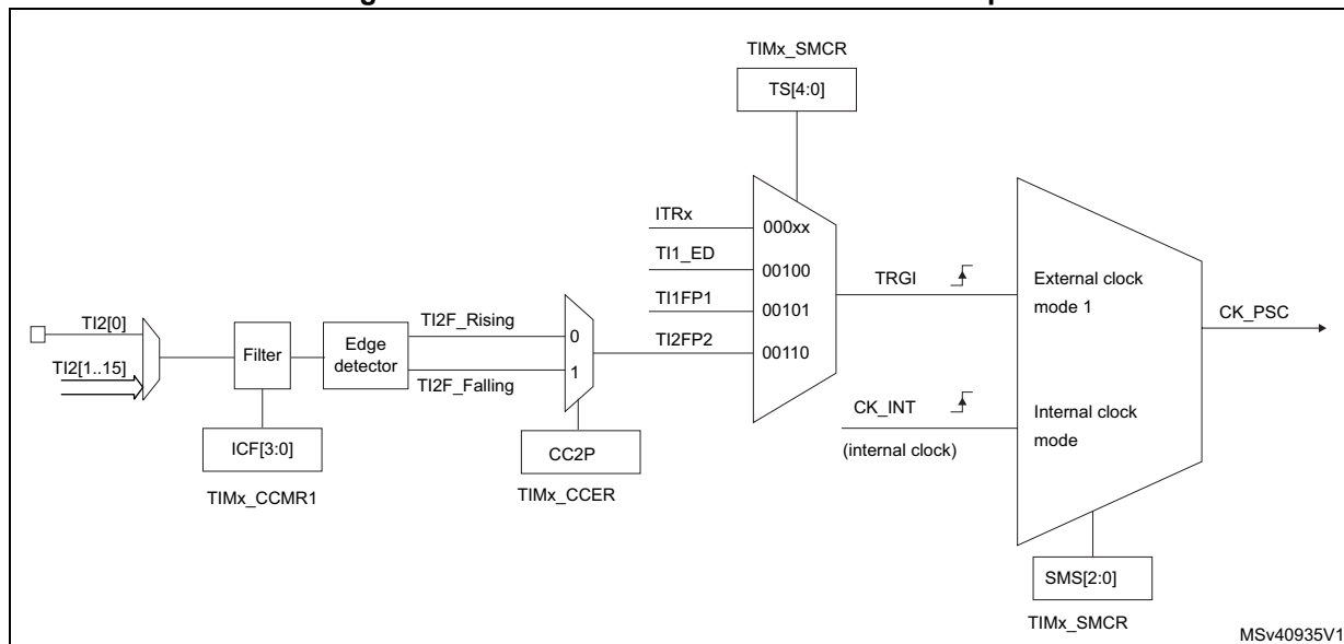
Figure 534. TI2 external clock connection example
