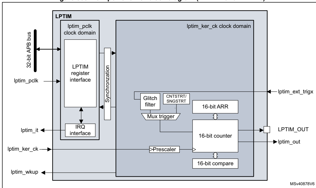
Figure 568. Low-power timer block diagram (LPTIM4 and LPTIM5)
