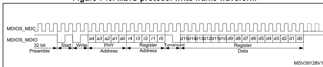
Figure 740. MDIO protocol write frame waveform
