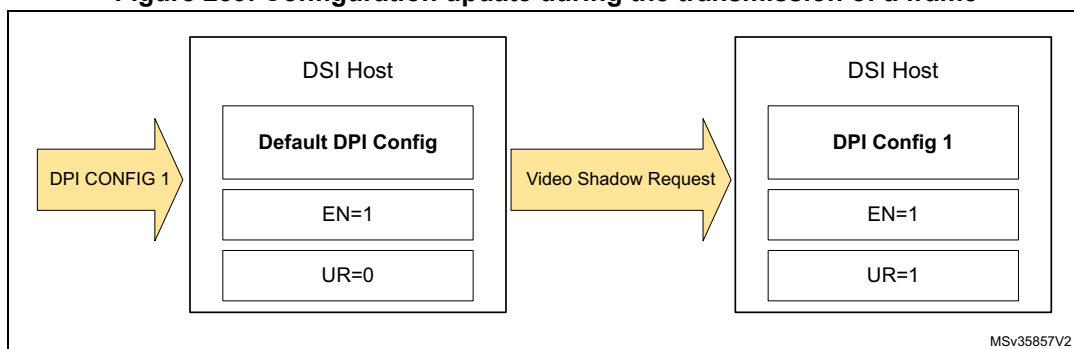
Figure 259. Configuration update during the transmission of a frame
