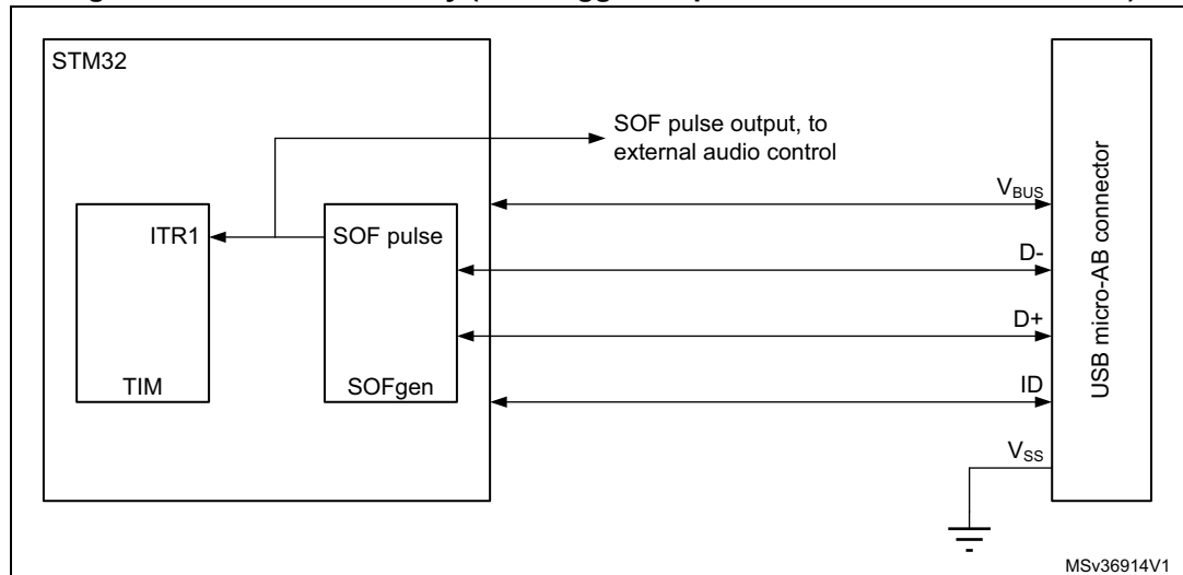
Figure 797. SOF connectivity (SOF trigger output to TIM and ITR1 connection)
