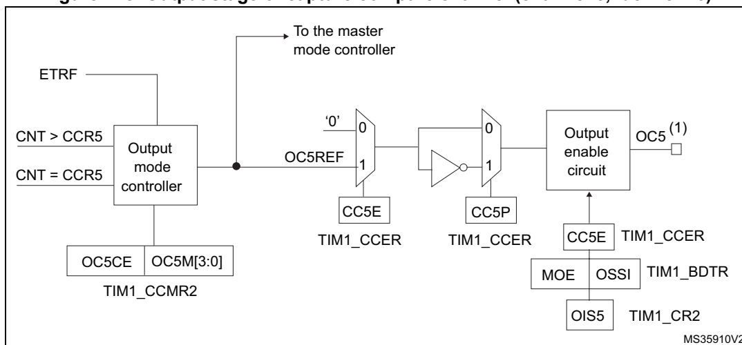
Figure 418. Output stage of capture/compare channel (channel 5, idem ch. 6)
