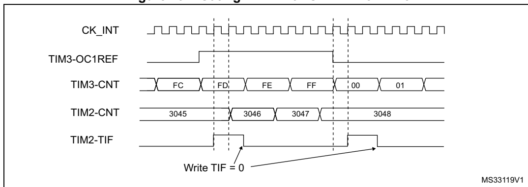
Figure 491. Gating TIM2 with OC1REF of TIM3
