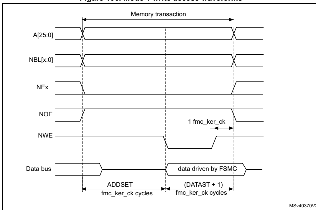
Figure 106. Mode 1 write access waveforms
