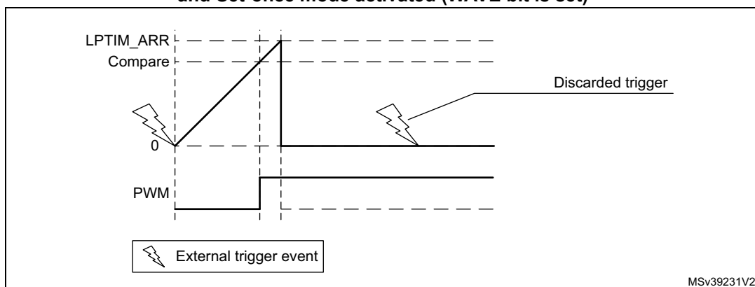
Figure 571. LPTIM output waveform, Single counting mode configuration and Set-once mode activated (WAVE bit is set)
