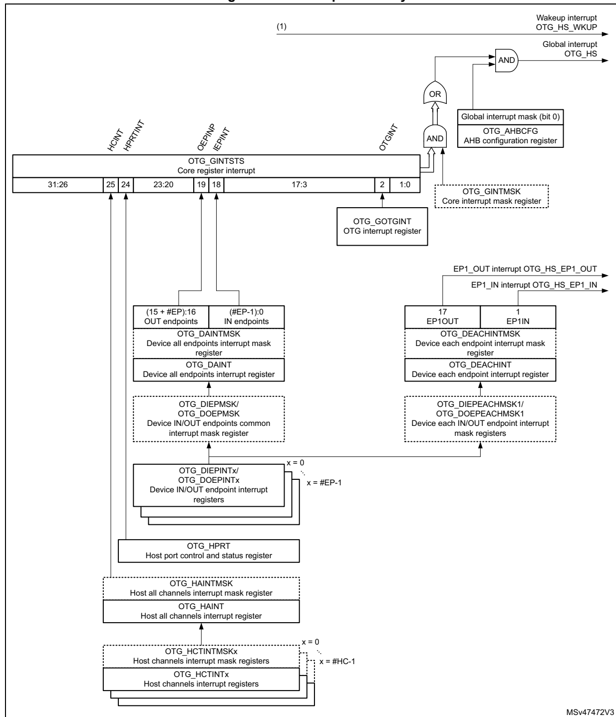
Figure 801. Interrupt hierarchy
