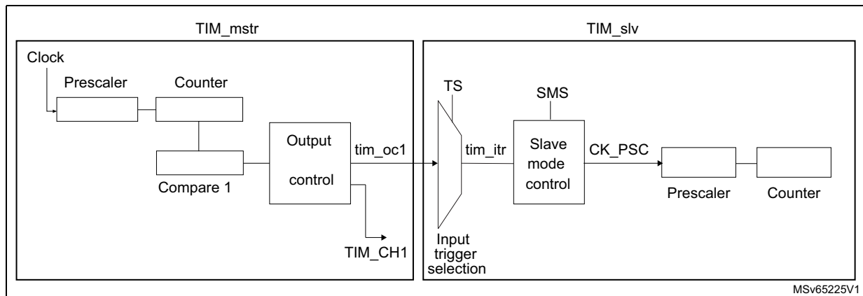
Figure 490. Master/slave connection example with 1 channel only timers
