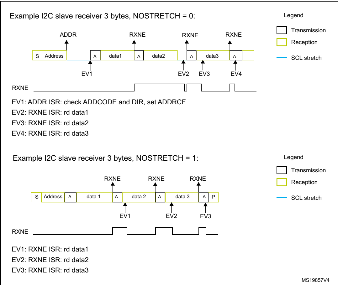
Figure 594. Transfer bus diagrams for I2C slave receiver (mandatory events only)
