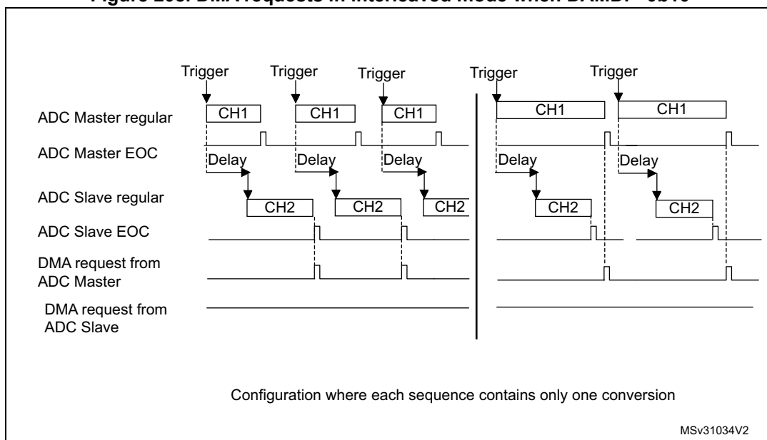
Figure 208. DMA requests in interleaved mode when DAMDF=0b10
