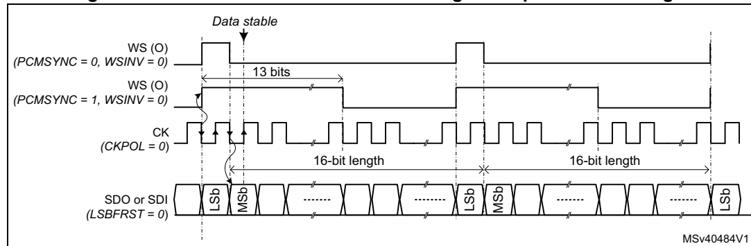
Figure 677. Master PCM when the frame length is equal the data length
