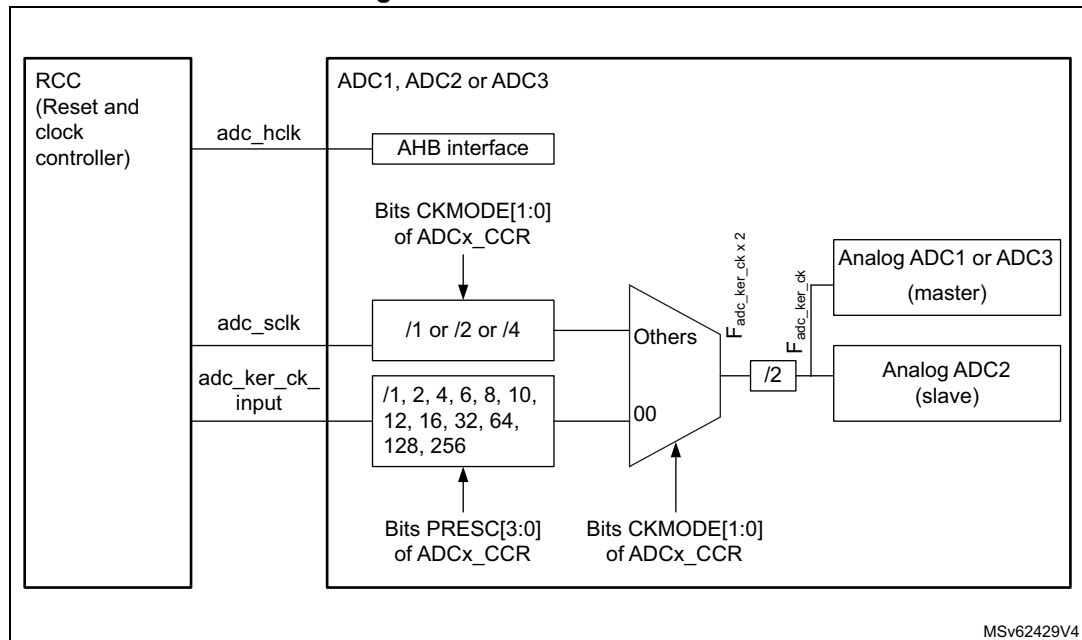
Figure 142. ADC Clock scheme
