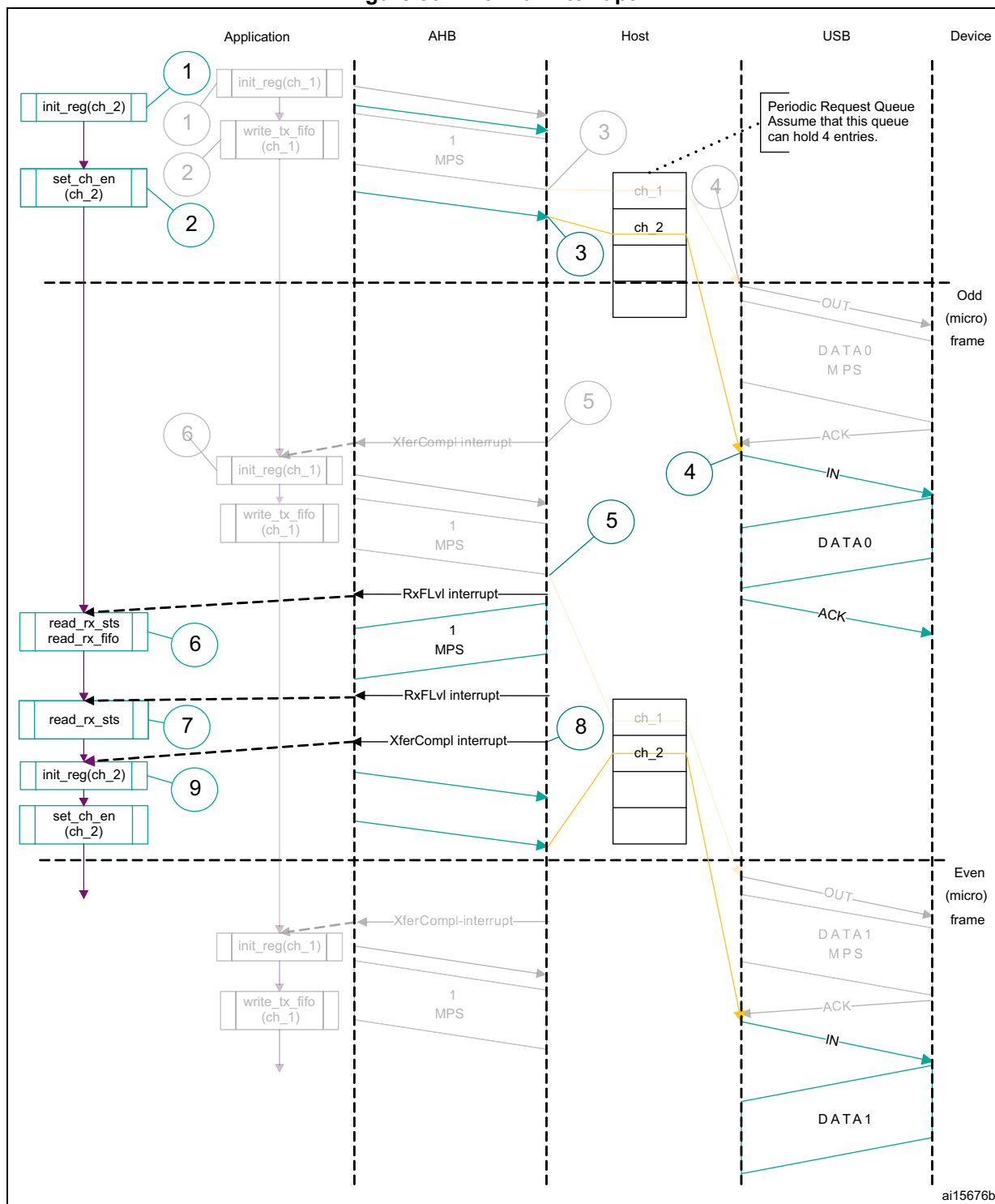
Figure 807. Normal interrupt IN
