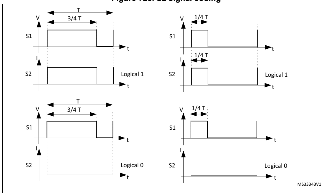
Figure 728. S2 signal coding
