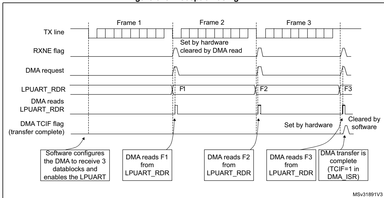
Figure 648. Reception using DMA
