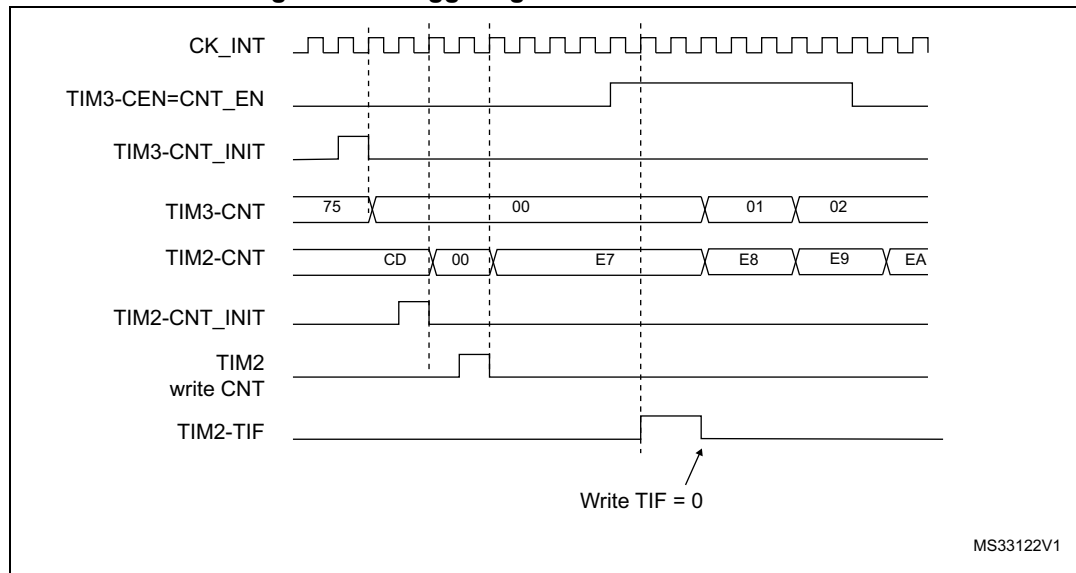
Figure 494. Triggering TIM2 with Enable of TIM3
