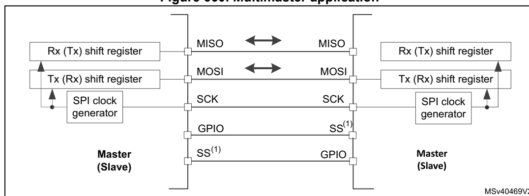
Figure 660. Multimaster application
