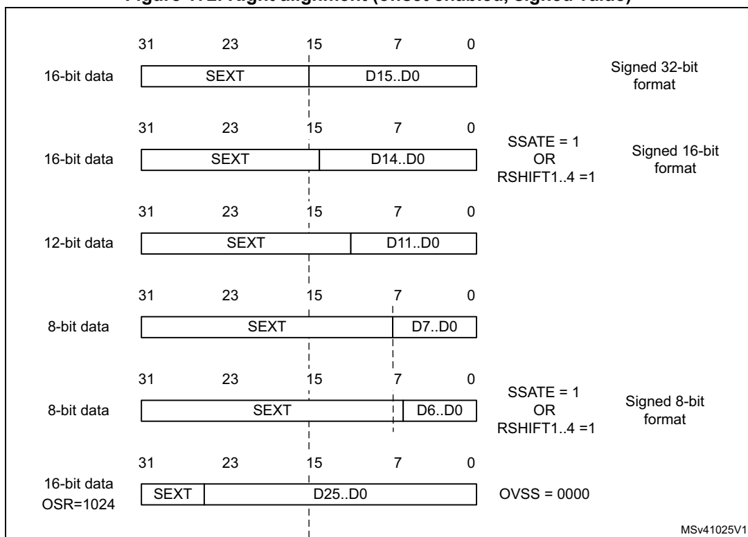
Figure 172. Right alignment (offset enabled, signed value)
