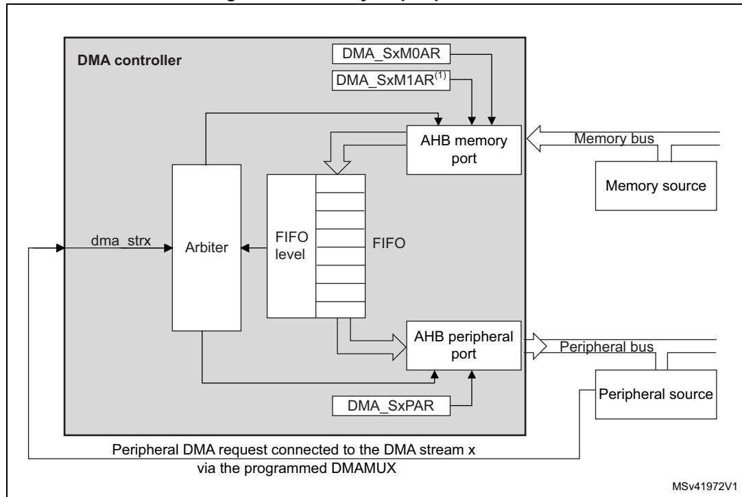
Figure 86. Memory-to-peripheral mode
