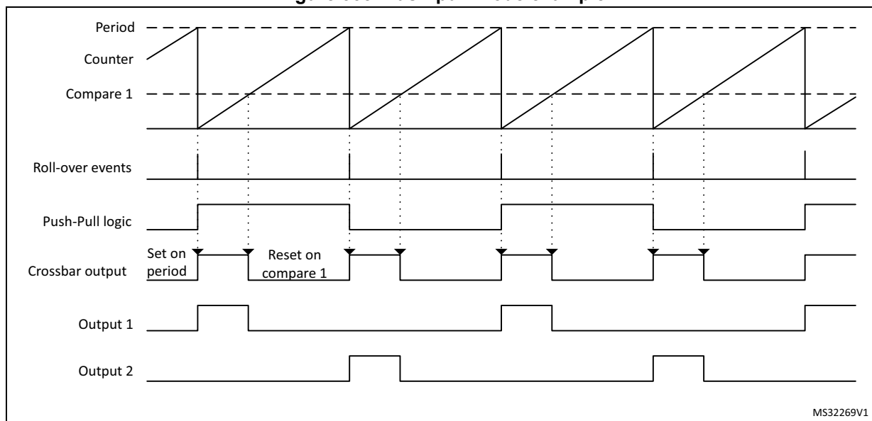
Figure 335. Push-pull mode example
