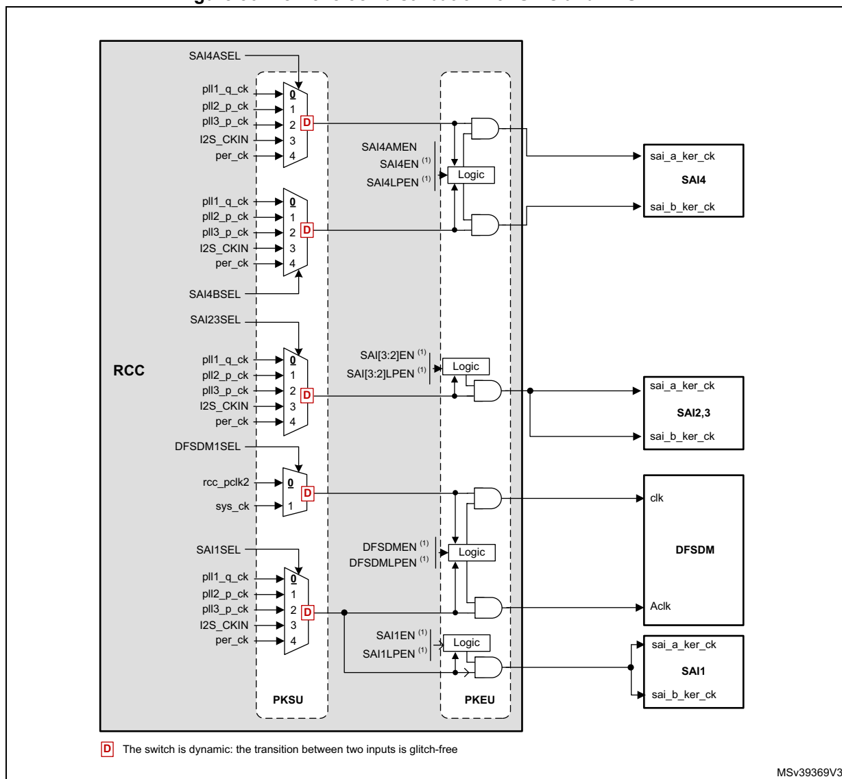
Figure 56. Kernel clock distribution for SAIs and DFSDM1
