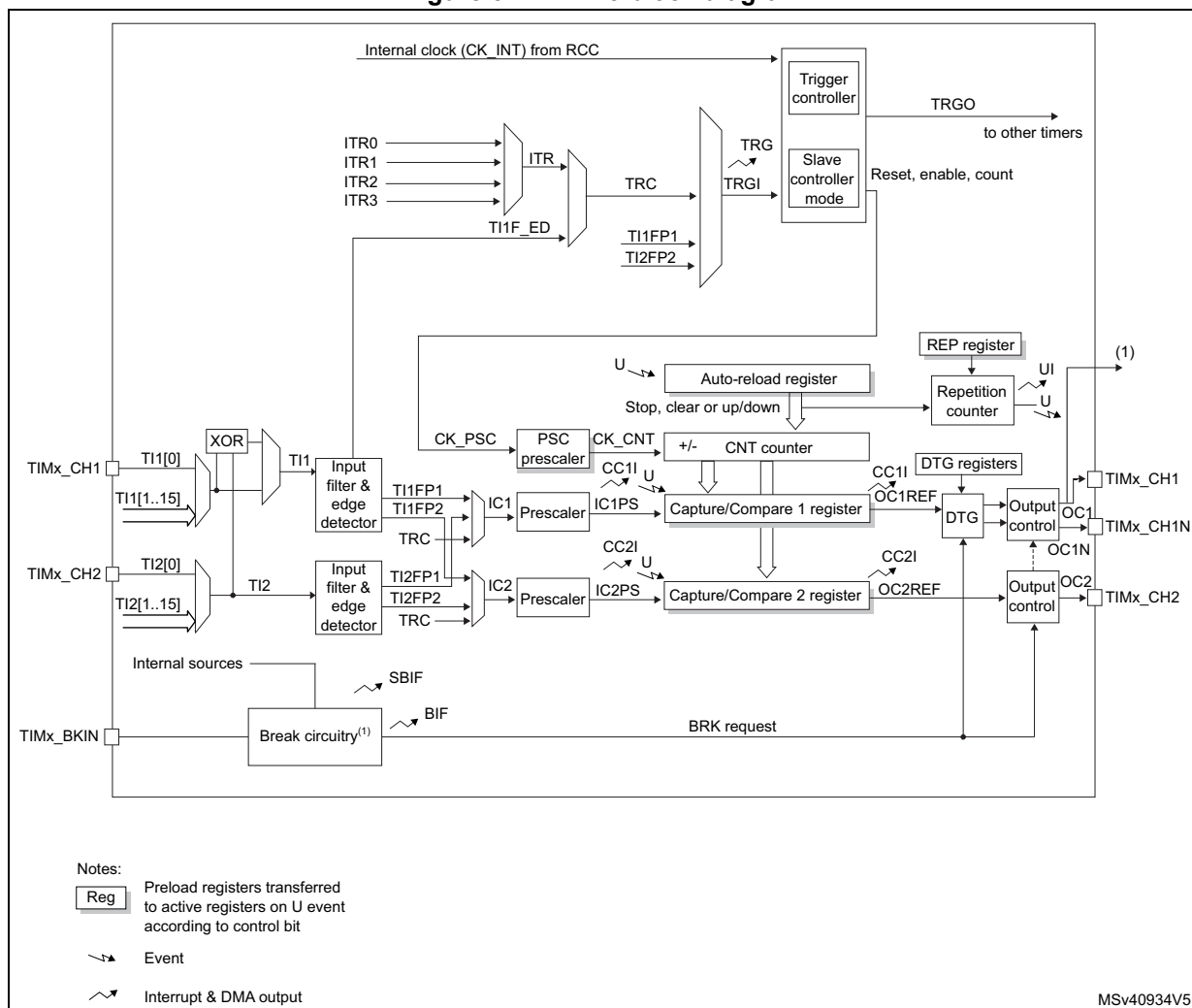
Figure 522. TIM15 block diagram
