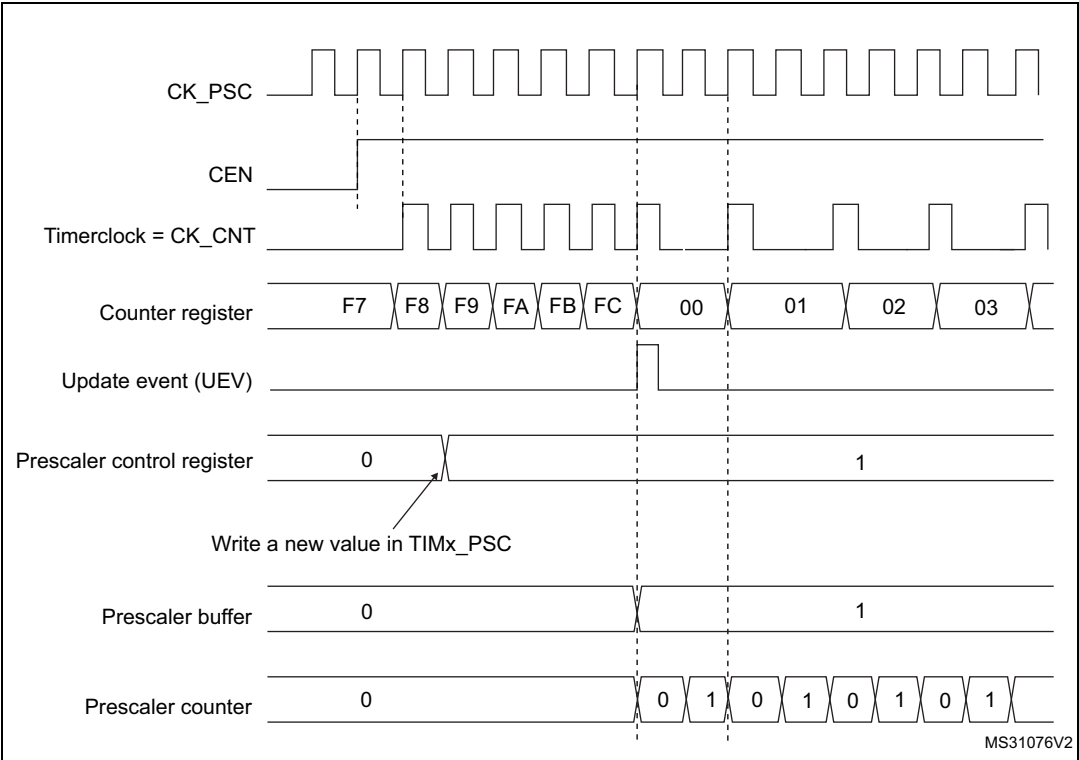
Figure 498. Counter timing diagram with prescaler division change from 1 to 2
