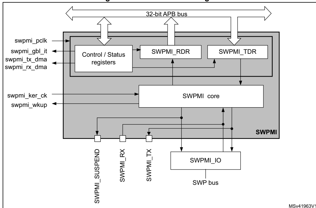
Figure 729. SWPMI block diagram
