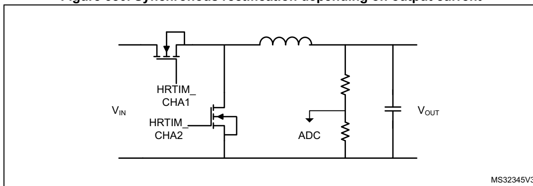
Figure 380. Synchronous rectification depending on output current
