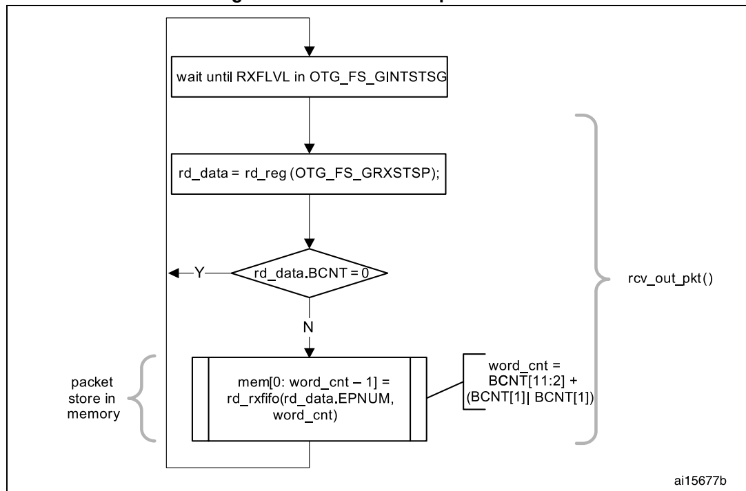
Figure 816. Receive FIFO packet read
