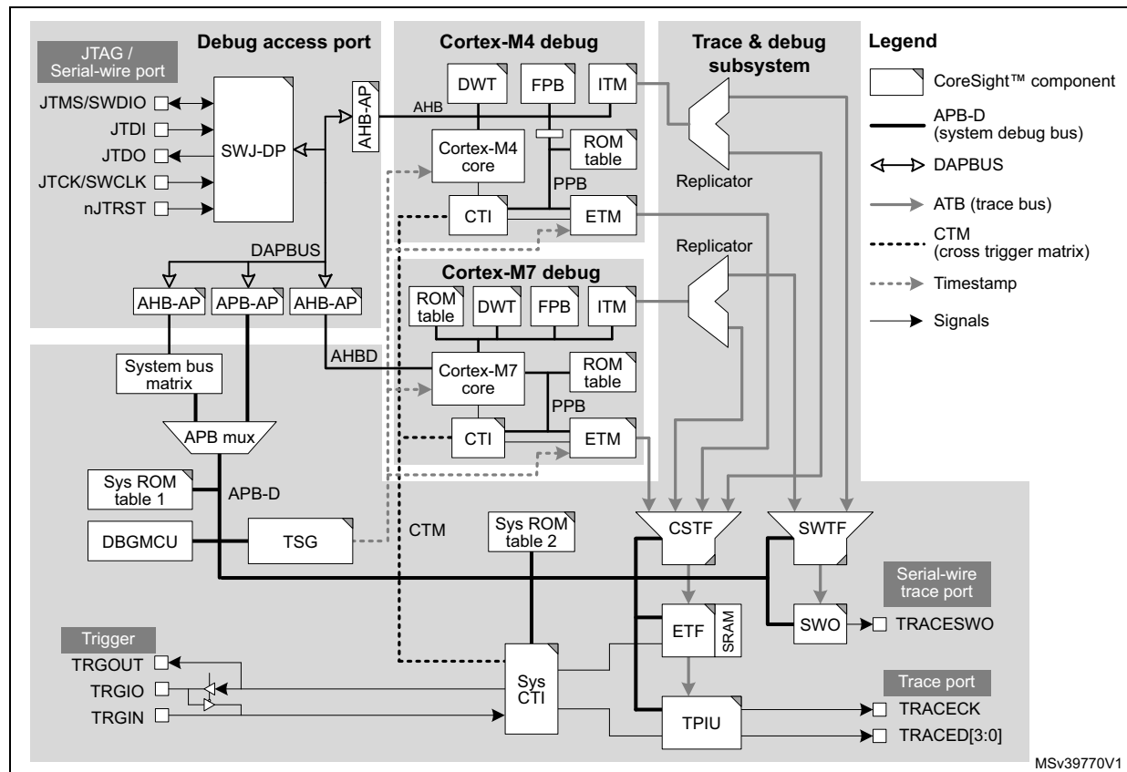
Figure 870. Block diagram of debug infrastructure
