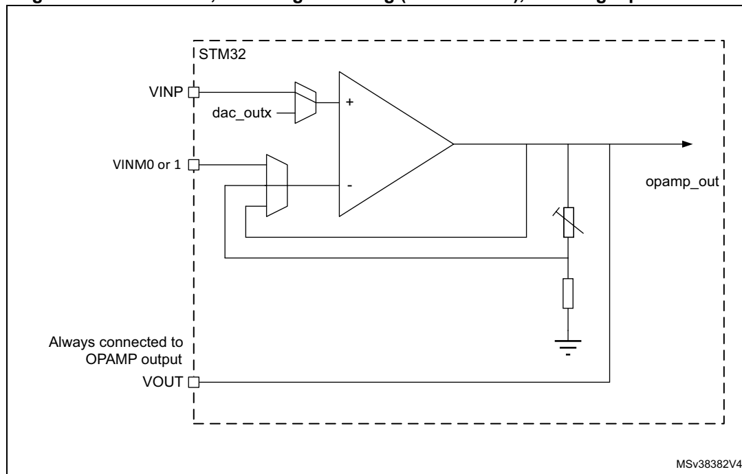
Figure 228. PGA mode, internal gain setting (x2/x4/x8/x16), inverting input not used
