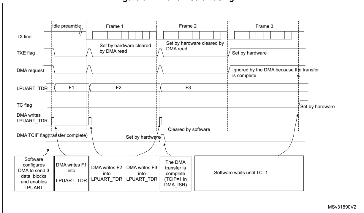
Figure 647. Transmission using DMA
