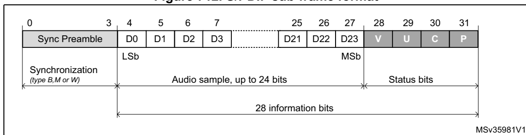
Figure 712. S/PDIF sub-frame format
