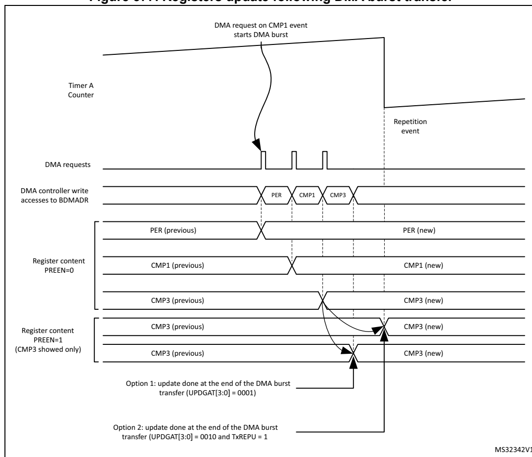
Figure 377. Registers update following DMA burst transfer
