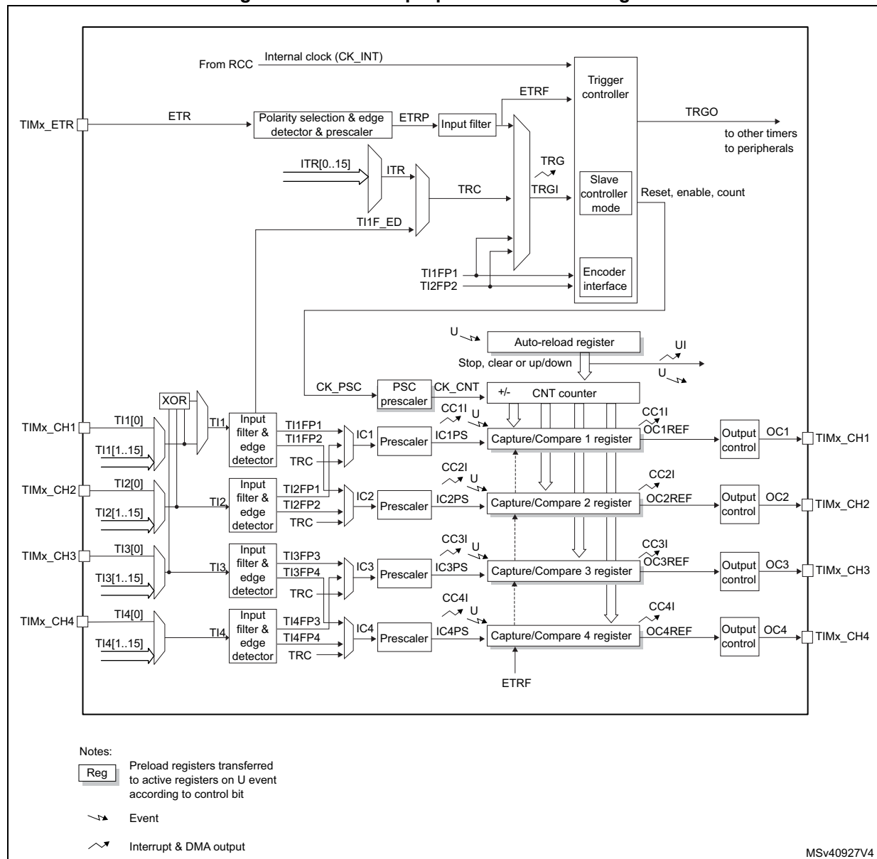
Figure 446. General-purpose timer block diagram
