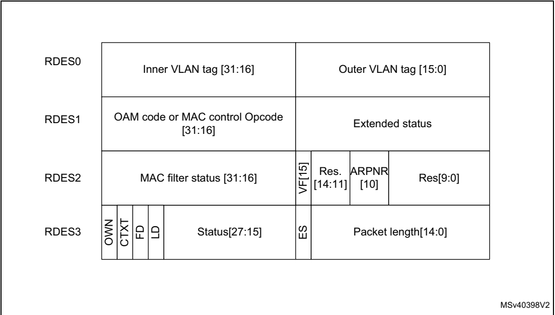
Figure 857. Receive normal descriptor (write-back format)
