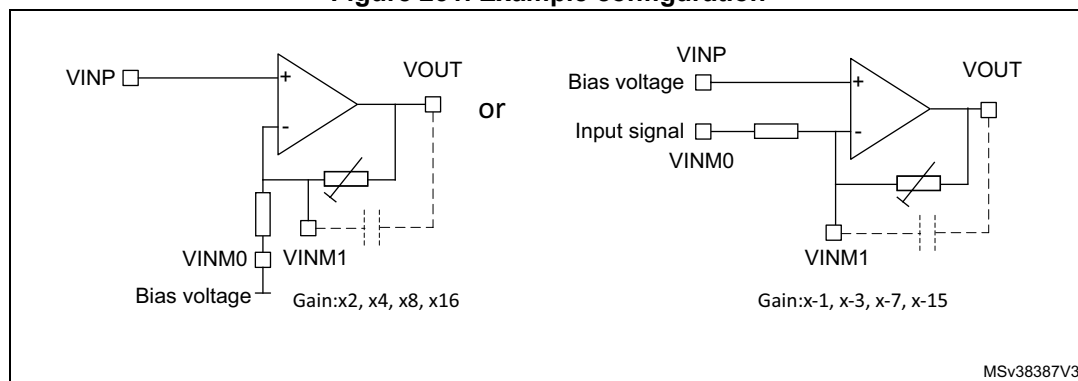
Figure 231. Example configuration
