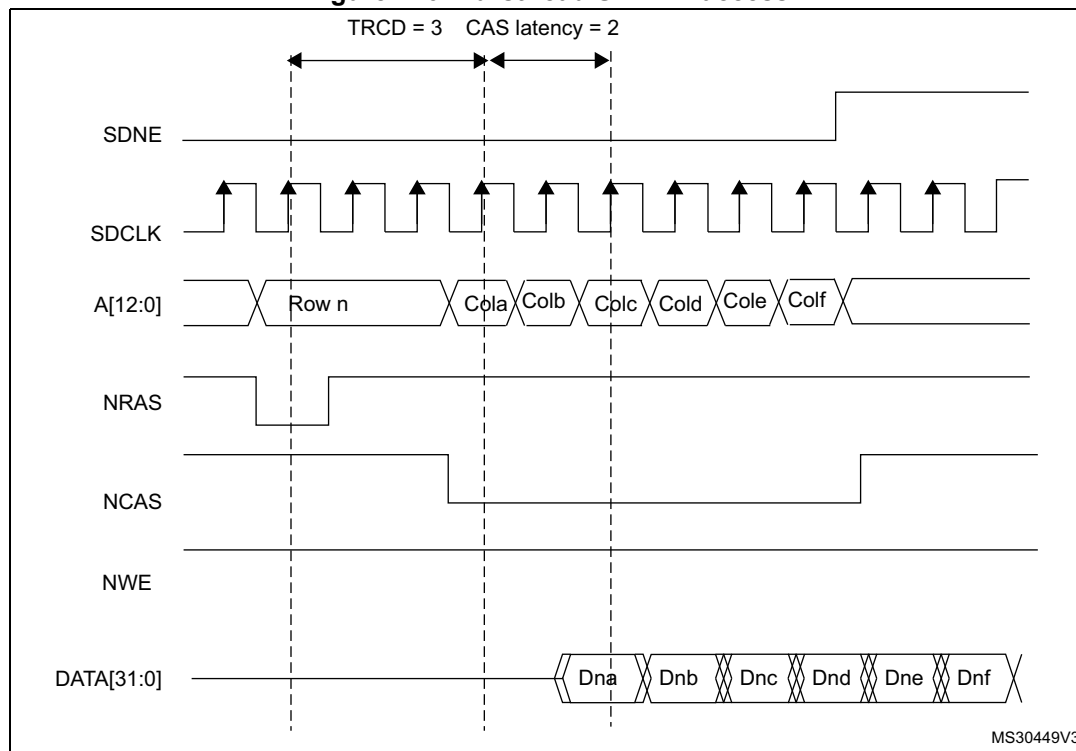
Figure 126. Burst read SDRAM access
