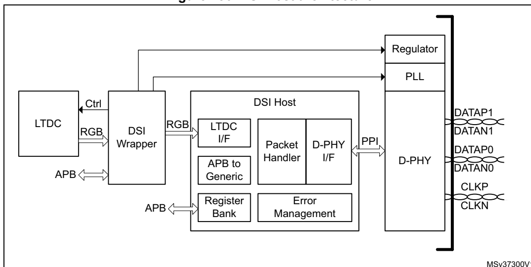
Figure 256. DSI Host architecture
