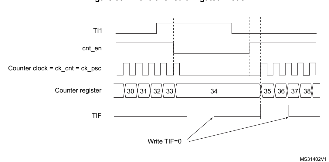
Figure 554. Control circuit in gated mode
