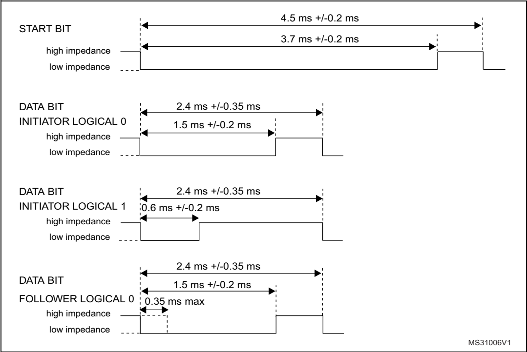
Figure 863. Bit timings
