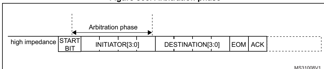
Figure 865. Arbitration phase
