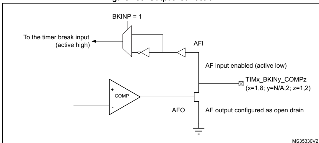
Figure 433. Output redirection
