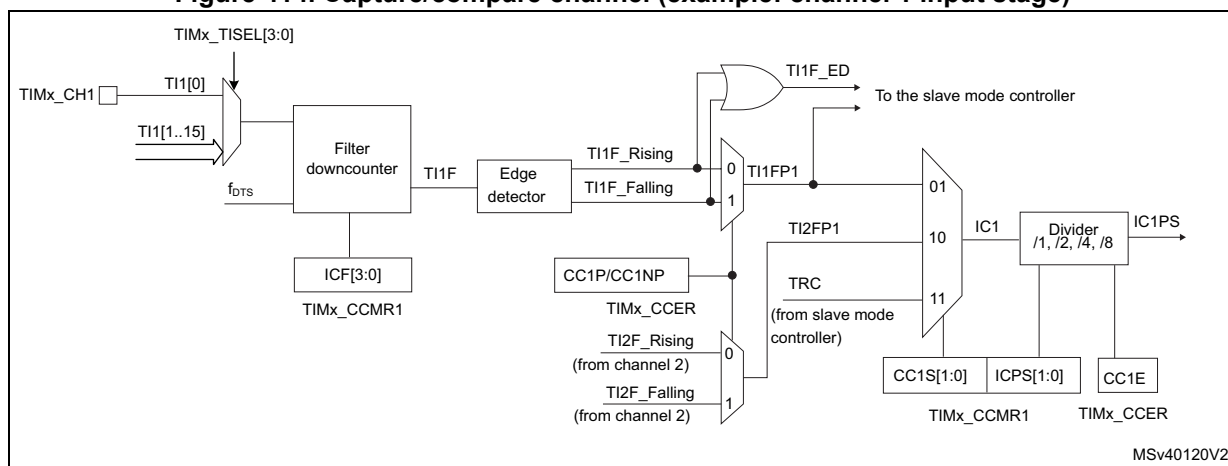
Figure 414. Capture/compare channel (example: channel 1 input stage)
