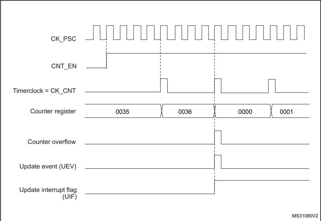
Figure 451. Counter timing diagram, internal clock divided by 4
