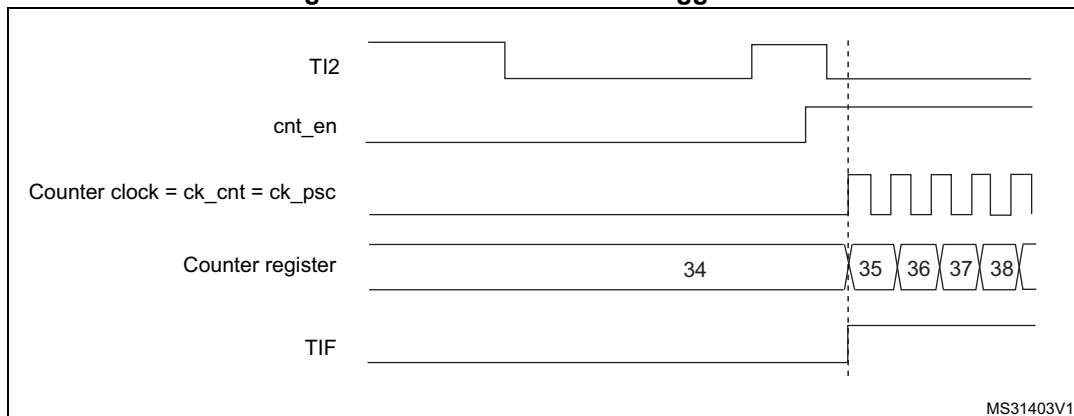
Figure 521. Control circuit in trigger mode
