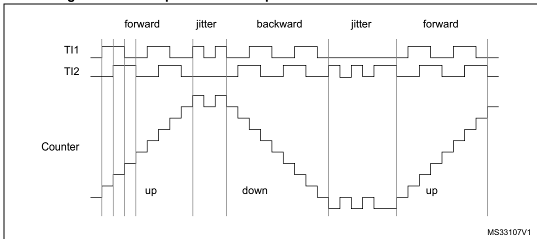
Figure 438. Example of counter operation in encoder interface mode.
