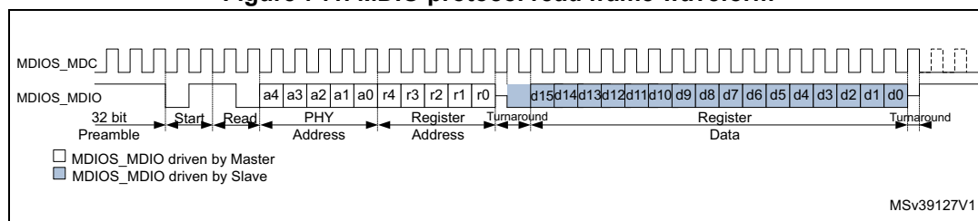
Figure 741. MDIO protocol read frame waveform
