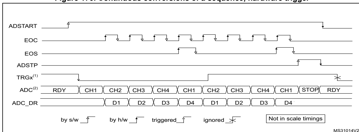
Figure 170. Continuous conversions of a sequence, hardware trigger
