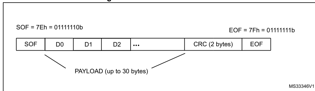
Figure 731. SWP frame structure
