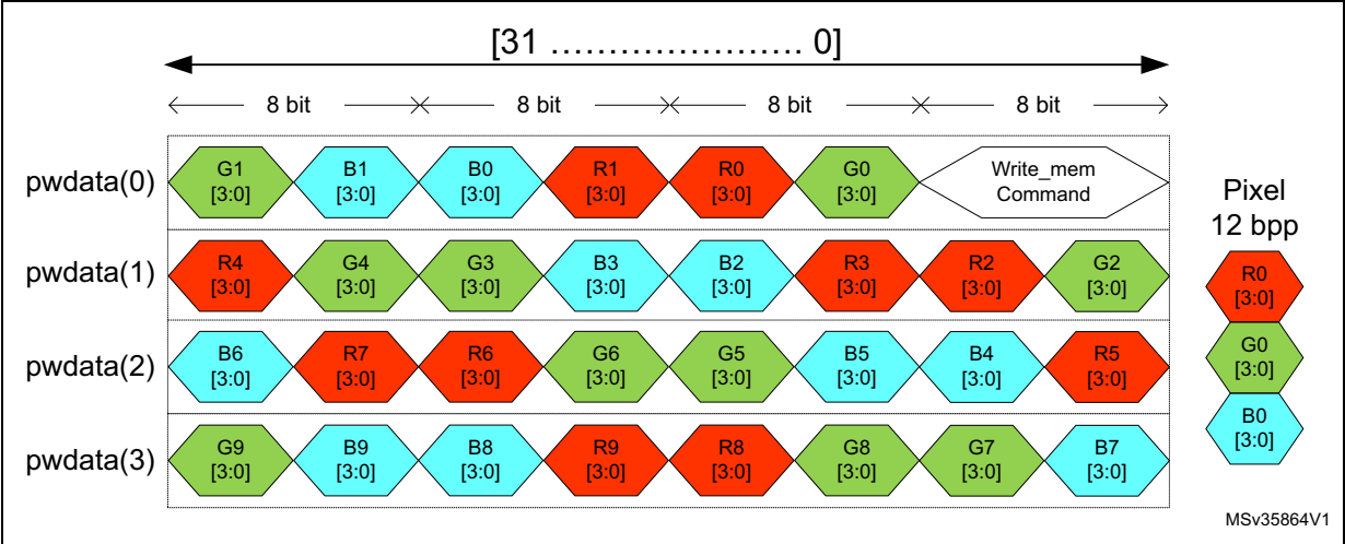
Figure 264. 12 bpp APB pixel to byte organization
