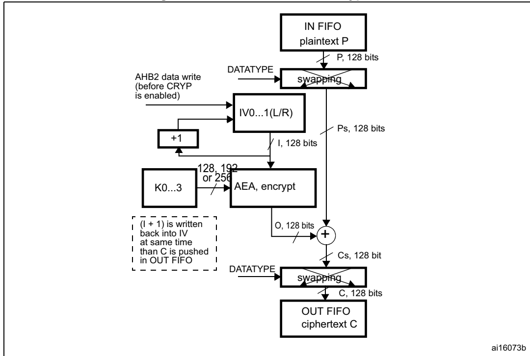
Figure 313. AES-CTR mode encryption
