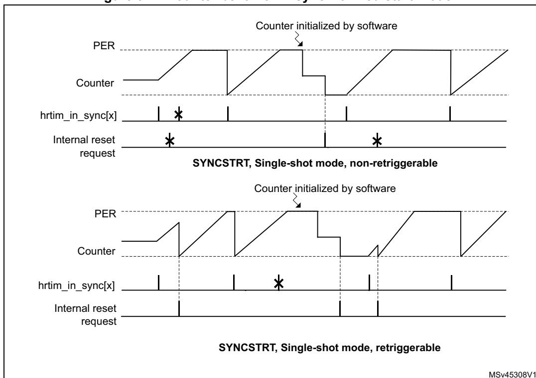
Figure 372. Counter behavior in synchronized start mode
