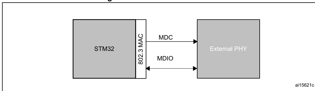
Figure 838. SMA Interface block
