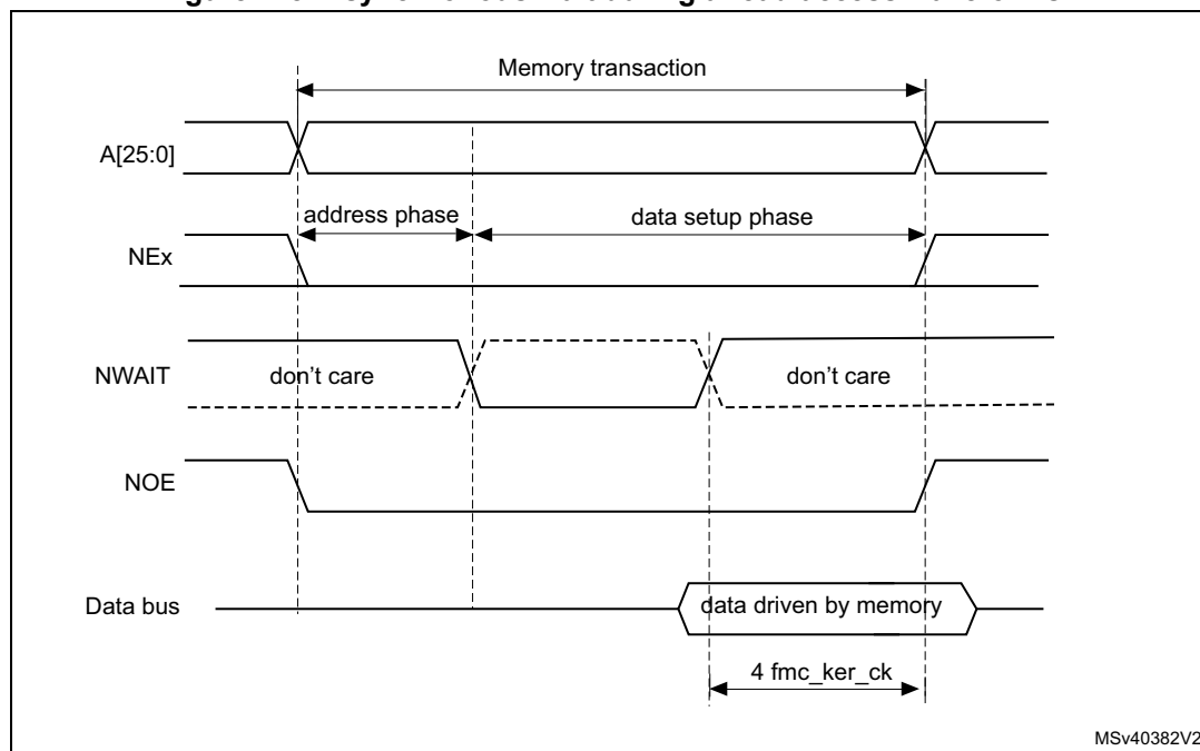
Figure 118. Asynchronous wait during a read access waveforms
