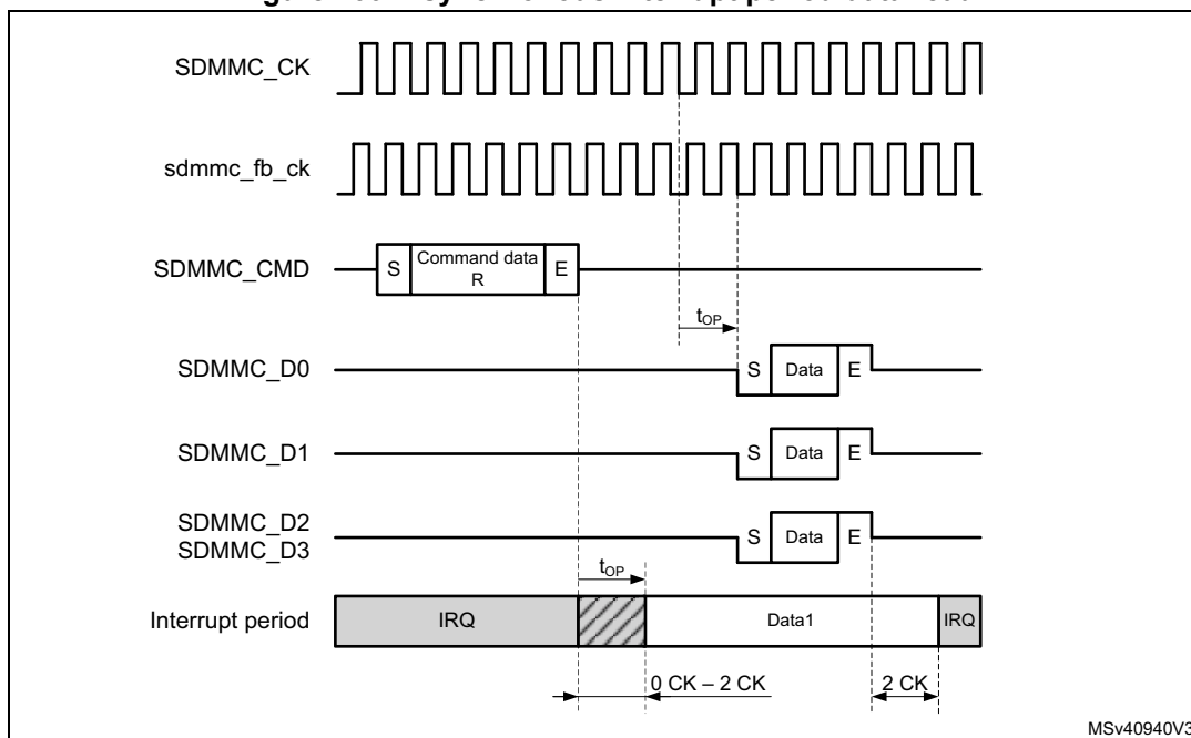
Figure 760. Asynchronous interrupt period data read
