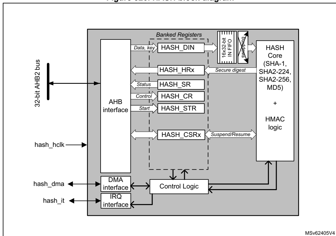
Figure 320. HASH block diagram
