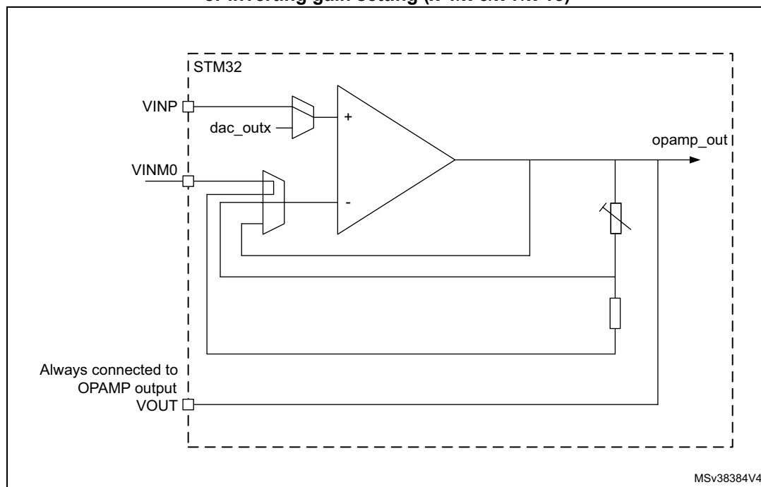
Figure 230. PGA mode, non-inverting gain setting (x2/x4/x8/x16) or inverting gain setting (x-1/x-3/x-7/x-15)
