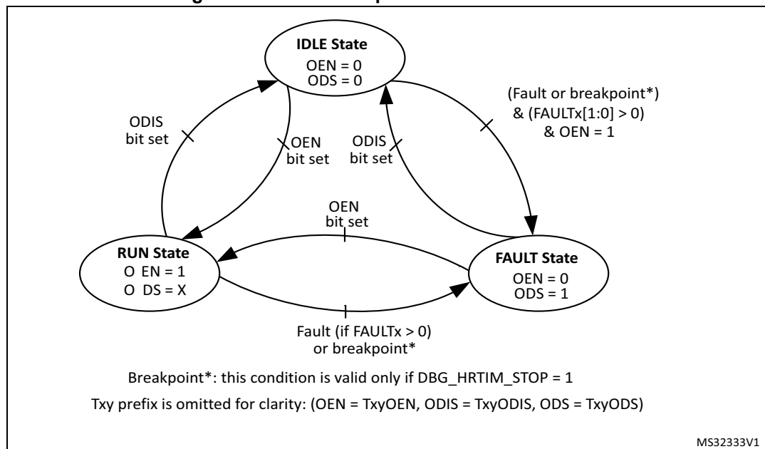
Figure 358. HRTIM output states and transitions
