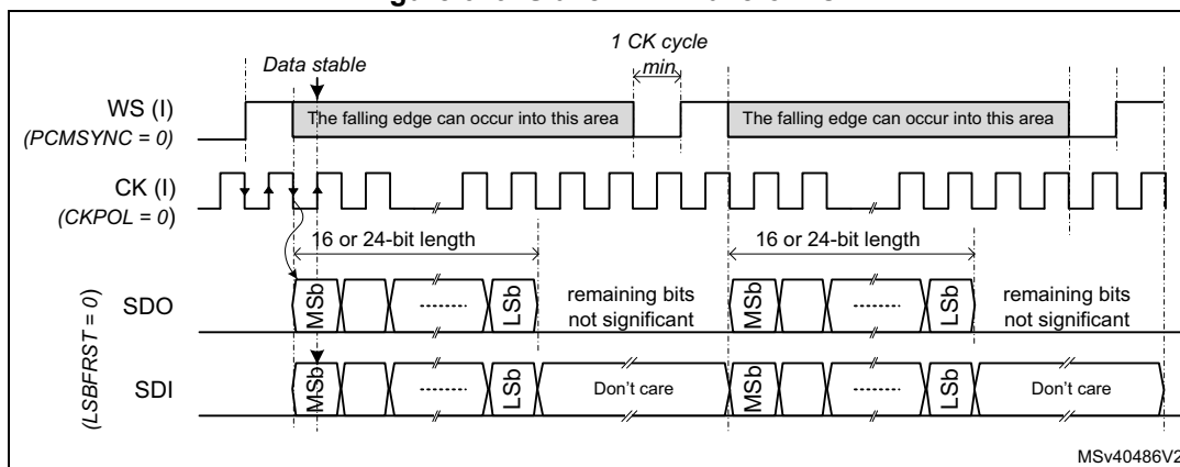
Figure 679. Slave PCM waveforms
