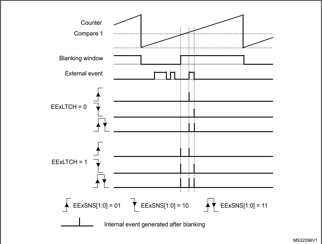
Figure 348. External trigger blanking with edge-sensitive trigger
