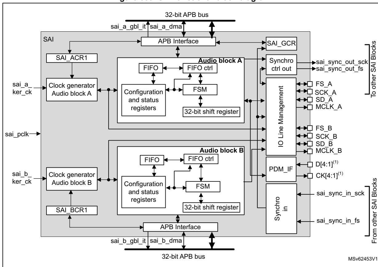
Figure 689. SAI functional block diagram
