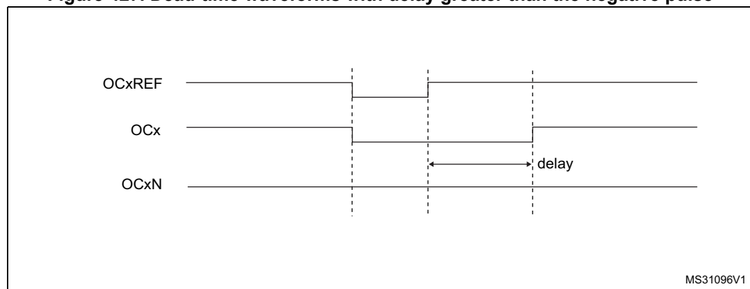
Figure 427. Dead-time waveforms with delay greater than the negative pulse
