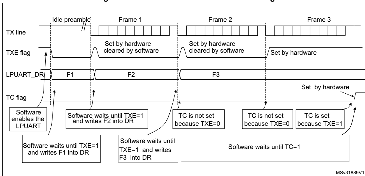
Figure 643. TC/TXE behavior when transmitting
