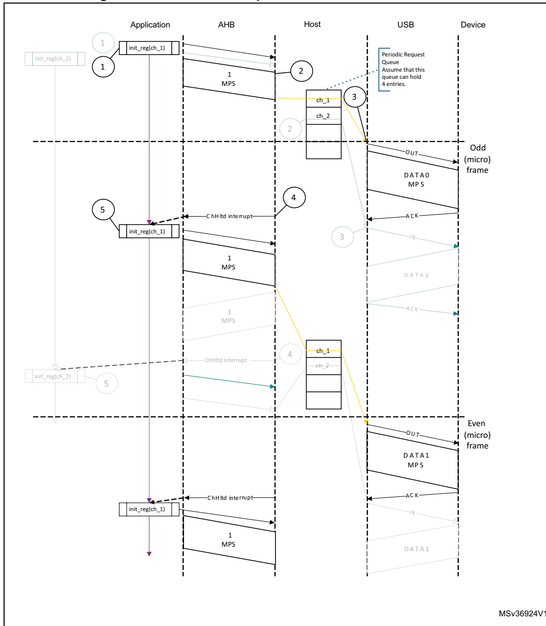
Figure 812. Normal interrupt OUT transactions - DMA mode
