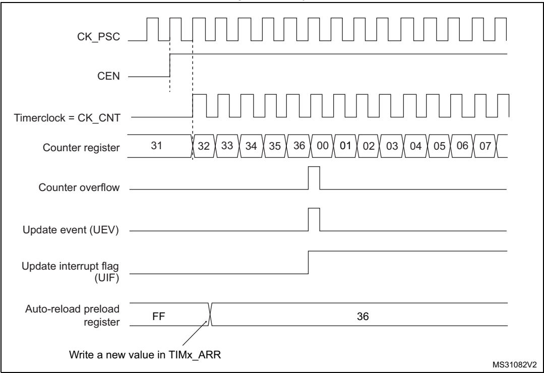
Figure 504. Counter timing diagram, update event when ARPE=0 (TIMx_ARR not preloaded)
