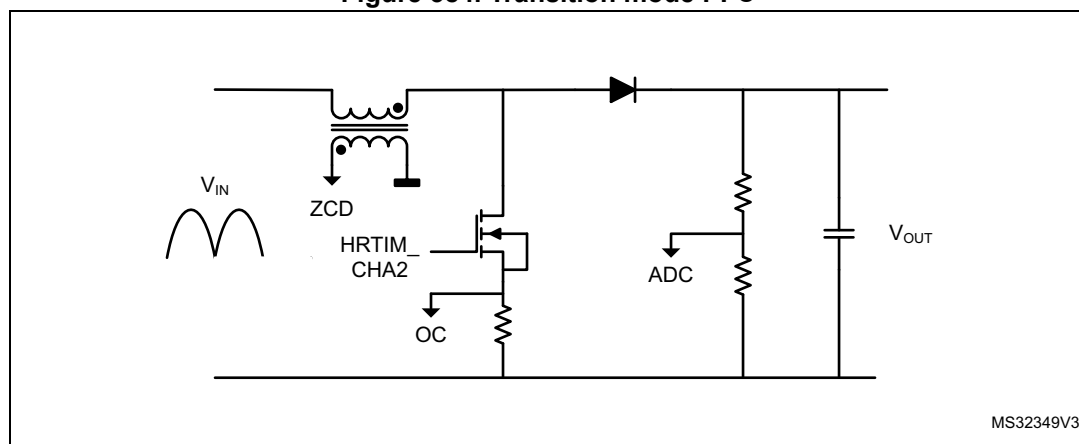
Figure 384. Transition mode PFC
