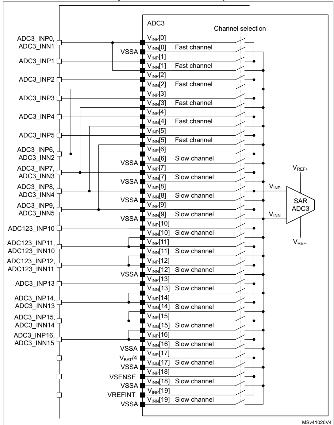
Figure 145. ADC3 connectivity
