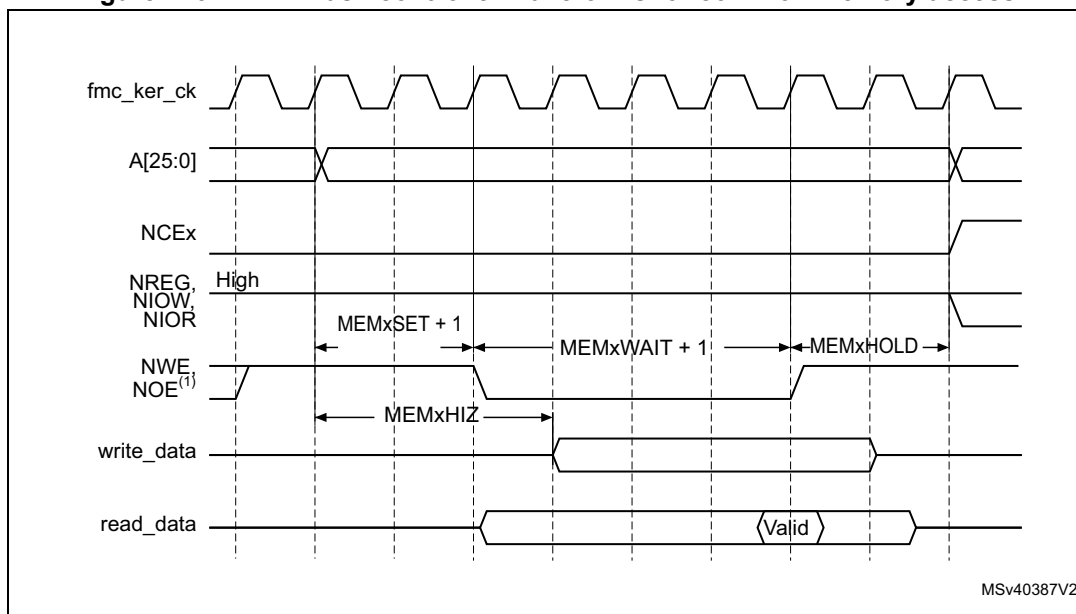
Figure 123. NAND flash controller waveforms for common memory access
