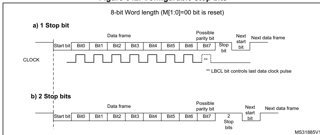
Figure 642. Configurable stop bits
