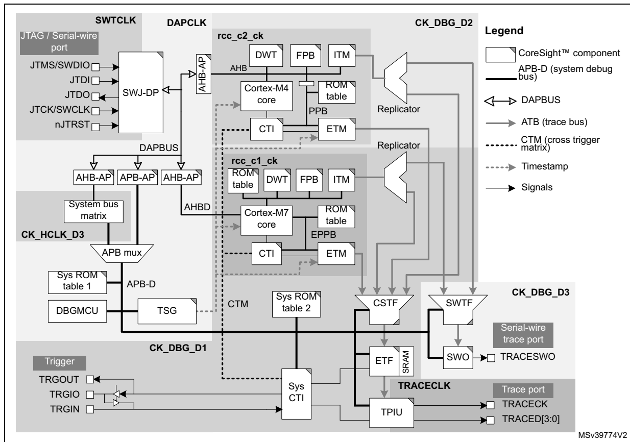
Figure 872. Clock domains of debug infrastructure
