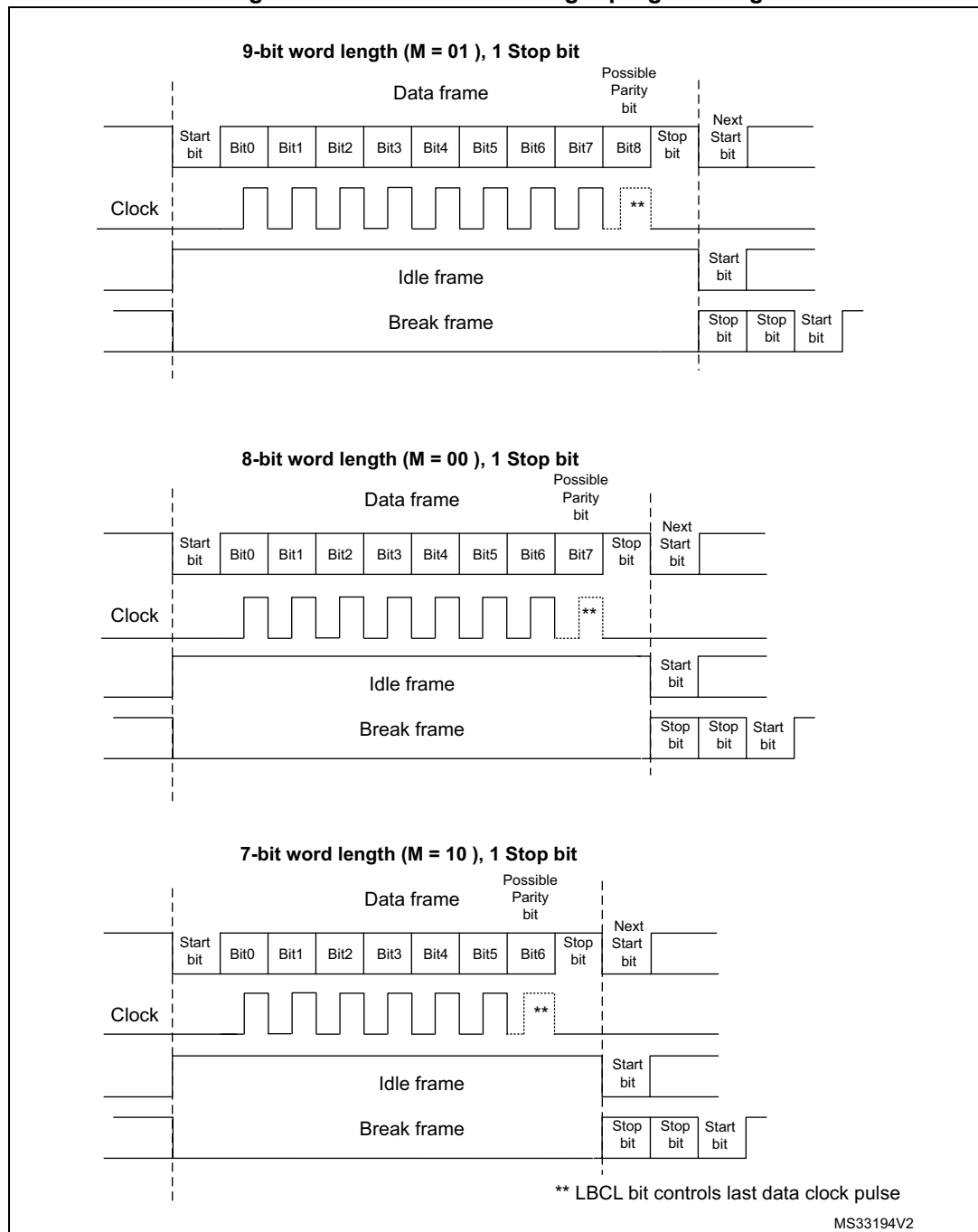
Figure 641. LPUART word length programming
