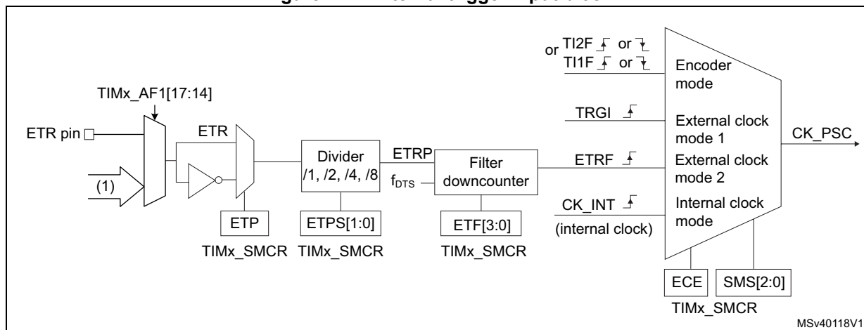
Figure 412. External trigger input block
