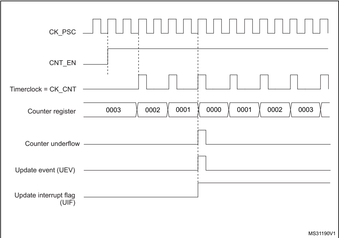
Figure 461. Counter timing diagram, internal clock divided by 2
