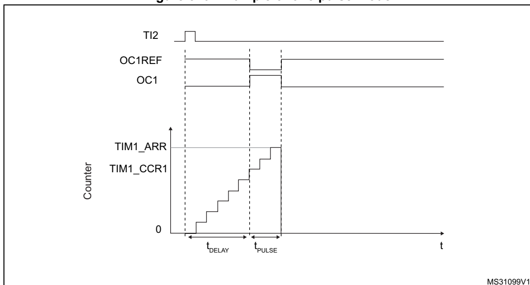
Figure 516. Example of one pulse mode.
