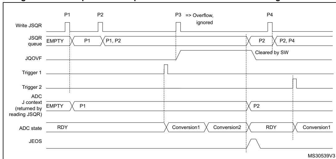
Figure 158. Example of JSQR queue of context with overflow during conversion
