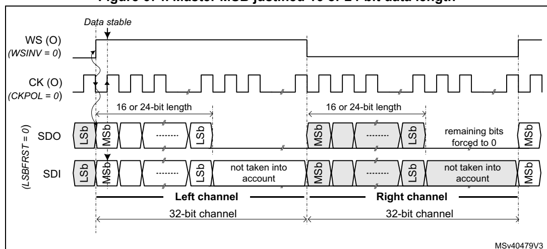
Figure 674. Master MSB justified 16 or 24-bit data length
