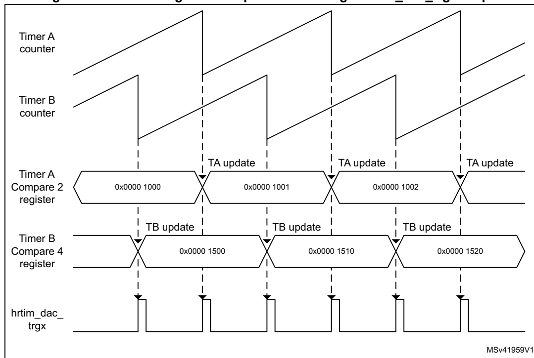
Figure 374. Combining several updates on a single hrtim_dac_trgx output
