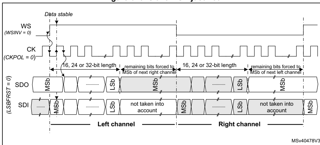
Figure 675. Slave MSB justified
