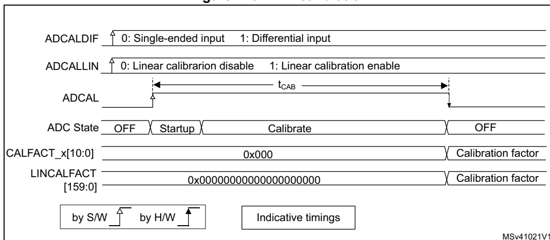
Figure 146. ADC calibration
