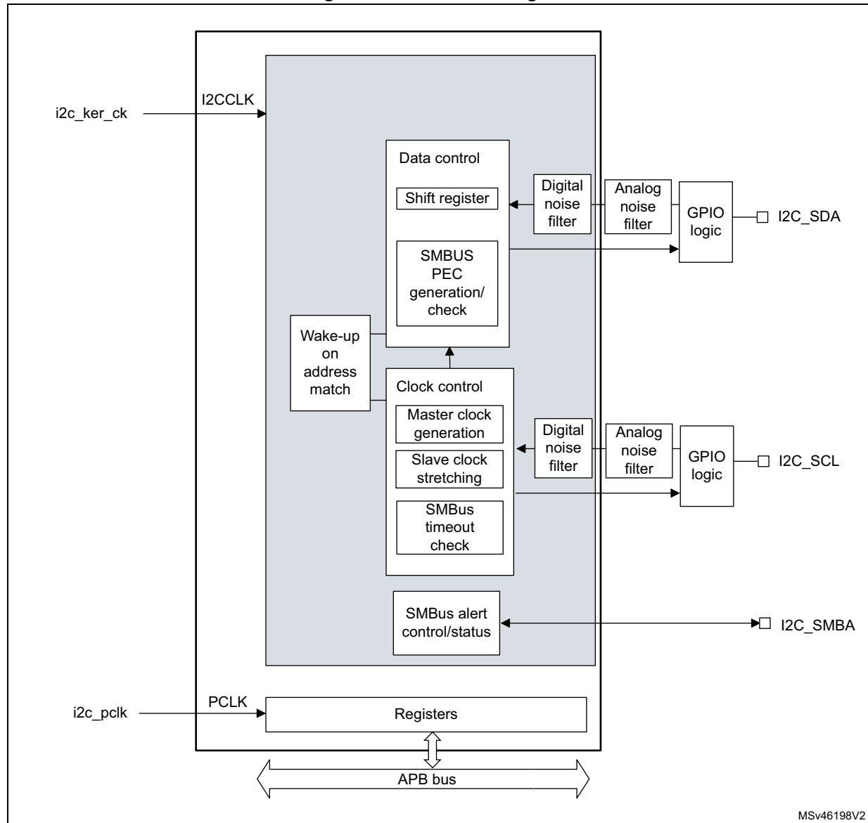
Figure 582. I2C block diagram
