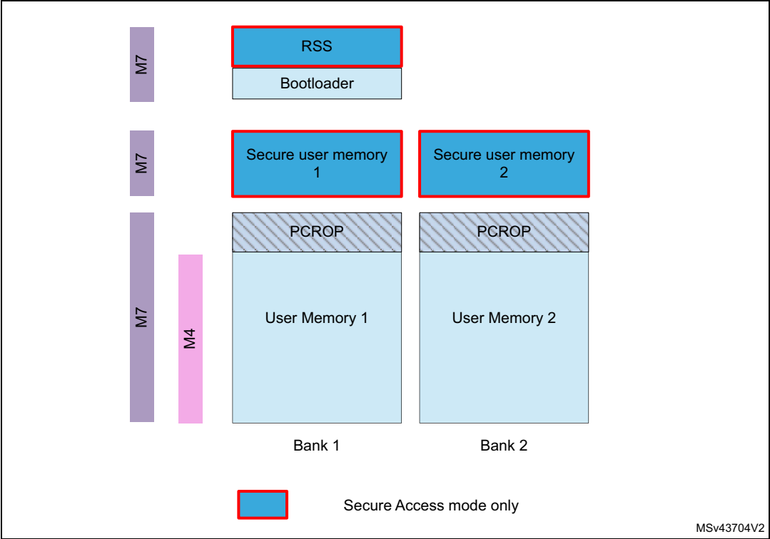
Figure 17. Core access to flash memory areas
