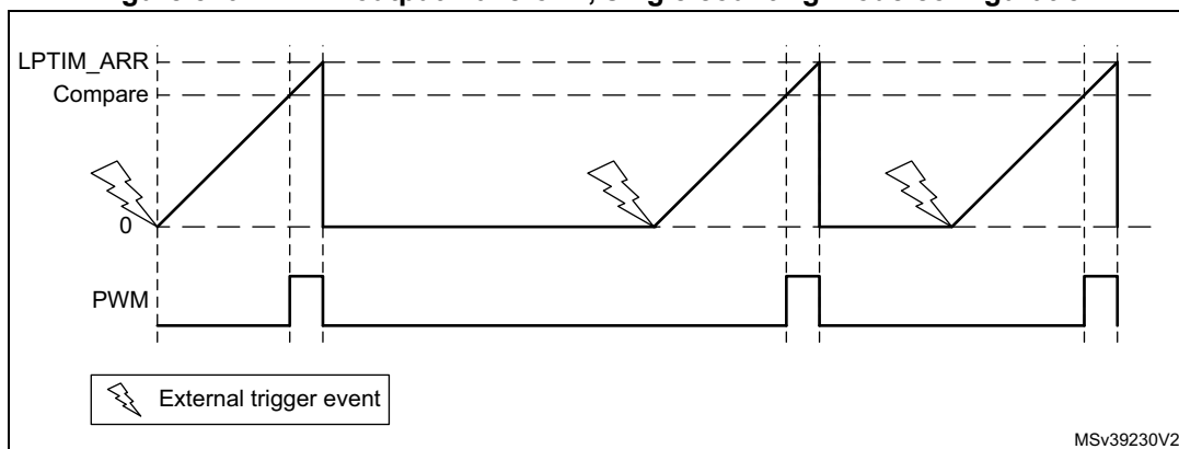
Figure 570. LPTIM output waveform, single counting mode configuration
