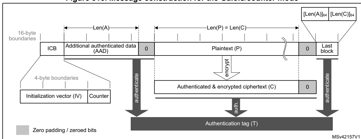
Figure 315. Message construction for the Galois/counter mode
