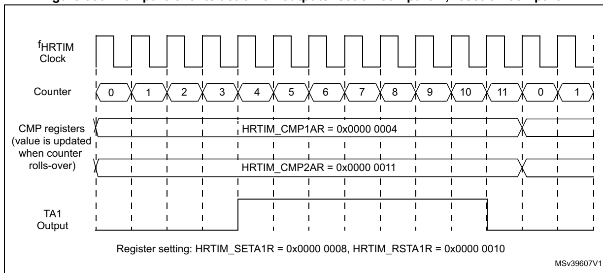
Figure 330. Compare events action on outputs: set on compare 1, reset on compare 2
