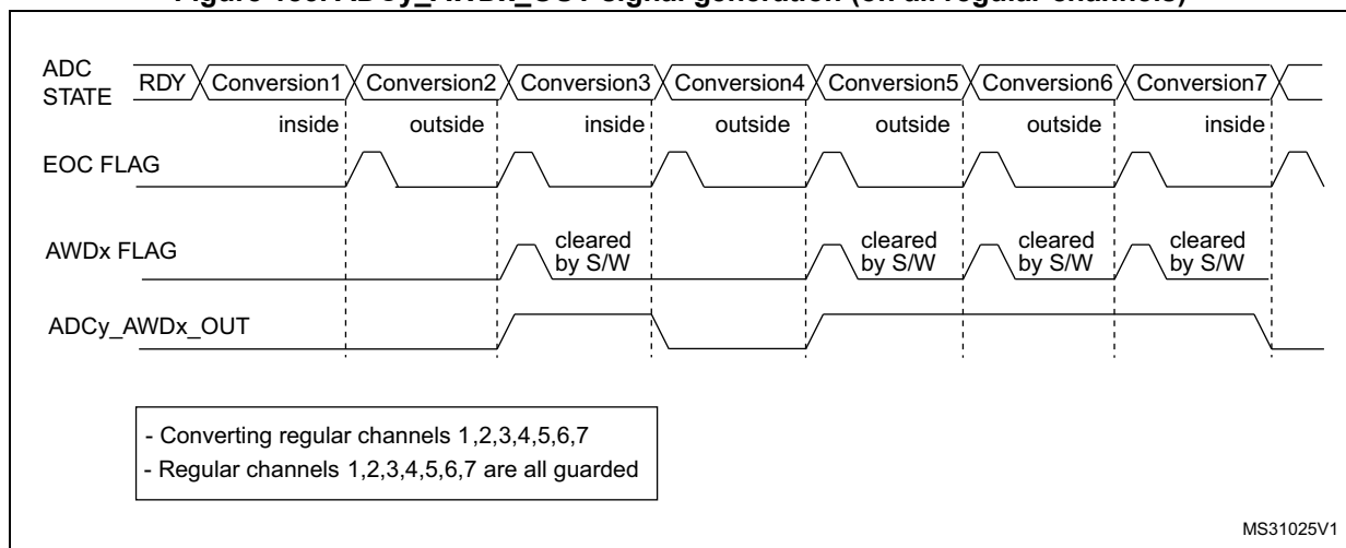
Figure 183. ADCy_AWDx_OUT signal generation (on all regular channels)
