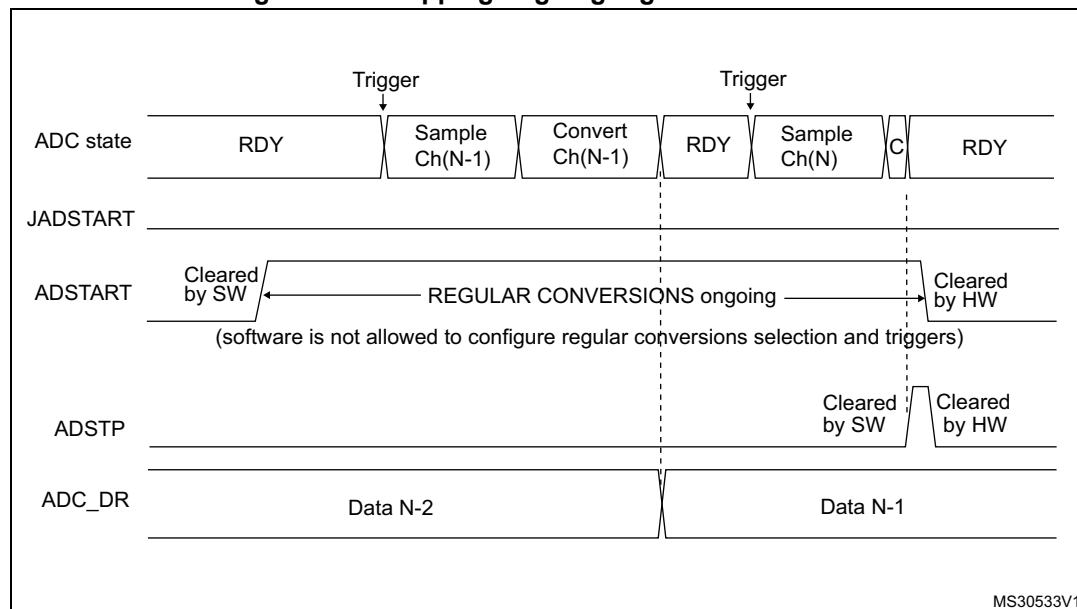
Figure 151. Stopping ongoing regular conversions
