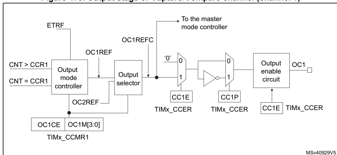
Figure 473. Output stage of Capture/Compare channel (channel 1)
