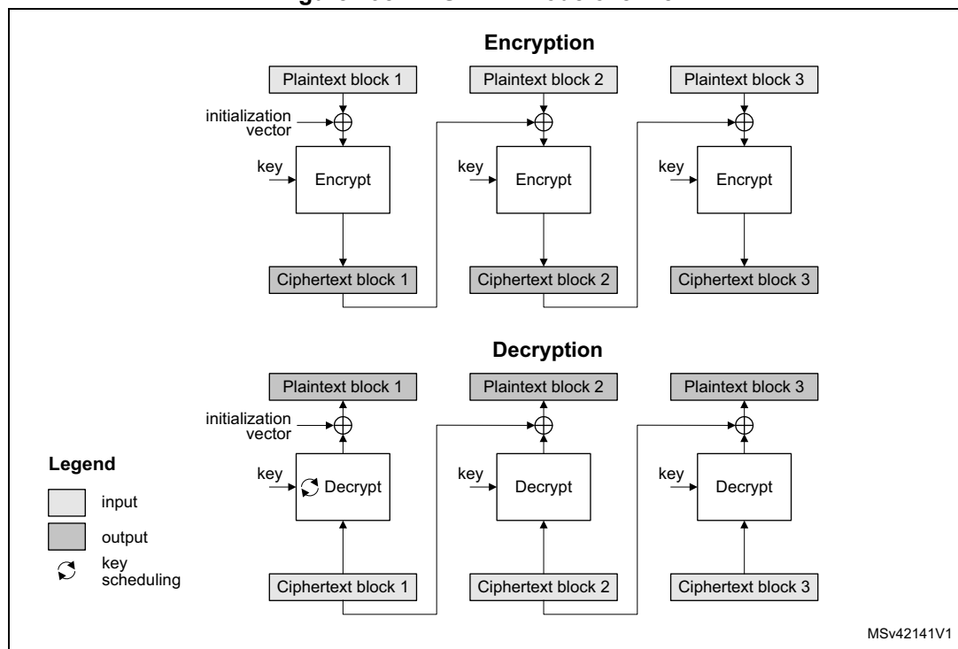
Figure 298. AES-CBC mode overview
