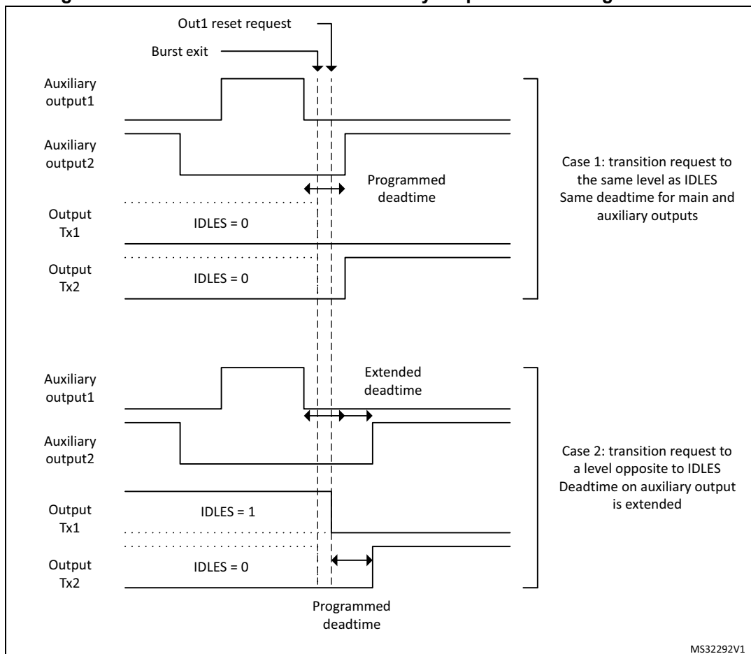
Figure 371. Deadtime distortion on auxiliary output when exiting burst mode
