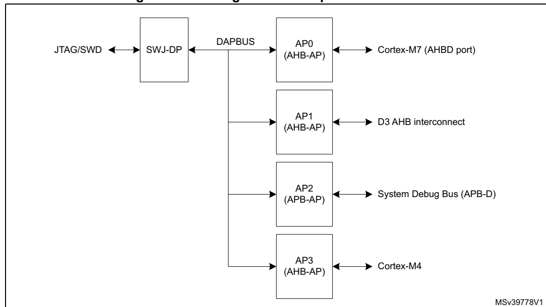
Figure 875. Debug and access port connections
