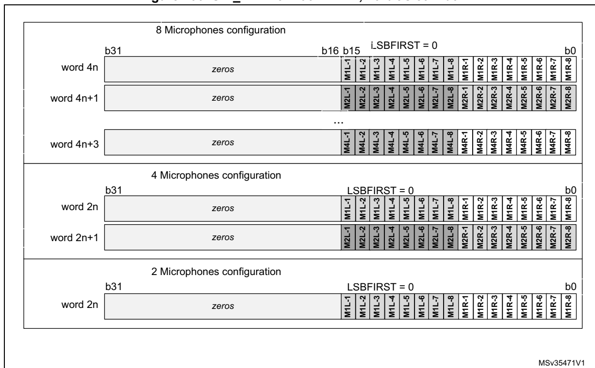
Figure 700. SAI_ADR format in TDM, 16-bit slot width
