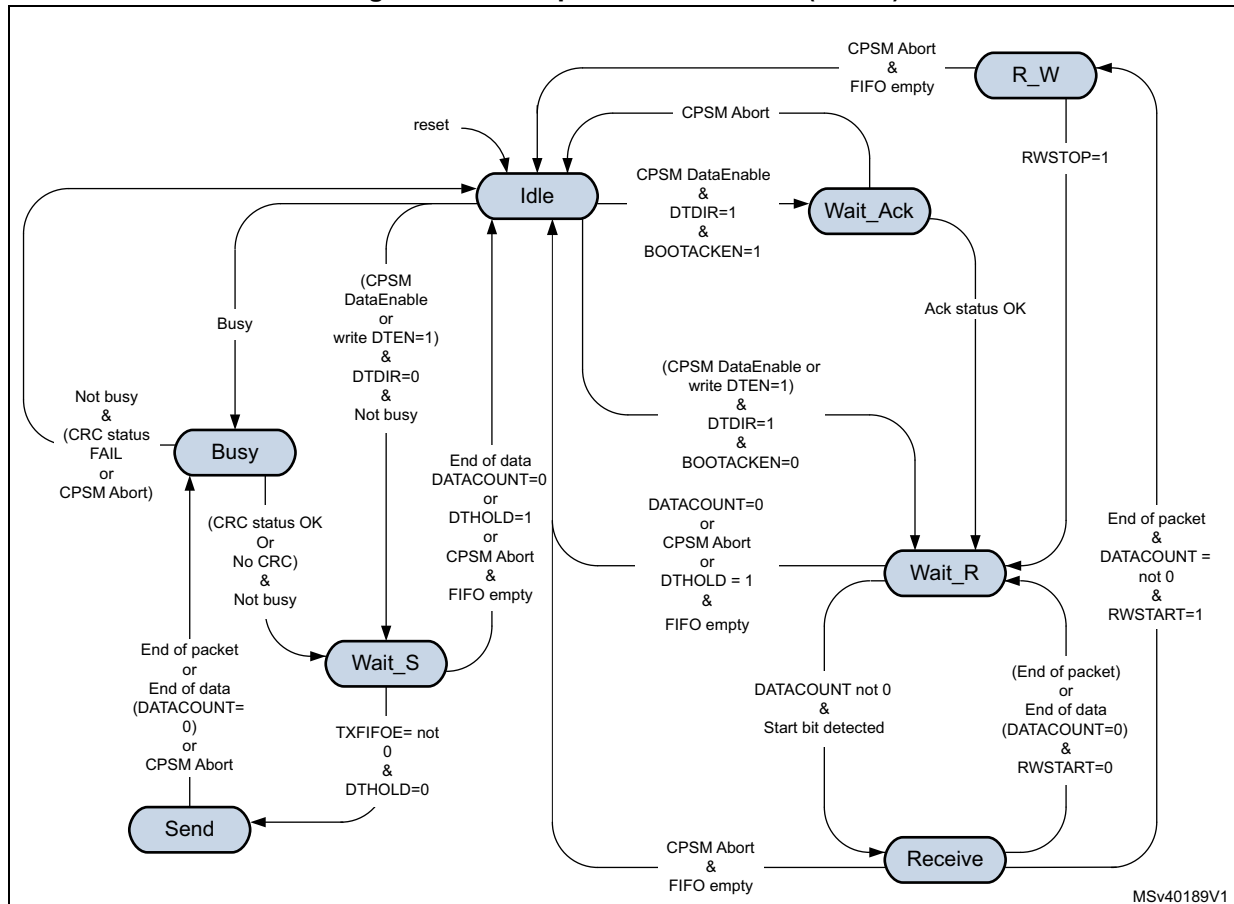
Figure 755. Data path state machine (DPSM)
