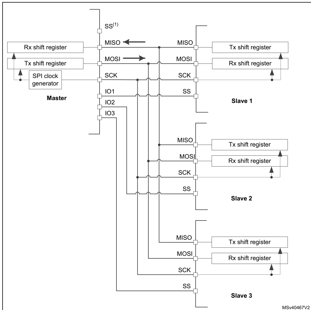
Figure 658. Master and three independent slaves at star topology
