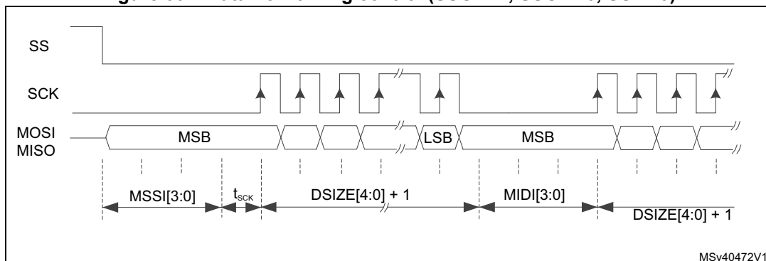
Figure 662. Data flow timing control ( SSOE=1 , SSOM=0 , SSM=0 )
