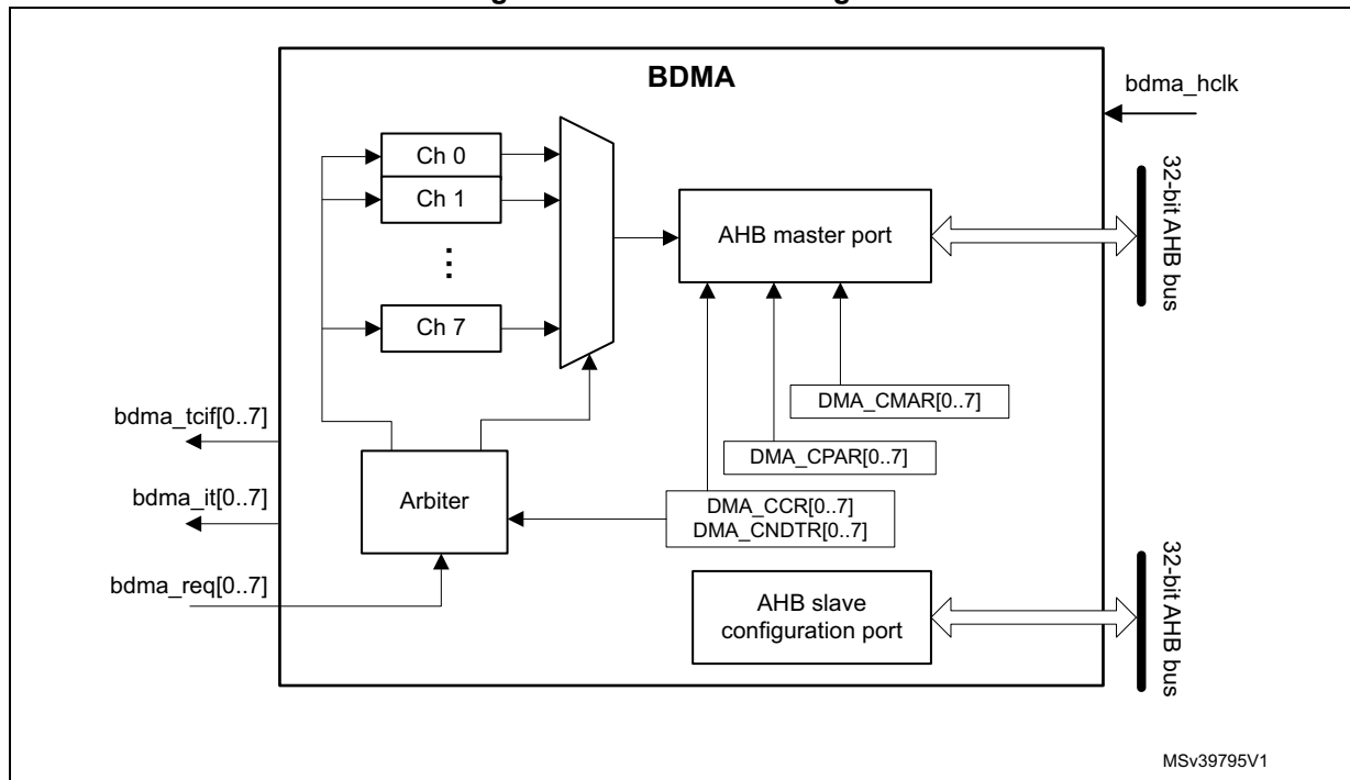
Figure 89. BDMA block diagram
