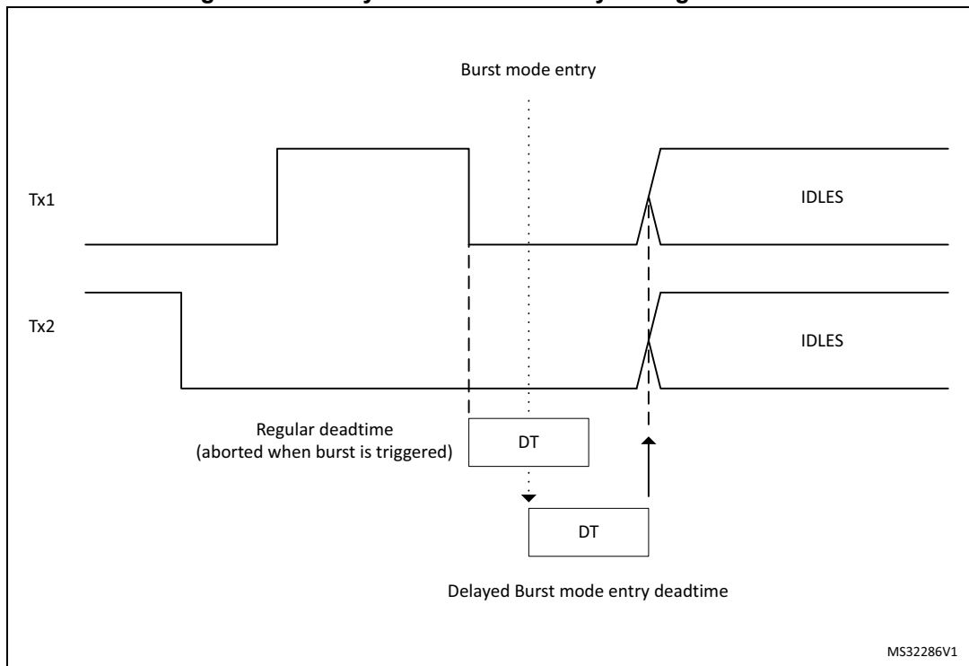
Figure 362. Delayed Burst mode entry during deadtime
