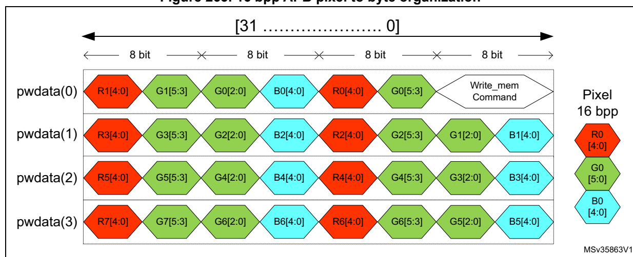
Figure 263. 16 bpp APB pixel to byte organization
