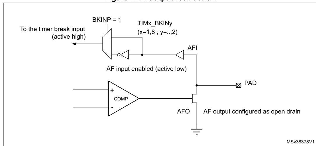
Figure 224. Output redirection
