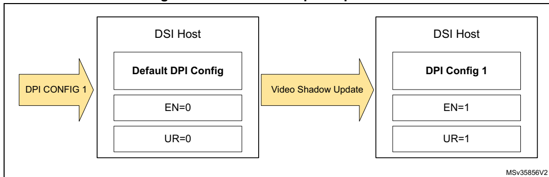
Figure 258. Immediate update procedure
