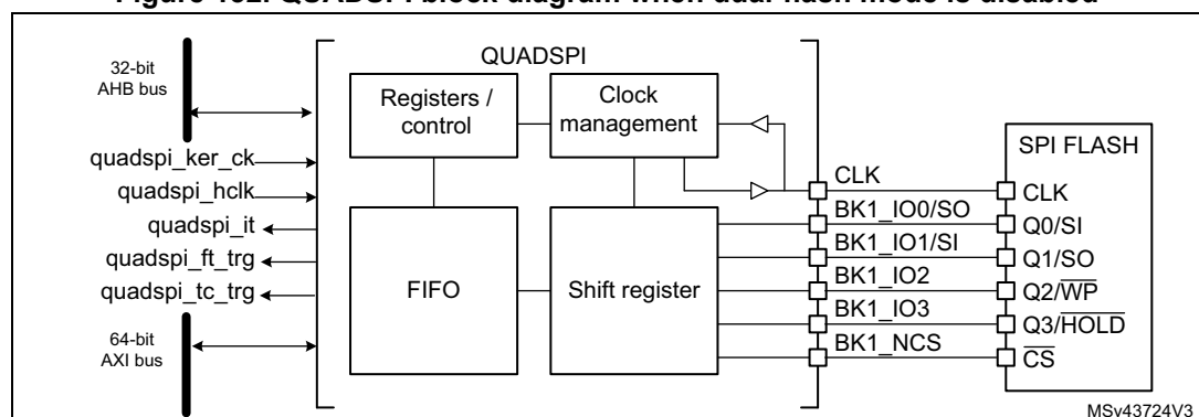
Figure 132. QUADSPI block diagram when dual-flash mode is disabled
