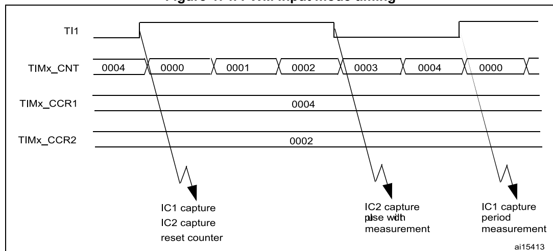
Figure 474. PWM input mode timing
