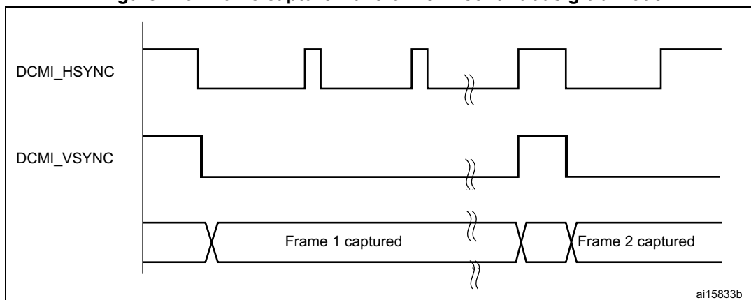
Figure 246. Frame capture waveforms in continuous grab mode
