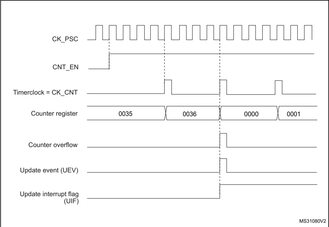
Figure 391. Counter timing diagram, internal clock divided by 4
