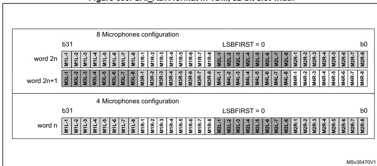
Figure 699. SAI_ADR format in TDM, 32-bit slot width
