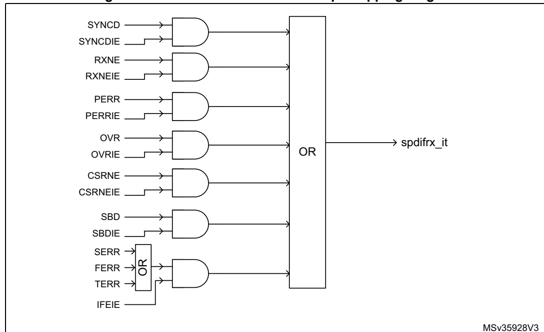
Figure 726. SPDIFRX interface interrupt mapping diagram
