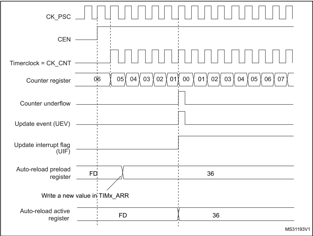
Figure 404. Counter timing diagram, update event with ARPE=1 (counter underflow)
