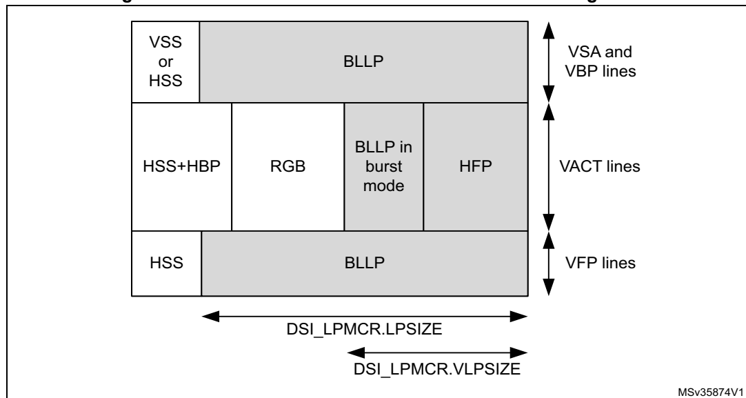
Figure 277. Location of LPSIZE and VLPSIZE in the image area
