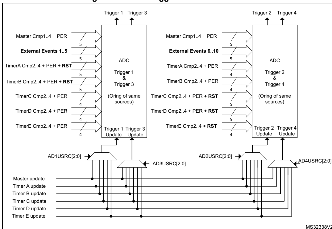
Figure 373. ADC trigger selection overview
