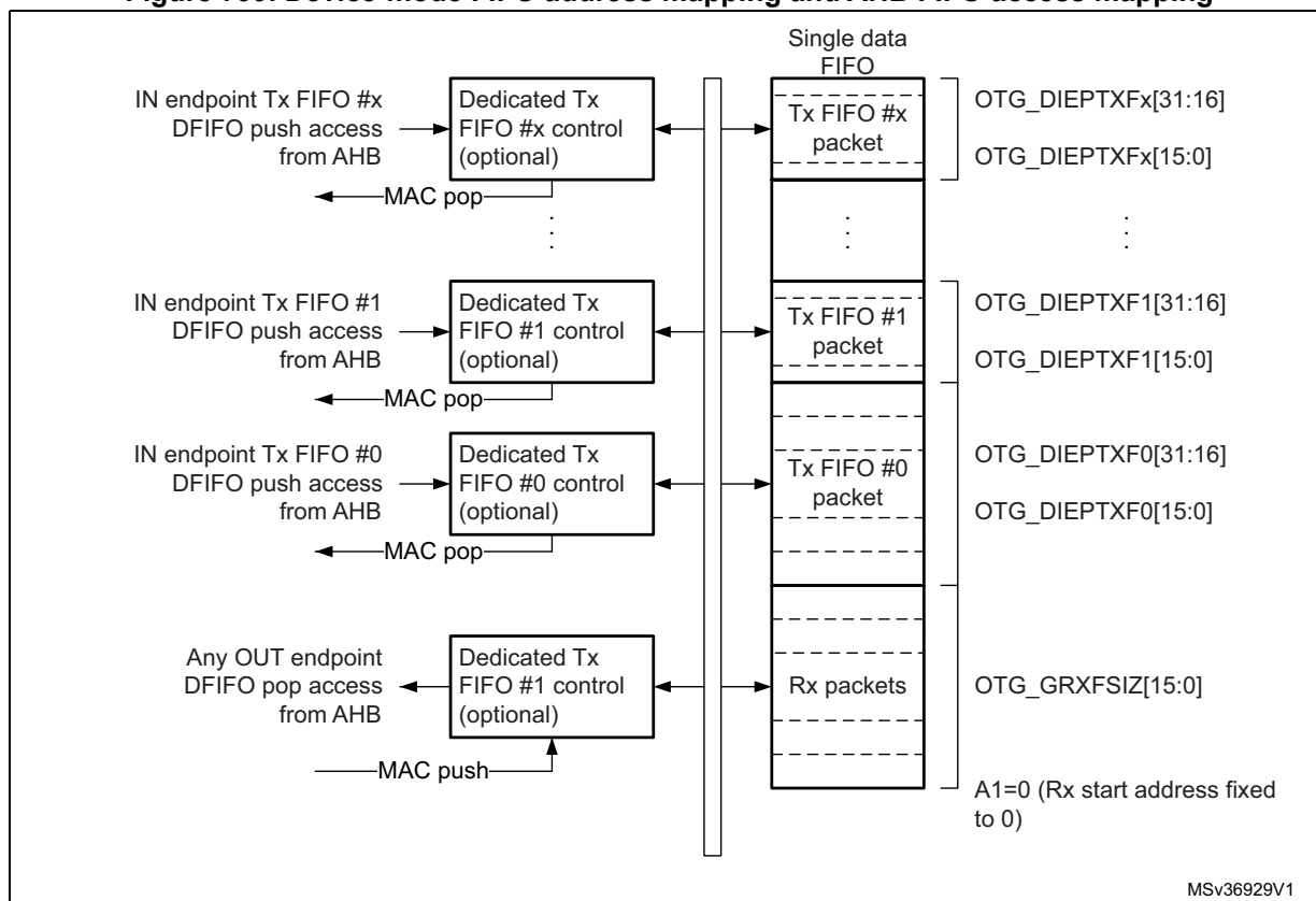
Figure 799. Device-mode FIFO address mapping and AHB FIFO access mapping
