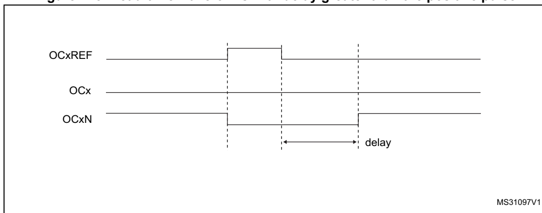
Figure 428. Dead-time waveforms with delay greater than the positive pulse
