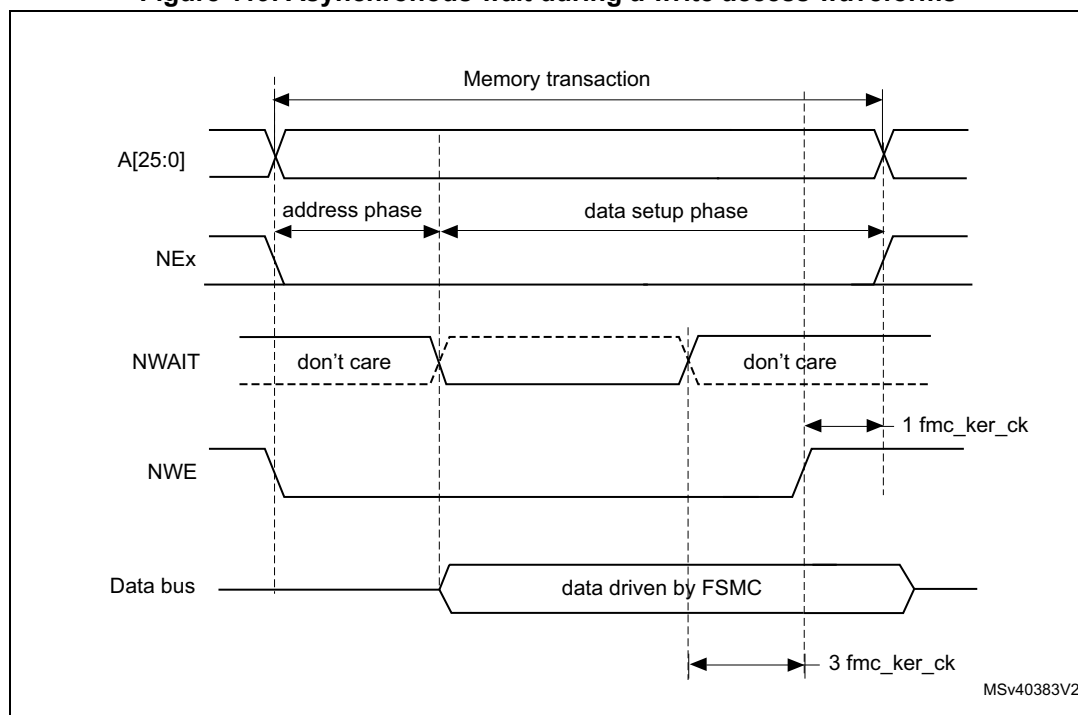
Figure 119. Asynchronous wait during a write access waveforms
