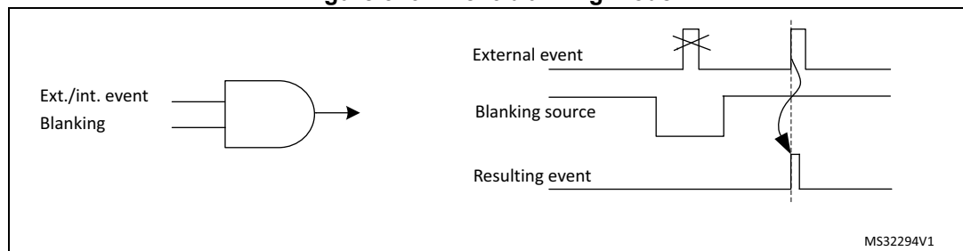
Figure 346. Event blanking mode
