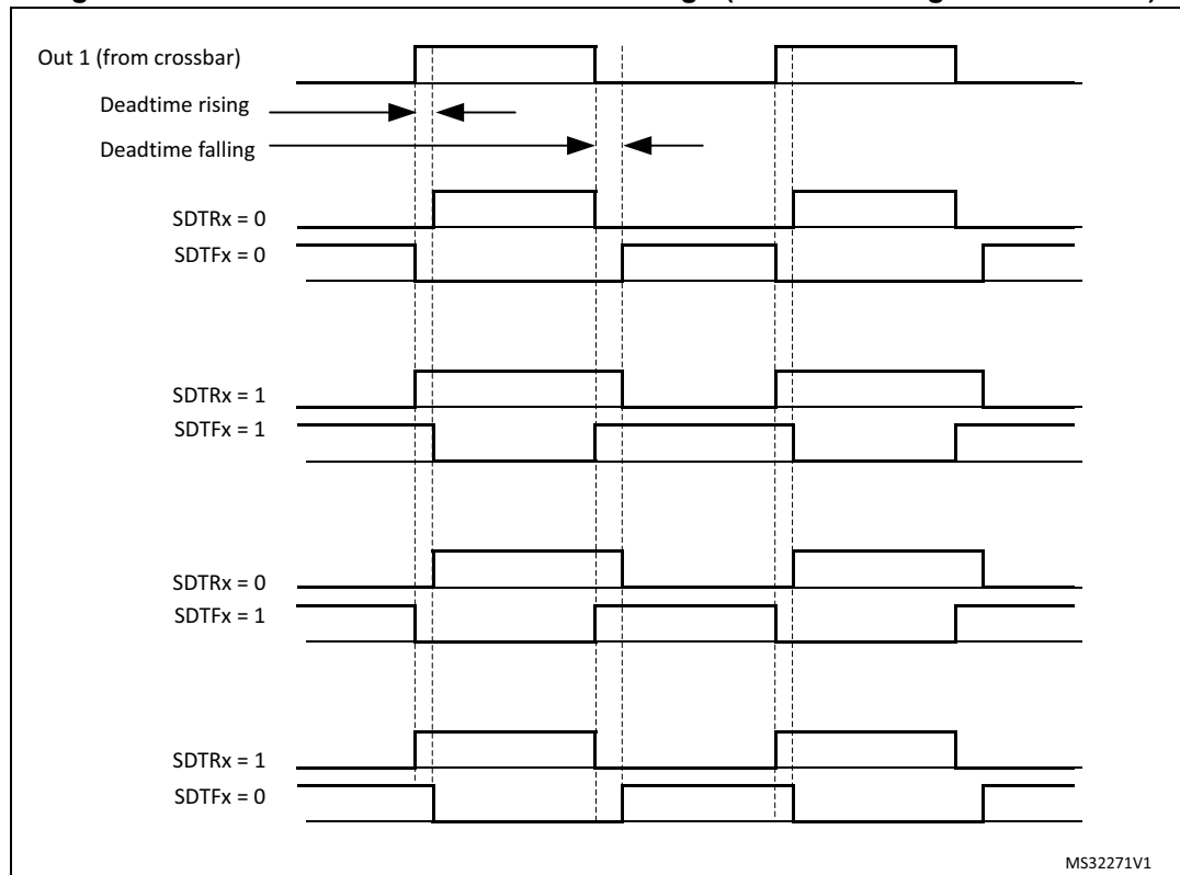
Figure 337. Deadtime insertion vs deadtime sign (1 indicates negative deadtime)
