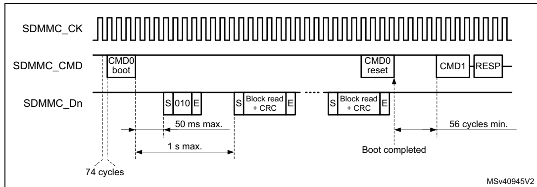
Figure 769. Alternative boot mode operation
