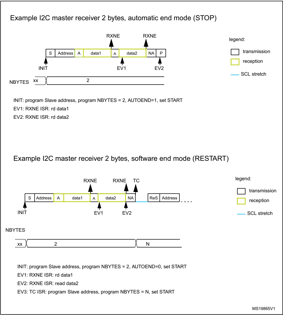
Figure 604. Transfer bus diagrams for I2C master receiver (mandatory events only)
