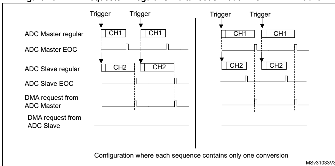
Figure 207. DMA requests in regular simultaneous mode when DAMDF=0b10
