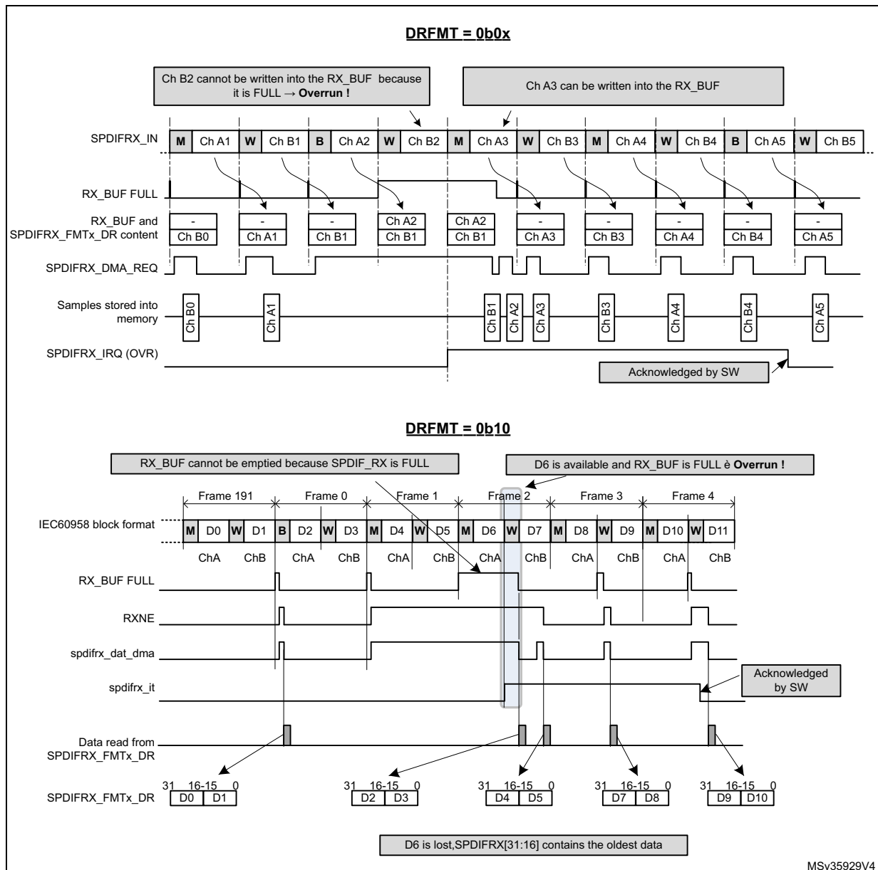
Figure 724. S/PDIF overrun error when RXSTEO = 0
