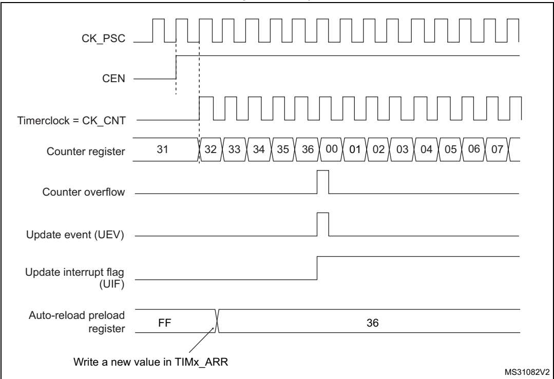
Figure 563. Counter timing diagram, update event when ARPE = 0 (TIMx_ARR not preloaded)
