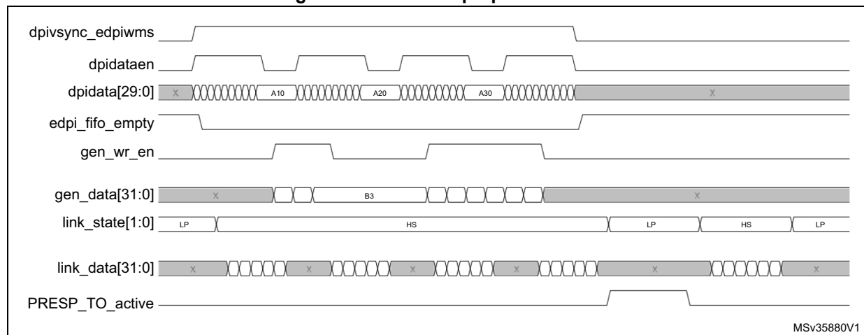
Figure 269. Effect of prep mode at 1
