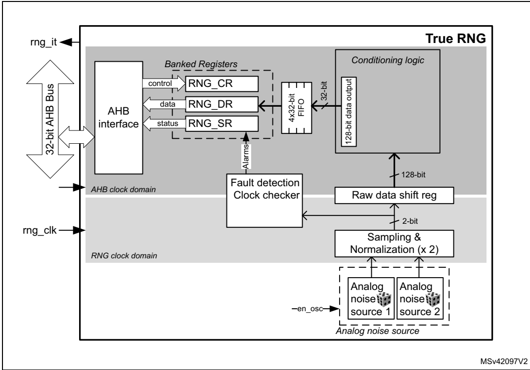
Figure 293. RNG block diagram
