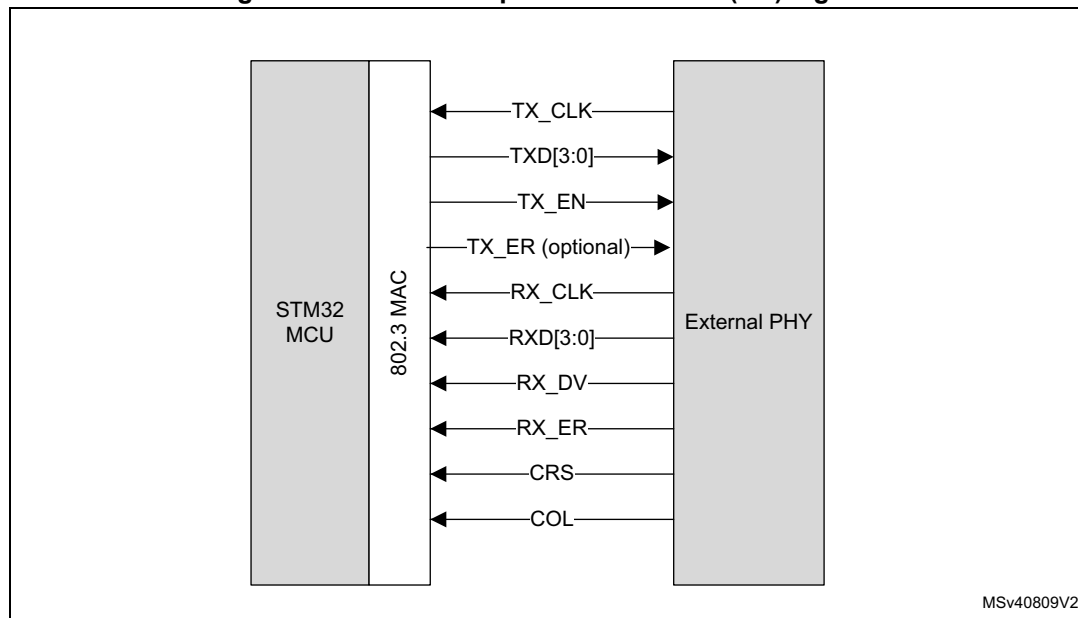
Figure 844. Media independent interface (MII) signals
