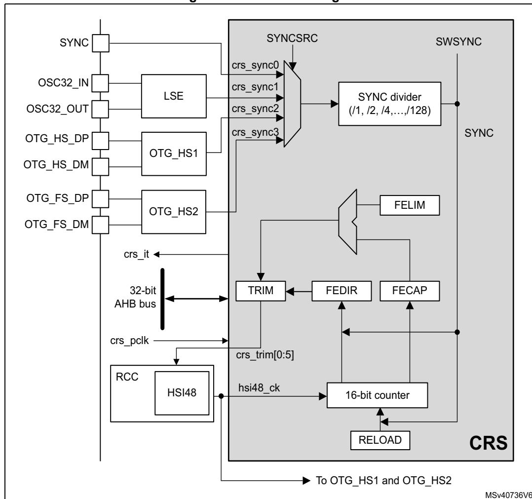
Figure 71. CRS block diagram
