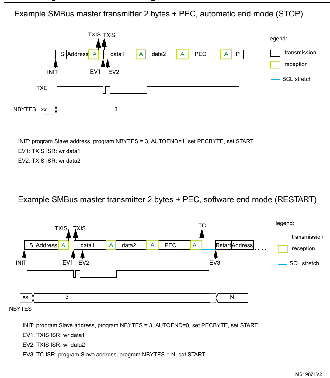
Figure 610. Bus transfer diagrams for SMBus master transmitter
