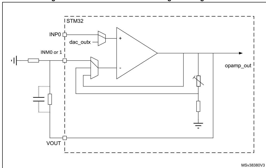
Figure 226. Standalone mode: external gain setting mode
