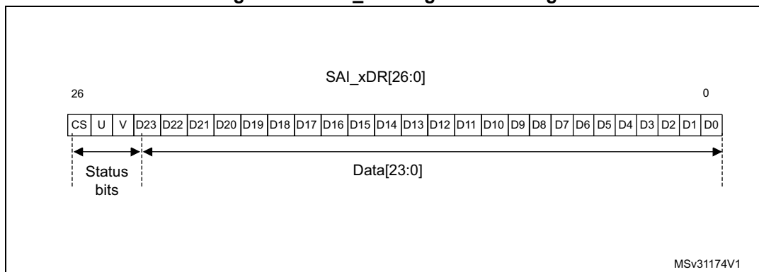
Figure 705. SAI_xDR register ordering
