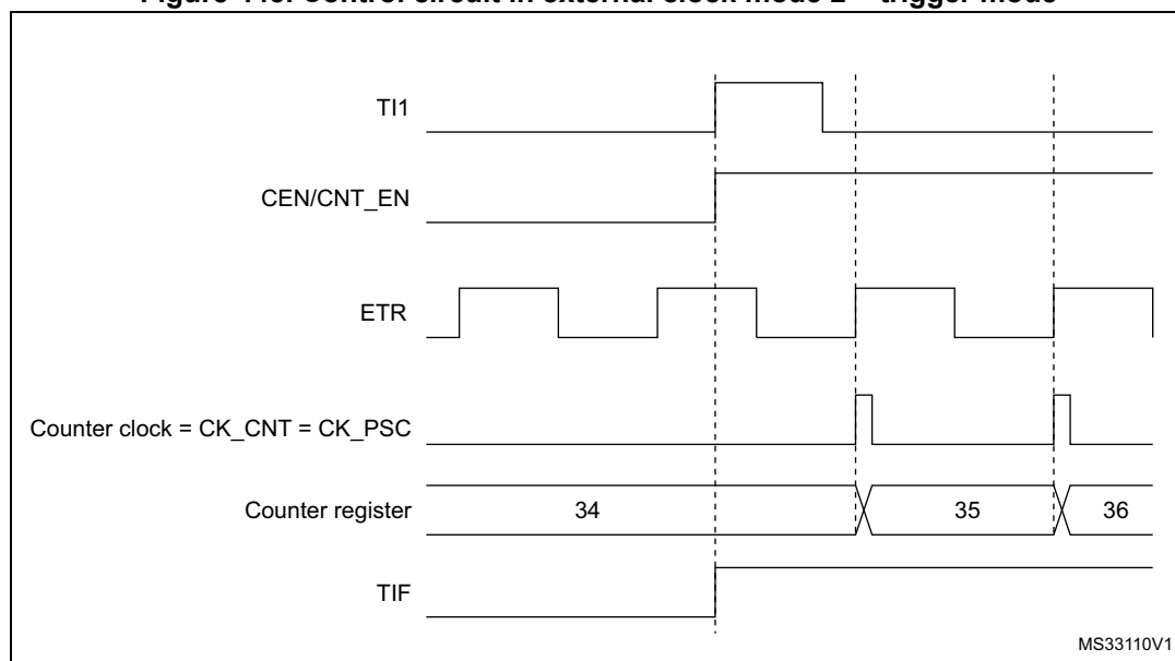
Figure 445. Control circuit in external clock mode 2 + trigger mode
