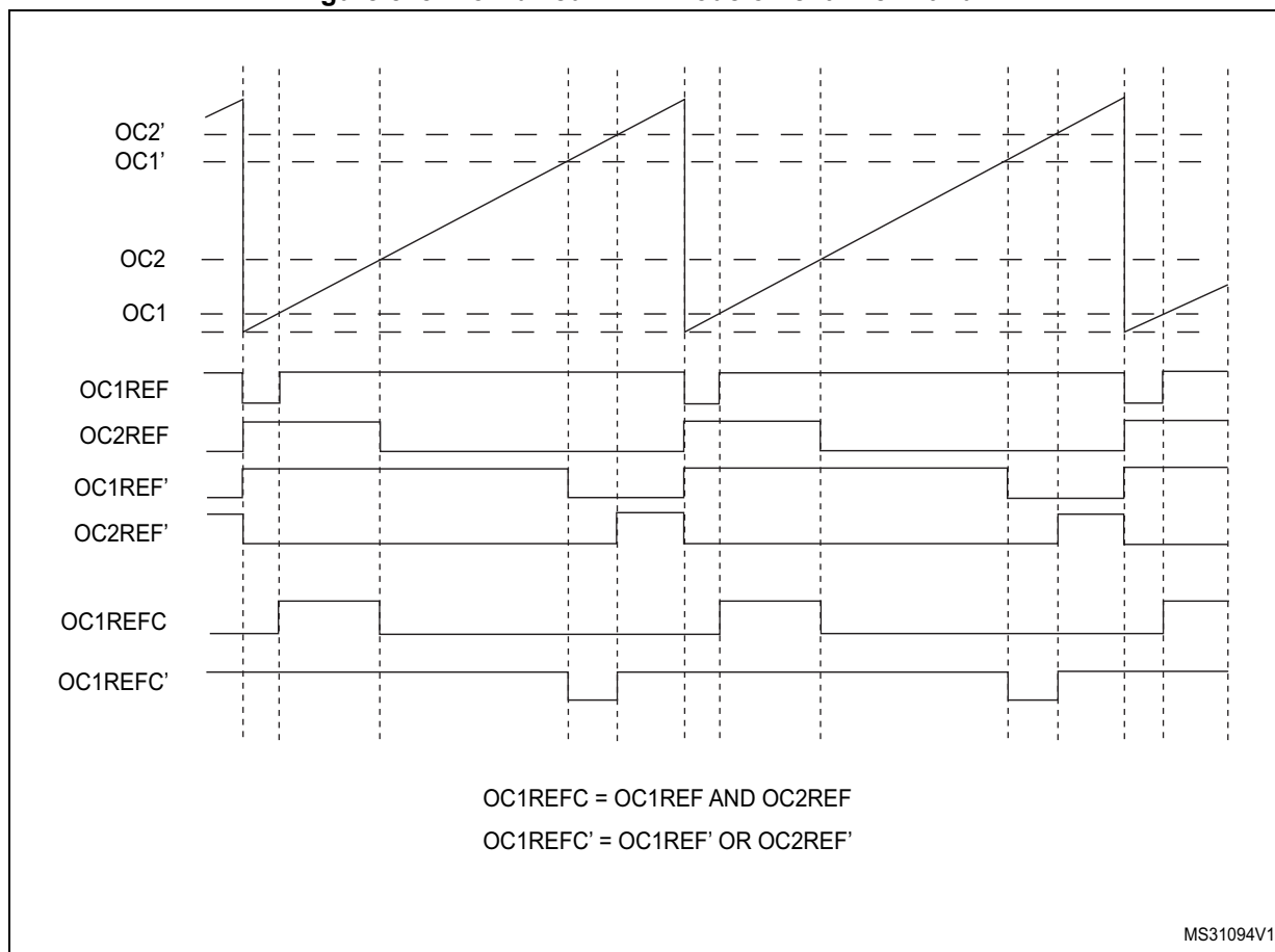
Figure 515. Combined PWM mode on channel 1 and 2
