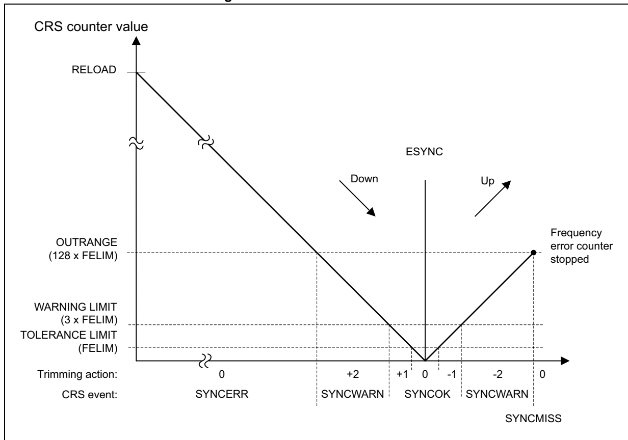
Figure 72. CRS counter behavior
