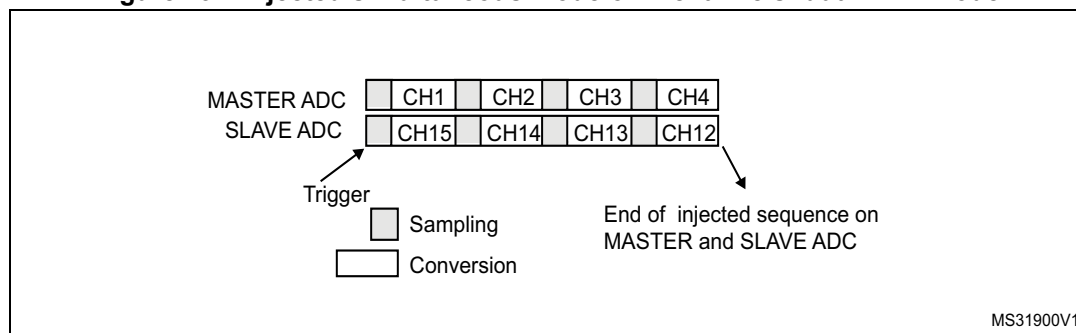
Figure 194. Injected simultaneous mode on 4 channels: dual ADC mode
