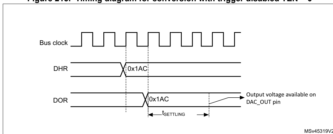
Figure 215. Timing diagram for conversion with trigger disabled TEN = 0
