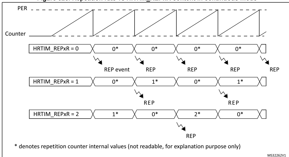
Figure 328. Repetition rate vs HRTIM_REPxR content in continuous mode
