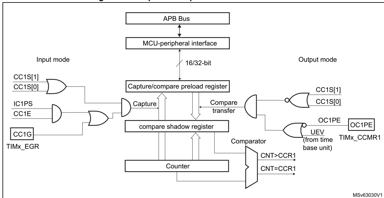
Figure 472. Capture/Compare channel 1 main circuit
