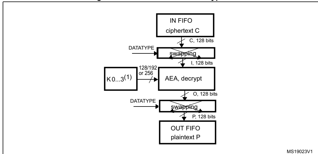
Figure 309. AES-ECB mode decryption
