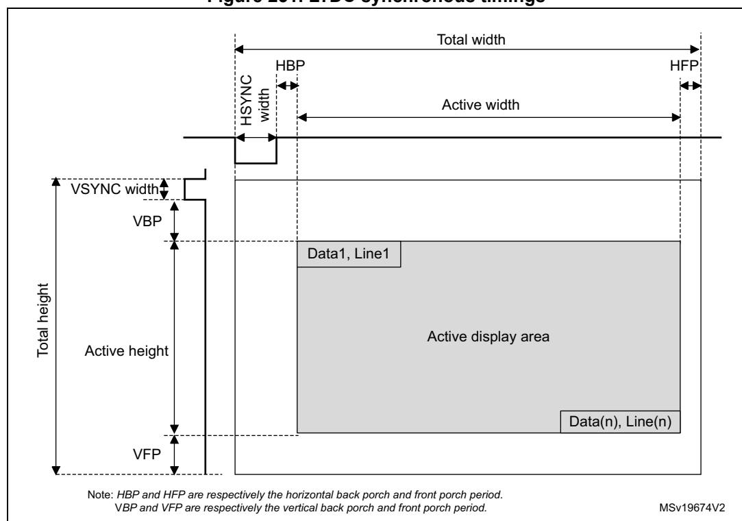
Figure 251. LTDC synchronous timings
