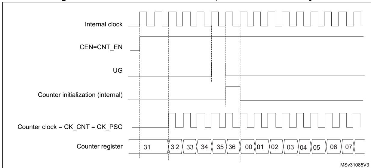
Figure 409. Control circuit in normal mode, internal clock divided by 1
