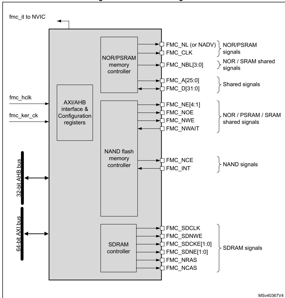
Figure 103. FMC block diagram
