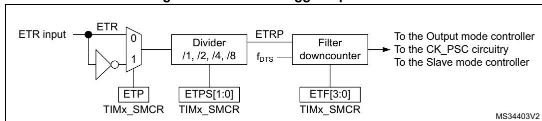
Figure 407. External trigger input block
