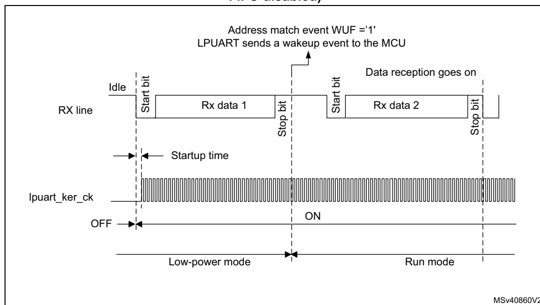
Figure 652. Wake-up event verified (wake-up event = address match, FIFO disabled)
