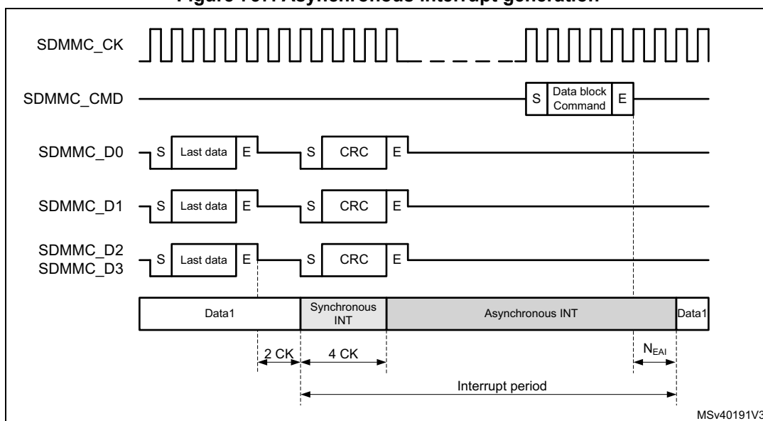
Figure 757. Asynchronous interrupt generation
