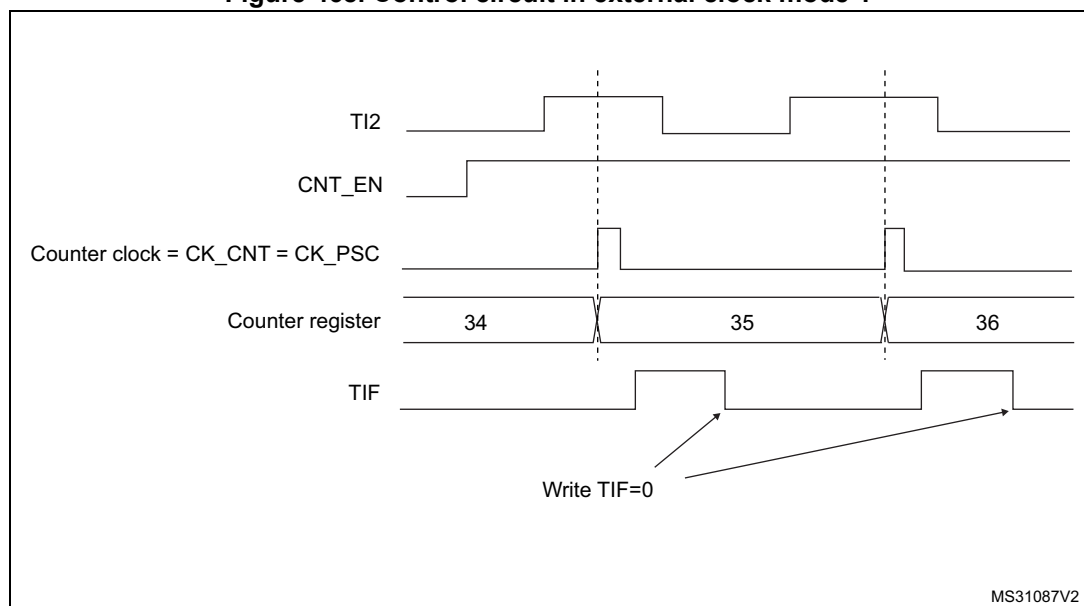
Figure 468. Control circuit in external clock mode 1
