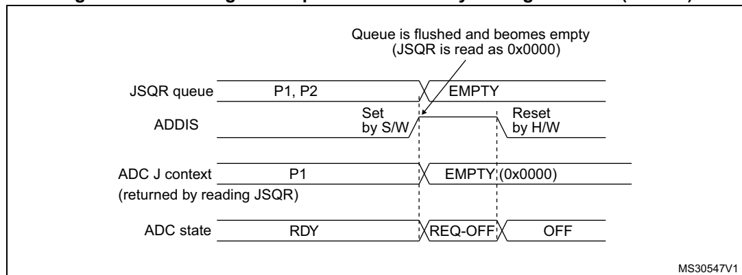
Figure 166. Flushing JSQR queue of context by setting ADDIS=1 (JQM=1)
