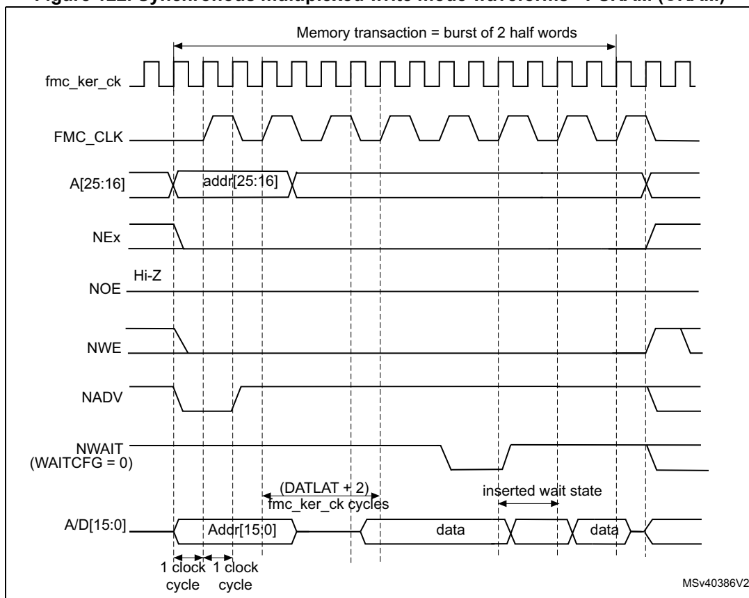
Figure 122. Synchronous multiplexed write mode waveforms - PSRAM (CRAM)
