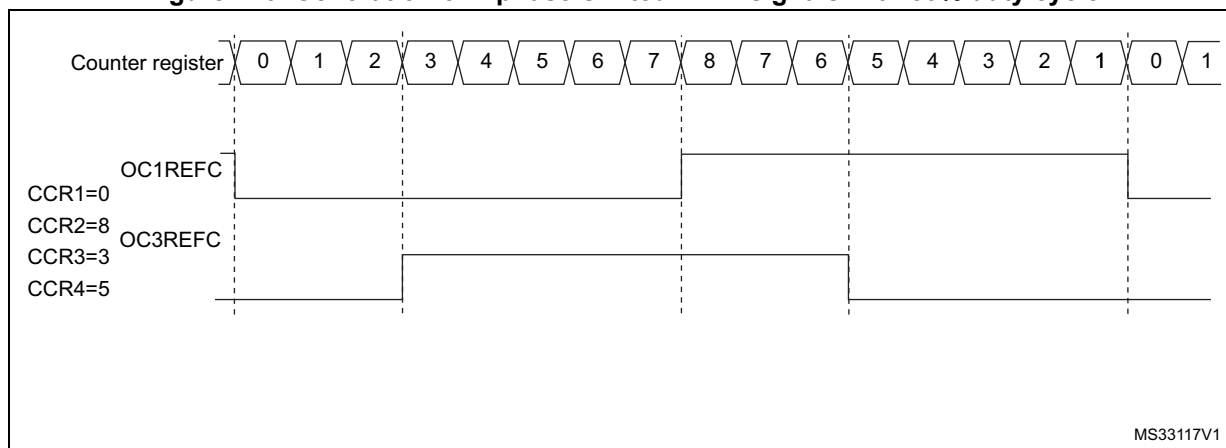
Figure 423. Generation of 2 phase-shifted PWM signals with 50% duty cycle
