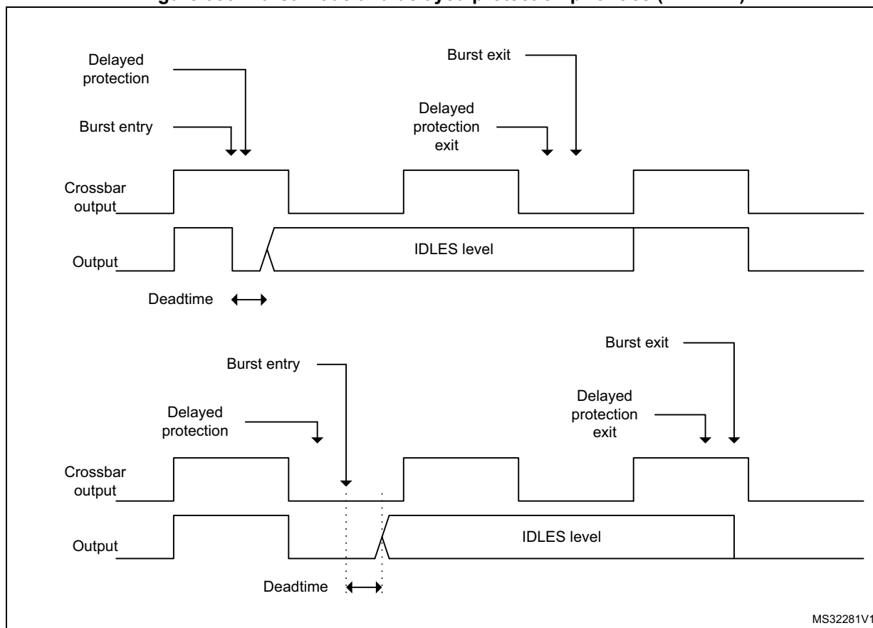
Figure 355. Burst mode and delayed protection priorities (DIDL = 1)
