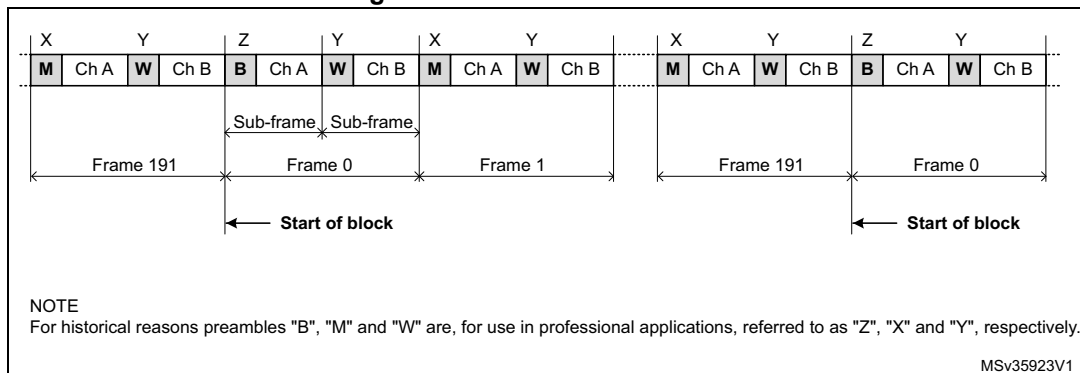
Figure 713. S/PDIF block format
