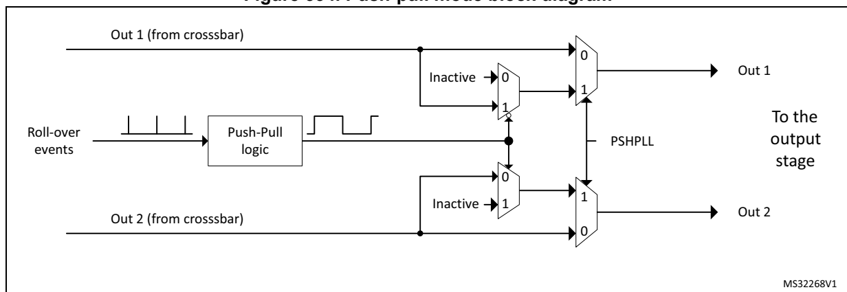
Figure 334. Push-pull mode block diagram
