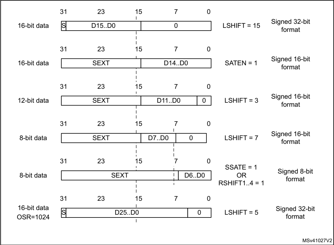
Figure 174. Left alignment (offset enabled, signed value)
