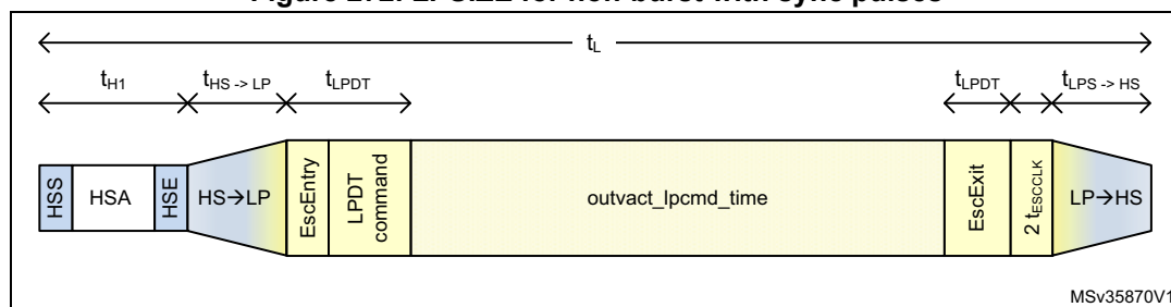
Figure 272. LPSIZE for non-burst with sync pulses
