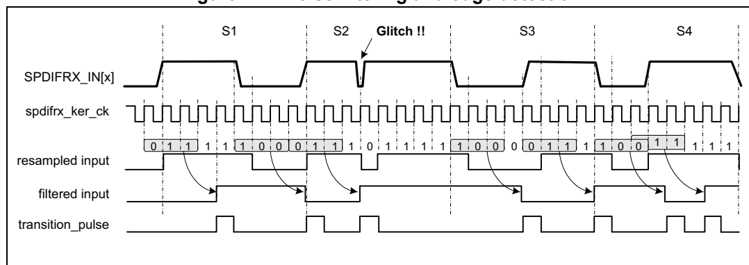
Figure 717. Noise filtering and edge detection
