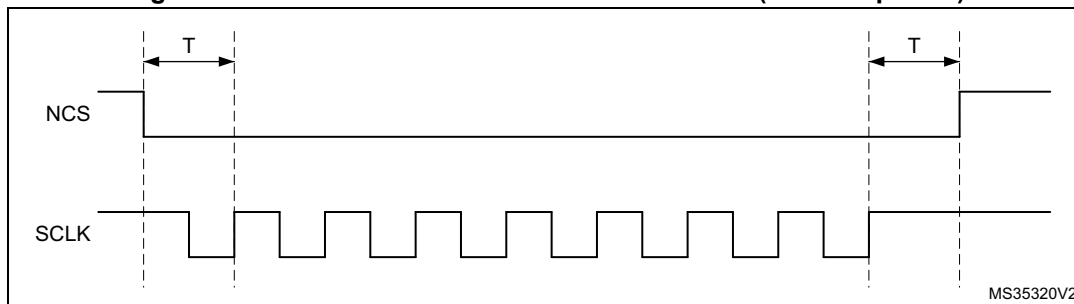
Figure 137. NCS when CKMODE = 1 in SDR mode ( T = \text{CLK period} )
