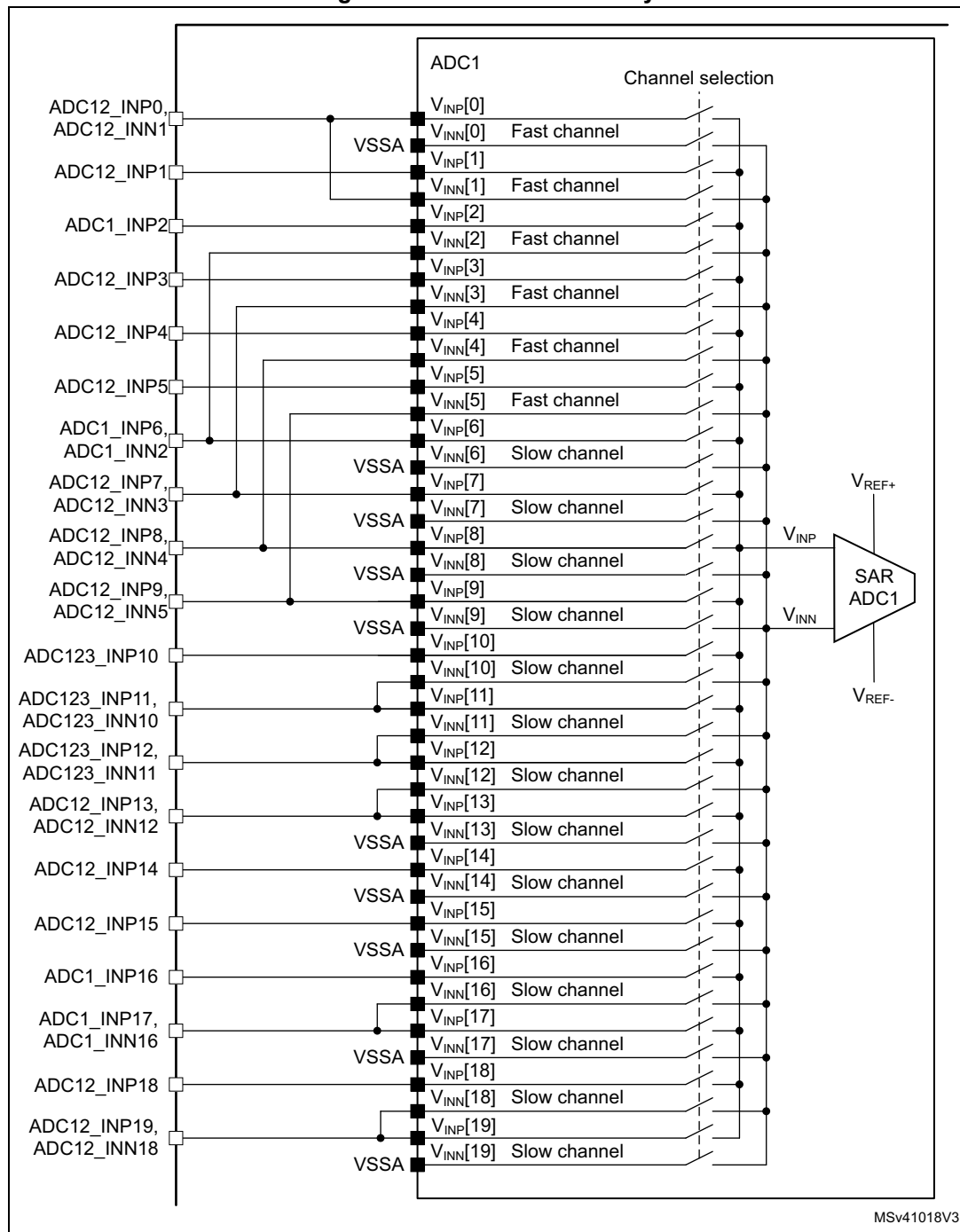
Figure 143. ADC1 connectivity
