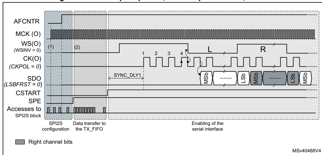
Figure 680. Startup sequence, I2S Philips standard, master
