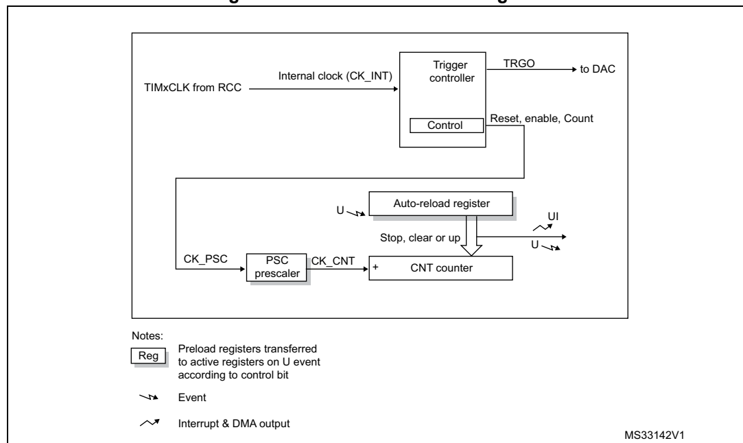
Figure 556. Basic timer block diagram
