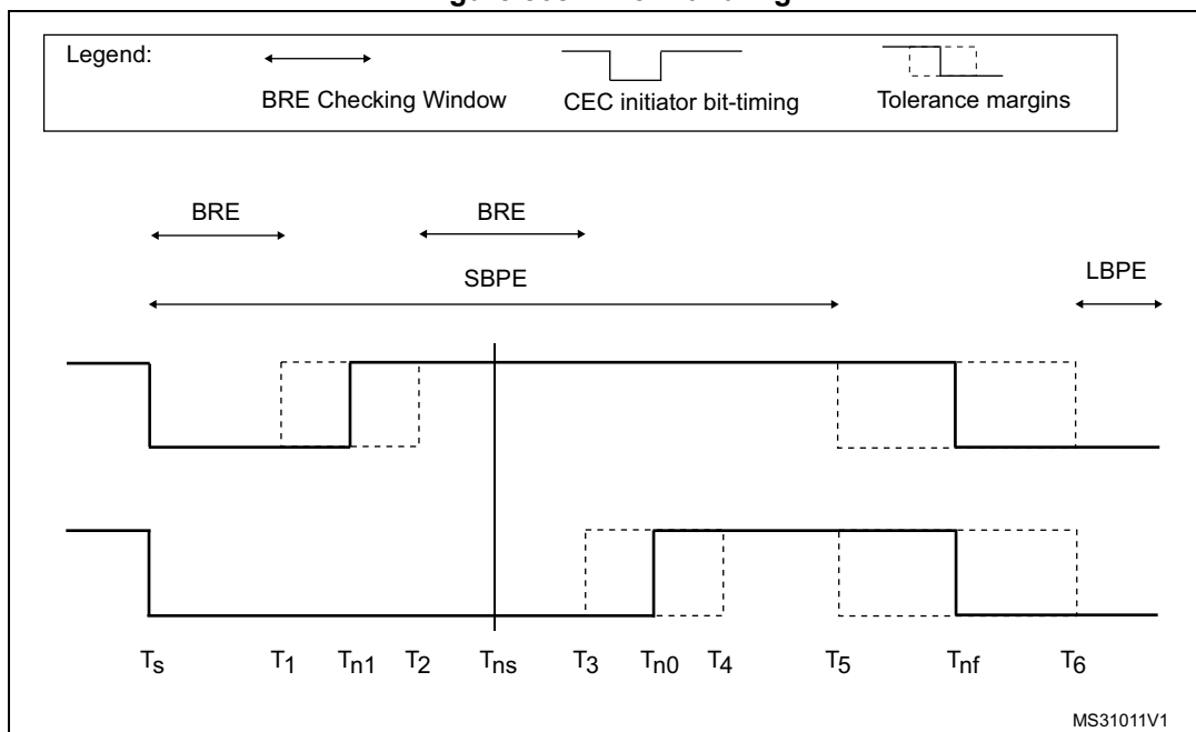
Figure 868. Error handling
