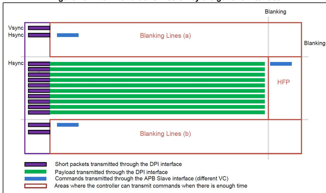
Figure 281. Command transmission by the generic interface
