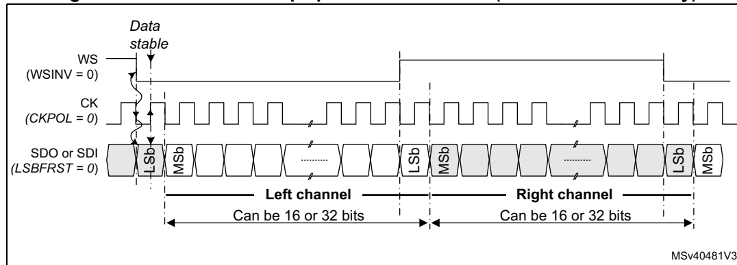
Figure 671. Master I2S Philips protocol waveforms (16/32-bit full accuracy)
