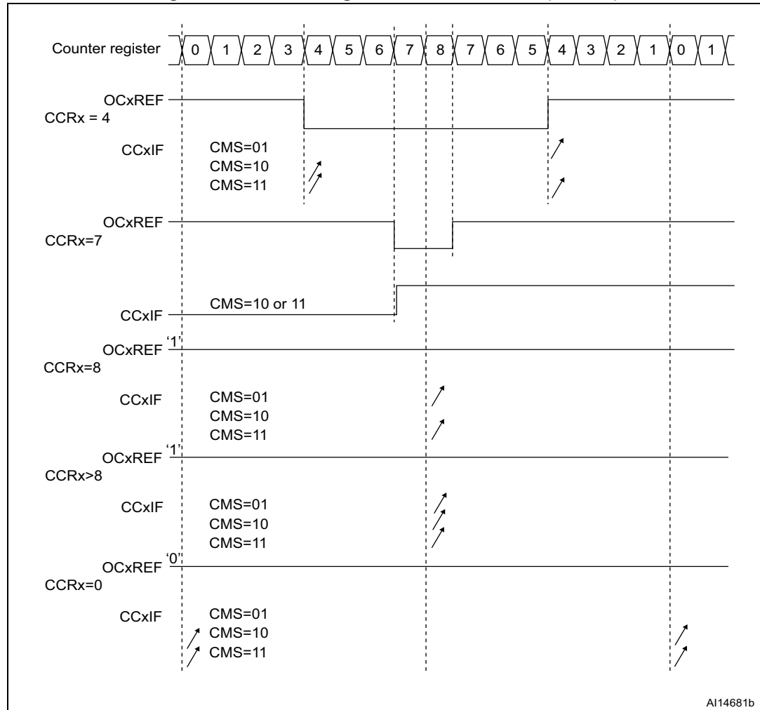
Figure 422. Center-aligned PWM waveforms (ARR=8)
