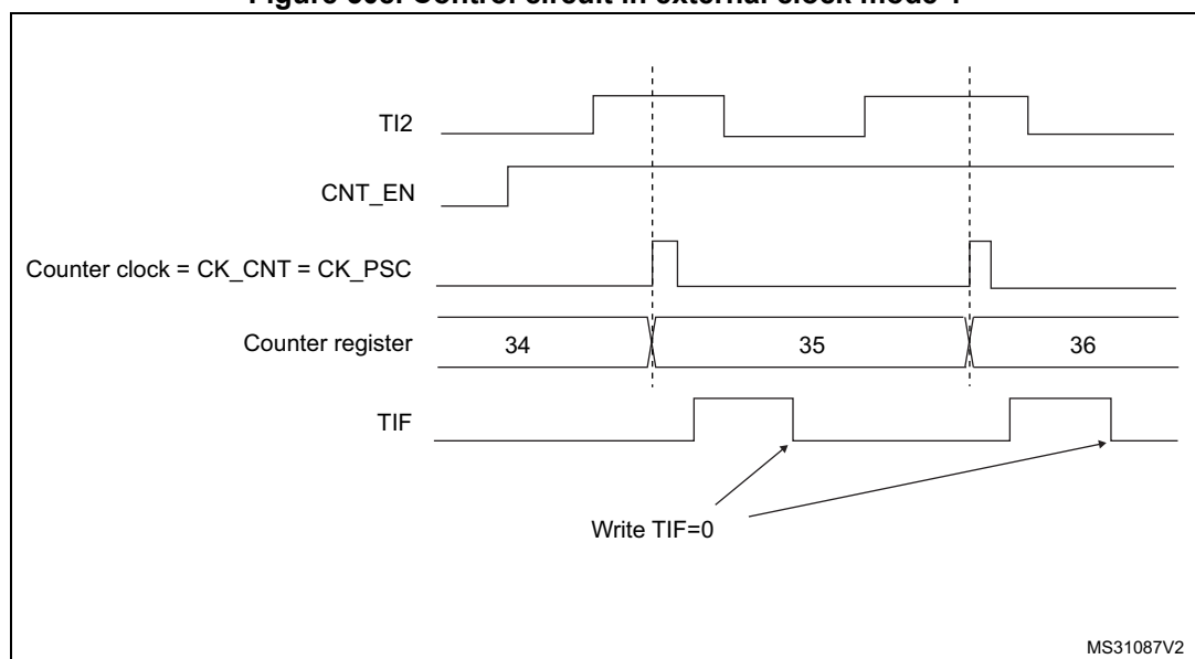
Figure 508. Control circuit in external clock mode 1
