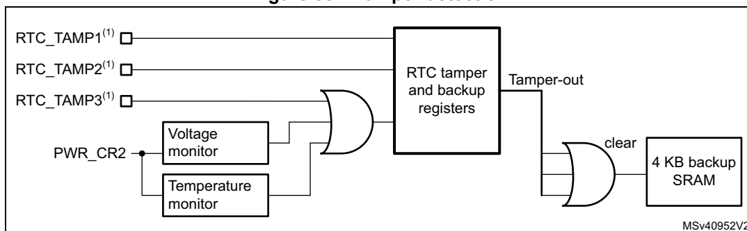
Figure 581. Tamper detection
