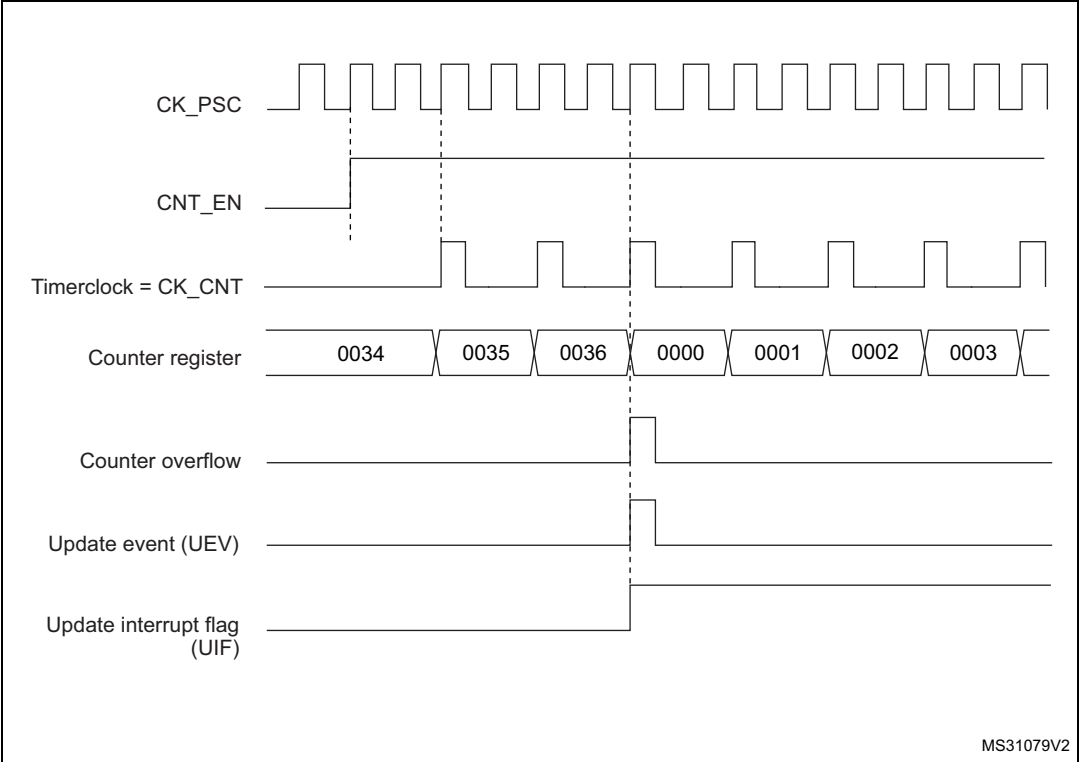
Figure 450. Counter timing diagram, internal clock divided by 2
