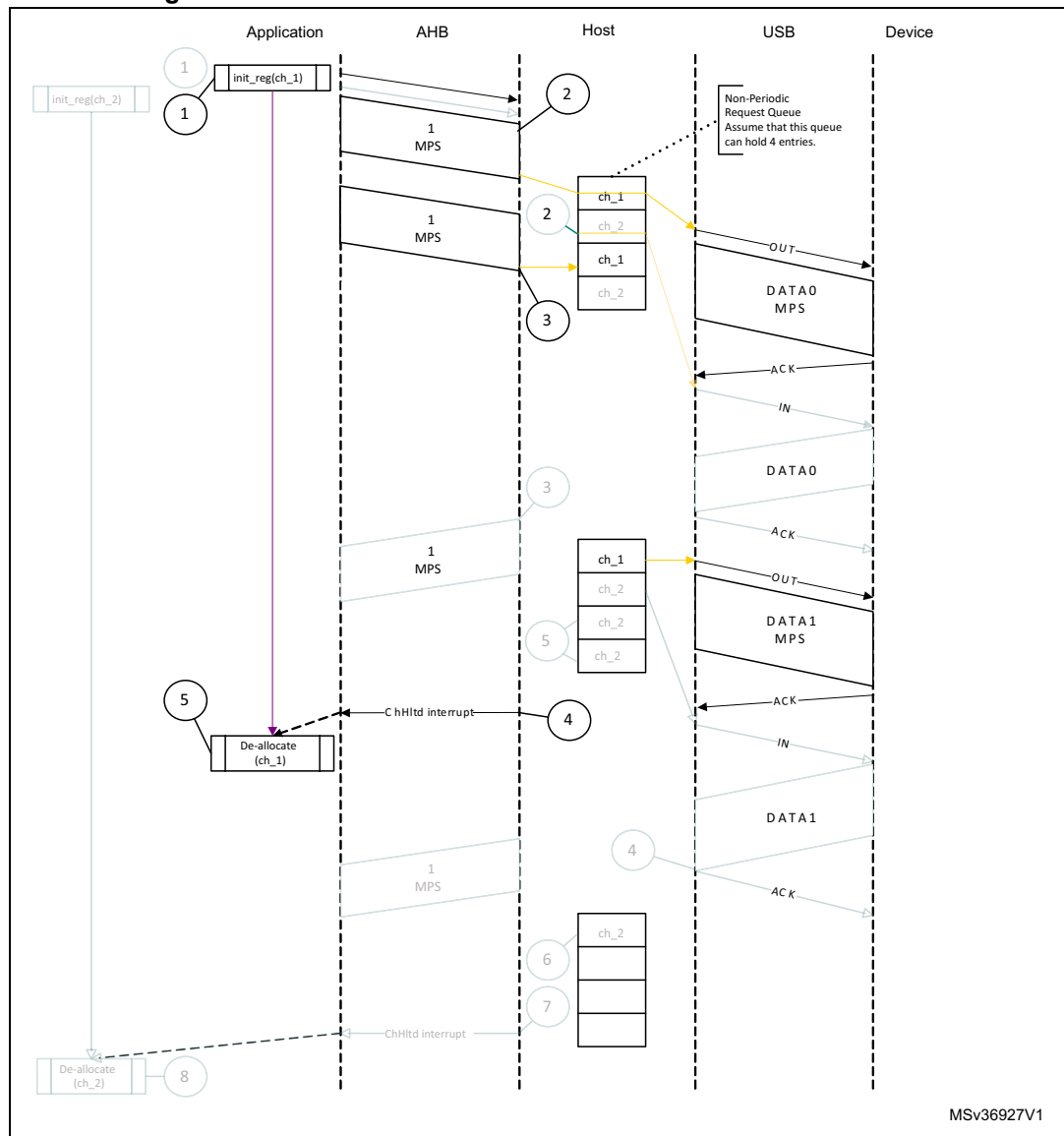
Figure 810. Normal bulk/control OUT/SETUP transactions - DMA
