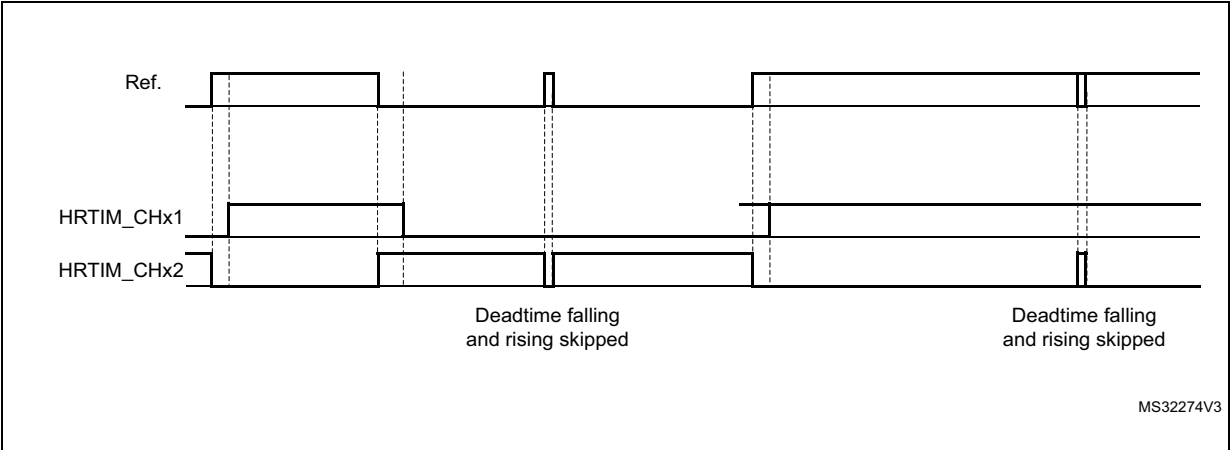
Figure 340. Complementary outputs for low pulse width (SDTRx = 0, SDTFx = 1)
