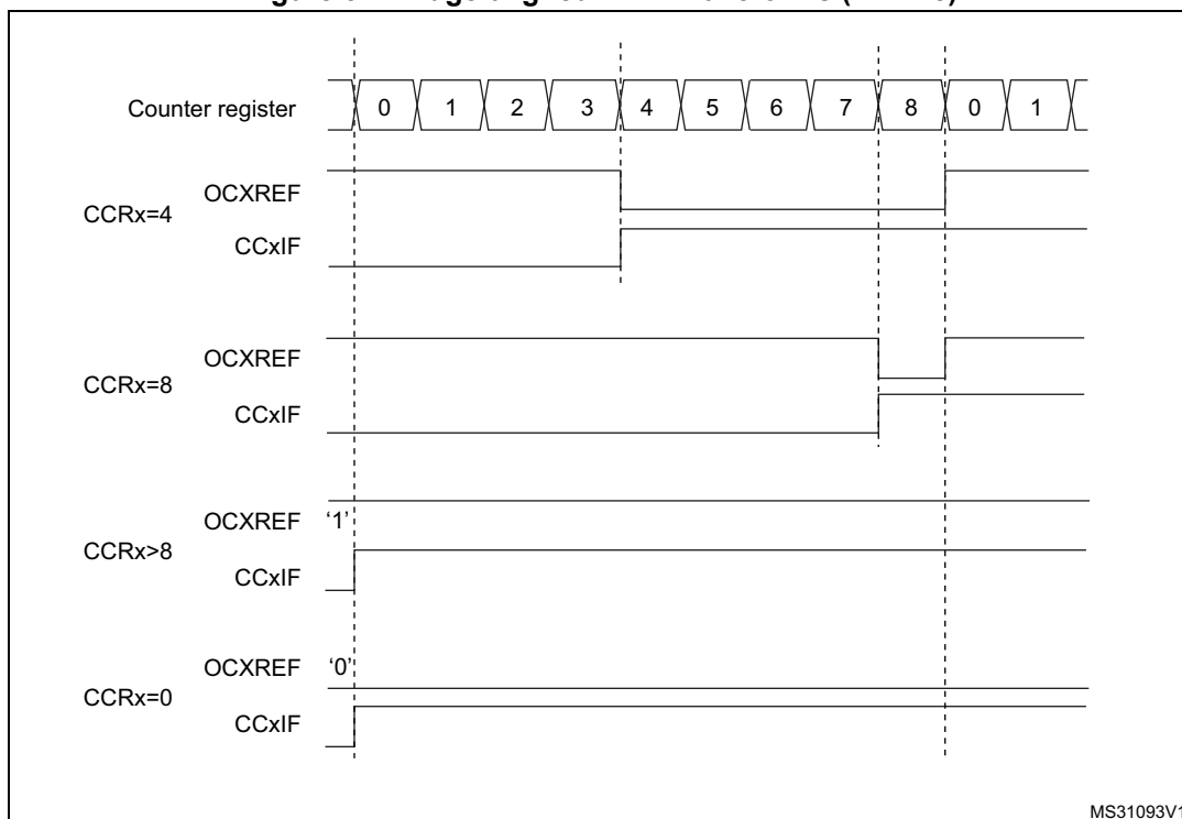
Figure 514. Edge-aligned PWM waveforms (ARR=8)
