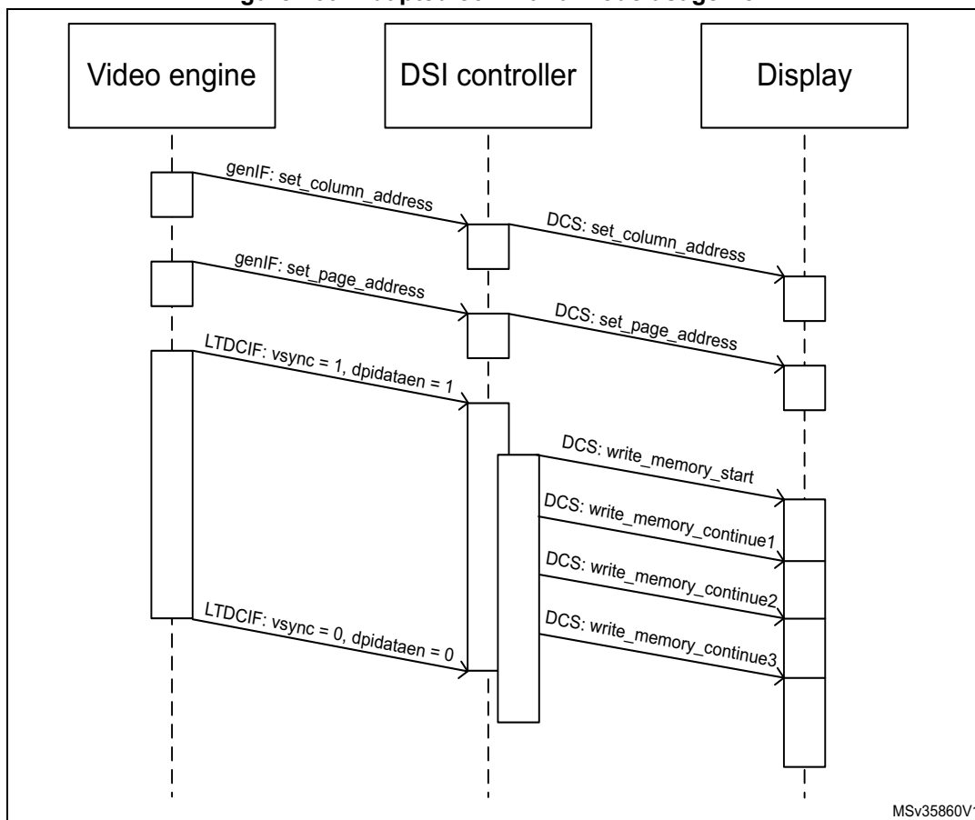
Figure 260. Adapted command mode usage flow
