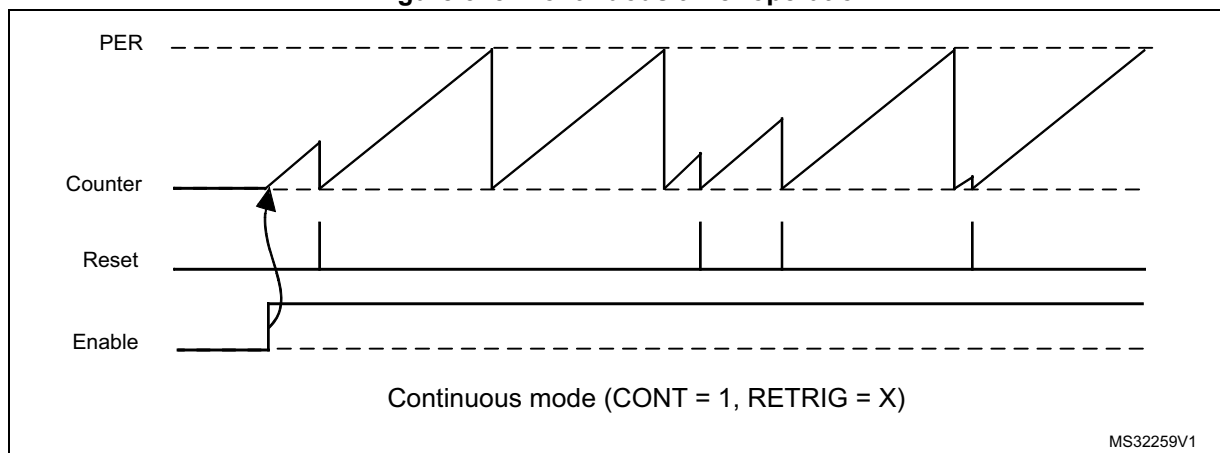
Figure 325. Continuous timer operation
