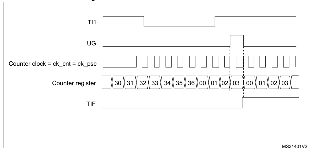
Figure 519. Control circuit in reset mode
