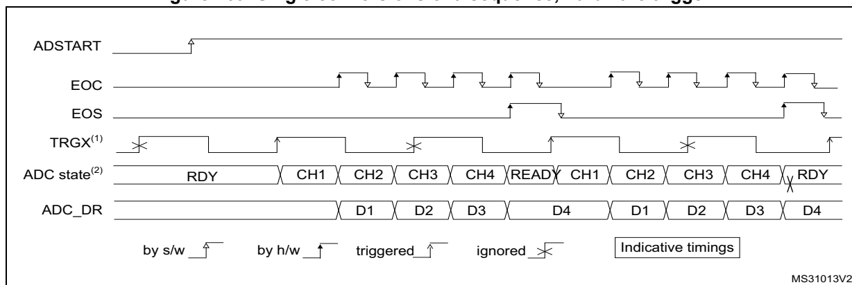
Figure 169. Single conversions of a sequence, hardware trigger
