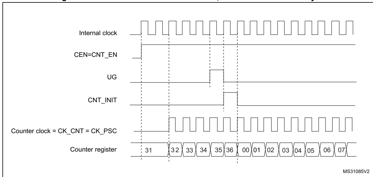
Figure 466. Control circuit in normal mode, internal clock divided by 1
