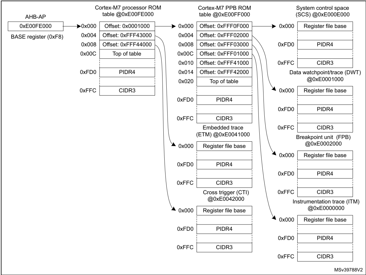
Figure 882. Cortex-M7 CoreSight topology
