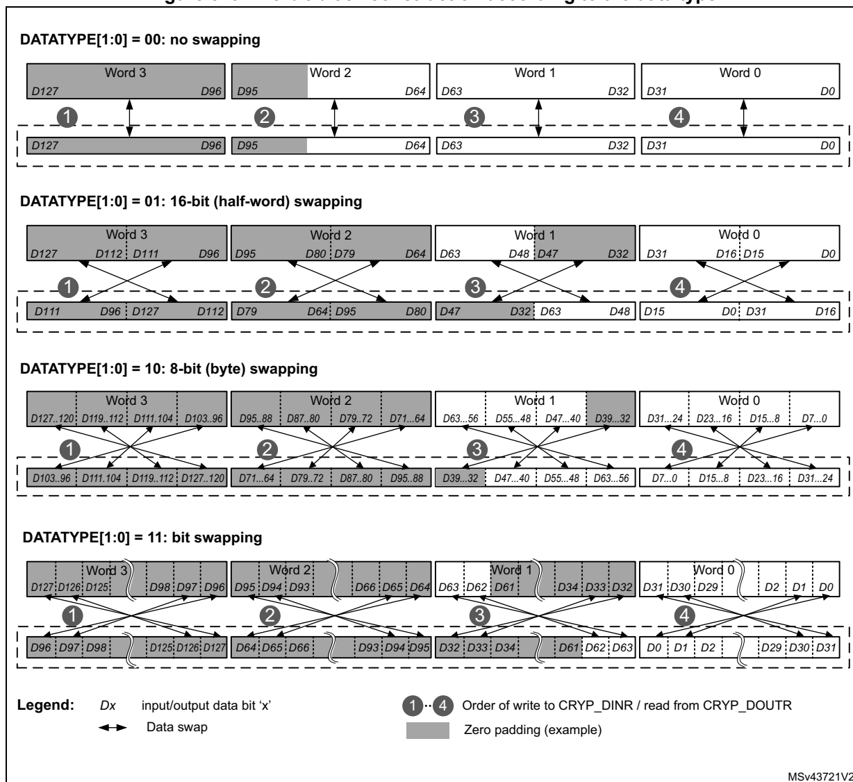
Figure 319. 128-bit block construction according to the data type
