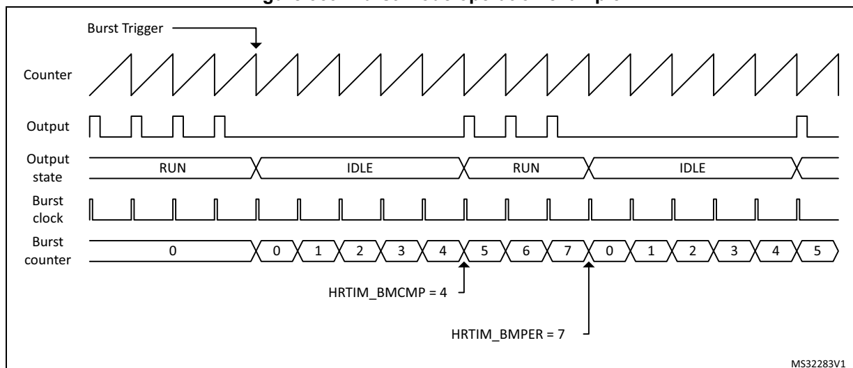
Figure 359. Burst mode operation example
