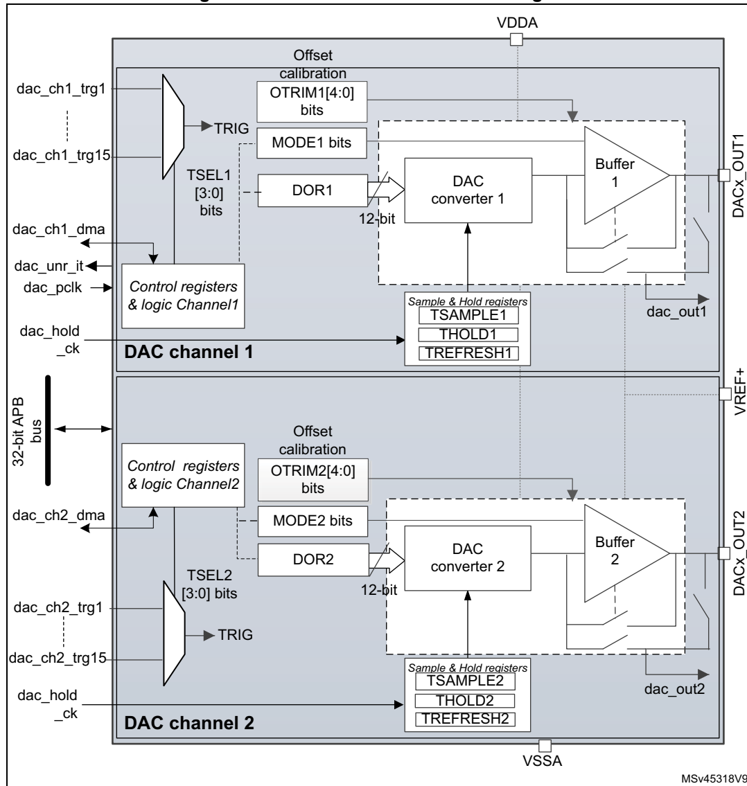
Figure 212. Dual-channel DAC block diagram
