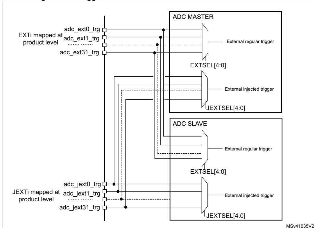
Figure 153. Triggers are shared between ADC master and ADC slave
