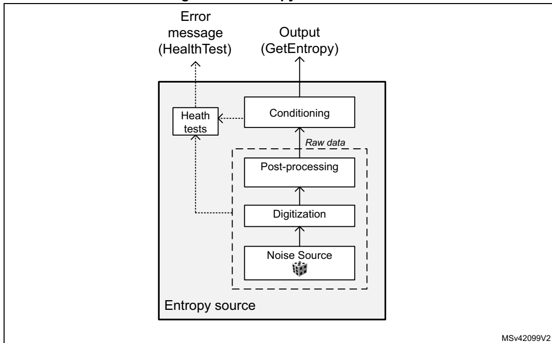
Figure 294. Entropy source model
