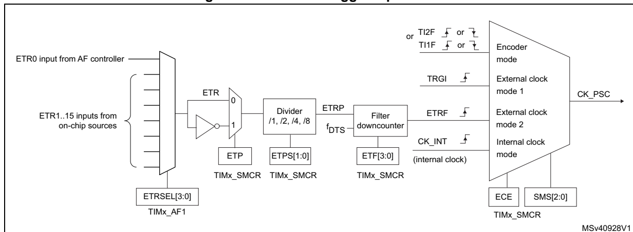
Figure 469. External trigger input block
