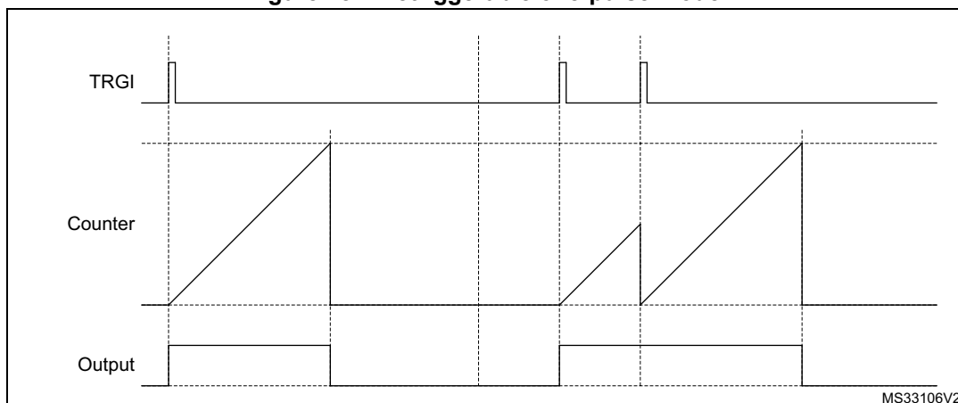
Figure 482. Retriggerable one-pulse mode.
