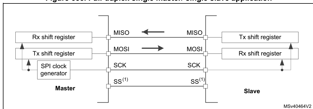
Figure 655. Full-duplex single master/ single slave application
