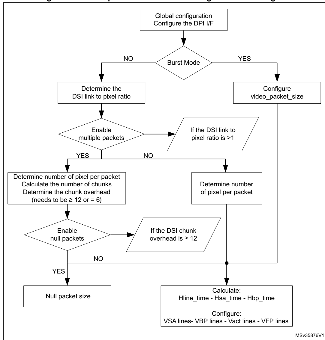
Figure 289. Video packet transmission configuration flow diagram
