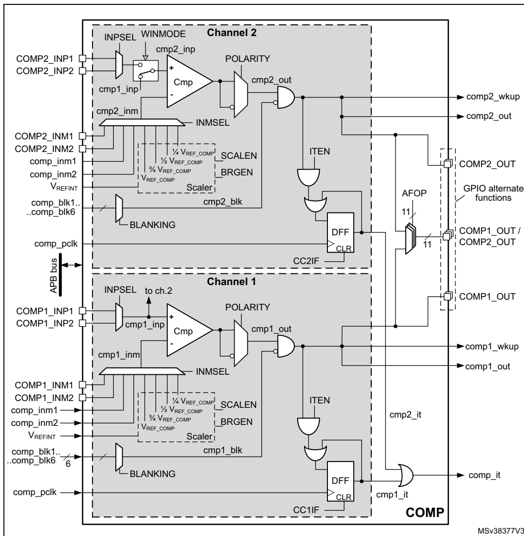
Figure 221. Comparator functional block diagram
