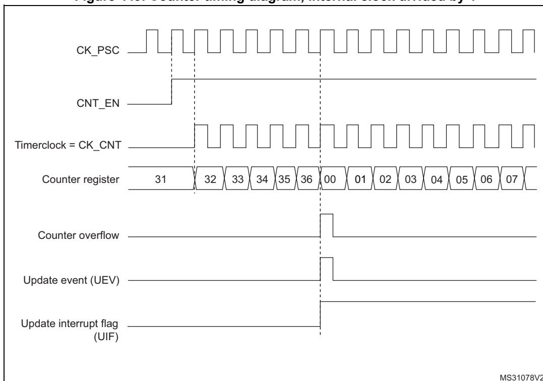
Figure 449. Counter timing diagram, internal clock divided by 1
