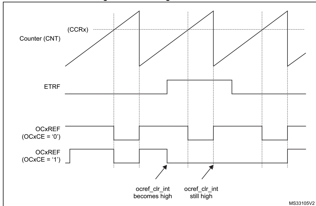
Figure 480. Clearing TIMx OCxREF
