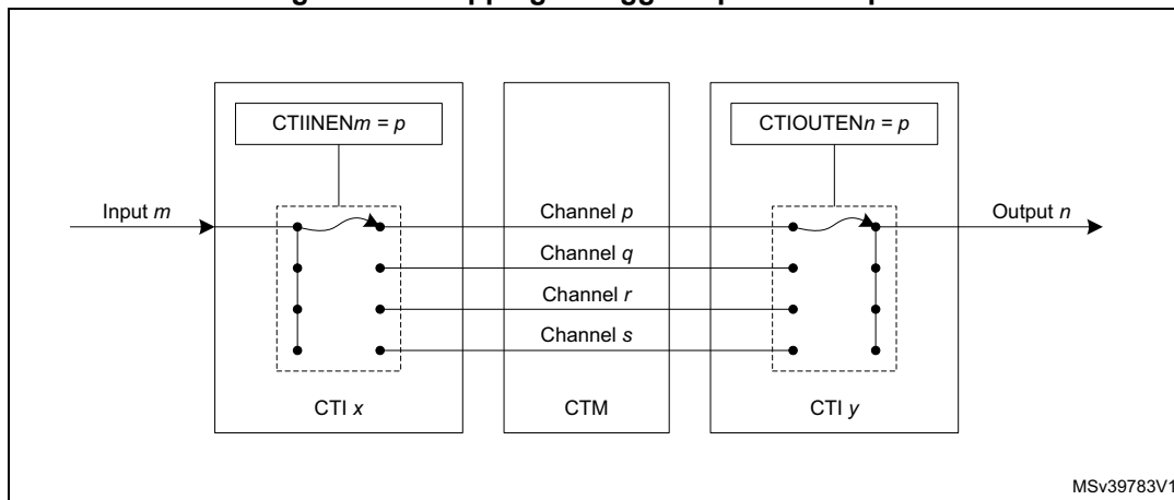
Figure 879. Mapping of trigger inputs to outputs
