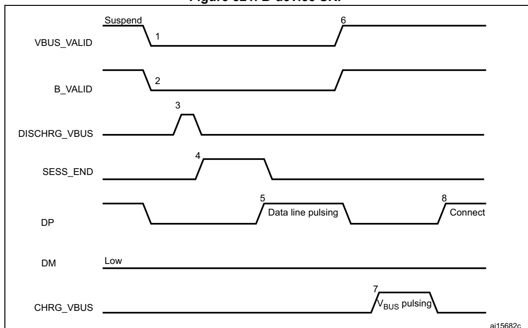
Figure 821. B-device SRP
