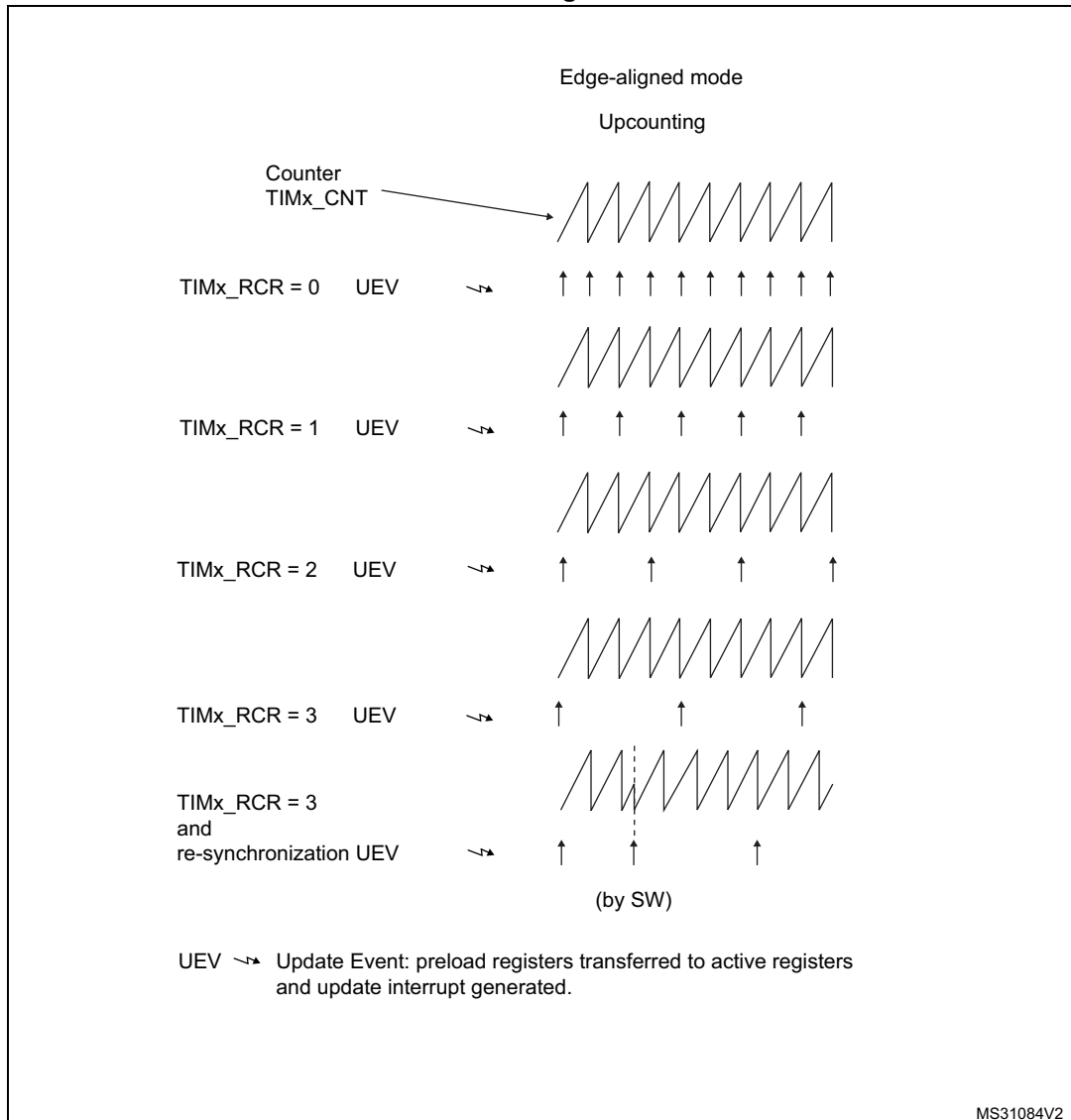
Figure 532. Update rate examples depending on mode and TIMx_RCR register settings
