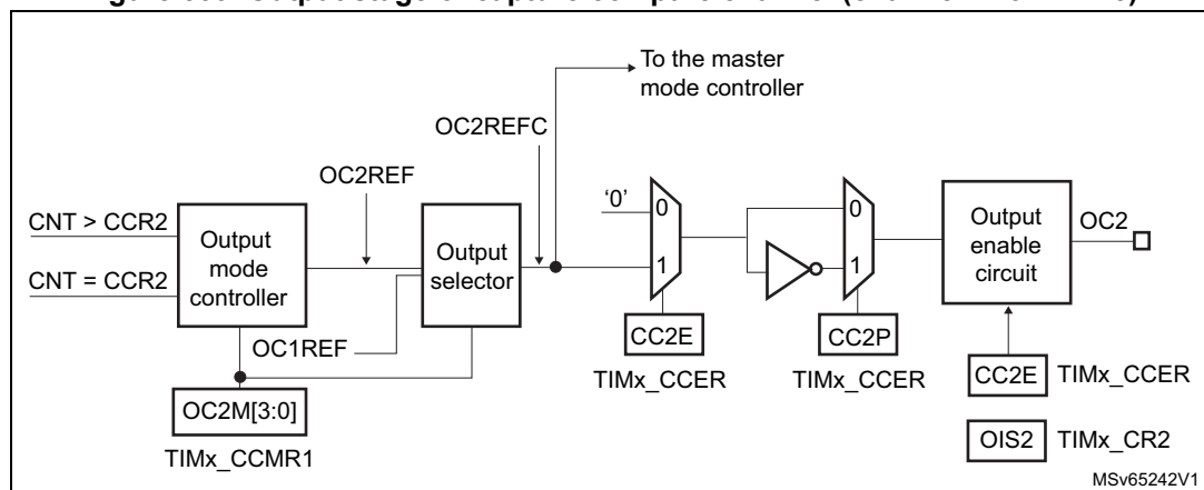
Figure 539. Output stage of capture/compare channel (channel 2 for TIM15)
