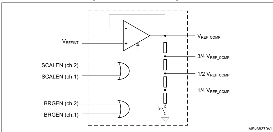
Figure 225. Scaler block diagram
