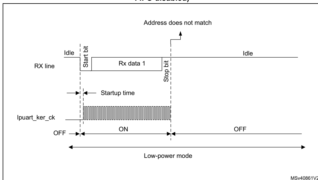
Figure 653. Wake-up event not verified (wake-up event = address match, FIFO disabled)
