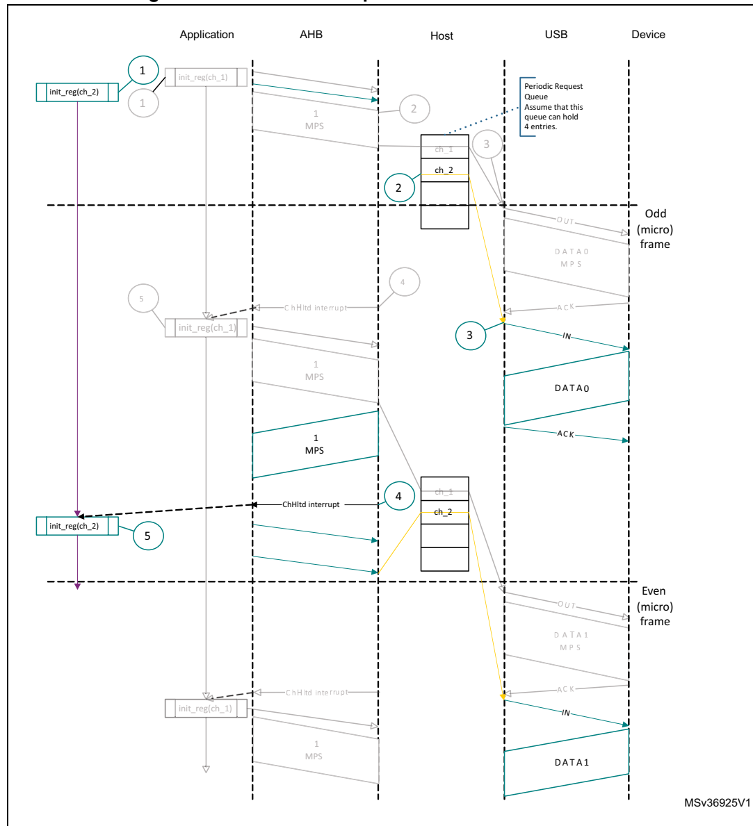
Figure 813. Normal interrupt IN transactions - DMA mode
