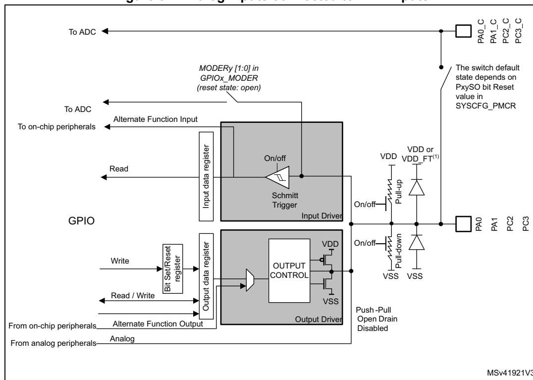
Figure 82. Analog inputs connected to ADC inputs
