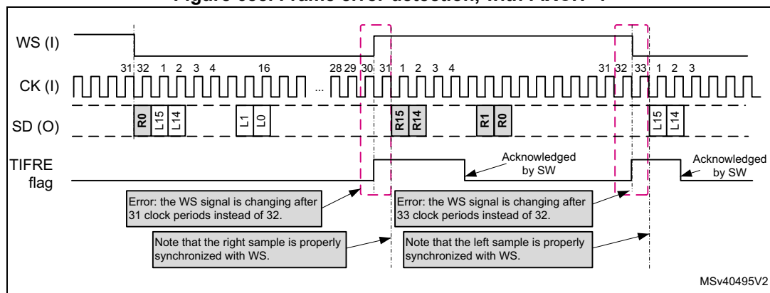
Figure 688. Frame error detection, with FIXCH=1
