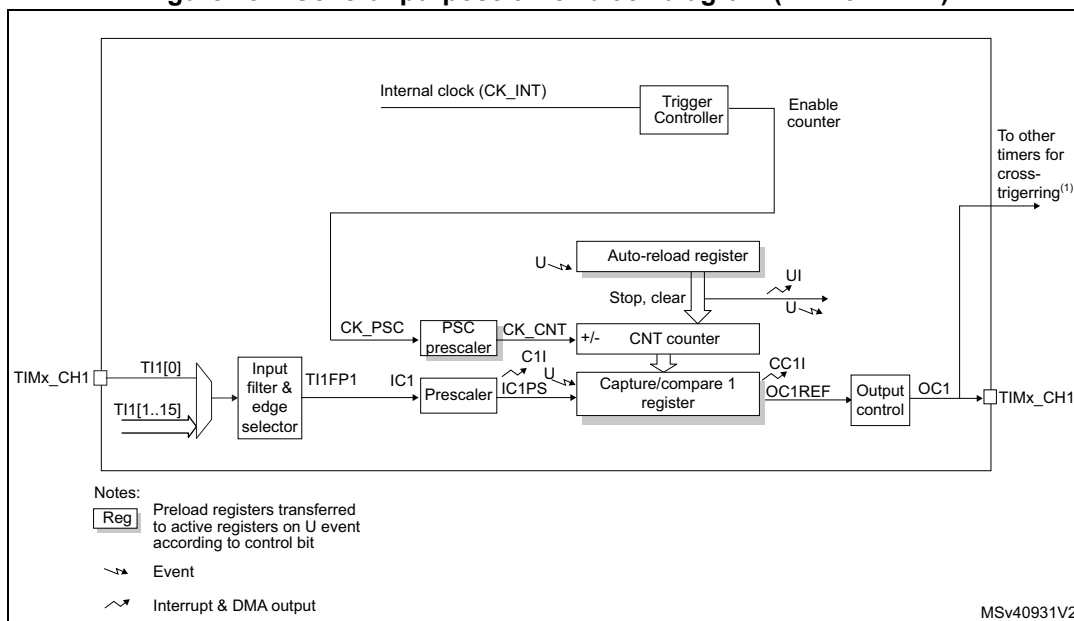
Figure 497. General-purpose timer block diagram (TIM13/TIM14)
