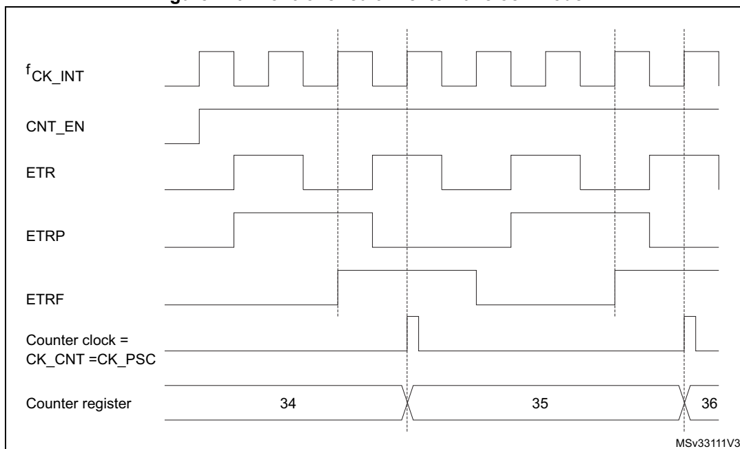
Figure 470. Control circuit in external clock mode 2
