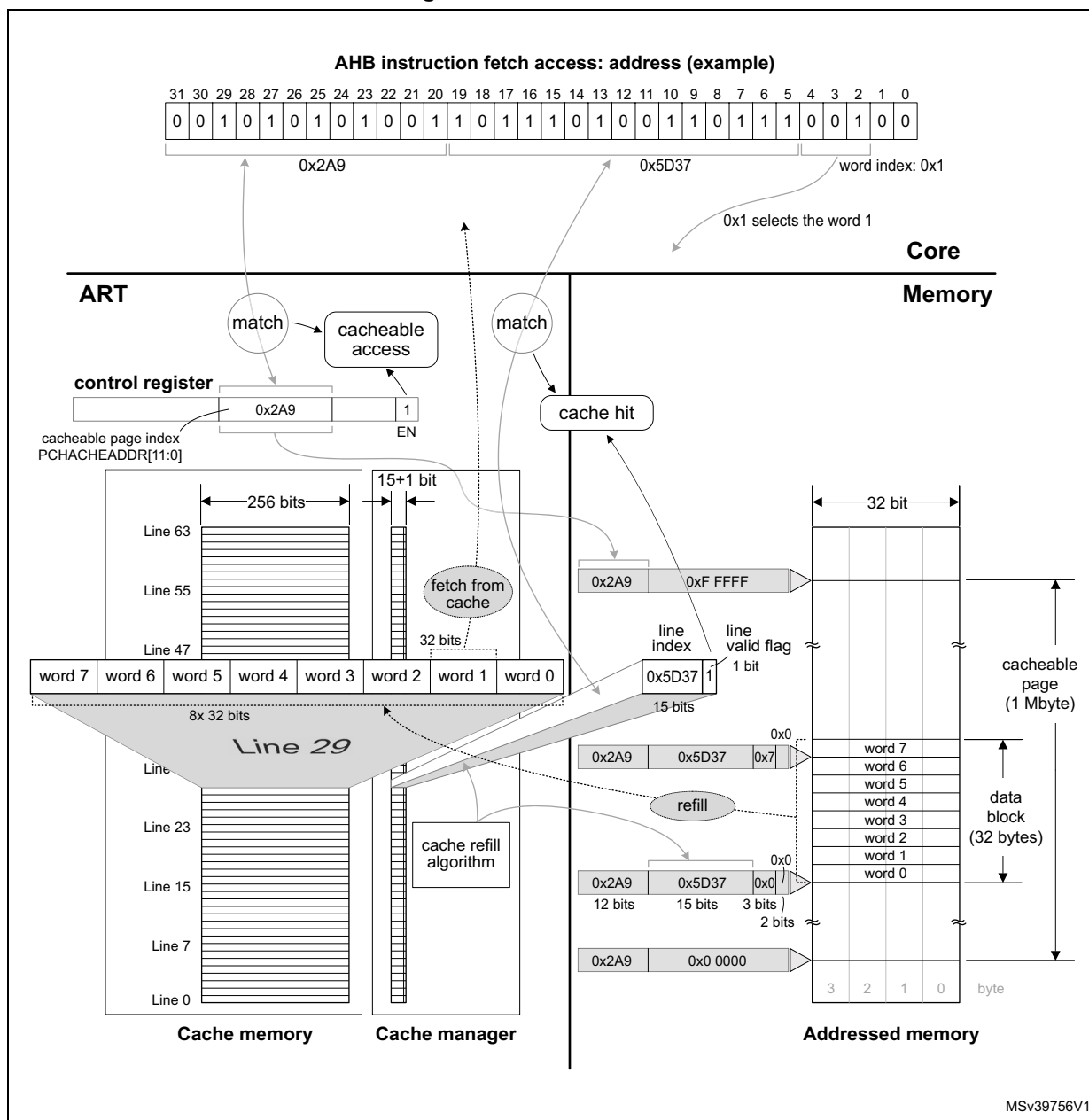
Figure 19. Instruction fetch from cache
