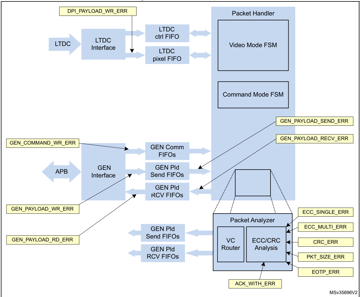
Figure 288. Error sources
