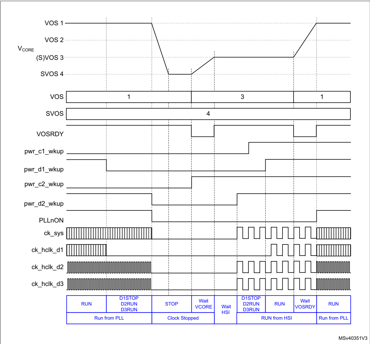
Figure 40. Dynamic voltage scaling behavior with D1, D2 and system in Stop mode
