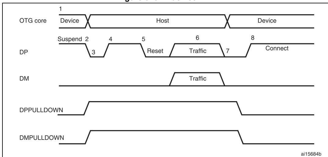
Figure 823. B-device HNP
