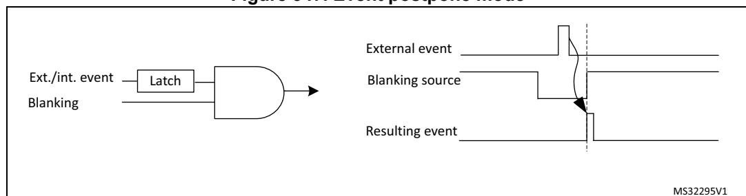
Figure 347. Event postpone mode
