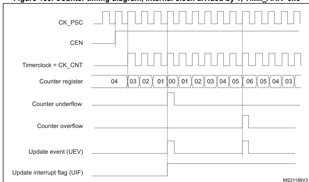
Figure 460. Counter timing diagram, internal clock divided by 1, TIMx_ARR=0x6
