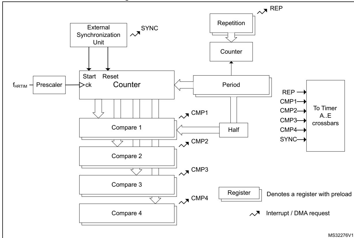
Figure 342. Master timer overview
