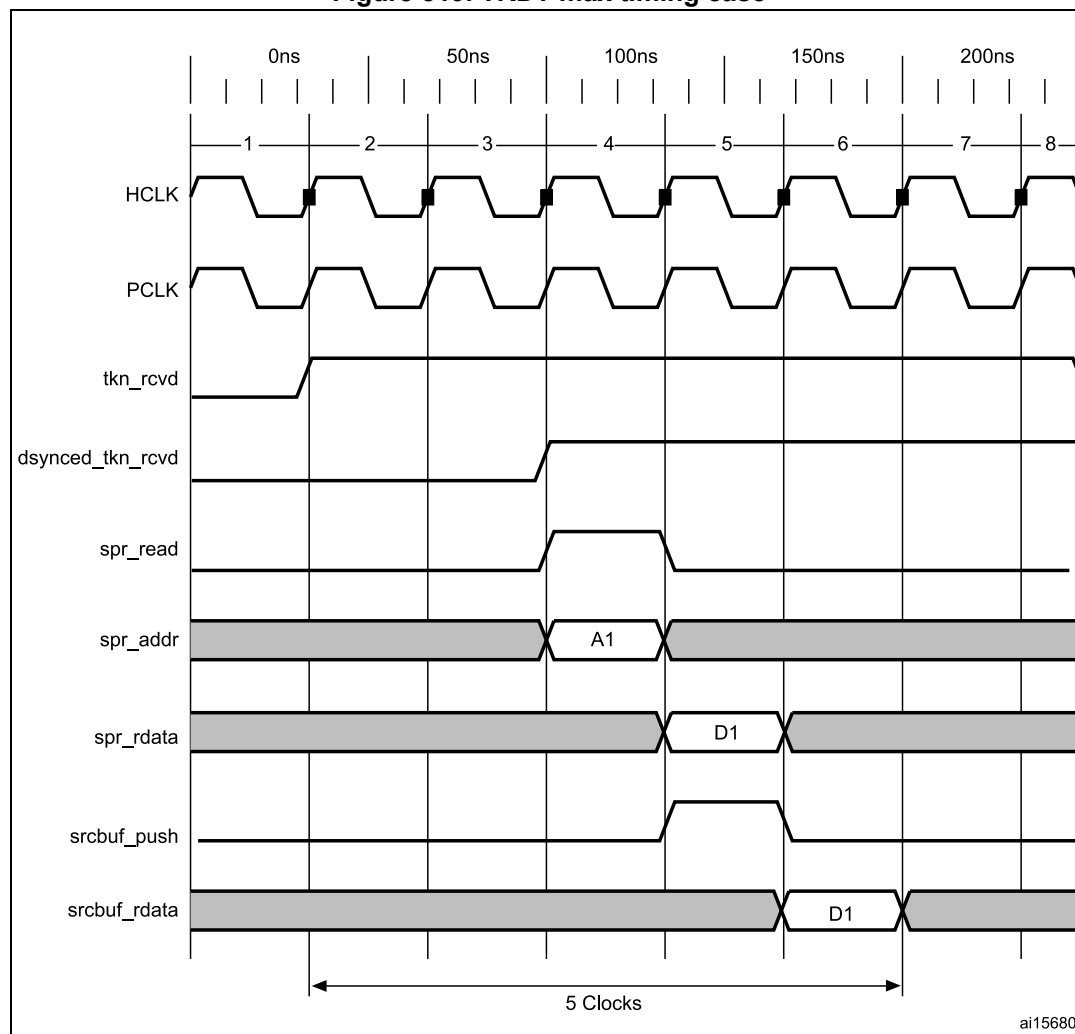
Figure 819. TRDT max timing case
