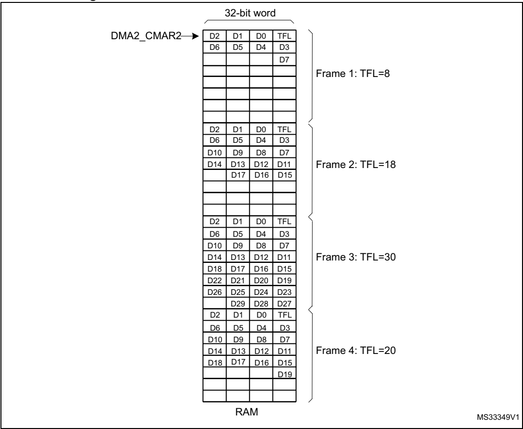
Figure 734. SWPMI Multi software buffer mode transmission
