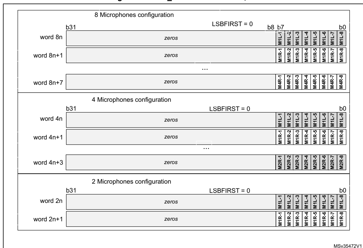
Figure 701. SAI_ADR format in TDM, 8-bit slot width
