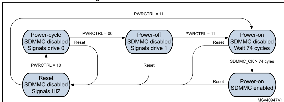
Figure 771. SDMMC state control
