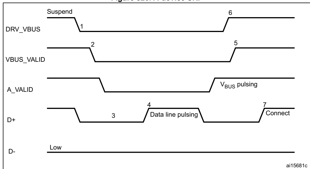
Figure 820. A-device SRP
