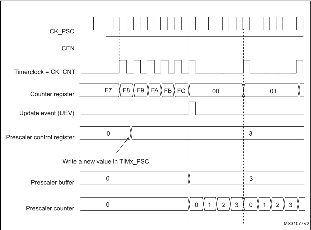
Figure 388. Counter timing diagram with prescaler division change from 1 to 4
