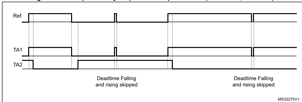
Figure 341. Complementary outputs for low pulse width (SDTRx = 1, SDTFx=0)
