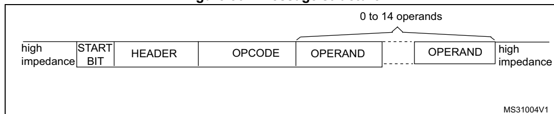
Figure 861. Message structure
