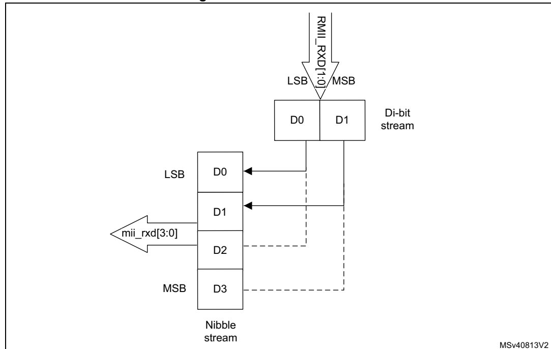
Figure 847. Receive bit order
