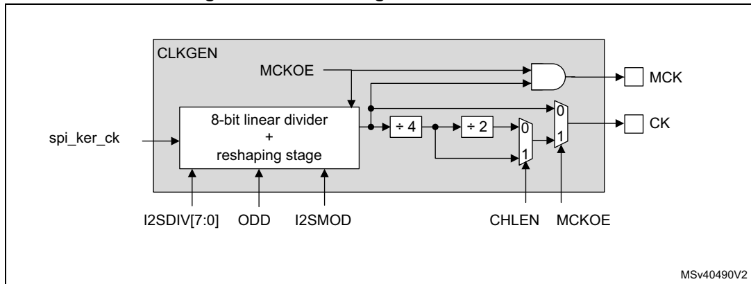
Figure 683. I 2 S clock generator architecture
