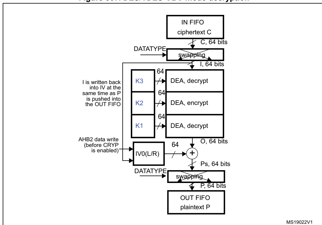
Figure 307. DES/TDES-CBC mode decryption
