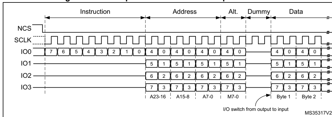
Figure 134. Example of read command in quad-SPI mode
