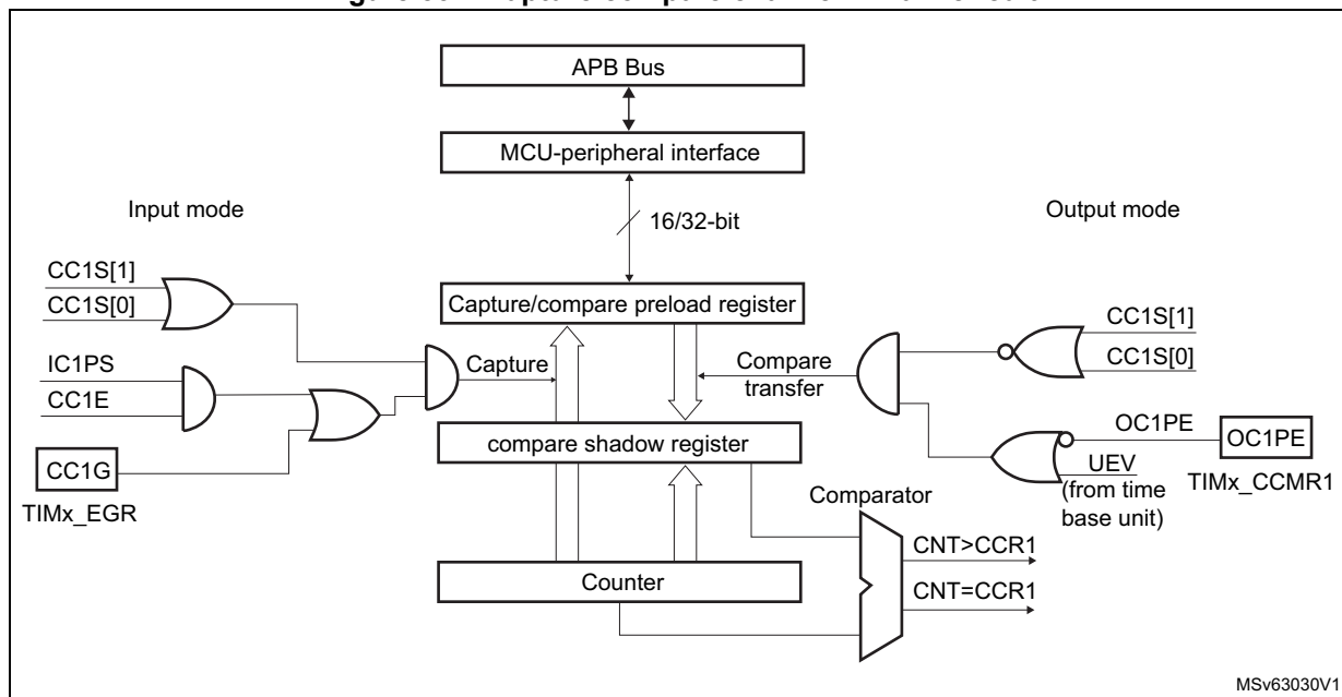
Figure 537. Capture/compare channel 1 main circuit
