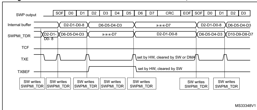
Figure 733. SWPMI No software buffer mode transmission, consecutive frames
