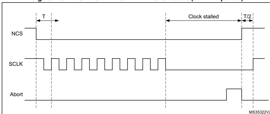
Figure 139. NCS when CKMODE = 1 with an abort ( T = \text{CLK period} )
