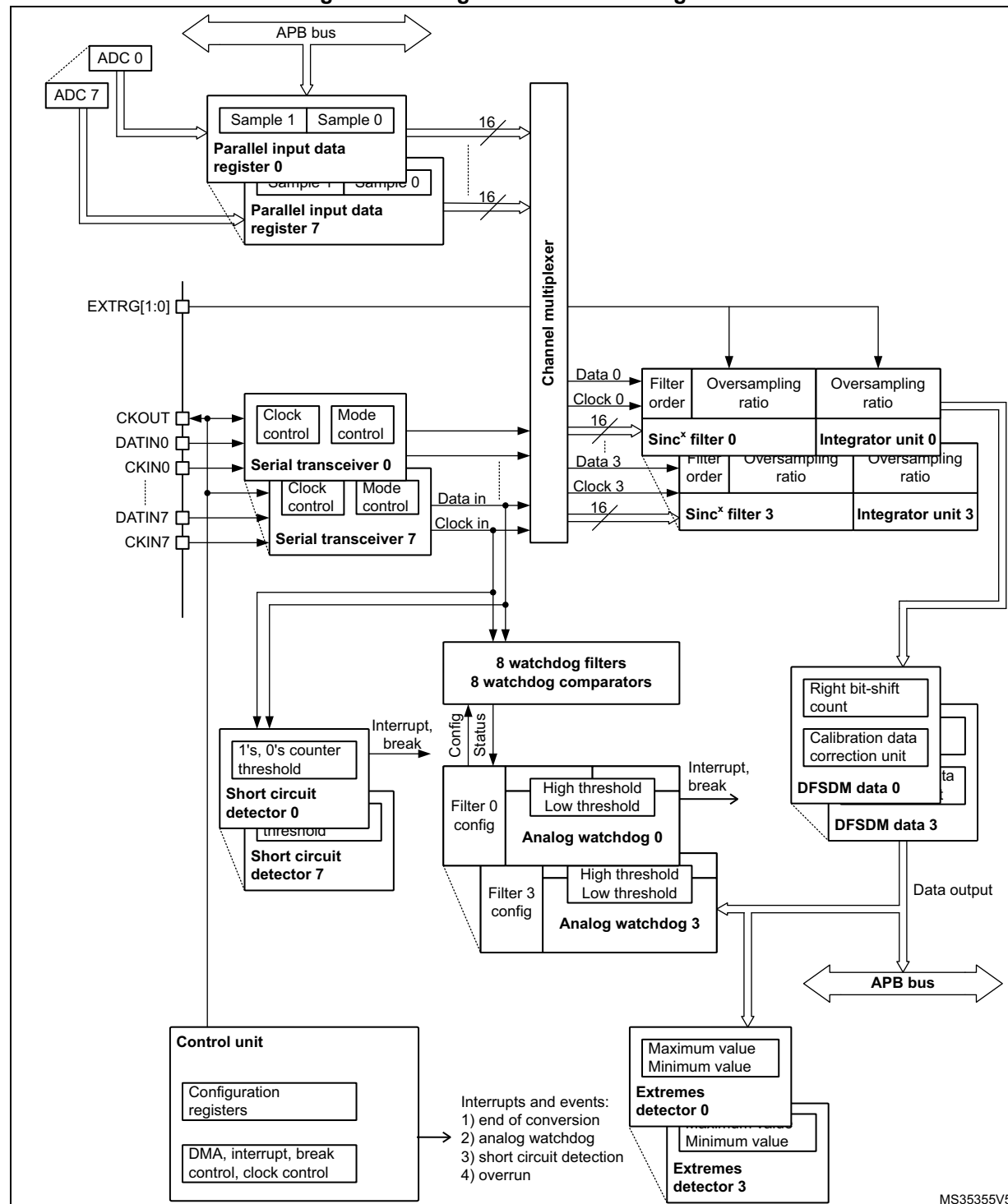
Figure 234. Single DFSDM block diagram
