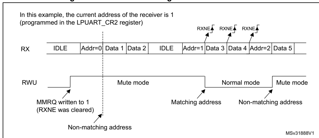
Figure 646. Mute mode using address mark detection
