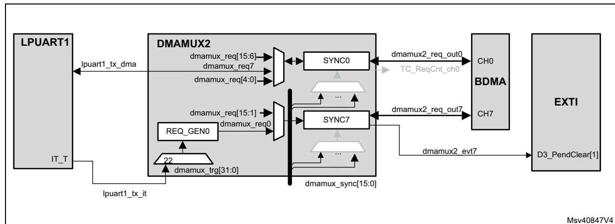
Figure 46. BDMA and DMAMUX2 interconnection
