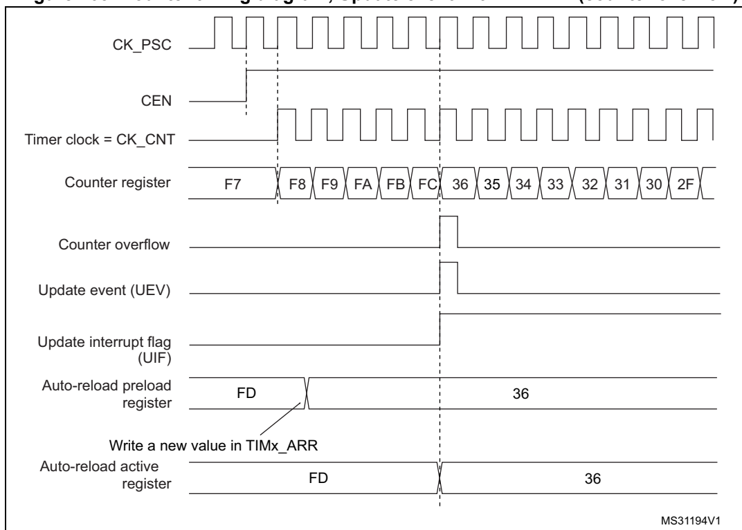
Figure 465. Counter timing diagram, Update event with ARPE=1 (counter overflow)
