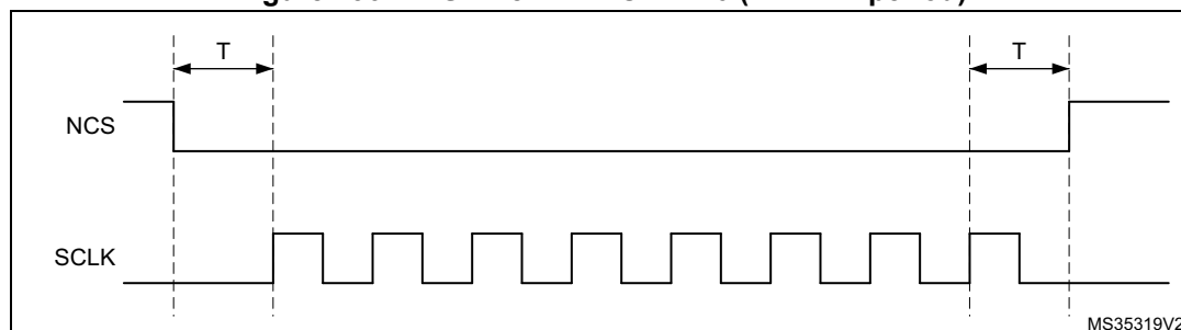
Figure 136. NCS when CKMODE = 0 (T = CLK period)
