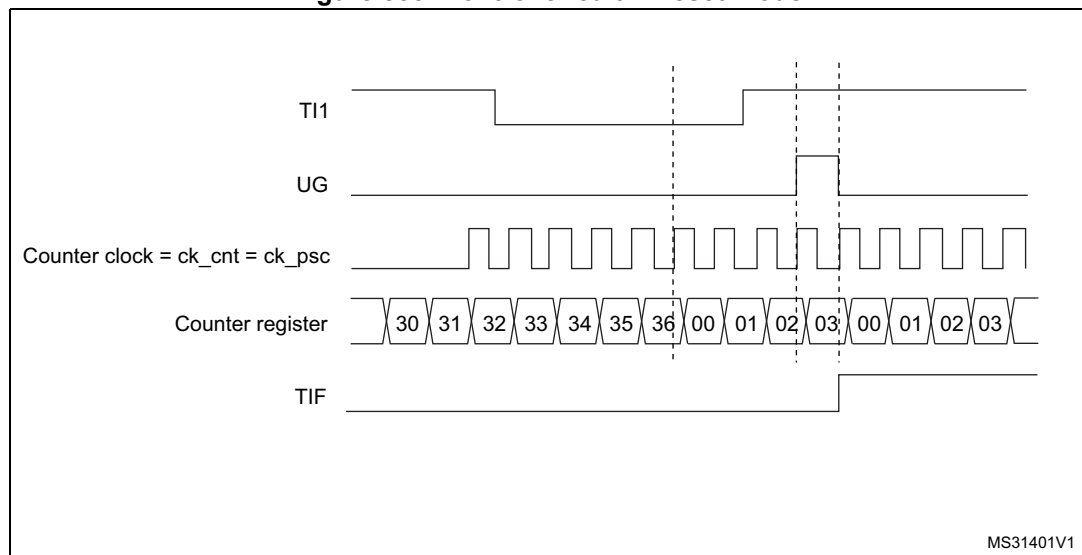
Figure 553. Control circuit in reset mode
