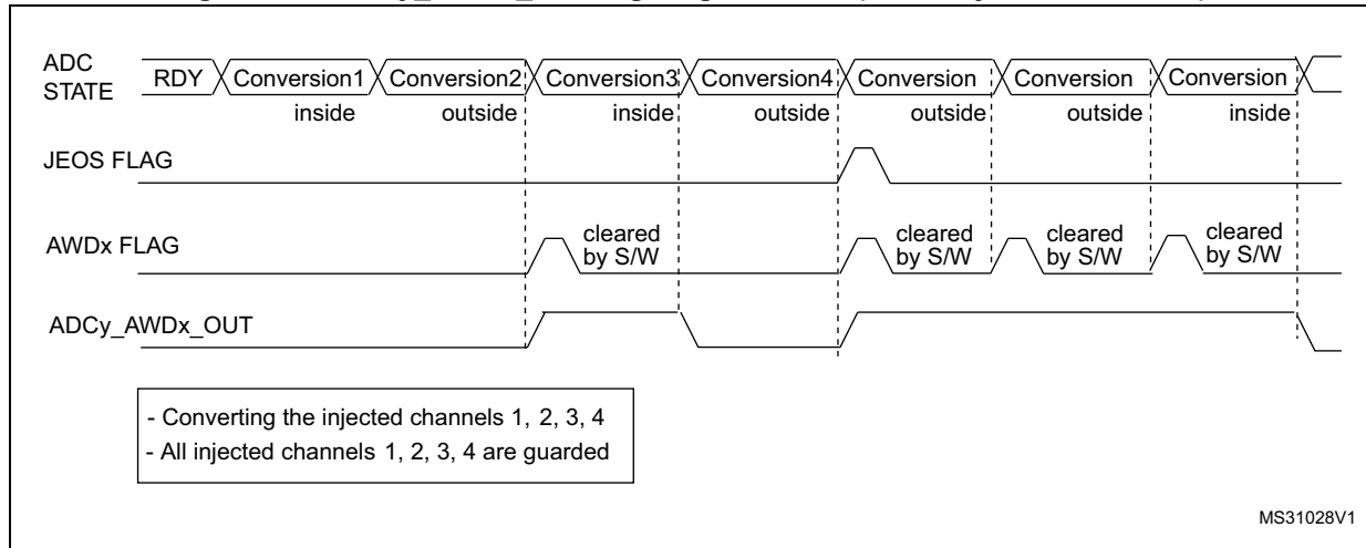
Figure 186. ADCy_AWDx_OUT signal generation (on all injected channels)
