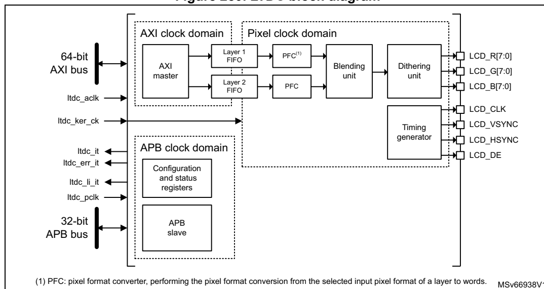
Figure 250. LTDC block diagram
