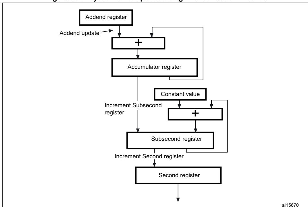
Figure 833. System time update using fine correction method
