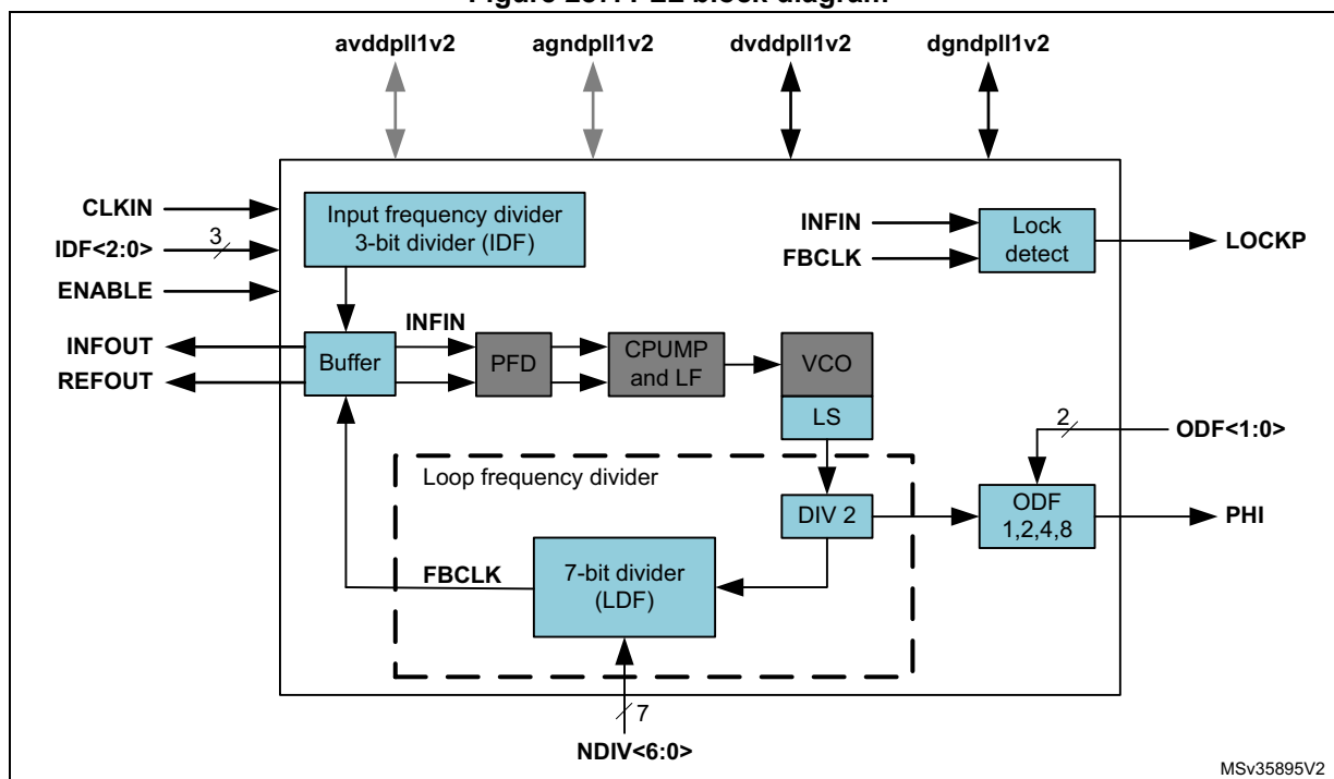
Figure 287. PLL block diagram
