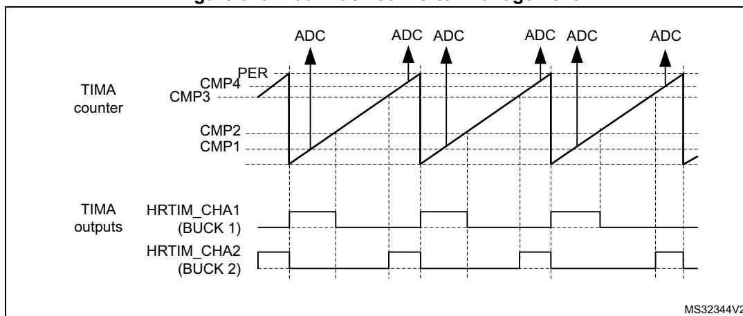
Figure 379. Dual Buck converter management
