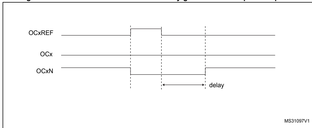
Figure 546. Dead-time waveforms with delay greater than the positive pulse.
