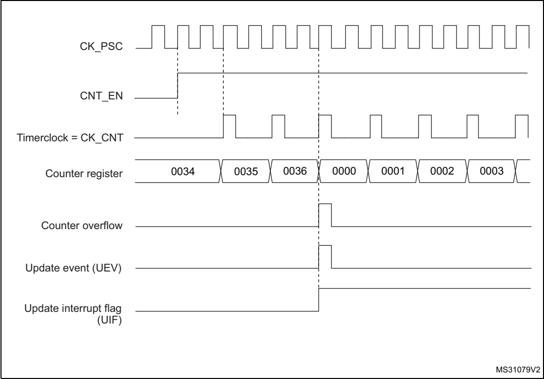
Figure 501. Counter timing diagram, internal clock divided by 2
