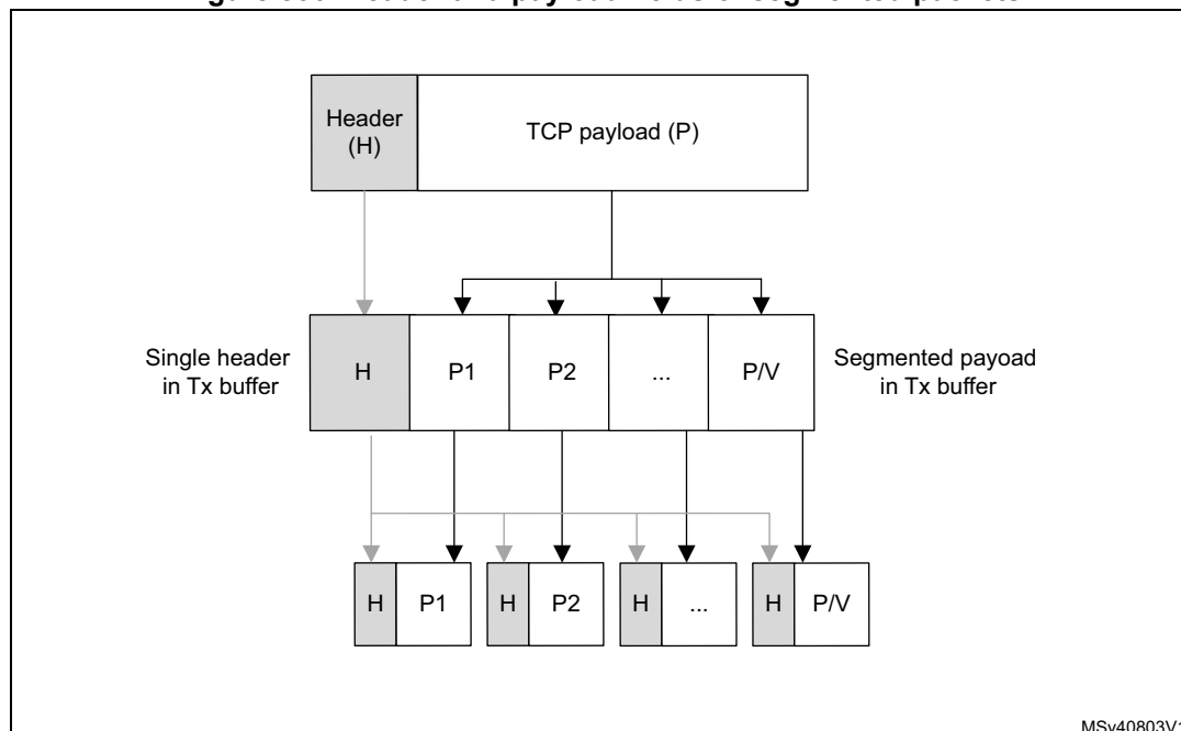
Figure 836. Header and payload fields of segmented packets
