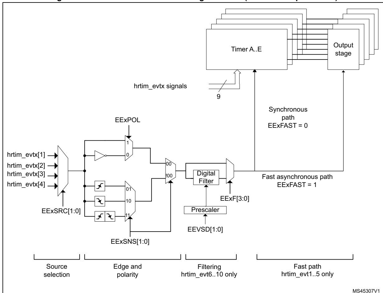
Figure 343. External event conditioning overview (1 channel represented)
