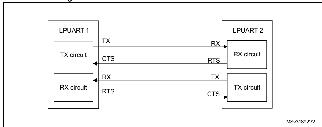
Figure 649. Hardware flow control between 2 LPUARTs
