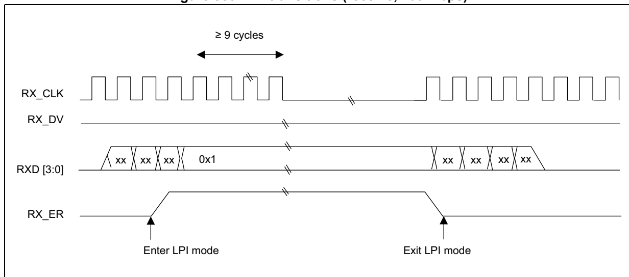
Figure 850. LPI transitions (receive, 100 Mbps)
