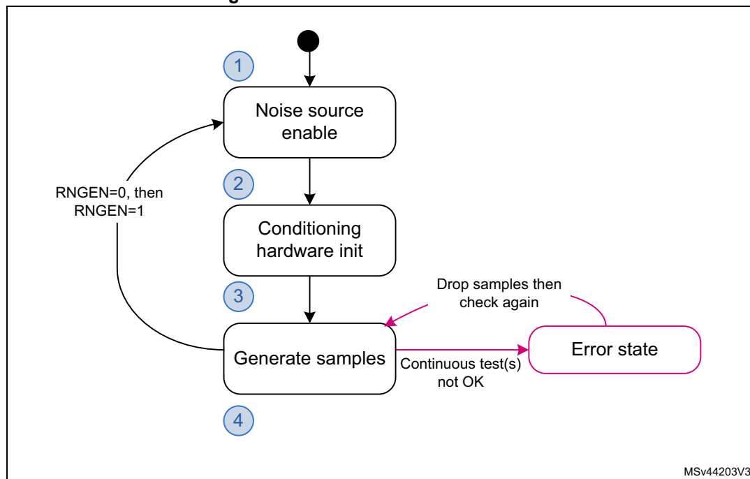
Figure 295. RNG initialization overview
