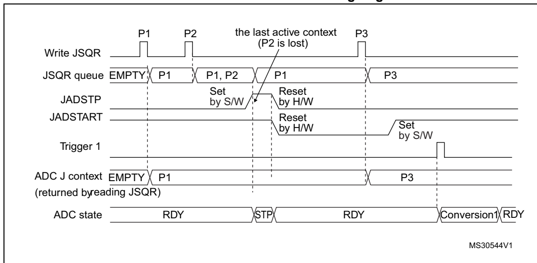
Figure 163. Flushing JSQR queue of context by setting JADSTP=1 (JQM=0). Case when JADSTP occurs outside an ongoing conversion
