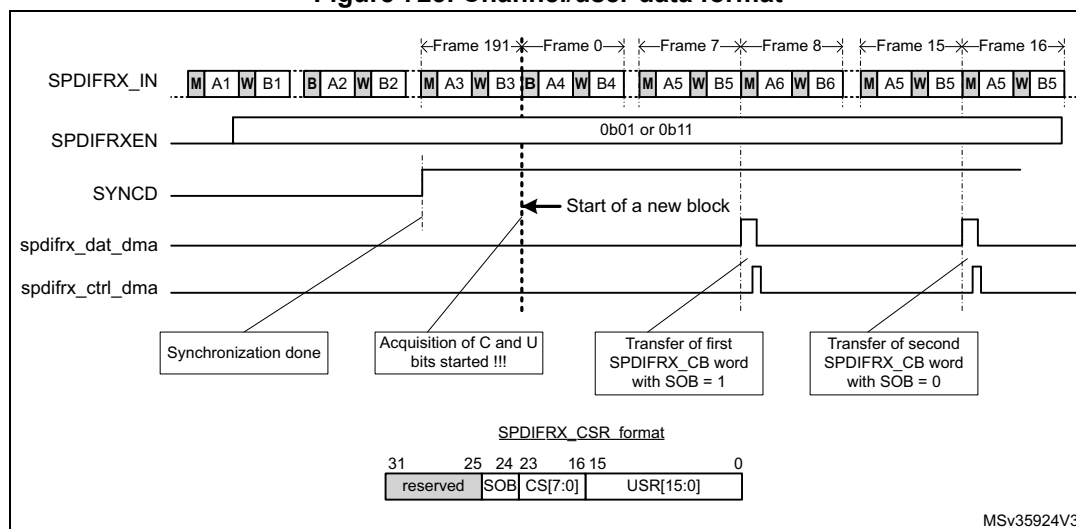
Figure 723. Channel/user data format
