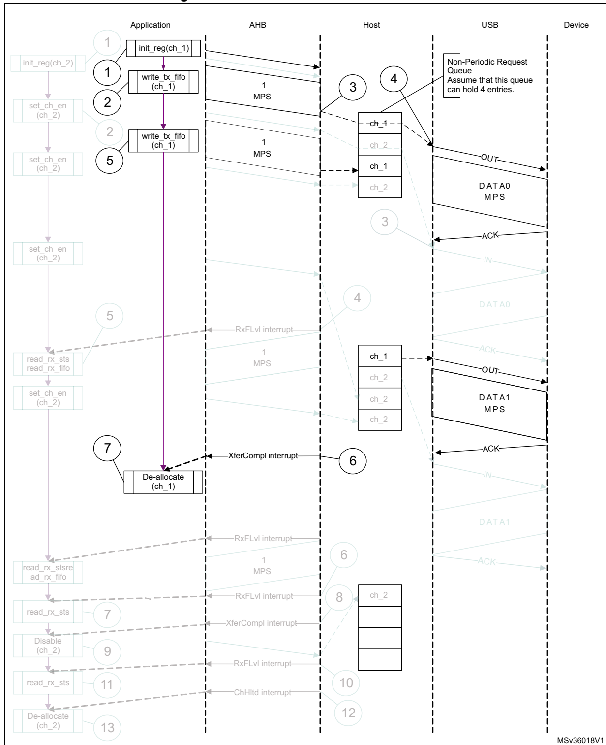
Figure 804. Normal bulk/control OUT/SETUP
