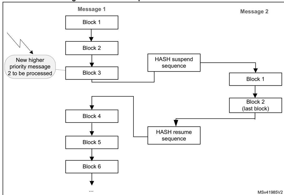
Figure 322. HASH suspend/resume mechanism
