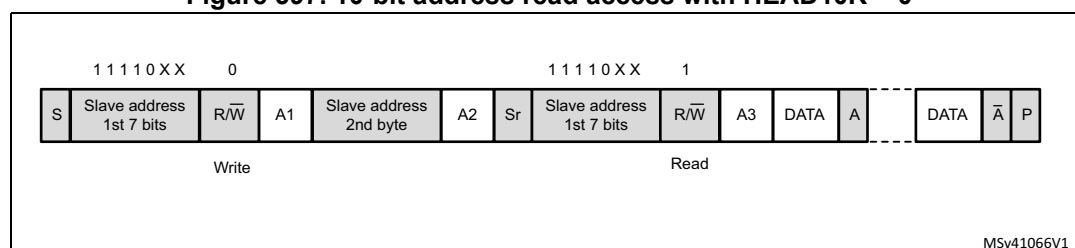
Figure 597. 10-bit address read access with HEAD10R = 0
