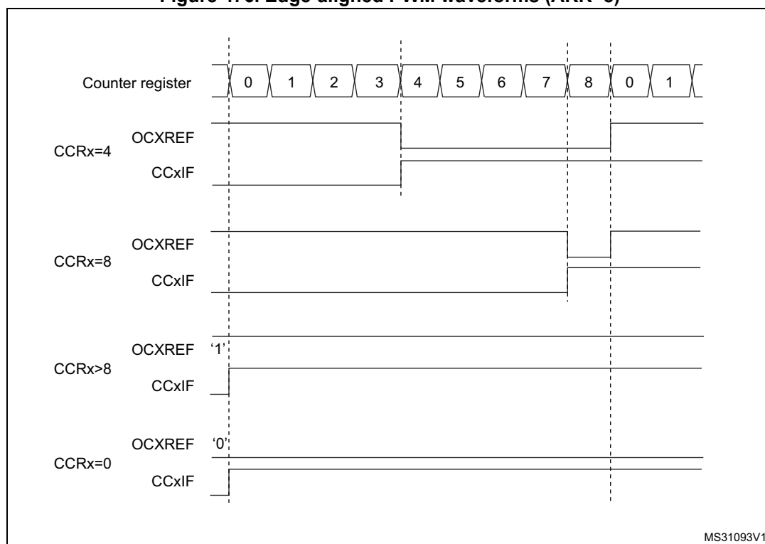
Figure 476. Edge-aligned PWM waveforms (ARR=8)
