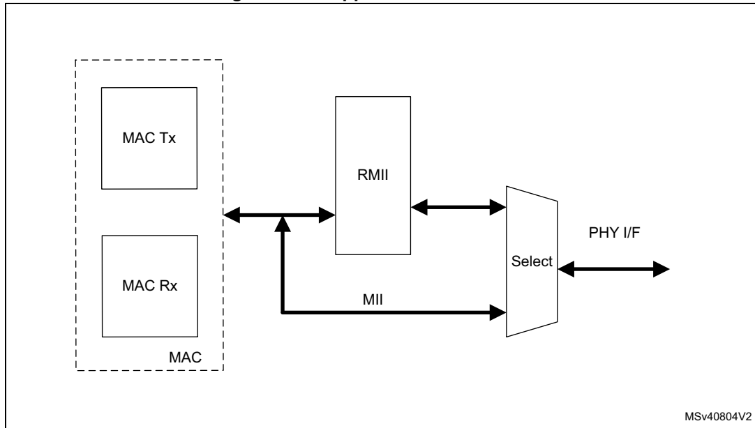
Figure 837. Supported PHY interfaces
