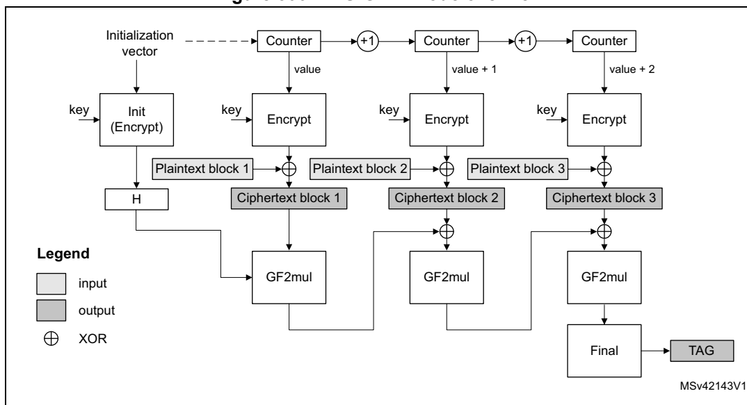
Figure 300. AES-GCM mode overview
