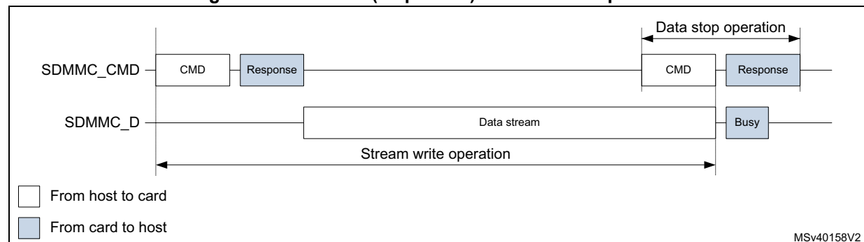
Figure 746. SDMMC (sequential) stream write operation
