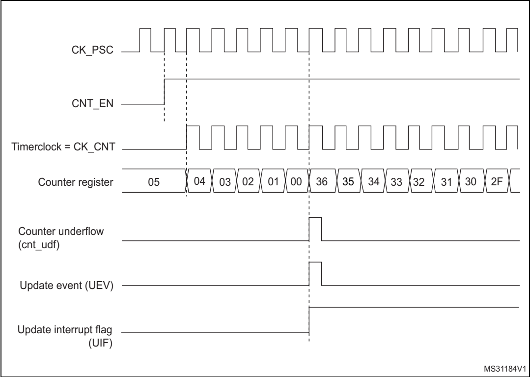
Figure 395. Counter timing diagram, internal clock divided by 1
