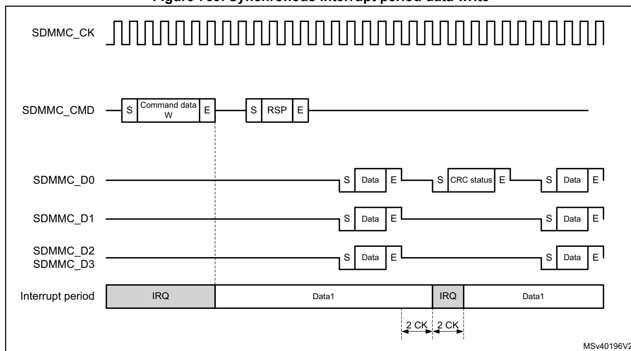
Figure 759. Synchronous interrupt period data write
