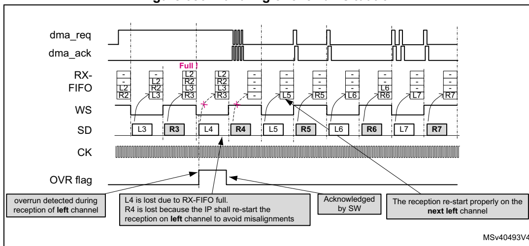
Figure 686. Handling of overrun situation
