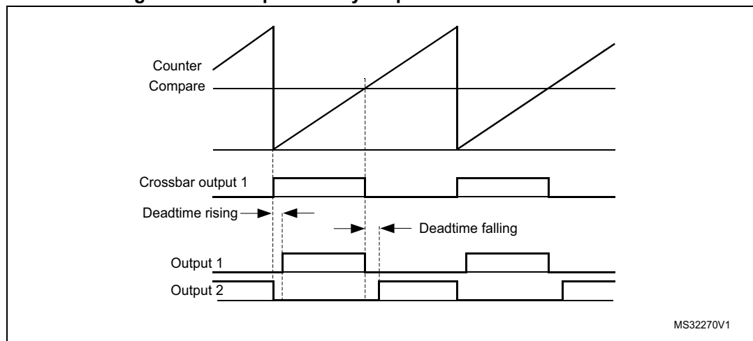
Figure 336. Complementary outputs with deadtime insertion
