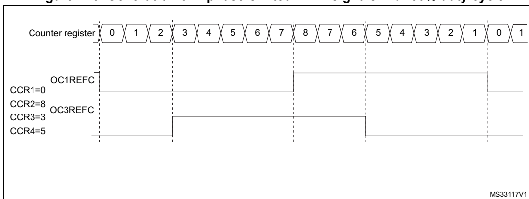
Figure 478. Generation of 2 phase-shifted PWM signals with 50% duty cycle
