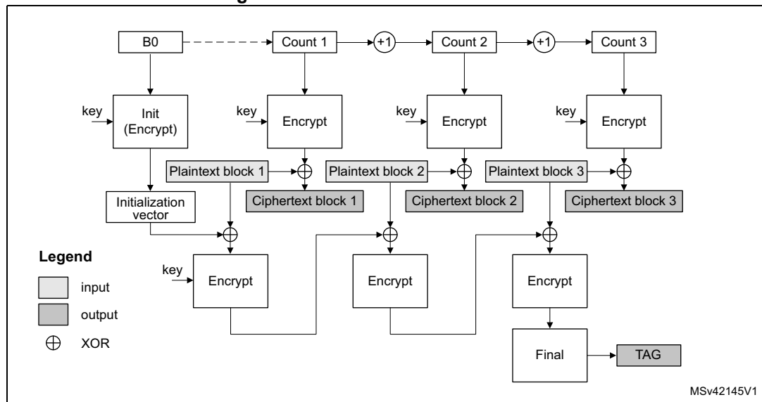
Figure 302. AES-CCM mode overview
