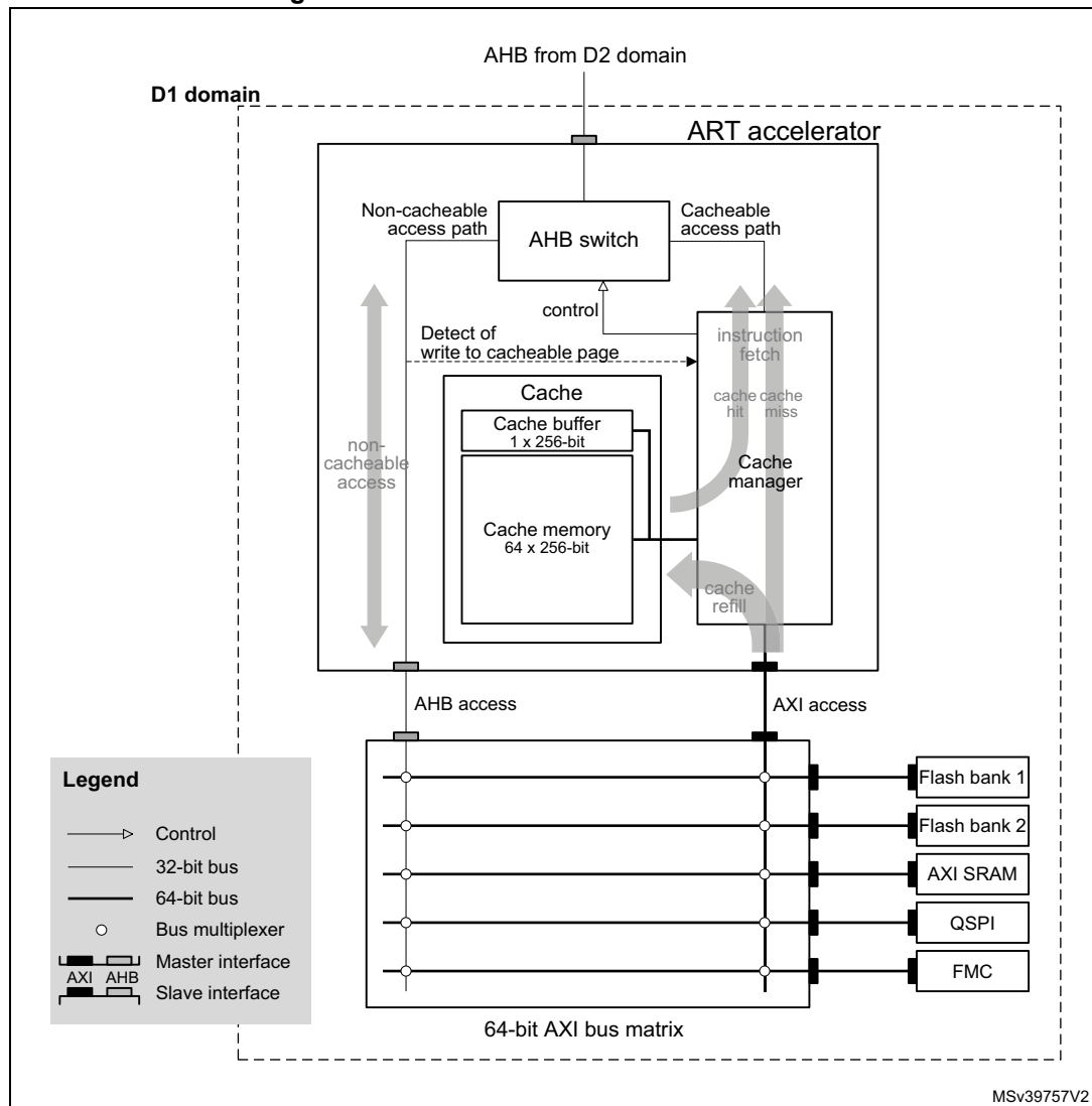
Figure 18. ART accelerator - block schematic
