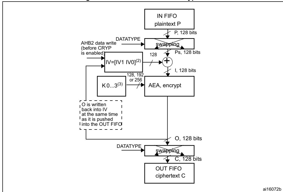
Figure 310. AES-CBC mode encryption
