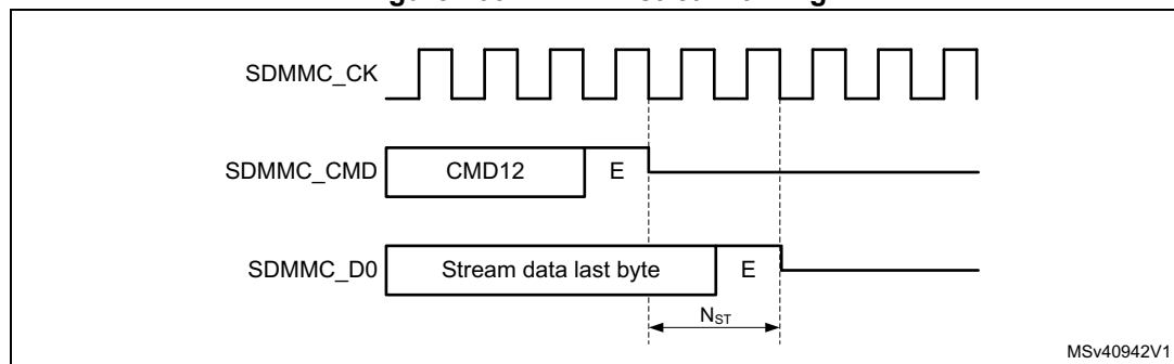
Figure 766. CMD12 stream timing
