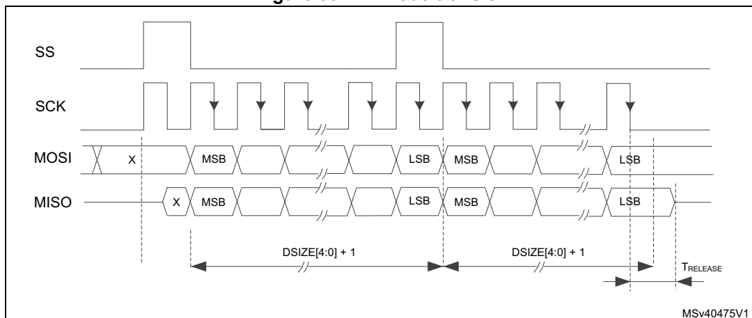
Figure 667. TI mode transfer
