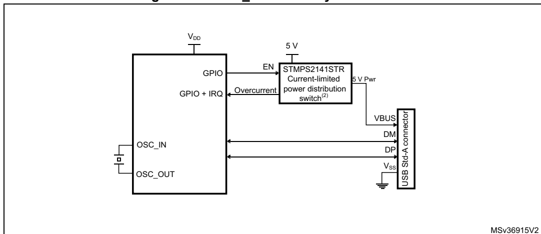
Figure 796. OTG_HS host-only connection
