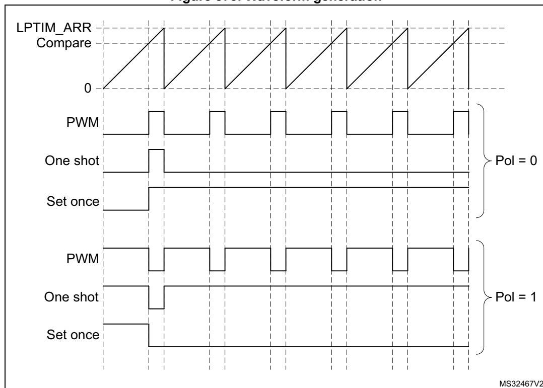
Figure 573. Waveform generation
