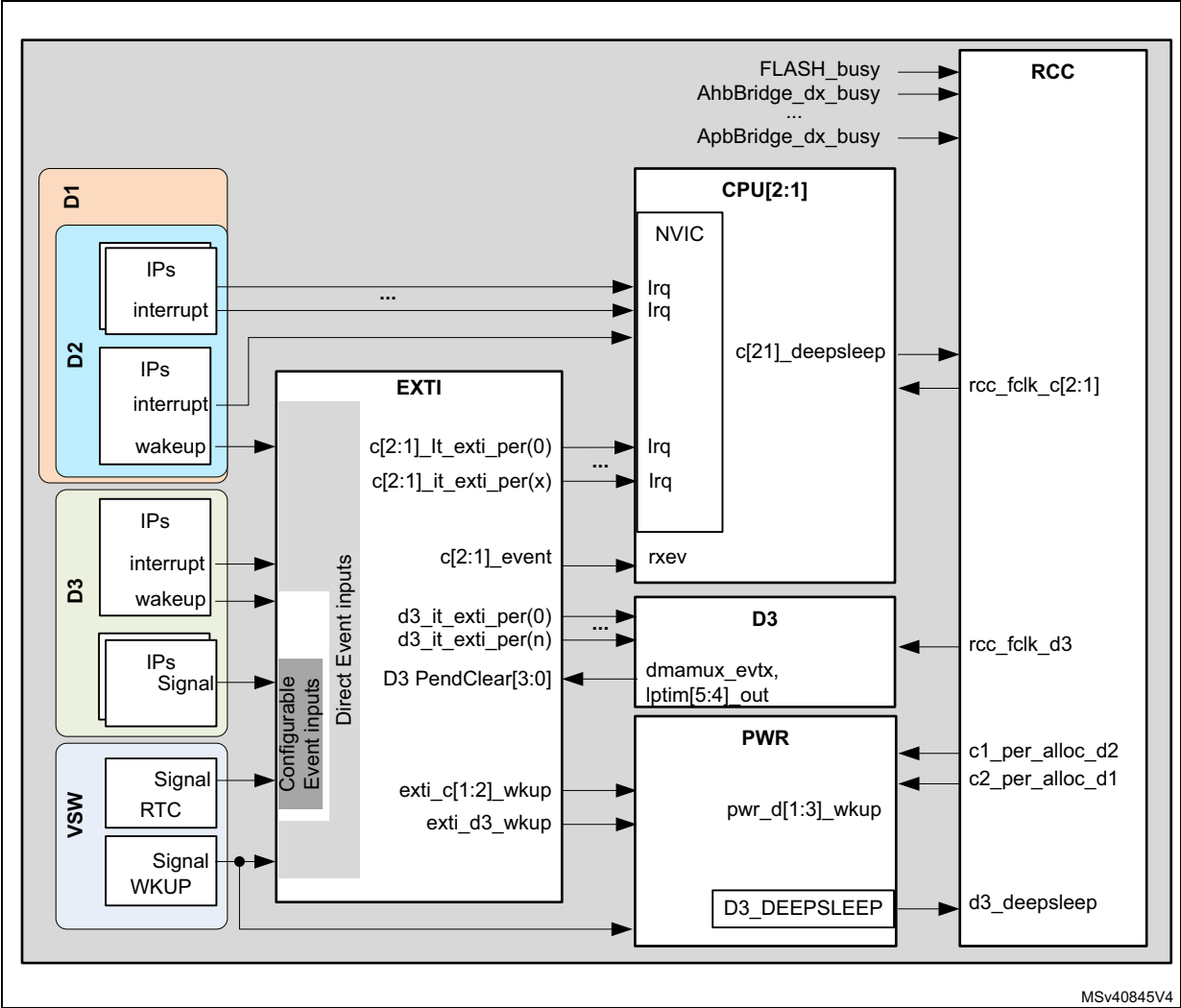
Figure 44. EXTI, RCC and PWR interconnections
