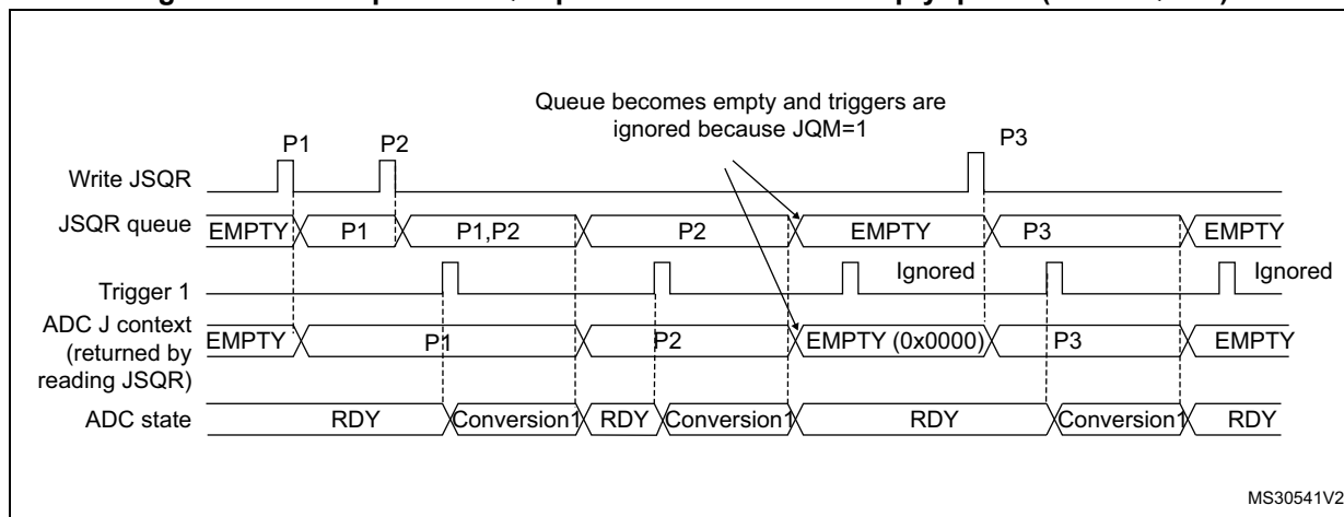
Figure 160. Example of JSQR queue of context with empty queue (case JQM=1)
