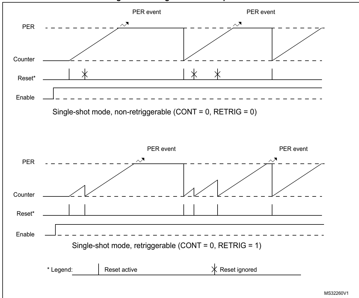
Figure 326. Single-shot timer operation
