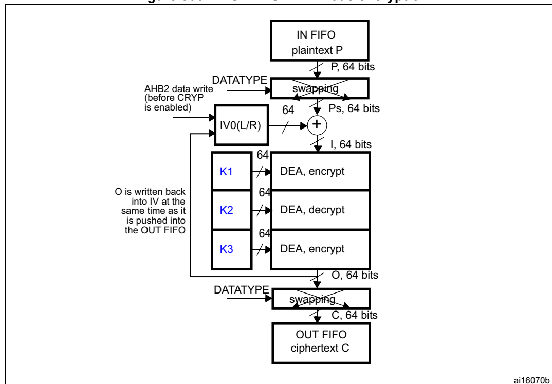
Figure 306. DES/TDES-CBC mode encryption
