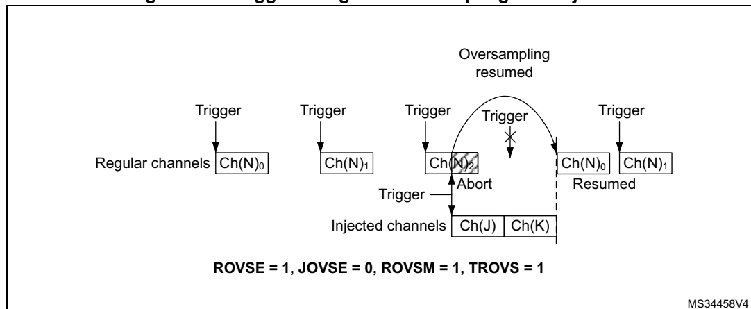
Figure 191. Triggered regular oversampling with injection
