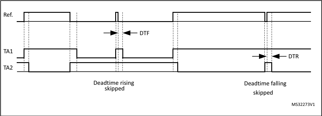
Figure 339. Complementary outputs for low pulse width (SDTRx = SDTFx = 1)
