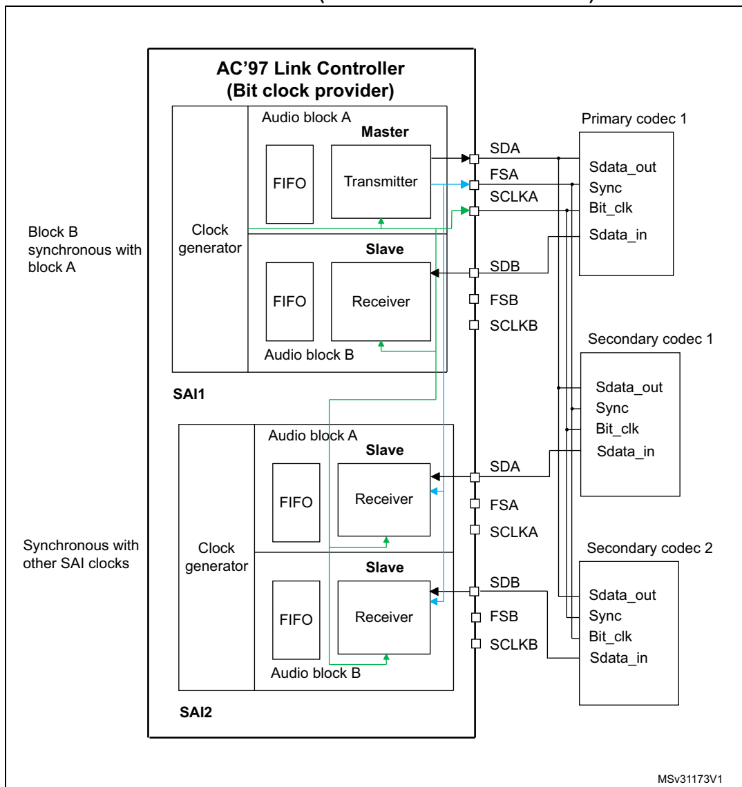
Figure 703. Example of typical AC'97 configuration on devices featuring at least 2 embedded SAIs (three external AC'97 decoders)
