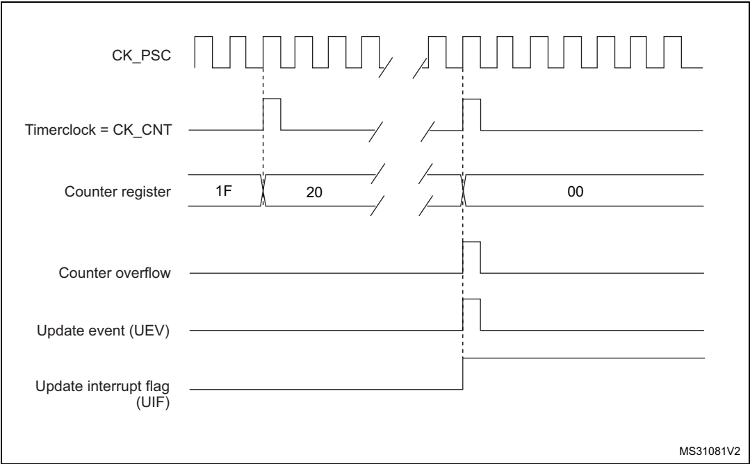
Figure 503. Counter timing diagram, internal clock divided by N
