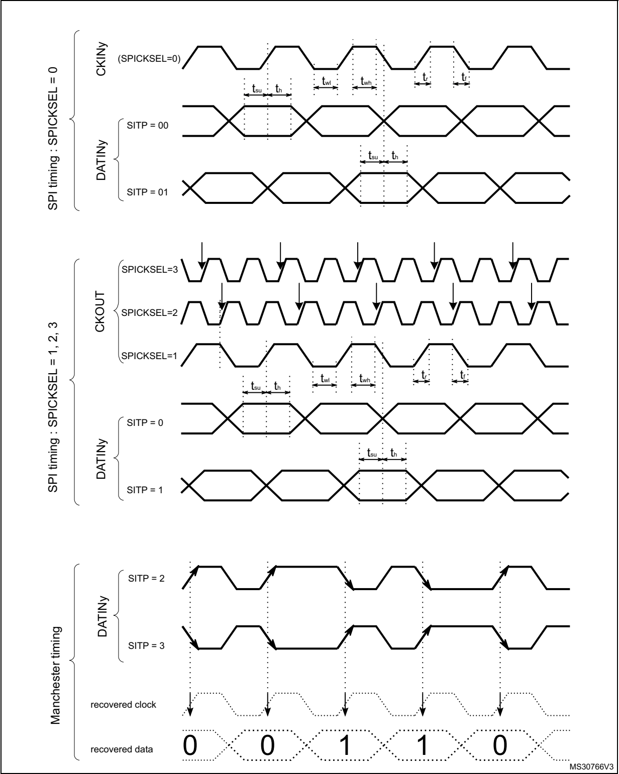
Figure 236. Channel transceiver timing diagrams
