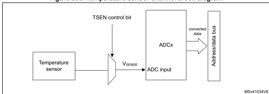
Figure 209. Temperature sensor channel block diagram
