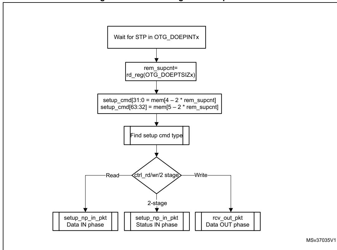
Figure 817. Processing a SETUP packet
