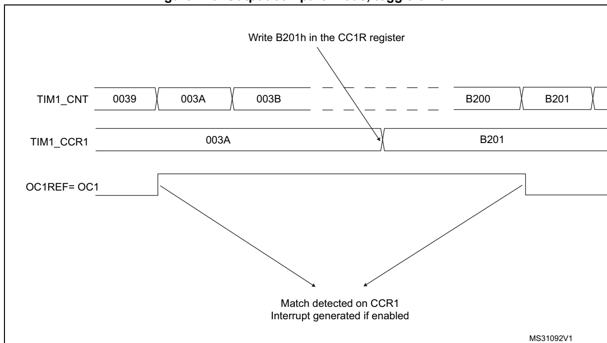
Figure 420. Output compare mode, toggle on OC1
