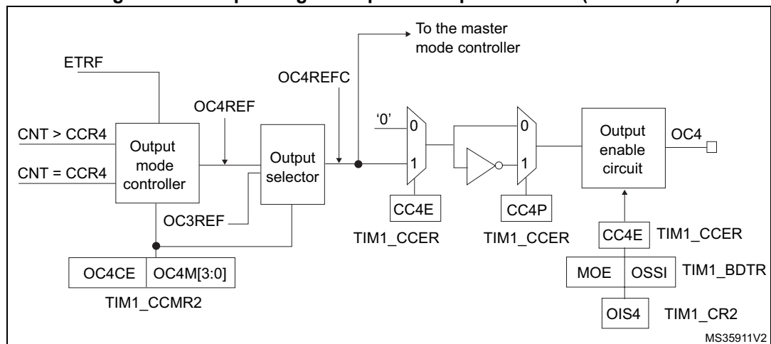
Figure 417. Output stage of capture/compare channel (channel 4)
