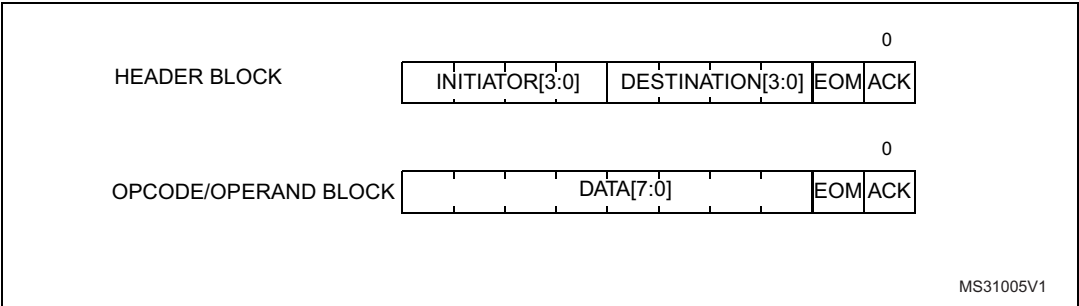
Figure 862. Blocks
