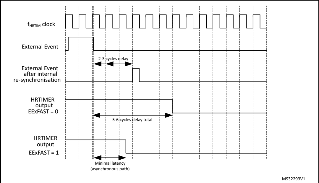
Figure 345. Latency to external events (output reset on external event)
