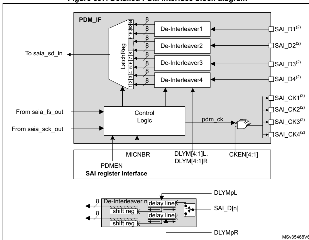
Figure 697. Detailed PDM interface block diagram
