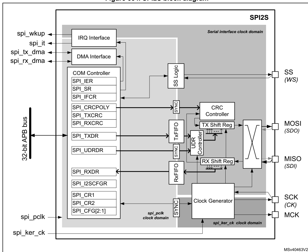
Figure 654. SPI2S block diagram
