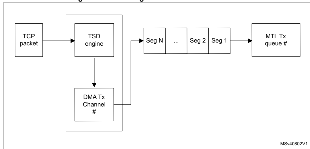
Figure 834. TCP segmentation offload overview
