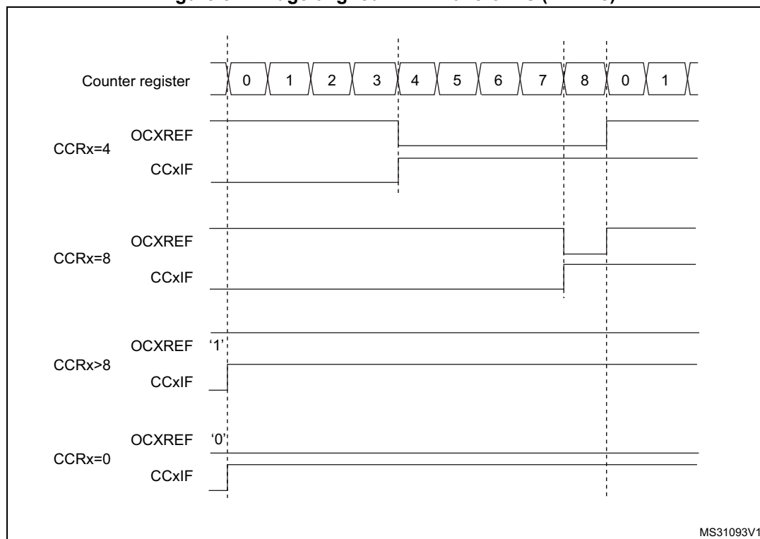
Figure 542. Edge-aligned PWM waveforms (ARR=8)
