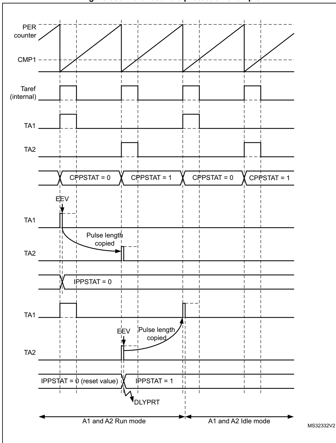
Figure 356. Balanced Idle protection example
