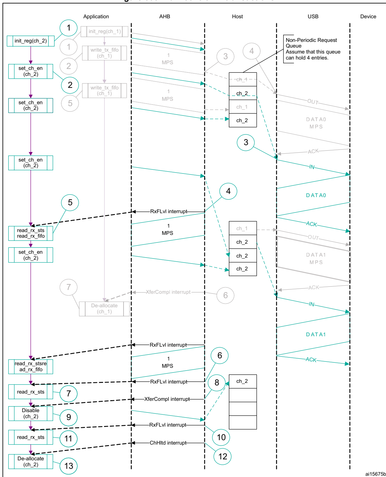
Figure 805. Bulk/control IN transactions
