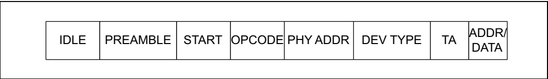
Figure 839. MDIO packet structure (Clause 45)
