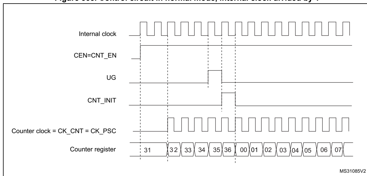
Figure 565. Control circuit in normal mode, internal clock divided by 1
