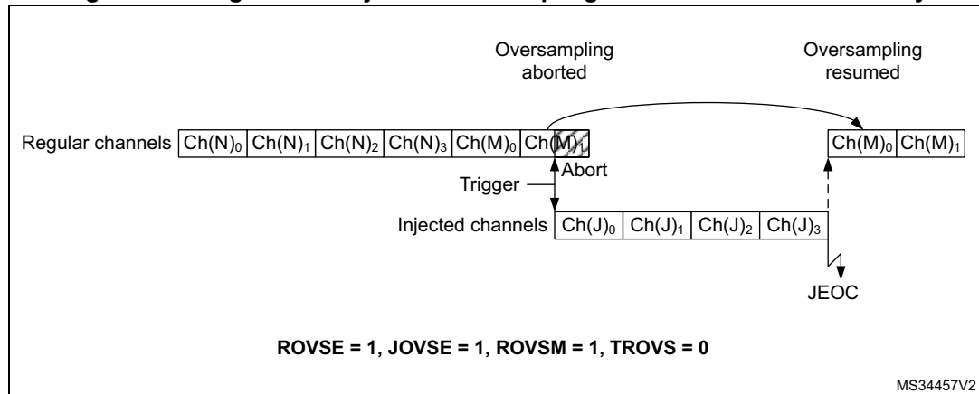
Figure 190. Regular and injected oversampling modes used simultaneously
