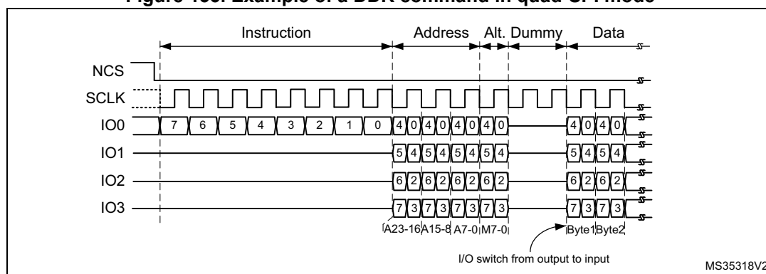
Figure 135. Example of a DDR command in quad-SPI mode
