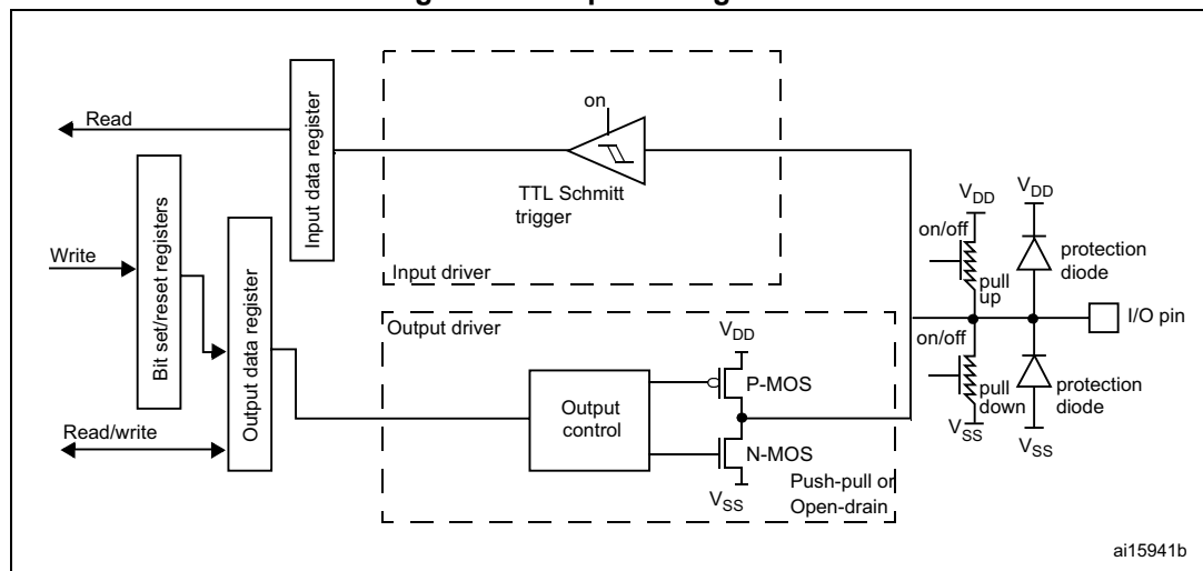
Figure 79. Output configuration
