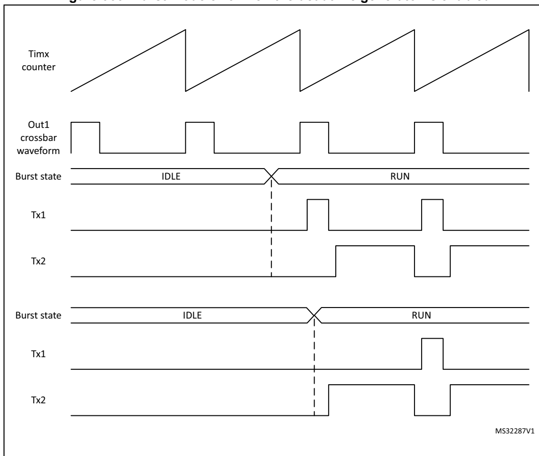
Figure 363. Burst mode exit when the deadtime generator is enabled
