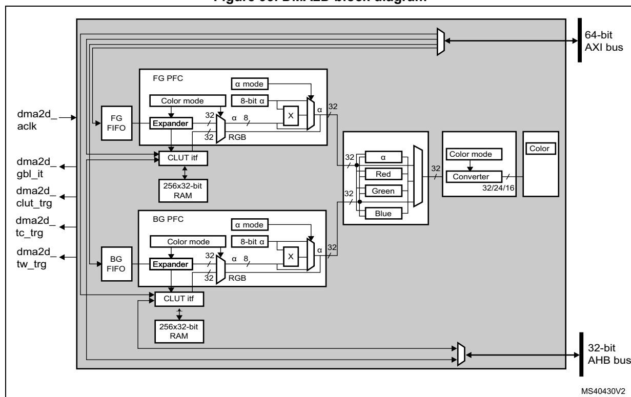
Figure 93. DMA2D block diagram
