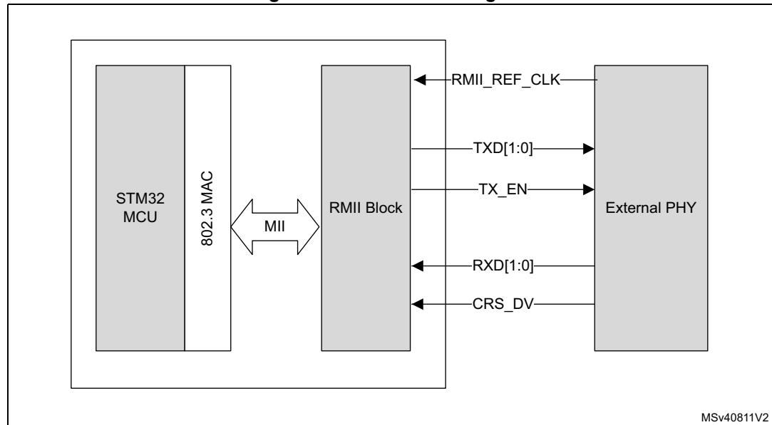
Figure 845. RMII block diagram
