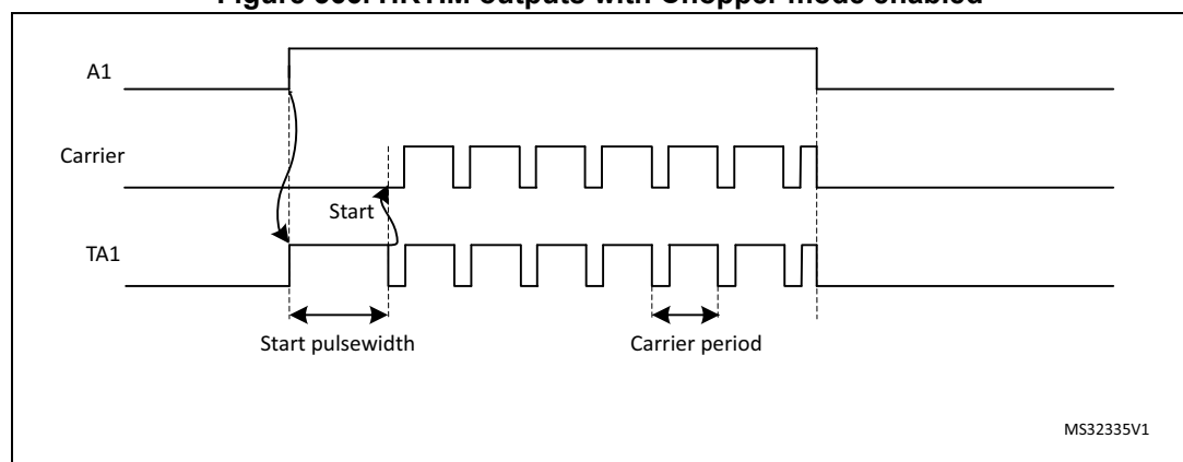
Figure 366. HRTIM outputs with Chopper mode enabled
