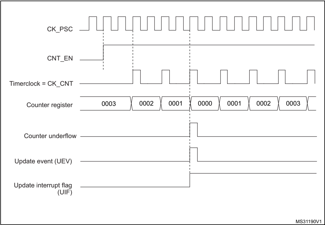
Figure 401. Counter timing diagram, internal clock divided by 2
