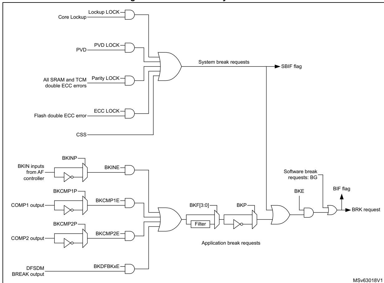
Figure 547. Break circuitry overview
