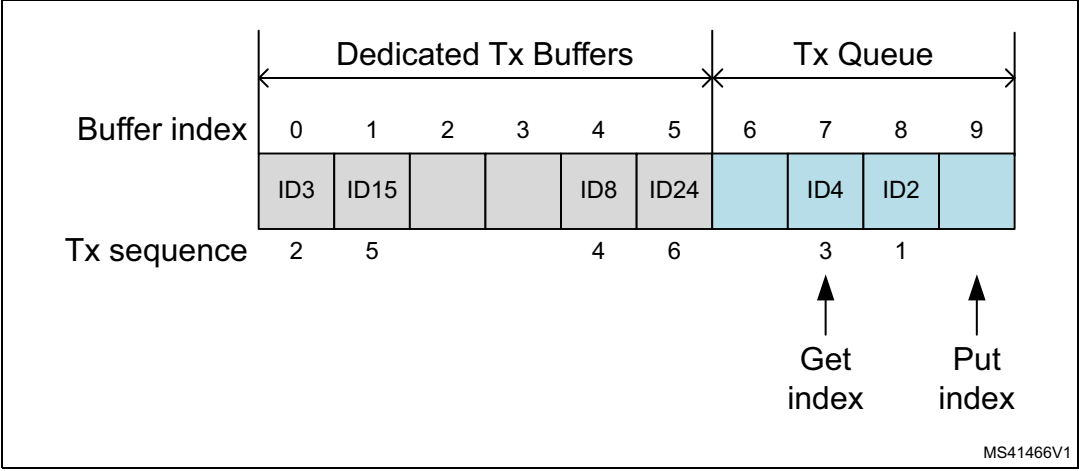
Figure 784. Example of mixed configuration dedicated Tx buffers / Tx queue
