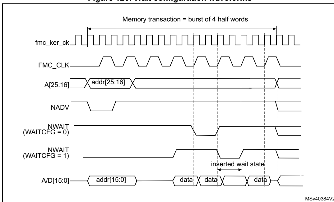
Figure 120. Wait configuration waveforms
