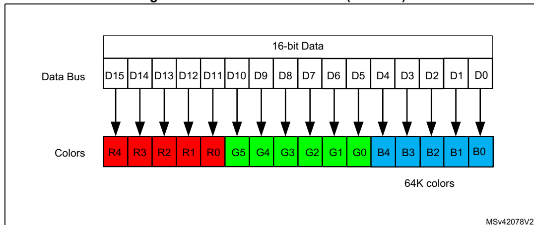
Figure 94. Intel 8080 16-bit mode (RGB565)
