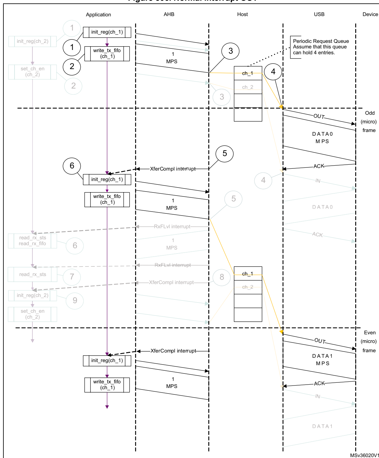
Figure 806. Normal interrupt OUT
