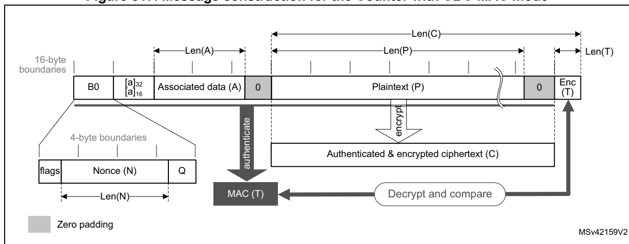
Figure 317. Message construction for the Counter with CBC-MAC mode
