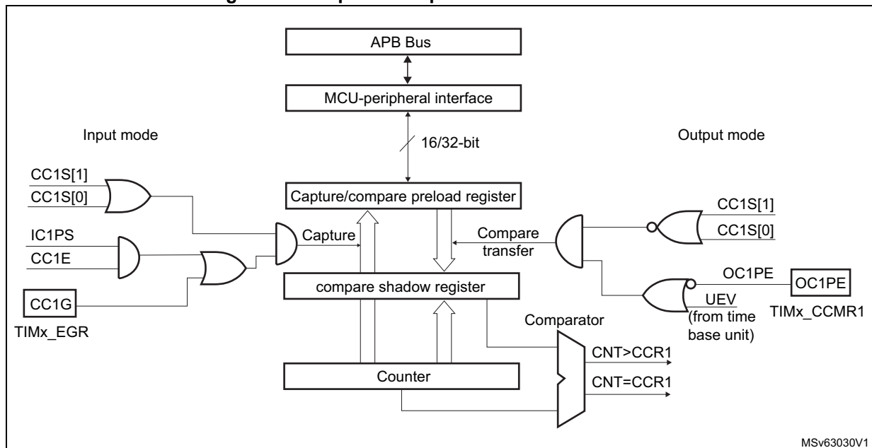
Figure 510. Capture/compare channel 1 main circuit
