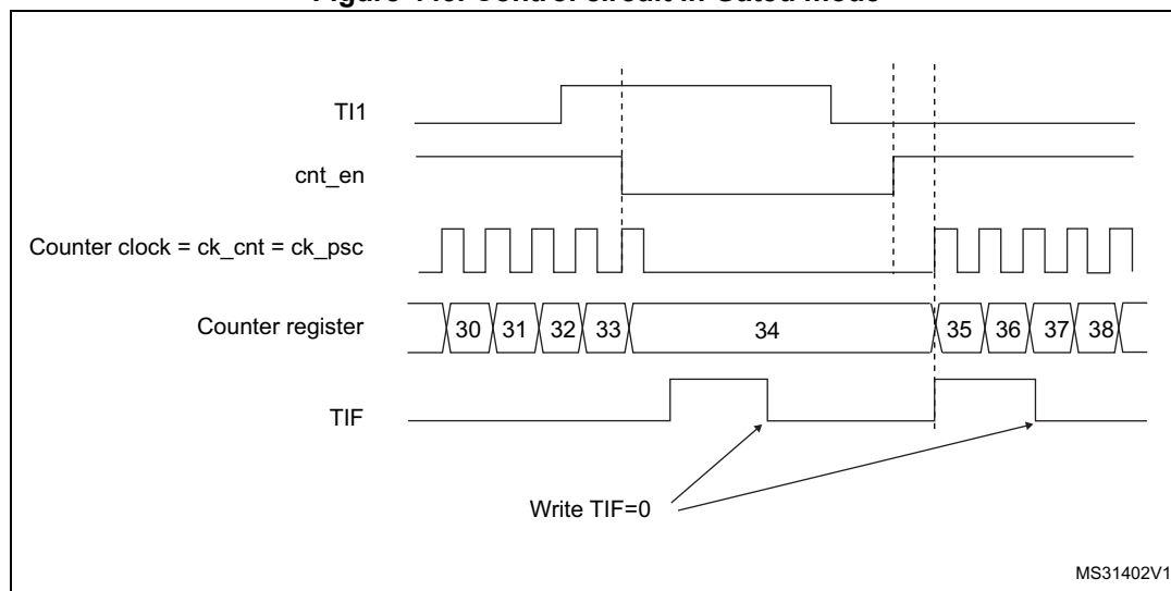
Figure 443. Control circuit in Gated mode
