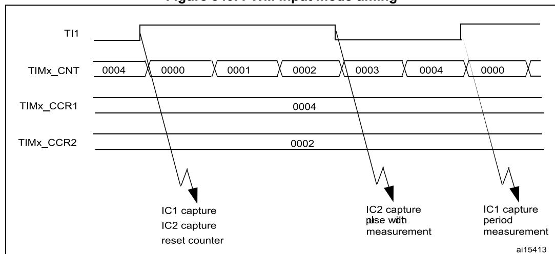
Figure 540. PWM input mode timing
