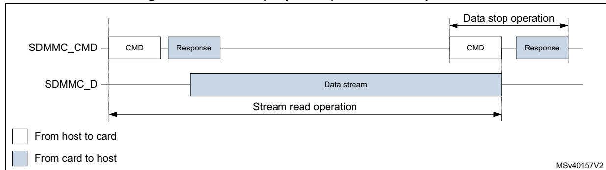
Figure 745. SDMMC (sequential) stream read operation
