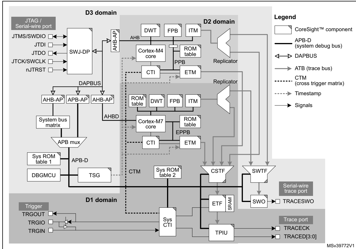
Figure 871. Power domains of debug infrastructure
