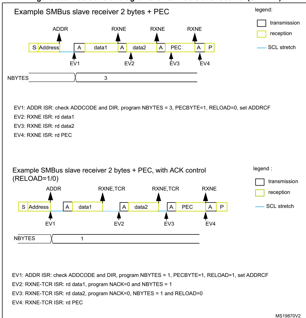
Figure 609. Bus transfer diagrams for SMBus slave receiver (SBC = 1)
