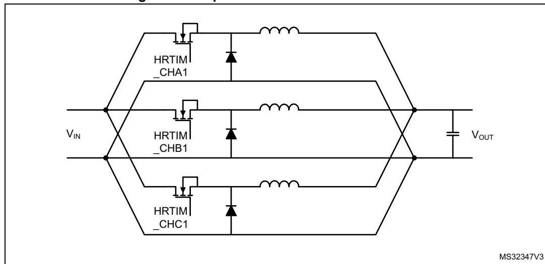
Figure 382. 3-phase interleaved buck converter
