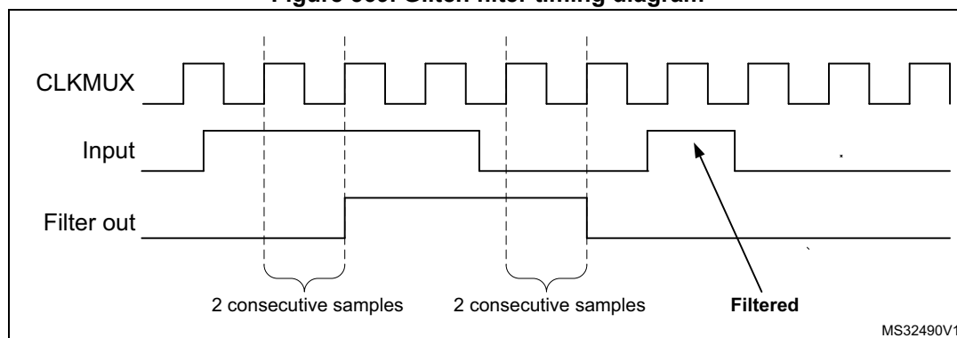
Figure 569. Glitch filter timing diagram
