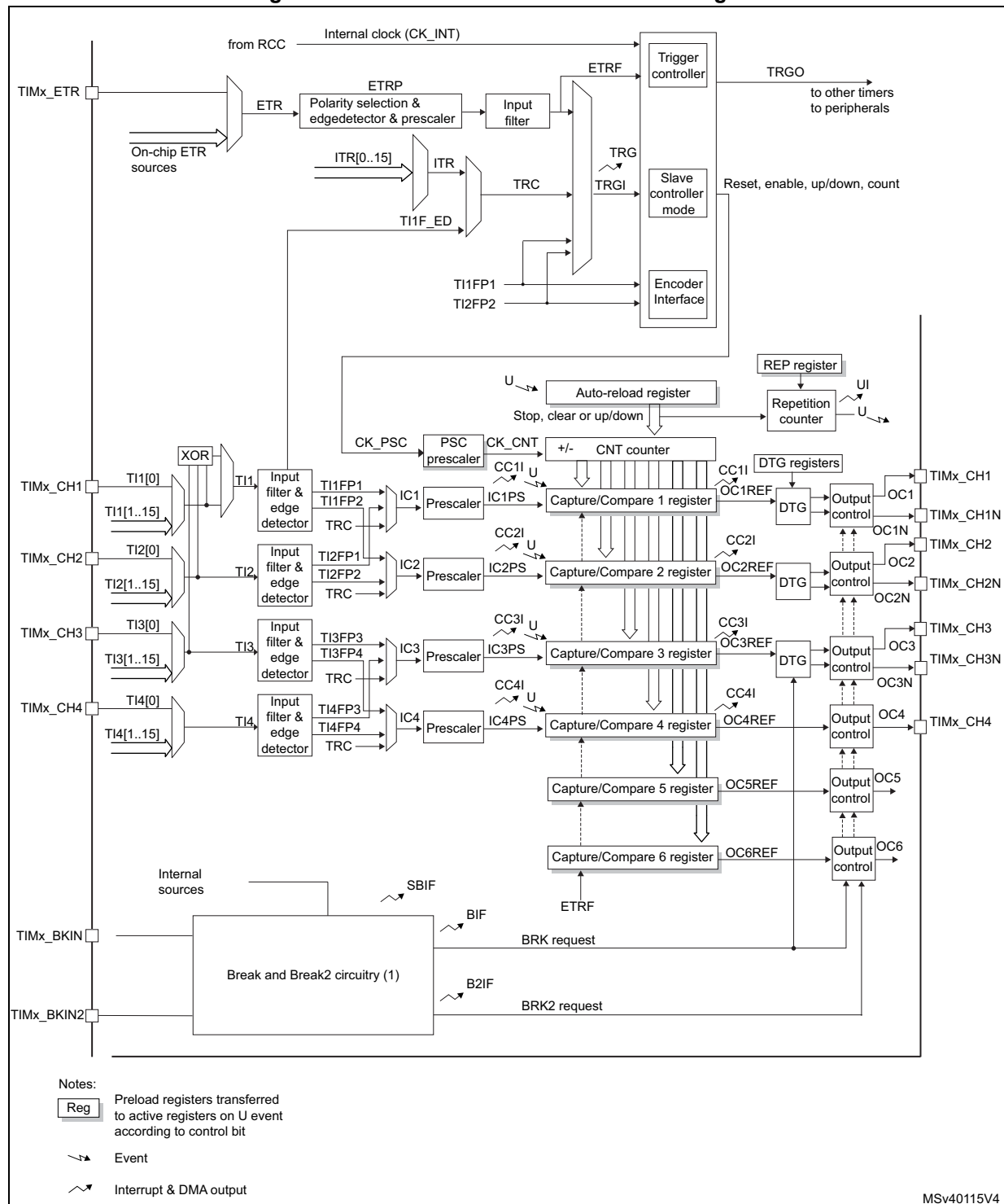
Figure 386. Advanced-control timer block diagram
