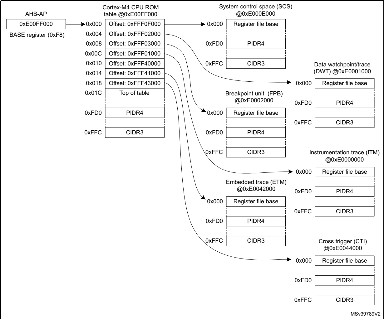
Figure 883. Cortex-M4 CoreSight Topology
