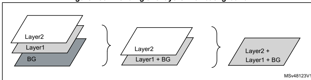
Figure 253. Blending two layers with background
