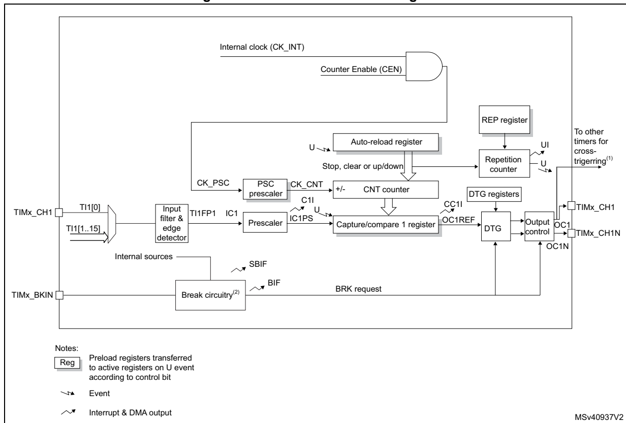
Figure 523. TIM16/TIM17 block diagram
