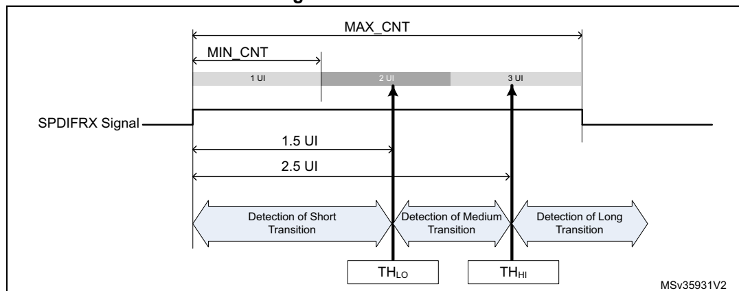
Figure 718. Thresholds
