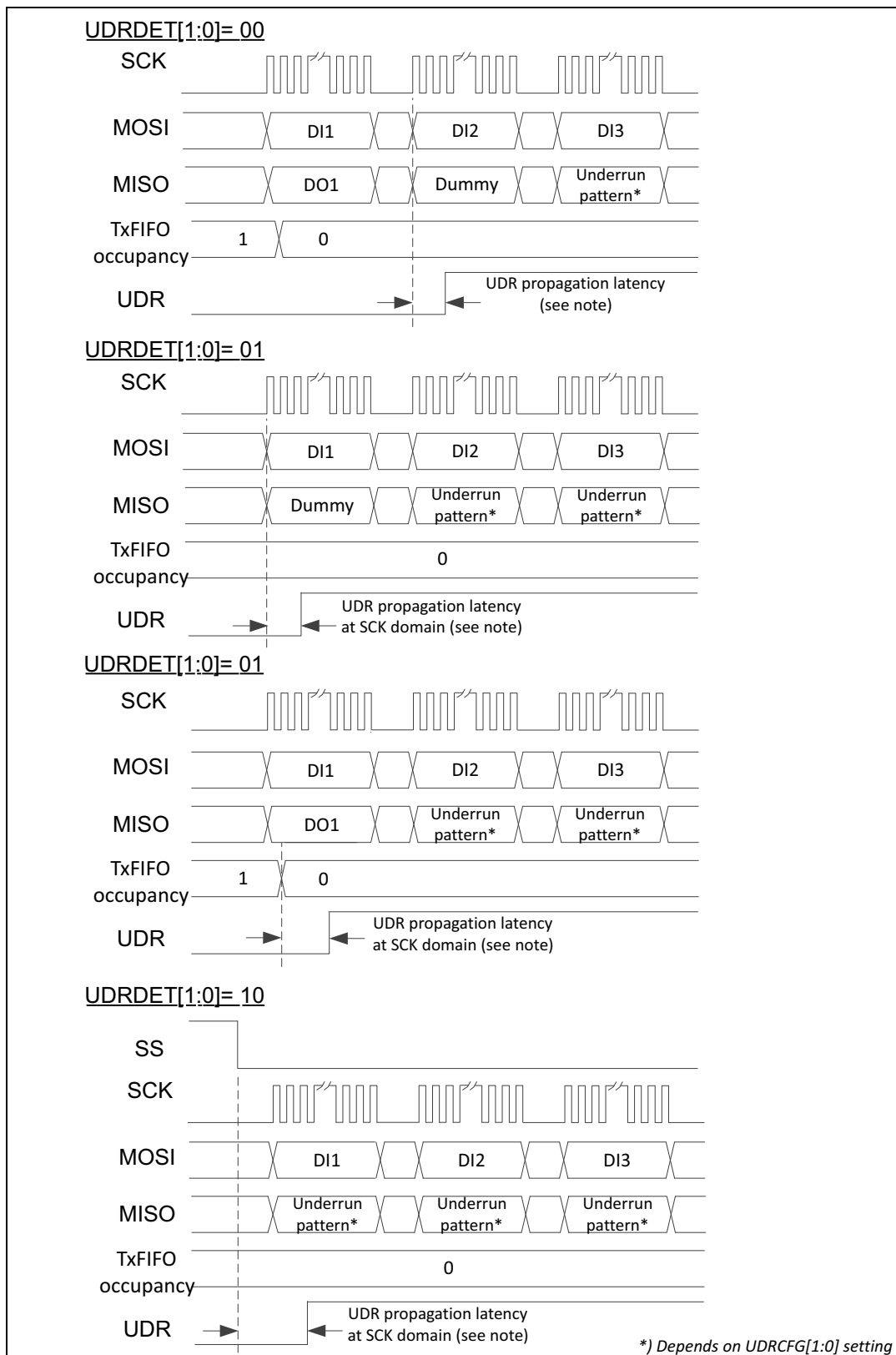
Figure 668. Optional configurations of slave behavior at detection of underrun condition
