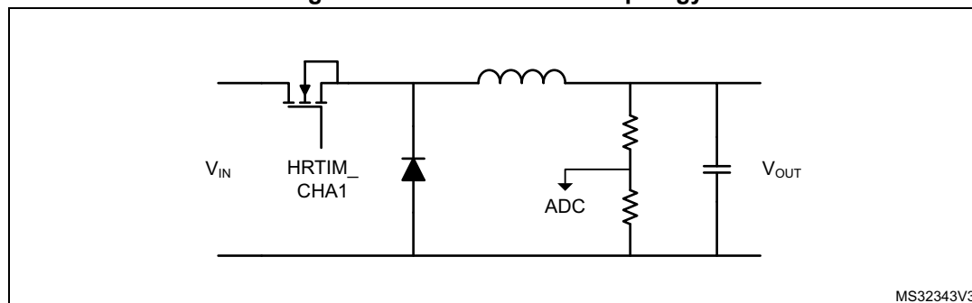
Figure 378. Buck converter topology
