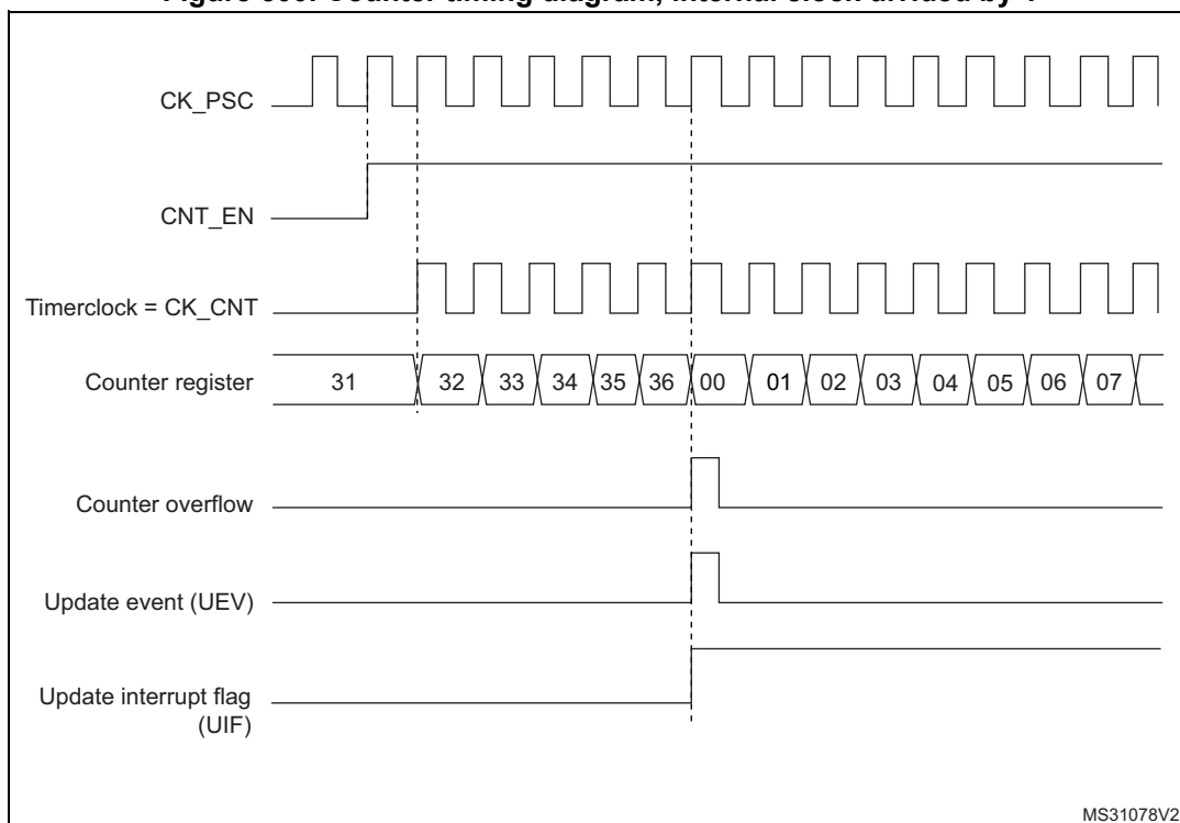
Figure 500. Counter timing diagram, internal clock divided by 1
