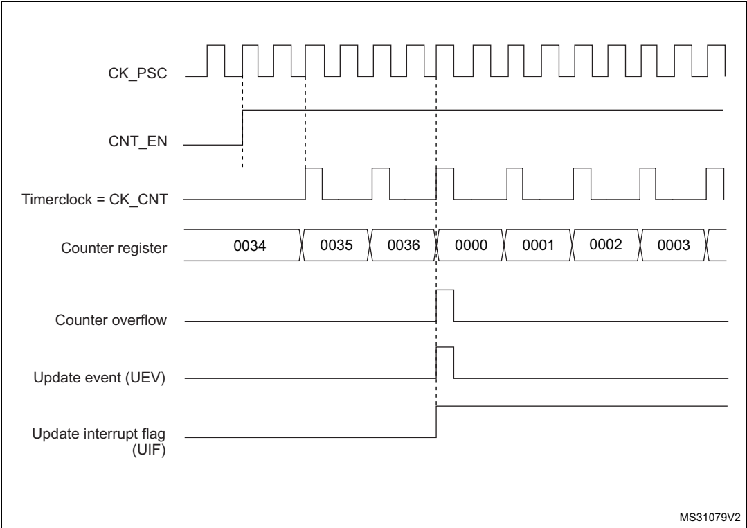
Figure 527. Counter timing diagram, internal clock divided by 2
