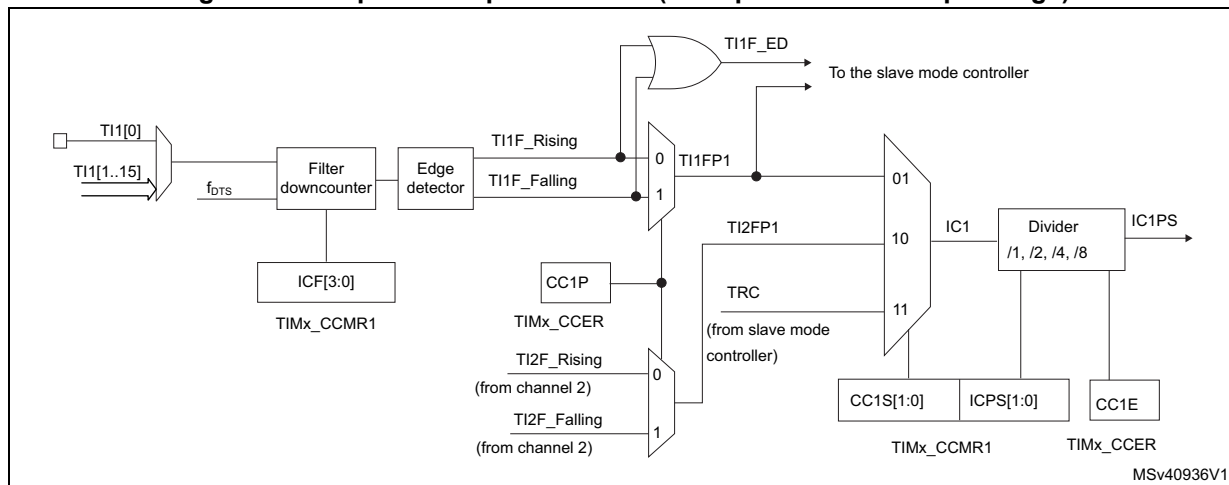
Figure 536. Capture/compare channel (example: channel 1 input stage)
