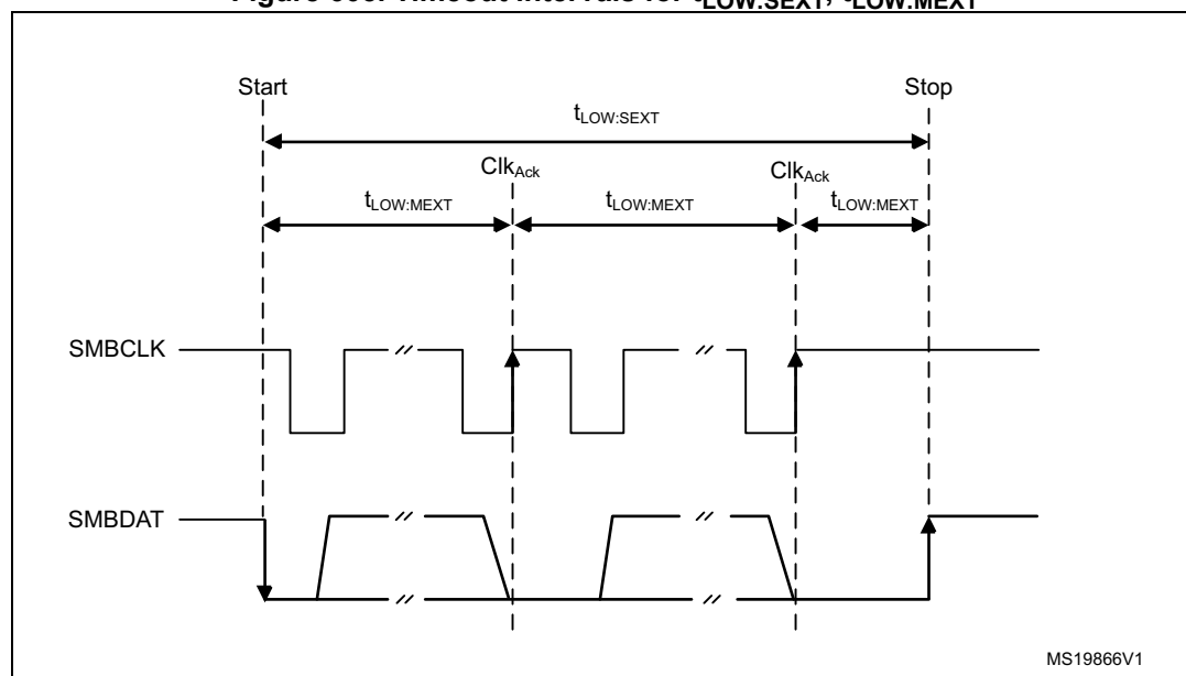
Figure 605. Timeout intervals for t_{\text{LOW:SEXT}} , t_{\text{LOW:MEXT}}
