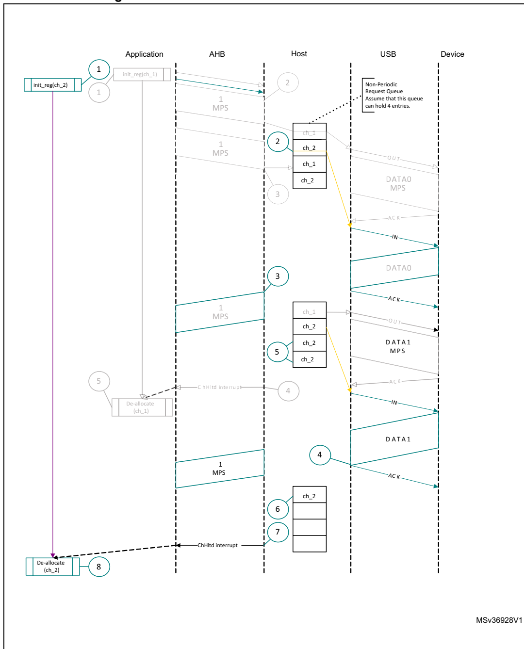
Figure 811. Normal bulk/control IN transaction - DMA
