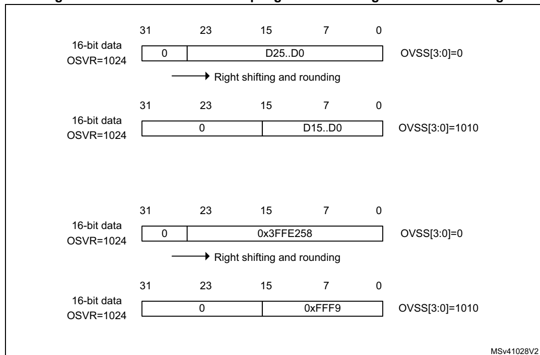
Figure 187. 16-bit result oversampling with 10-bits right shift and rounding
