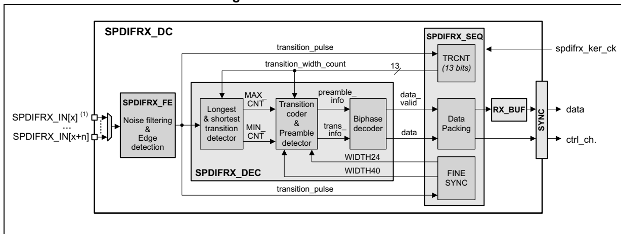
Figure 716. SPDIFRX decoder
