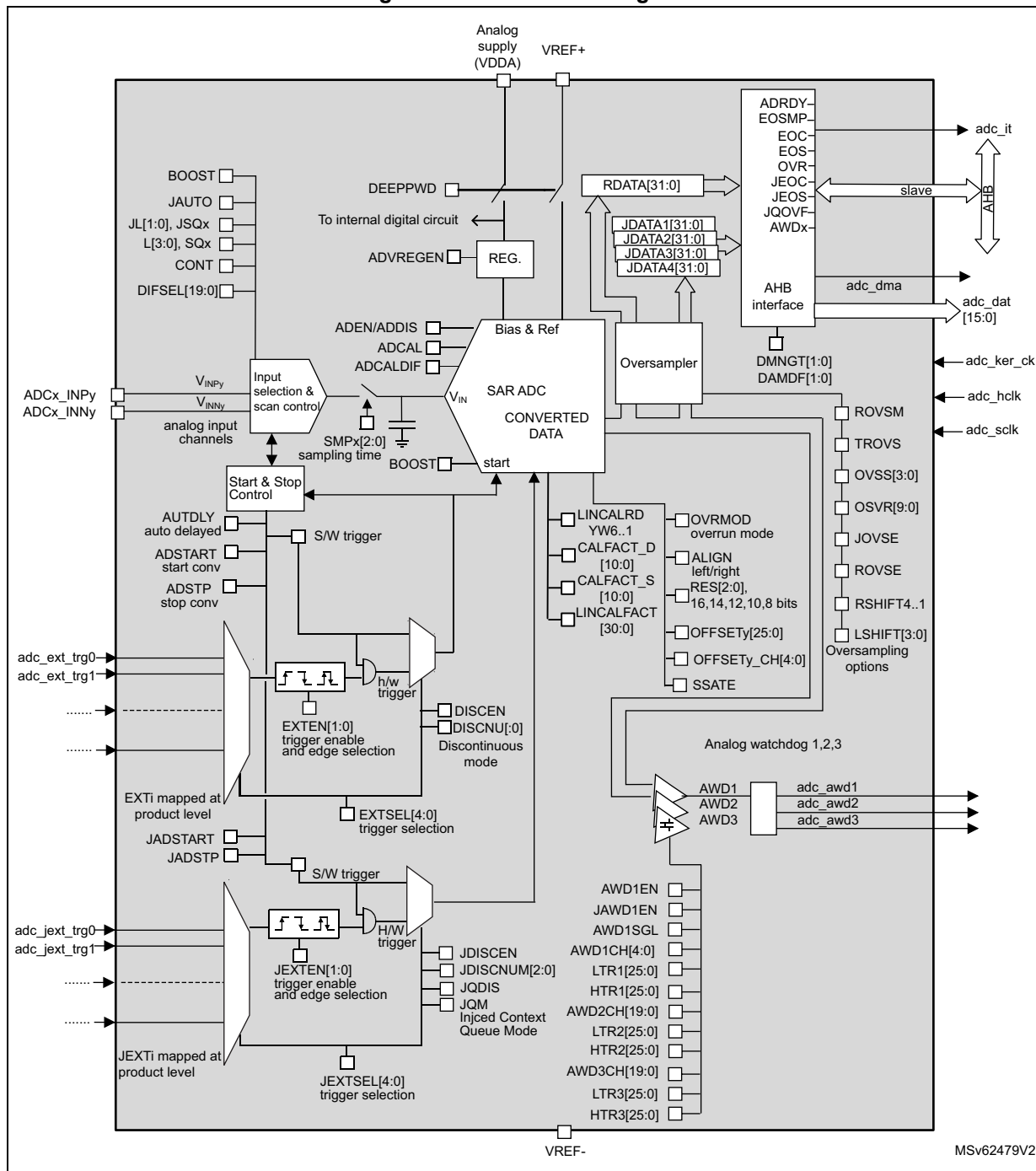
Figure 141. ADC block diagram
