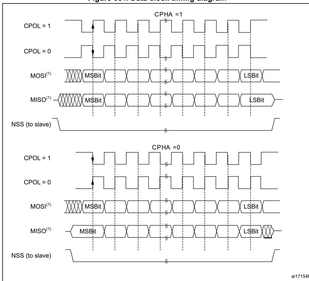
Figure 664. Data clock timing diagram
