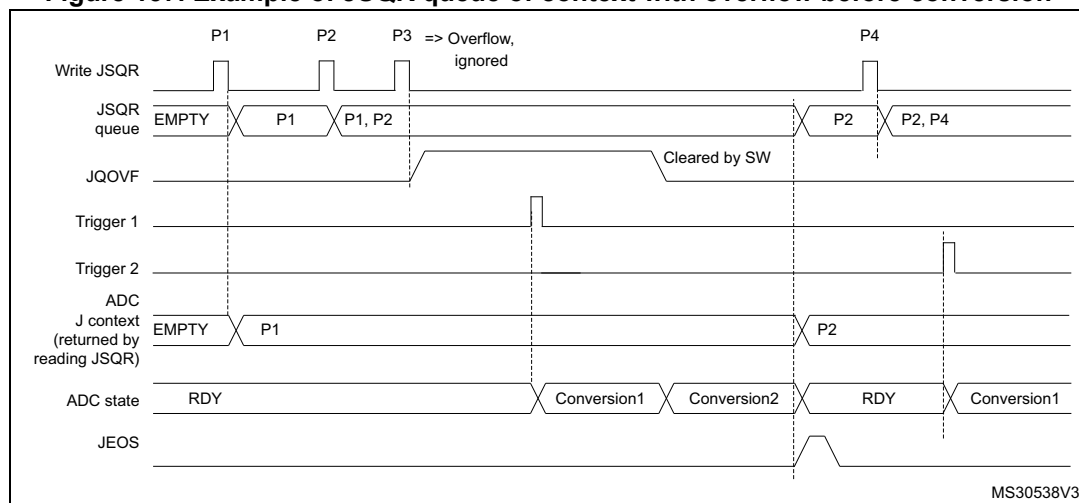
Figure 157. Example of JSQR queue of context with overflow before conversion
