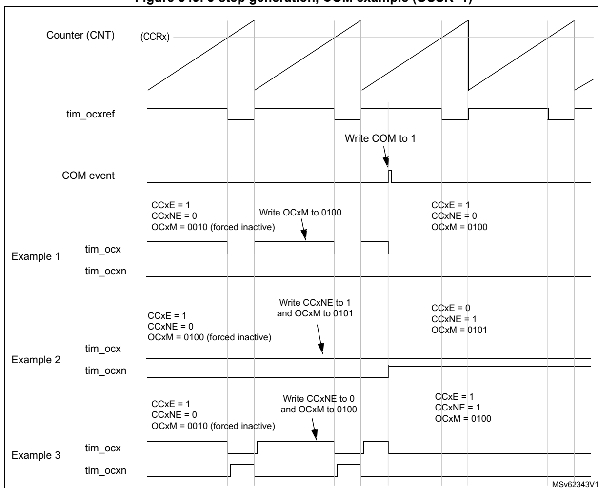
Figure 549. 6-step generation, COM example (OSSR=1)
