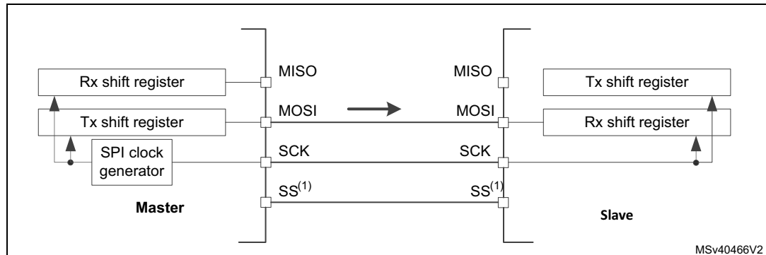
Figure 657. Simplex single master/single slave application (master in transmit-only/ slave in receive-only mode)
