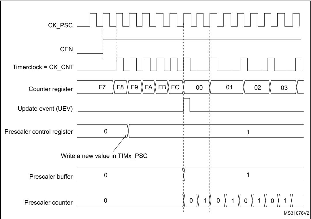
Figure 387. Counter timing diagram with prescaler division change from 1 to 2
