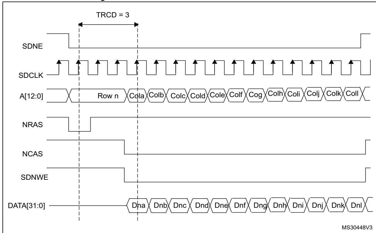
Figure 125. Burst write SDRAM access waveforms
