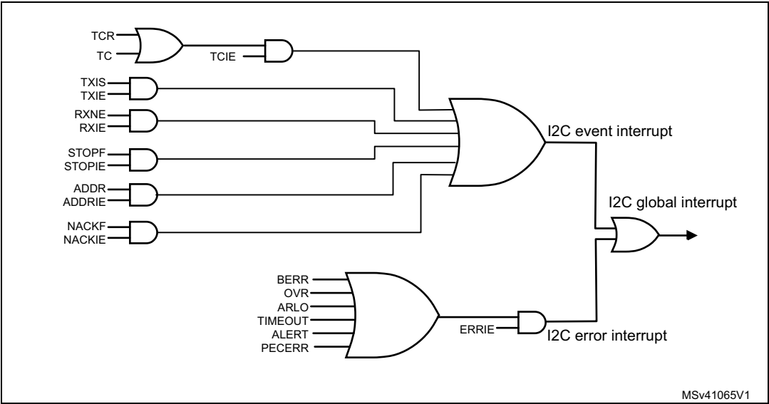
Figure 612. I2C interrupt mapping diagram
