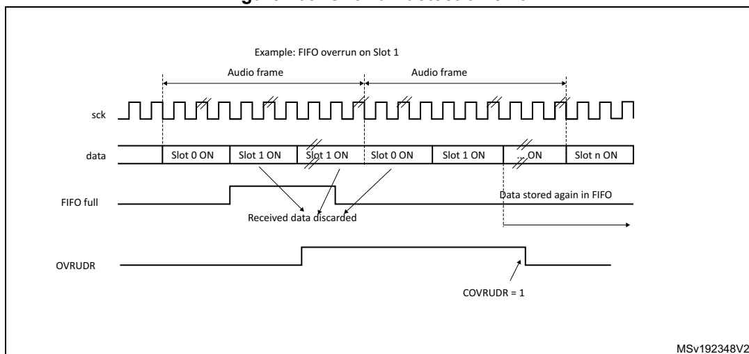
Figure 709. Overrun detection error
