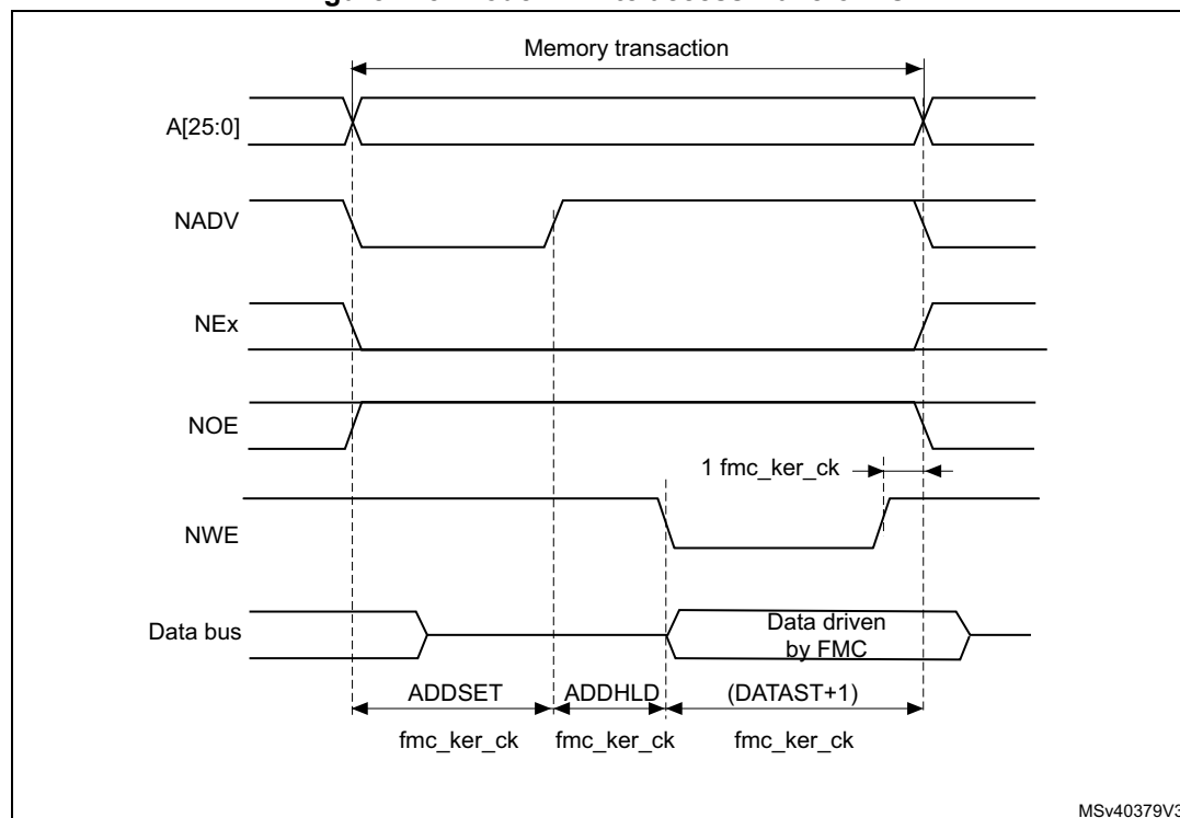
Figure 115. Mode D write access waveforms
