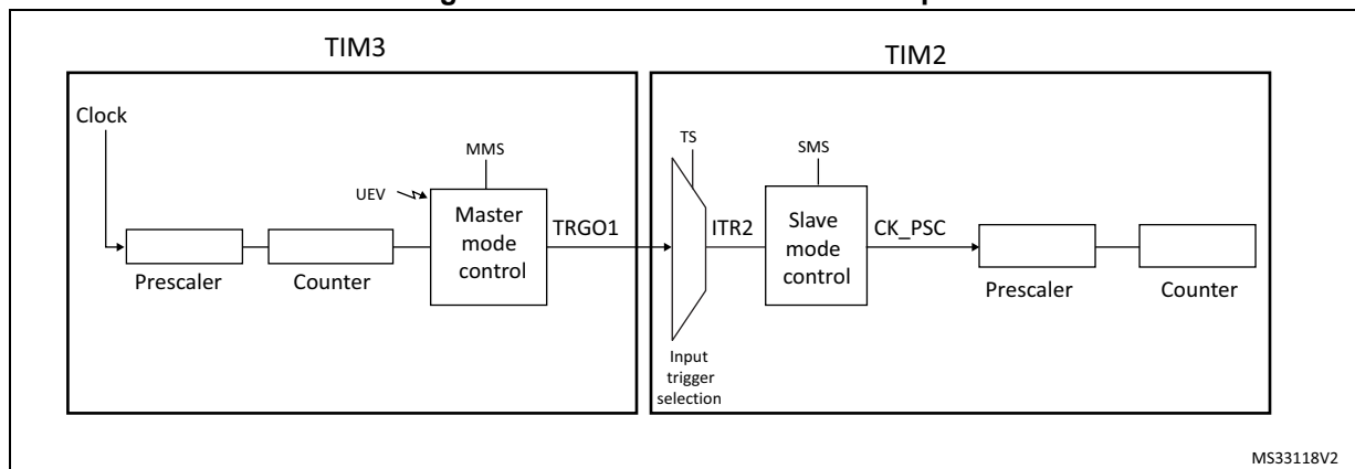
Figure 489. Master/Slave timer example
