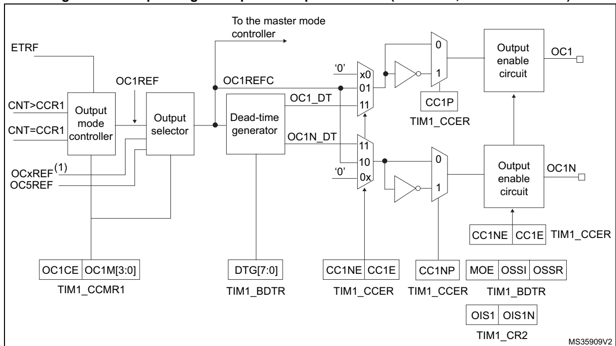
Figure 416. Output stage of capture/compare channel (channel 1, idem ch. 2 and 3)
