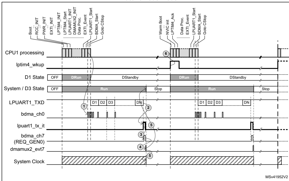
Figure 47. Timing diagram of LPUART1 transmission with D3 domain in Autonomous mode
