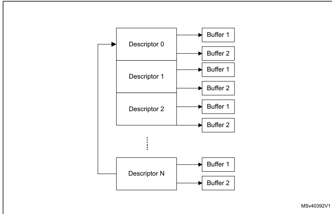
Figure 851. Descriptor ring structure
