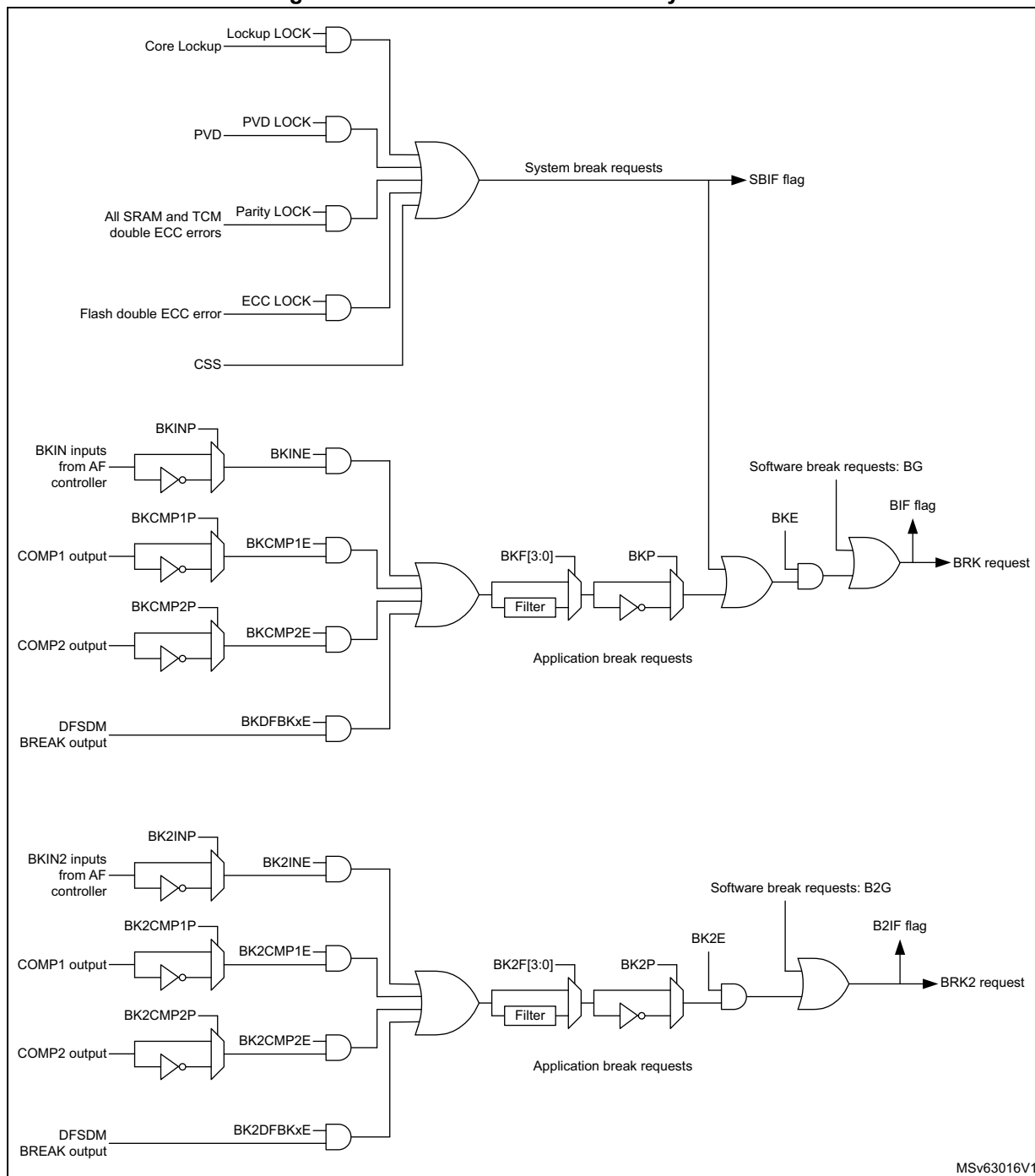
Figure 429. Break and Break2 circuitry overview
