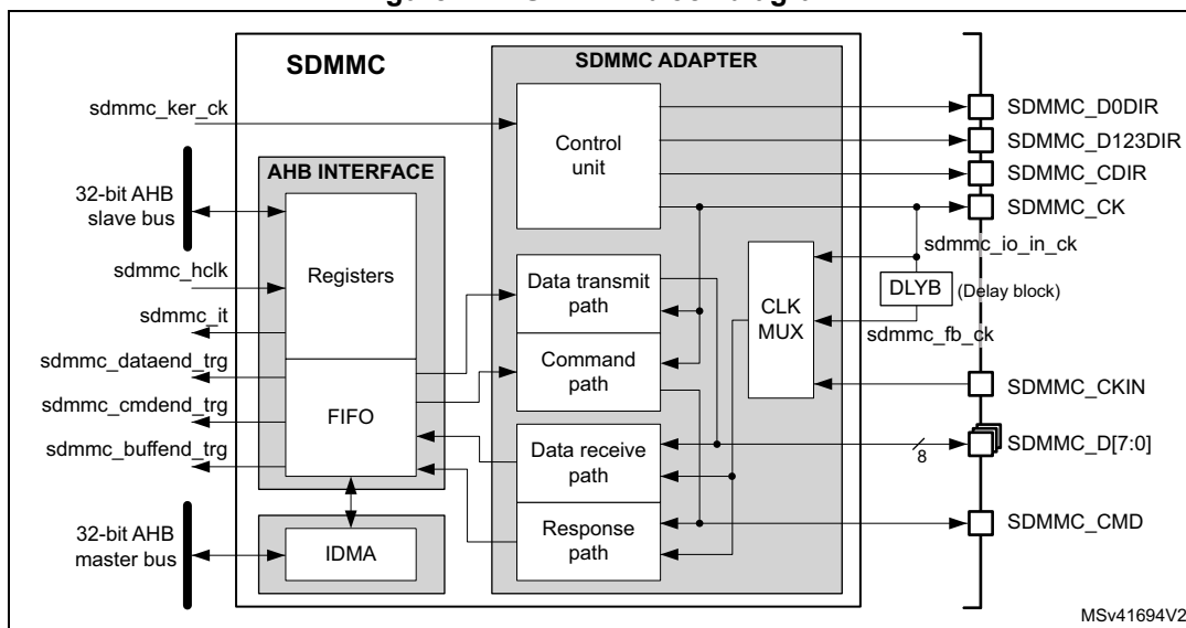
Figure 747. SDMMC block diagram
