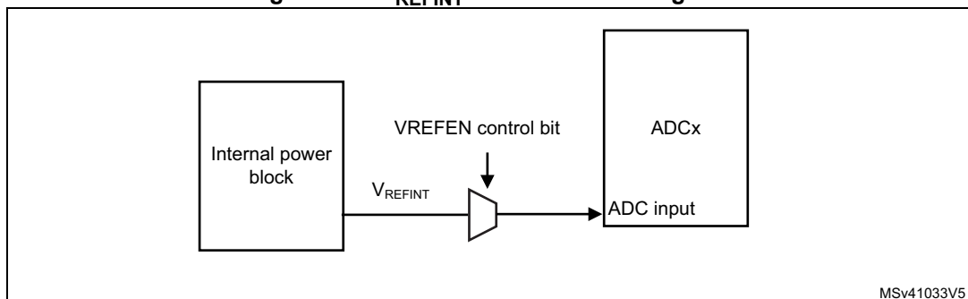
Figure 211. V_{REFINT} channel block diagram
