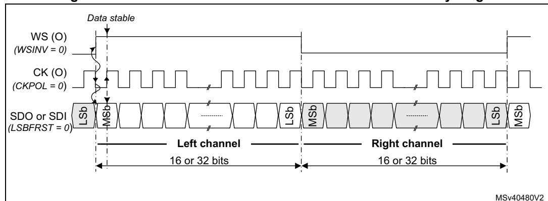
Figure 673. Master MSB Justified 16-bit or 32-bit full-accuracy length
