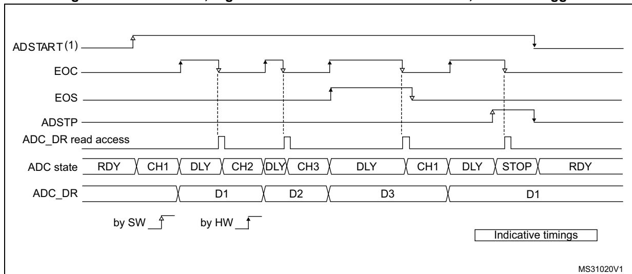
Figure 177. AUTDLY=1, regular conversion in continuous mode, software trigger
