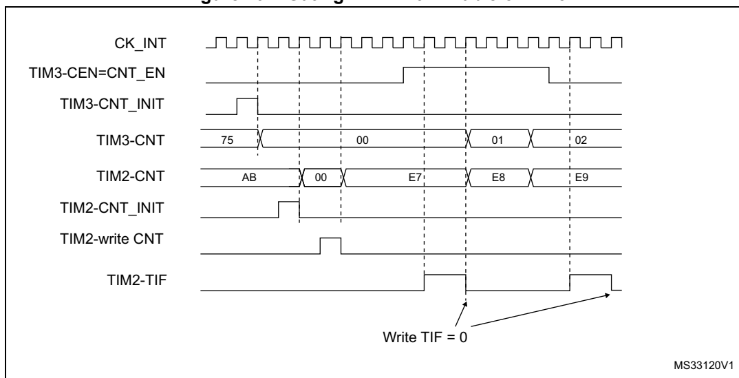
Figure 492. Gating TIM2 with Enable of TIM3
