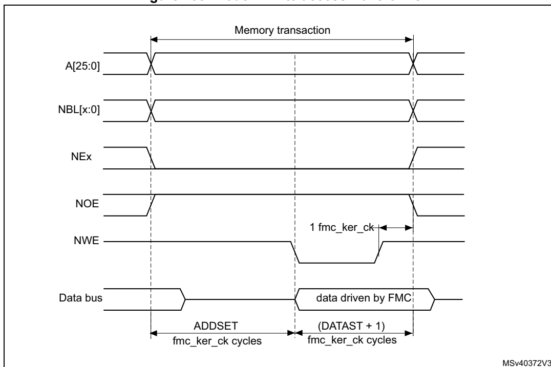
Figure 108. Mode A write access waveforms
