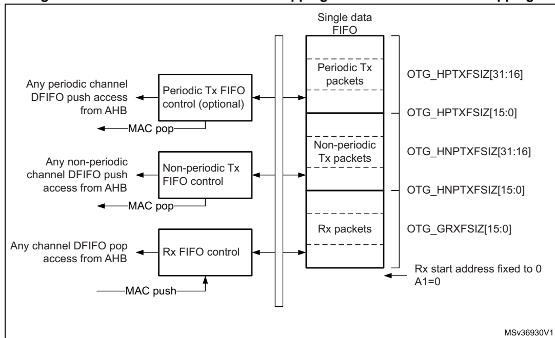
Figure 800. Host-mode FIFO address mapping and AHB FIFO access mapping
