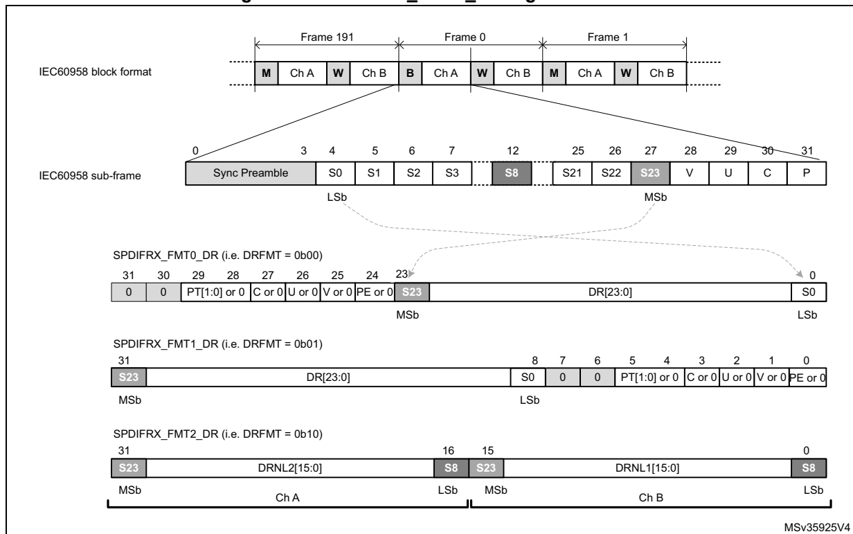
Figure 722. SPDIFRX_FMTx_DR register format
