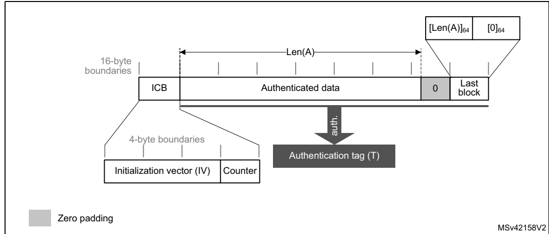
Figure 316. Message construction for the Galois Message Authentication Code mode
