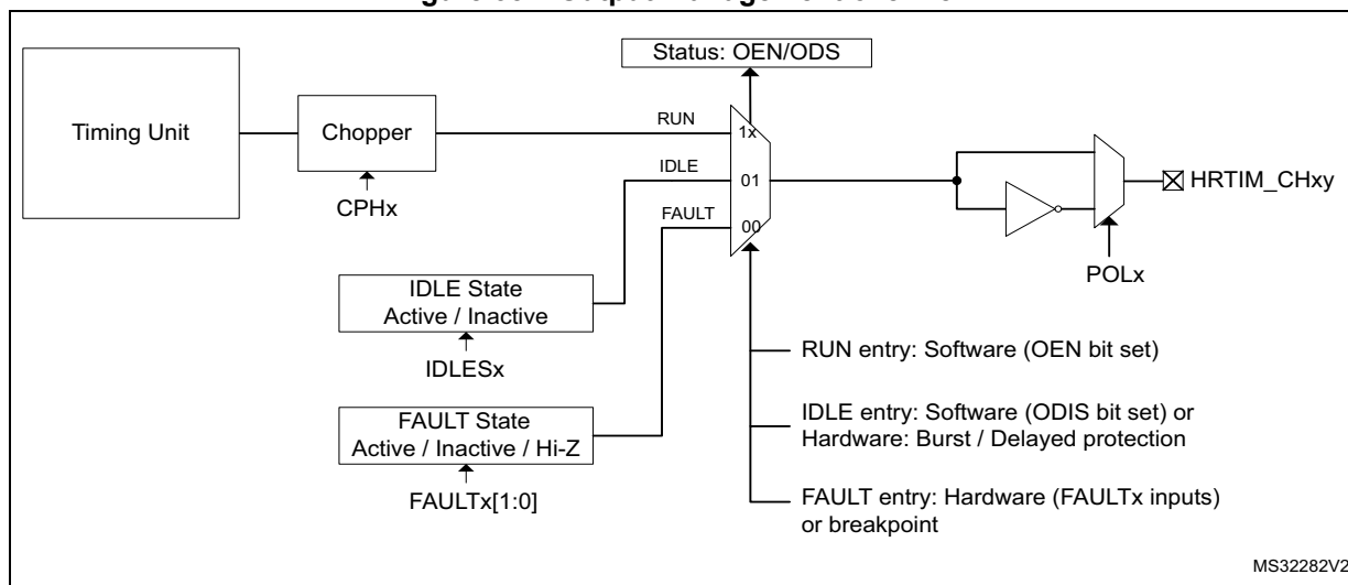
Figure 357. Output management overview
