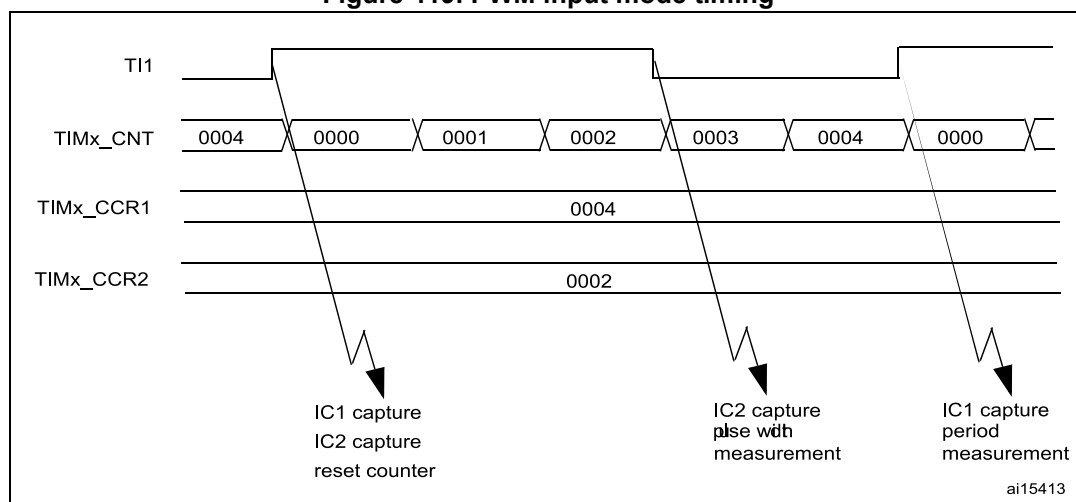
Figure 419. PWM input mode timing
