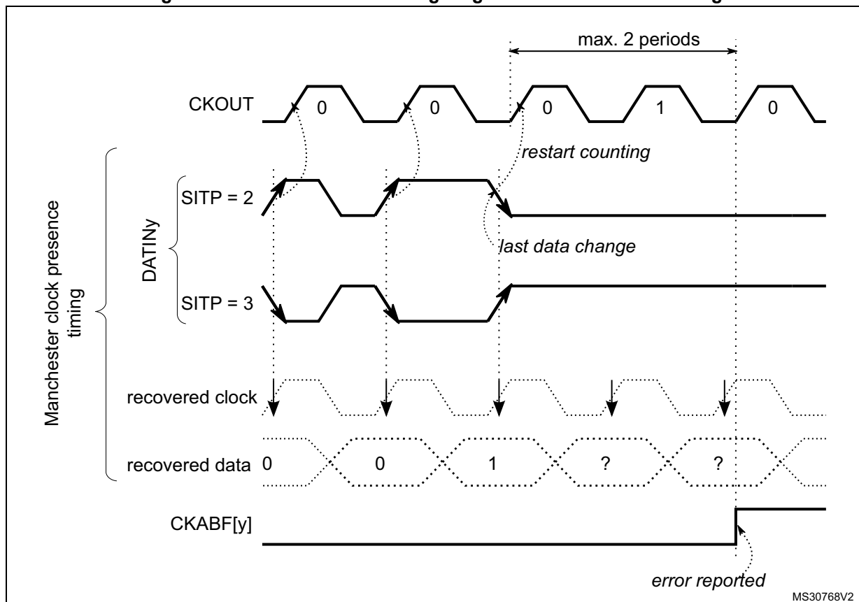
Figure 238. Clock absence timing diagram for Manchester coding
