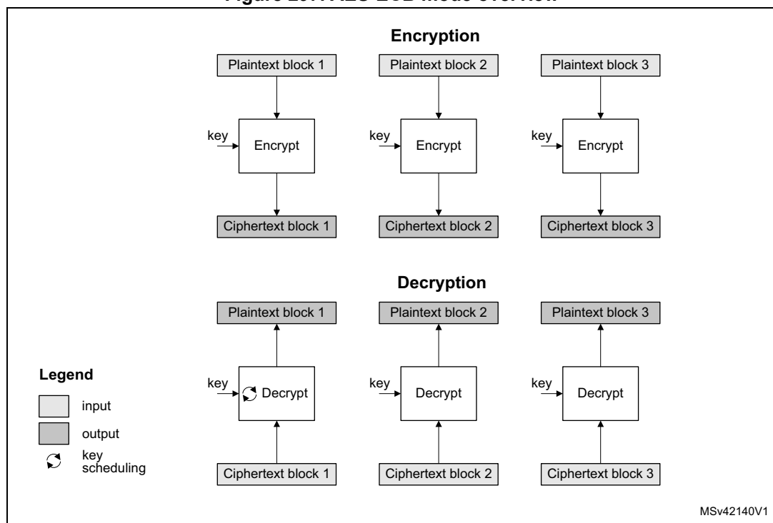
Figure 297. AES-ECB mode overview
