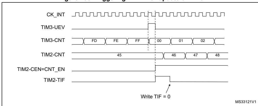
Figure 493. Triggering TIM2 with update of TIM3
