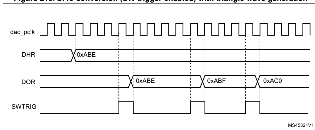
Figure 219. DAC conversion (SW trigger enabled) with triangle wave generation
