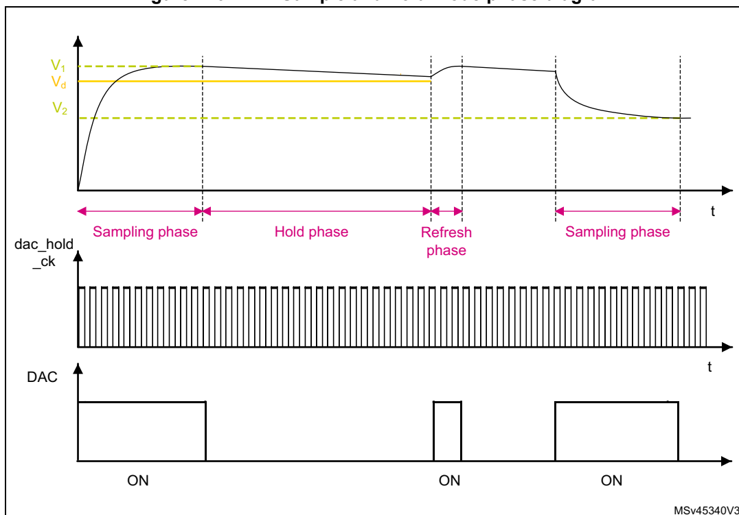
Figure 220. DAC Sample and hold mode phase diagram
