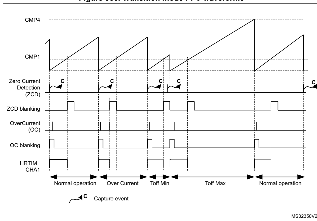
Figure 385. Transition mode PFC waveforms
