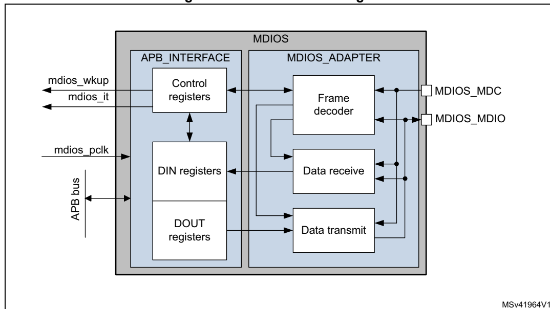
Figure 739. MDIOS block diagram
