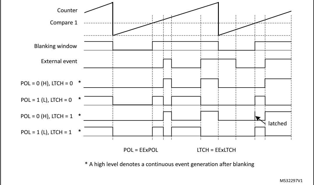
Figure 349. External trigger blanking, level sensitive triggering
