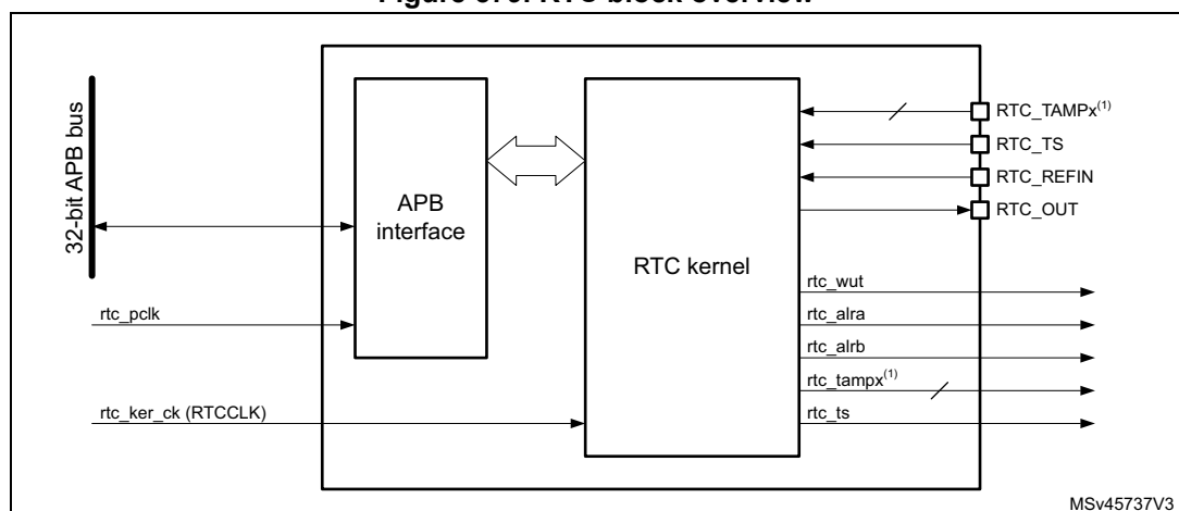
Figure 579. RTC block overview
