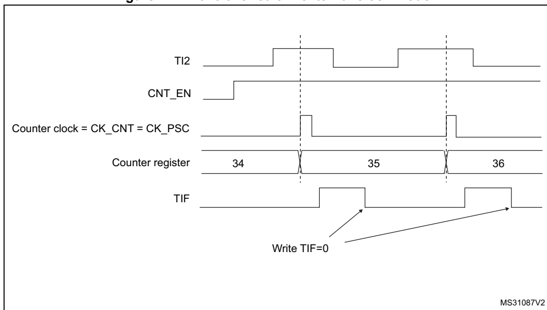
Figure 411. Control circuit in external clock mode 1
