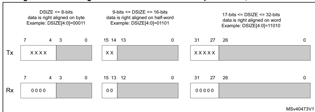
Figure 665. Data alignment when data size is not equal to 8-bit, 16-bit or 32-bit
