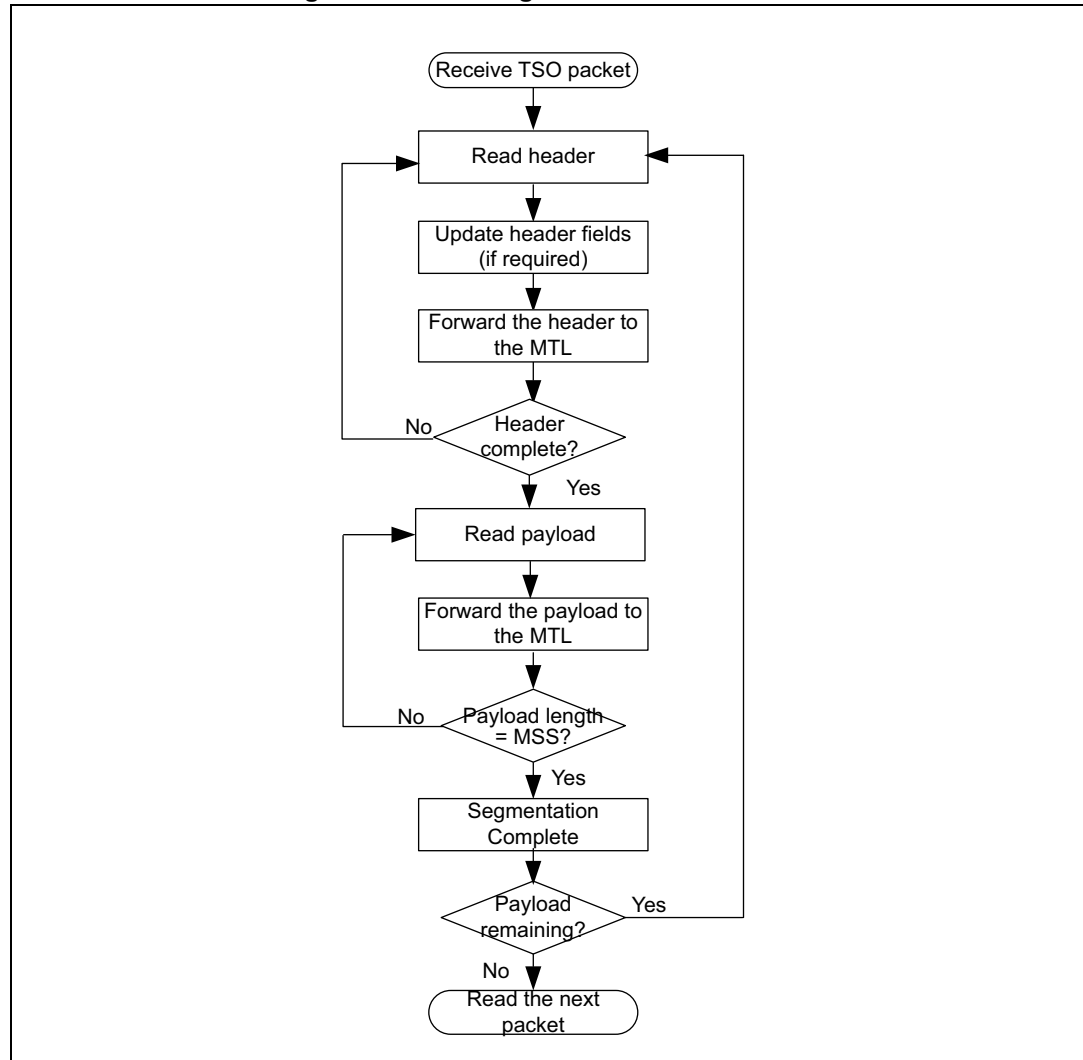
Figure 835. TCP segmentation offload flow
