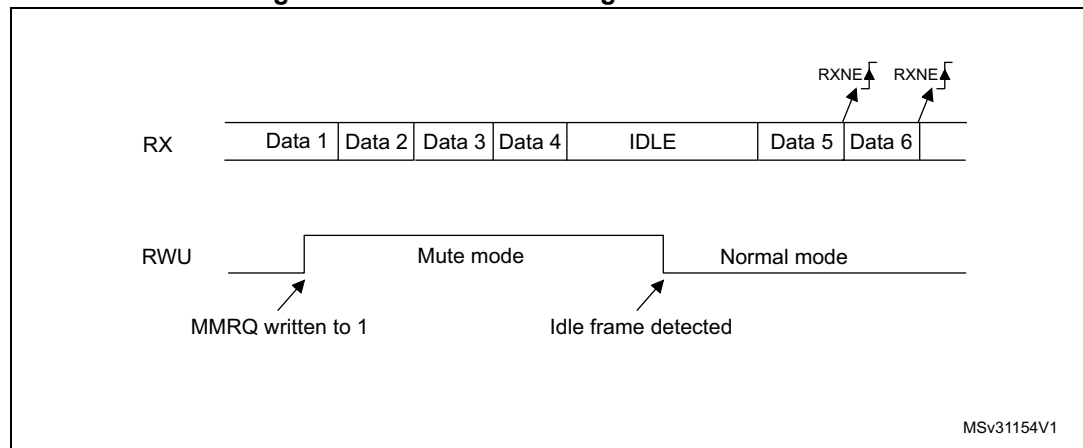
Figure 645. Mute mode using Idle line detection
