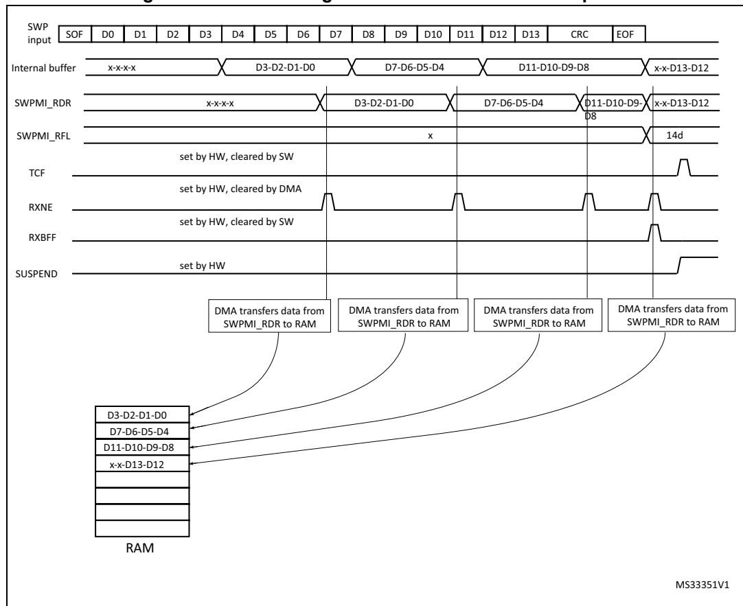
Figure 736. SWPMI single software buffer mode reception
