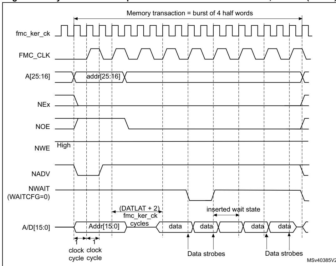
Figure 121. Synchronous multiplexed read mode waveforms - NOR, PSRAM (CRAM)
