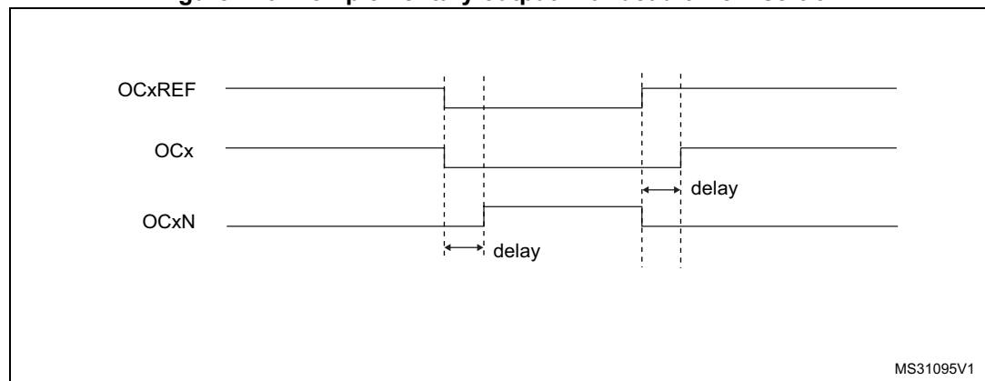
Figure 426. Complementary output with dead-time insertion
