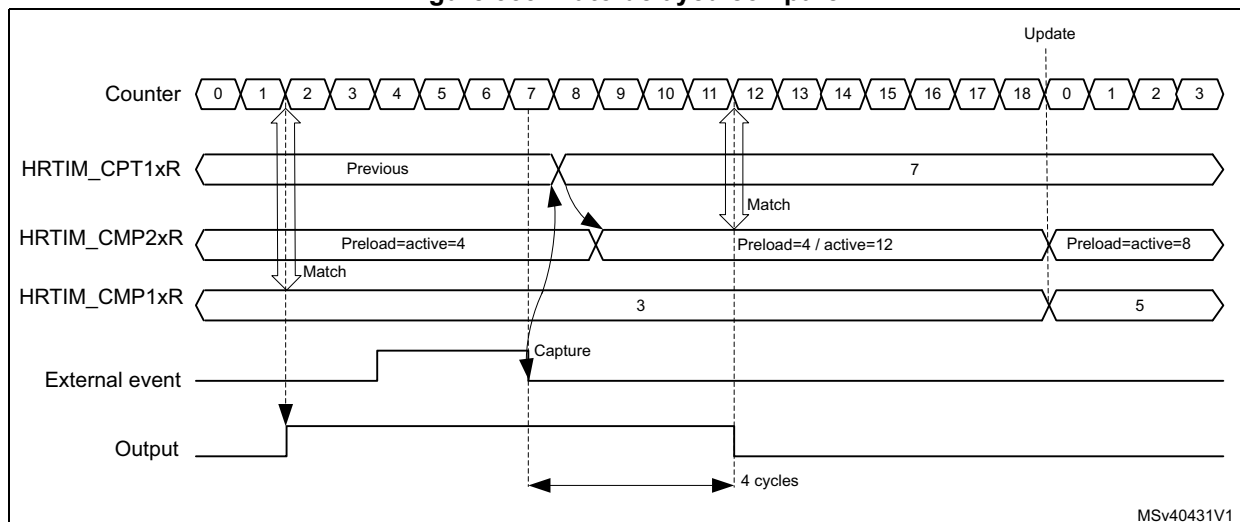
Figure 333. Auto-delayed compare
