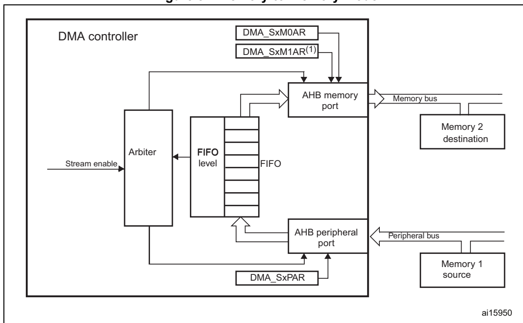
Figure 87. Memory-to-memory mode
