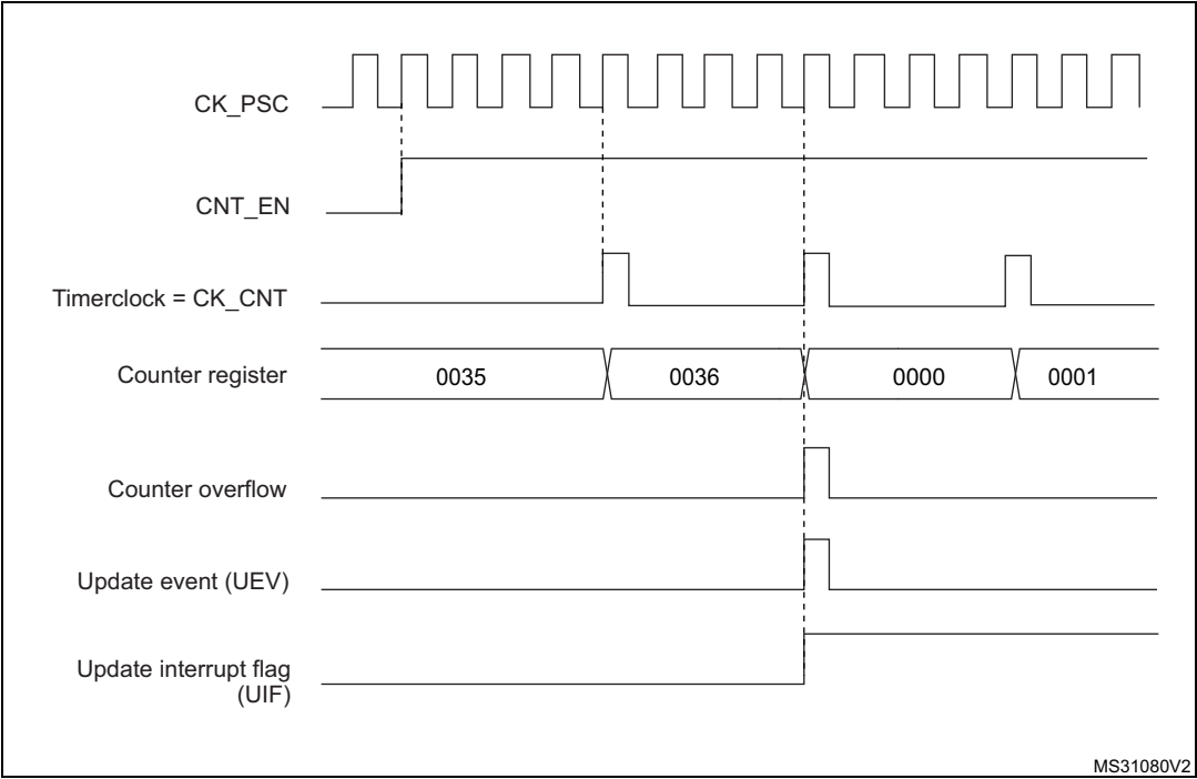
Figure 502. Counter timing diagram, internal clock divided by 4
