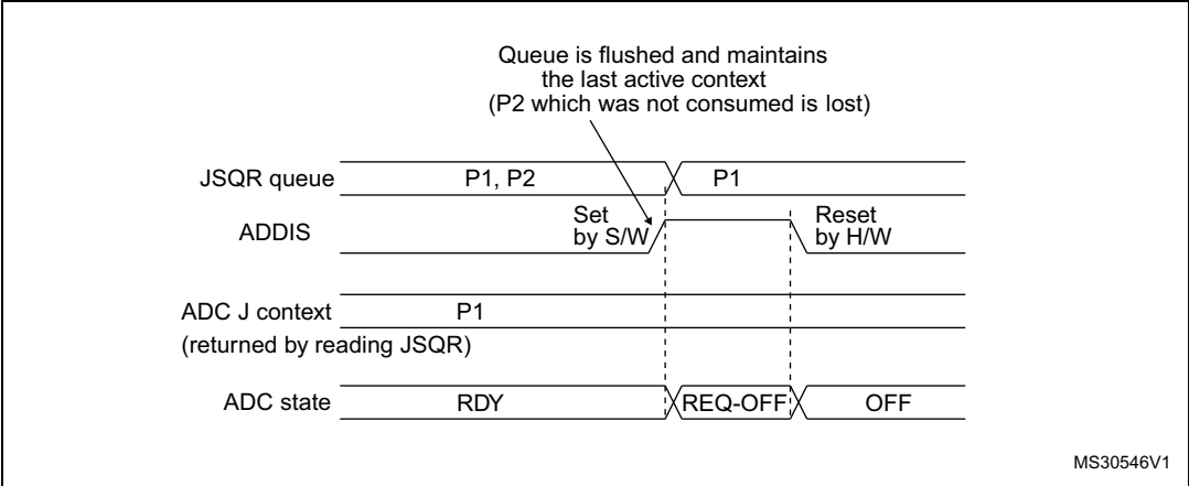
Figure 165. Flushing JSQR queue of context by setting ADDIS=1 (JQM=0)
