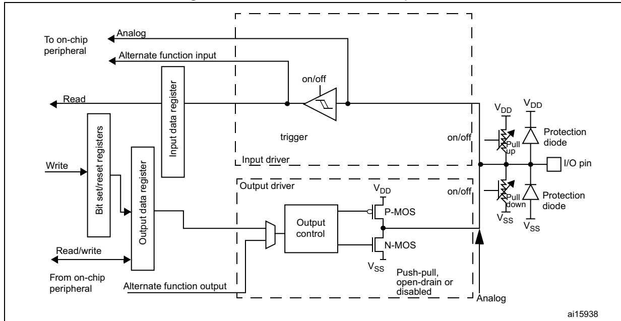
Figure 76. Basic structure of an I/O port bit
