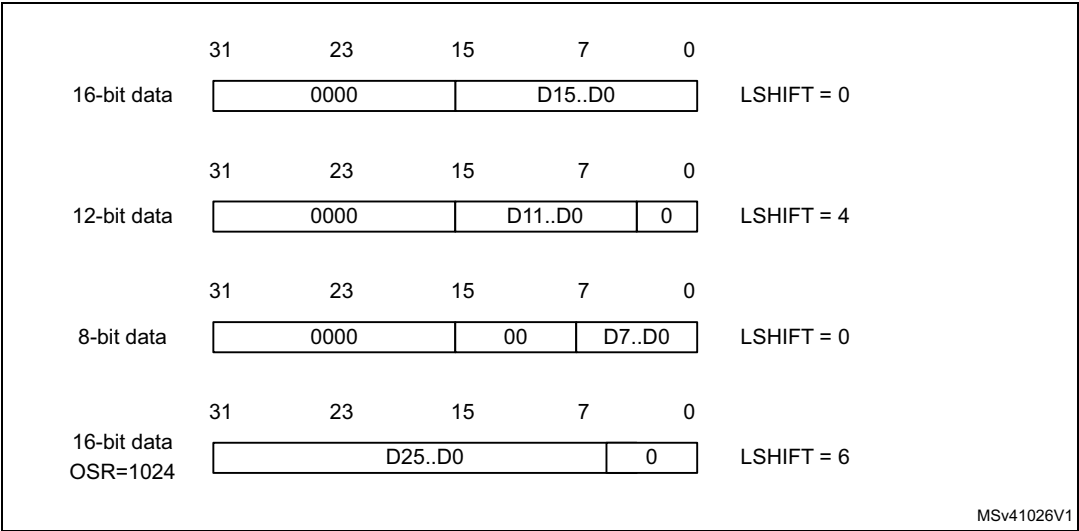
Figure 173. Left alignment (offset disabled, unsigned value)
