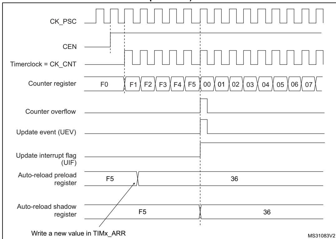
Figure 505. Counter timing diagram, update event when ARPE=1 (TIMx_ARR preloaded)
