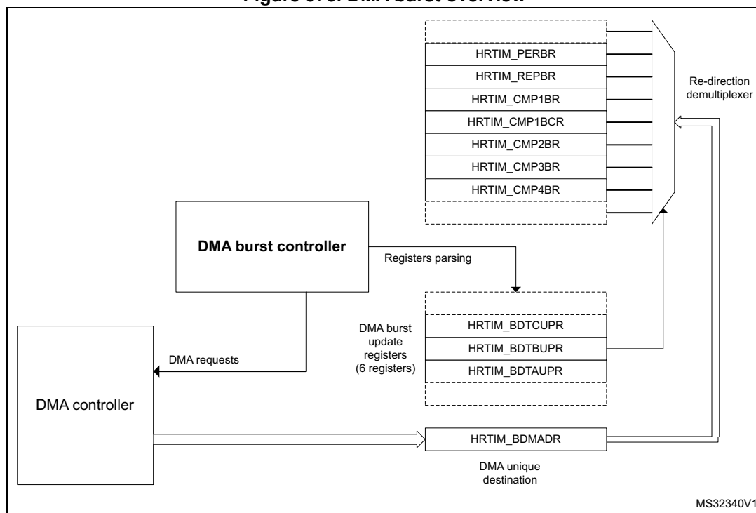
Figure 375. DMA burst overview
