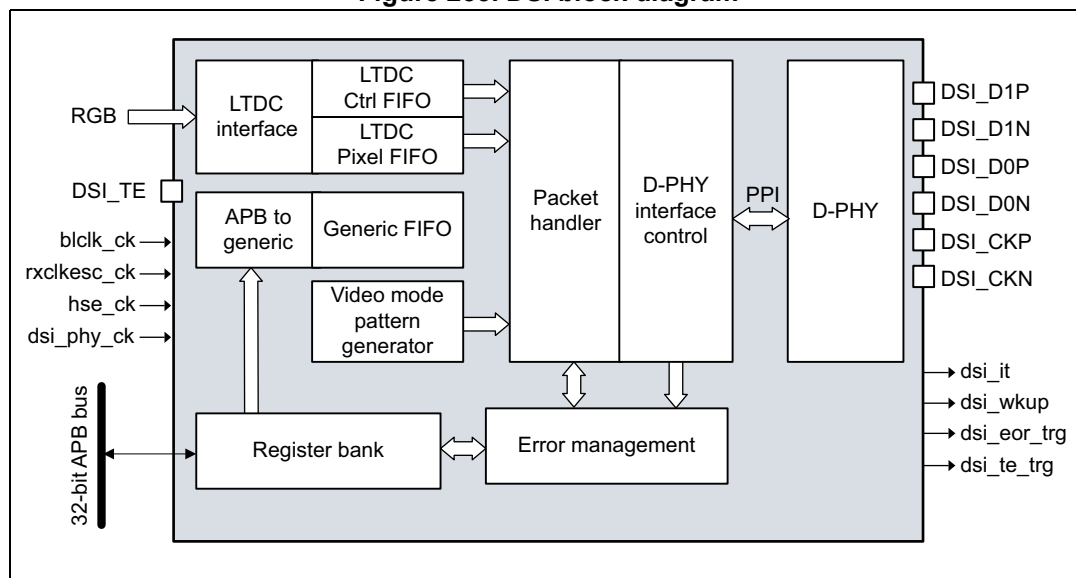
Figure 255. DSI block diagram
