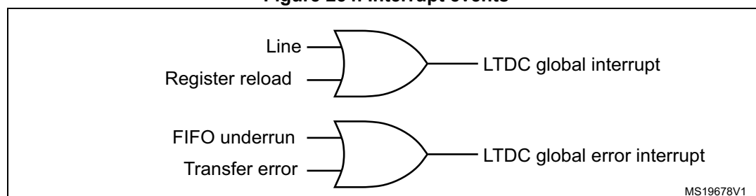
Figure 254. Interrupt events
