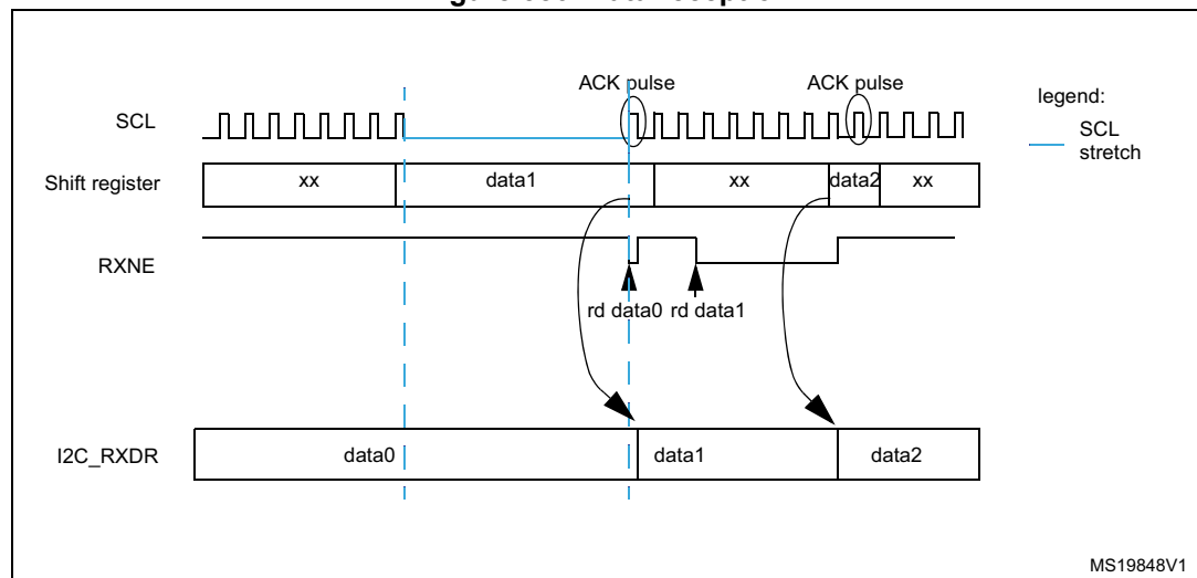
Figure 586. Data reception
