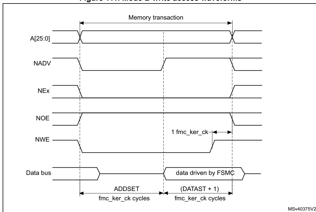
Figure 111. Mode B write access waveforms
