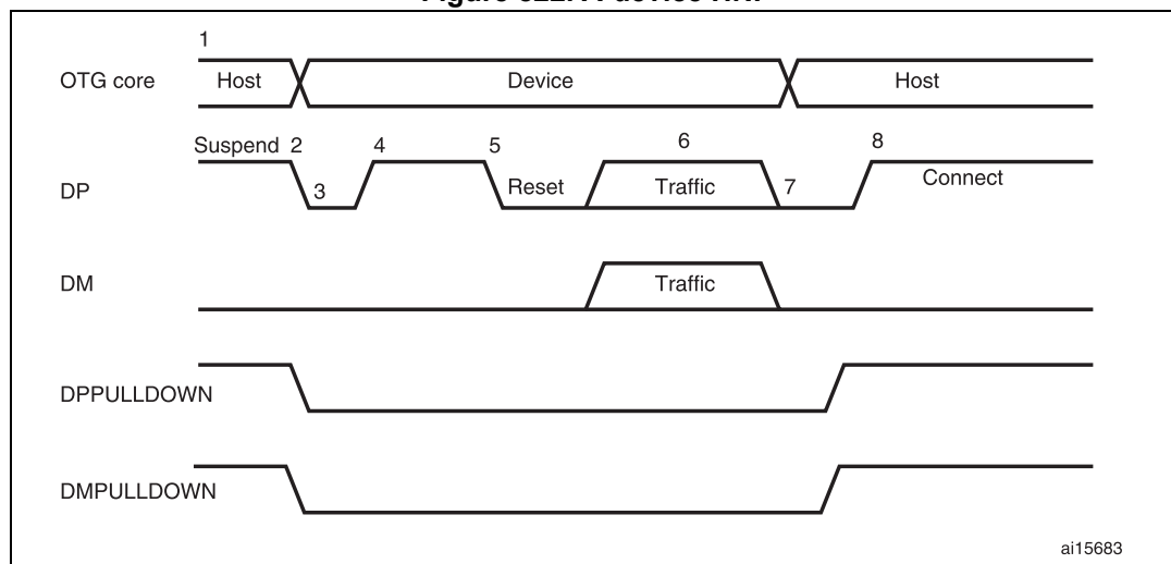
Figure 822. A-device HNP
