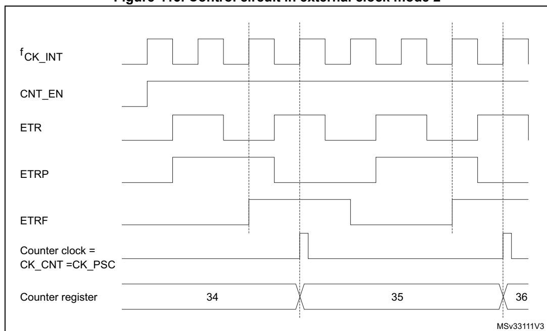
Figure 413. Control circuit in external clock mode 2
