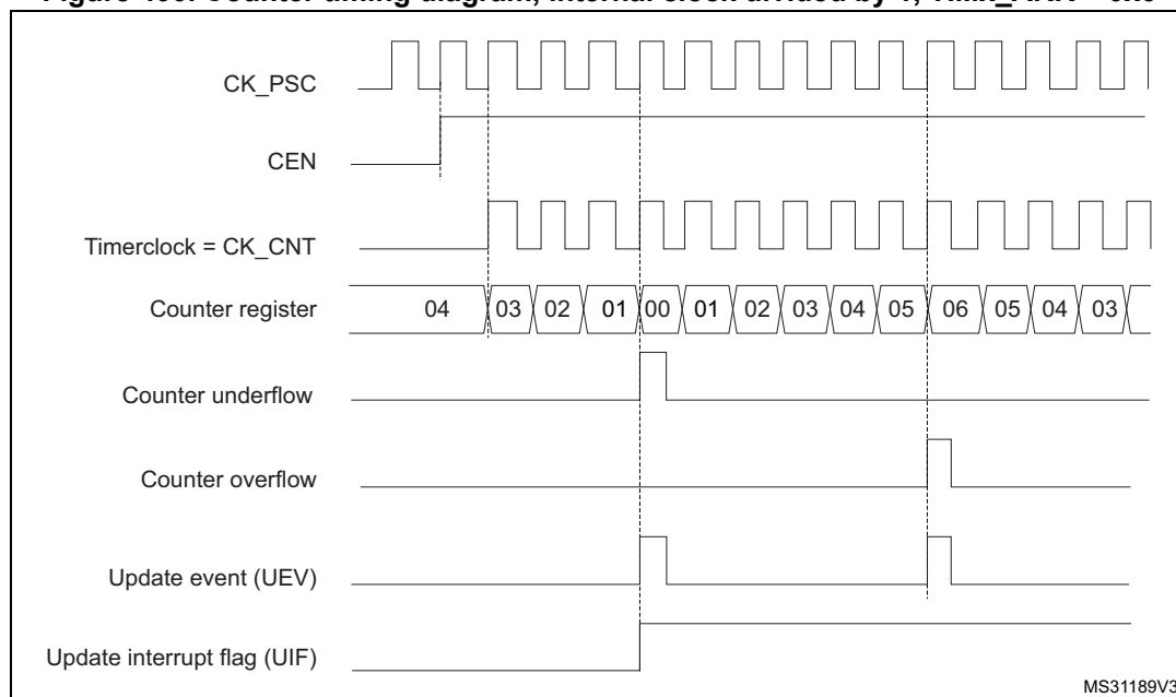
Figure 400. Counter timing diagram, internal clock divided by 1, TIMx_ARR = 0x6
