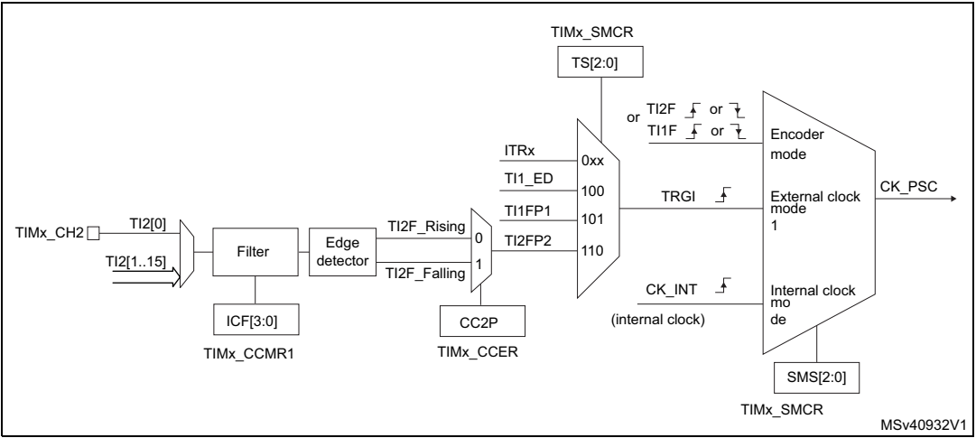
Figure 507. TI2 external clock connection example
