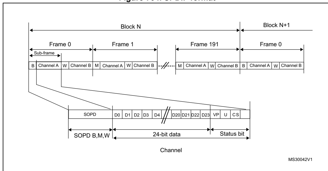
Figure 704. SPDIF format
