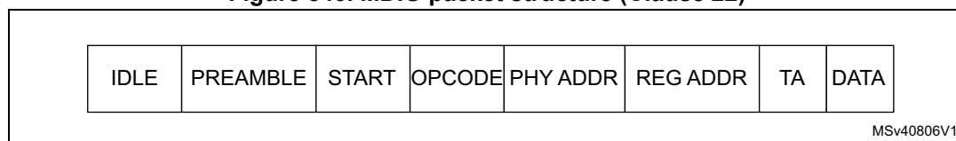
Figure 840. MDIO packet structure (Clause 22)
