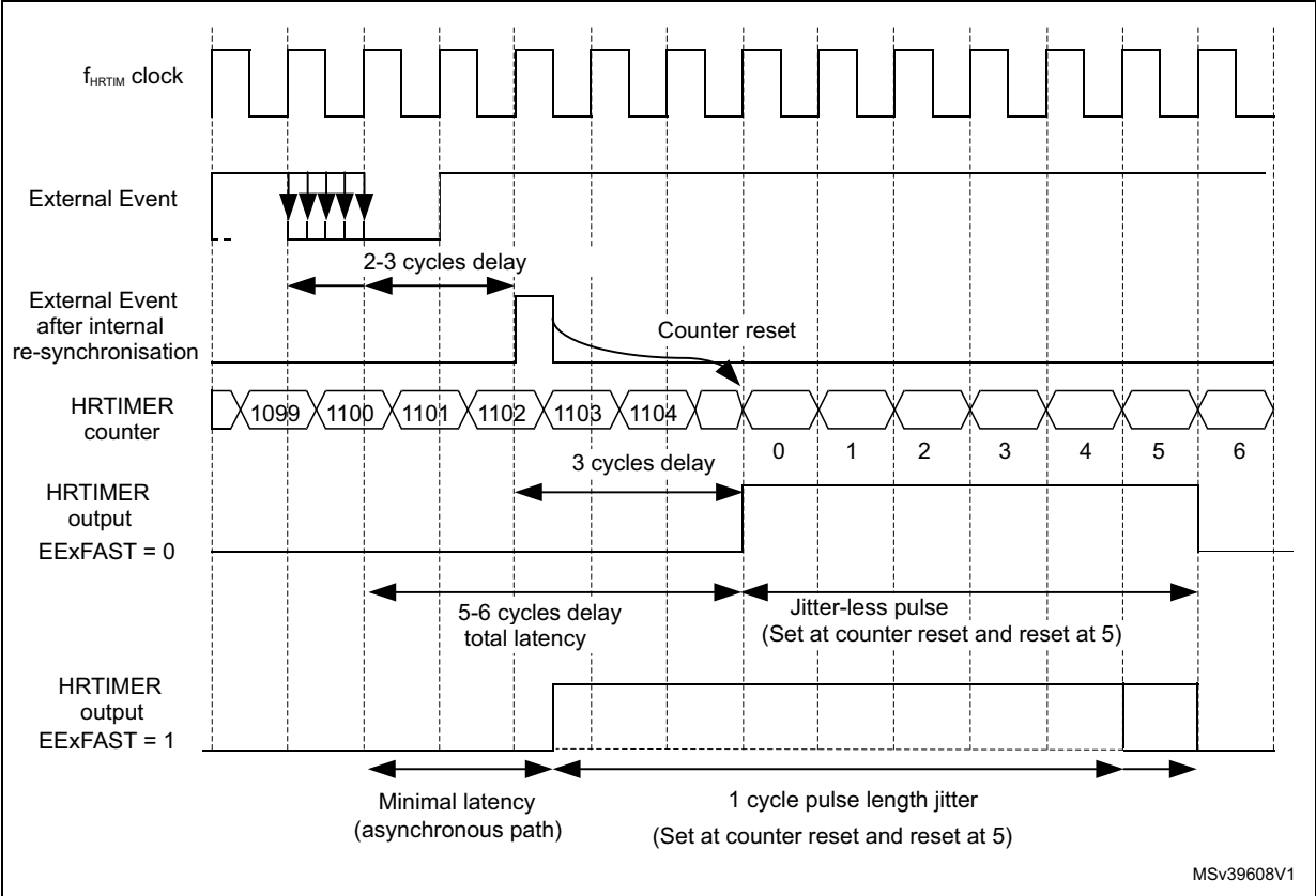
Figure 344. Latency to external events falling edge (counter reset and output set)
