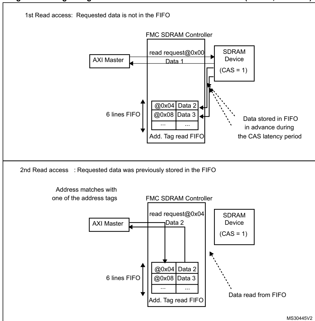
Figure 127. Logic diagram of Read access with RBURST bit set (CAS=2, RPIPE=0)
