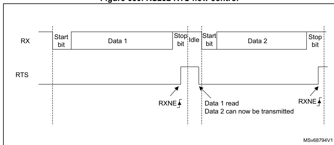
Figure 650. RS232 RTS flow control
