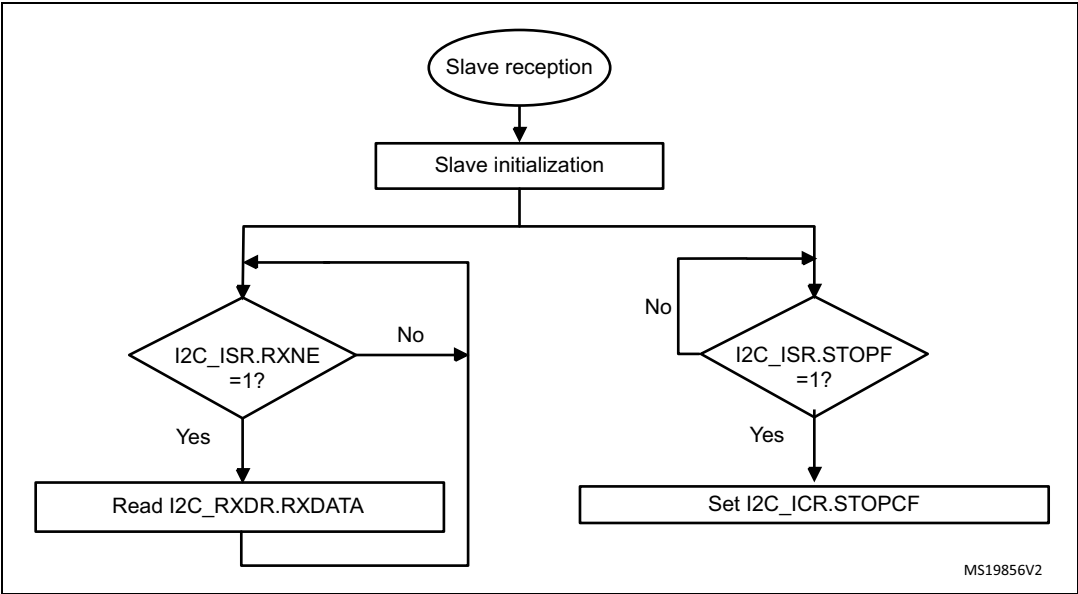
Figure 593. Transfer sequence flow for slave receiver with NOSTRETCH = 1
