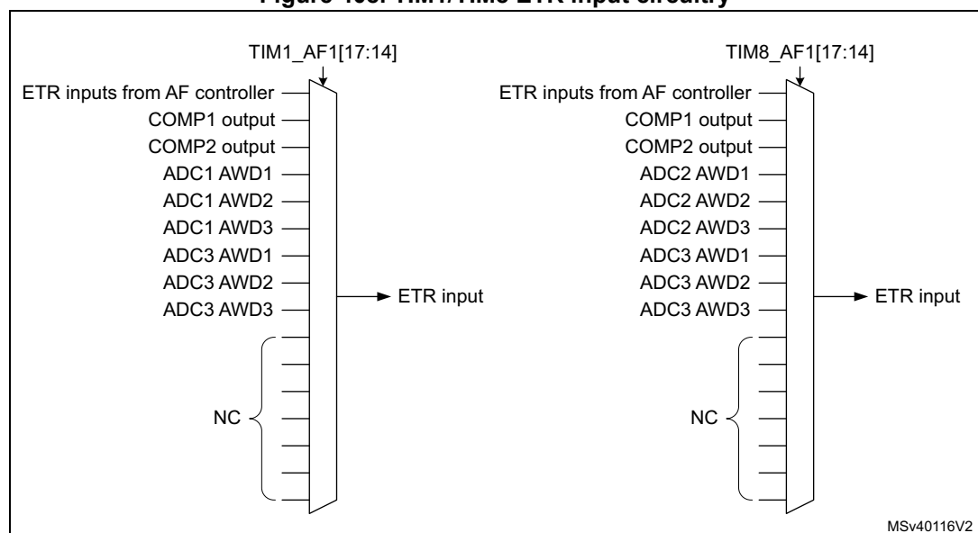
Figure 408. TIM1/TIM8 ETR input circuitry
