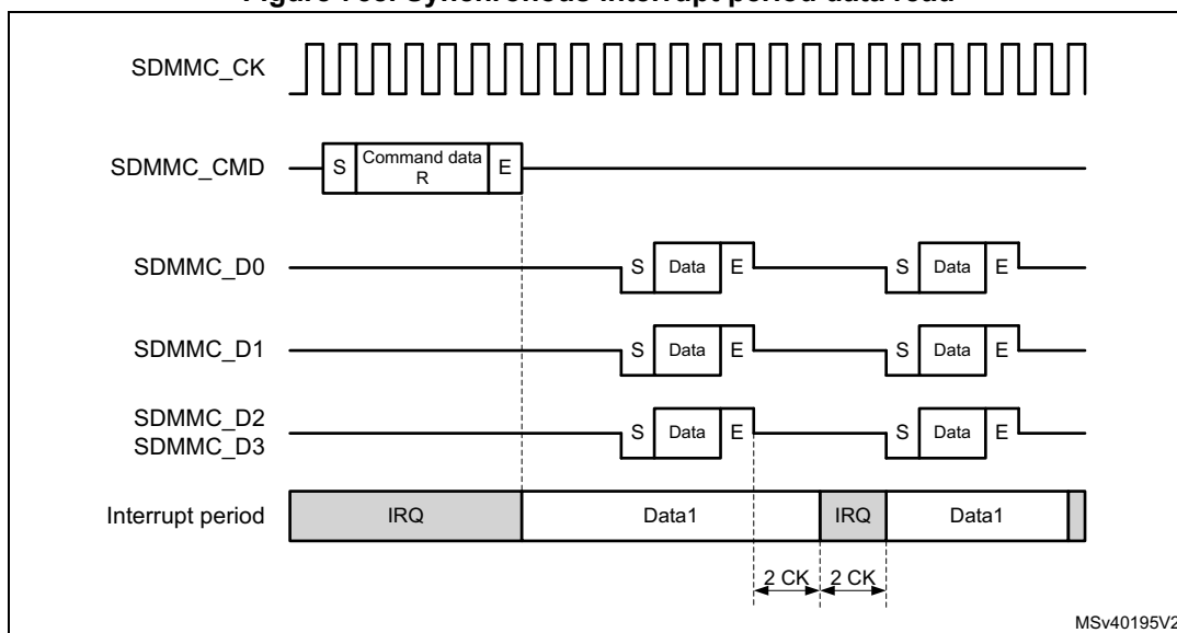
Figure 758. Synchronous interrupt period data read
