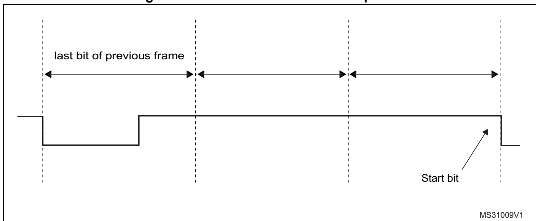
Figure 866. SFT of three nominal bit periods
