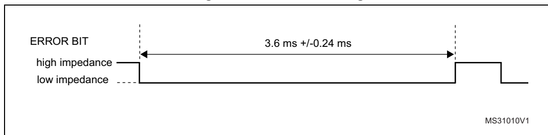
Figure 867. Error bit timing
