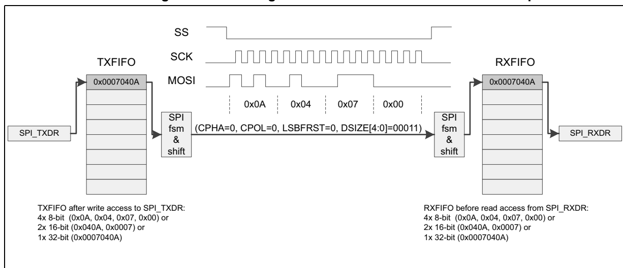
Figure 666. Packing data in FIFO for transmission and reception
