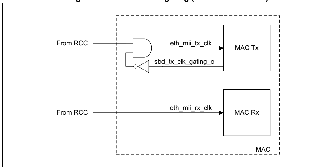
Figure 849. LPI Tx clock gating (when LPITCSE = 1)
