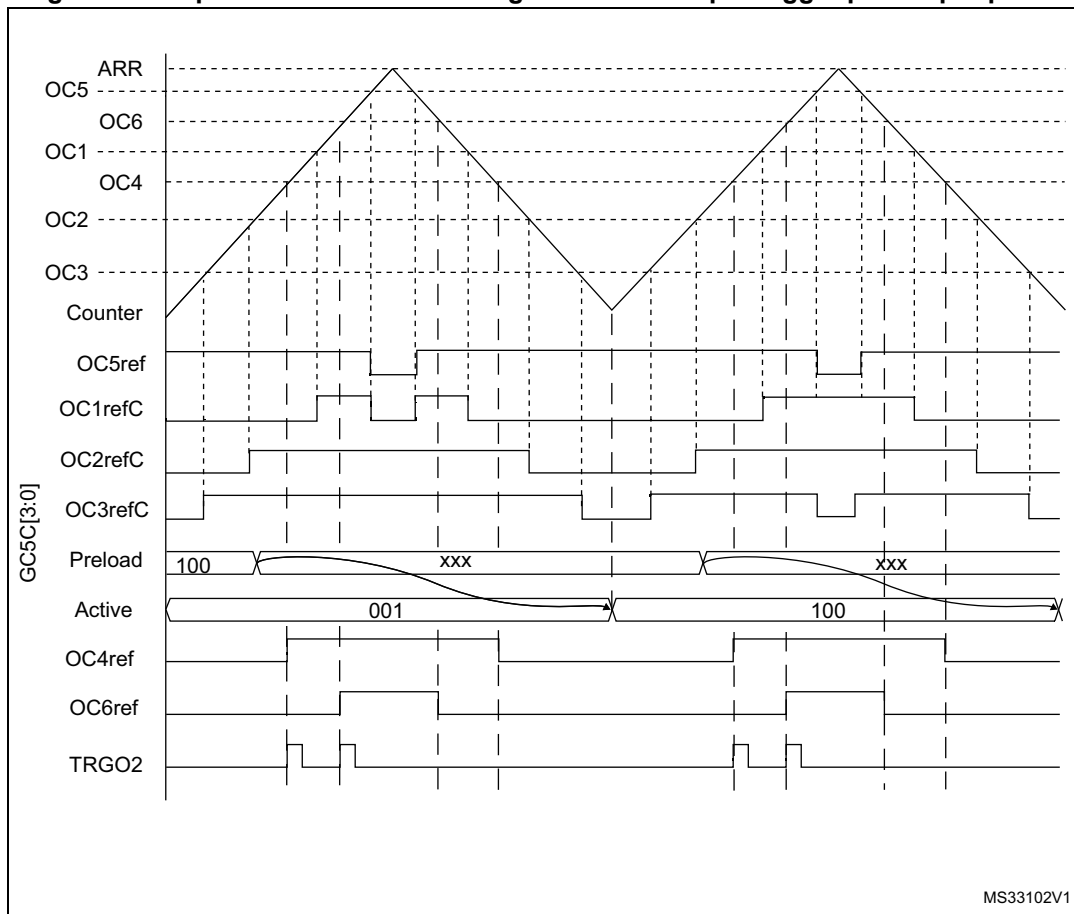
Figure 425. 3-phase combined PWM signals with multiple trigger pulses per period
