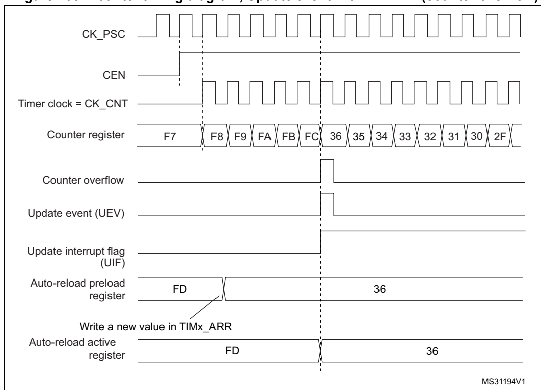
Figure 405. Counter timing diagram, Update event with ARPE=1 (counter overflow)
