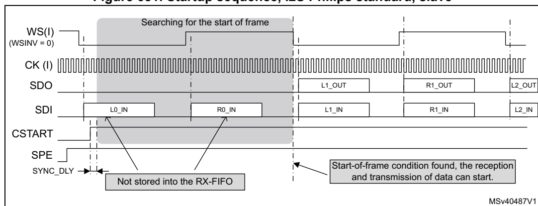
Figure 681. Startup sequence, I2S Philips standard, slave
