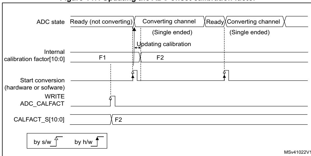
Figure 147. Updating the ADC offset calibration factor
