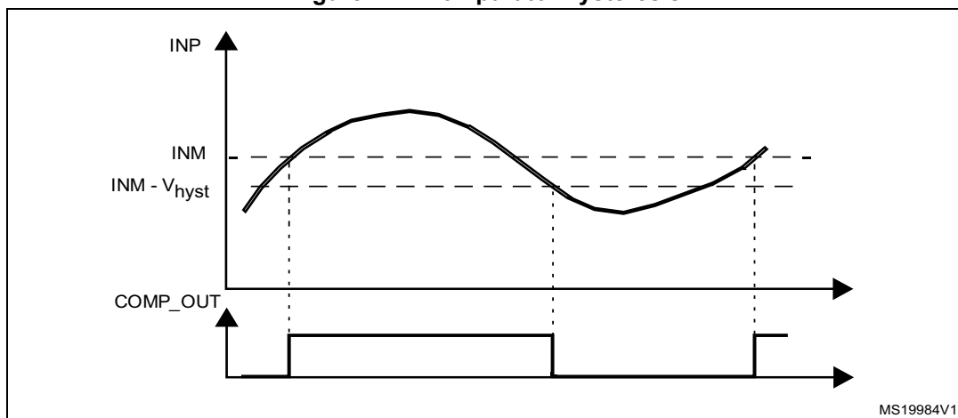
Figure 222. Comparator hysteresis
