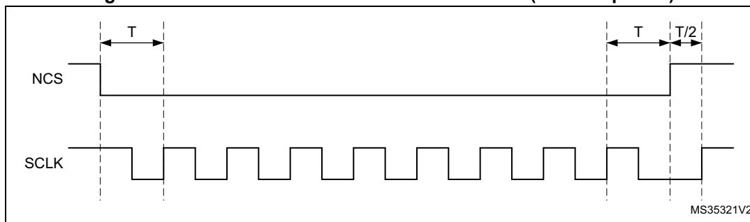
Figure 138. NCS when CKMODE = 1 in DDR mode ( T = \text{CLK period} )
