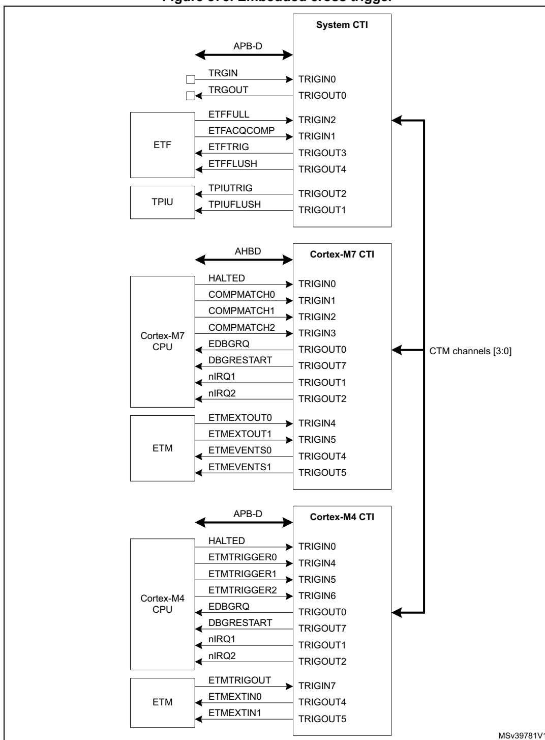
Figure 878. Embedded cross trigger
