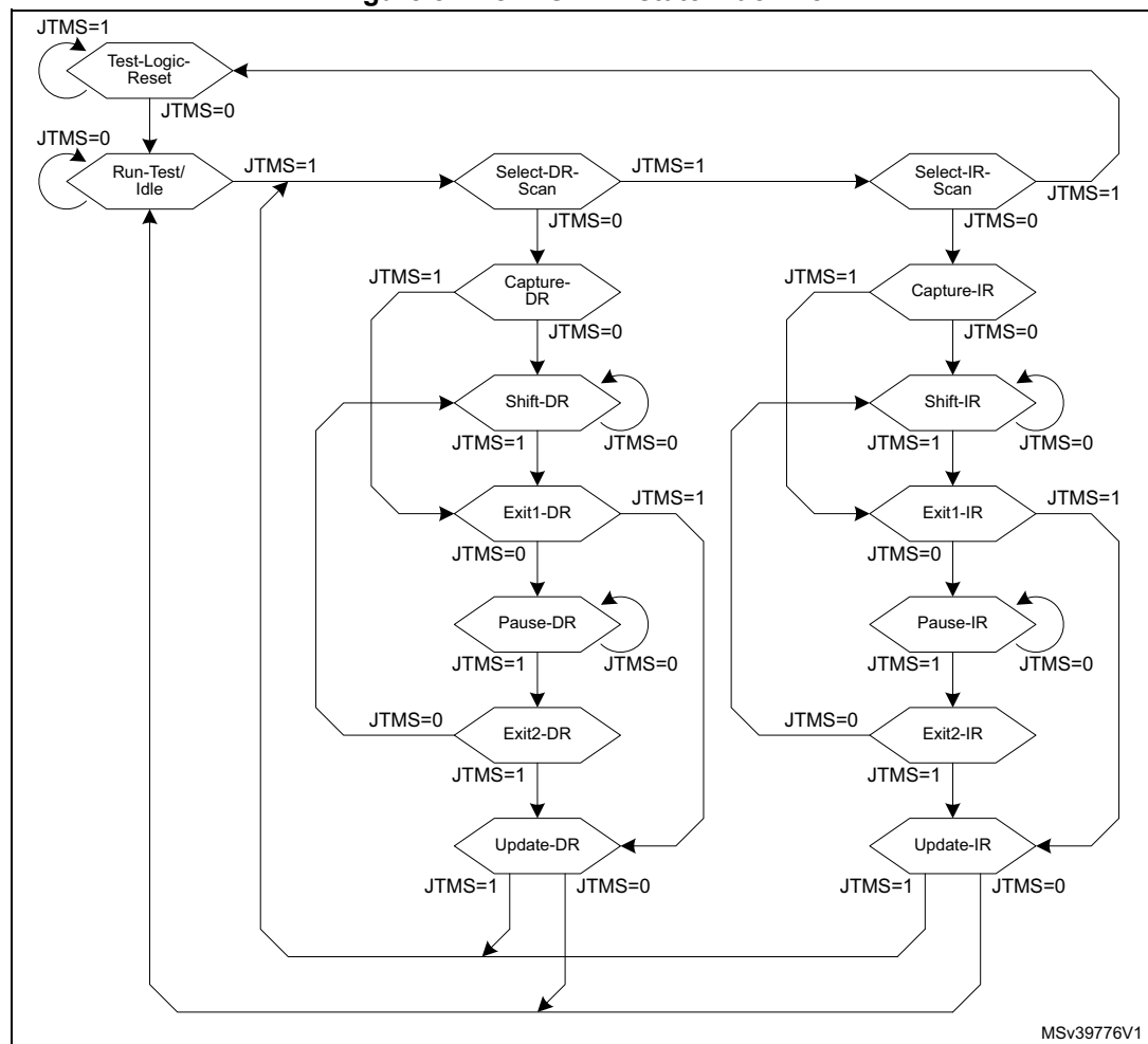
Figure 874. JTAG TAP state machine
