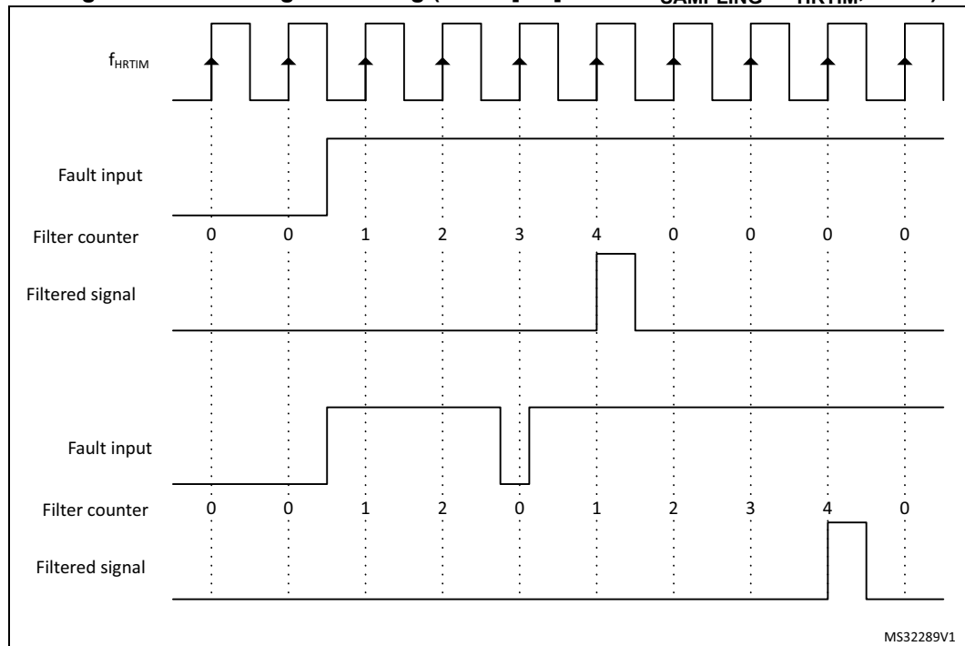
Figure 368. Fault signal filtering (FLTxF[3:0]= 0010: f_{\text{SAMPLING}} = f_{\text{HRTIM}} , N = 4)
