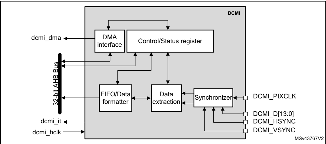
Figure 242. DCMI block diagram
