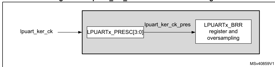
Figure 644. lpuart_ker_ck clock divider block diagram
