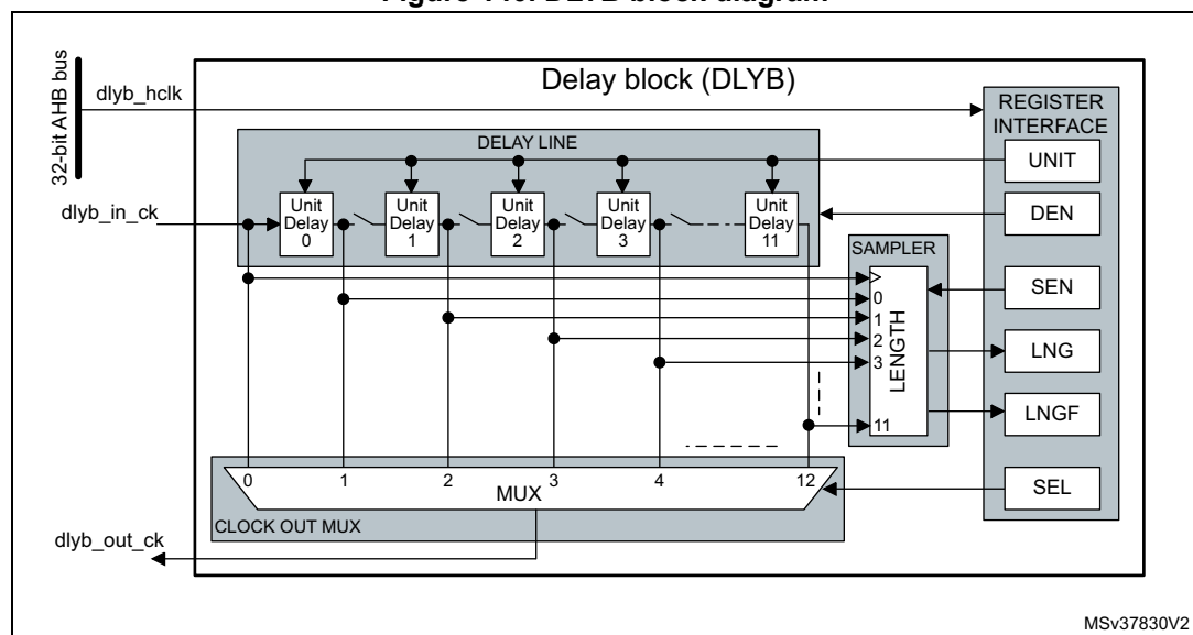
Figure 140. DLYB block diagram
