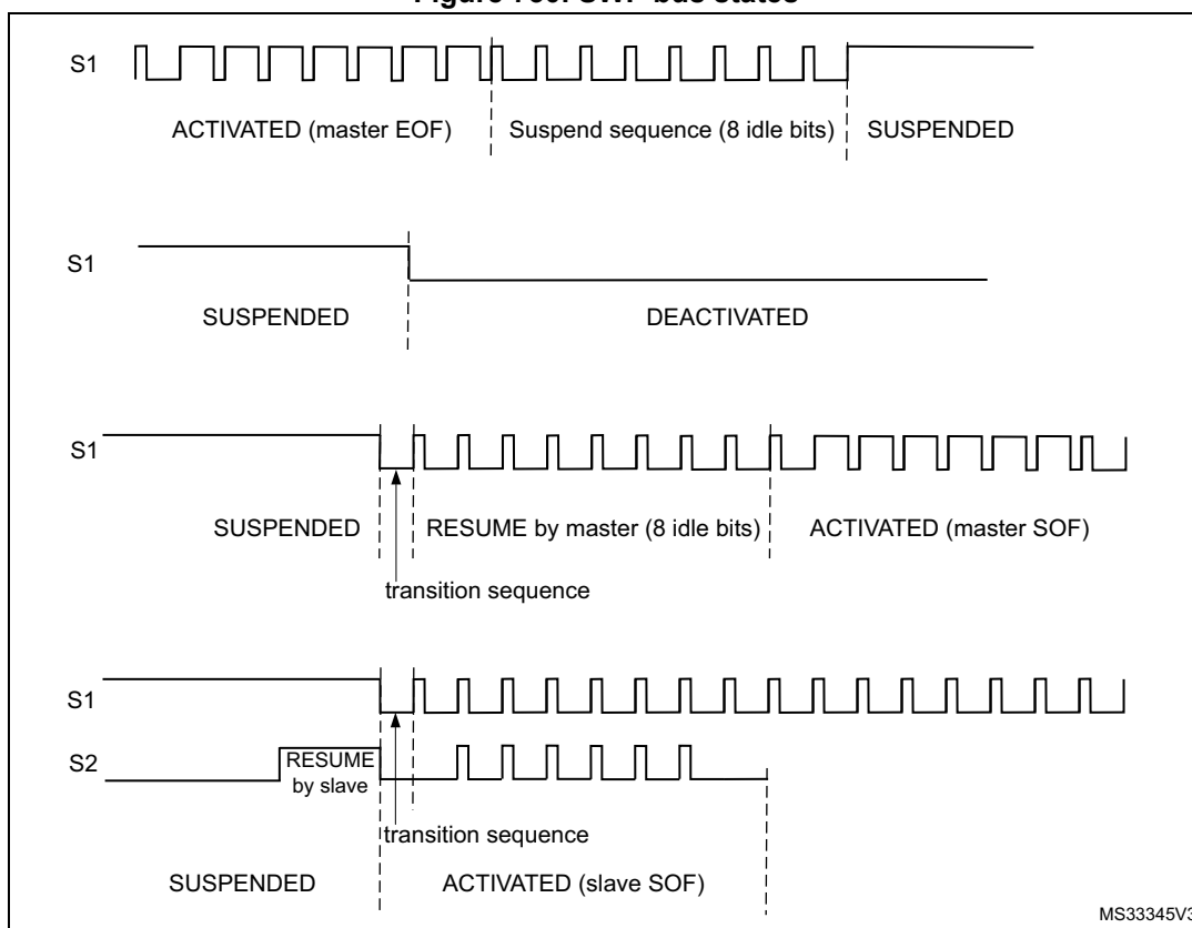
Figure 730. SWP bus states
