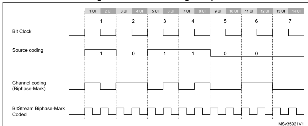
Figure 715. Channel coding example
