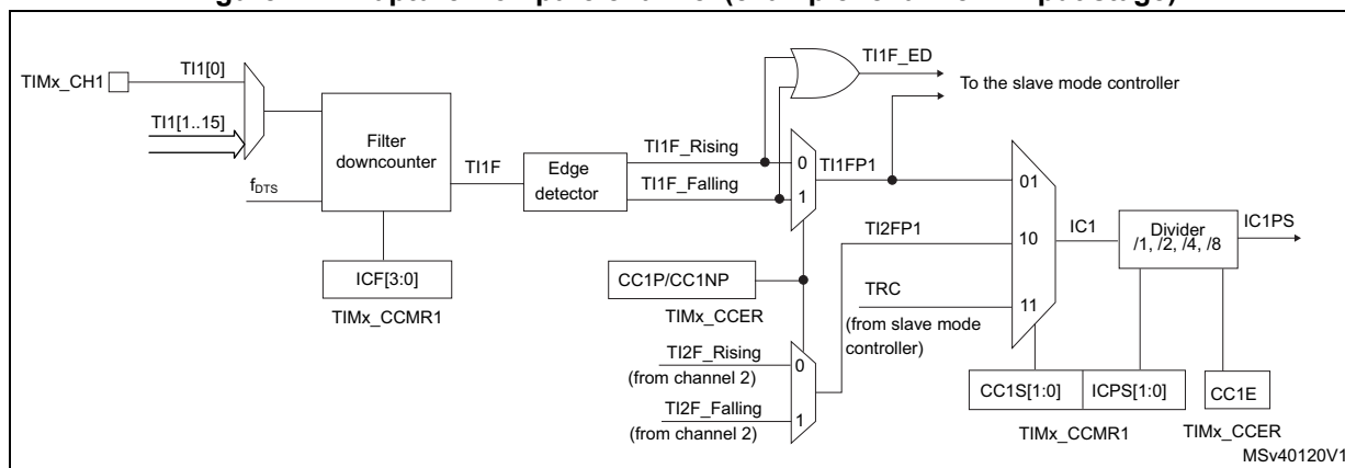
Figure 471. Capture/Compare channel (example: channel 1 input stage)
