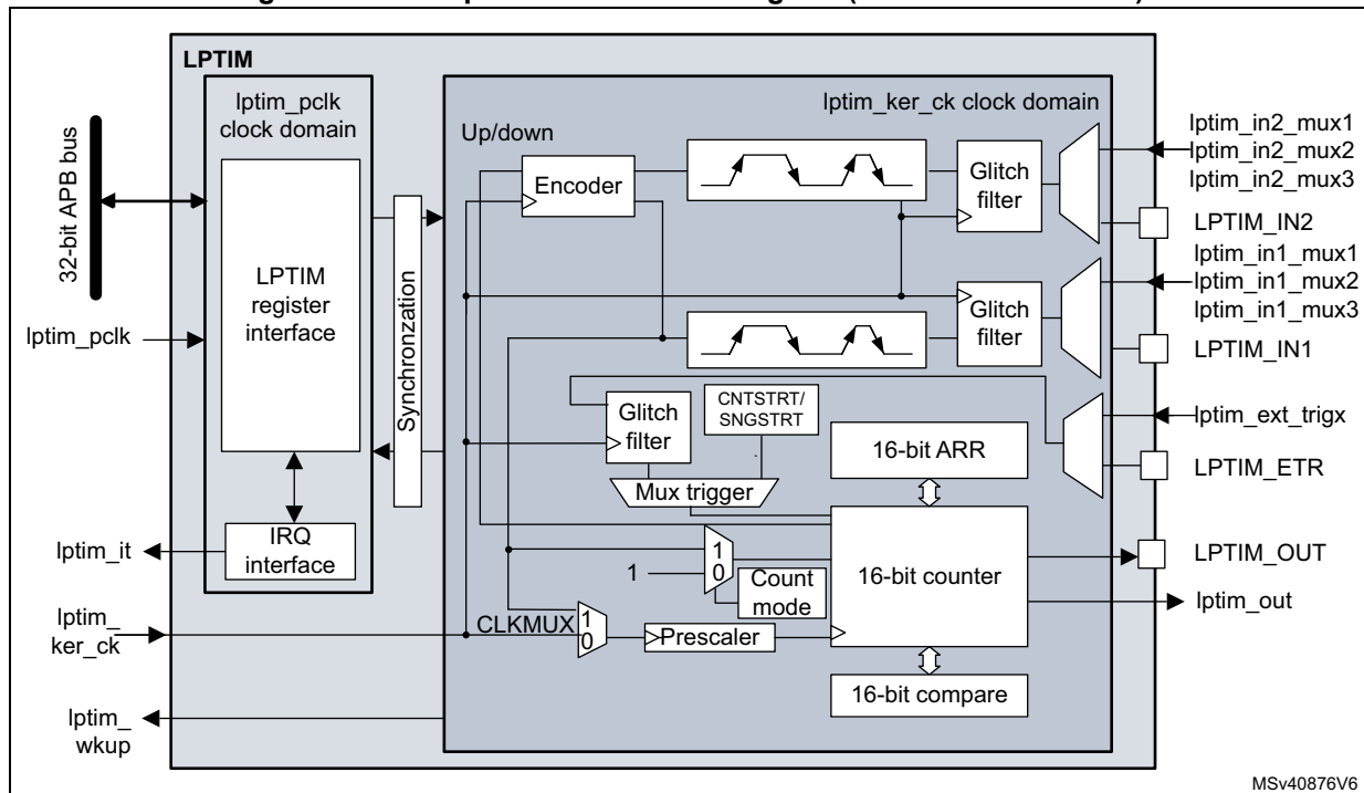
Figure 566. Low-power timer block diagram (LPTIM1 and LPTIM2)
