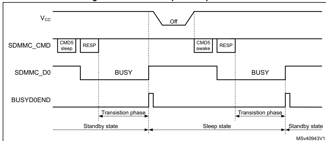
Figure 767. CMD5 Sleep Awake procedure
