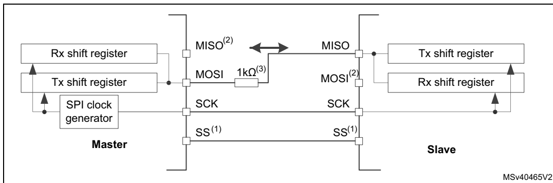
Figure 656. Half-duplex single master/ single slave application
