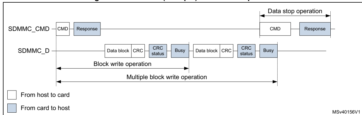
Figure 744. SDMMC (multiple) block write operation
