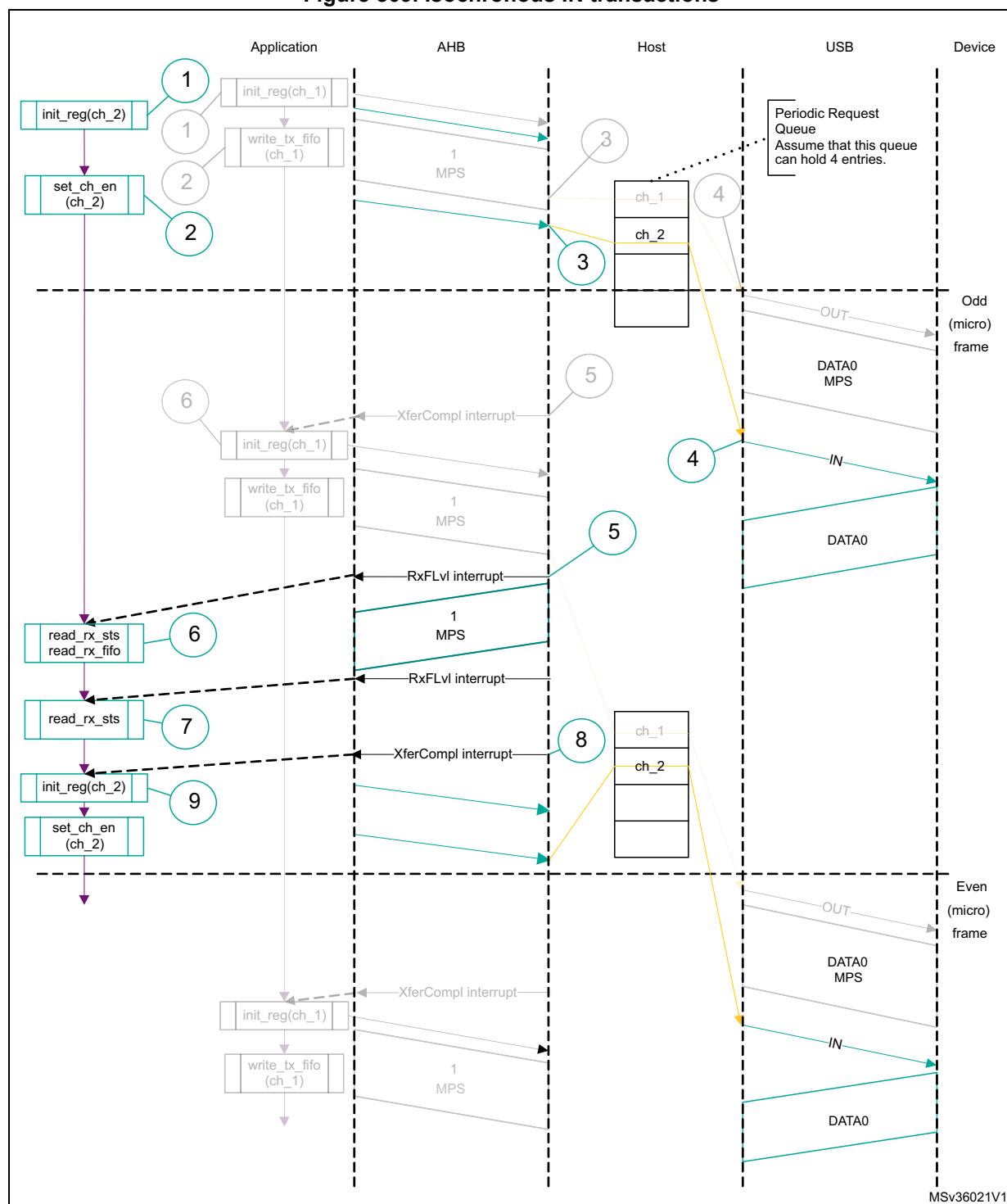
Figure 809. Isochronous IN transactions
