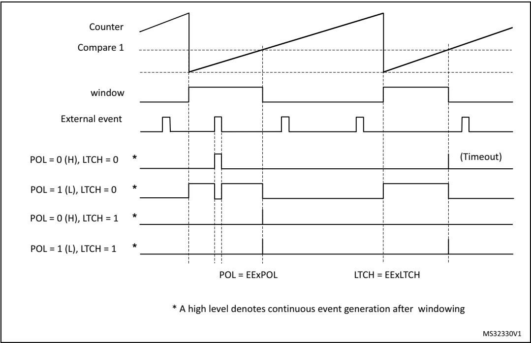
Figure 352. External trigger windowing, level sensitive triggering
