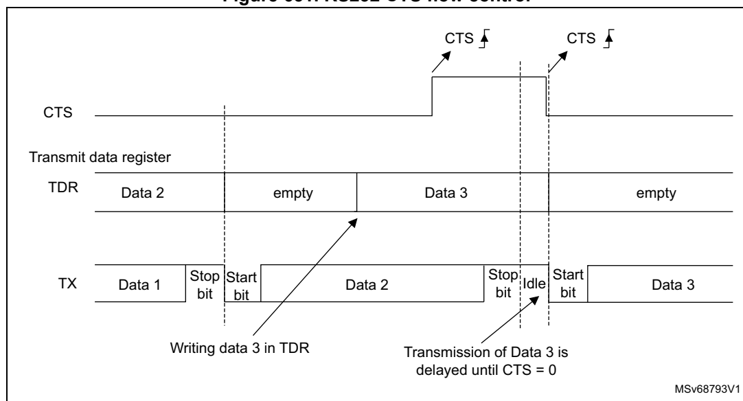
Figure 651. RS232 CTS flow control
