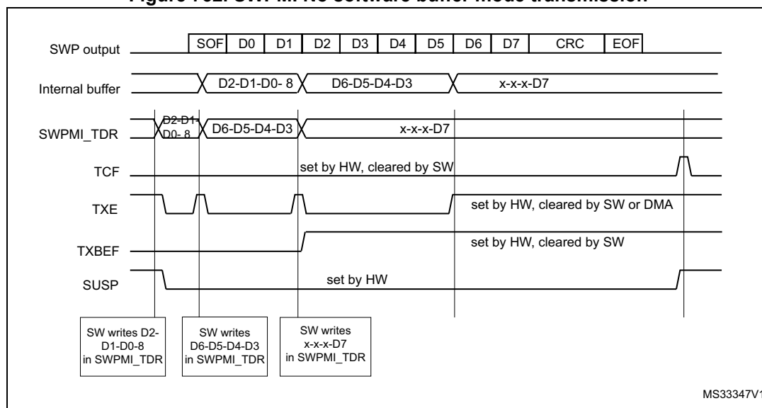
Figure 732. SWPMI No software buffer mode transmission
