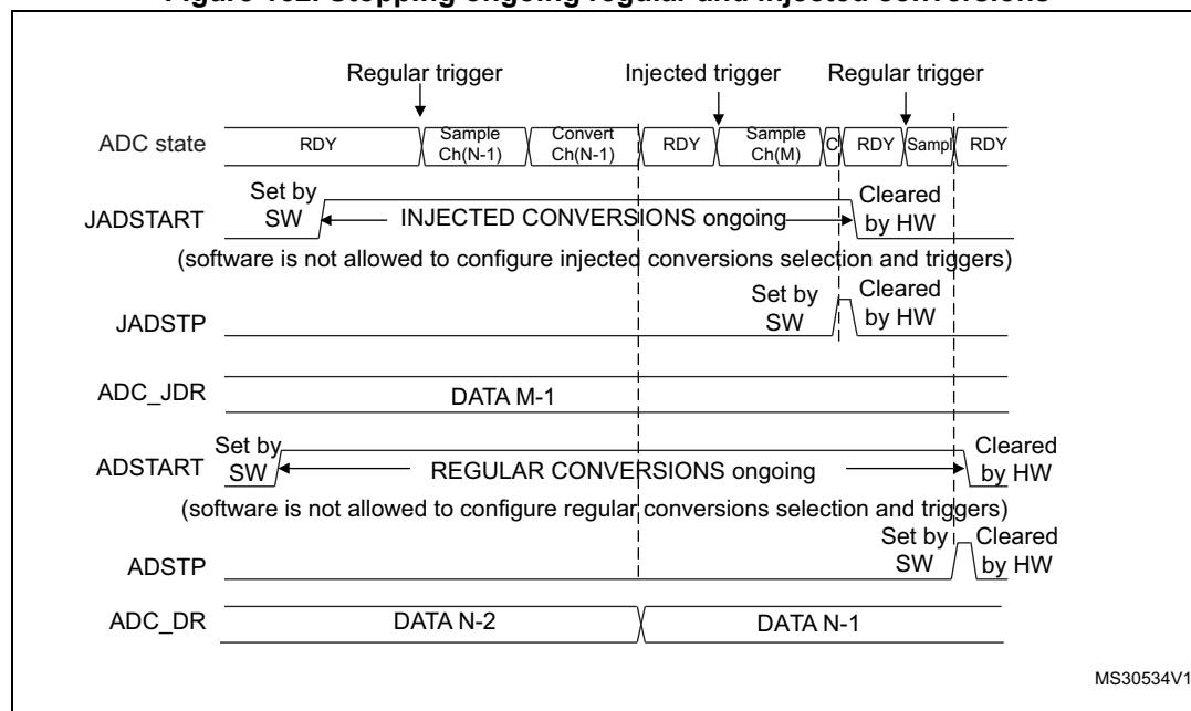
Figure 152. Stopping ongoing regular and injected conversions
