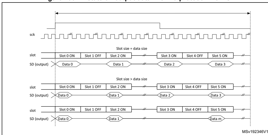
Figure 708. Tristate on output data line in a protocol like I2S
