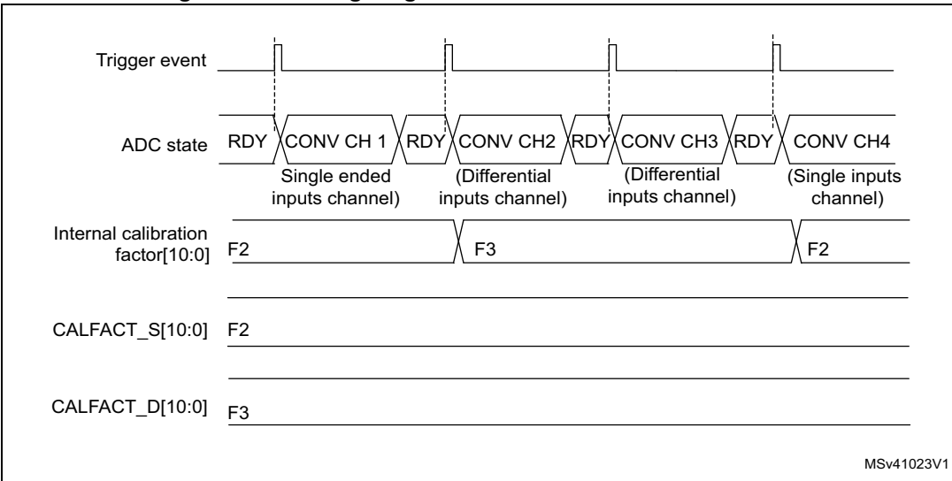
Figure 148. Mixing single-ended and differential channels
