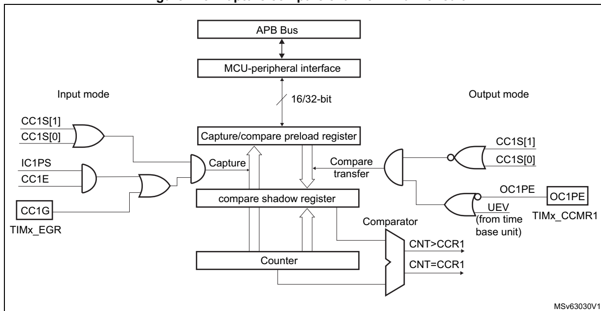
Figure 415. Capture/compare channel 1 main circuit
