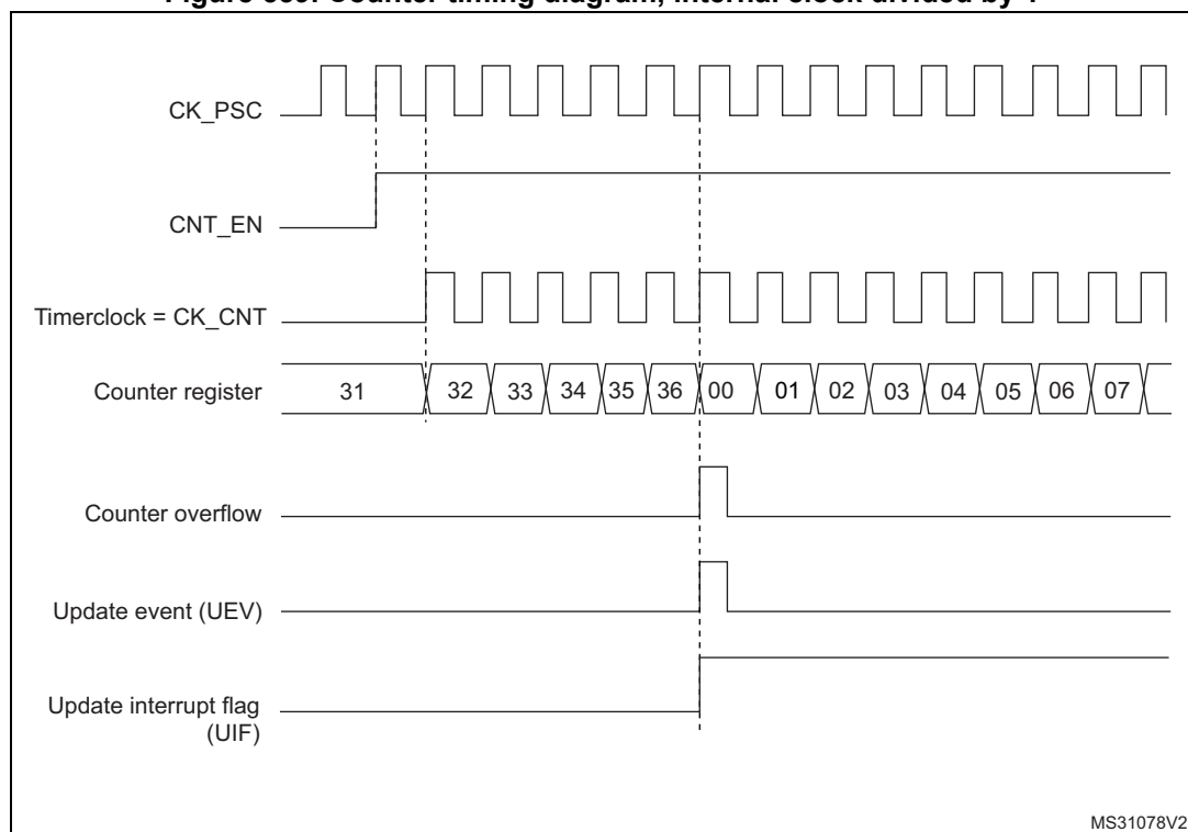
Figure 559. Counter timing diagram, internal clock divided by 1
