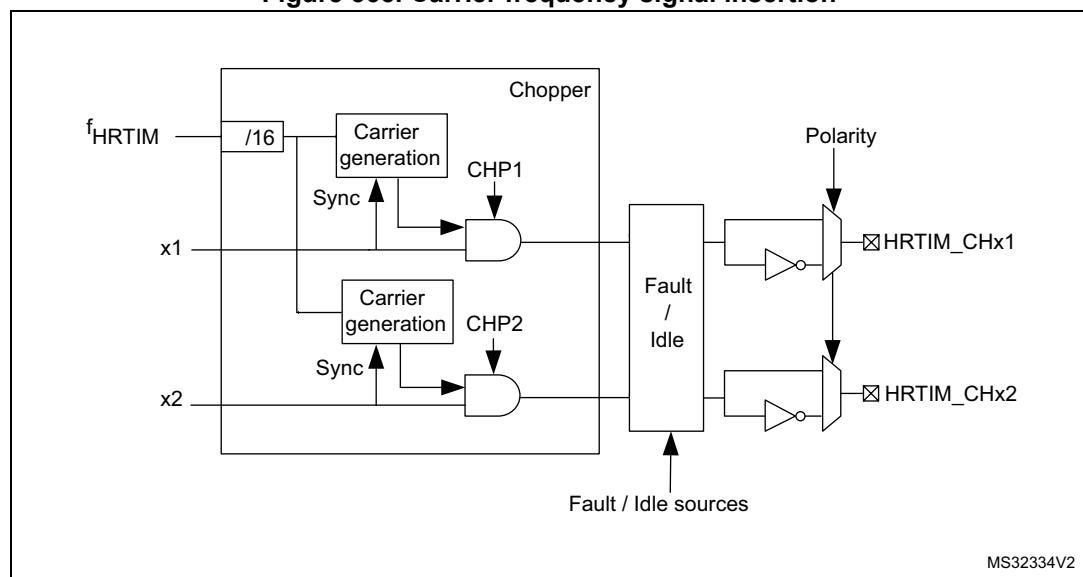
Figure 365. Carrier frequency signal insertion
