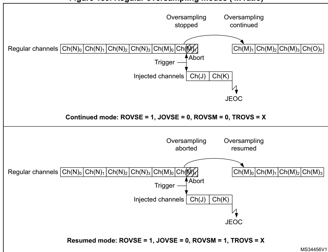
Figure 189. Regular oversampling modes (4x ratio)
