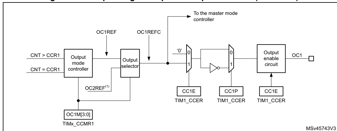
Figure 511. Output stage of capture/compare channel (channel 1)
