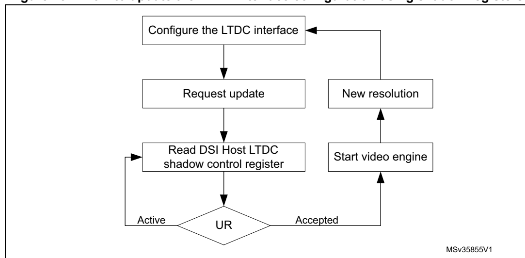
Figure 257. Flow to update the LTDC interface configuration using shadow registers
