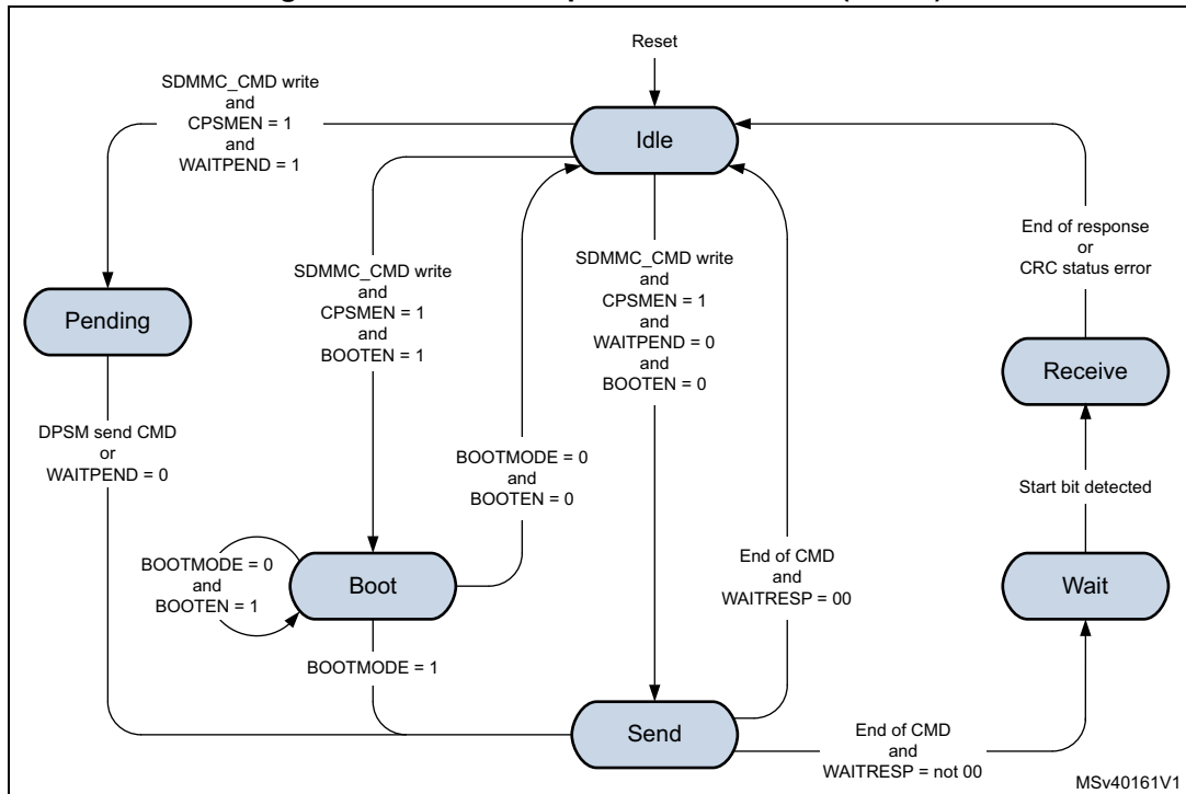
Figure 751. Command path state machine (CPSM)
