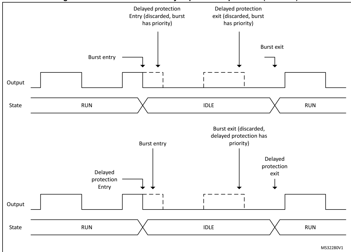
Figure 354. Burst mode and delayed protection priorities (DIDL = 0)
