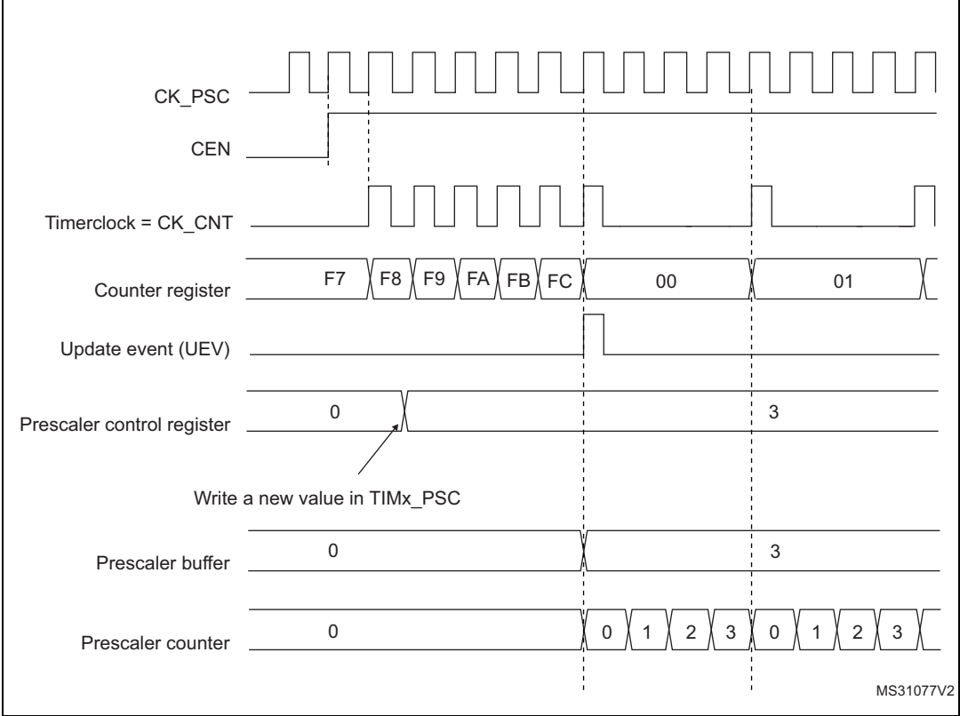
Figure 558. Counter timing diagram with prescaler division change from 1 to 4
