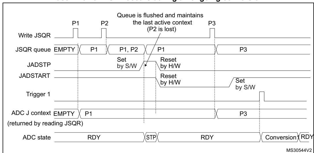
Figure 161. Flushing JSQR queue of context by setting JADSTP=1 (JQM=0). Case when JADSTP occurs during an ongoing conversion.
