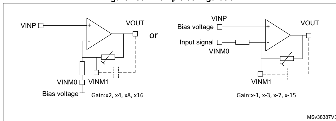
Figure 233. Example configuration
