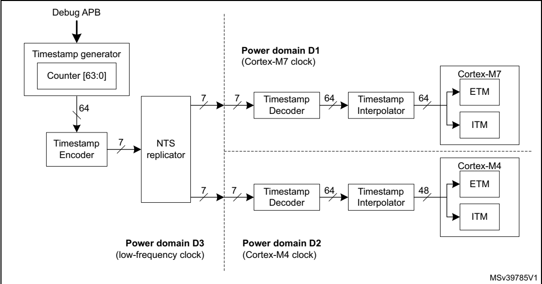
Figure 877. Global timestamp distribution
