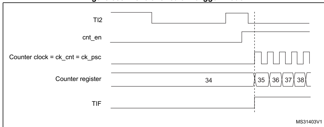
Figure 555. Control circuit in trigger mode
