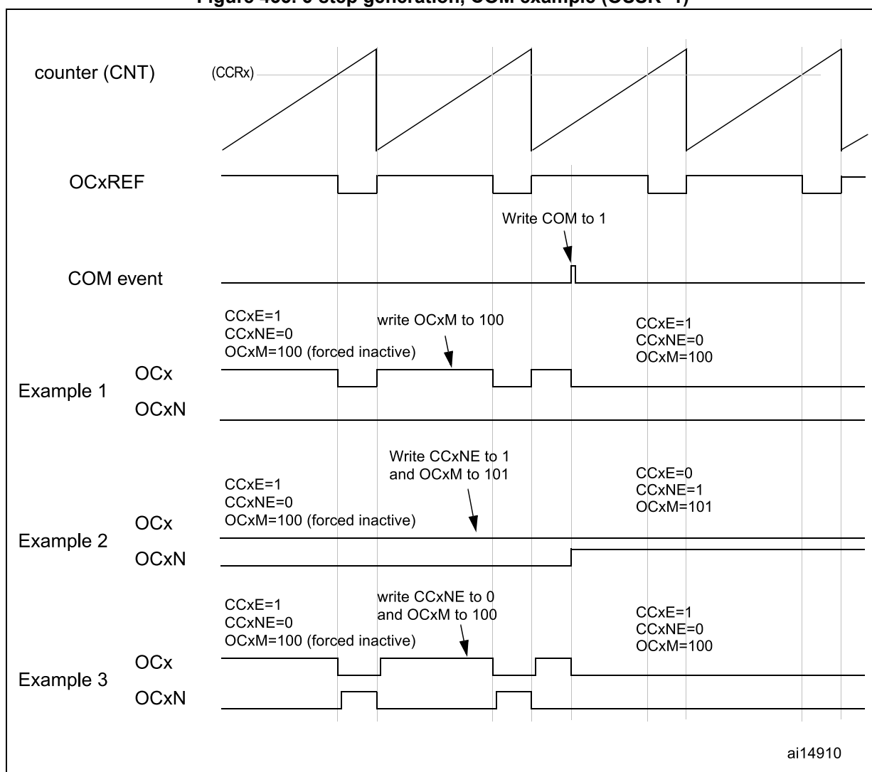
Figure 435. 6-step generation, COM example (OSSR=1)
