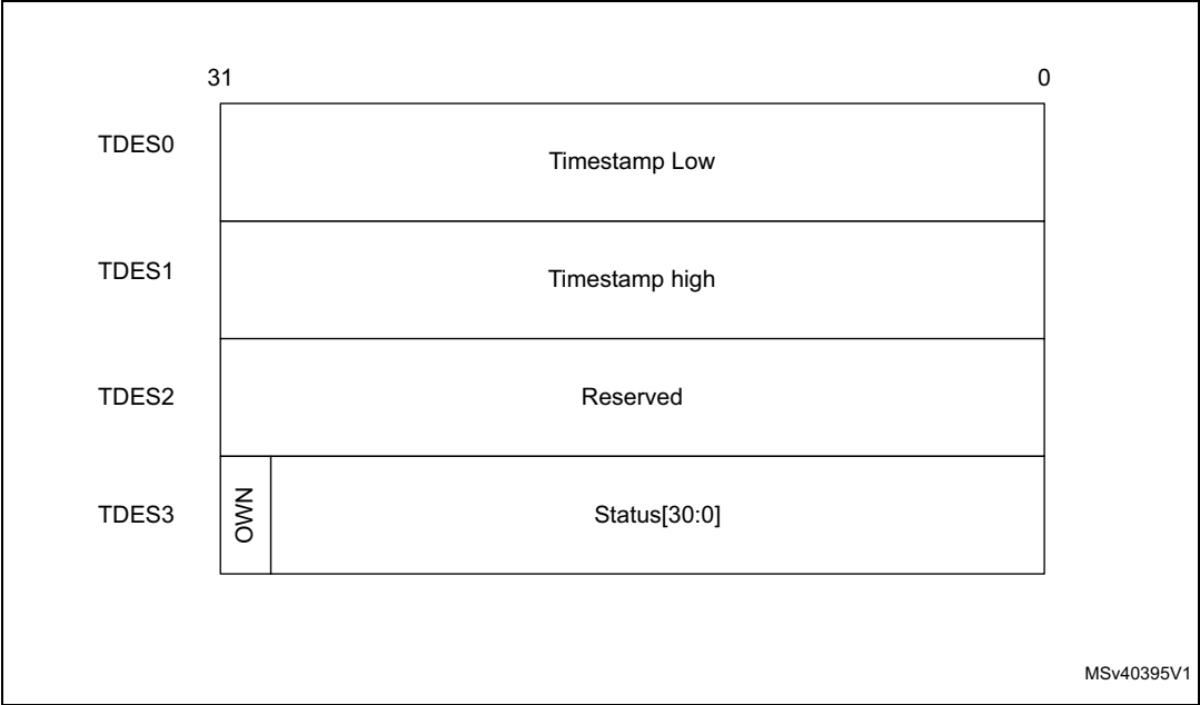
Figure 854. Transmit descriptor write-back format
