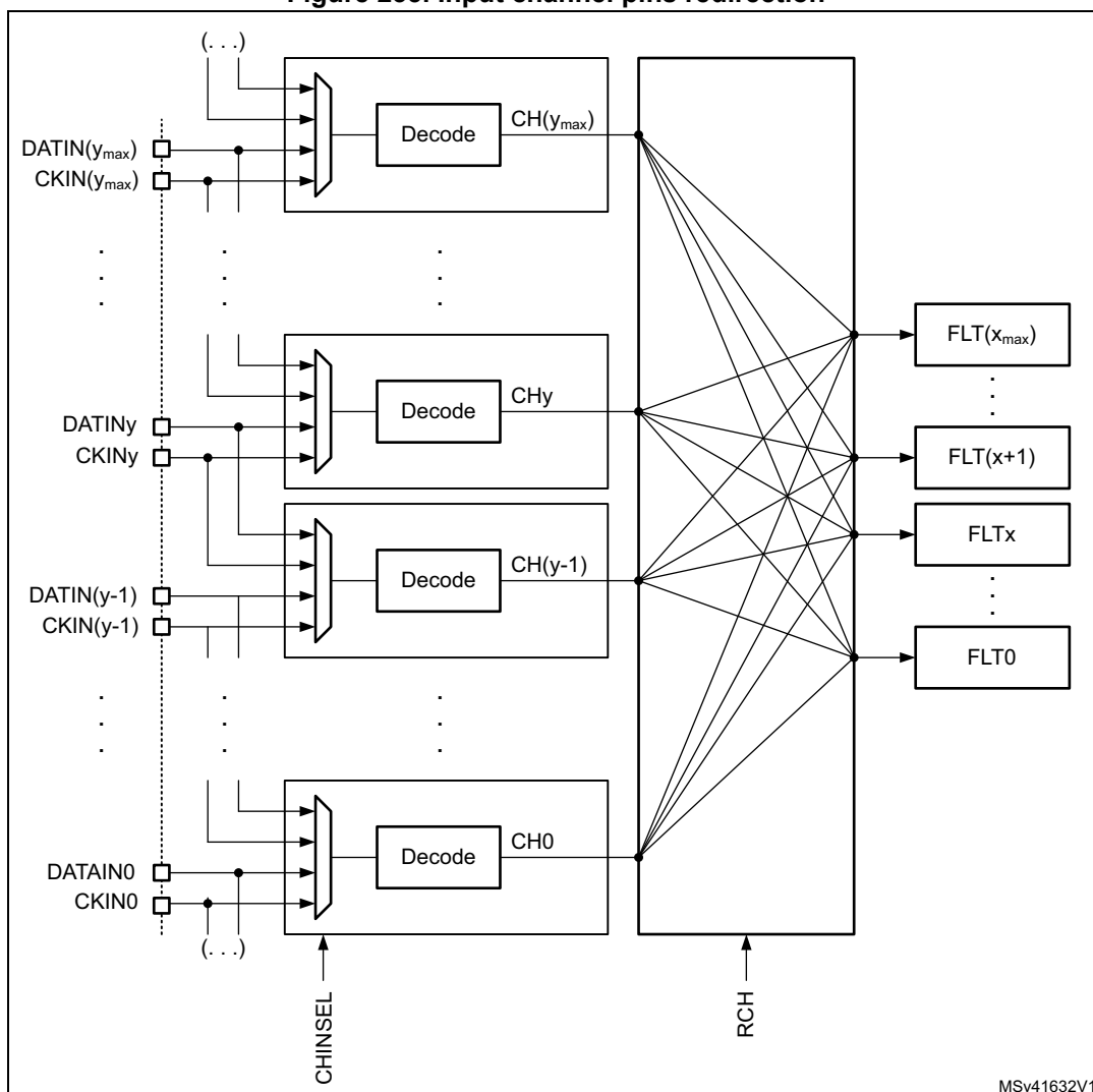
Figure 235. Input channel pins redirection
