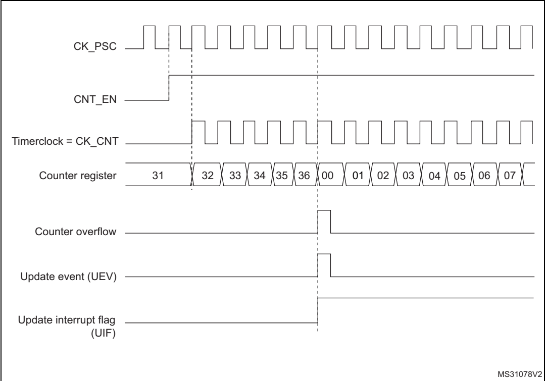
Figure 389. Counter timing diagram, internal clock divided by 1
