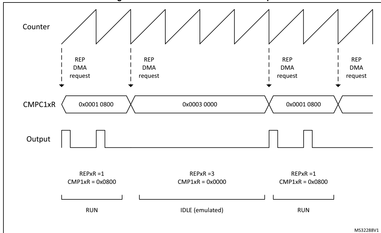
Figure 364. Burst mode emulation example
