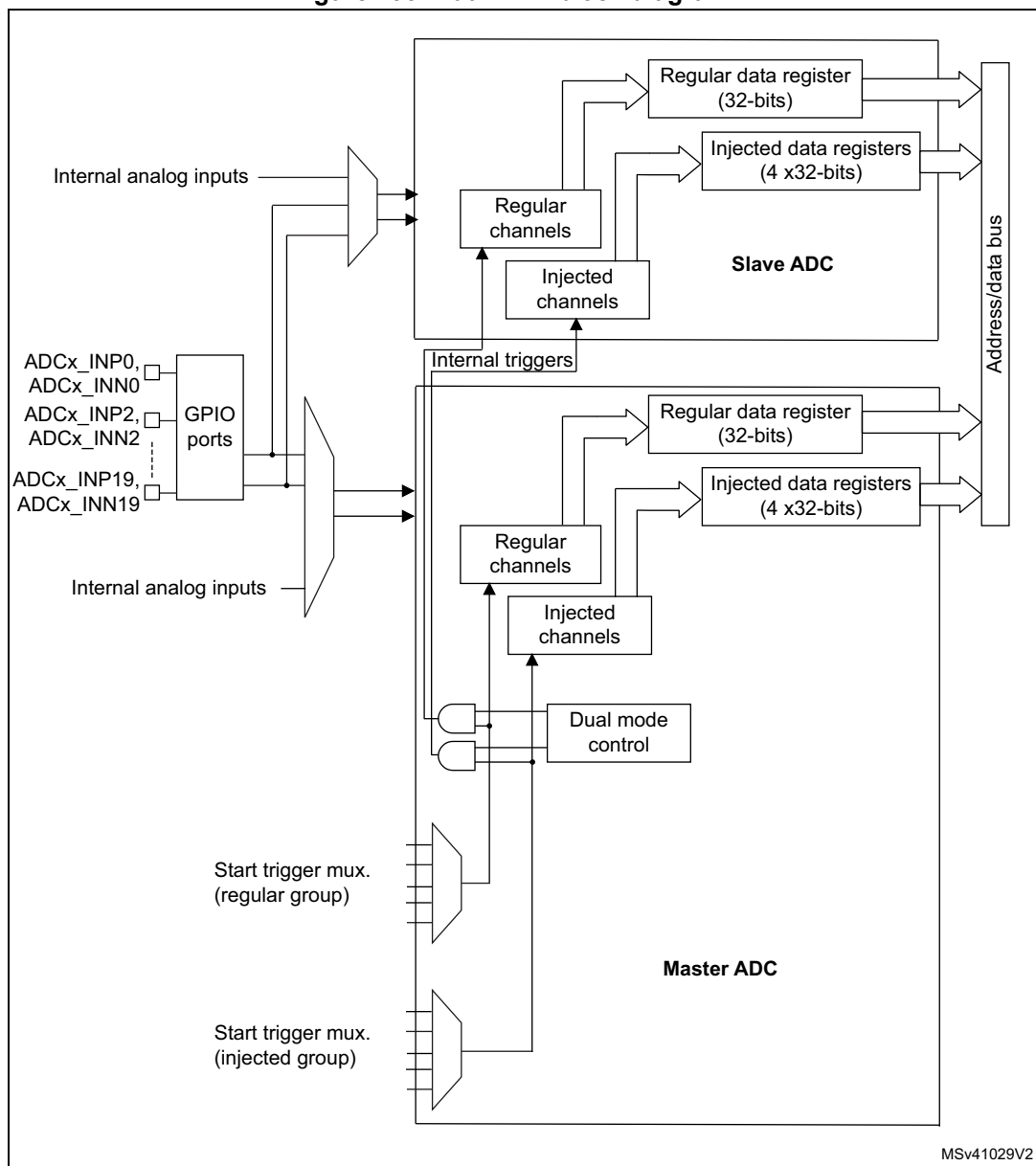
Figure 193. Dual ADC block diagram (1)
