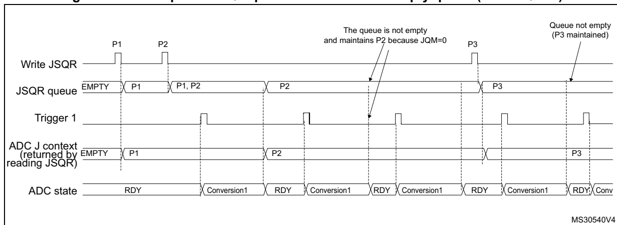
Figure 159. Example of JSQR queue of context with empty queue (case JQM=0)
