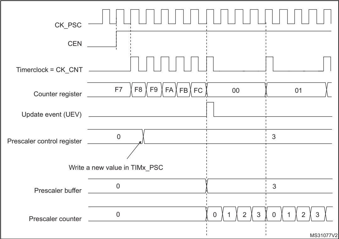
Figure 499. Counter timing diagram with prescaler division change from 1 to 4
