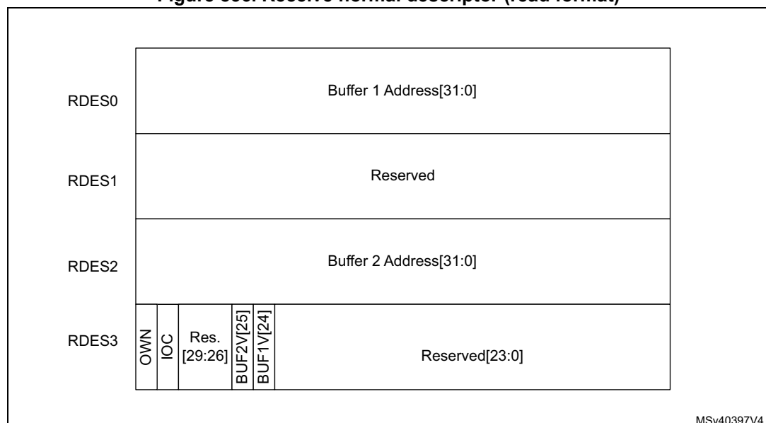
Figure 856. Receive normal descriptor (read format)
