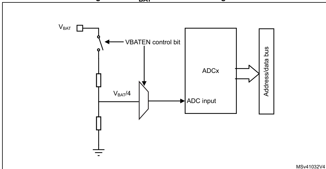
Figure 210. V_{BAT} channel block diagram
