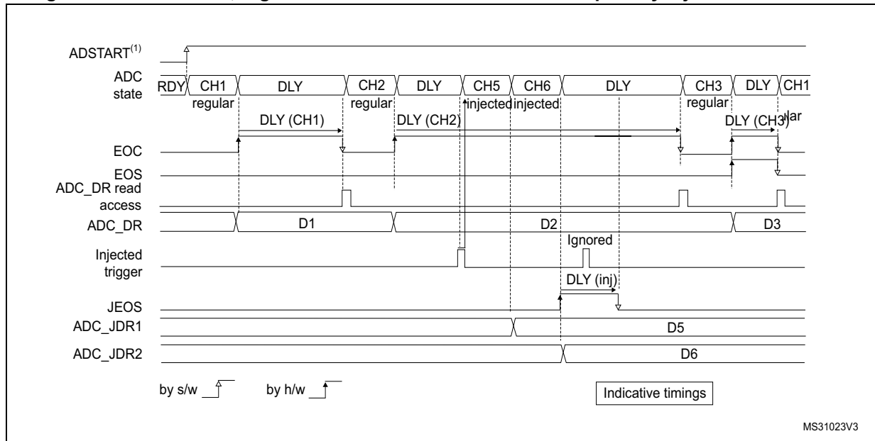
Figure 180. AUTDLY=1, regular continuous conversions interrupted by injected conversions
