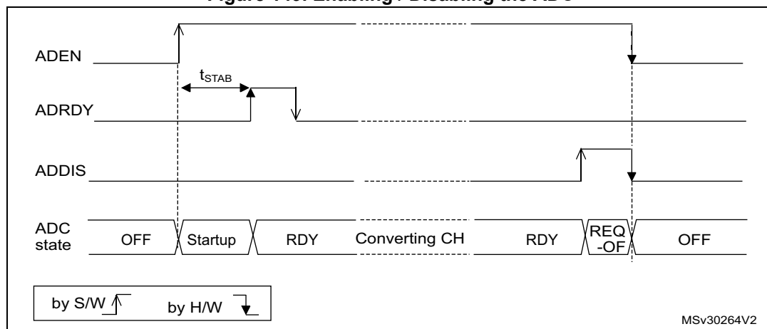
Figure 149. Enabling / Disabling the ADC
