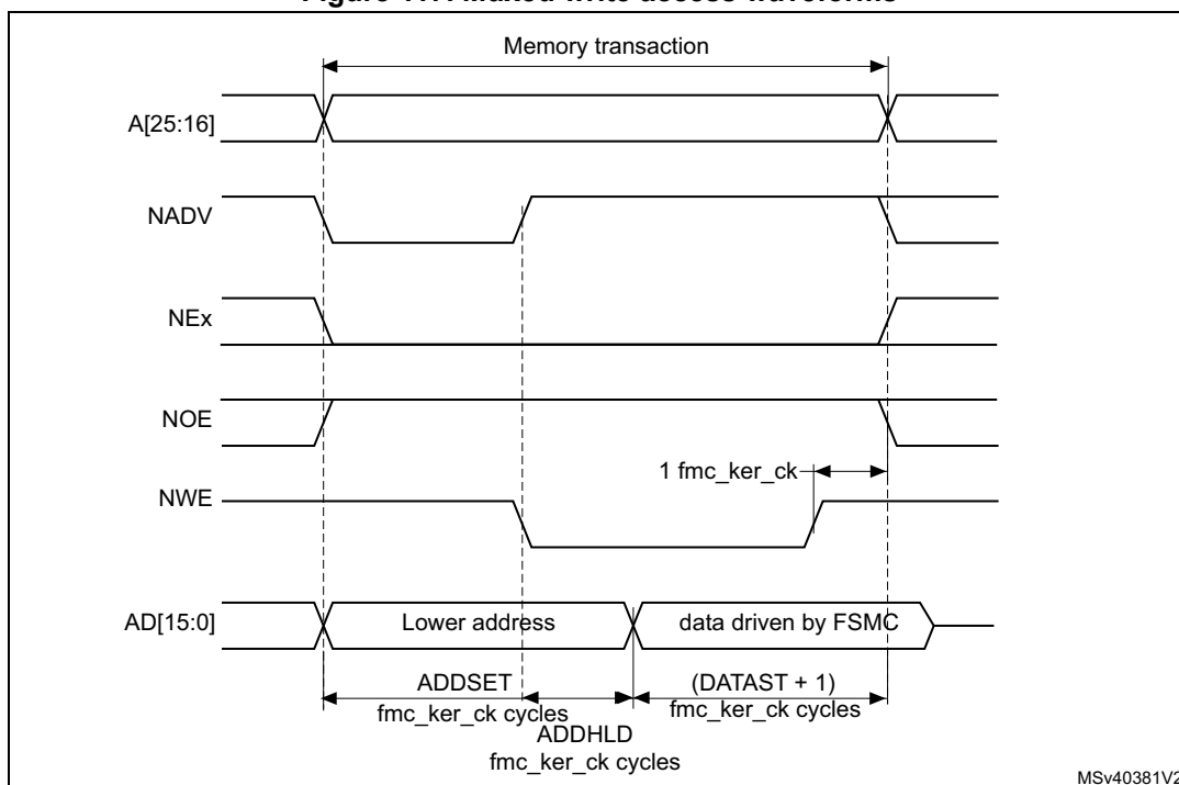
Figure 117. Muxed write access waveforms
