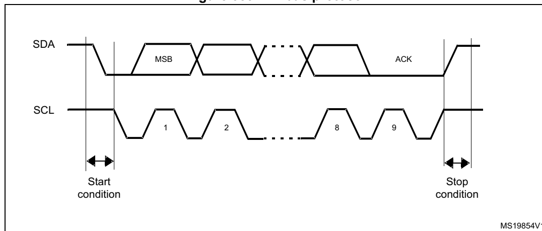
Figure 583. I 2 C bus protocol
