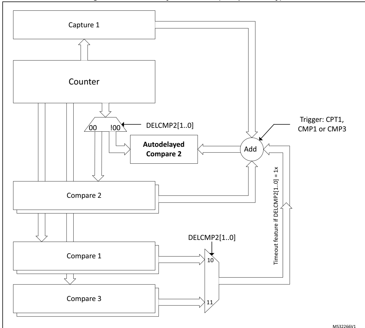
Figure 332. Auto-delayed overview (Compare 2 only)
