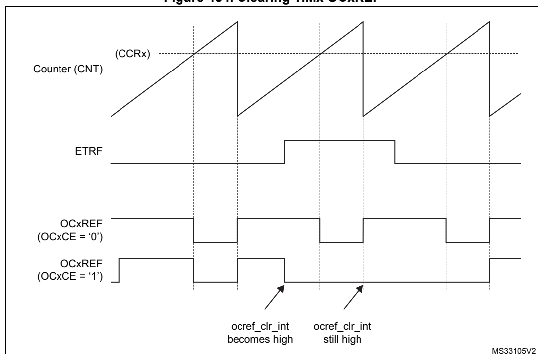
Figure 434. Clearing TIMx OCxREF
