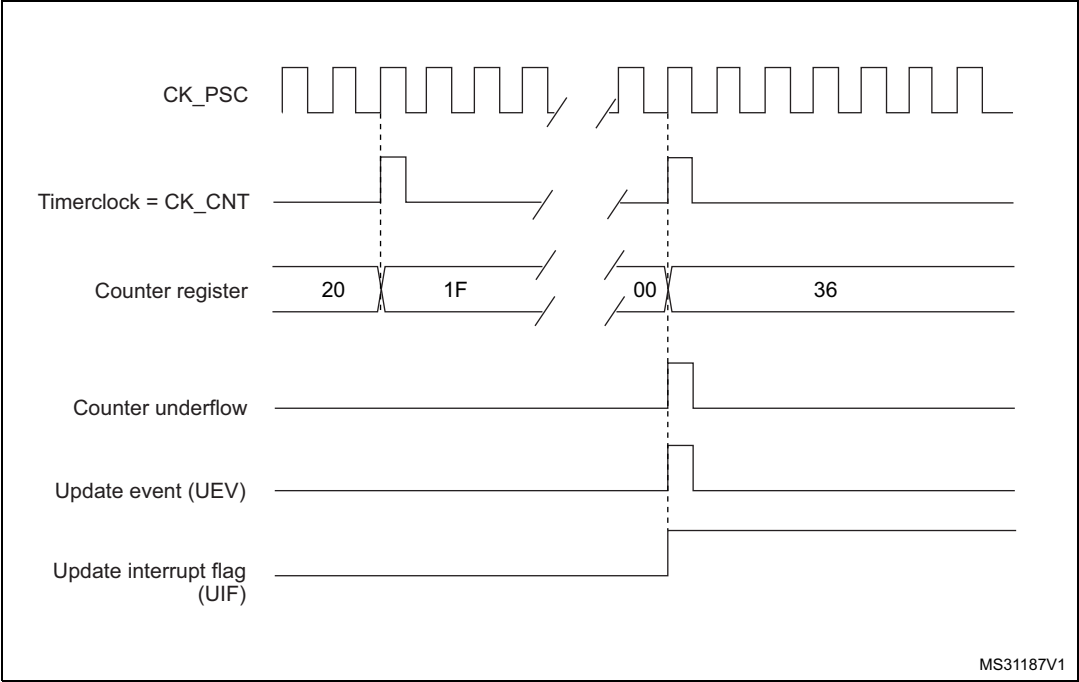
Figure 398. Counter timing diagram, internal clock divided by N
