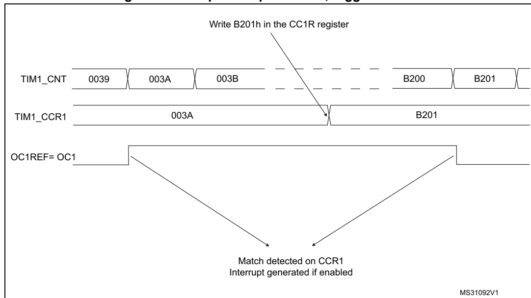
Figure 513. Output compare mode, toggle on OC1.
