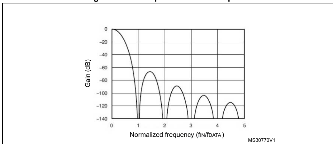
Figure 241. Example: Sinc 3 filter response
