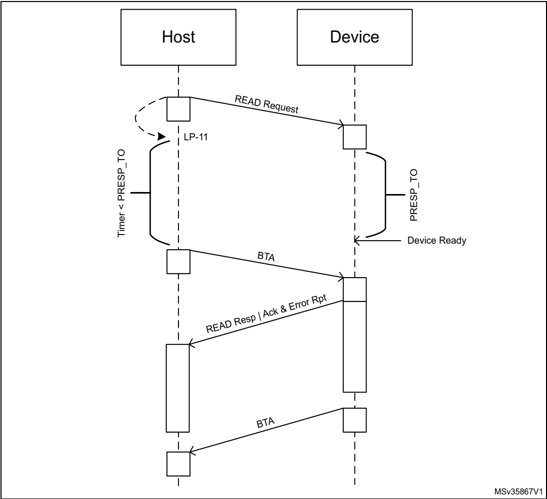
Figure 267. Timing of PRESP_TO after a read request (HS or LP)
