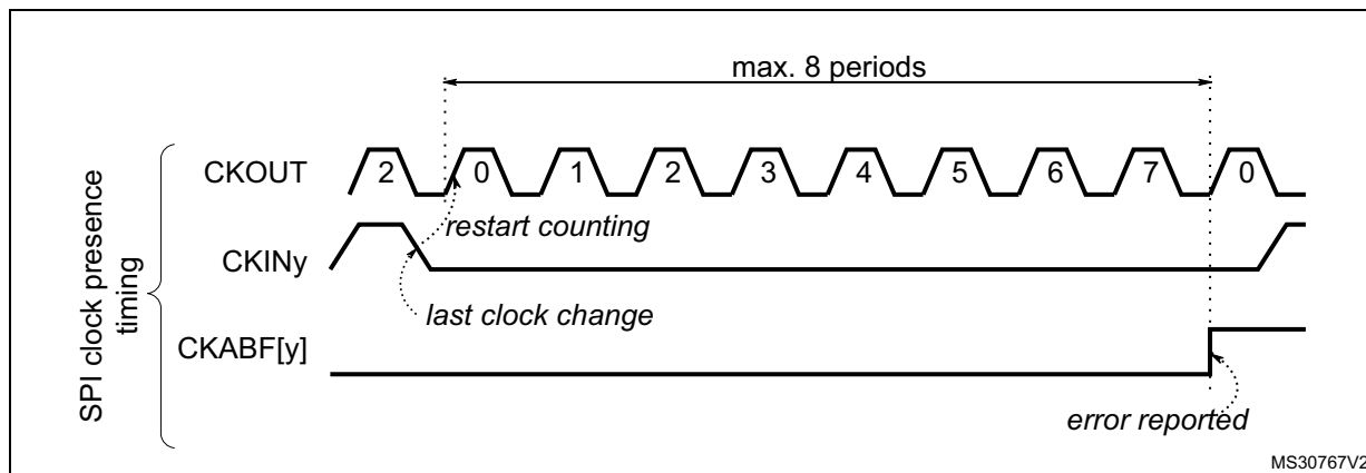
Figure 237. Clock absence timing diagram for SPI
