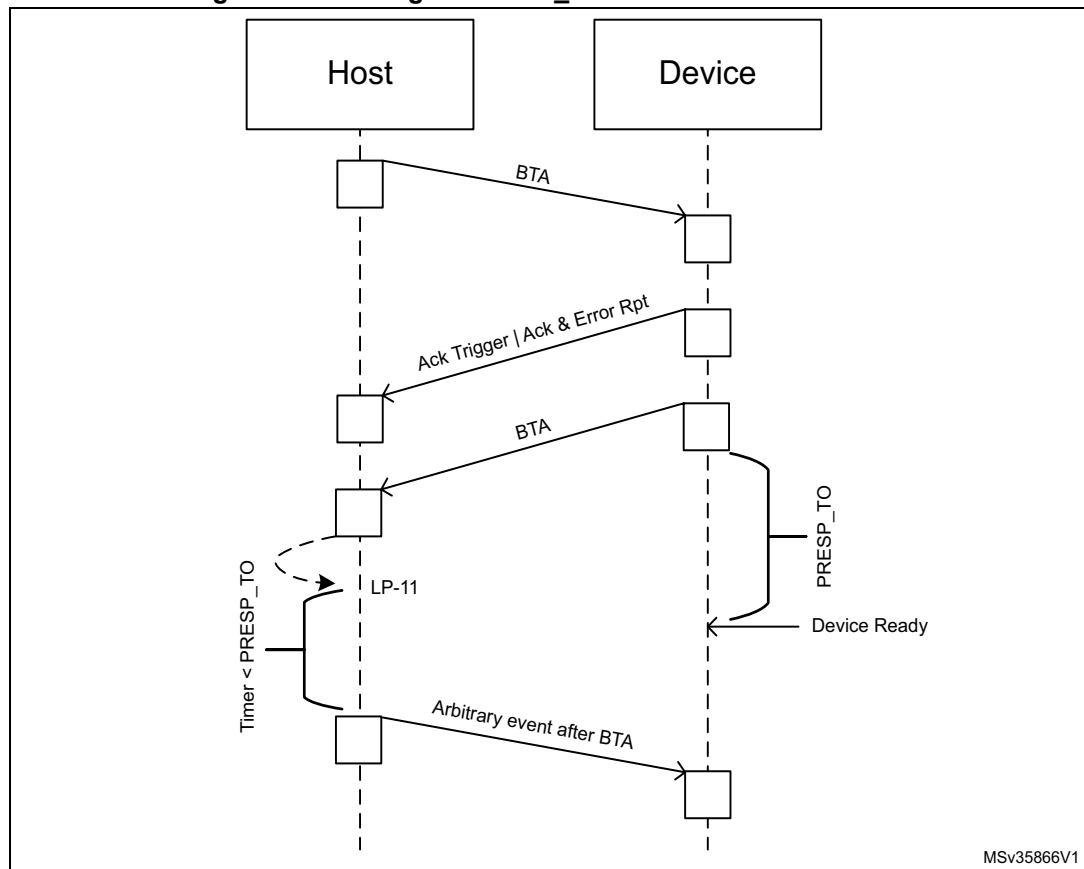
Figure 266. Timing of PRESP_TO after a bus-turn-around
