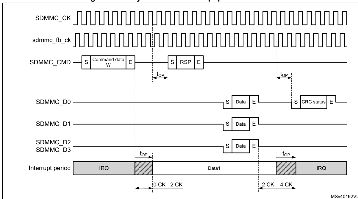
Figure 761. Asynchronous interrupt period data write
