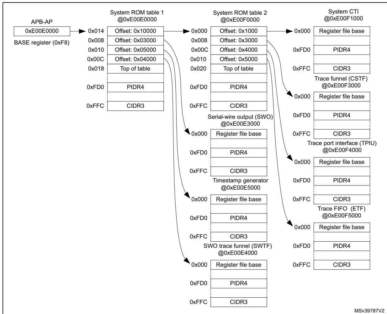
Figure 876. APB-D CoreSight component topology
