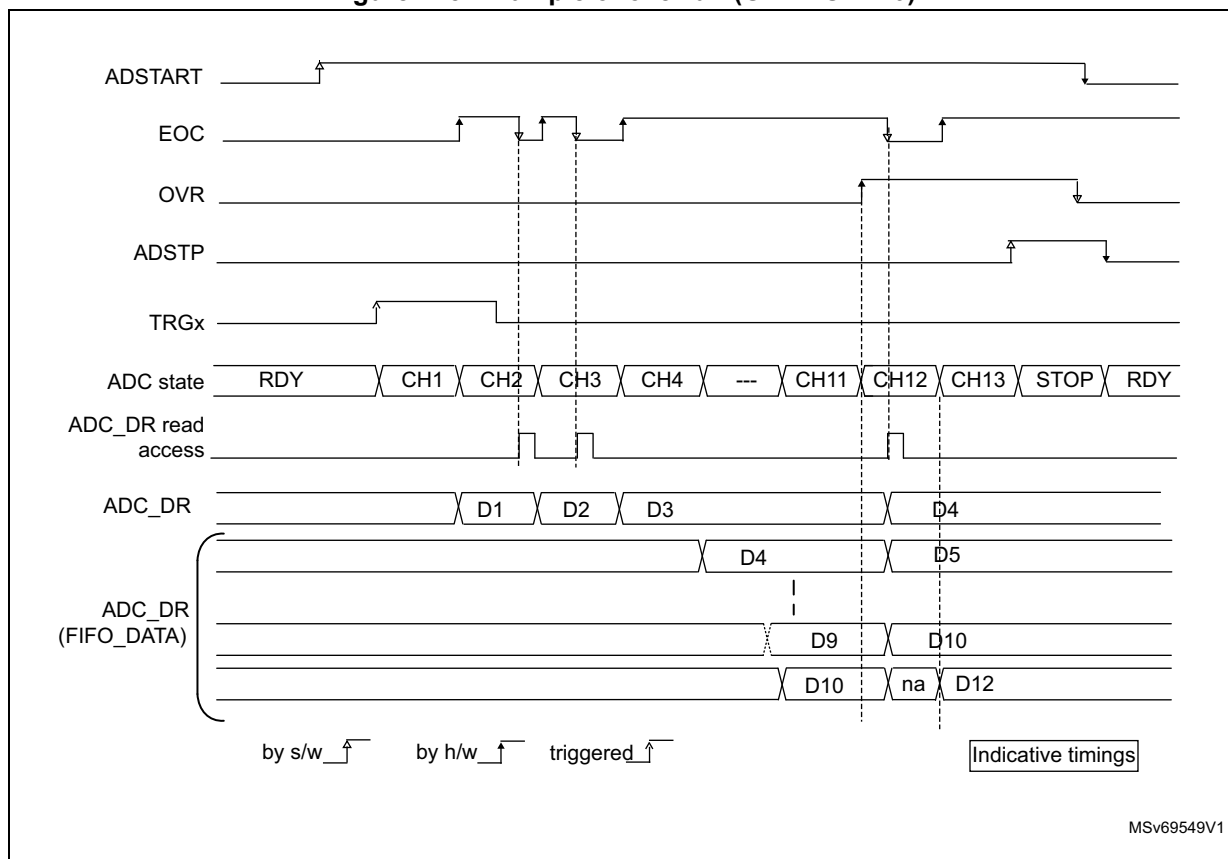
Figure 176. Example of overrun (OVRMOD = 1)
