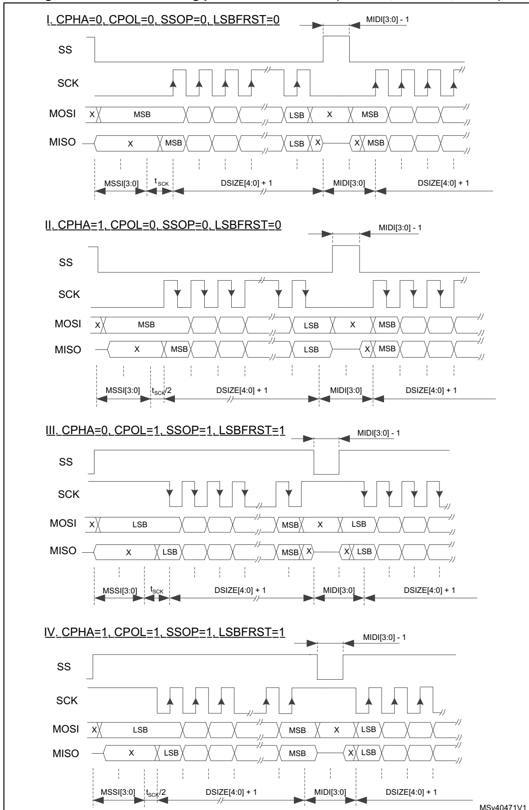
Figure 663. SS interleaving pulses between data (SSOE=1, SSOM=1,SSM=0)
