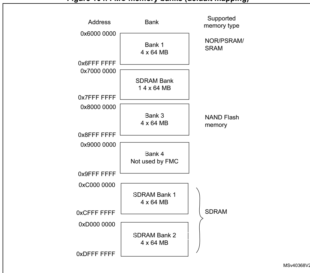
Figure 104. FMC memory banks (default mapping)
