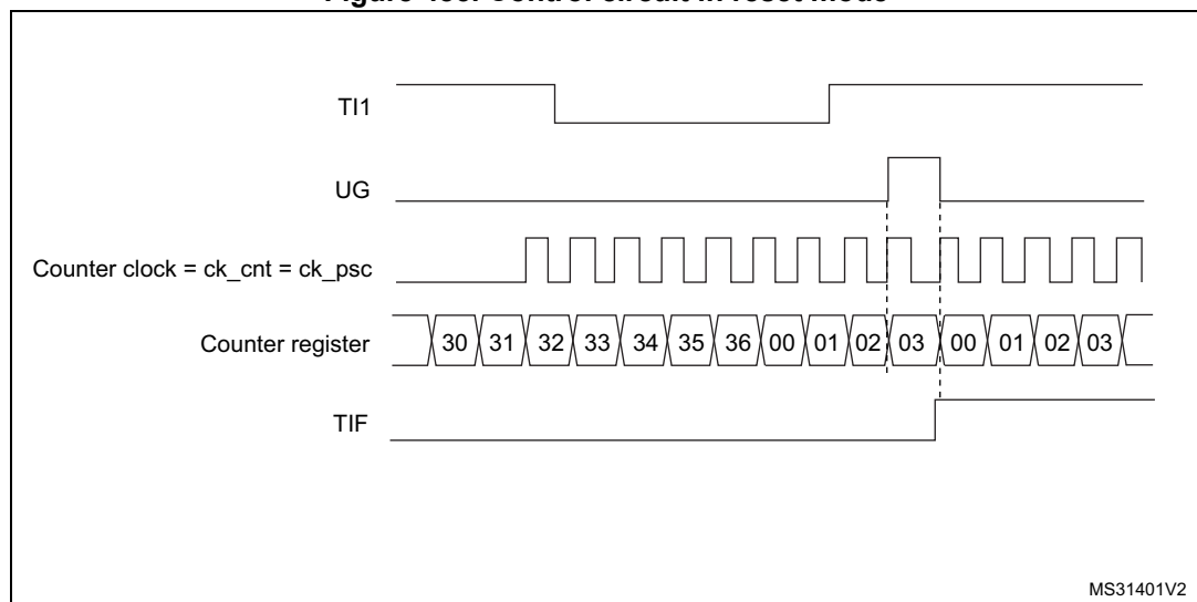
Figure 485. Control circuit in reset mode
