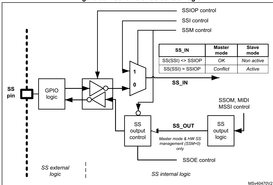
Figure 661. Scheme of SS control logic
