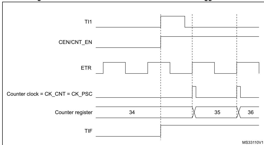
Figure 488. Control circuit in external clock mode 2 + trigger mode
