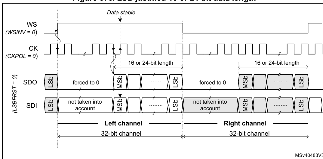
Figure 676. LSB justified 16 or 24-bit data length
