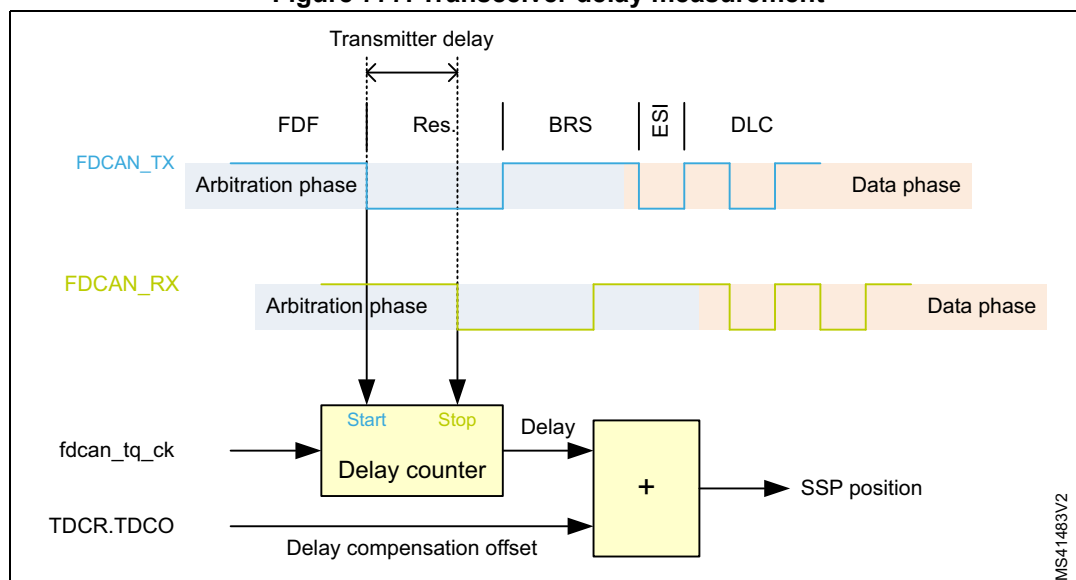
Figure 777. Transceiver delay measurement
