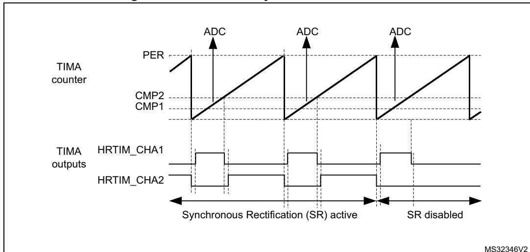
Figure 381. Buck with synchronous rectification
