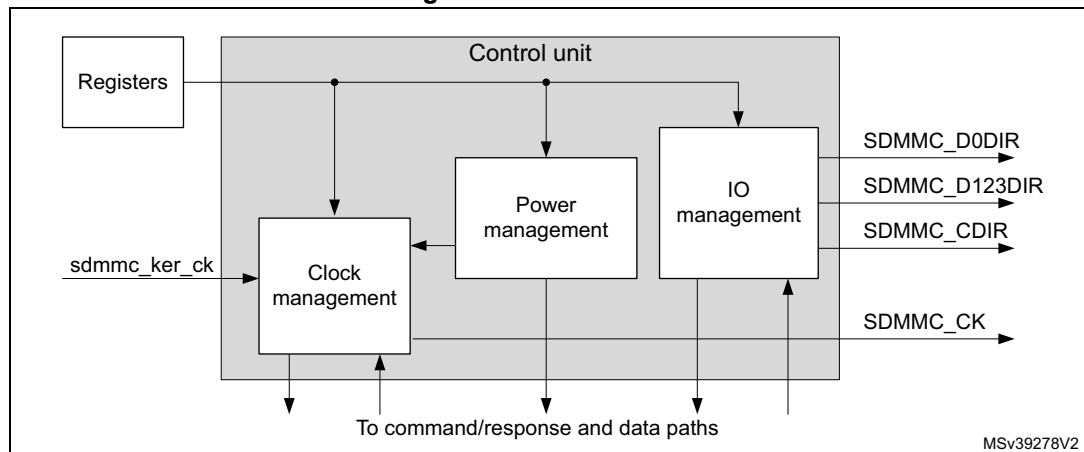
Figure 749. Control unit
