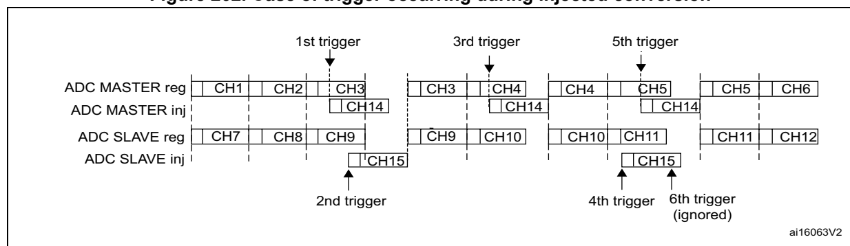
Figure 202. Case of trigger occurring during injected conversion
