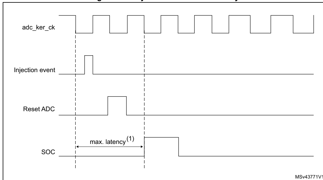
Figure 154. Injected conversion latency
