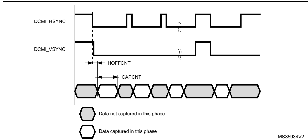
Figure 248. Data capture waveforms
