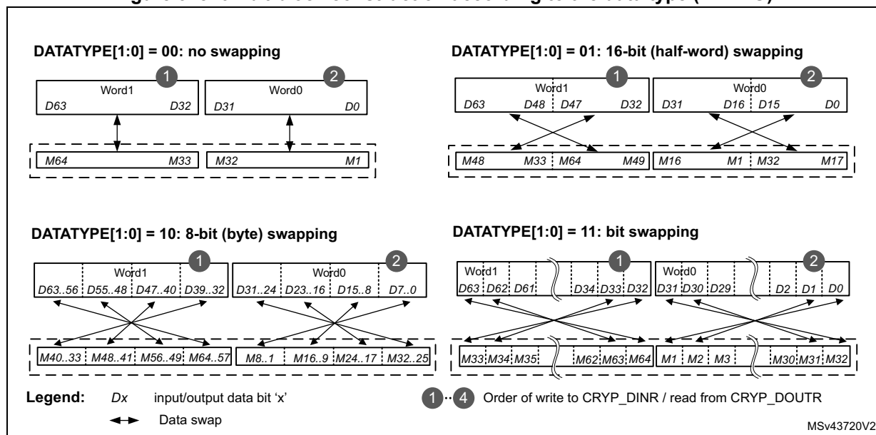
Figure 318. 64-bit block construction according to the data type (IN FIFO)
