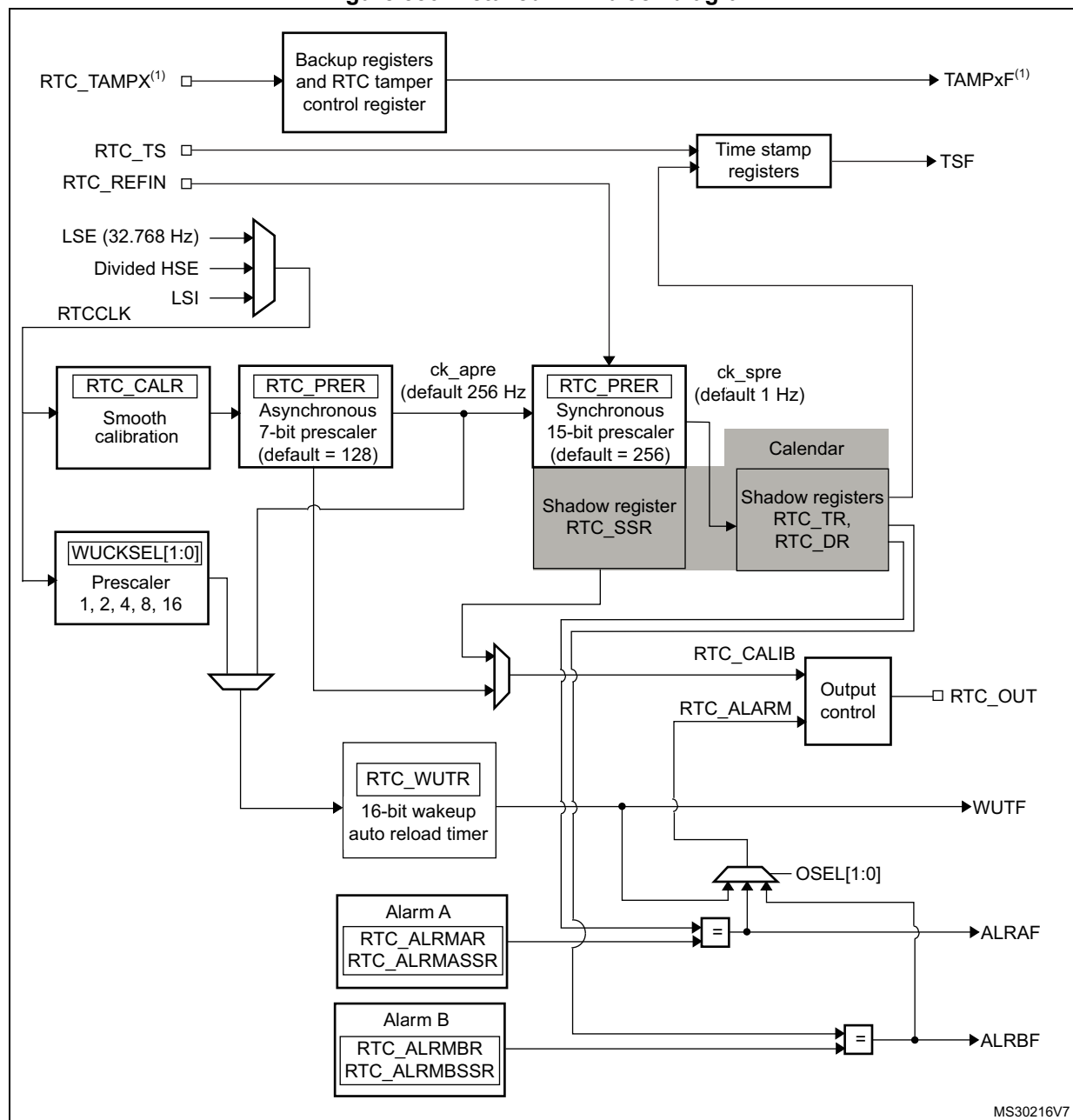
Figure 580. Detailed RTC block diagram
