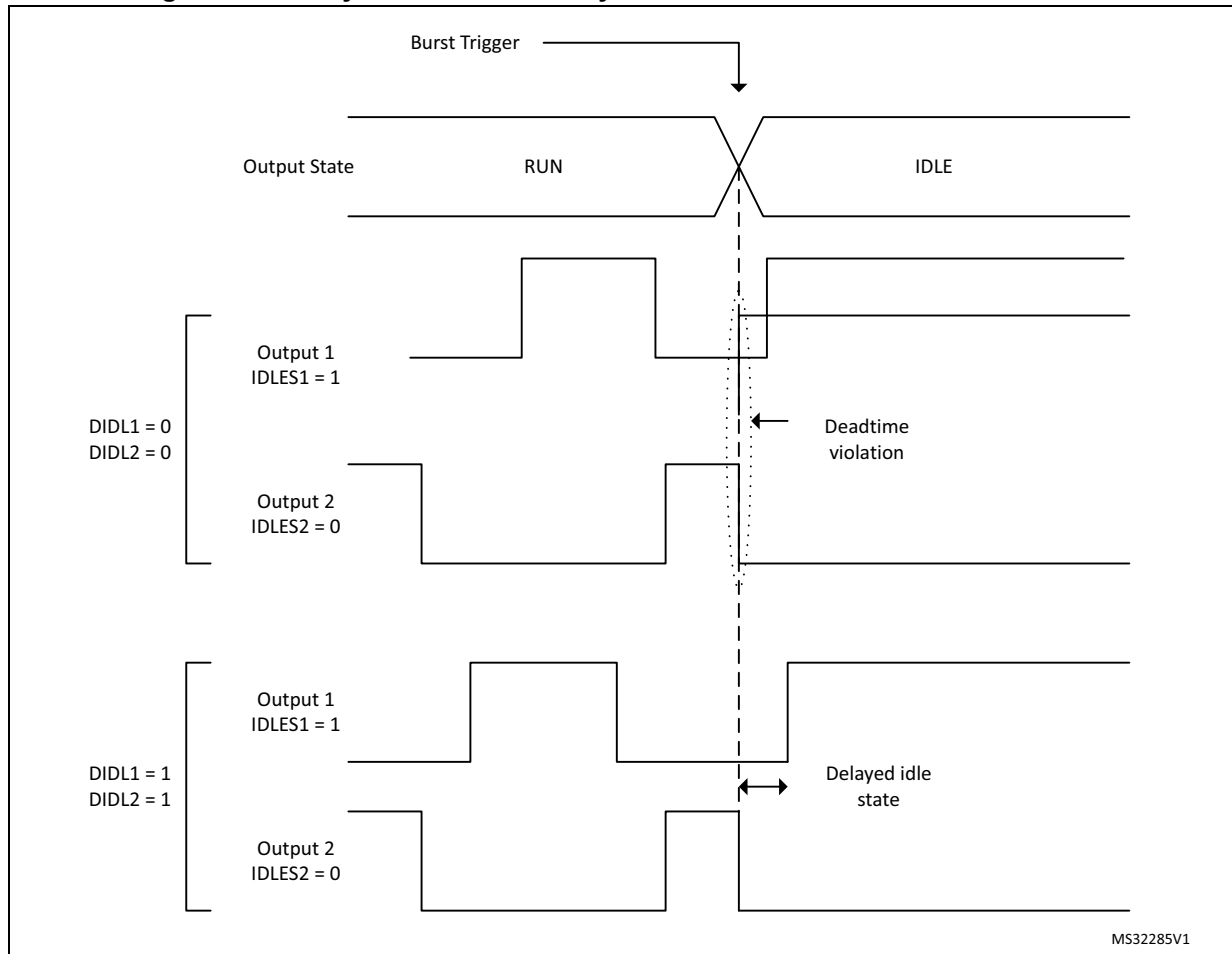
Figure 361. Delayed burst mode entry with deadtime enabled and IDLESx = 1
