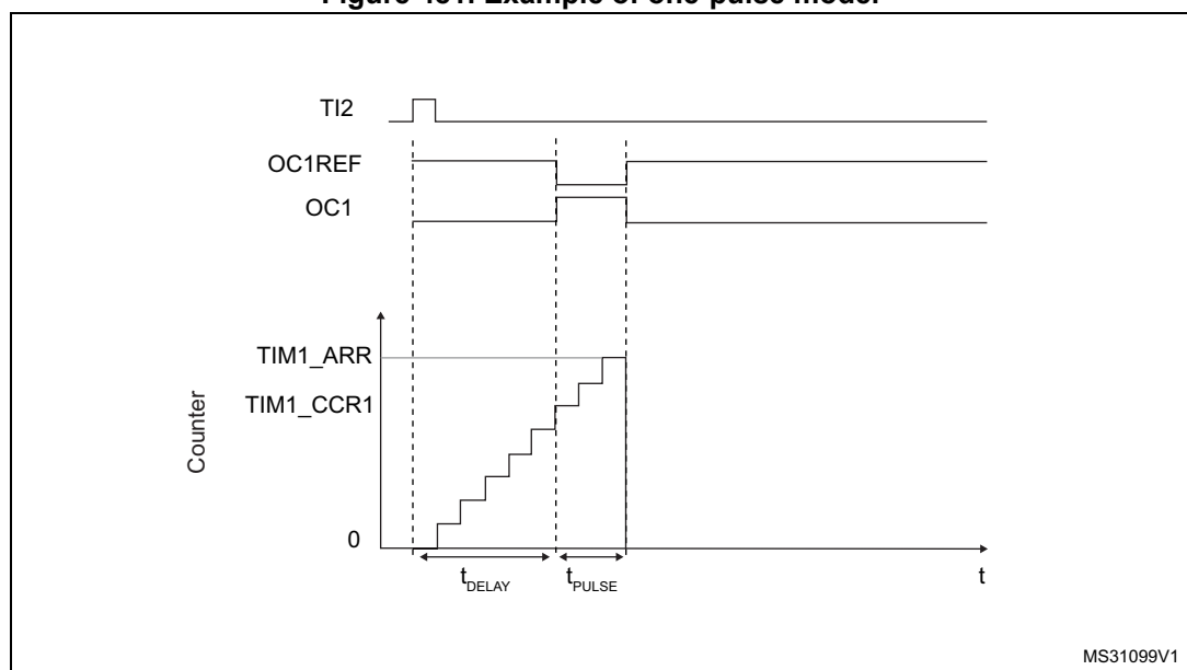
Figure 481. Example of one-pulse mode.
