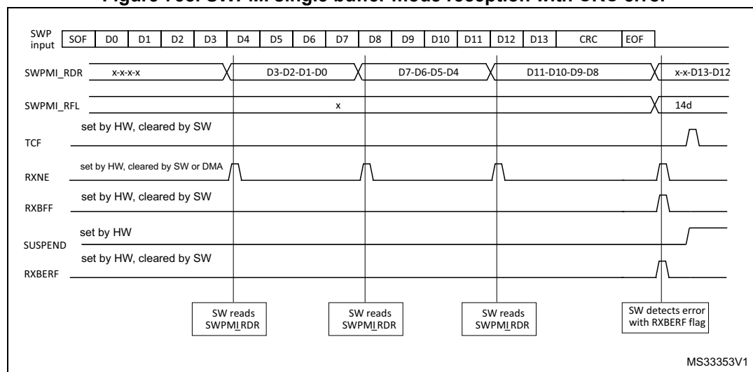
Figure 738. SWPMI single buffer mode reception with CRC error
