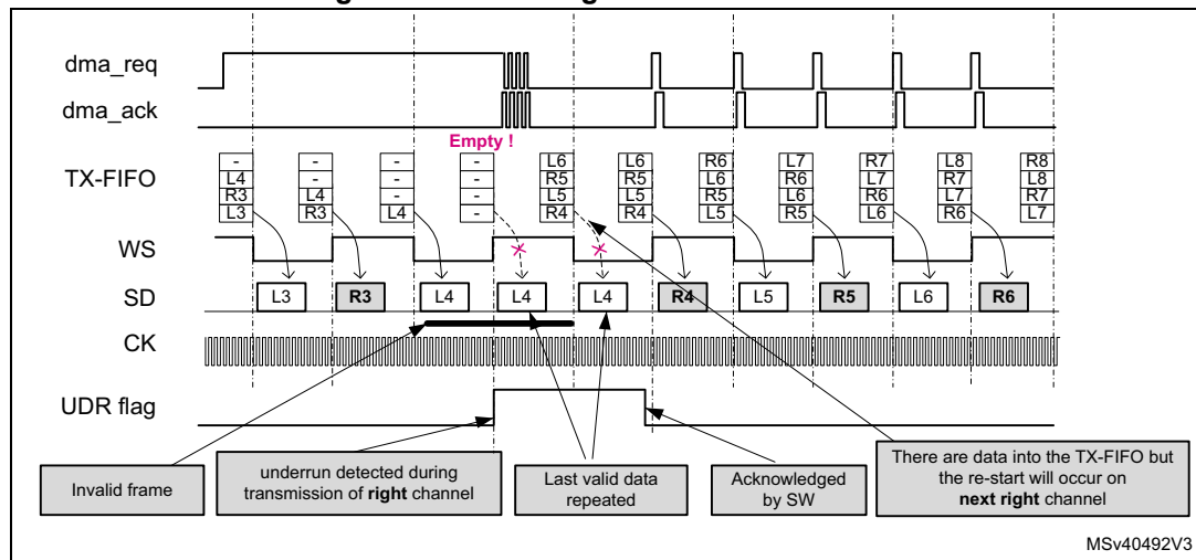
Figure 685. Handling of underrun situation
