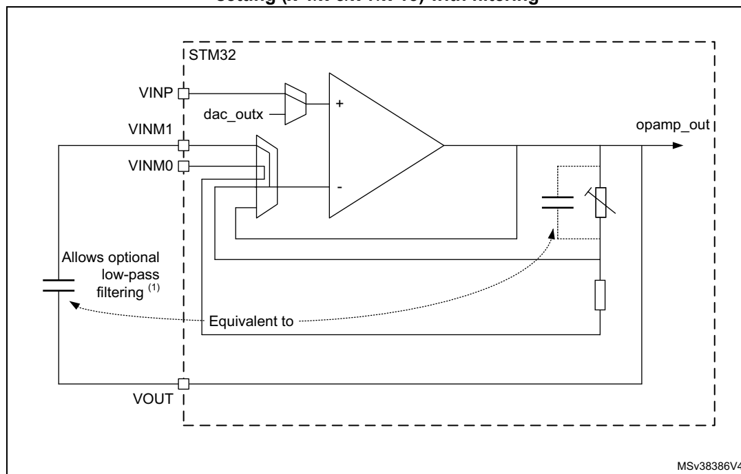
Figure 232. PGA mode, non-inverting gain setting (x2/x4/x8/x16) or inverting gain setting (x-1/x-3/x-7/x-15) with filtering
