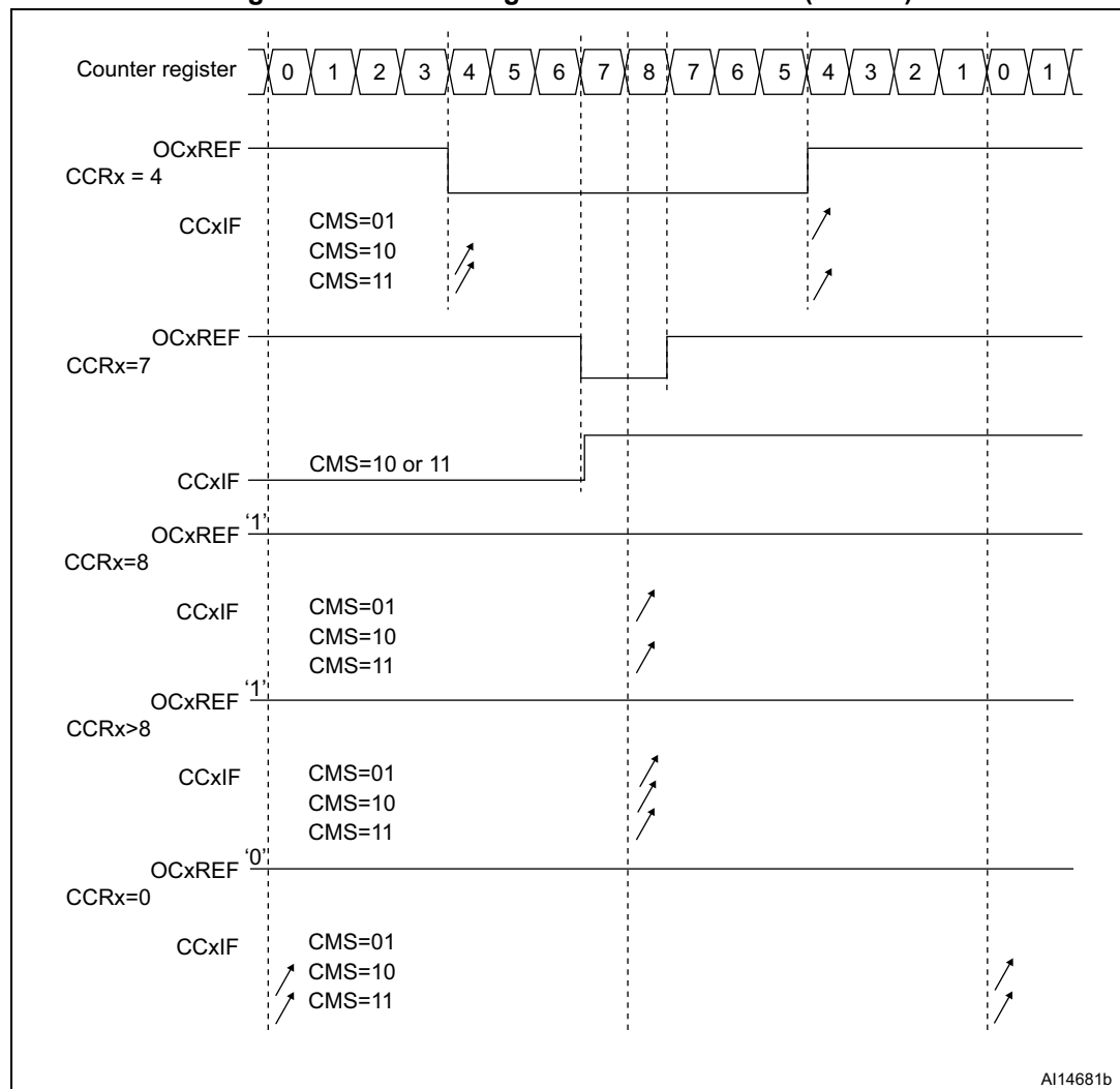
Figure 477. Center-aligned PWM waveforms (ARR=8)
