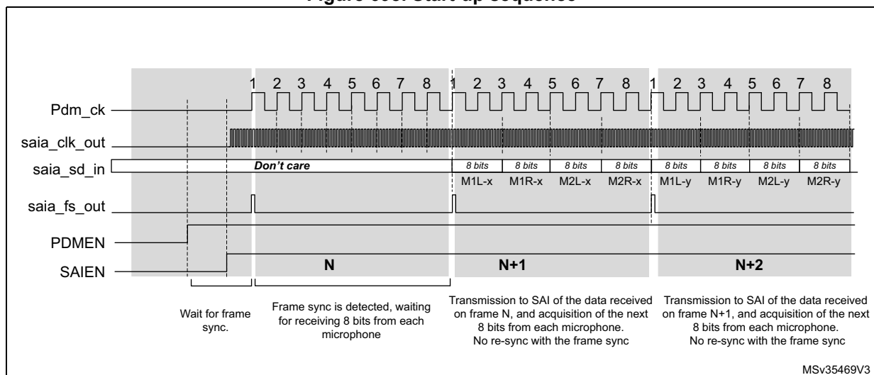
Figure 698. Start-up sequence
