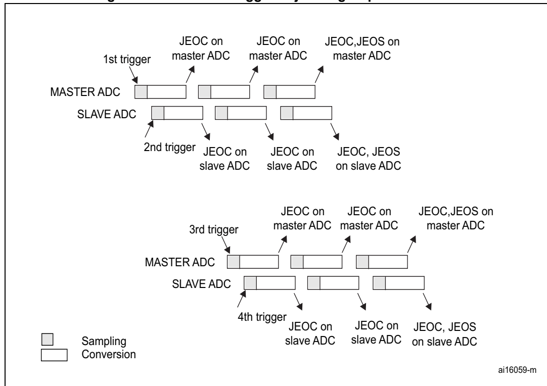
Figure 199. Alternate trigger: injected group of each ADC
