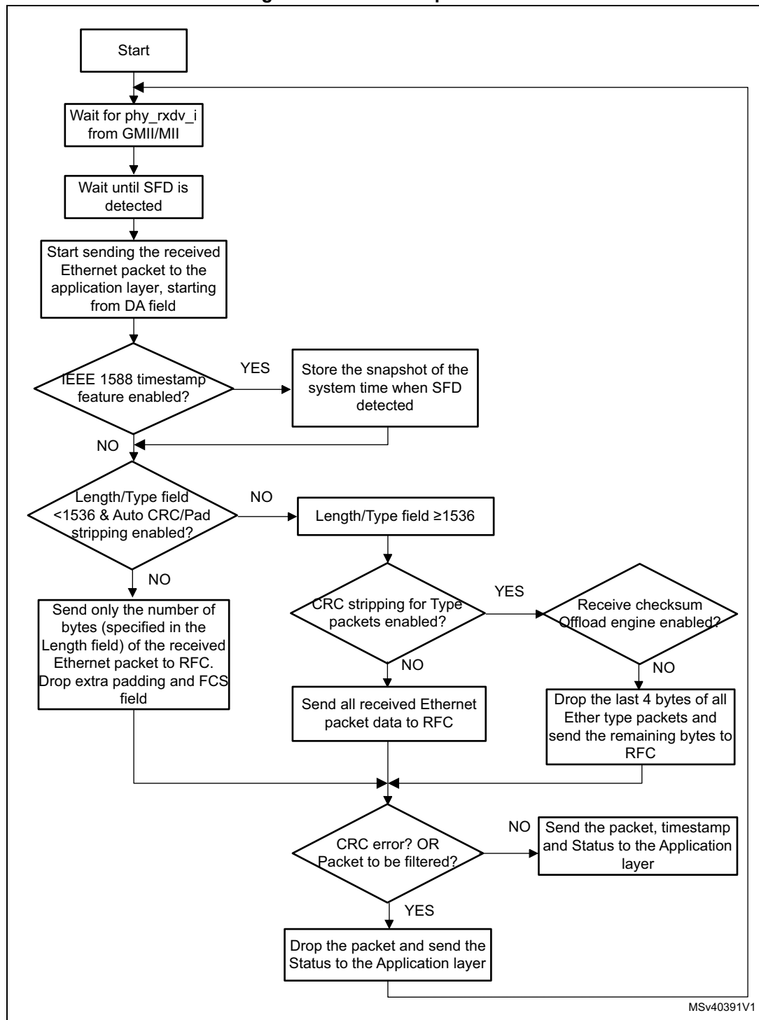
Figure 829. MAC reception flow
