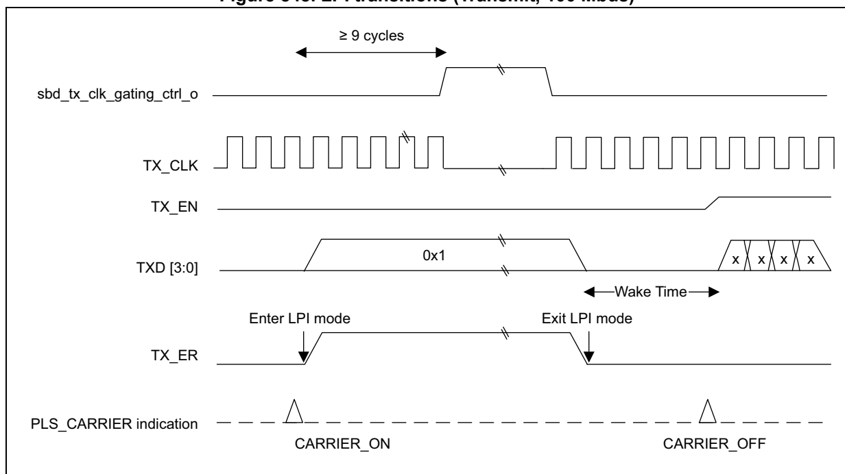
Figure 848. LPI transitions (Transmit, 100 Mbps)
