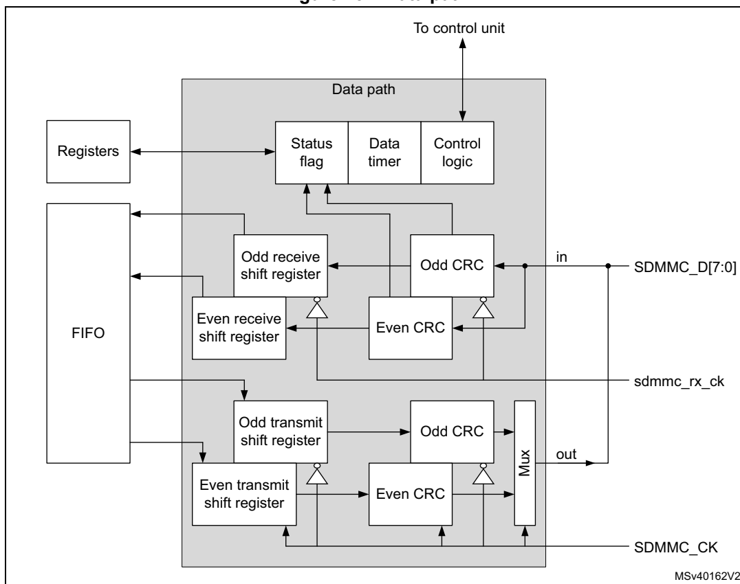
Figure 752. Data path
