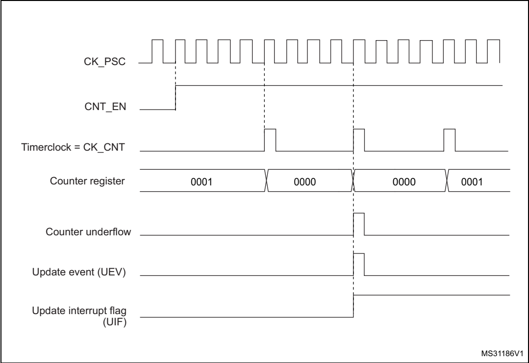
Figure 397. Counter timing diagram, internal clock divided by 4
