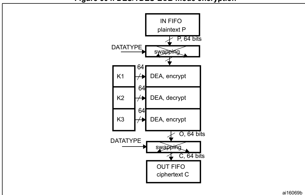
Figure 304. DES/TDES-ECB mode encryption
