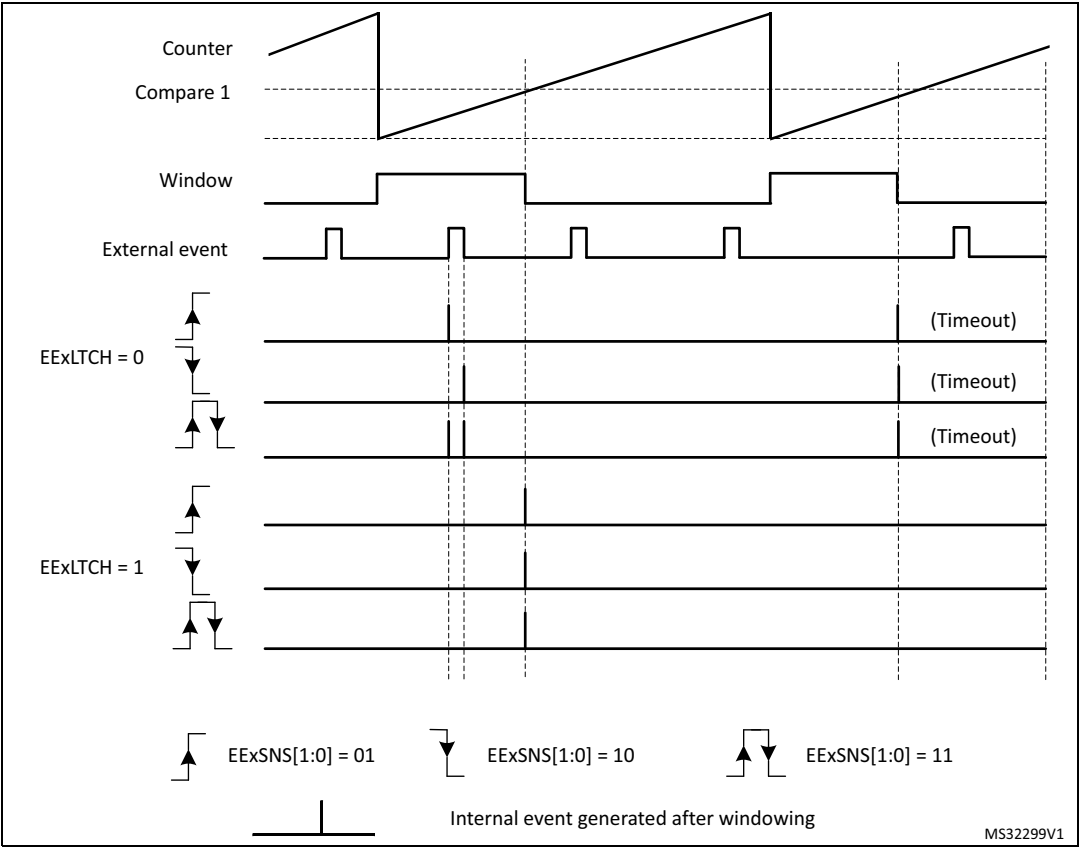
Figure 351. External trigger windowing with edge-sensitive trigger
