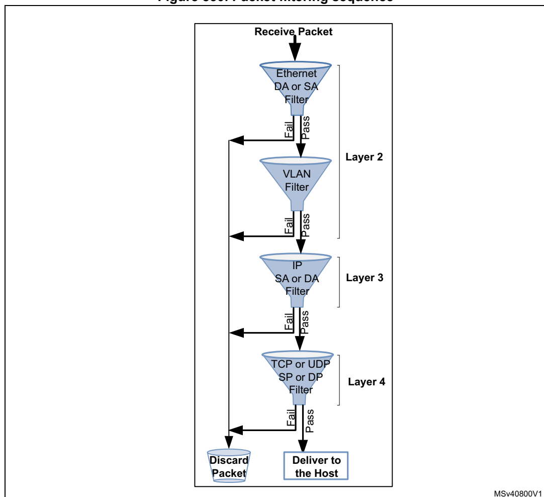
Figure 830. Packet filtering sequence
