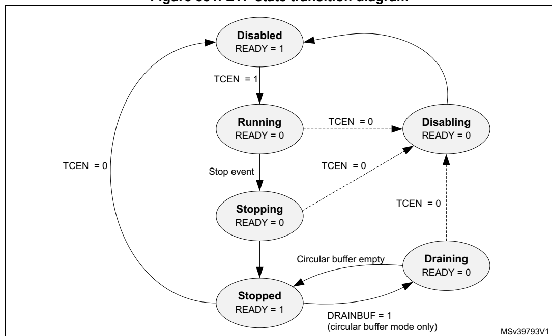
Figure 881. ETF state transition diagram
