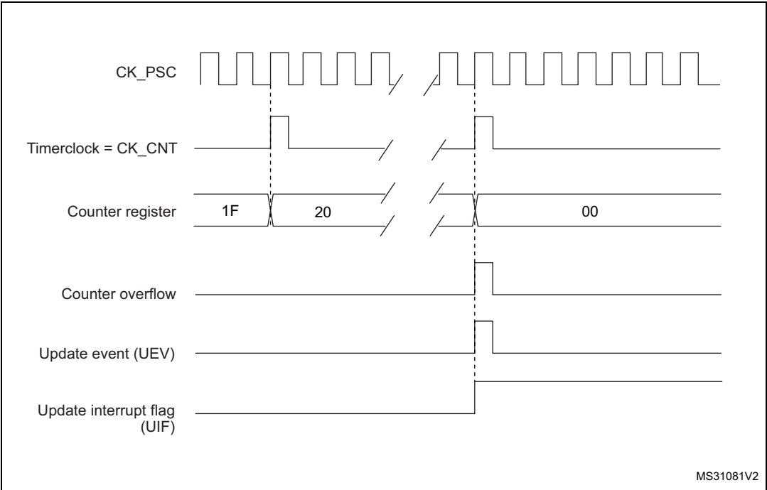
Figure 562. Counter timing diagram, internal clock divided by N
