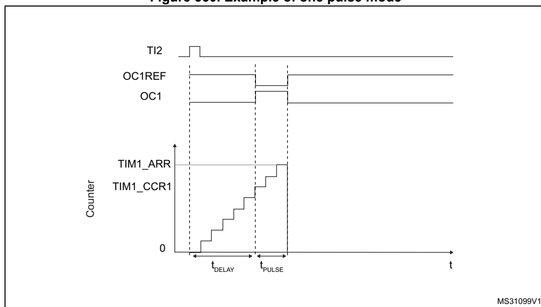
Figure 550. Example of one pulse mode
