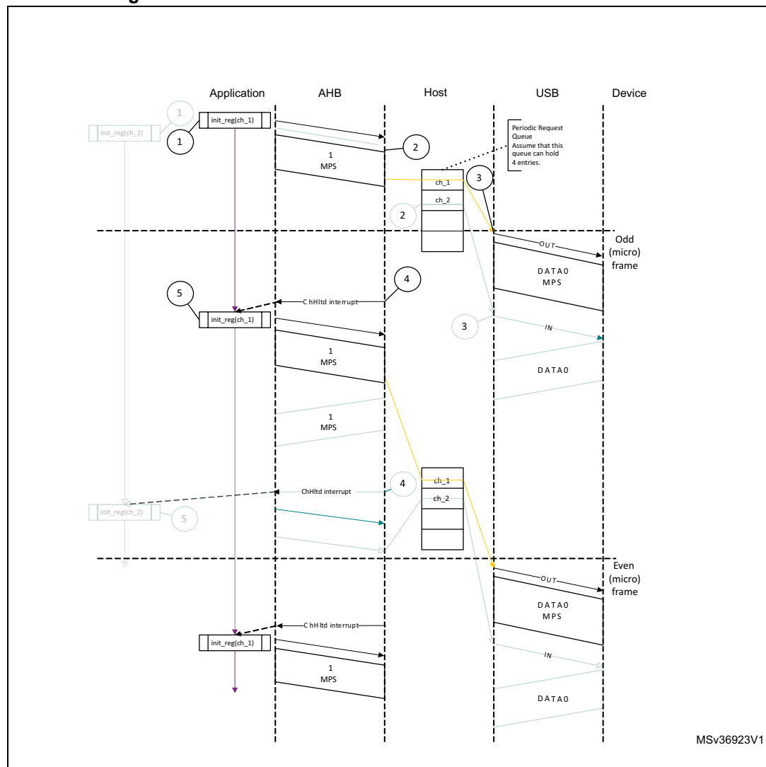
Figure 814. Normal isochronous OUT transaction - DMA mode
