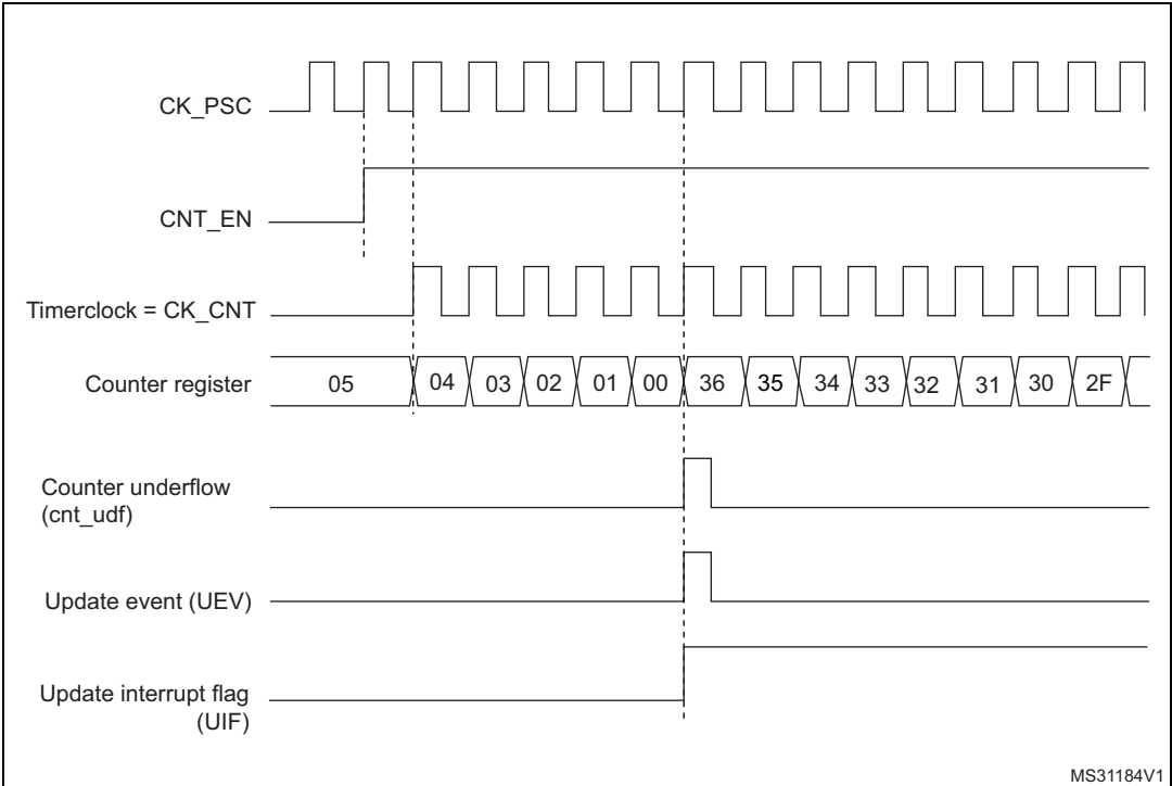
Figure 455. Counter timing diagram, internal clock divided by 1
