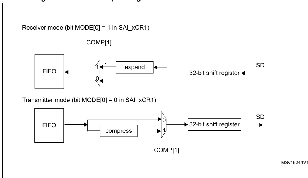
Figure 706. Data companding hardware in an audio block in the SAI
