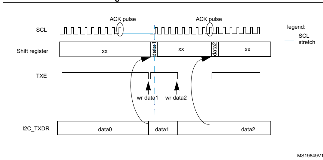
Figure 587. Data transmission
