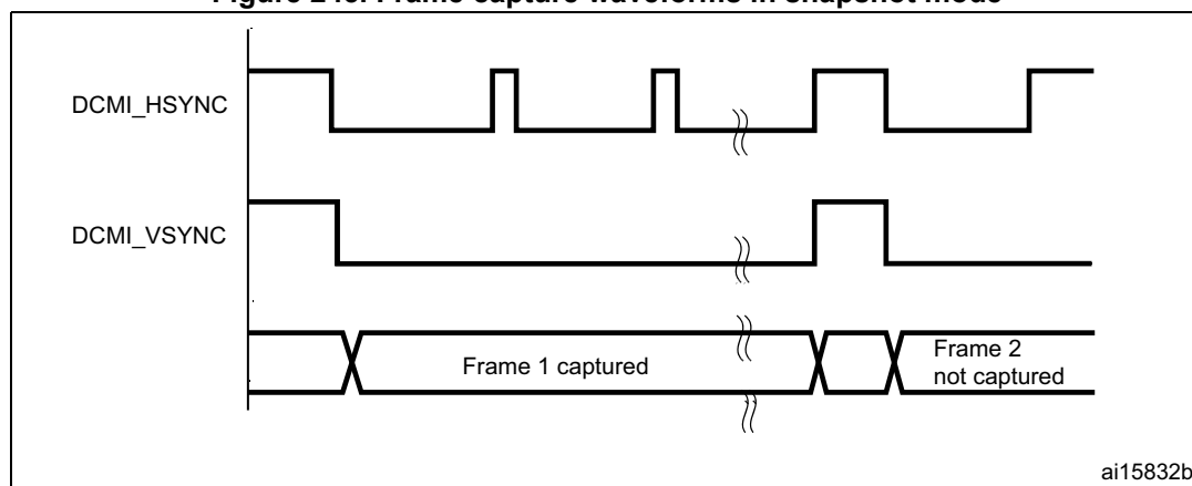
Figure 245. Frame capture waveforms in snapshot mode
