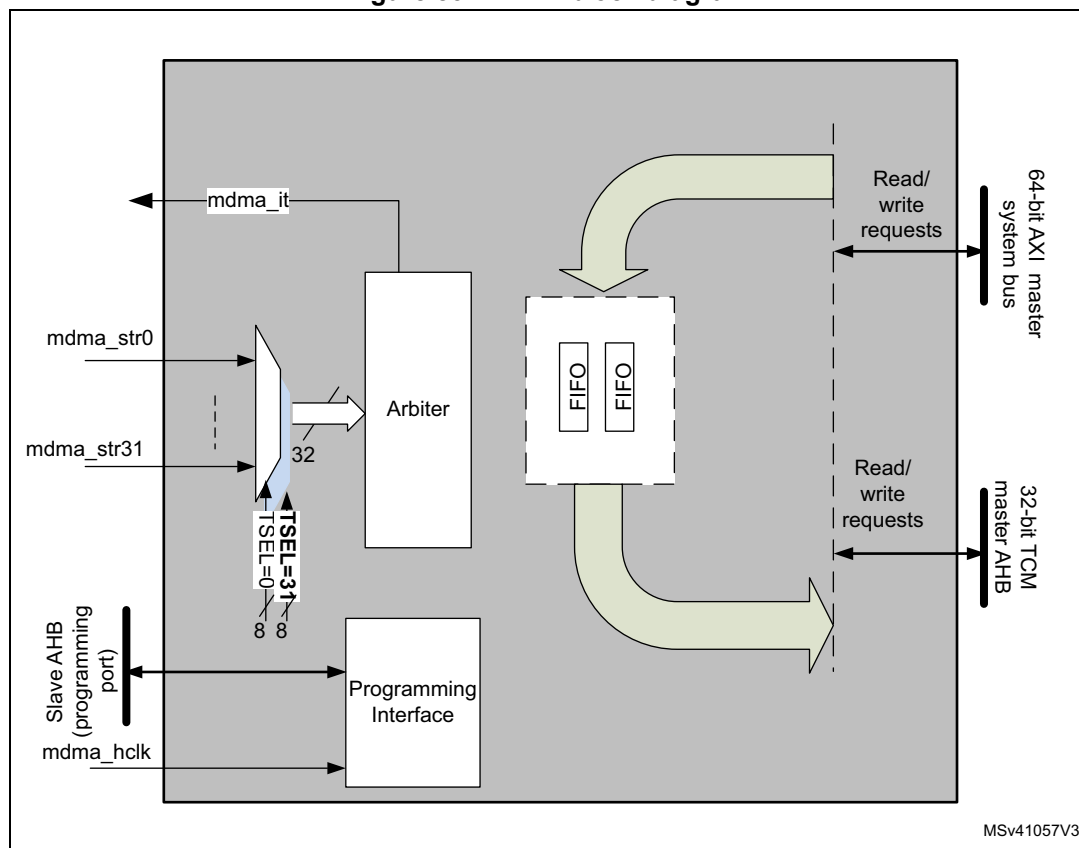
Figure 83. MDMA block diagram
