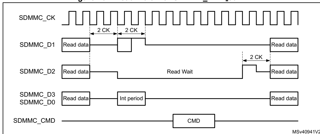
Figure 764. Read Wait with SDMMC_CLK < 50 MHz
