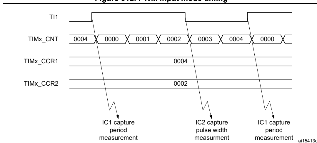
Figure 512. PWM input mode timing
