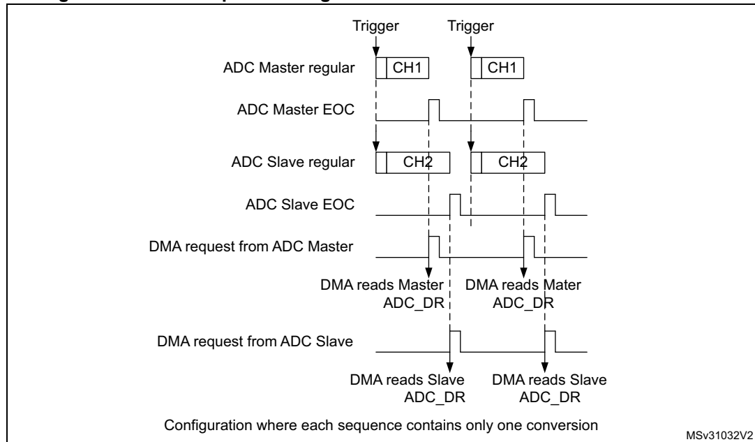
Figure 206. DMA Requests in regular simultaneous mode when DAMDF=0b00
