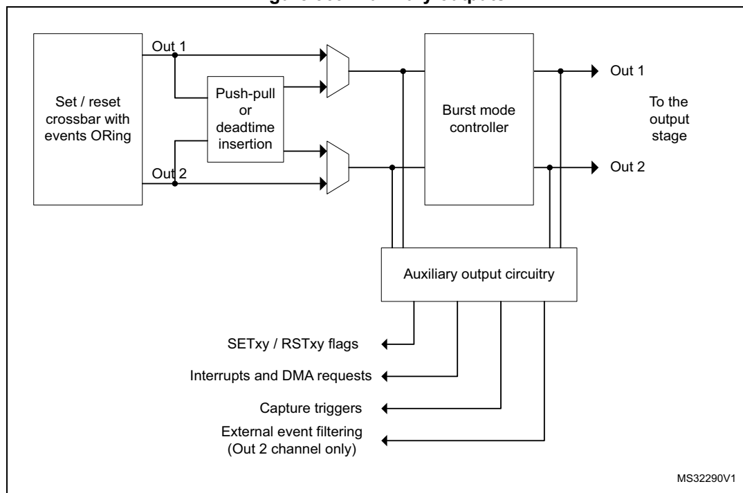
Figure 369. Auxiliary outputs
