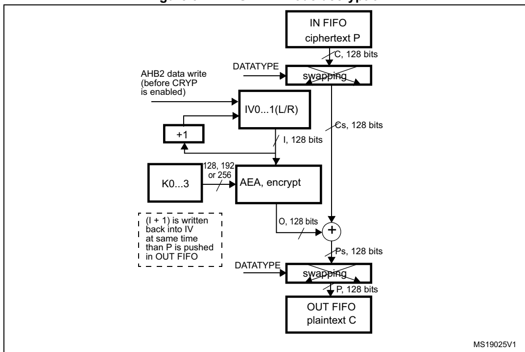
Figure 314. AES-CTR mode decryption
