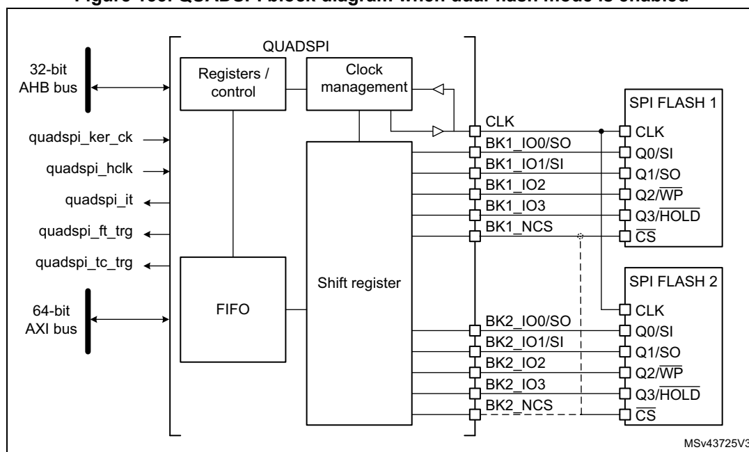
Figure 133. QUADSPI block diagram when dual-flash mode is enabled
