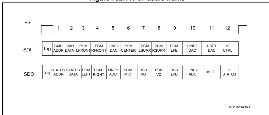
Figure 702. AC'97 audio frame
