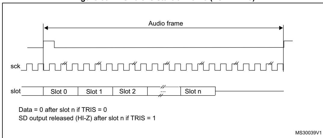
Figure 692. FS role is start of frame (FSDEF = 0)
