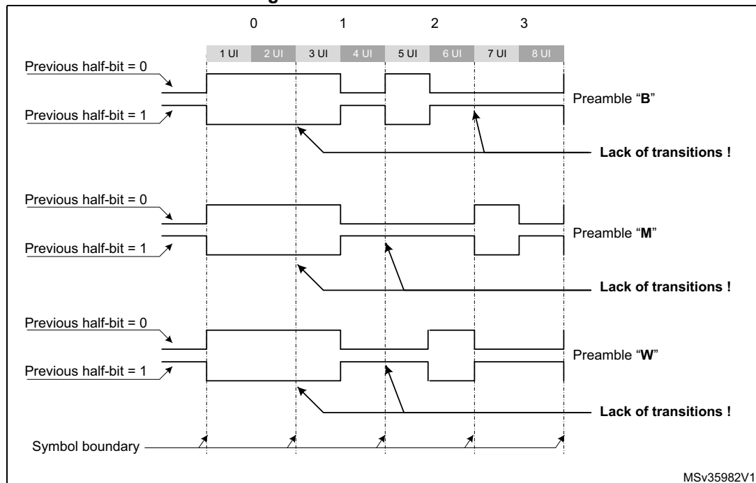
Figure 714. S/PDIF Preambles
