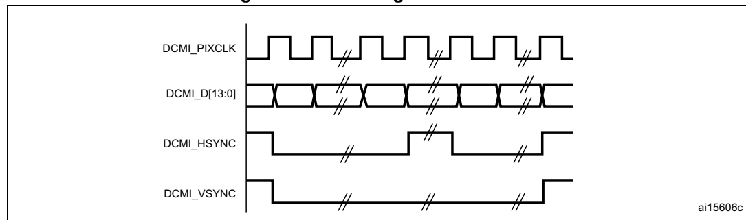
Figure 243. DCMI signal waveforms
