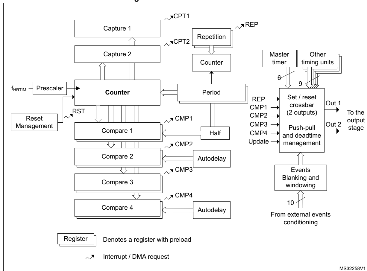
Figure 324. Timer A..E overview
