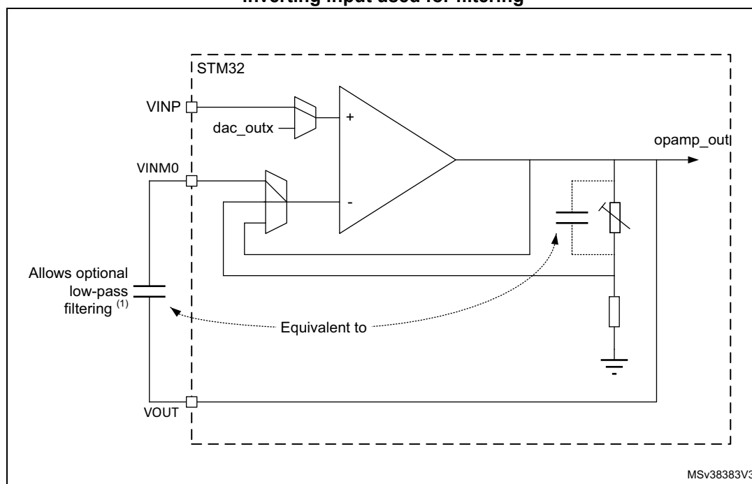
Figure 229. PGA mode, internal gain setting (x2/x4/x8/x16), inverting input used for filtering
