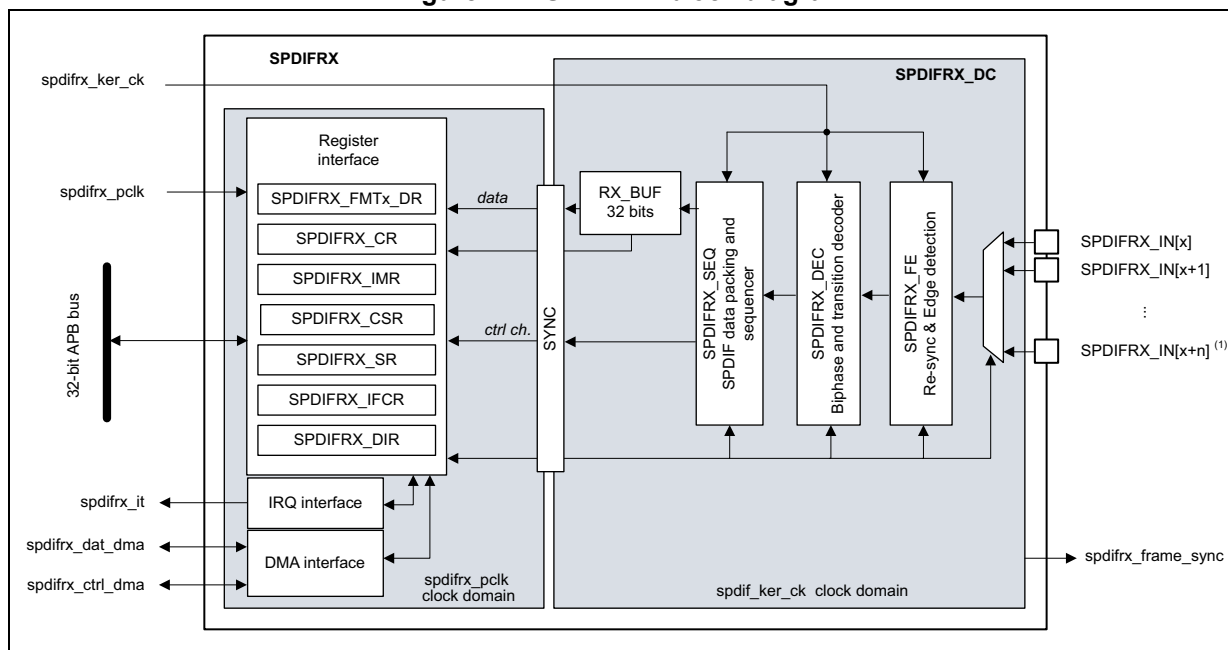
Figure 711. SPDIFRX block diagram
