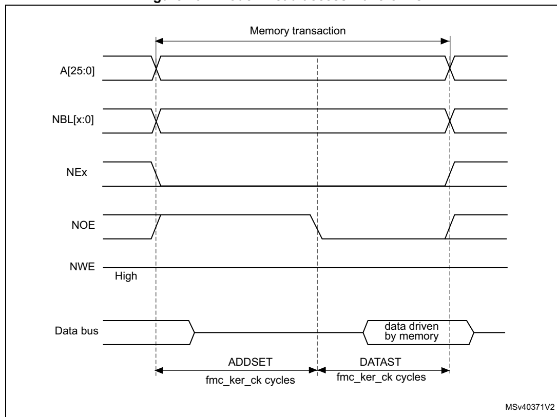
Figure 107. Mode A read access waveforms
