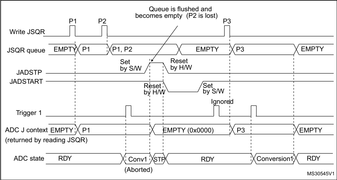
Figure 164. Flushing JSQR queue of context by setting JADSTP=1 (JQM=1)
