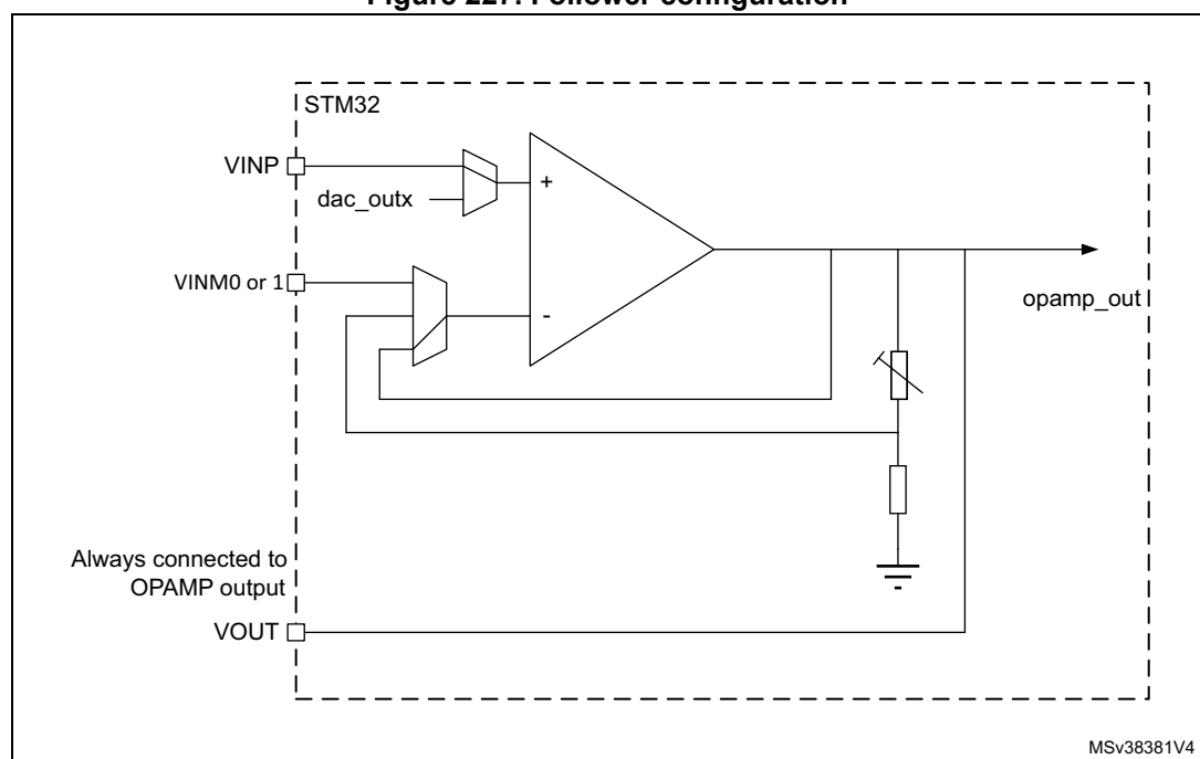
Figure 227. Follower configuration
