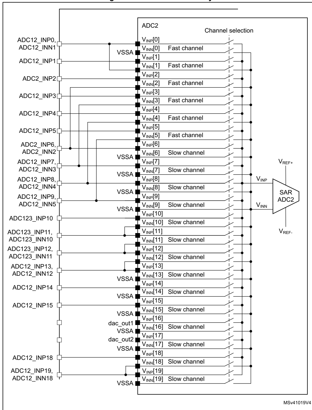
Figure 144. ADC2 connectivity
