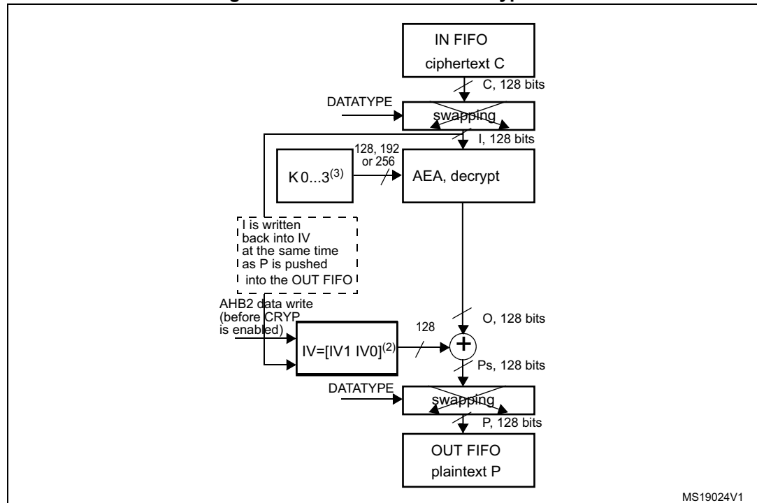
Figure 311. AES-CBC mode decryption
