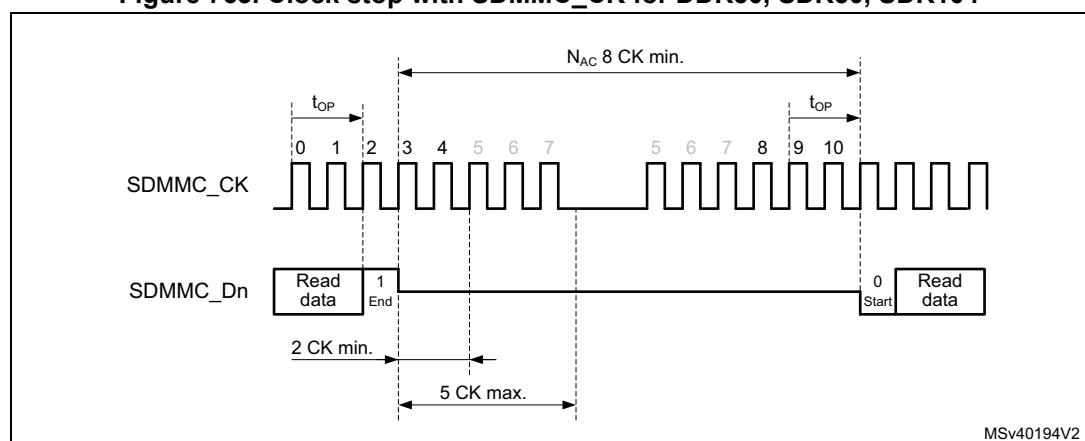
Figure 763. Clock stop with SDMMC_CK for DDR50, SDR50, SDR104
