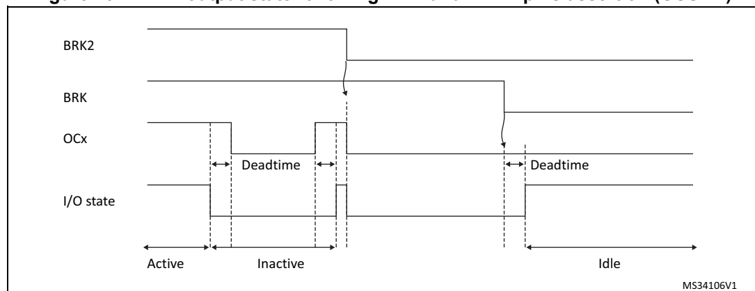
Figure 431. PWM output state following BRK and BRK2 pins assertion (OSSl=1)
