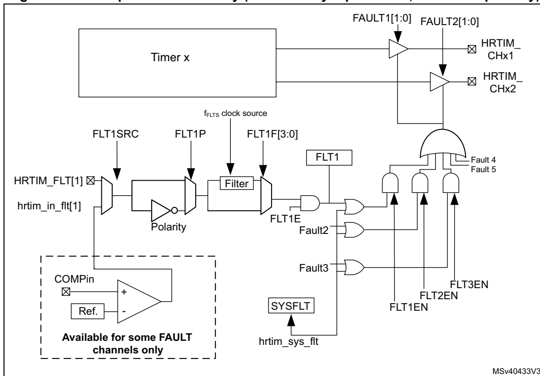
Figure 367. Fault protection circuitry (FAULT1 fully represented, FAULT2..5 partially)
