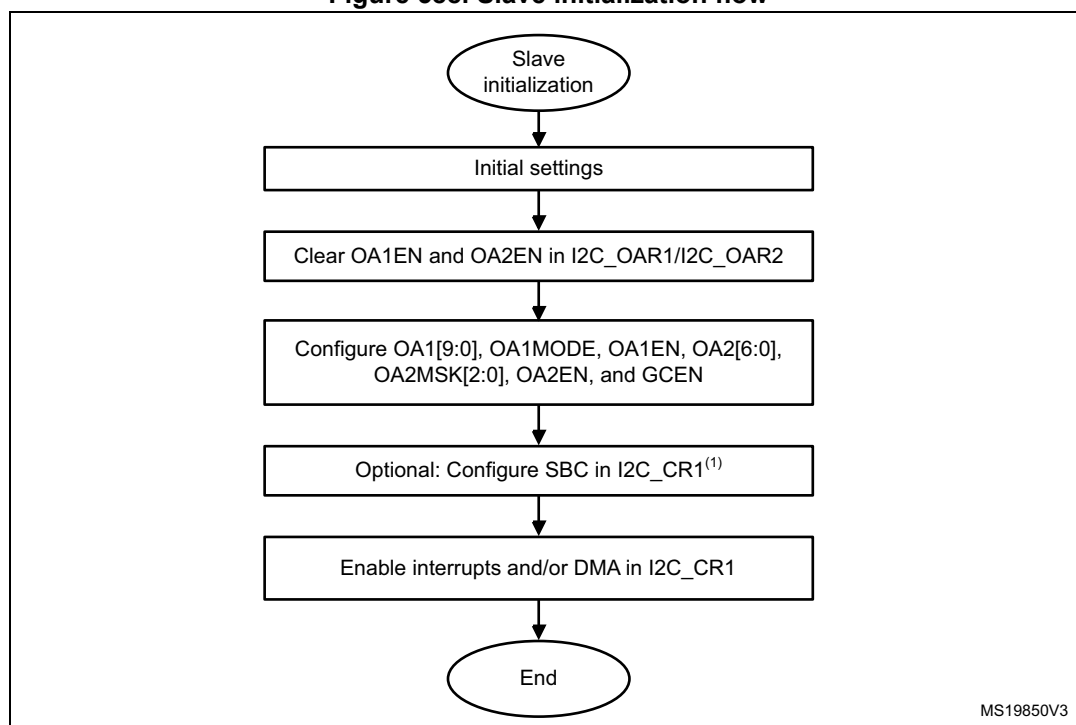
Figure 588. Slave initialization flow
