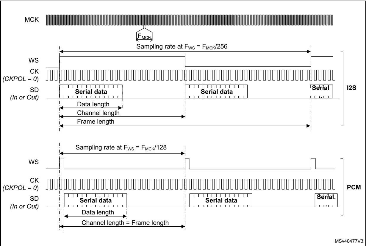
Figure 670. Waveform examples
