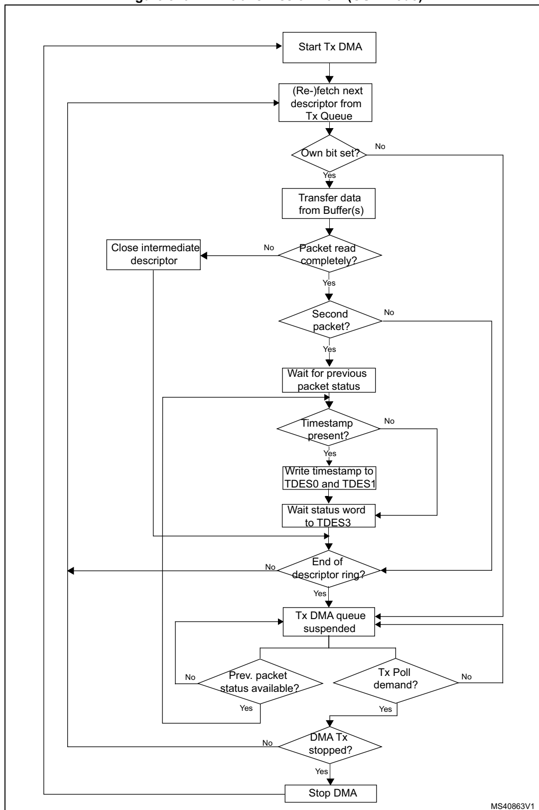
Figure 826. DMA transmission flow (OSP mode)
