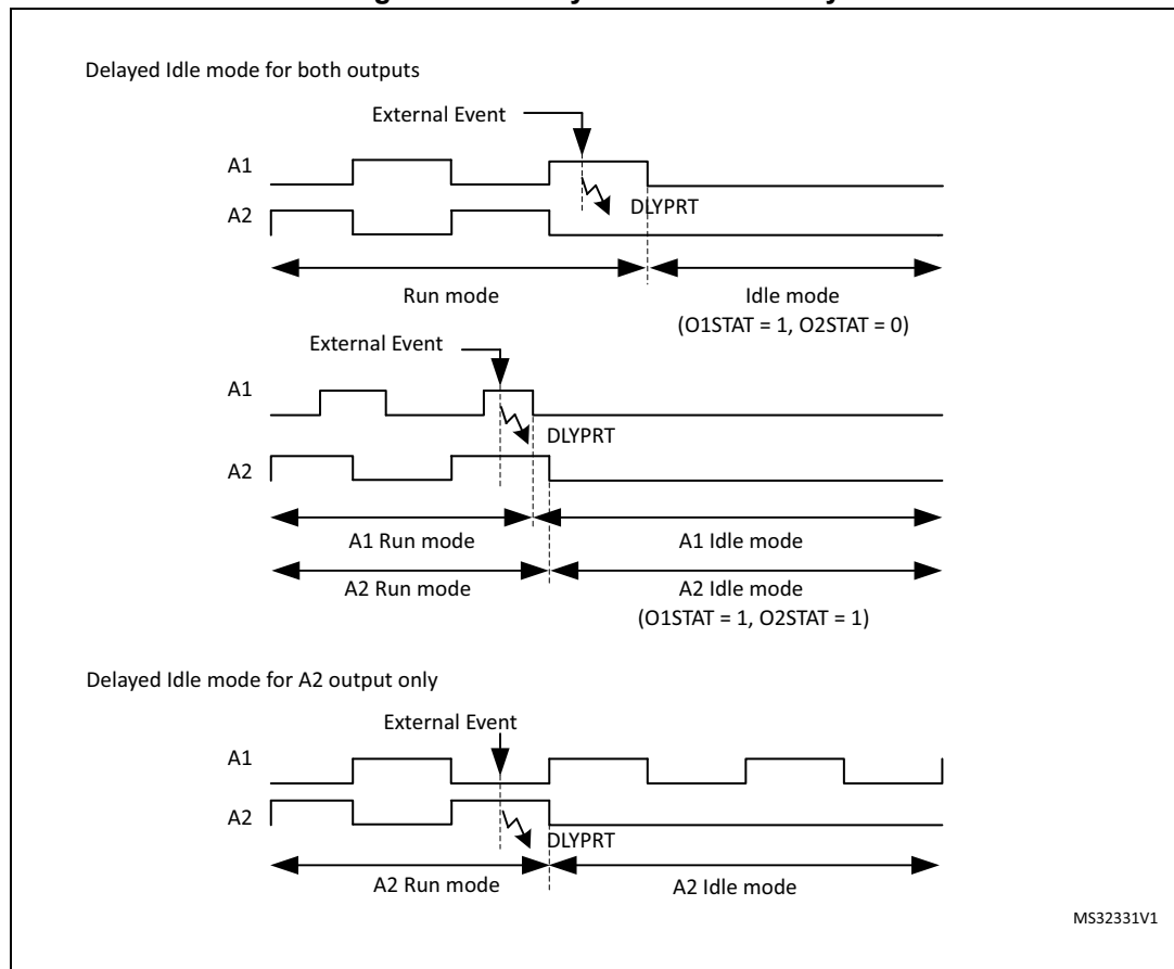
Figure 353. Delayed Idle mode entry
