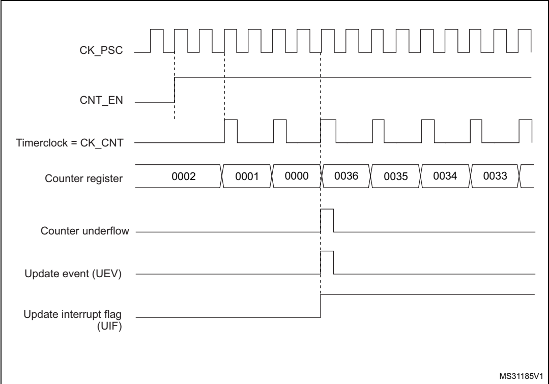
Figure 396. Counter timing diagram, internal clock divided by 2
