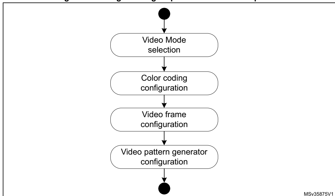
Figure 290. Programming sequence to send a test pattern
