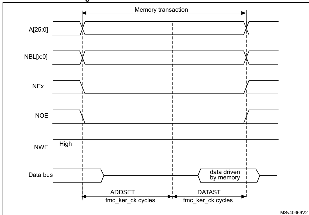
Figure 105. Mode 1 read access waveforms
