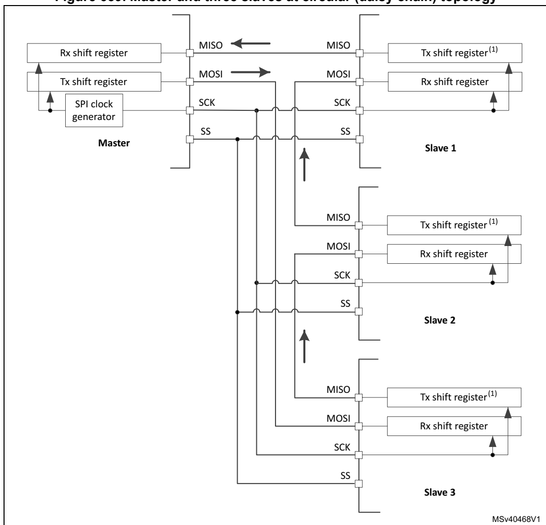
Figure 659. Master and three slaves at circular (daisy chain) topology
