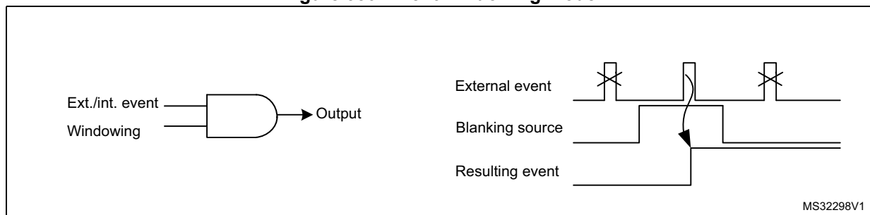
Figure 350. Event windowing mode
