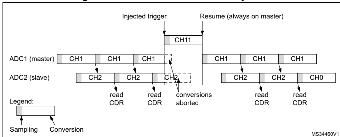
Figure 198. Interleaved conversion with injection
