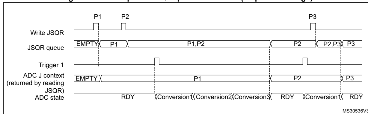
Figure 155. Example of JSQR queue of context (sequence change)
