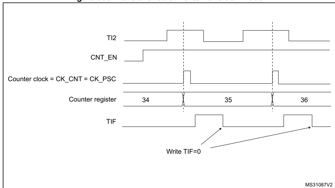
Figure 535. Control circuit in external clock mode 1
