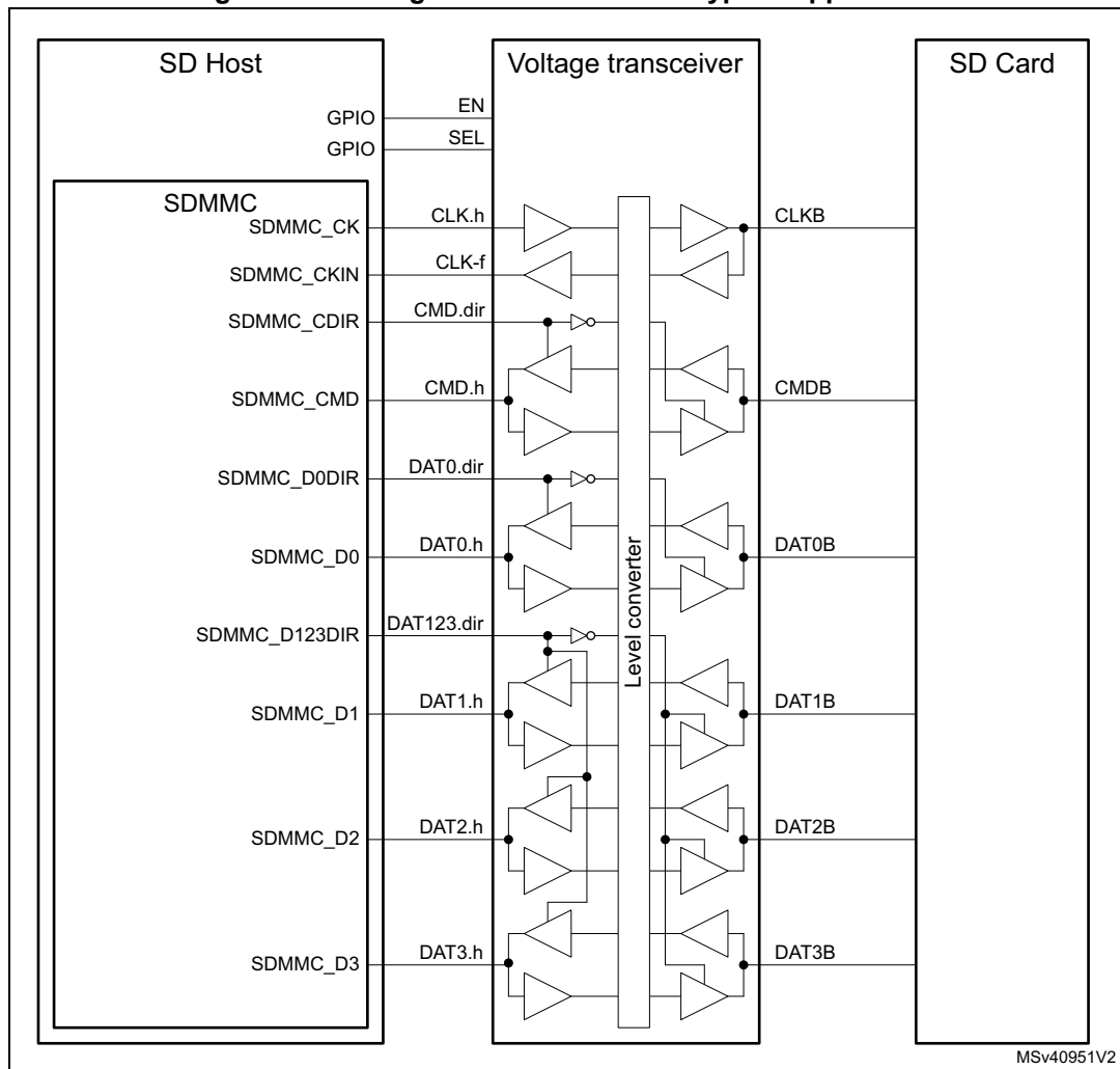
Figure 774. Voltage switch transceiver typical application
