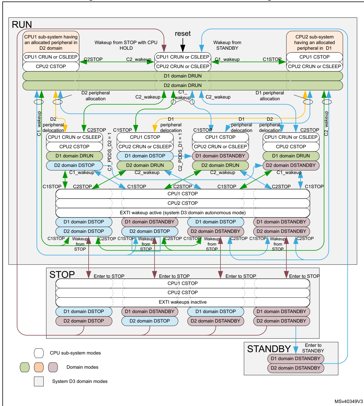
Figure 38. Power control modes detailed state diagram
