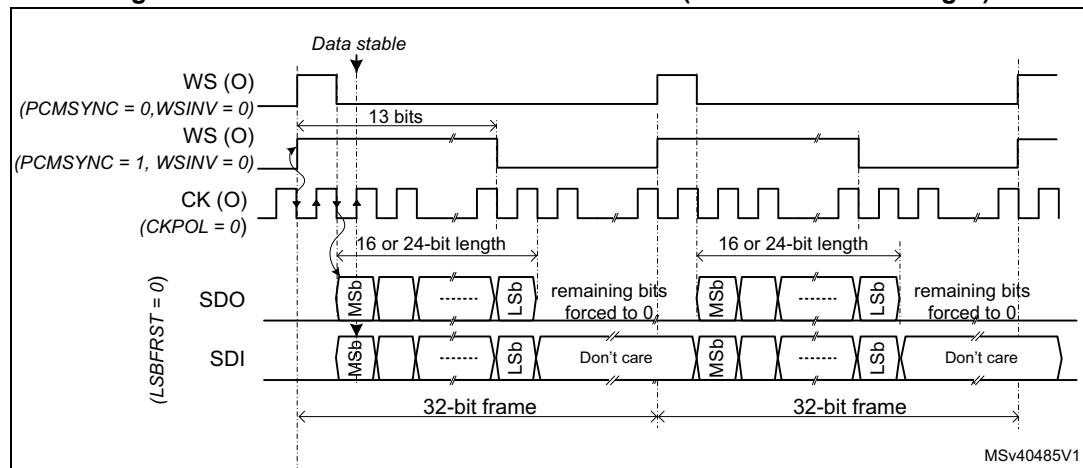
Figure 678. Master PCM standard waveforms (16 or 24-bit data length)
