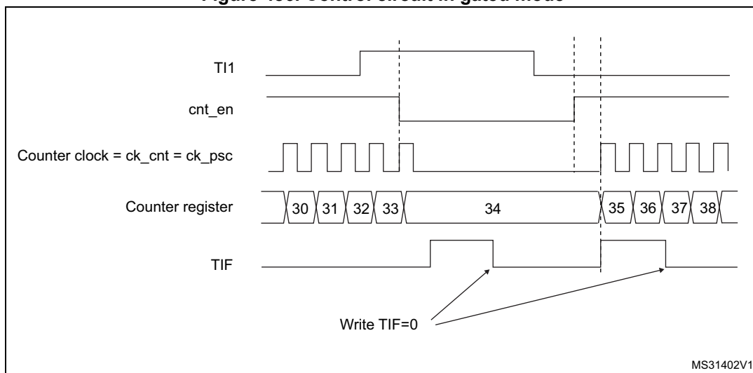
Figure 486. Control circuit in gated mode
