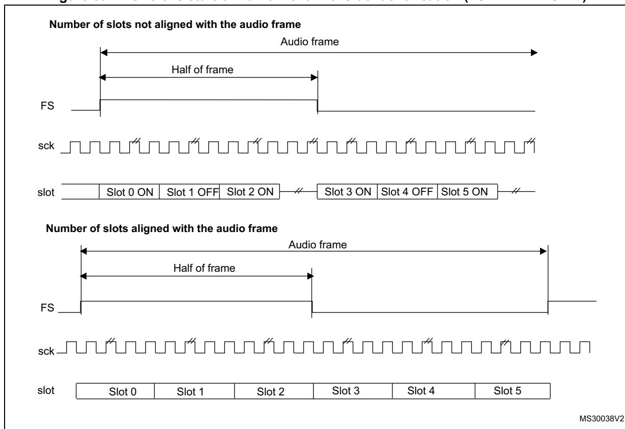
Figure 691. FS role is start of frame + channel side identification (FSDEF = TRIS = 1)
