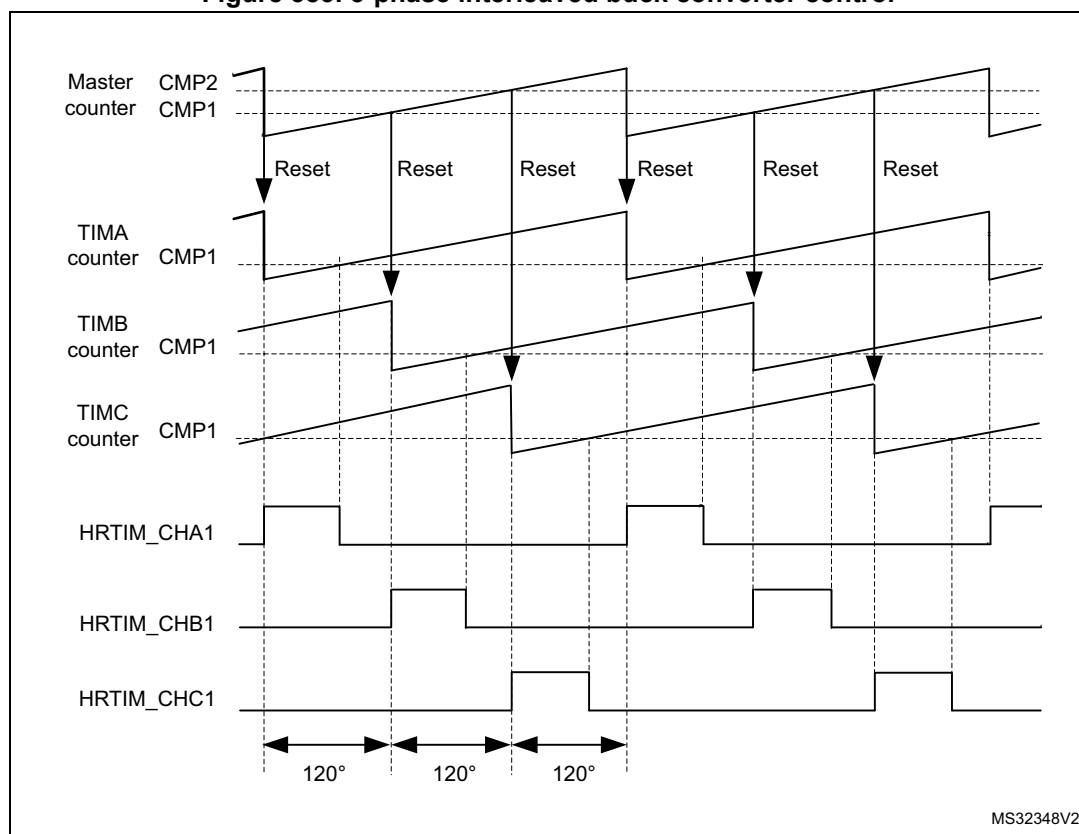
Figure 383. 3-phase interleaved buck converter control
