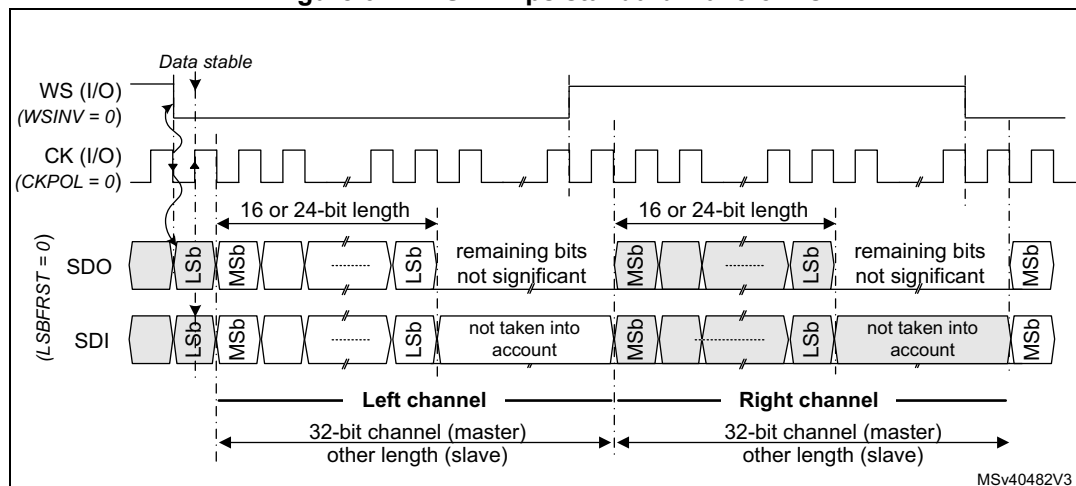
Figure 672. I2S Philips standard waveforms
