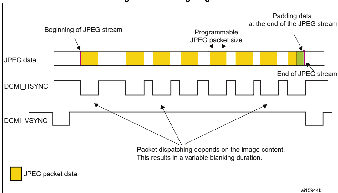
Figure 244. Timing diagram
