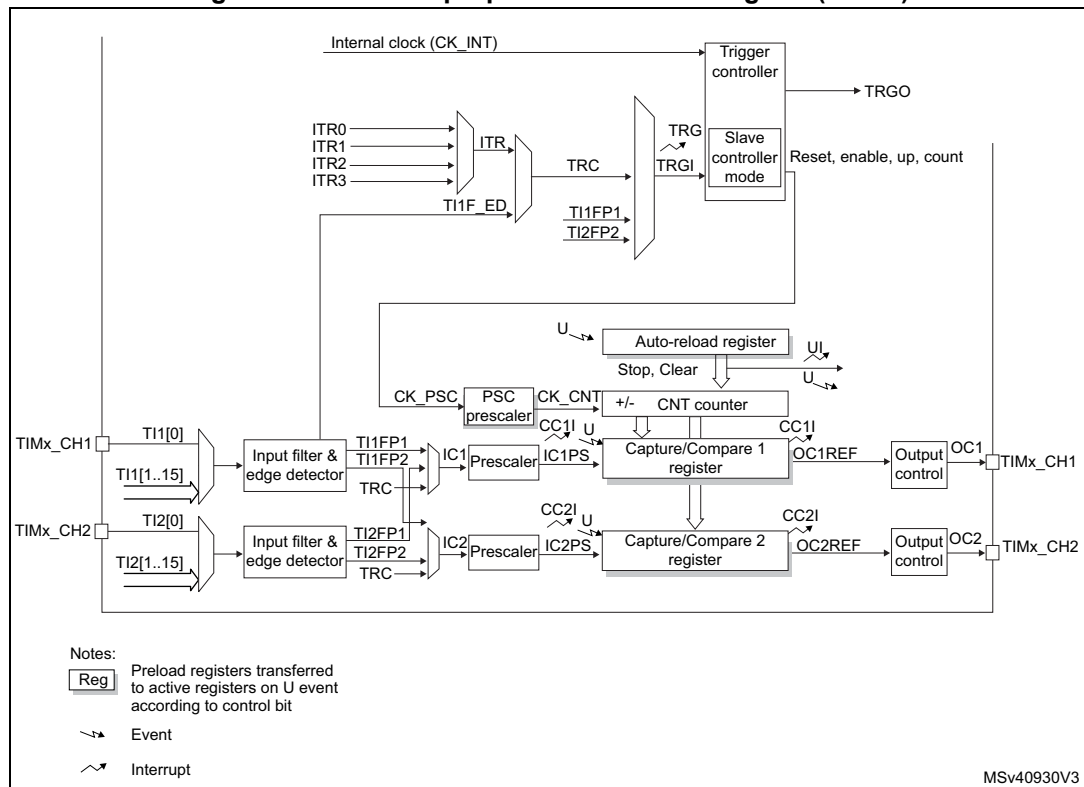
Figure 496. General-purpose timer block diagram (TIM12)
