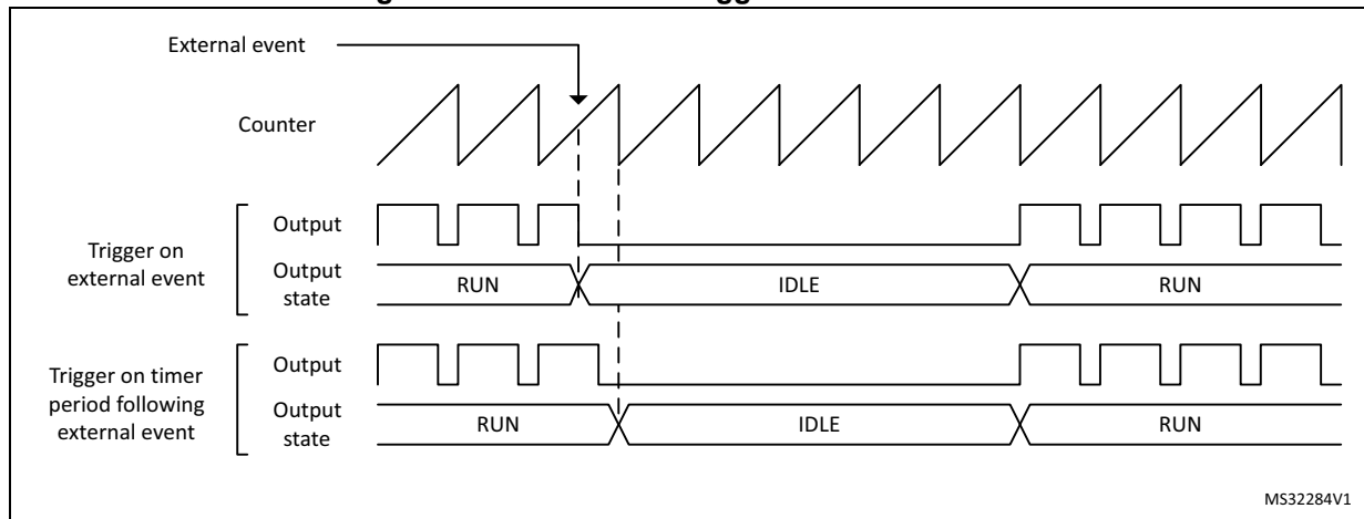
Figure 360. Burst mode trigger on external event
