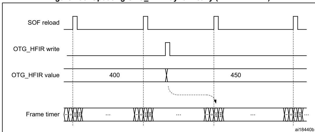
Figure 798. Updating OTG_HFIR dynamically (RLDCTRL = 1)
