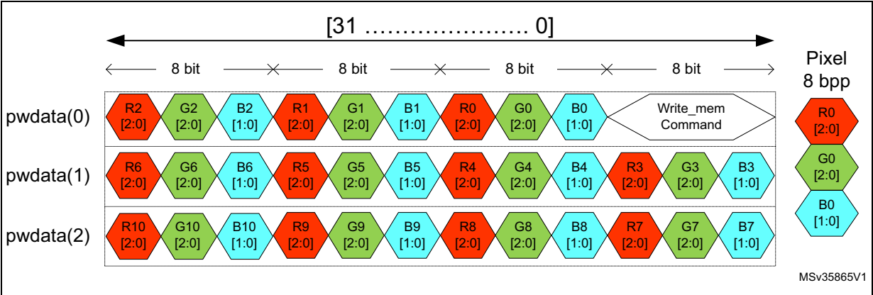
Figure 265. 8 bpp APB pixel to byte organization
