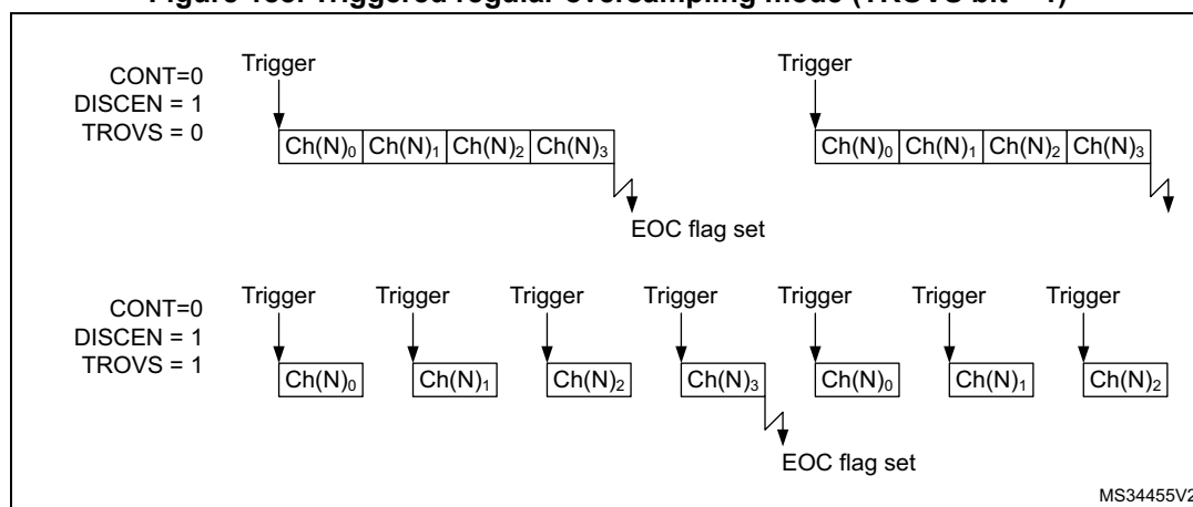
Figure 188. Triggered regular oversampling mode (TROVS bit = 1)
