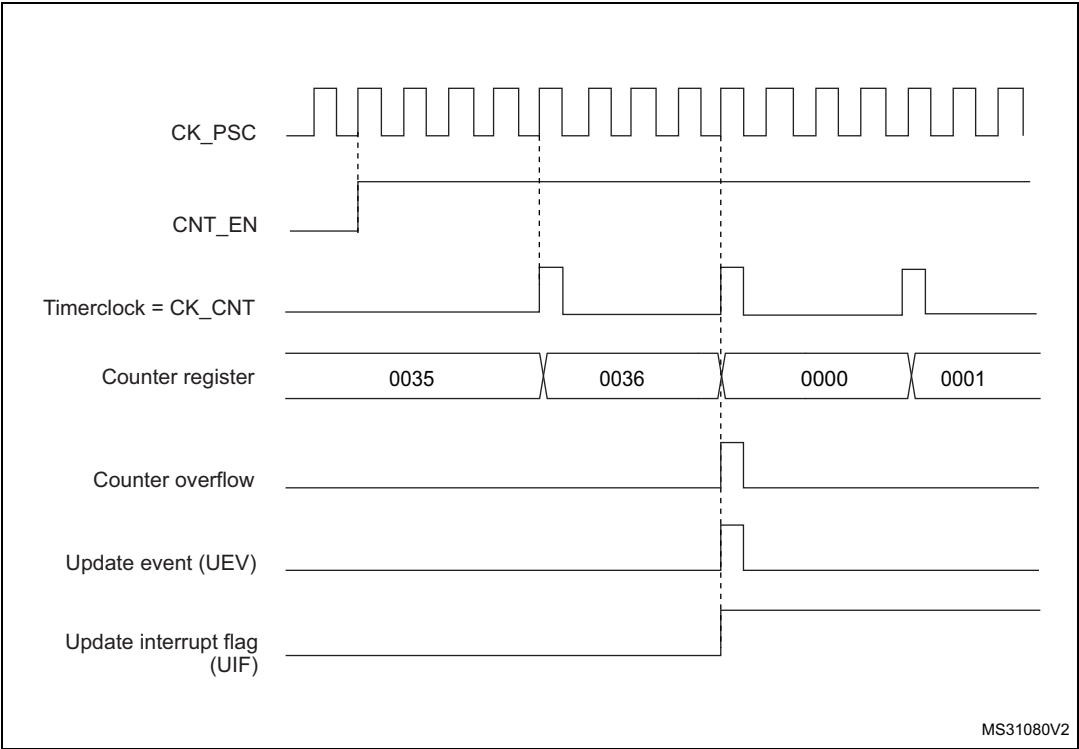
Figure 561. Counter timing diagram, internal clock divided by 4
