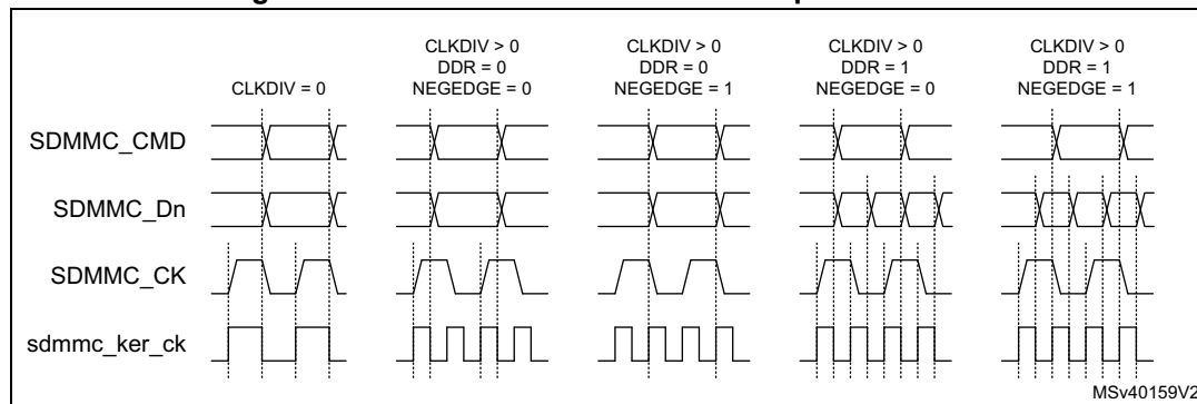
Figure 748. SDMMC Command and data phase relation
