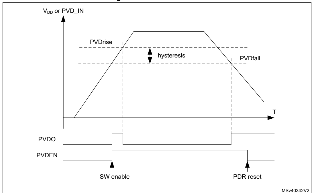
Figure 31. PVD thresholds
