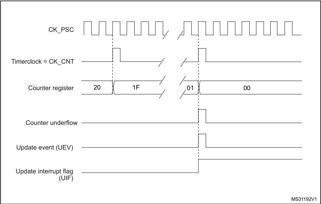
Figure 403. Counter timing diagram, internal clock divided by N
