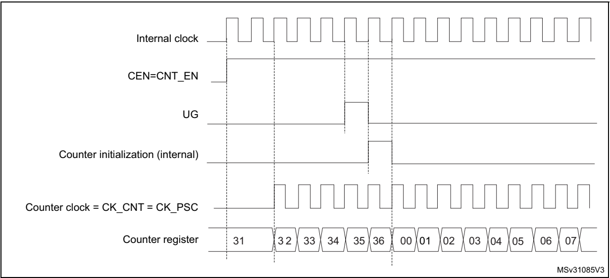
Figure 506. Control circuit in normal mode, internal clock divided by 1
