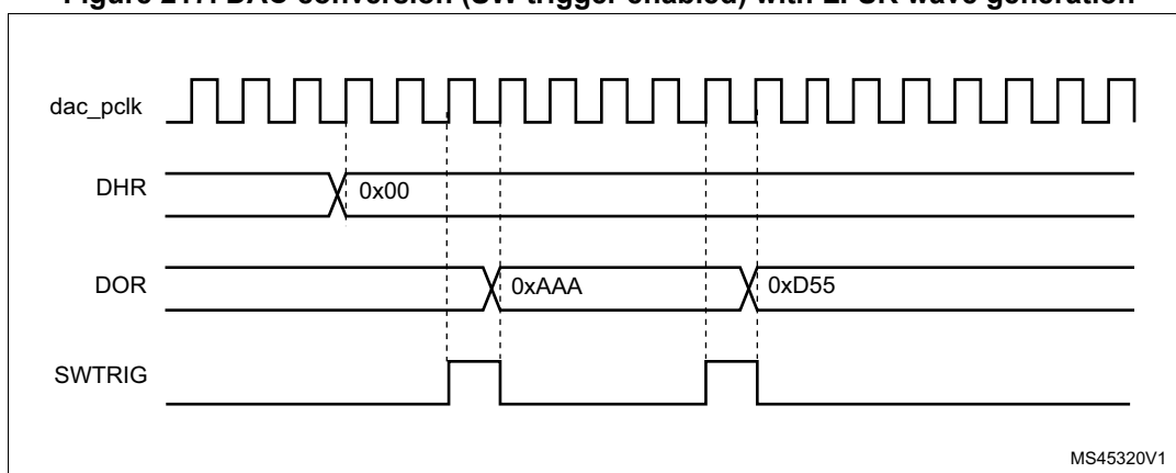
Figure 217. DAC conversion (SW trigger enabled) with LFSR wave generation
