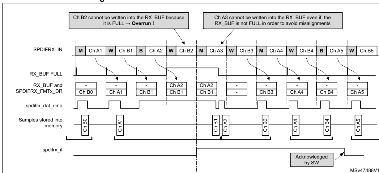
Figure 725. S/PDIF overrun error when RXSTEO = 1
