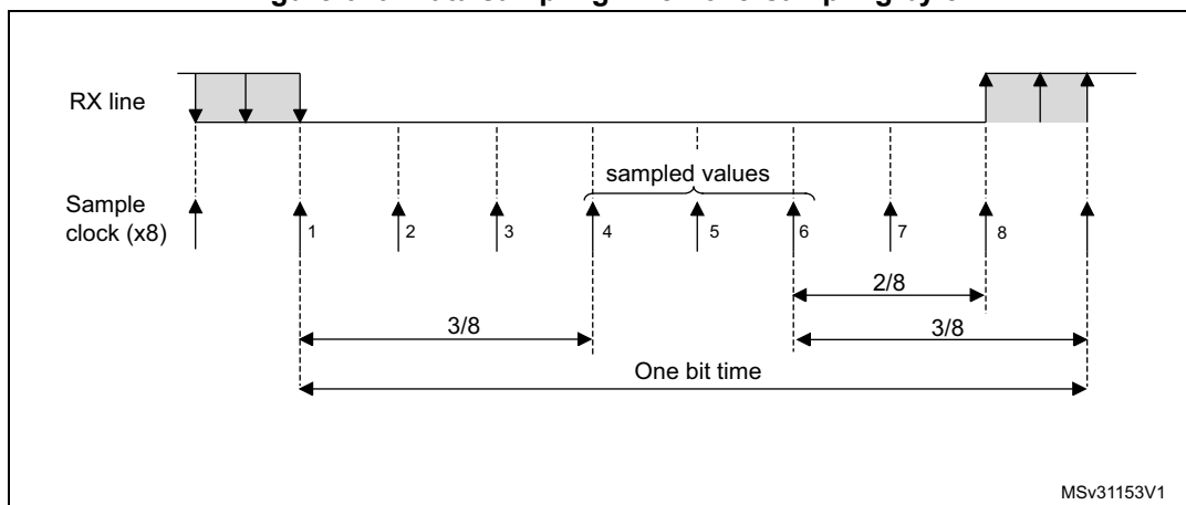
Figure 620. Data sampling when oversampling by 8
