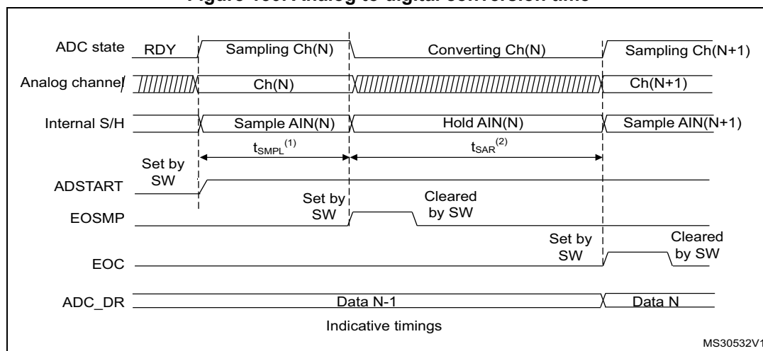
Figure 150. Analog to digital conversion time
