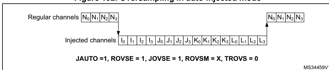
Figure 192. Oversampling in auto-injected mode
