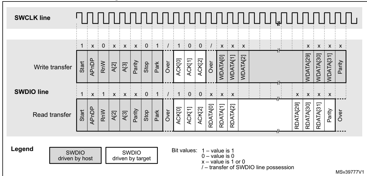
Figure 873. SWD successful data transfer
