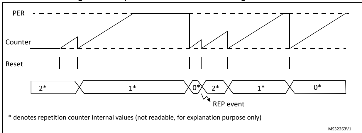
Figure 329. Repetition counter behavior in single-shot mode
