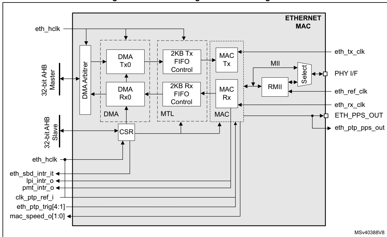
Figure 824. Ethernet high-level block diagram
