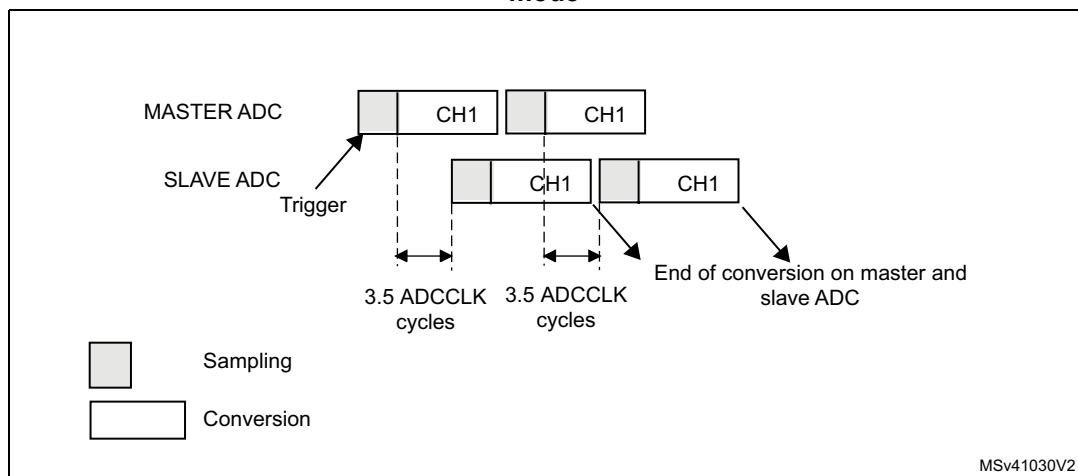
Figure 196. Interleaved mode on 1 channel in continuous conversion mode: dual ADC mode
