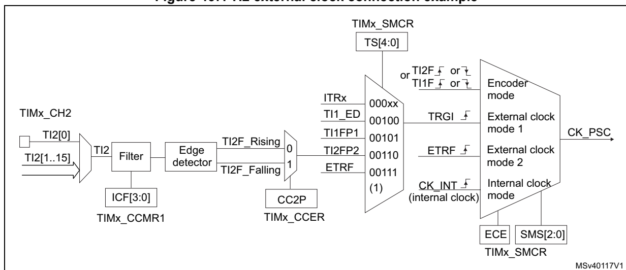
Figure 467. TI2 external clock connection example
