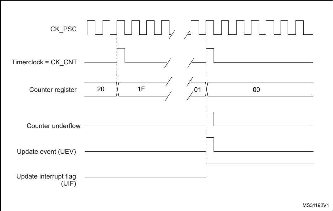
Figure 463. Counter timing diagram, internal clock divided by N
