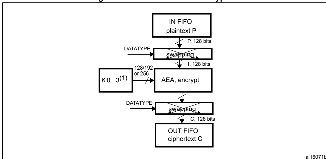
Figure 308. AES-ECB mode encryption
