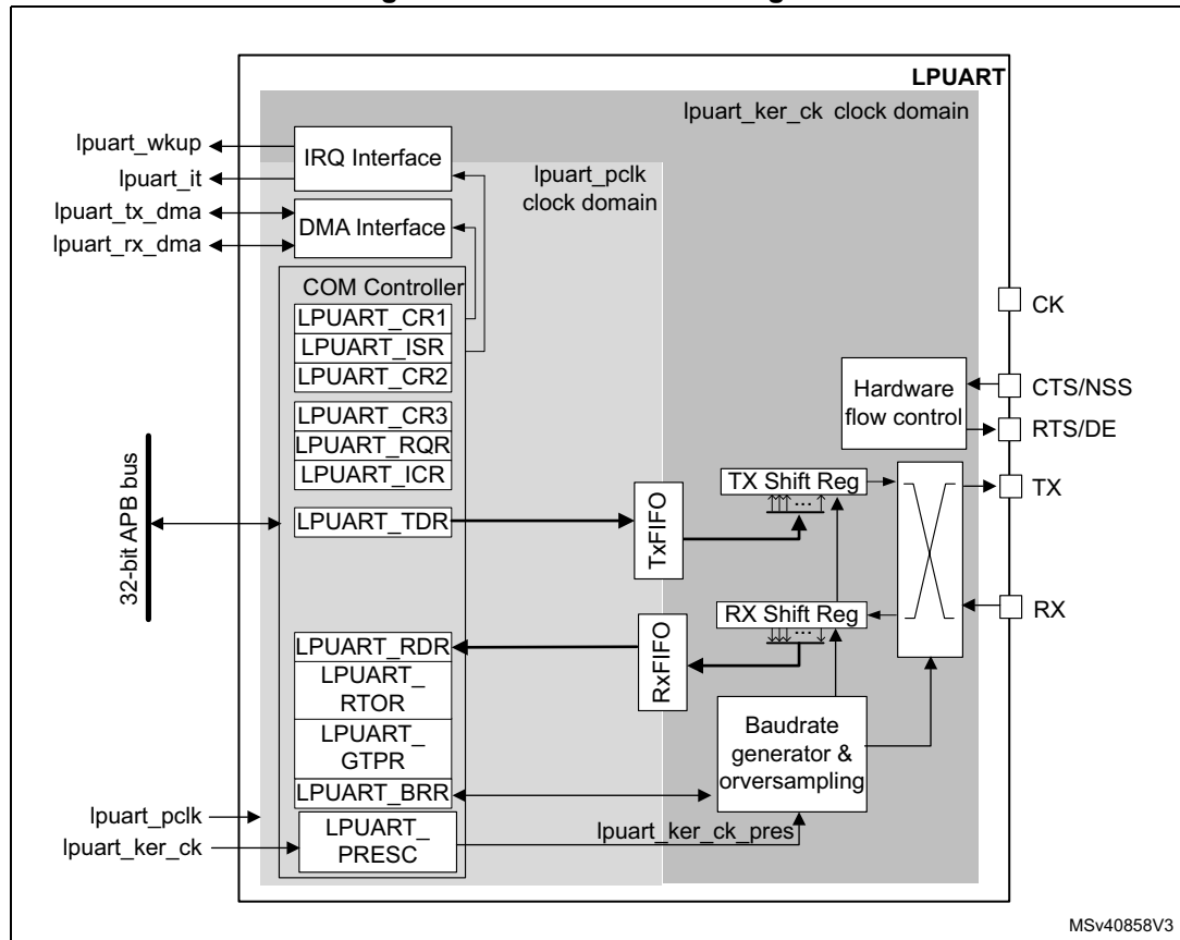
Figure 640. LPUART block diagram
