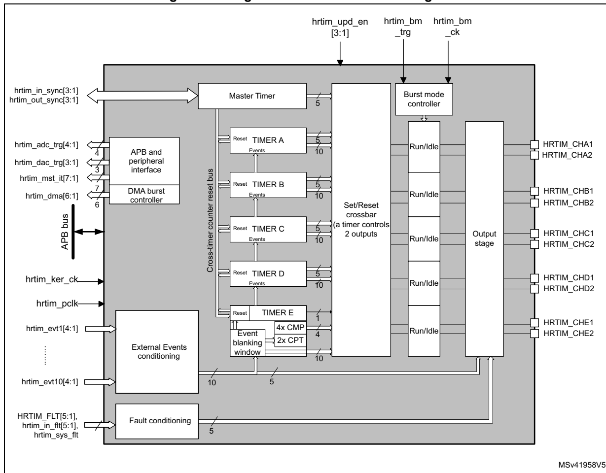
Figure 323. High-resolution timer block diagram
