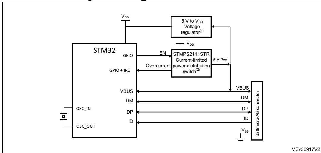
Figure 794. OTG_HS A-B device connection
