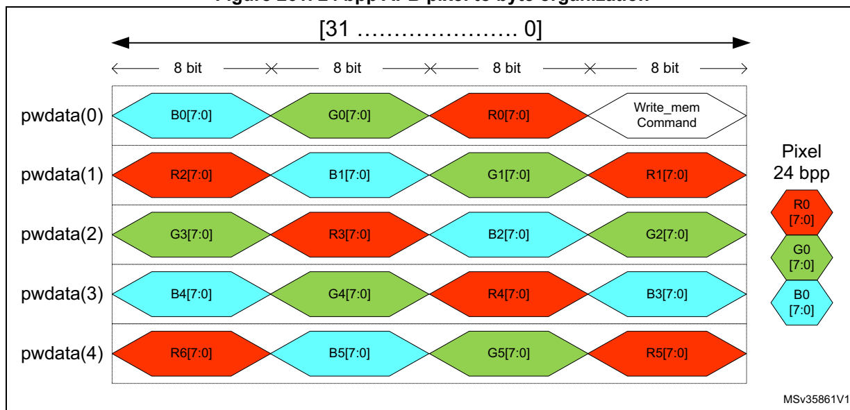
Figure 261. 24 bpp APB pixel to byte organization
