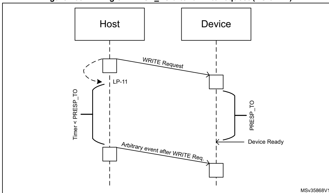
Figure 268. Timing of PRESP_TO after a write request (HS or LP)
