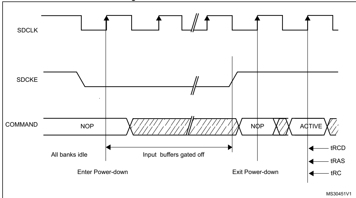
Figure 131. Power-down mode
