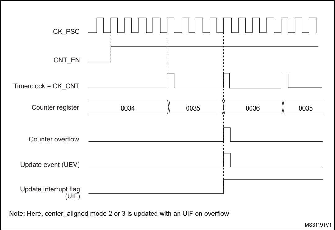
Figure 462. Counter timing diagram, internal clock divided by 4, TIMx_ARR=0x36
