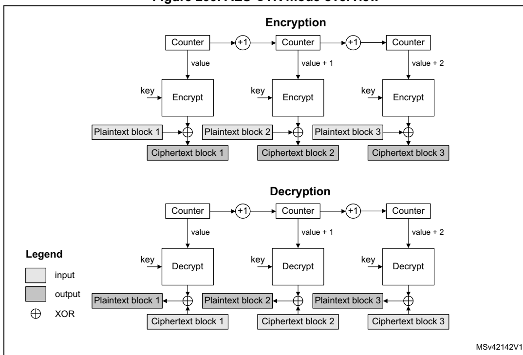
Figure 299. AES-CTR mode overview
