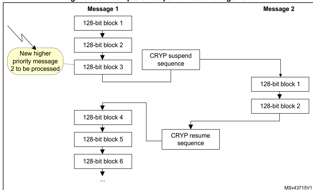
Figure 303. Example of suspend mode management
