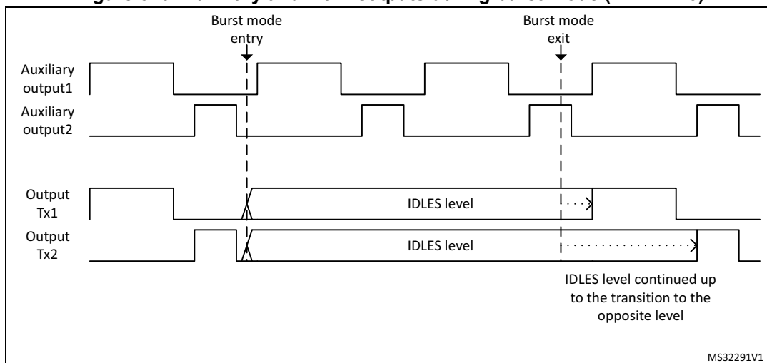
Figure 370. Auxiliary and main outputs during burst mode (DIDLx = 0)
