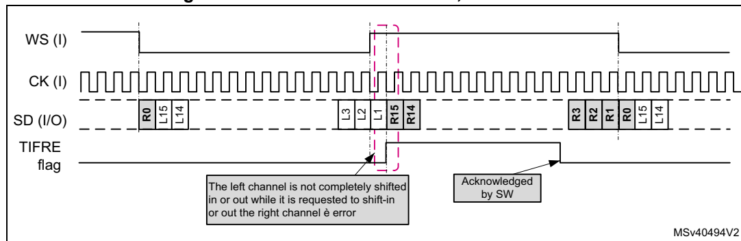
Figure 687. Frame error detection, with FIXCH=0
