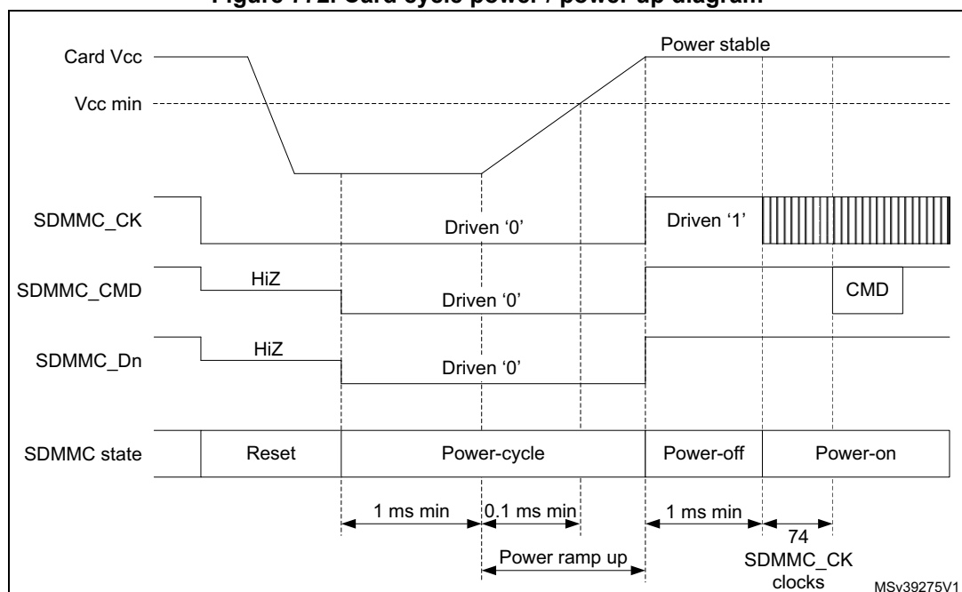
Figure 772. Card cycle power / power up diagram
