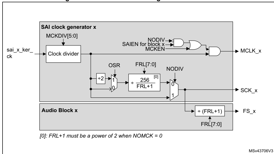
Figure 695. Audio block clock generator overview
