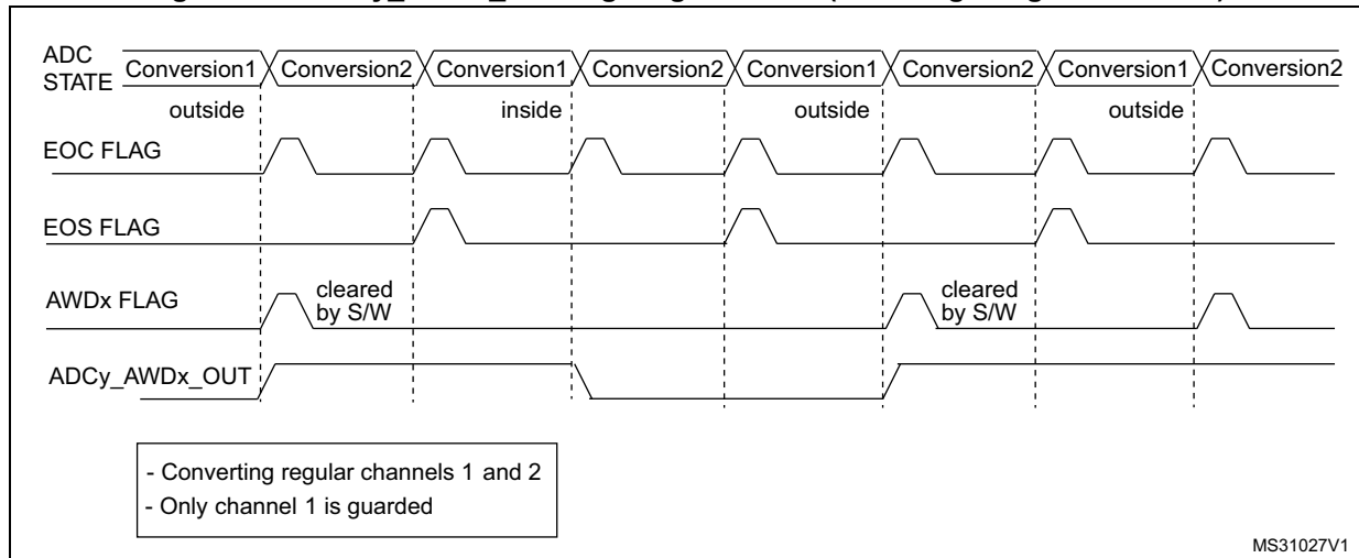
Figure 185. ADCy_AWDx_OUT signal generation (on a single regular channel)
