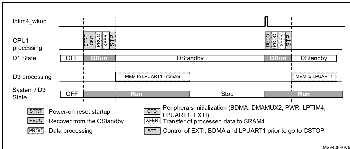
Figure 45. Timing diagram of SRAM4-to-LPUART1 transfer with BDMA and D3 domain in Autonomous mode
