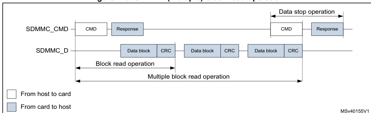
Figure 743. SDMMC (multiple) block read operation
