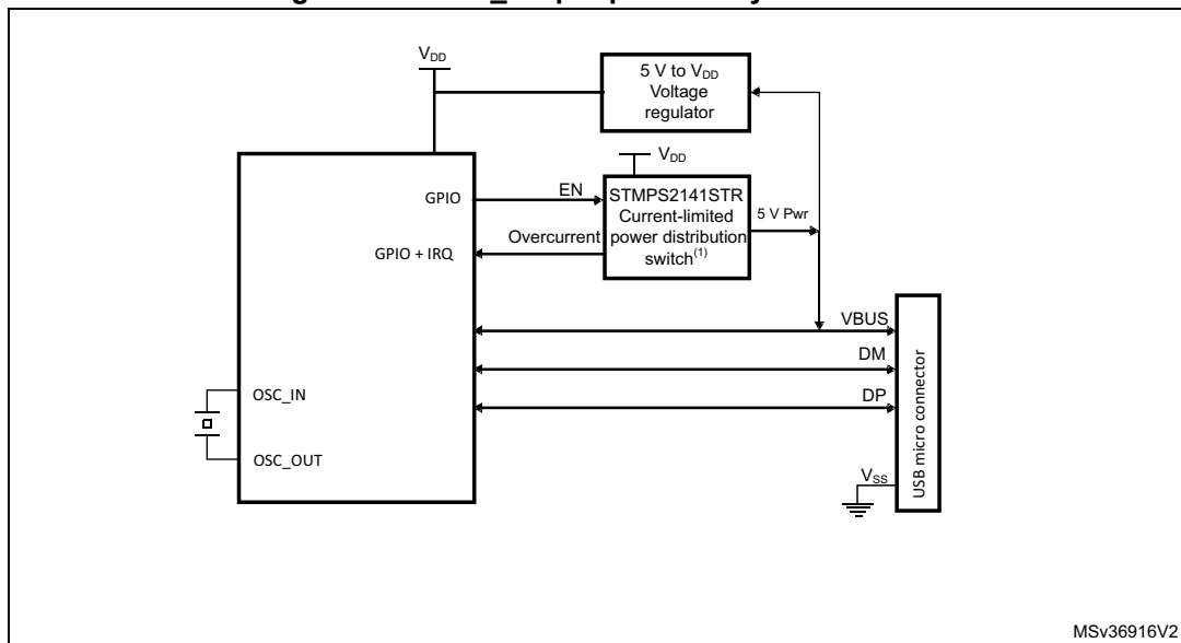
Figure 795. OTG_HS peripheral-only connection
