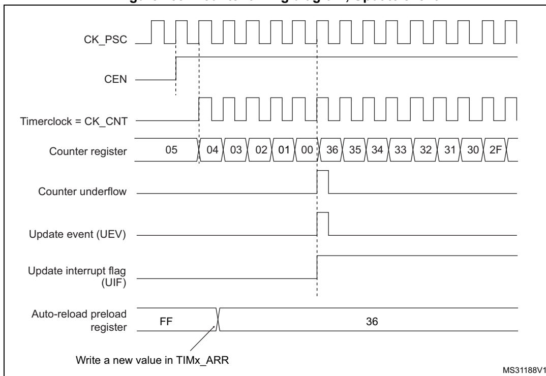
Figure 459. Counter timing diagram, Update event
