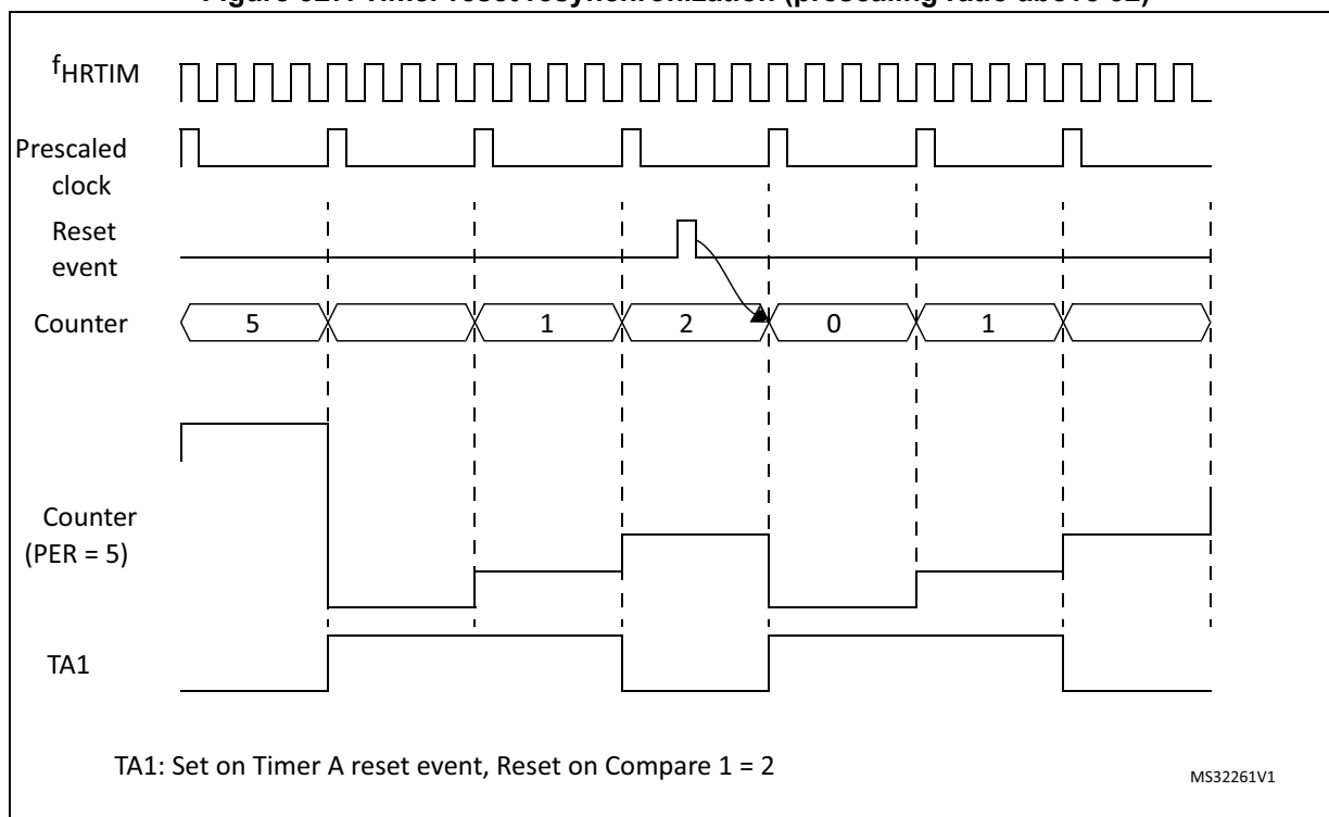
Figure 327. Timer reset resynchronization (prescaling ratio above 32)
