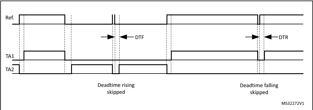
Figure 338. Complementary outputs for low pulse width (SDTRx = SDTFx = 0)
