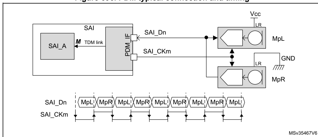
Figure 696. PDM typical connection and timing
