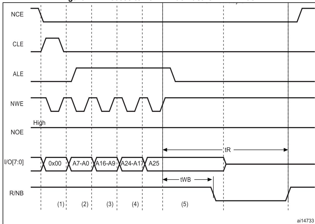
Figure 124. Access to non 'CE don't care' NAND-flash
