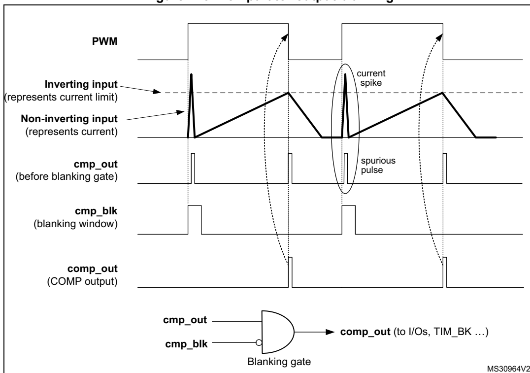
Figure 223. Comparator output blanking
