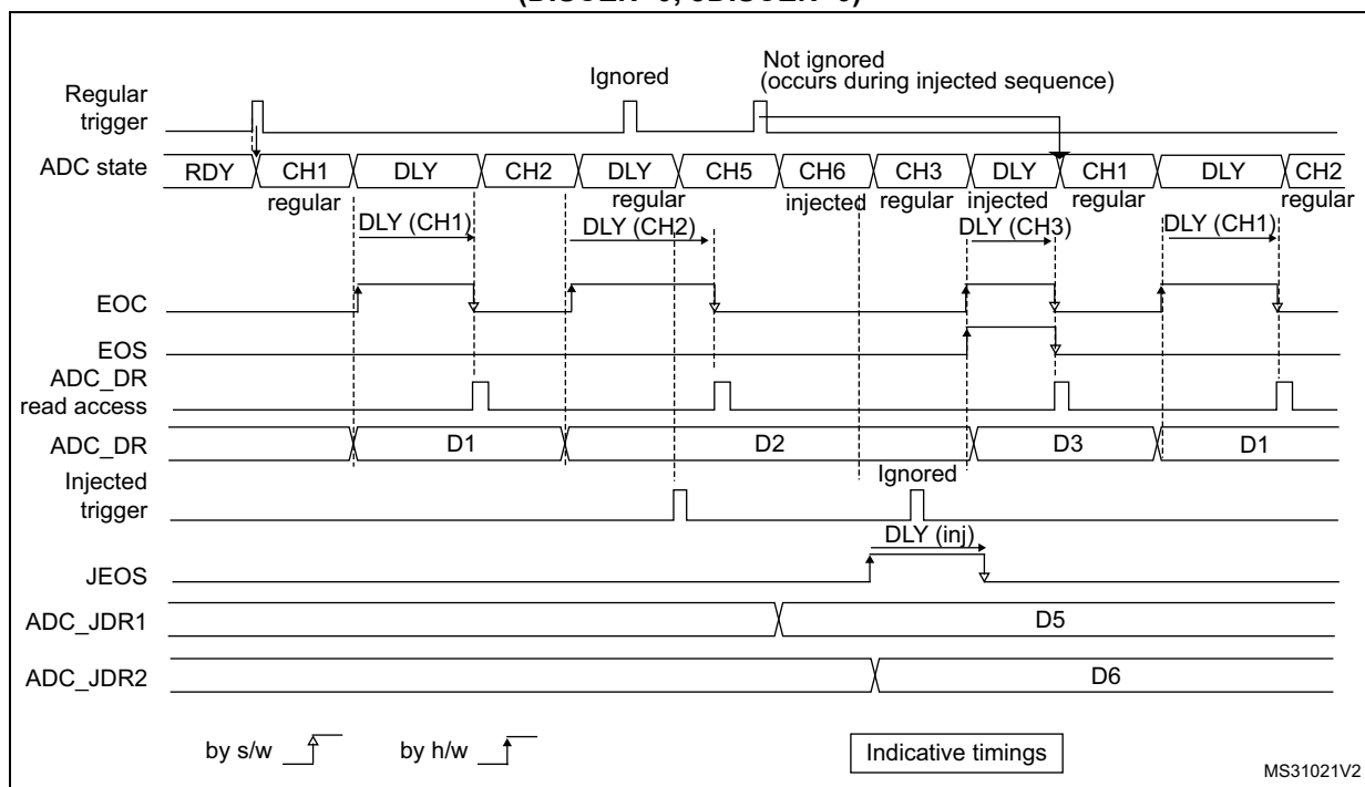
Figure 178. AUTDLY=1, regular HW conversions interrupted by injected conversions (DISCEN=0; JDISCEN=0)
