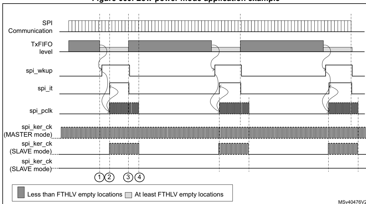
Figure 669. Low-power mode application example
