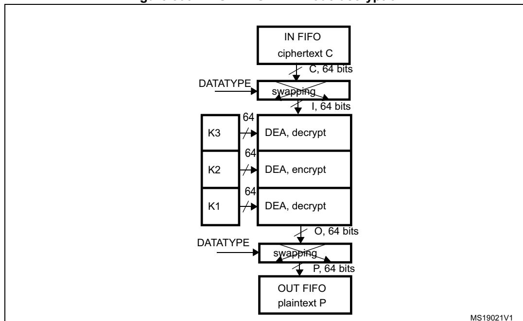
Figure 305. DES/TDES-ECB mode decryption
