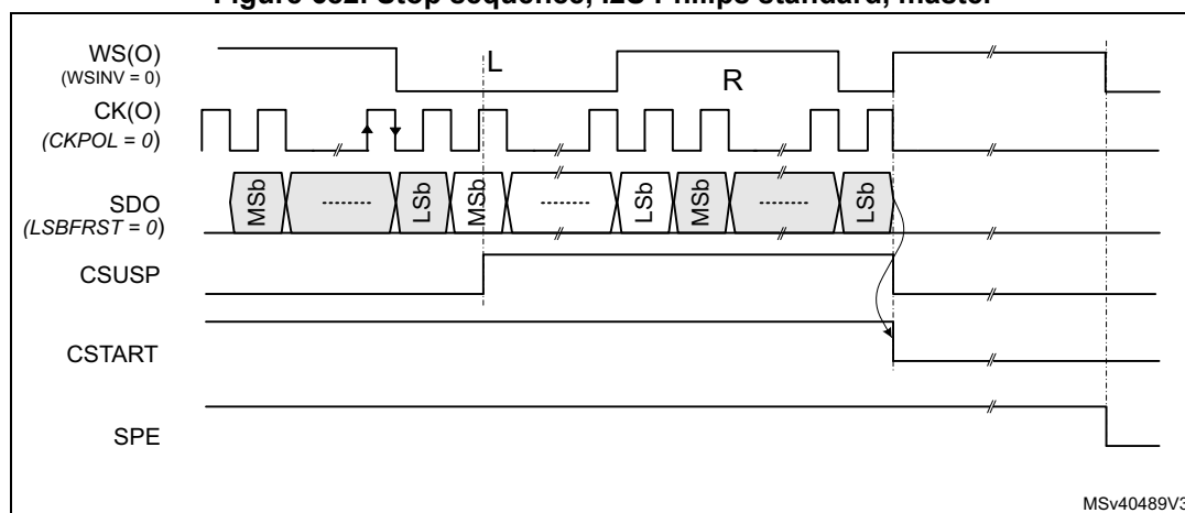
Figure 682. Stop sequence, I2S Philips standard, master
