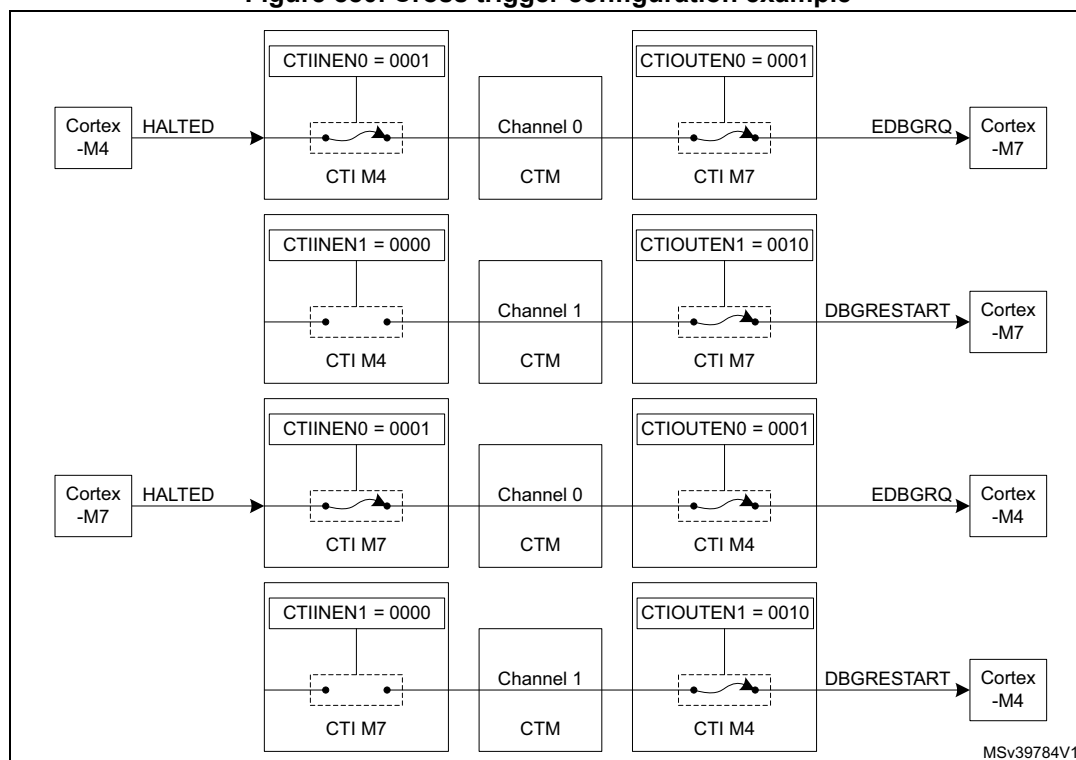
Figure 880. Cross trigger configuration example
