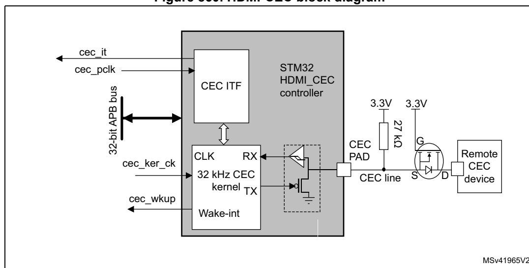
Figure 860. HDMI-CEC block diagram
