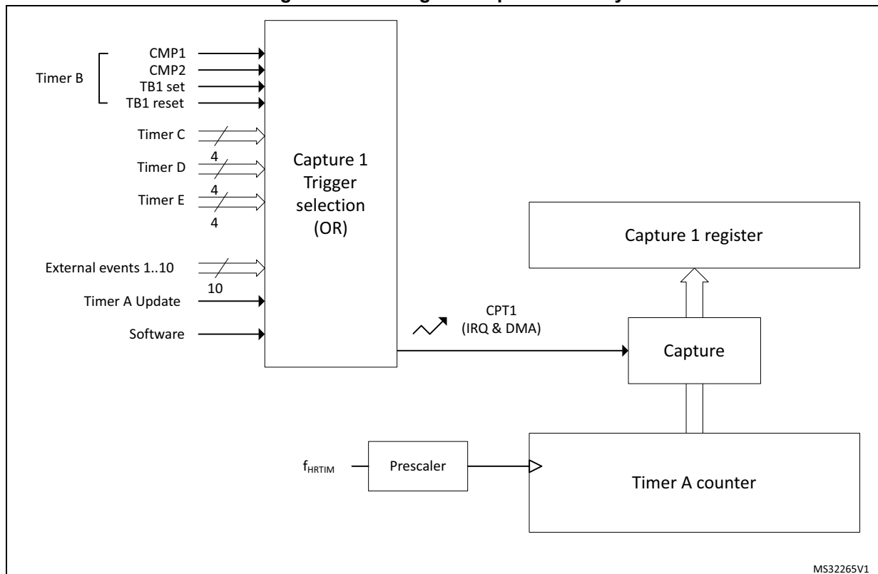
Figure 331. Timing unit capture circuitry
