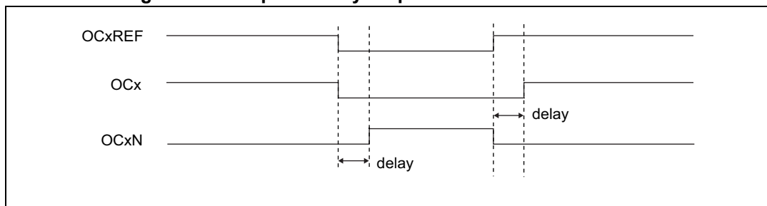
Figure 84. Complementary output with dead-time insertion.
