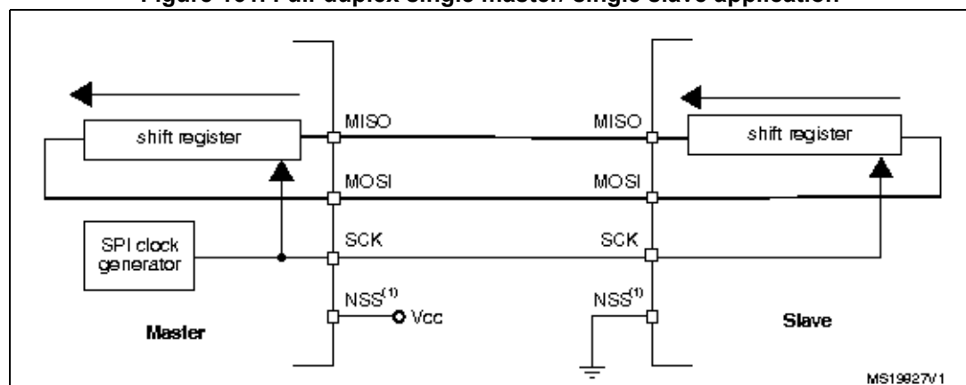
Figure 161. Full-duplex single master/ single slave application
