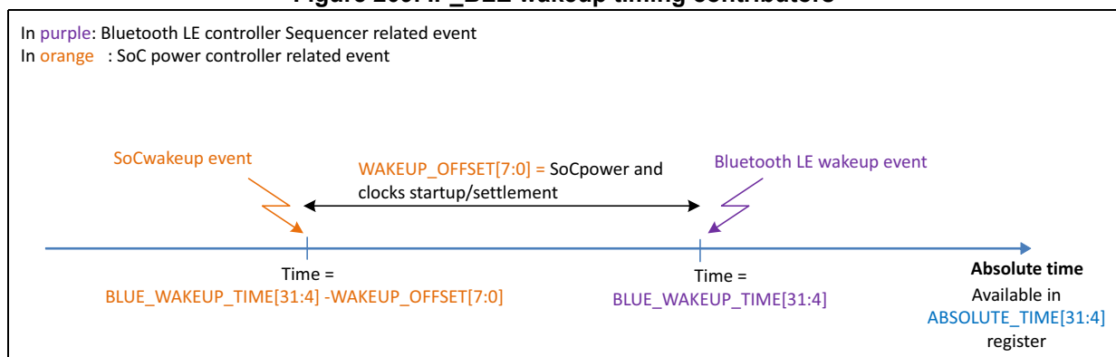
Figure 209. IP_BLE wakeup timing contributors
