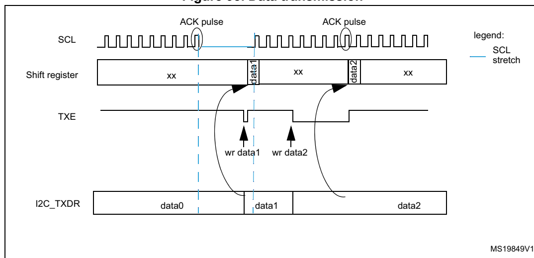
Figure 98. Data transmission
