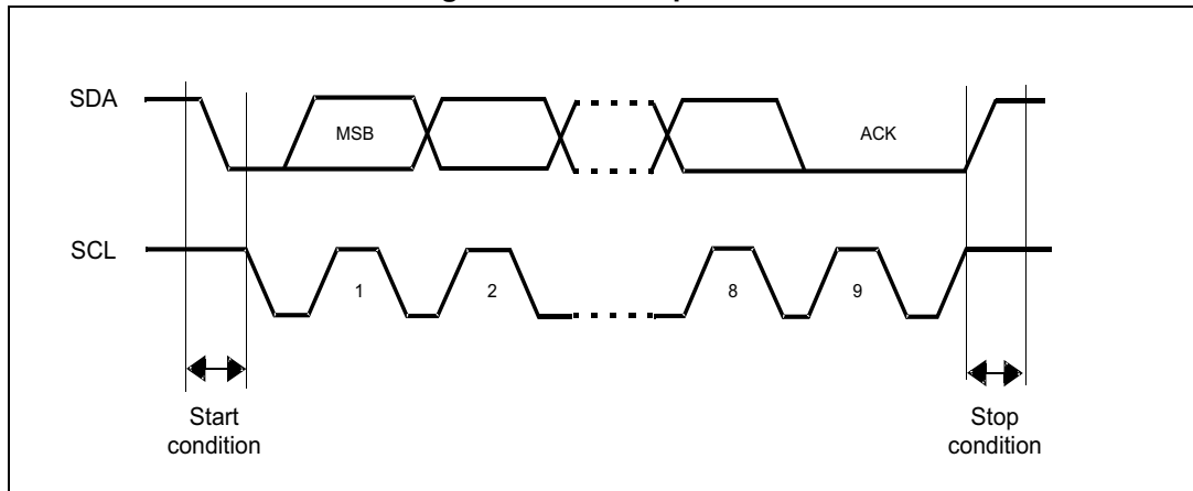
Figure 94. I 2 C bus protocol
