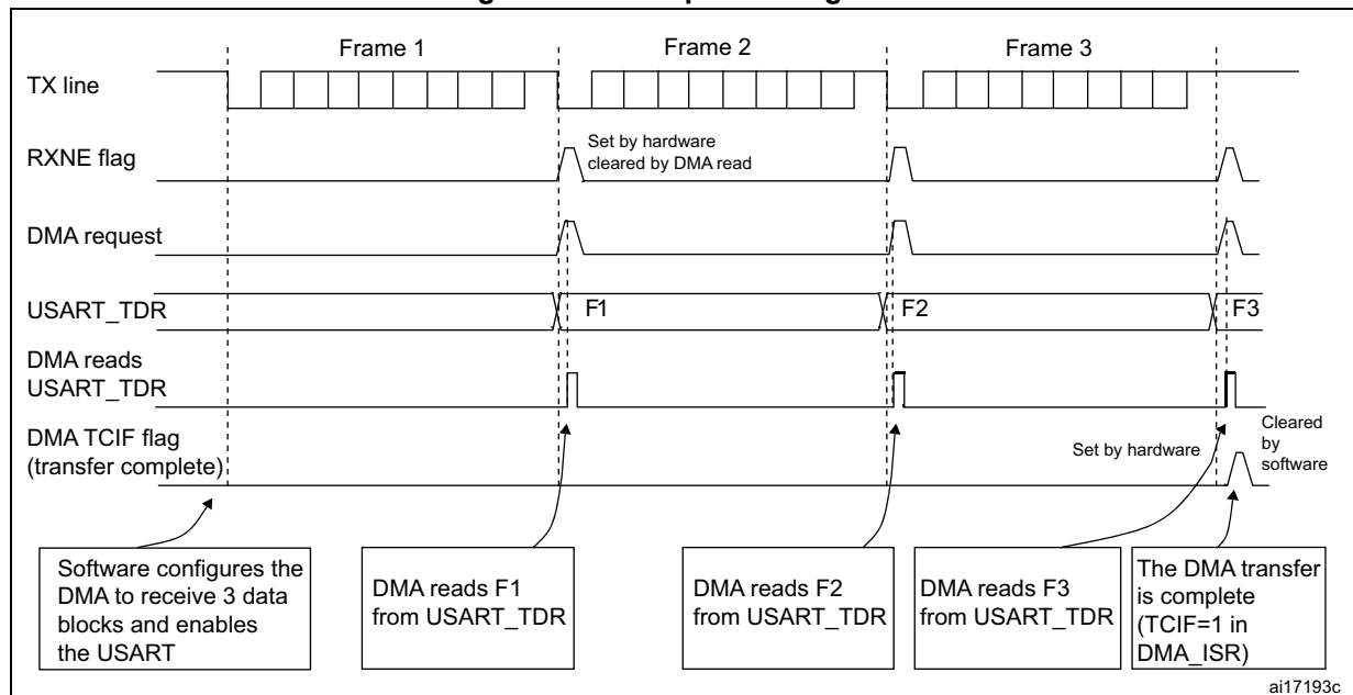
Figure 156. Reception using DMA
