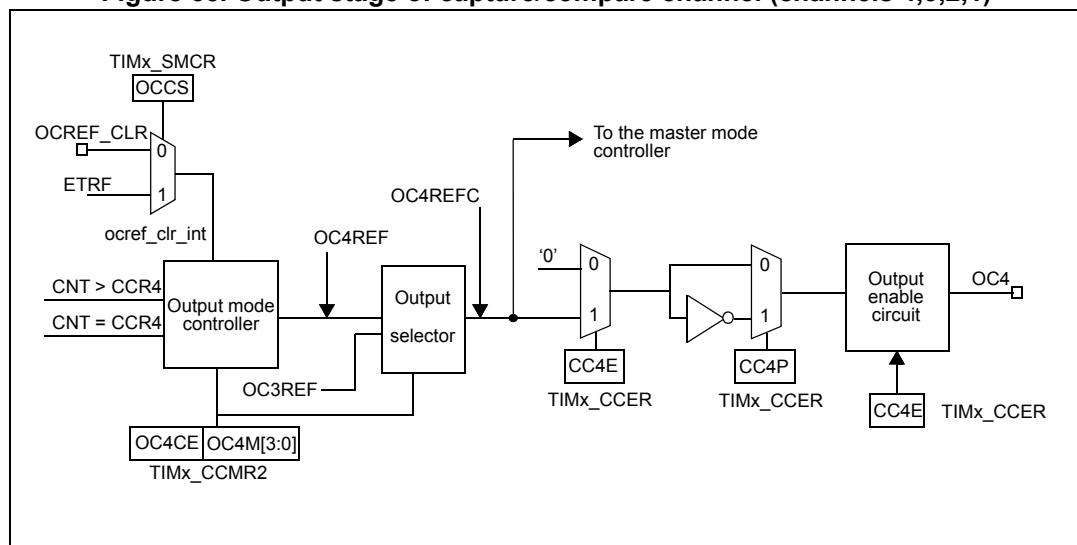
Figure 55. Output stage of capture/compare channel (channels 4,3,2,1)
