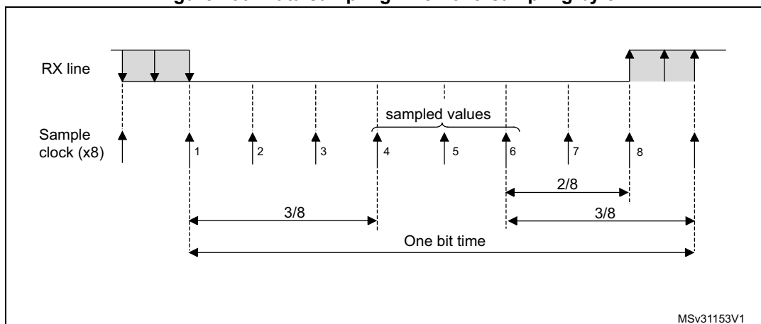
Figure 130. Data sampling when oversampling by 8
