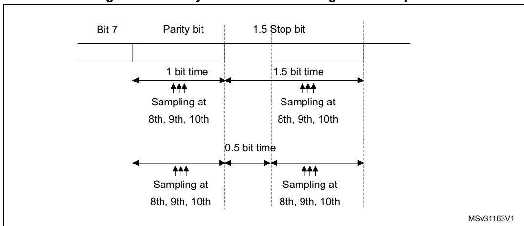
Figure 140. Parity error detection using the 1.5 stop bits
