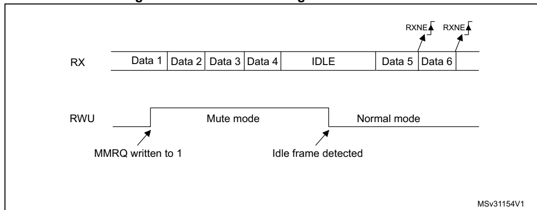
Figure 153. Mute mode using Idle line detection
