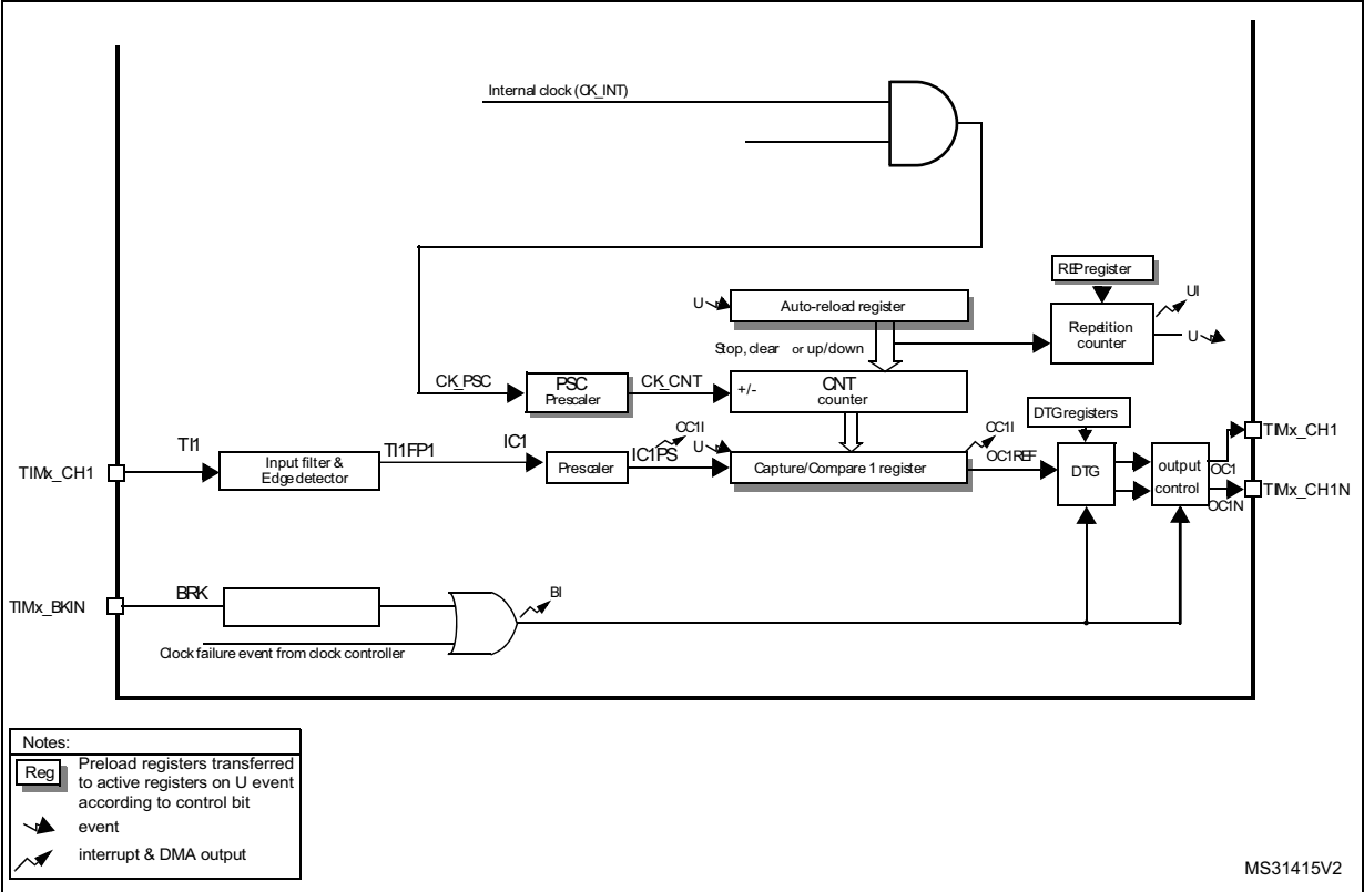
Figure 68. TIM16 and TIM17 block diagram
