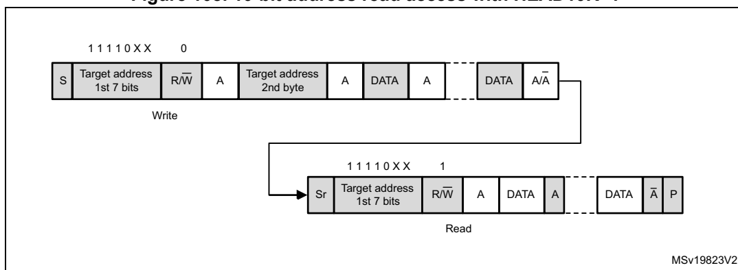
Figure 108. 10-bit address read access with HEAD10R=1
