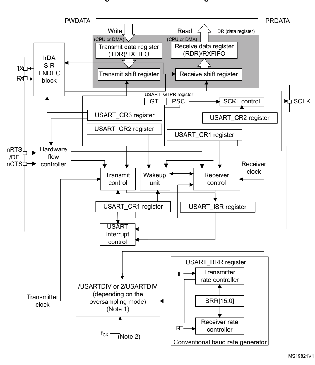
Figure 123. USART block diagram
