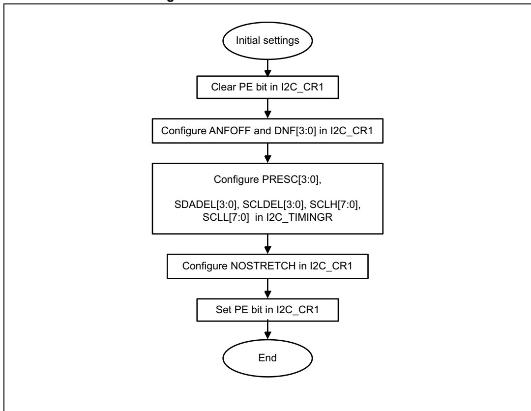
Figure 96. I2C initialization flowchart
