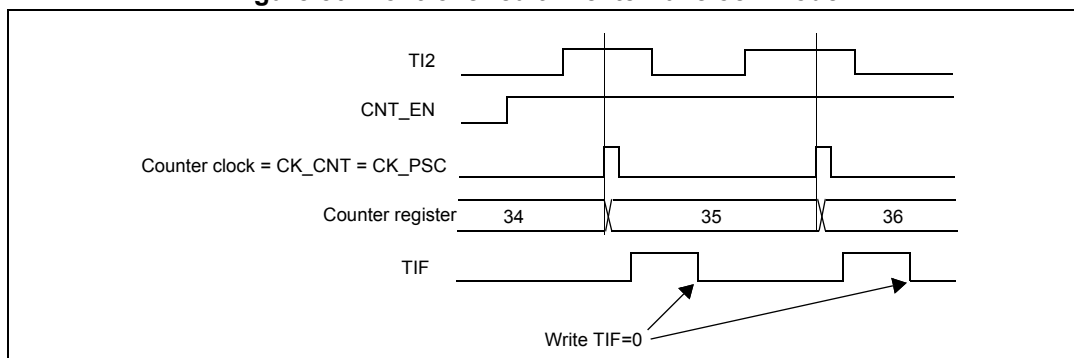
Figure 50. Control circuit in external clock mode 1
