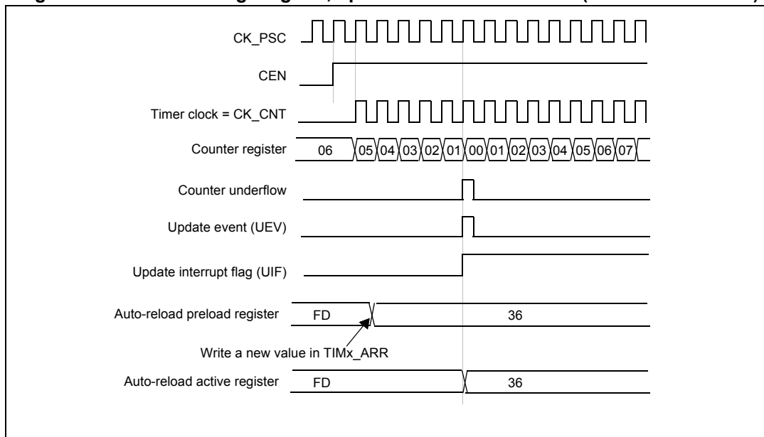
Figure 44. Counter timing diagram, update event with ARPE=1 (counter underflow)
