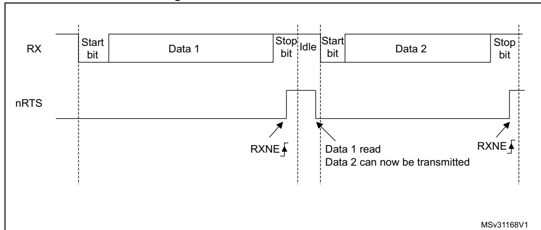
Figure 146. RS232 RTS flow control
