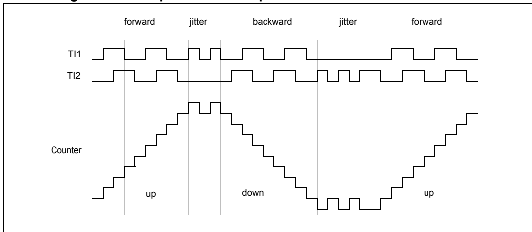
Figure 65. Example of counter operation in encoder interface mode.
