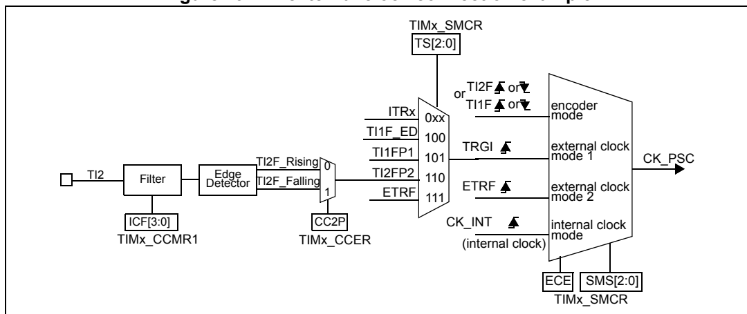
Figure 49. TI2 external clock connection example
