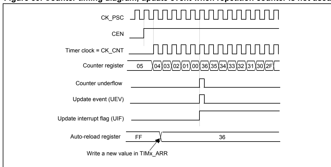
Figure 39. Counter timing diagram, update event when repetition counter is not used
