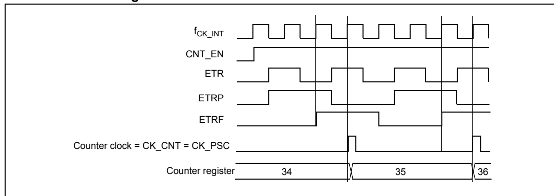
Figure 52. Control circuit in external clock mode 2
