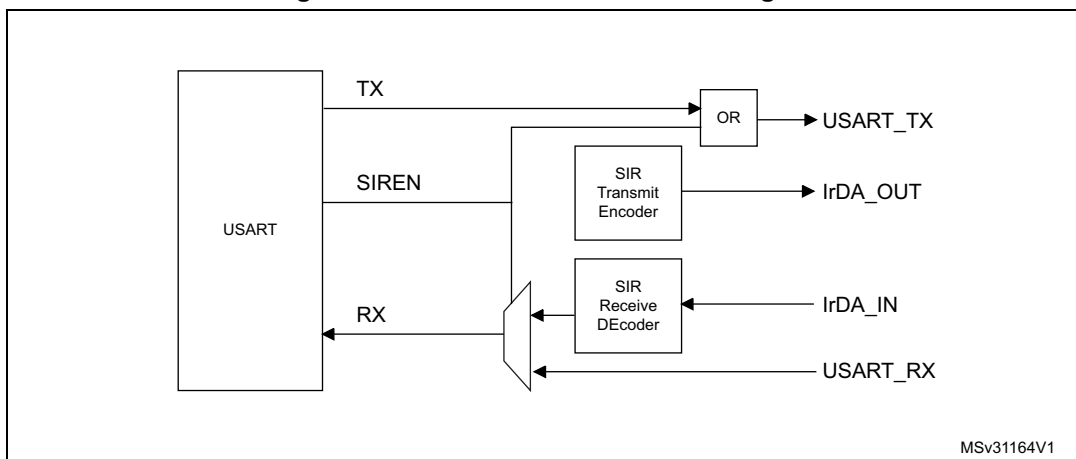
Figure 141. IrDA SIR ENDEC- block diagram
