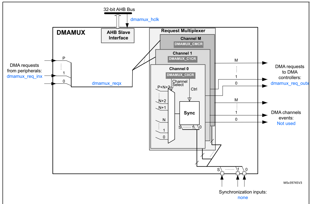
Figure 19. DMAMUX block diagram
