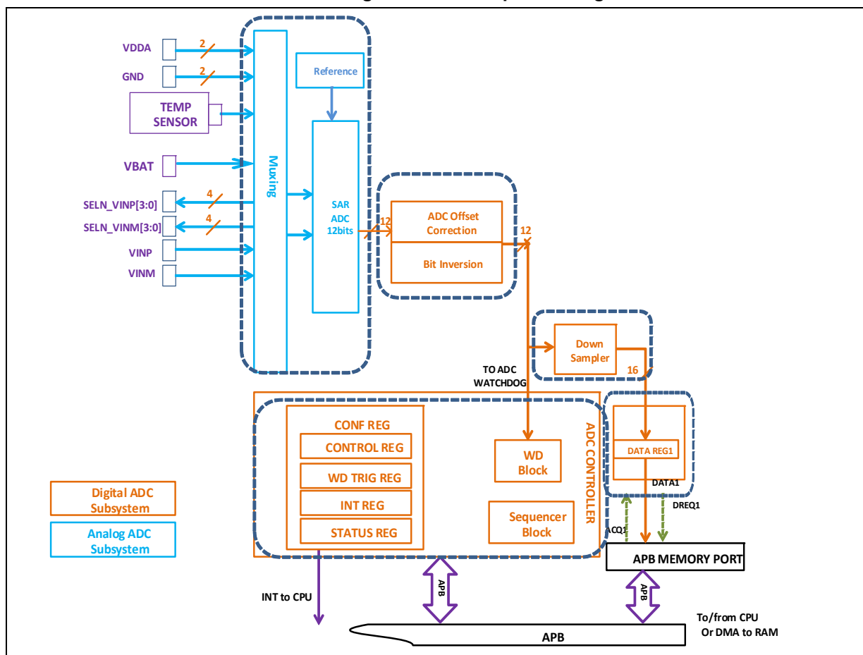
Figure 20. ADC top level diagram
