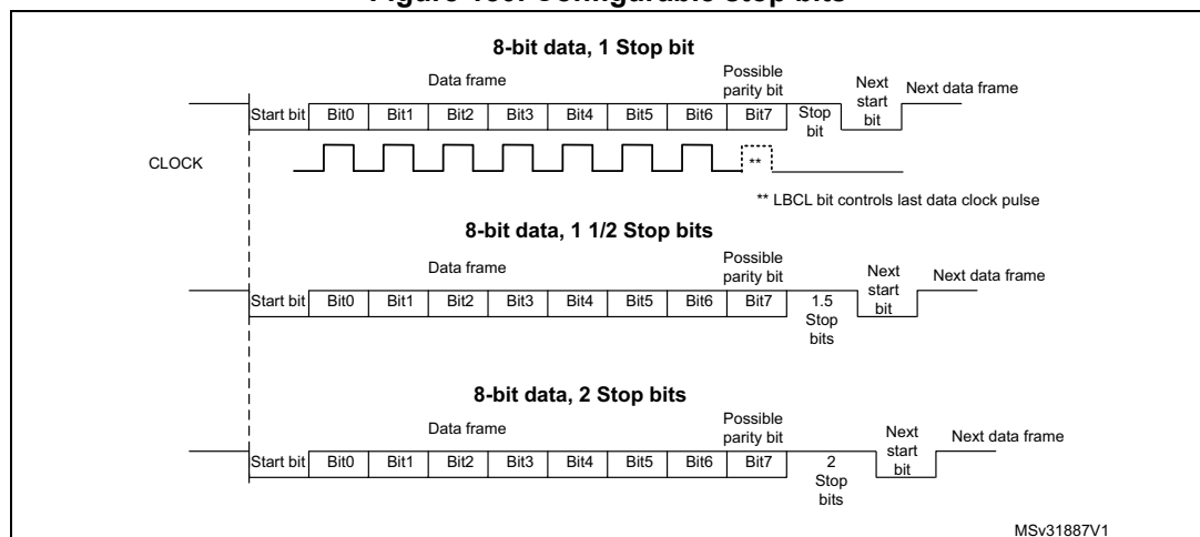
Figure 150. Configurable stop bits
