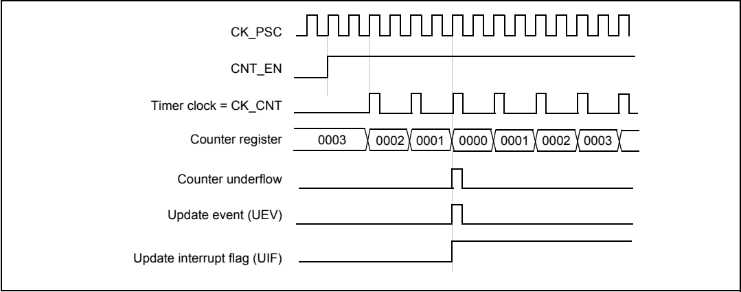
Figure 41. Counter timing diagram, internal clock divided by 2
