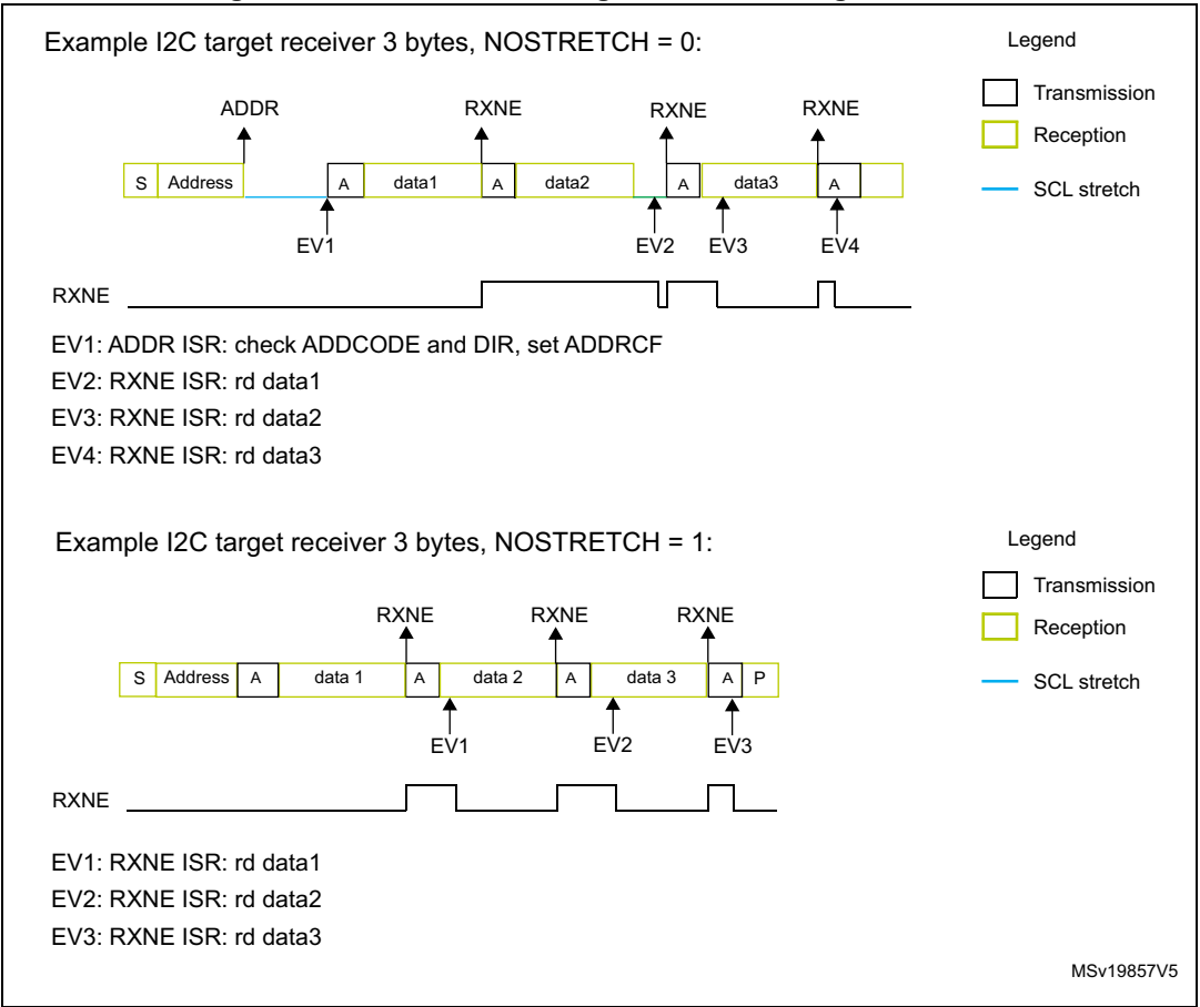
Figure 105. Transfer bus diagrams for I2C target receiver
