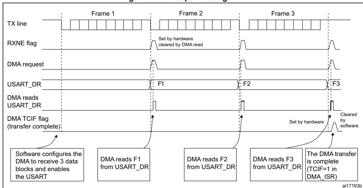
Figure 144. Reception using DMA
