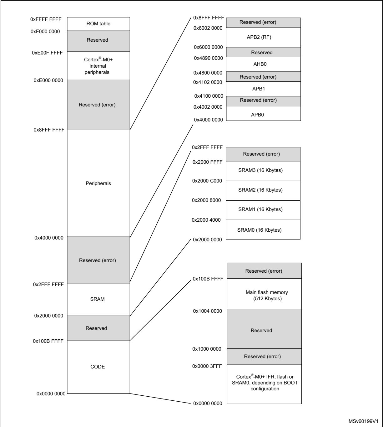
Figure 2. Memory map
