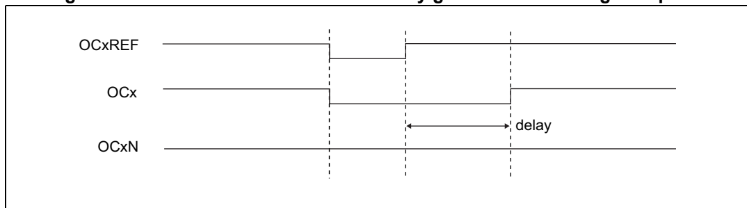
Figure 85. Dead-time waveforms with delay greater than the negative pulse.
