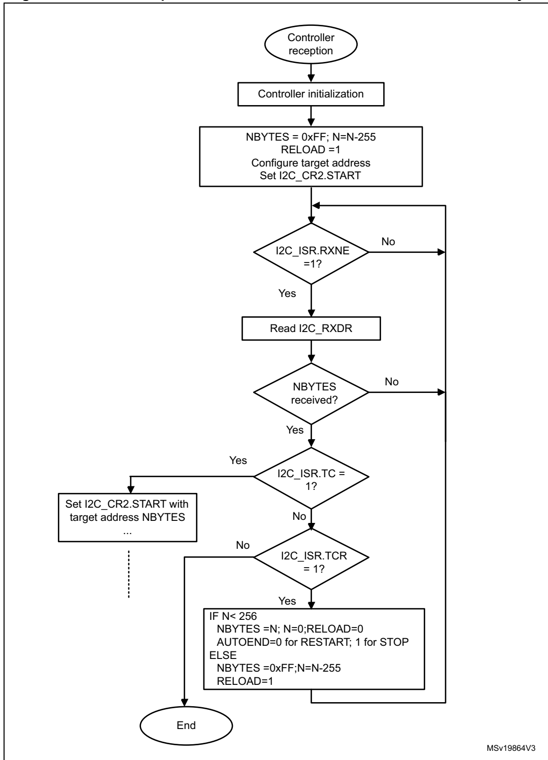
Figure 113. Transfer sequence flowchart for I2C controller receiver for N > 255 bytes
