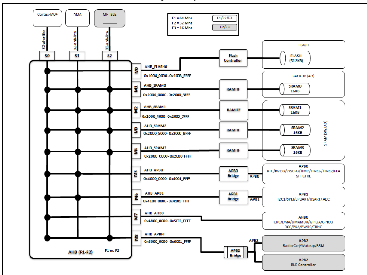
Figure 1. System architecture
