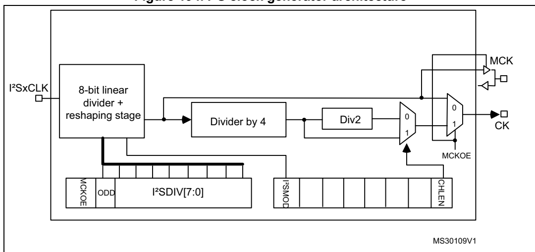
Figure 194. I 2 S clock generator architecture
