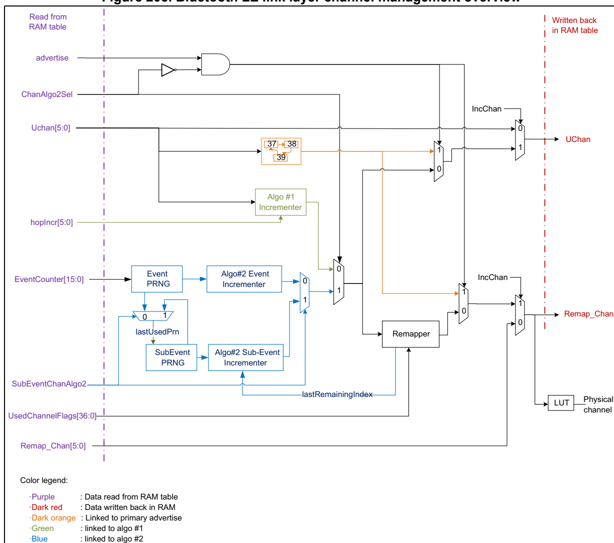
Figure 205. Bluetooth LE link layer channel management overview
