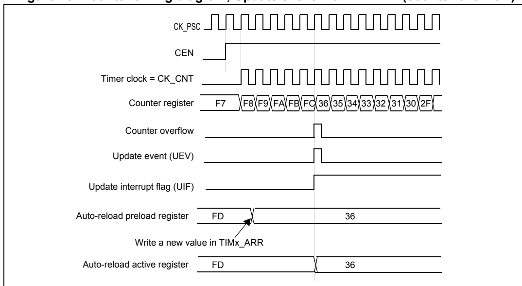
Figure 45. Counter timing diagram, Update event with ARPE=1 (counter overflow)
