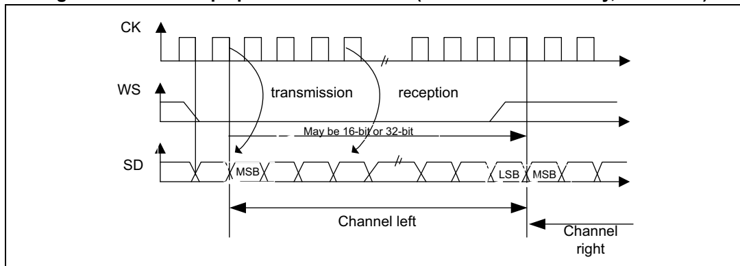
Figure 176. I 2 S Philips protocol waveforms (16/32-bit full accuracy, CPOL = 0)
