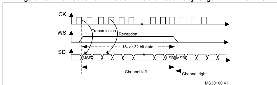
Figure 182. MSB Justified 16-bit or 32-bit full-accuracy length with CPOL = 0
