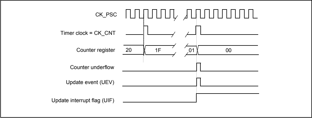
Figure 43. Counter timing diagram, internal clock divided by N
