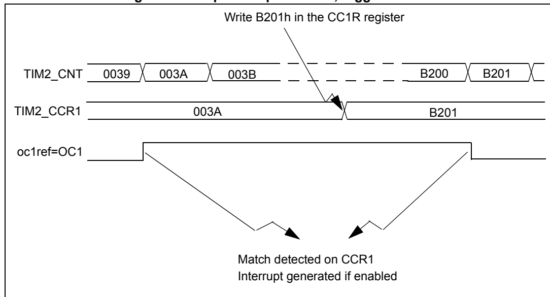
Figure 57. Output compare mode, toggle on OC1
