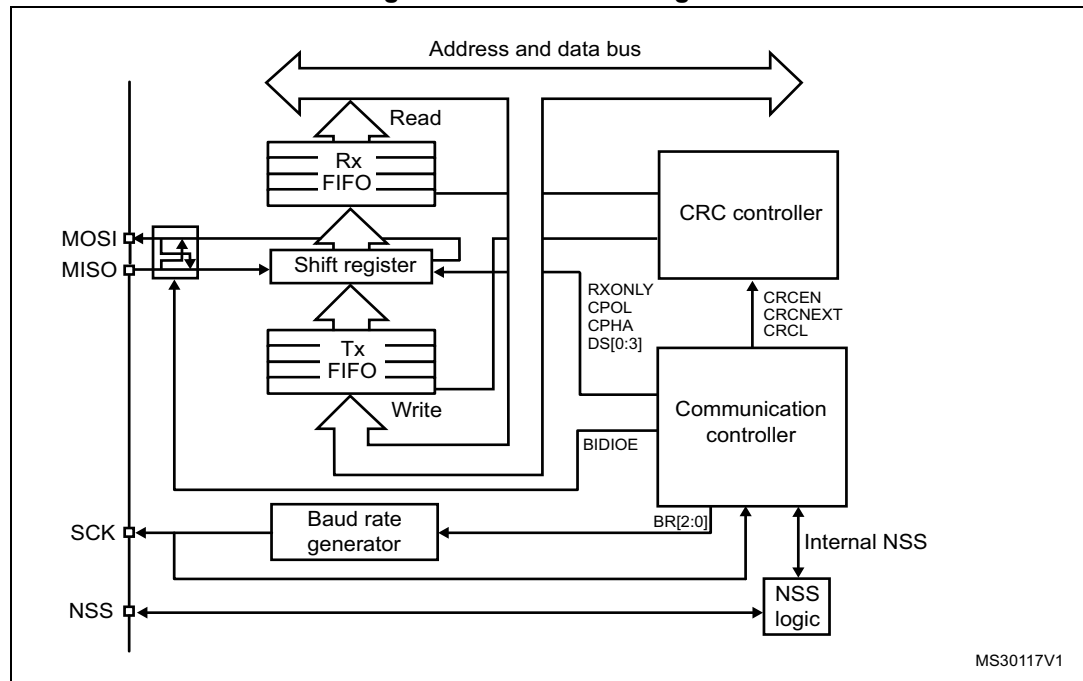
Figure 160. SPI block diagram
