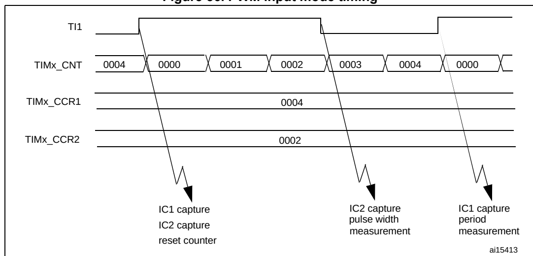
Figure 56. PWM input mode timing
