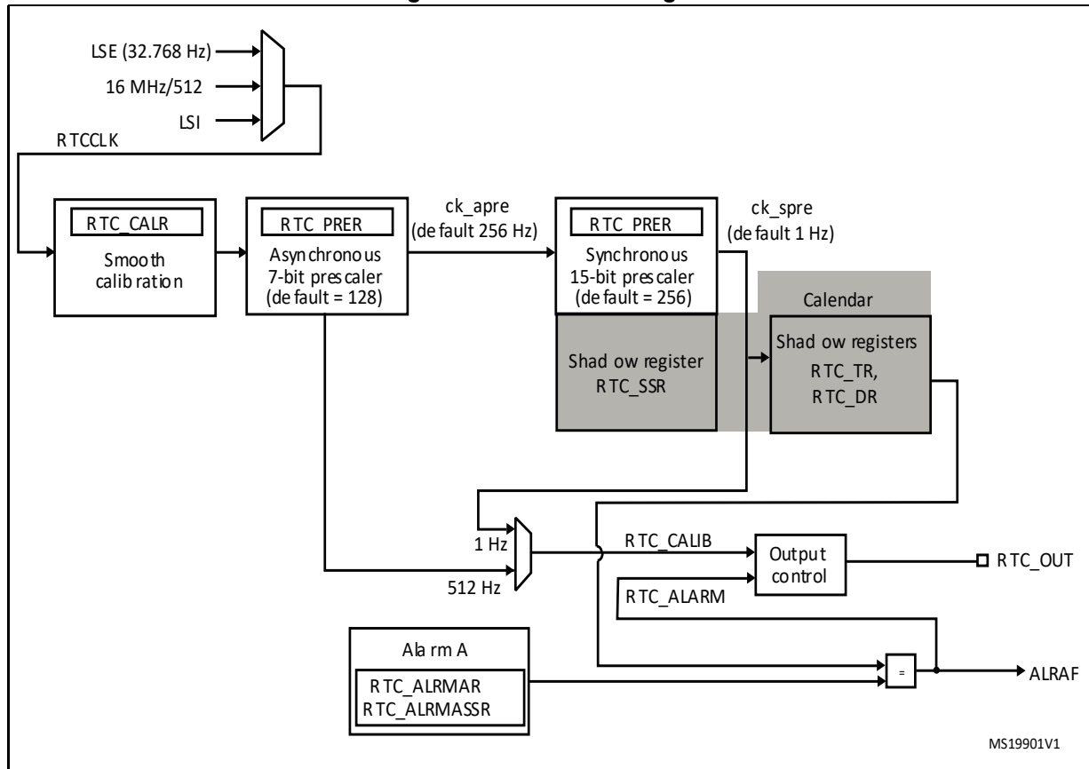
Figure 91. RTC block diagram
