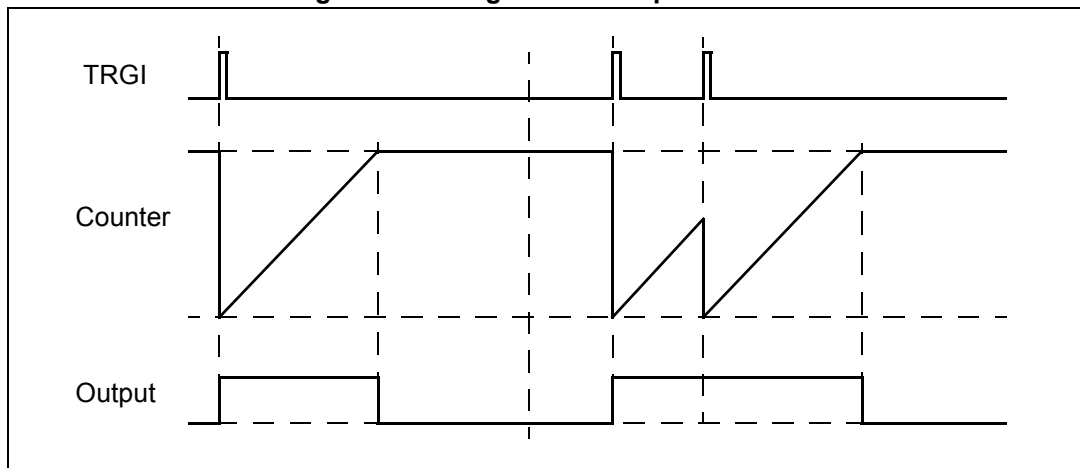
Figure 64. Retriggerable one pulse mode
