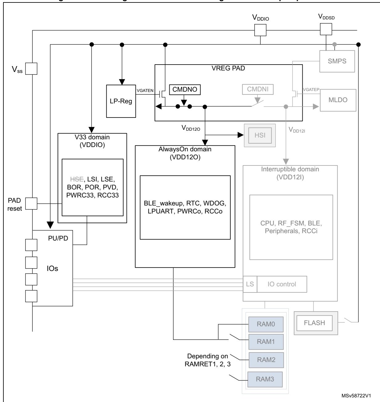
Figure 7. Power regulators and SMPS configuration in Deepstop mode (a)
