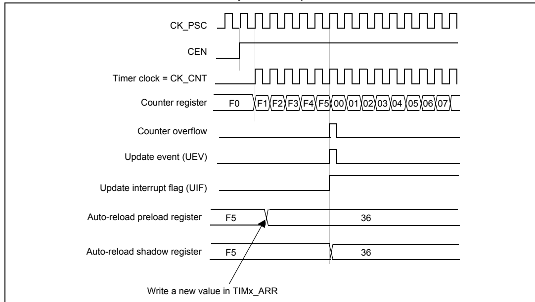
Figure 34. Counter timing diagram, update event when ARPE=1 (TIMx_ARR preloaded)
