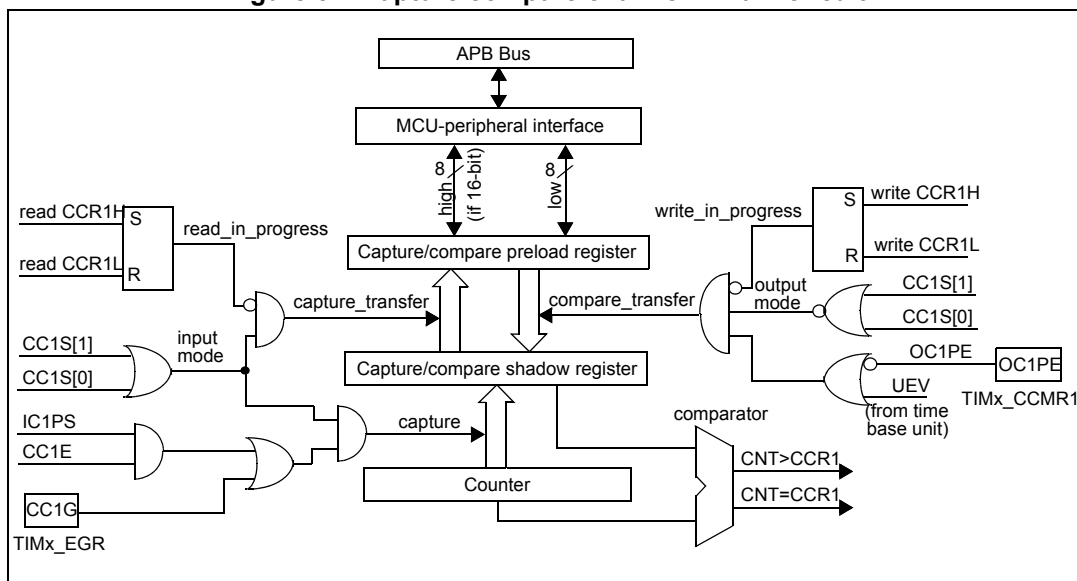
Figure 54. Capture/compare channel 1 main circuit
