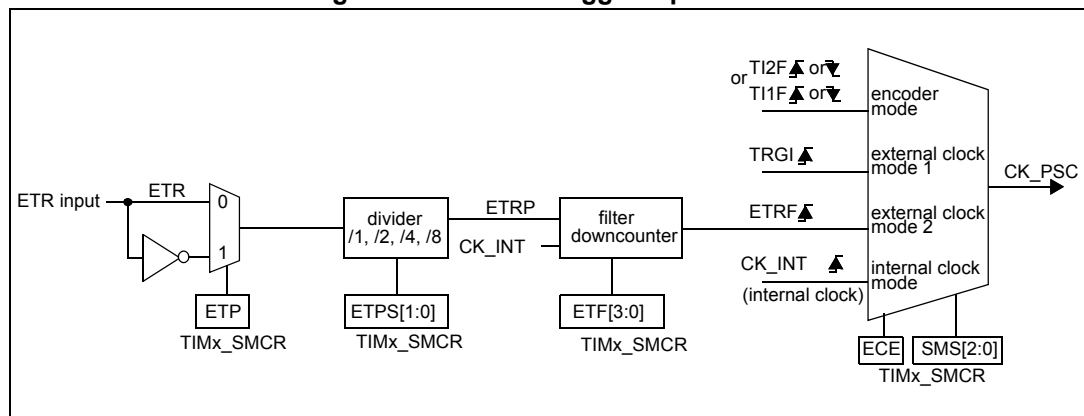
Figure 47. External trigger input block
