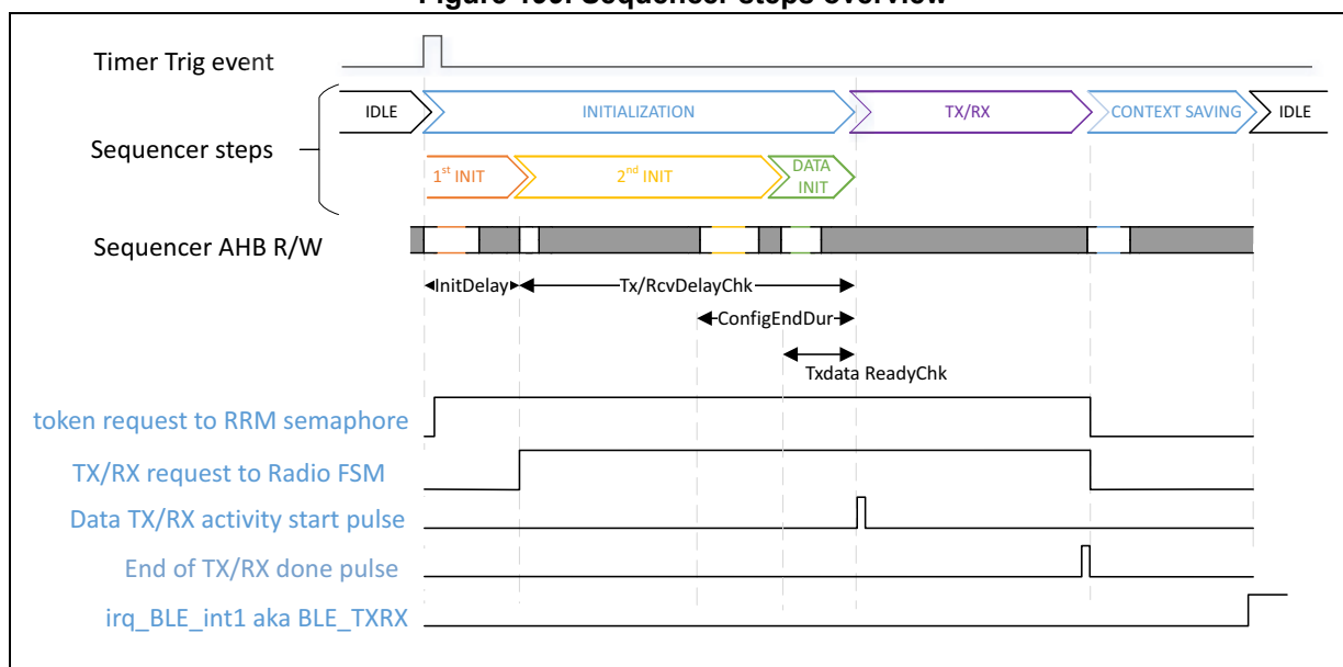
Figure 199. Sequencer steps overview
