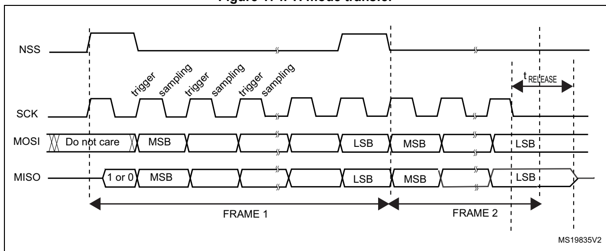
Figure 174. TI mode transfer
