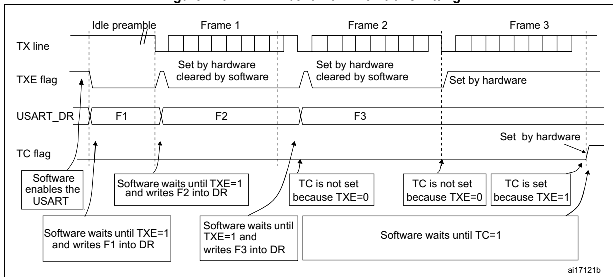
Figure 126. TC/TXE behavior when transmitting
