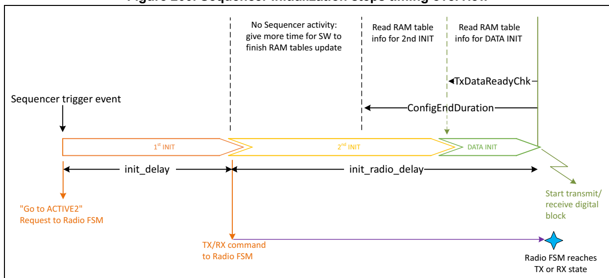
Figure 200. Sequencer Initialization steps timing overview
