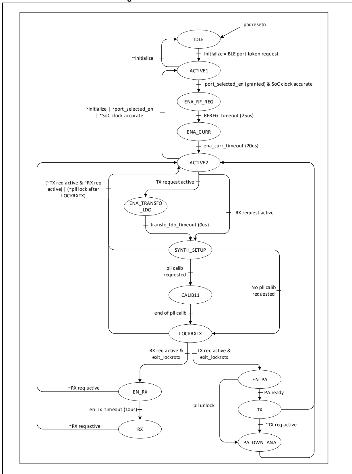
Figure 198. Radio FSM overview
