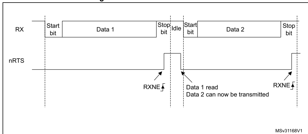
Figure 158. RS232 RTS flow control
