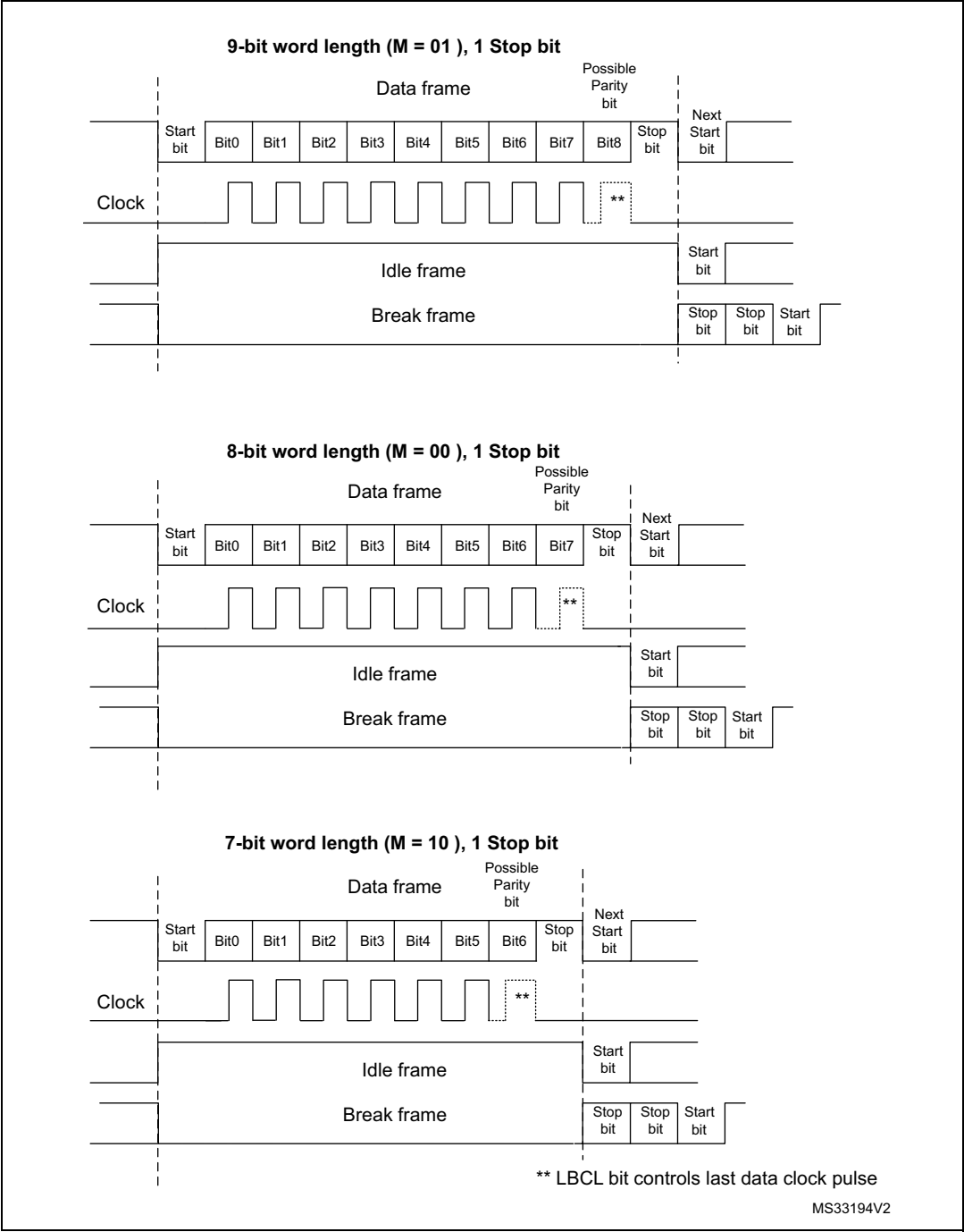
Figure 124. Word length programming
