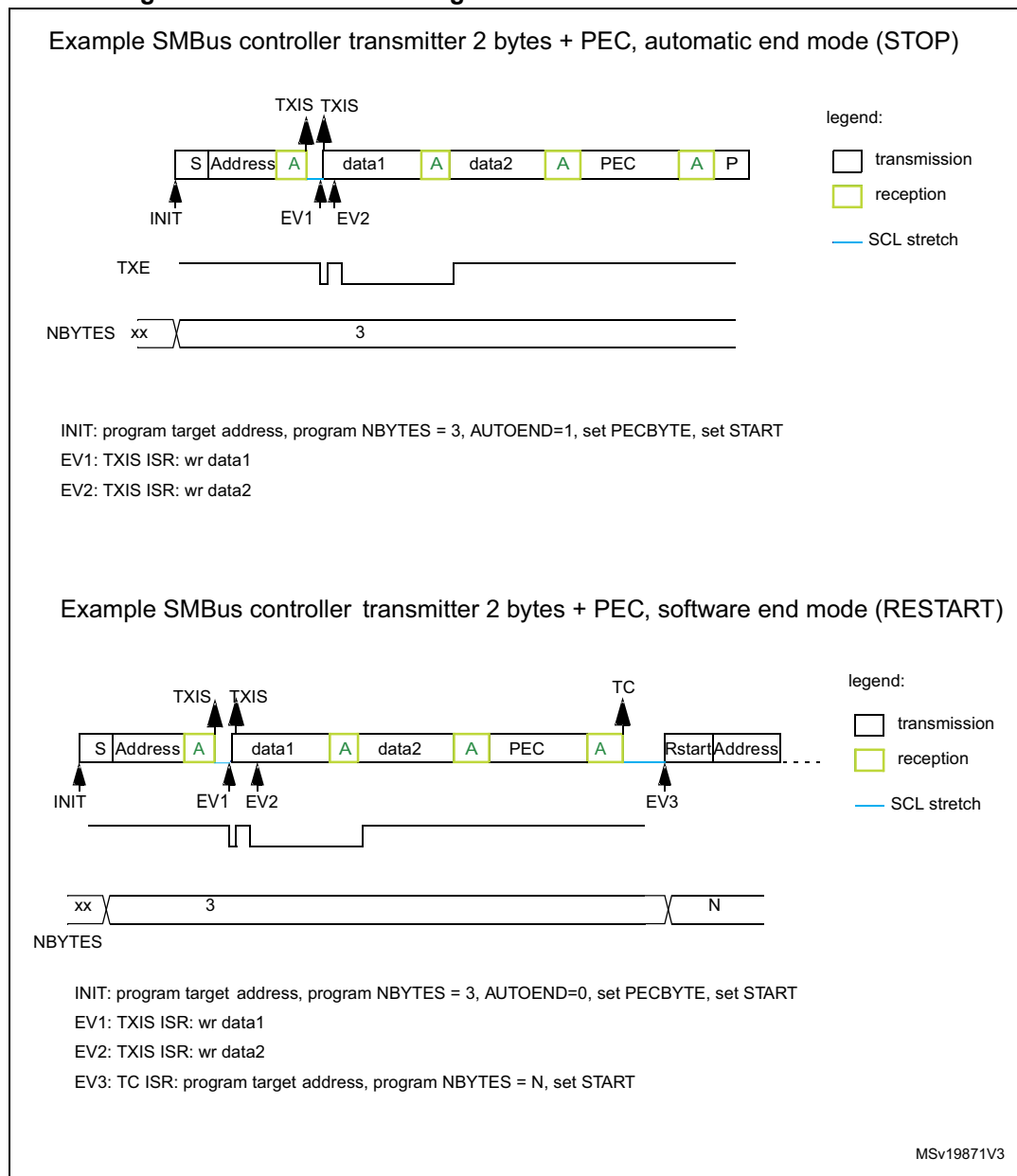
Figure 120. Bus transfer diagrams for SMBus controller transmitter
