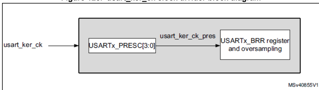
Figure 128. usart_ker_ck clock divider block diagram
