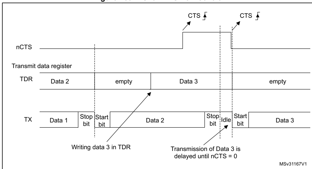
Figure 159. RS232 CTS flow control
