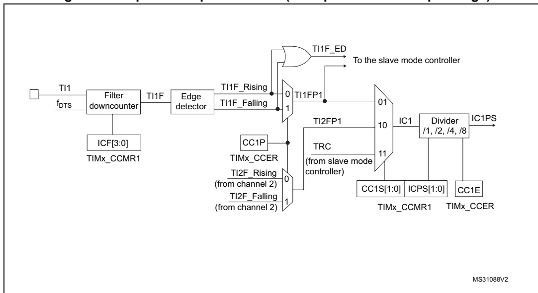
Figure 79. Capture/compare channel (example: channel 1 input stage)
