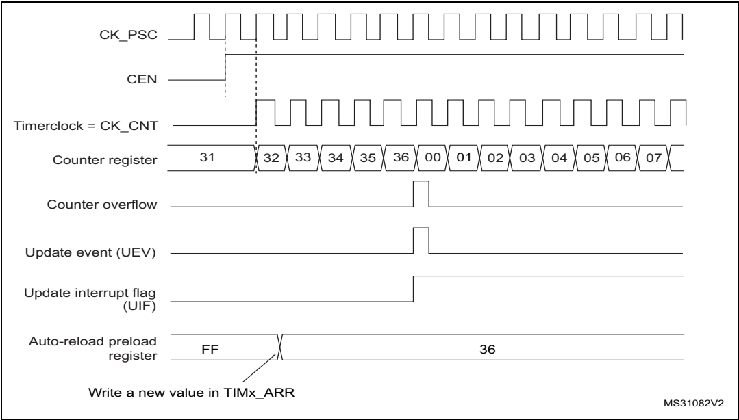
Figure 75. Counter timing diagram, update event when ARPE=0 (TIMx_ARR not preloaded)
