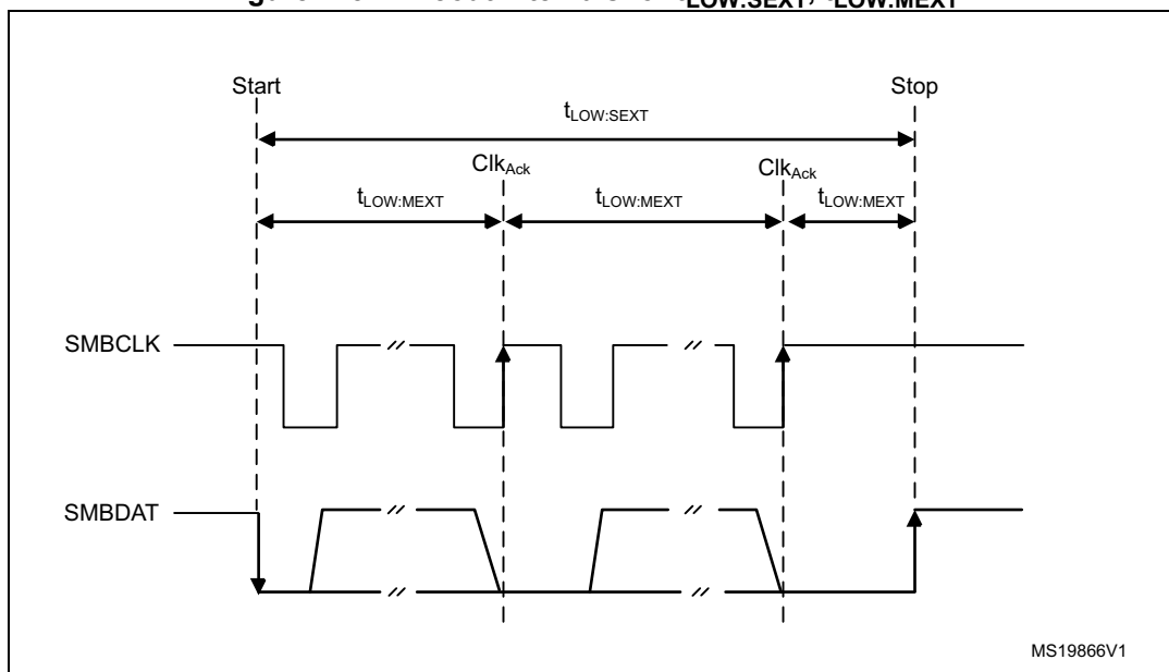
Figure 115. Timeout intervals for t_{\text{LOW:SEXT}} , t_{\text{LOW:MEXT}}
