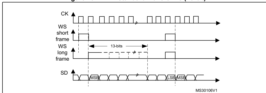
Figure 191. PCM standard waveforms (16-bit)
