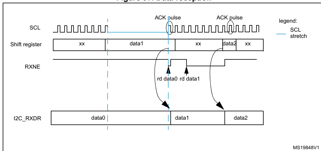
Figure 97. Data reception
