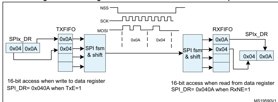
Figure 168. Packing data in FIFO for transmission and reception
