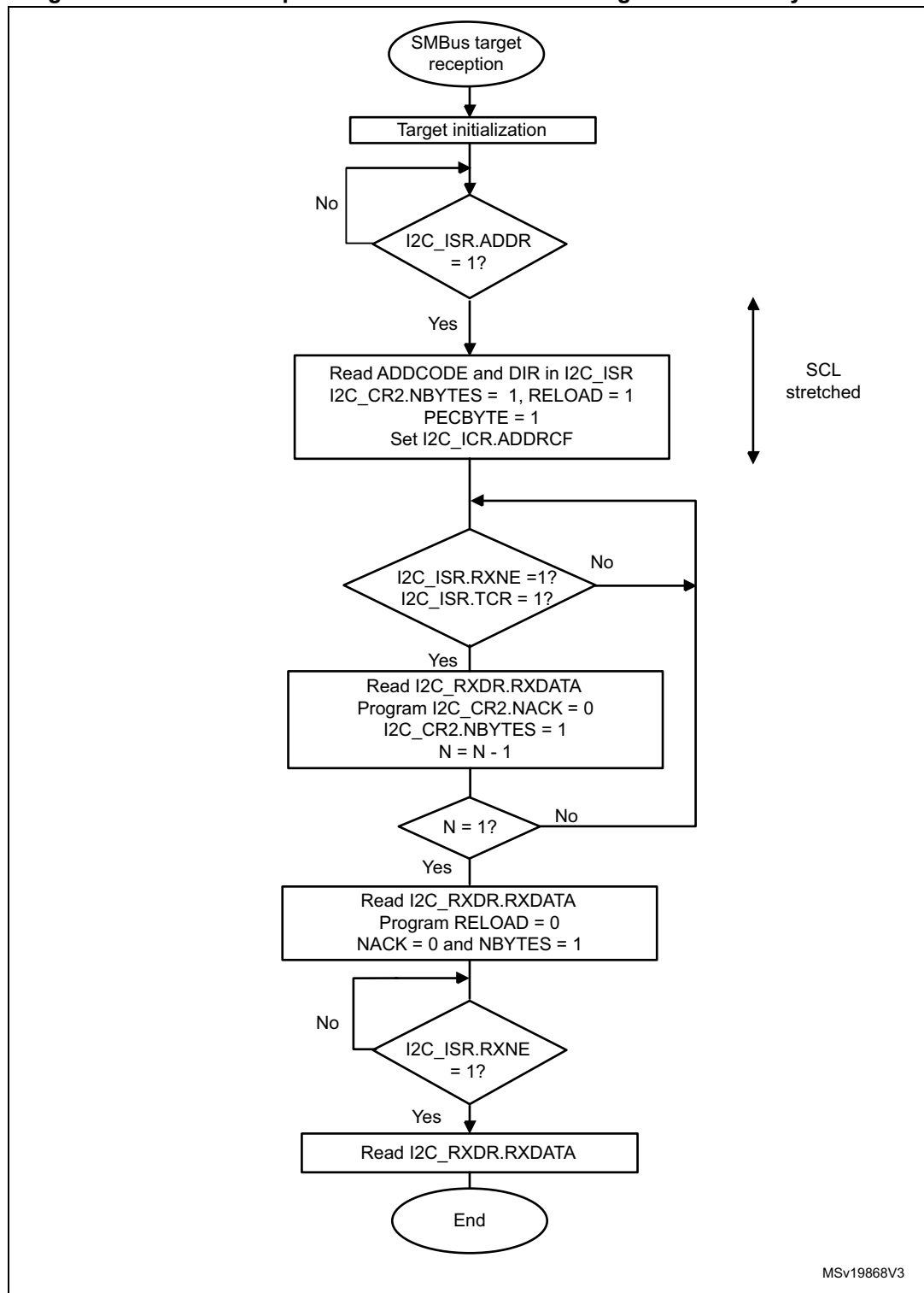
Figure 118. Transfer sequence flowchart for SMBus target receiver N Bytes + PEC
