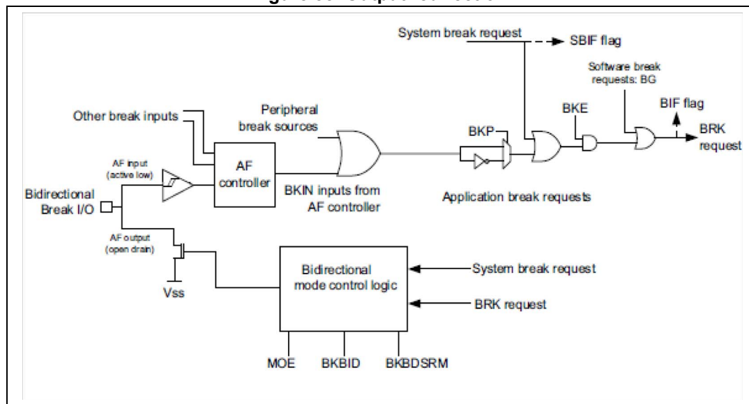
Figure 88. Output redirection
