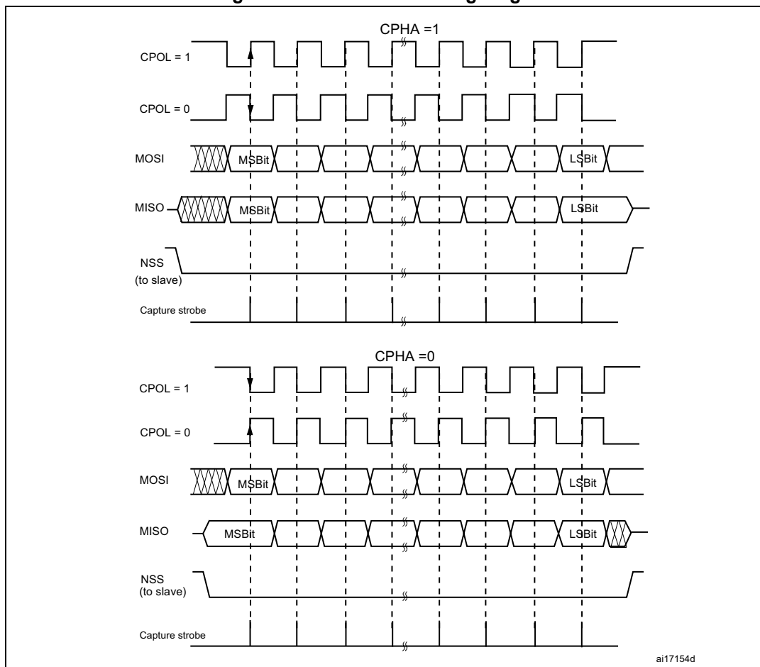
Figure 166. Data clock timing diagram
