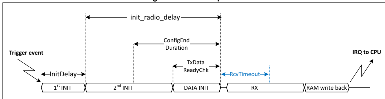
Figure 202. RX sequence
