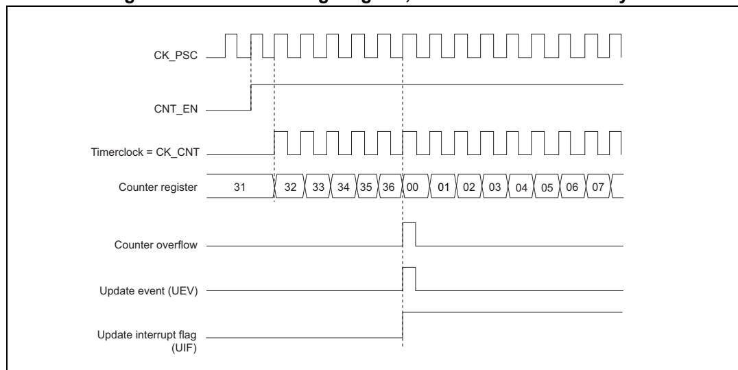
Figure 71. Counter timing diagram, internal clock divided by 1
