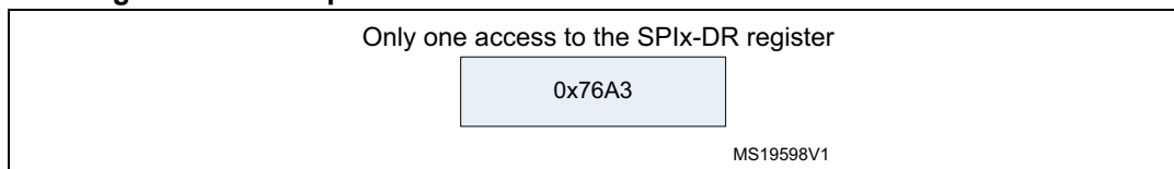
Figure 190. Example of 16-bit data frame extended to 32-bit channel frame
