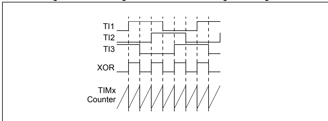
Figure 67. Measuring time interval between edges on 3 signals
