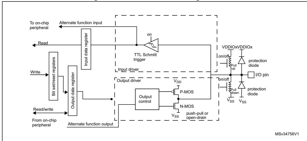
Figure 17. Alternate function configuration
