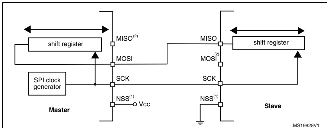
Figure 162. Half-duplex single master/ single slave application
