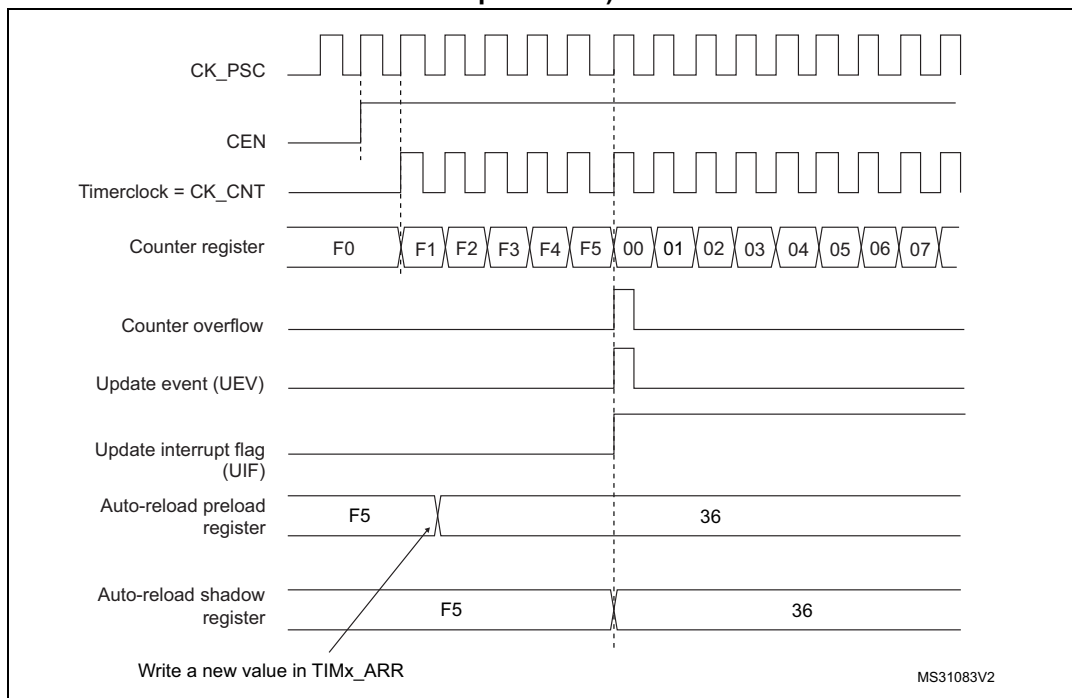
Figure 76. Counter timing diagram, update event when ARPE=1 (TIMx_ARR preloaded)
