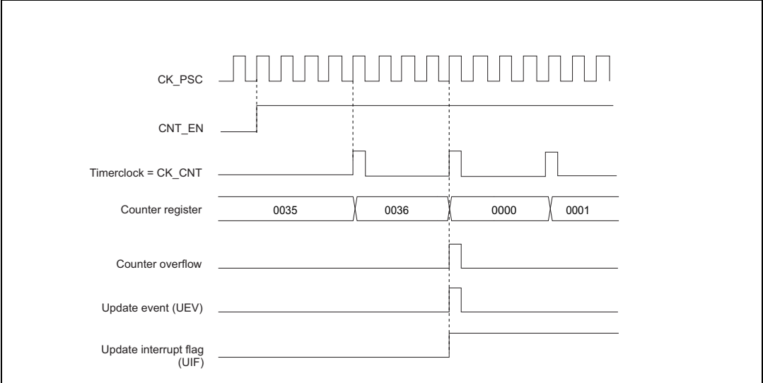
Figure 73. Counter timing diagram, internal clock divided by 4
