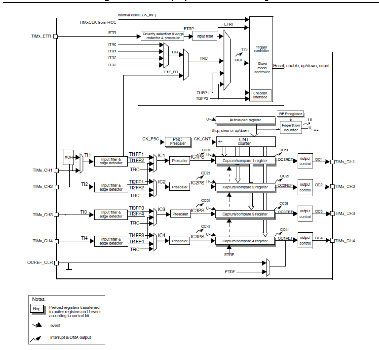
Figure 26. General purpose timer block diagram
