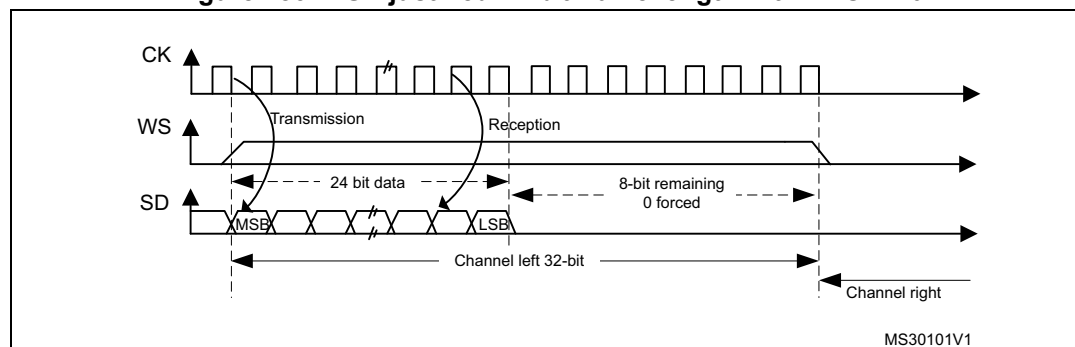
Figure 183. MSB justified 24-bit frame length with CPOL = 0
