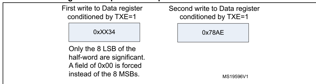
Figure 187. Operations required to transmit 0x3478AE
