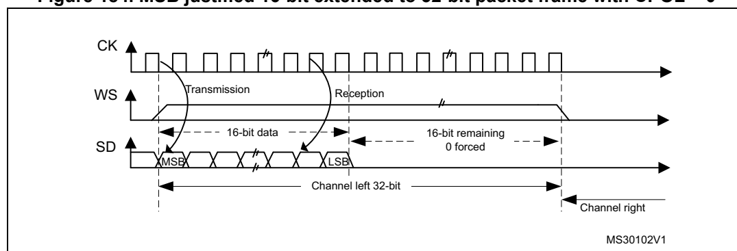
Figure 184. MSB justified 16-bit extended to 32-bit packet frame with CPOL = 0
