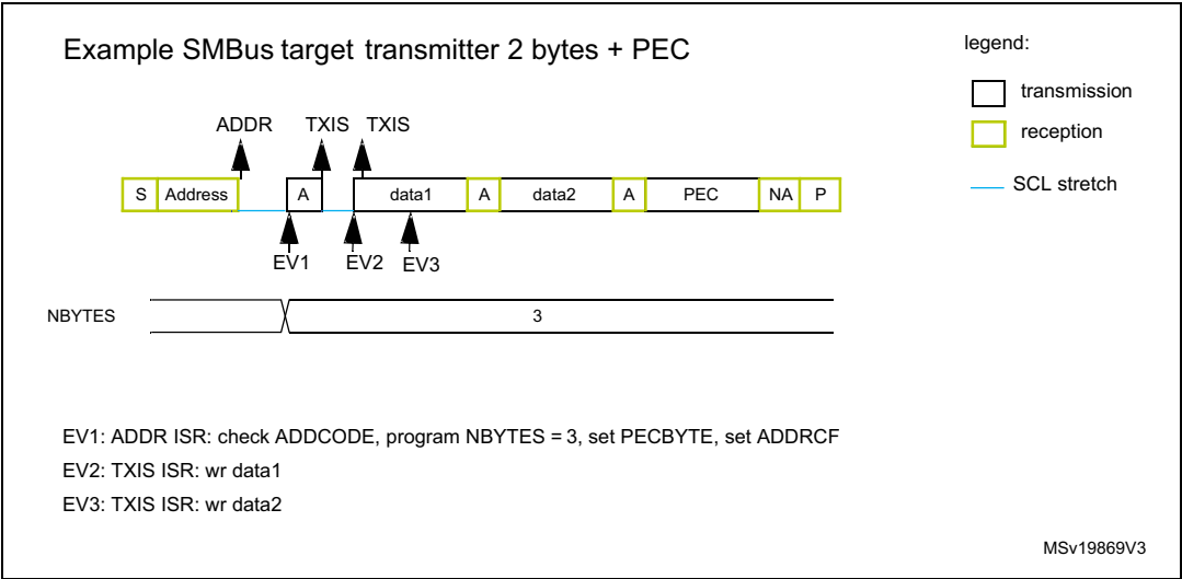
Figure 117. Transfer bus diagrams for SMBus target transmitter (SBC=1)
