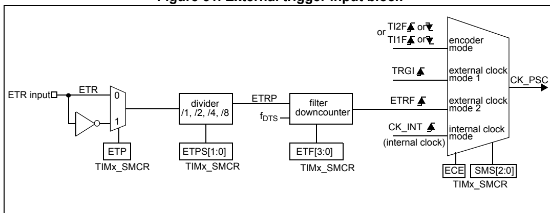
Figure 51. External trigger input block
