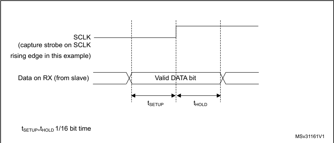
Figure 138. RX data setup/hold time
