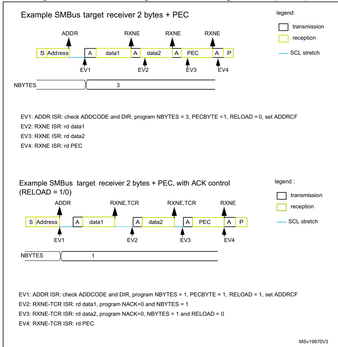
Figure 119. Bus transfer diagrams for SMBus target receiver (SBC=1)
