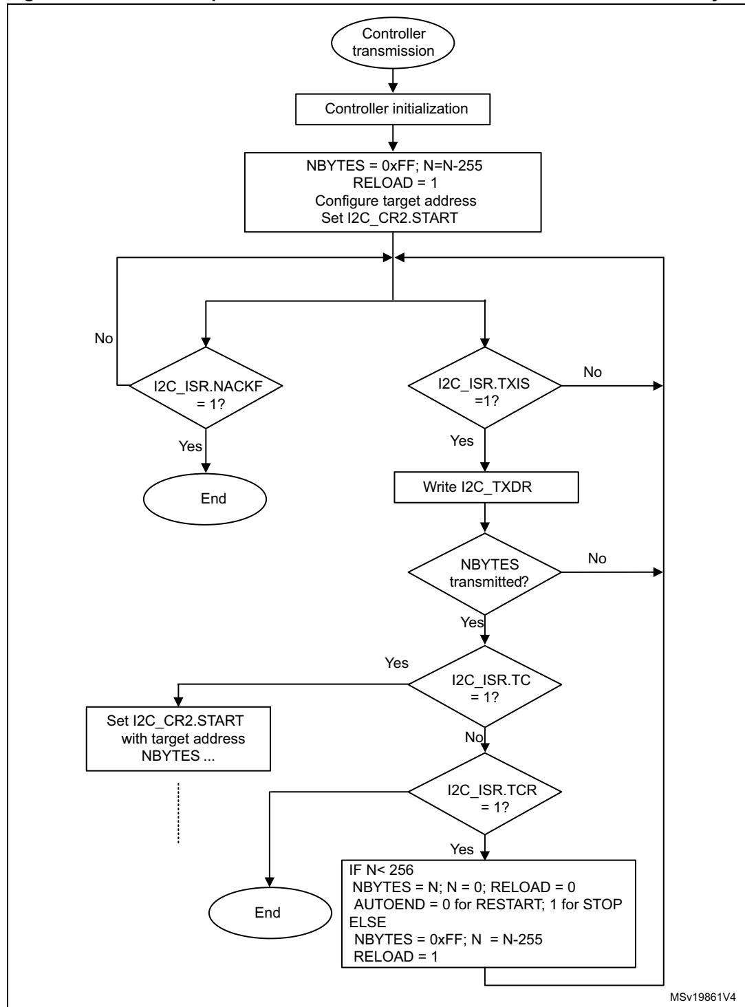
Figure 110. Transfer sequence flowchart for I2C controller transmitter for N&gt;255 bytes
