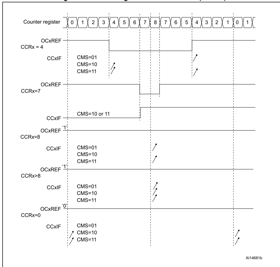
Figure 59. Center-aligned PWM waveforms (ARR=8)
