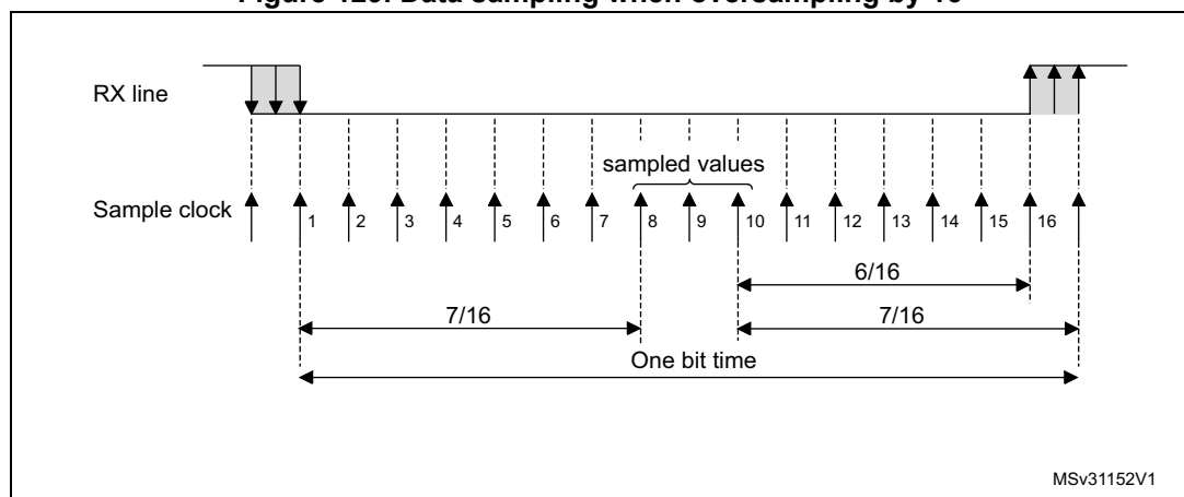
Figure 129. Data sampling when oversampling by 16
