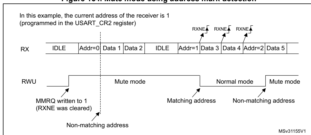
Figure 154. Mute mode using address mark detection
