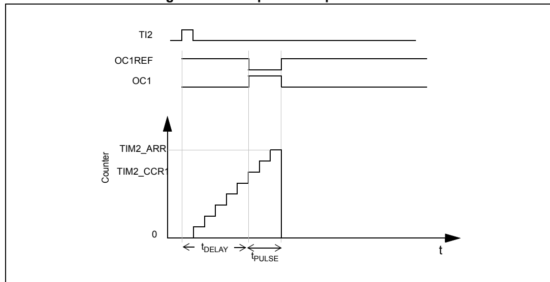
Figure 63. Example of one pulse mode.
