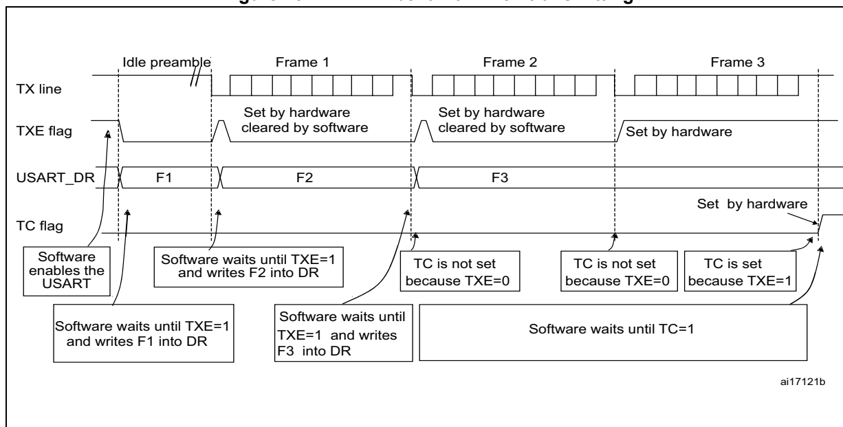
Figure 151. TC/TXE behavior when transmitting
