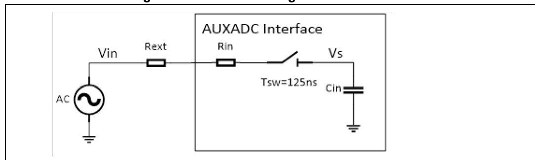
Figure 22. Effect of analog source resistance
