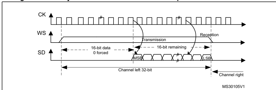
Figure 189. LSB justified 16-bit extended to 32-bit packet frame with CPOL = 0
