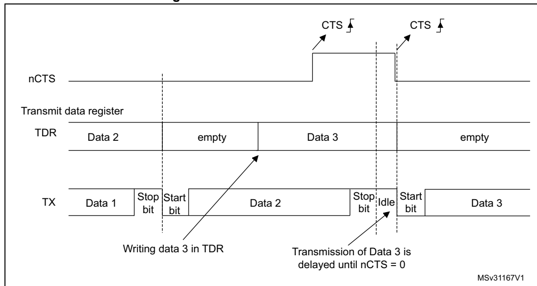
Figure 147. RS232 CTS flow control
