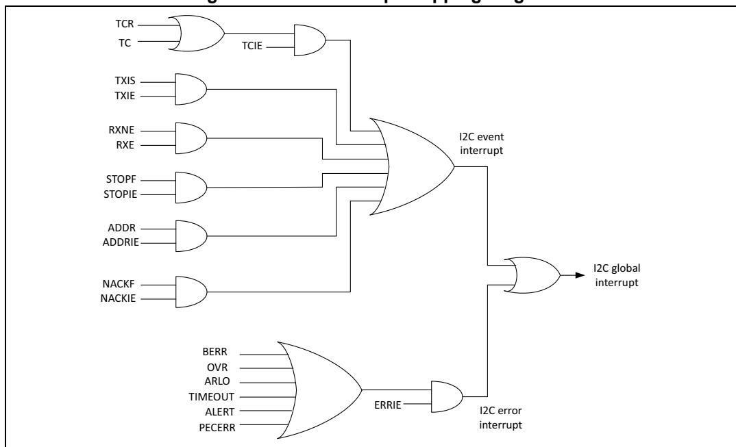
Figure 122. I2C interrupt mapping diagram
