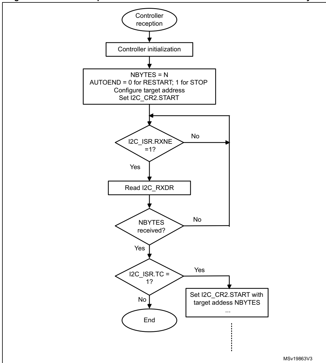
Figure 112. Transfer sequence flowchart for I2C controller receiver for N \leq 255 bytes
