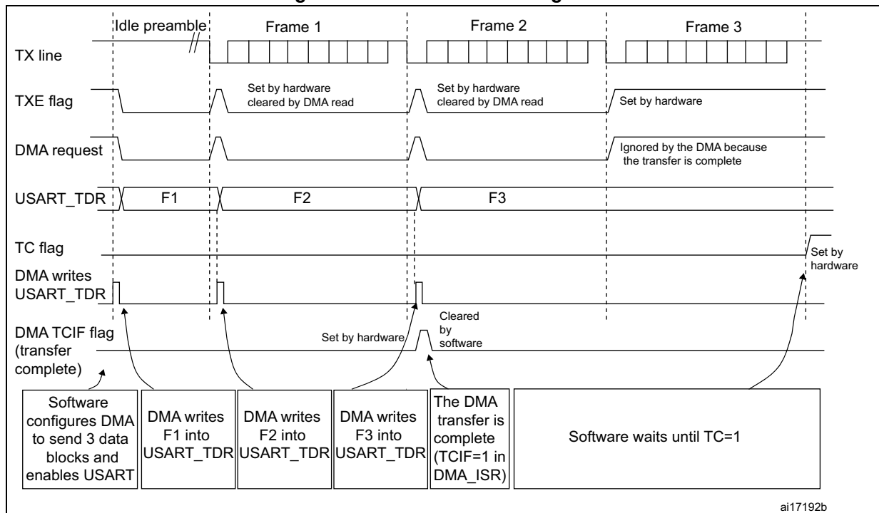
Figure 155. Transmission using DMA
