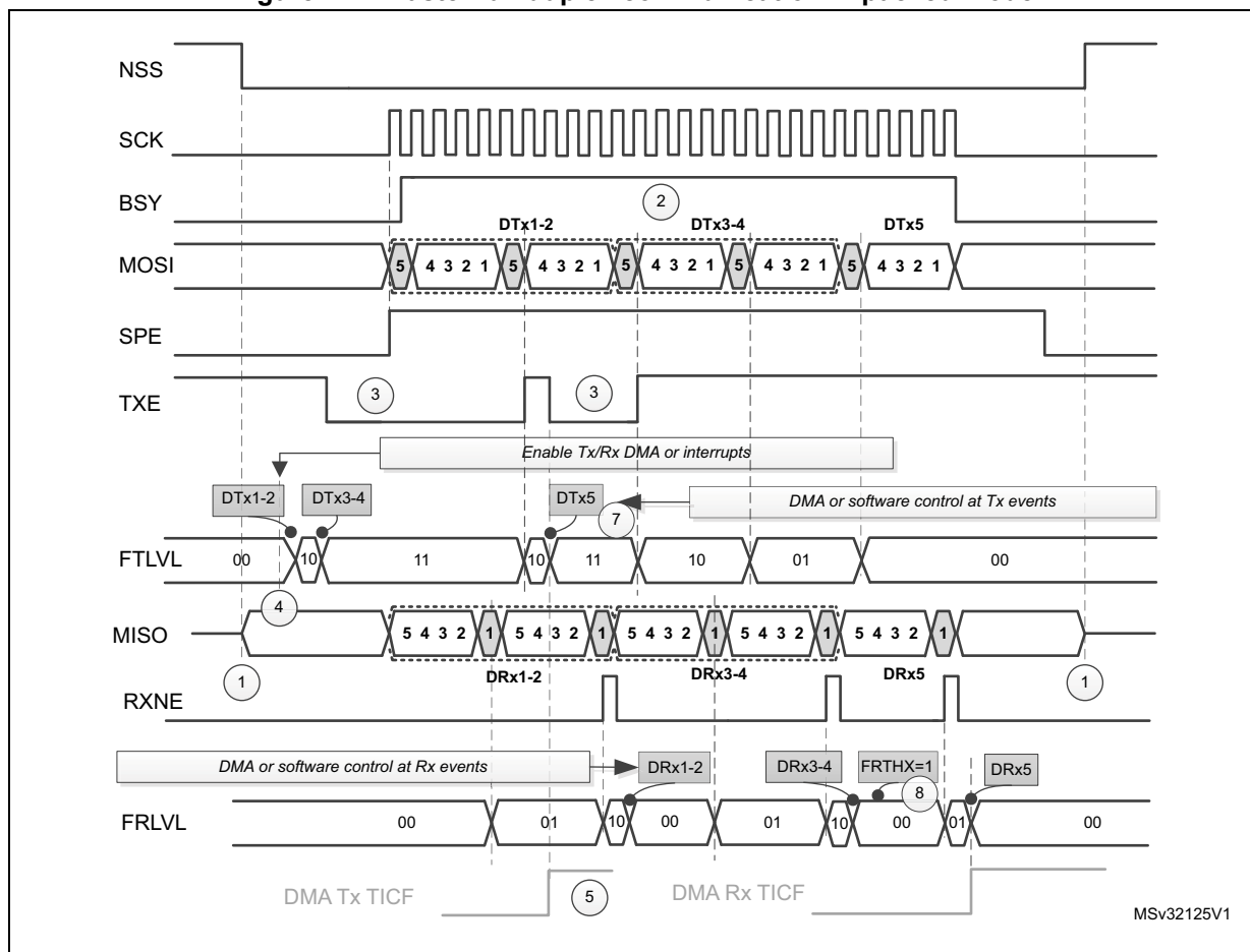
Figure 172. Master full duplex communication in packed mode
