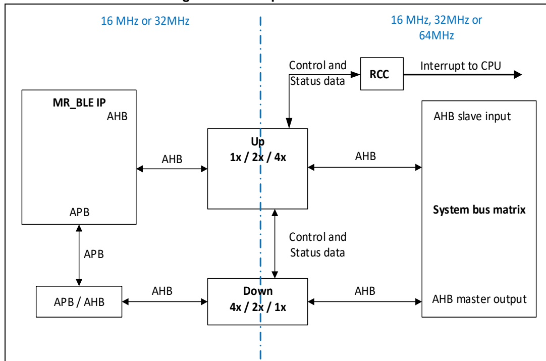
Figure 3. AHB up/down converter
