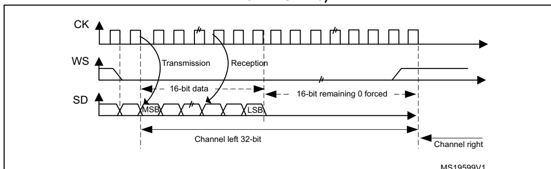
Figure 180. I 2 S Philips standard (16-bit extended to 32-bit packet frame with CPOL = 0)
