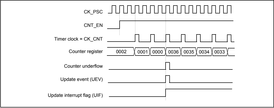
Figure 36. Counter timing diagram, internal clock divided by 2
