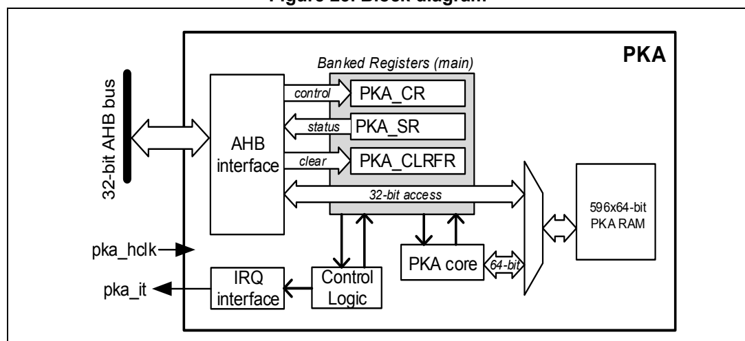
Figure 23. Block diagram
