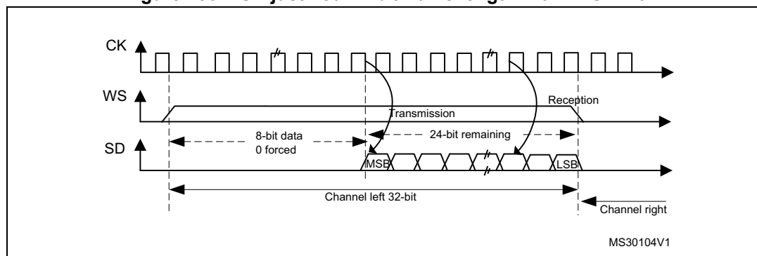
Figure 186. LSB justified 24-bit frame length with CPOL = 0
