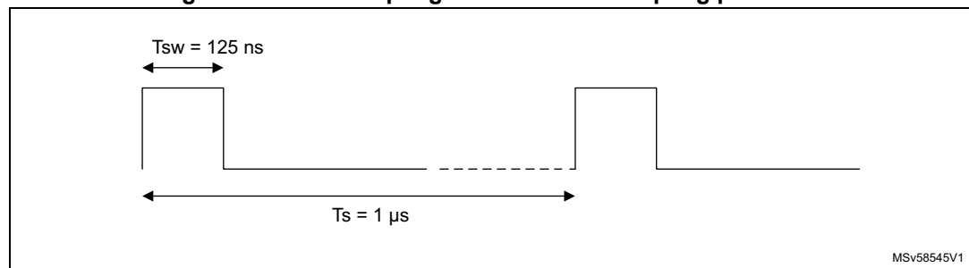
Figure 21. ADC sampling time T_{sw} and sampling period T_s
