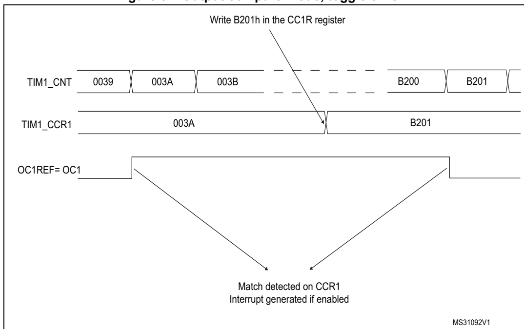
Figure 82. Output compare mode, toggle on OC1
