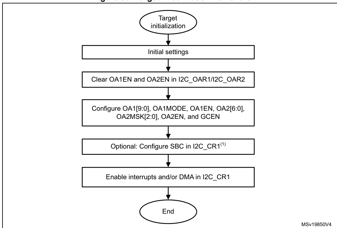
Figure 99. Target initialization flowchart
