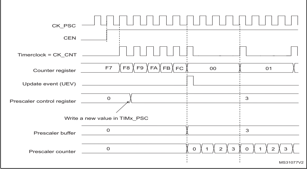
Figure 70. Counter timing diagram with prescaler division change from 1 to 4
