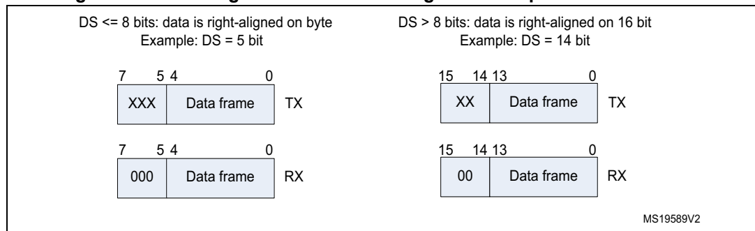
Figure 167. Data alignment when data length is not equal to 8-bit or 16-bit
