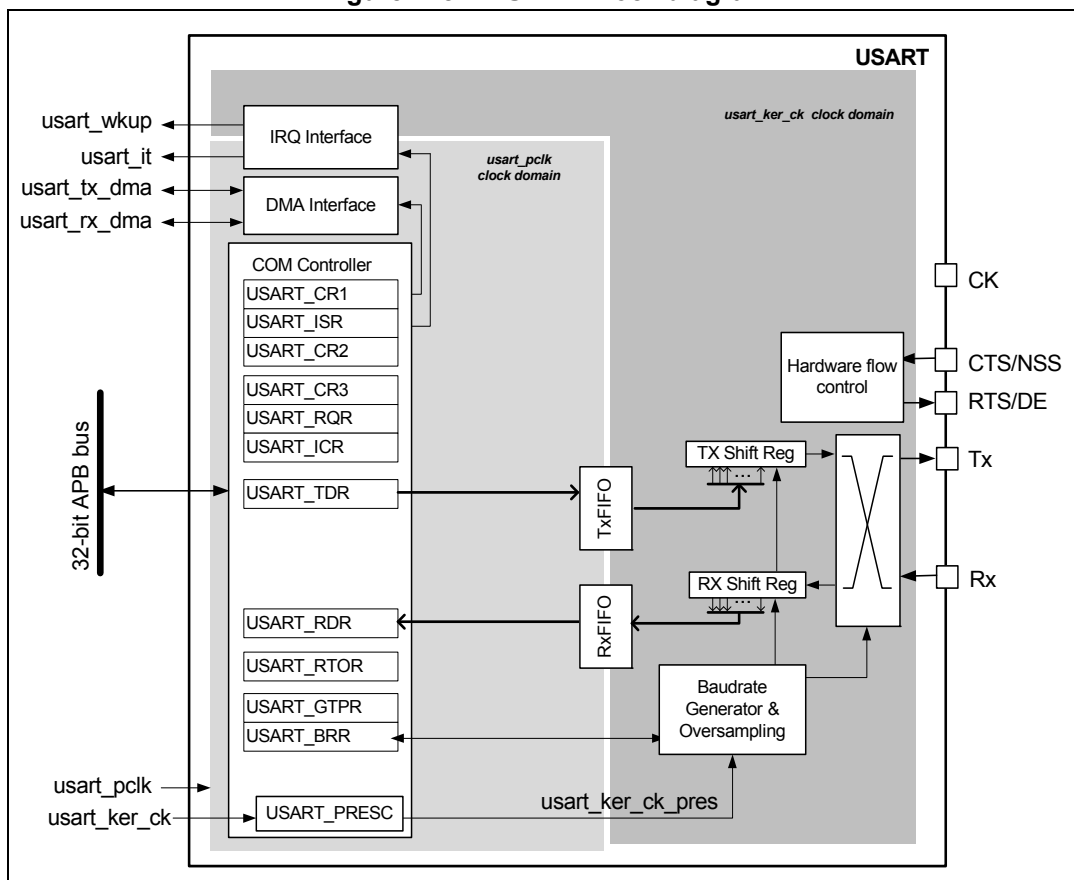
Figure 148. LPUART Block diagram
