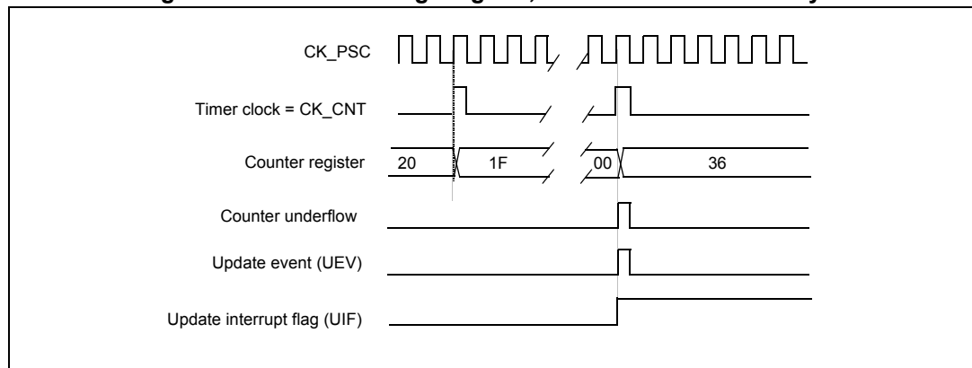
Figure 39. Counter timing diagram, update event when repetition counter is not used
