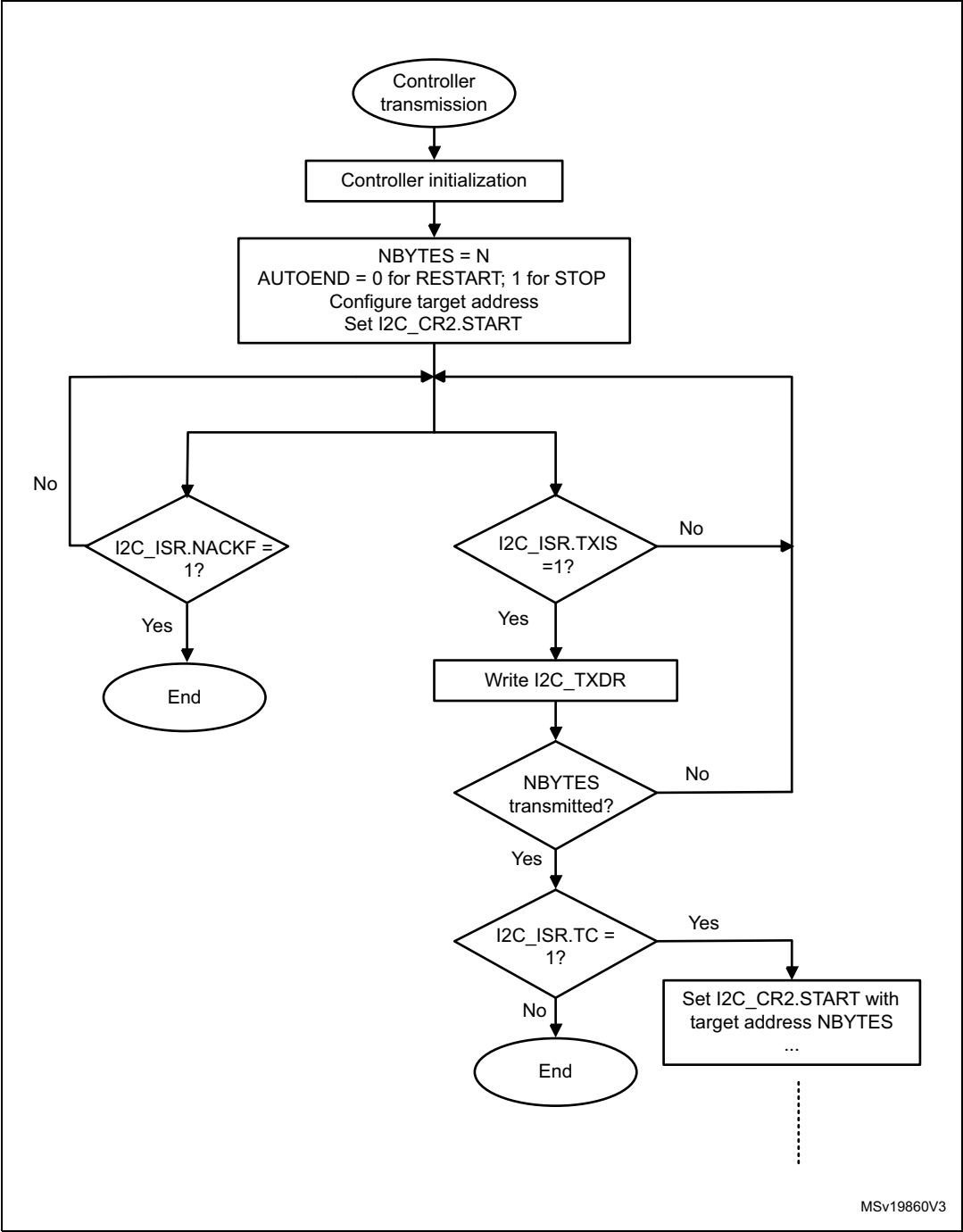
Figure 109. Transfer sequence flowchart for I2C controller transmitter for N≤255 bytes
