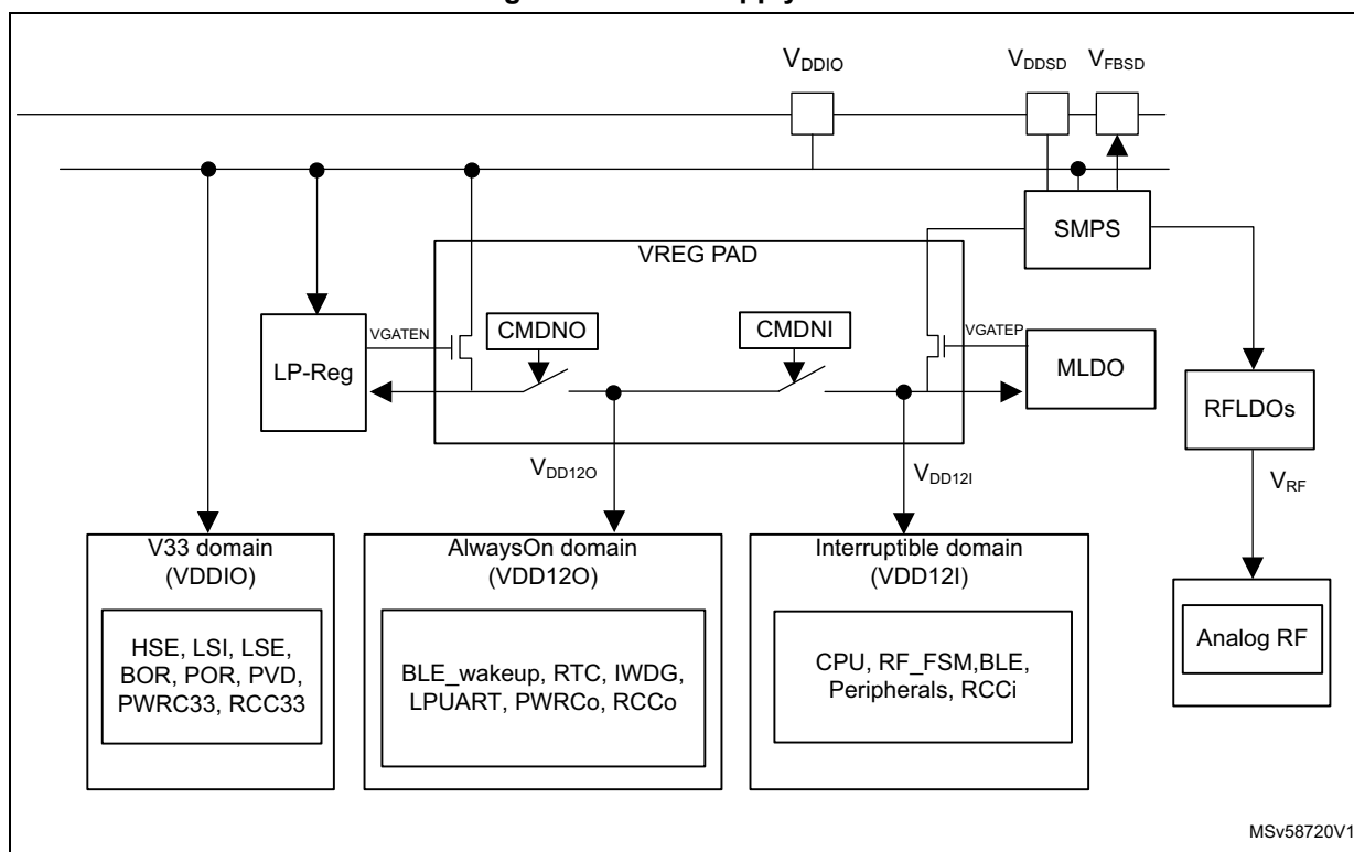
Figure 4. Power supply domains overview
