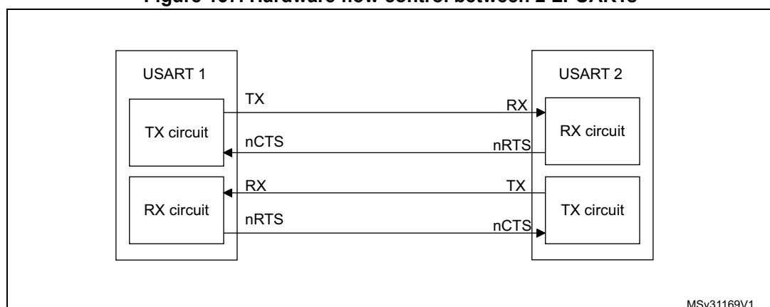
Figure 157. Hardware flow control between 2 LPUARTs
