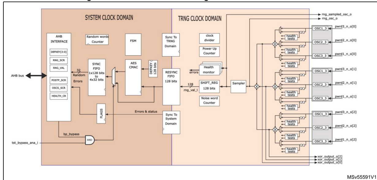
Figure 24. TRNG core embedding in the TRNG Core Block
