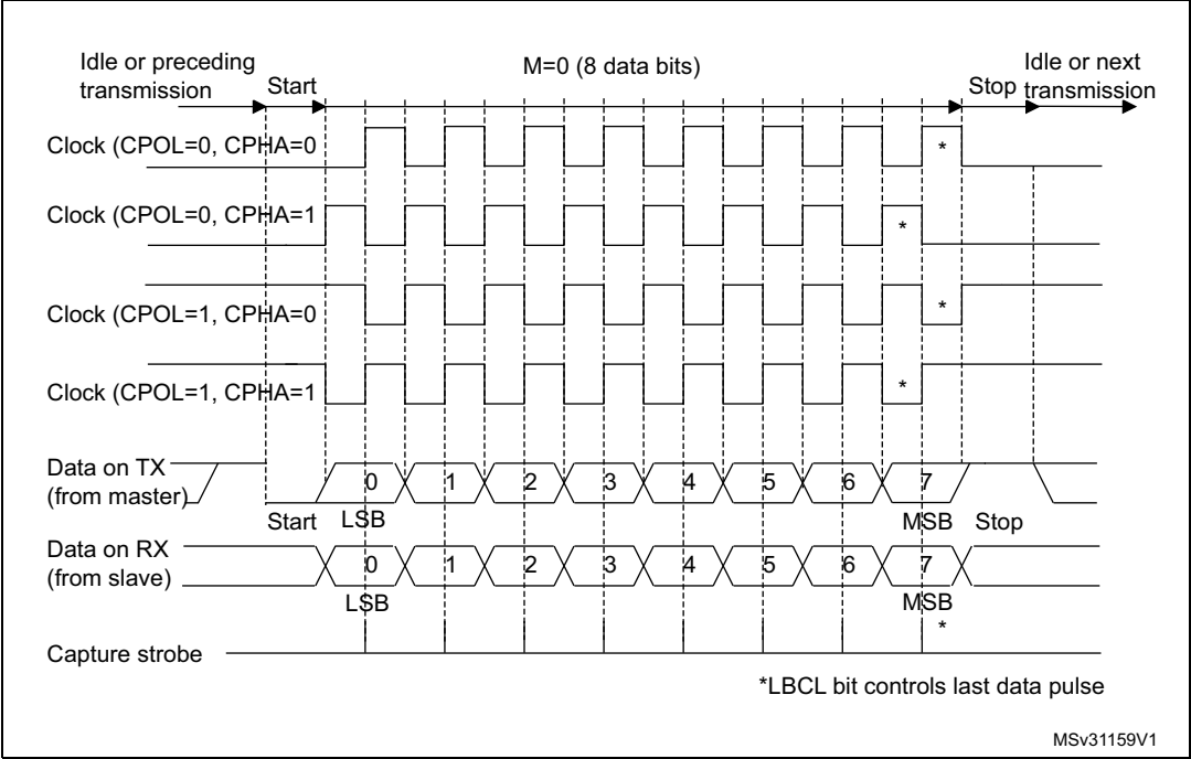
Figure 136. USART data clock timing diagram (M=0)
