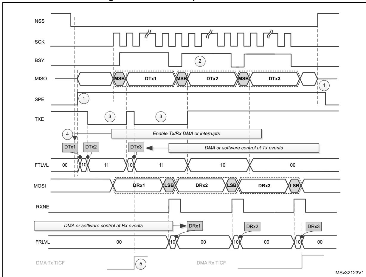
Figure 170. Slave full duplex communication
