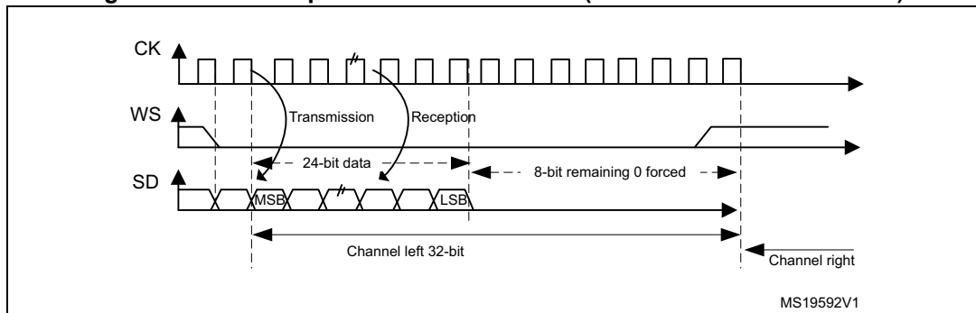
Figure 177. I 2 S Philips standard waveforms (24-bit frame with CPOL = 0)
