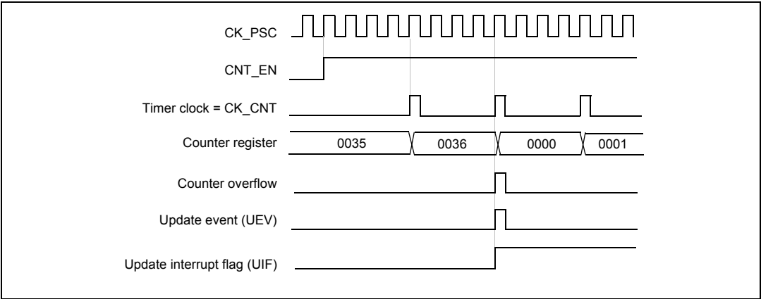
Figure 31. Counter timing diagram, internal clock divided by 4
