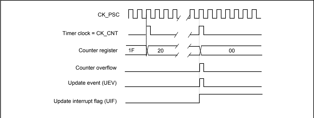
Figure 32. Counter timing diagram, internal clock divided by N
