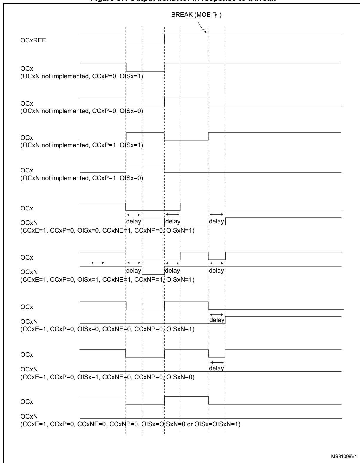
Figure 87. Output behavior in response to a break
