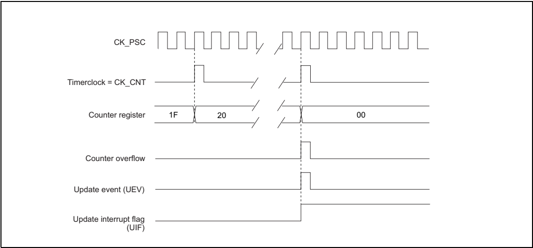
Figure 74. Counter timing diagram, internal clock divided by N
