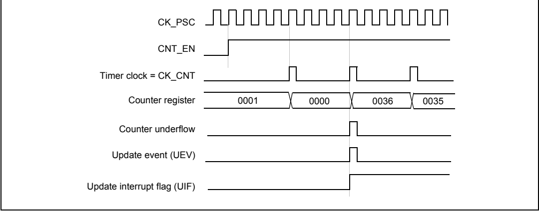
Figure 37. Counter timing diagram, internal clock divided by 4
