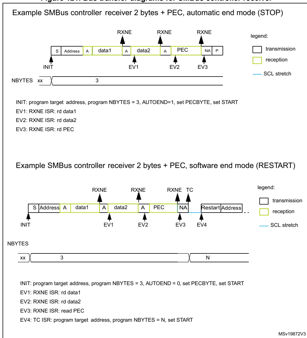
Figure 121. Bus transfer diagrams for SMBus controller receiver
