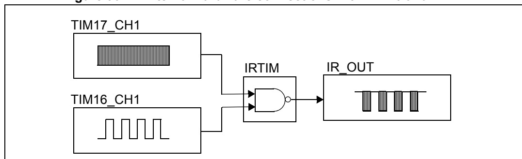
Figure 90. IR internal hardware connections with TIM16 and TIM17
