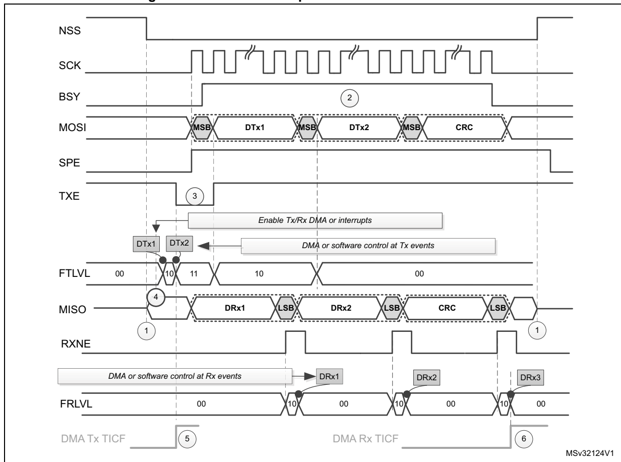
Figure 171. Master full duplex communication with CRC
