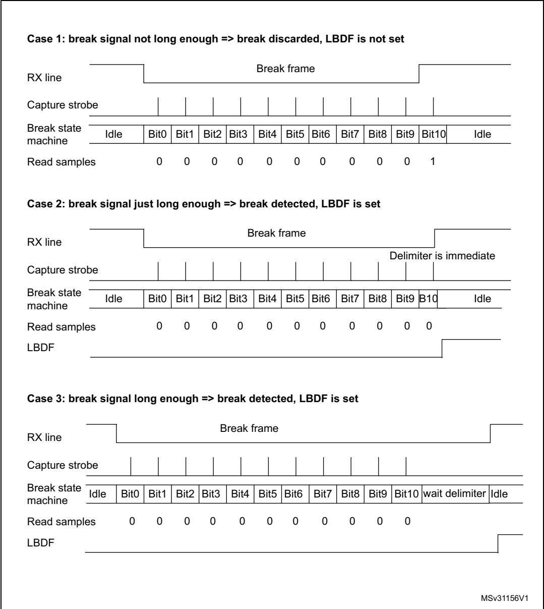
Figure 133. Break detection in LIN mode (11-bit break length - LBDL bit is set)
