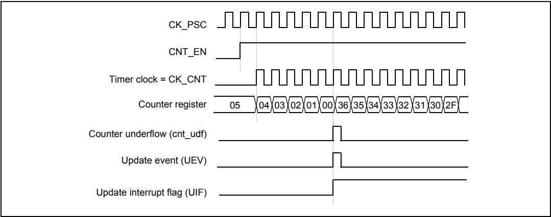
Figure 35. Counter timing diagram, internal clock divided by 1
