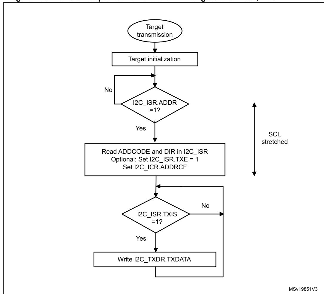
Figure 100. Transfer sequence flowchart for I2C target transmitter, NOSTRETCH=0
