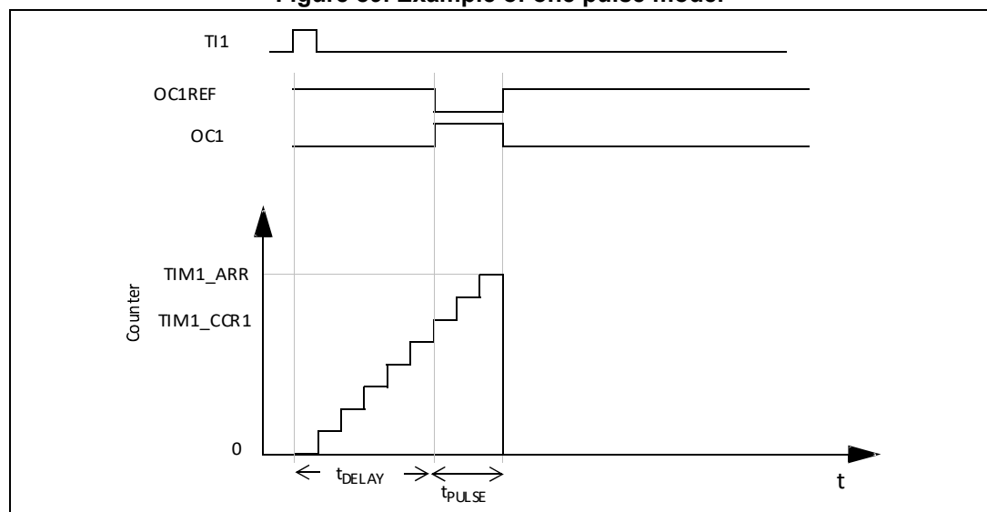
Figure 89. Example of one pulse mode.
