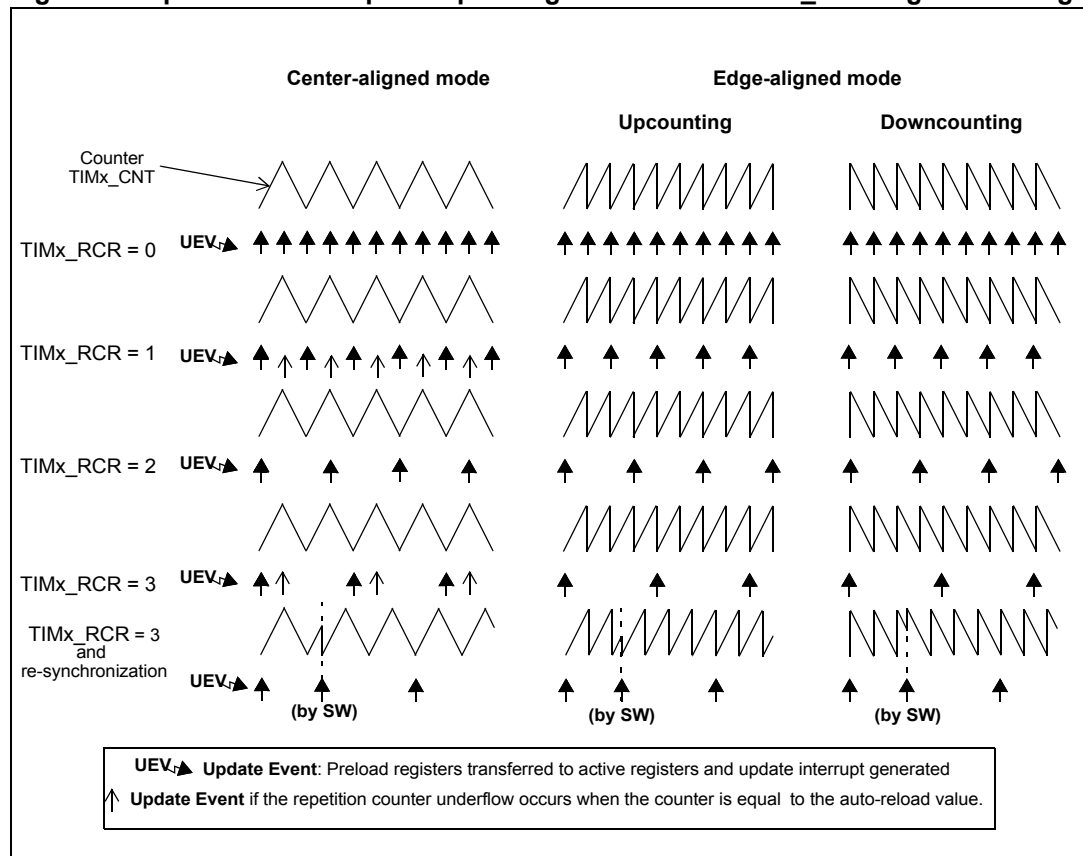
Figure 46. Update rate examples depending on mode and TIMx_RCR register settings
