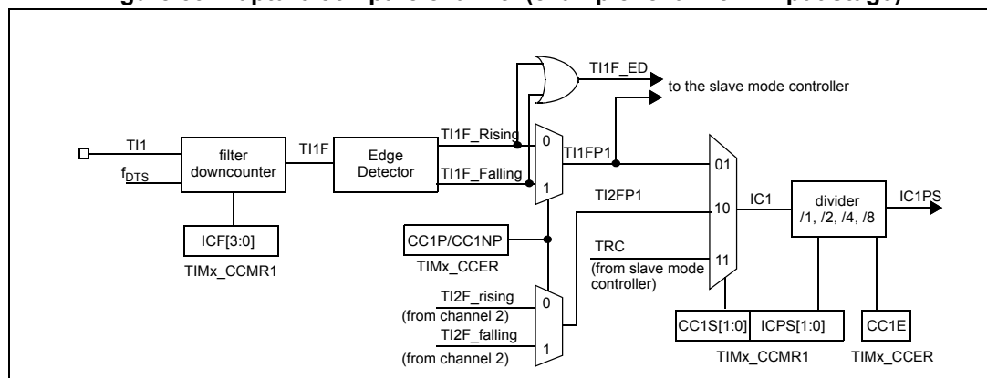
Figure 53. Capture/compare channel (example: channel 1 input stage)
