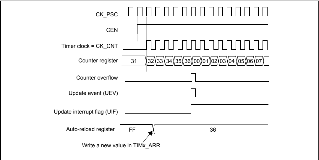
Figure 33. Counter timing diagram, update event when ARPE=0 (TIMx_ARR not preloaded)
