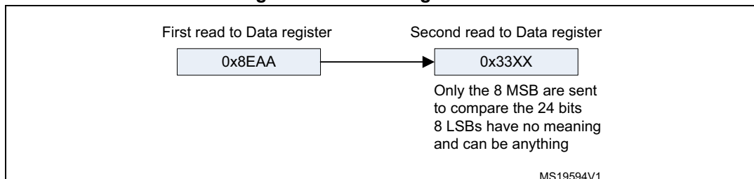
Figure 179. Receiving 0x8EAA33
