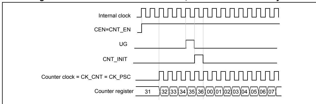
Figure 48. Control circuit in normal mode, internal clock divided by 1
