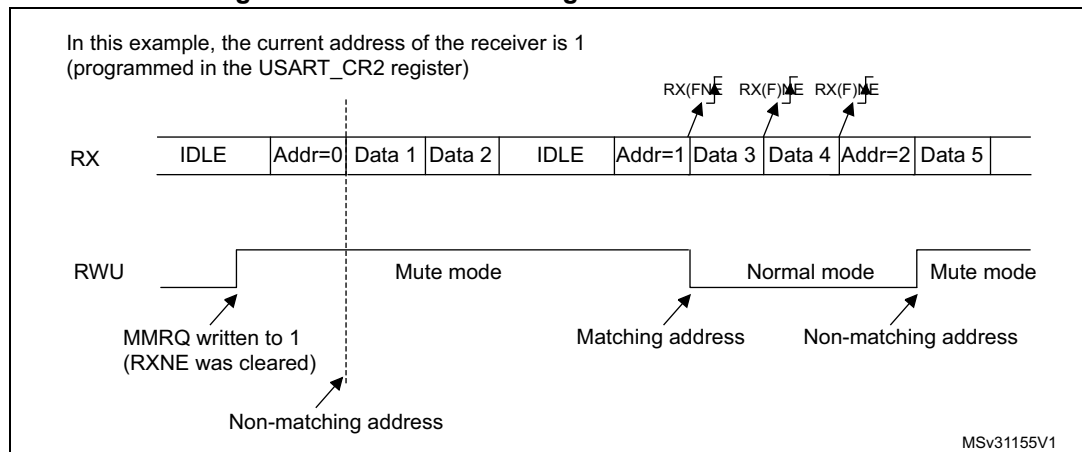
Figure 132. Mute mode using address mark detection
