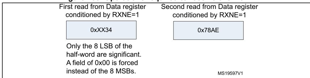
Figure 188. Operations required to receive 0x3478AE
