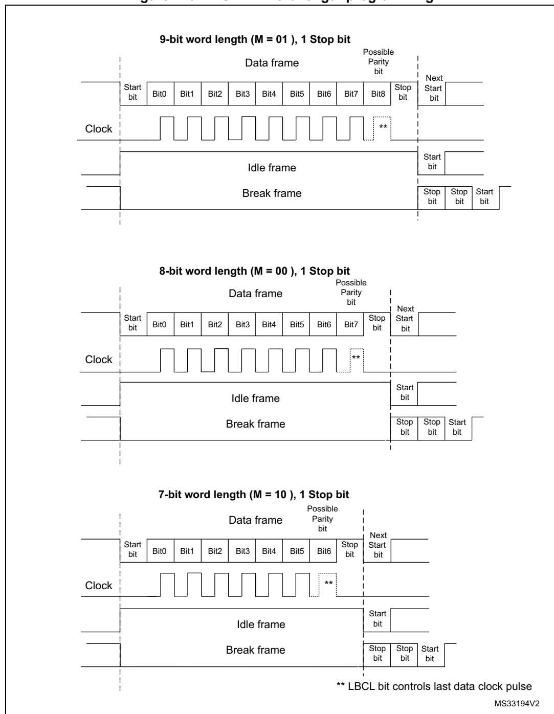
Figure 149. LPUART Word length programming
