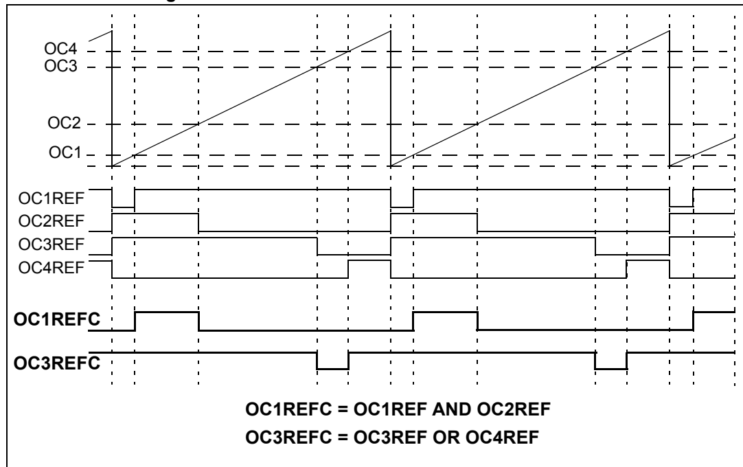
Figure 61. Combined PWM mode on channel 1 and 3
