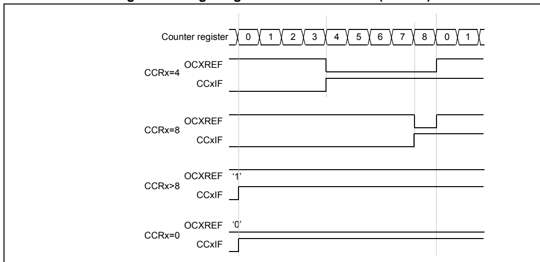
Figure 58. Edge-aligned PWM waveforms (ARR=8)
