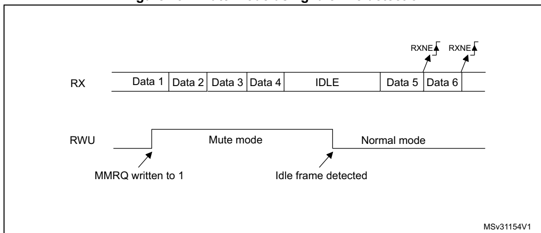
Figure 131. Mute mode using Idle line detection
