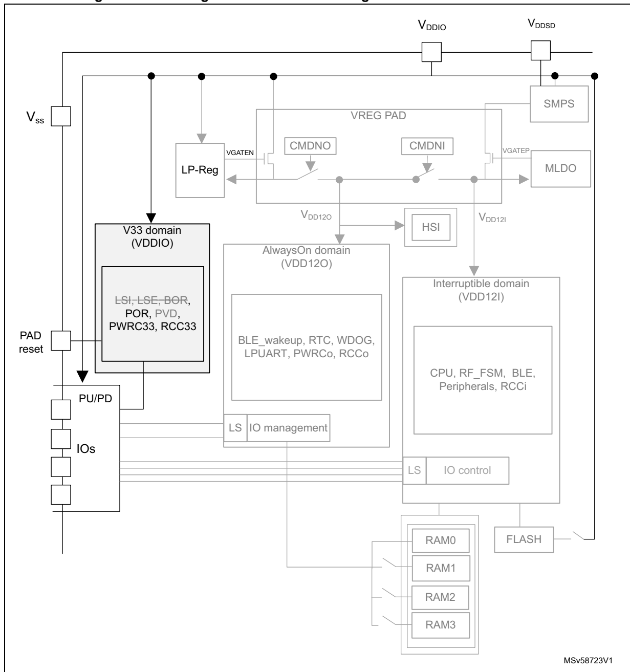
Figure 8. Power regulators and SMPS configuration in Shutdown mode (a)
