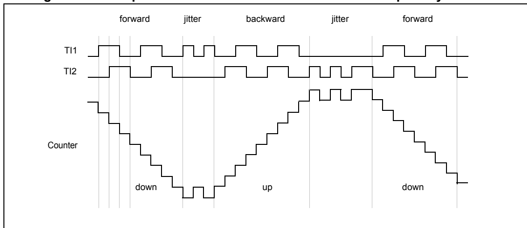
Figure 66. Example of encoder interface mode with TI1FP1 polarity inverted.
