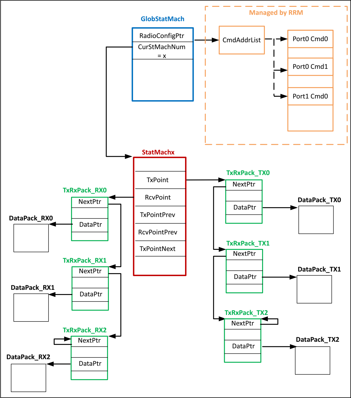
Figure 203. RAM tables dependencies overview
