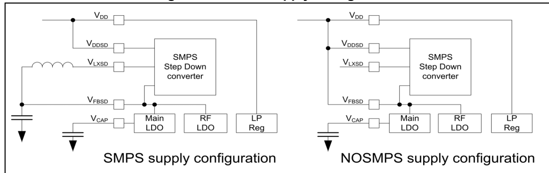
Figure 10. Power supply configuration
