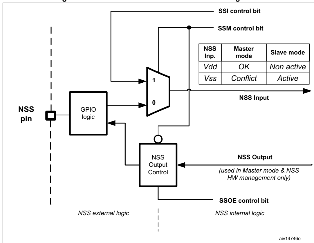
Figure 165. Hardware/software slave select management
