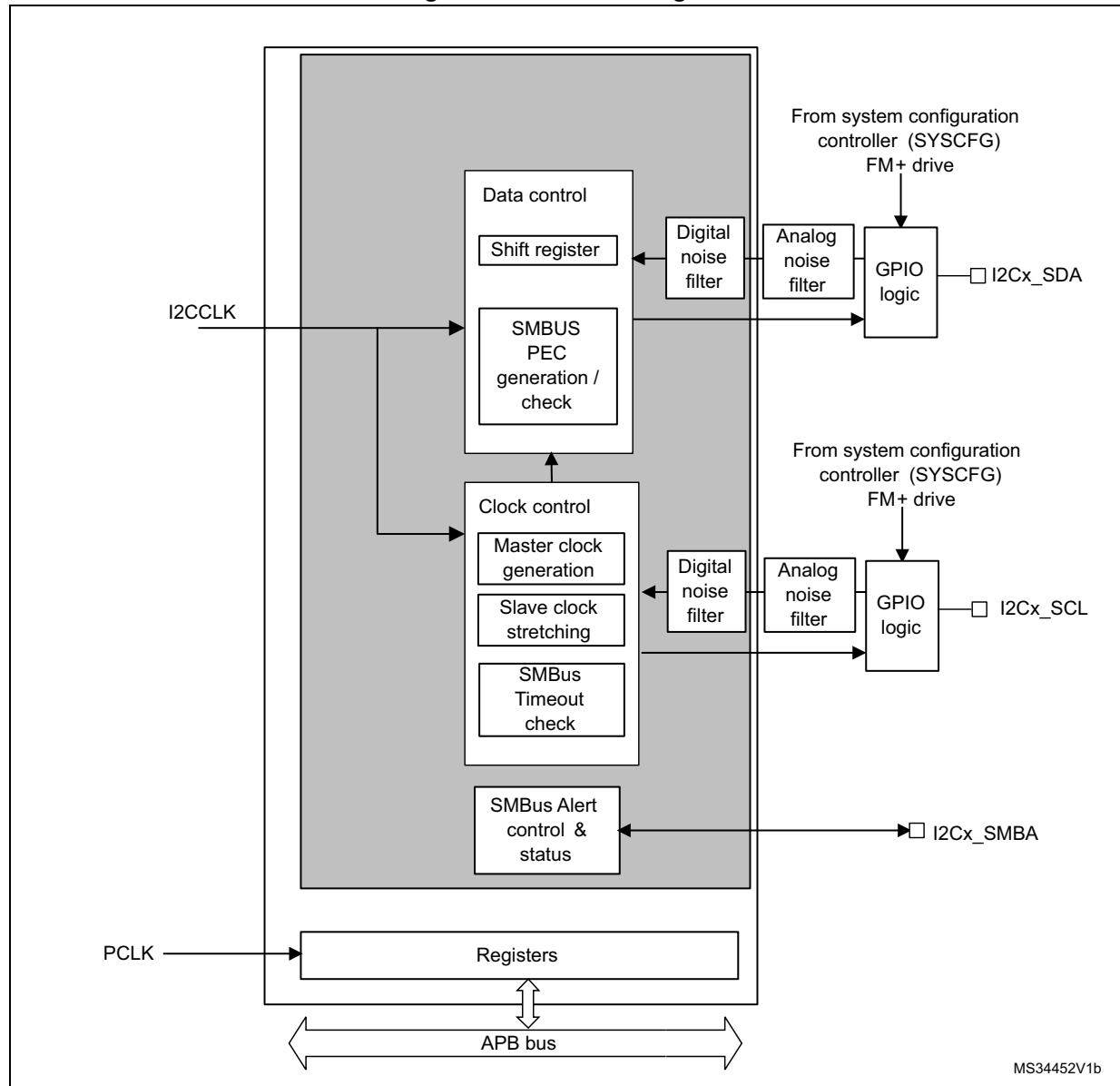
Figure 93. I2C block diagram
