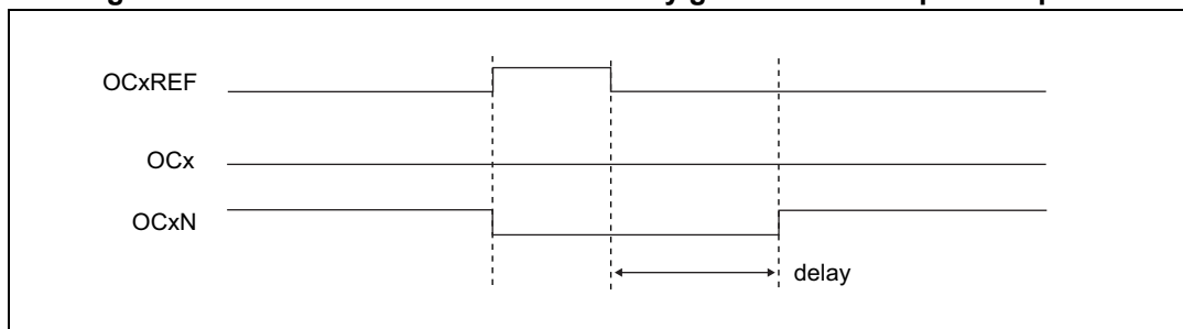
Figure 86. Dead-time waveforms with delay greater than the positive pulse.
