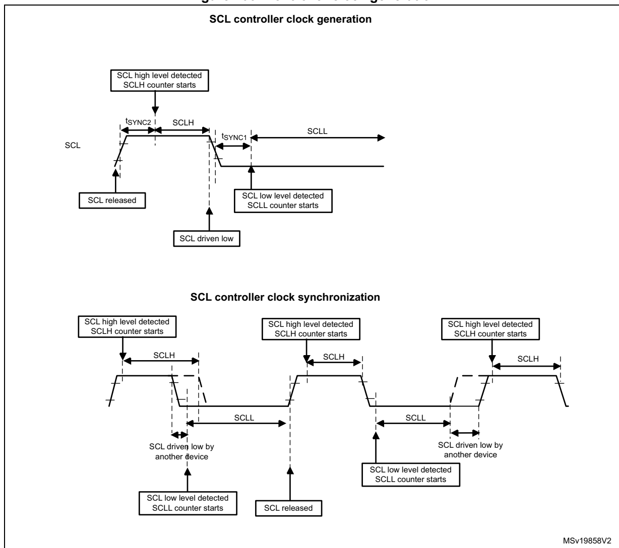
Figure 106. Controller clock generation
