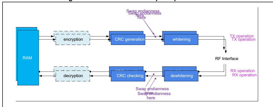
Figure 208. MSBFirst feature principle overview
