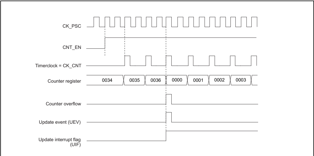
Figure 72. Counter timing diagram, internal clock divided by 2
