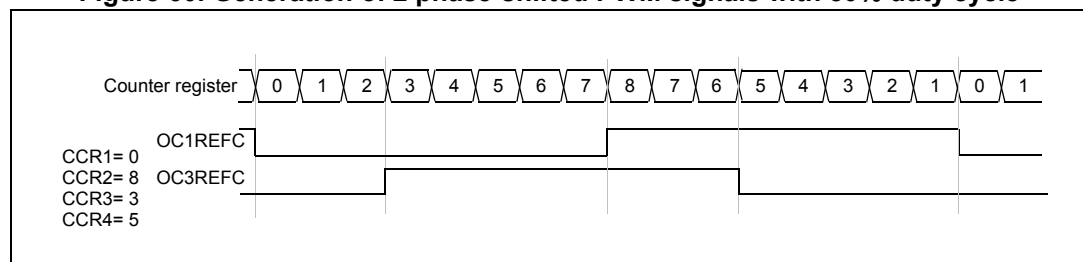
Figure 60. Generation of 2 phase-shifted PWM signals with 50% duty cycle
