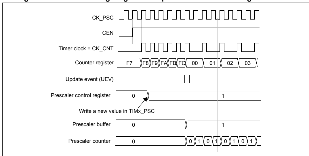
Figure 27. Counter timing diagram with prescaler division change from 1 to 2
