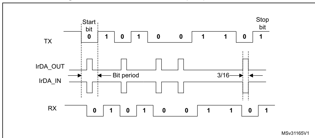
Figure 142. IrDA data modulation (3/16) -Normal Mode
