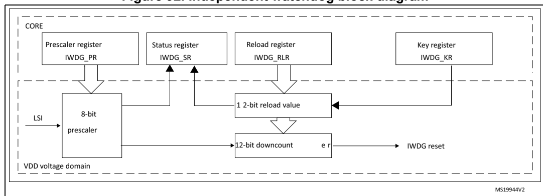
Figure 92. Independent watchdog block diagram
