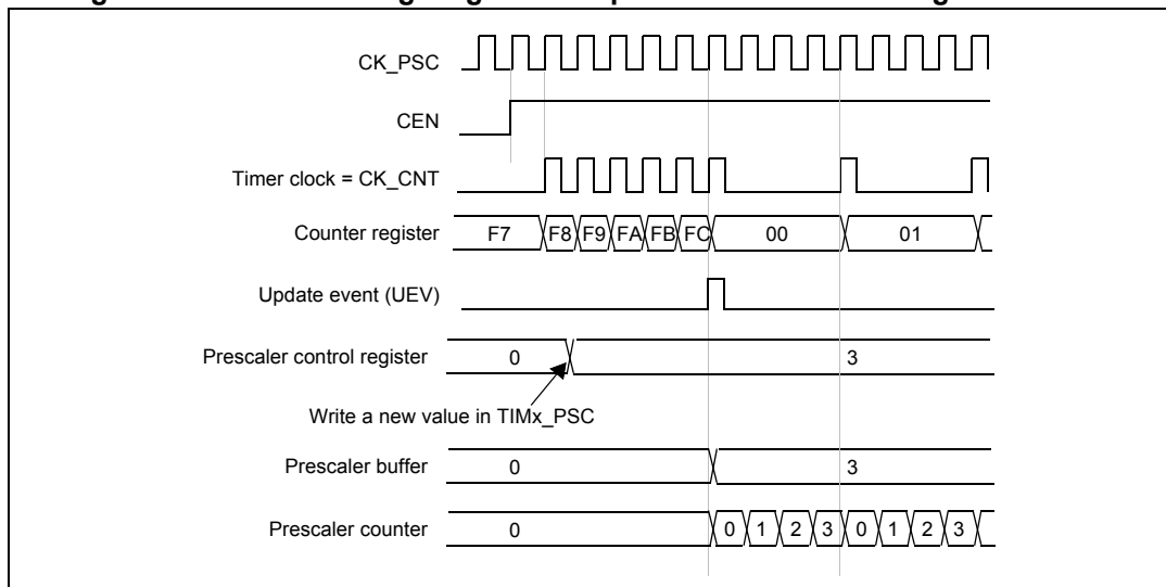
Figure 28. Counter timing diagram with prescaler division change from 1 to 4
