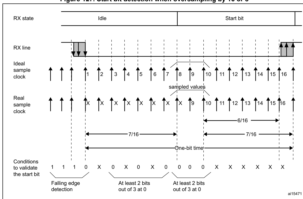
Figure 127. Start bit detection when oversampling by 16 or 8
