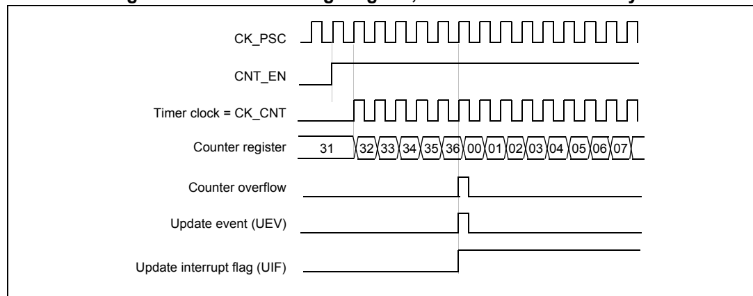
Figure 29. Counter timing diagram, internal clock divided by 1
