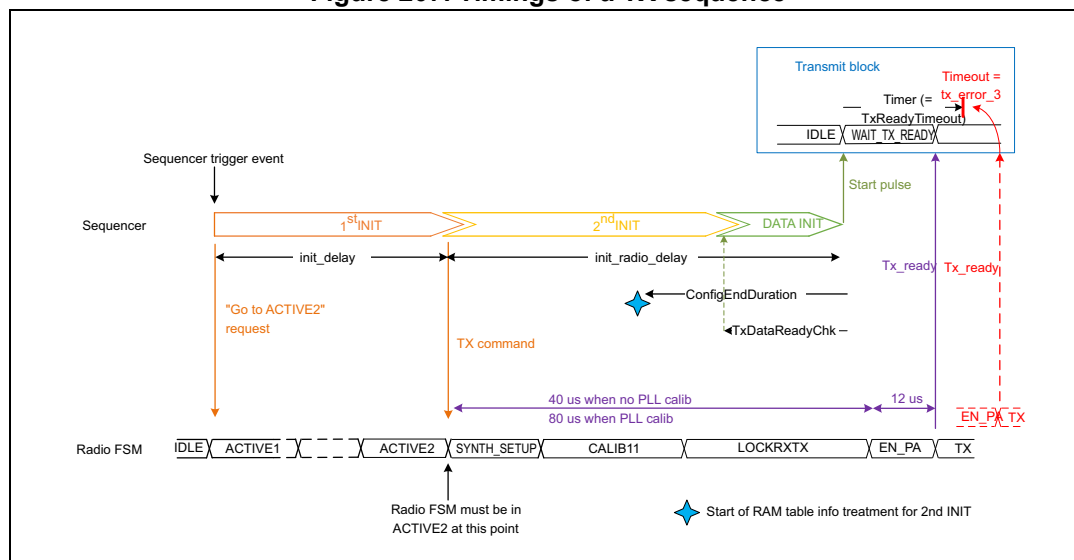
Figure 207. Timings of a TX sequence
