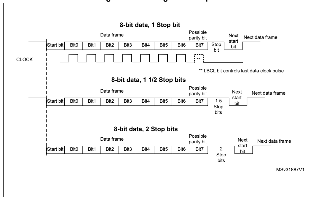
Figure 125. Configurable stop bits
