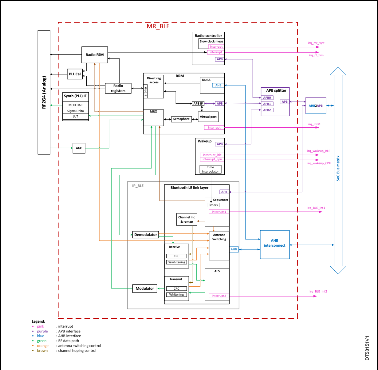
Figure 195. Radio controller MR_BLE architecture overview
