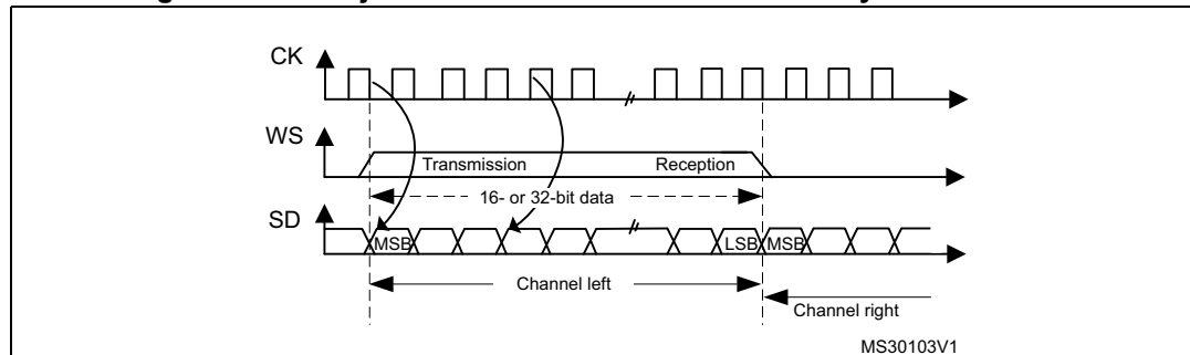
Figure 185. LSB justified 16-bit or 32-bit full-accuracy with CPOL = 0
