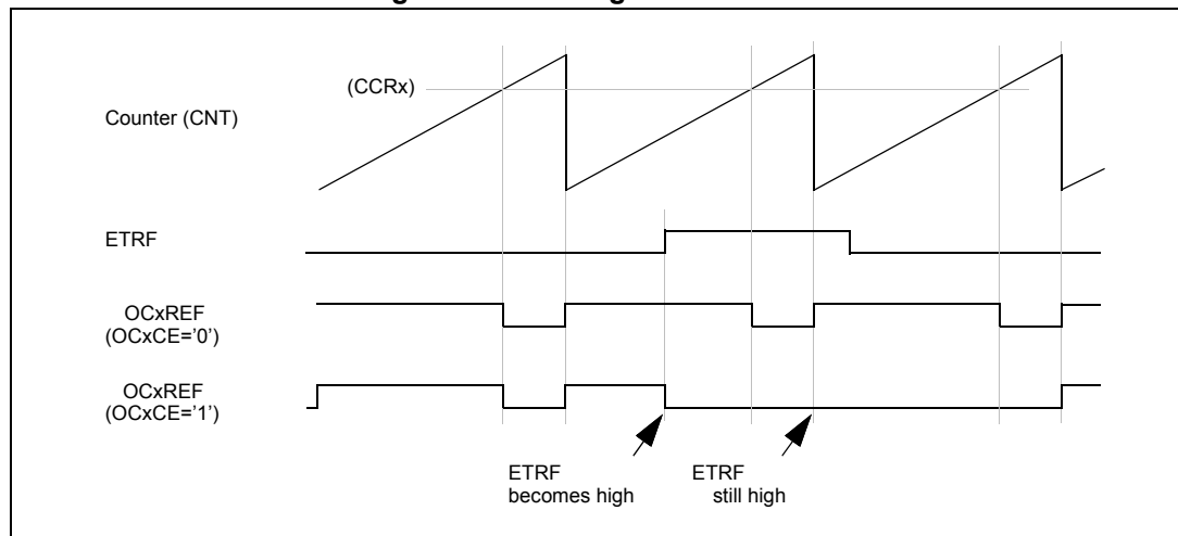
Figure 62. Clearing TIMx OCxREF
