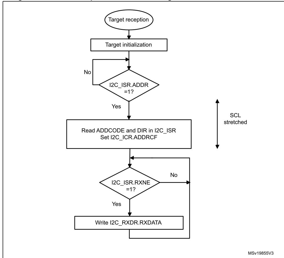
Figure 103. Transfer sequence flowchart for target receiver with NOSTRETCH=0
