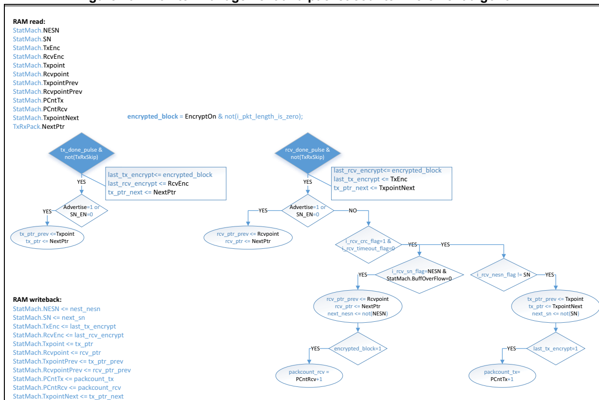
Figure 204. Pointer management and packet counter increment algorithm
