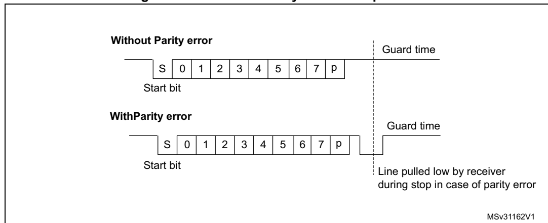
Figure 139. ISO 7816-3 asynchronous protocol
