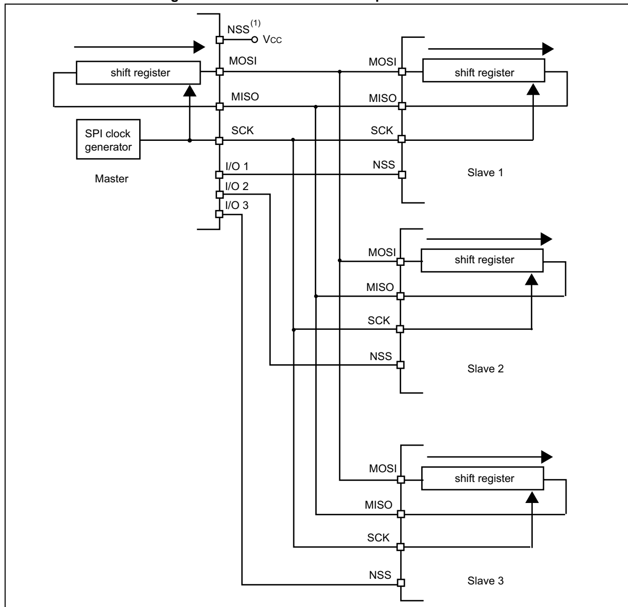
Figure 164. Master and three independent slaves
