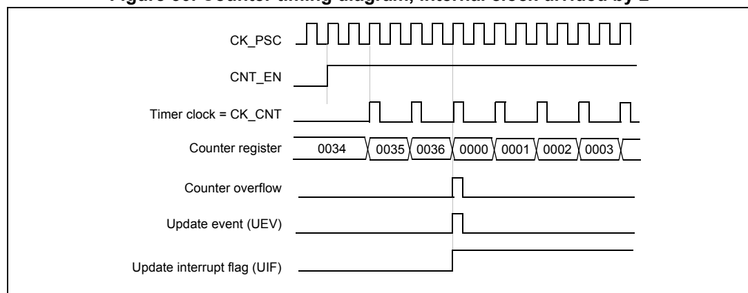
Figure 30. Counter timing diagram, internal clock divided by 2
