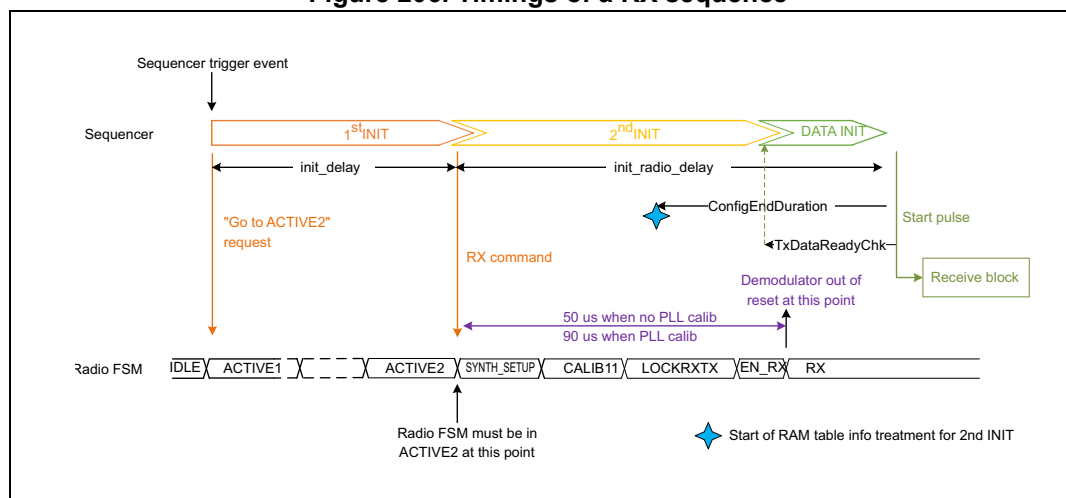
Figure 206. Timings of a RX sequence
