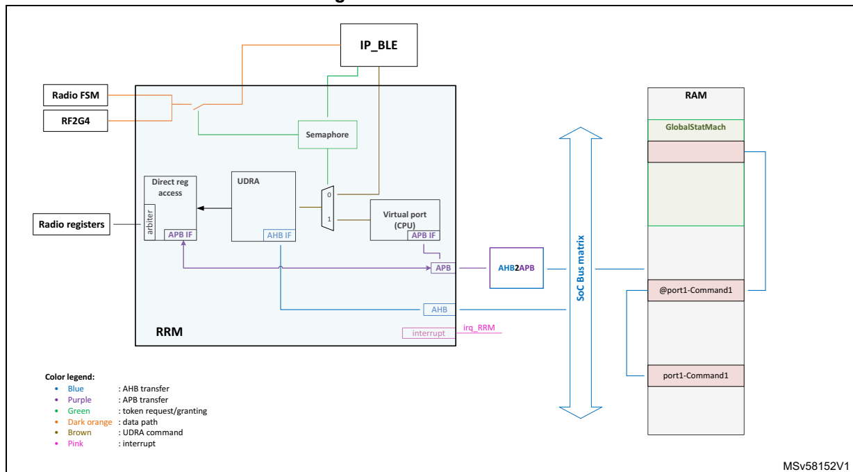
Figure 196. RRM overview
