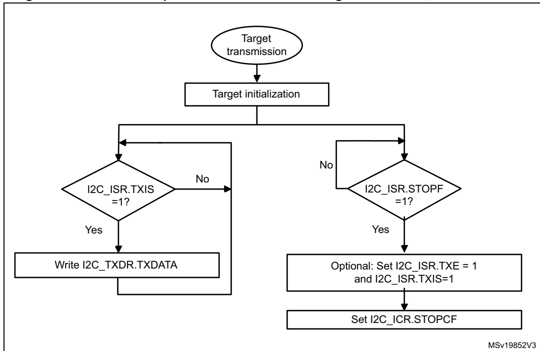
Figure 101. Transfer sequence flowchart for I2C target transmitter, NOSTRETCH=1
