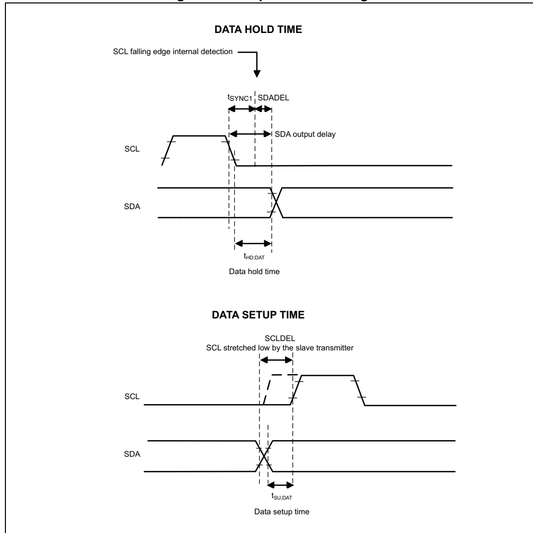
Figure 95. Setup and hold timings
