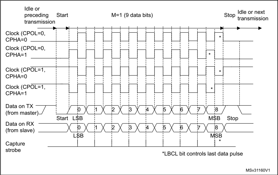
Figure 137. USART data clock timing diagram (M bits = 01)
