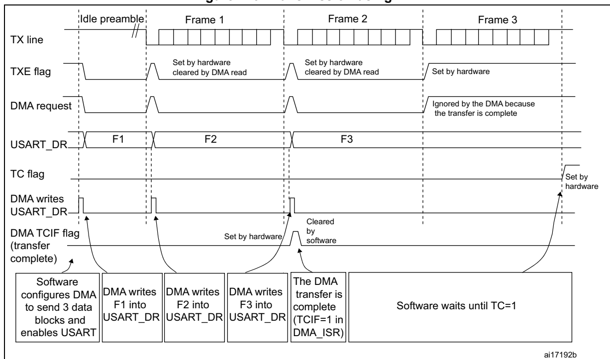
Figure 143. Transmission using DMA
