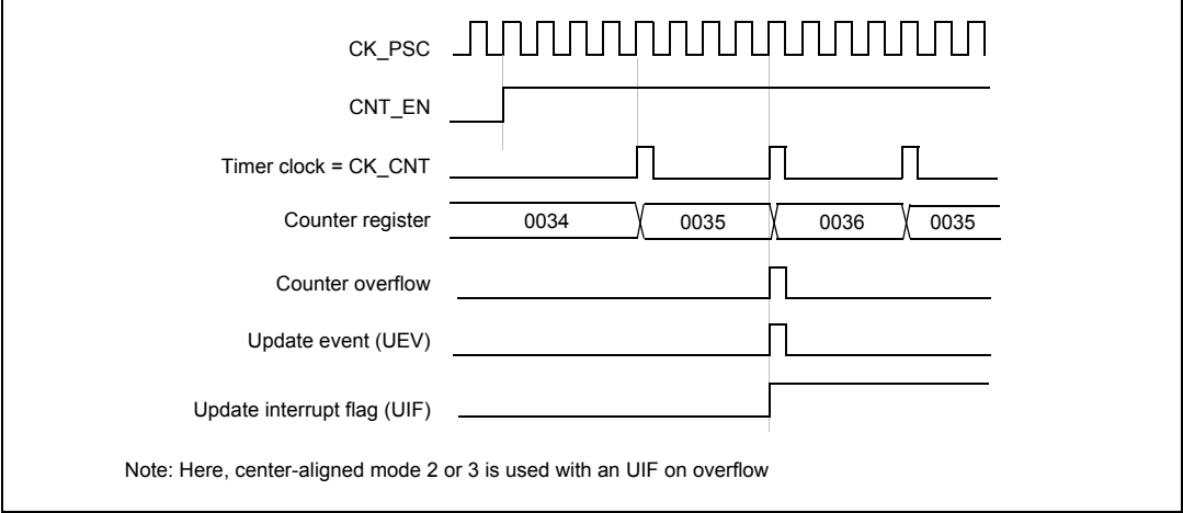
Figure 42. Counter timing diagram, internal clock divided by 4, TIMx_ARR=0x36
