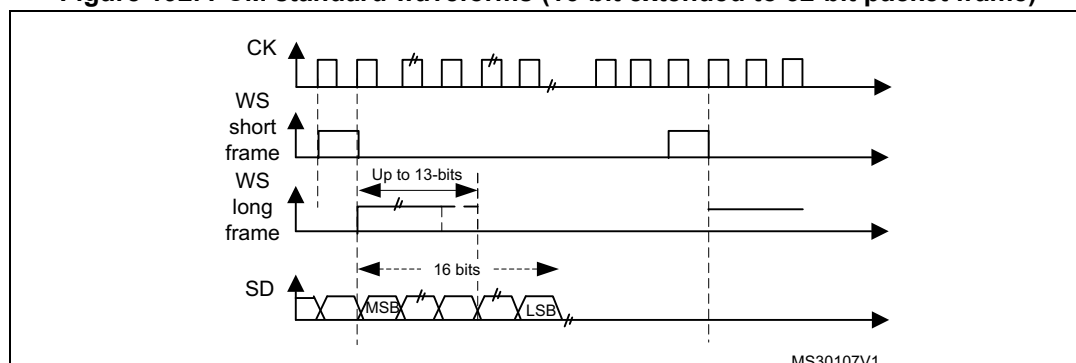
Figure 192. PCM standard waveforms (16-bit extended to 32-bit packet frame)
