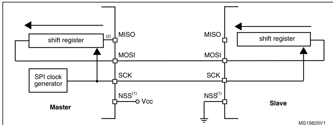
Figure 163. Simplex single master/single slave application (master in transmit-only/ slave in receive-only mode)
