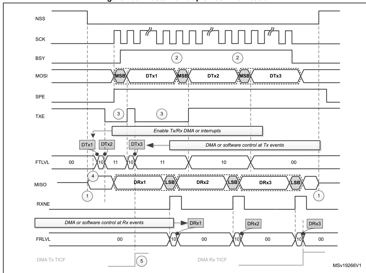
Figure 169. Master full duplex communication
