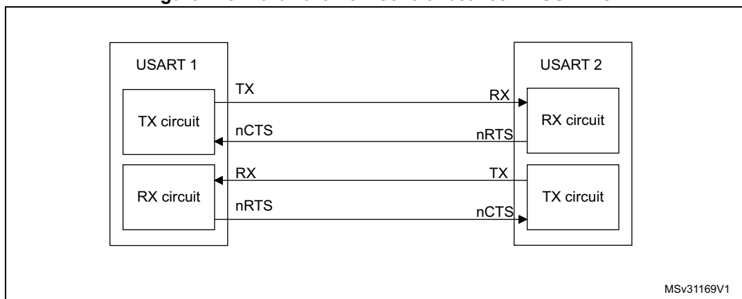
Figure 145. Hardware flow control between 2 USARTs
