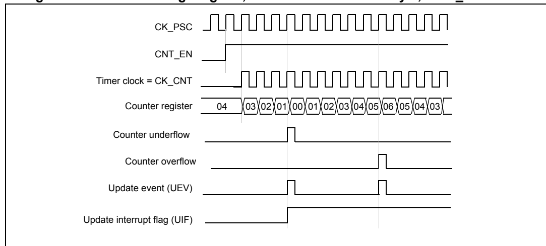
Figure 40. Counter timing diagram, internal clock divided by 1, TIMx_ARR = 0x6
