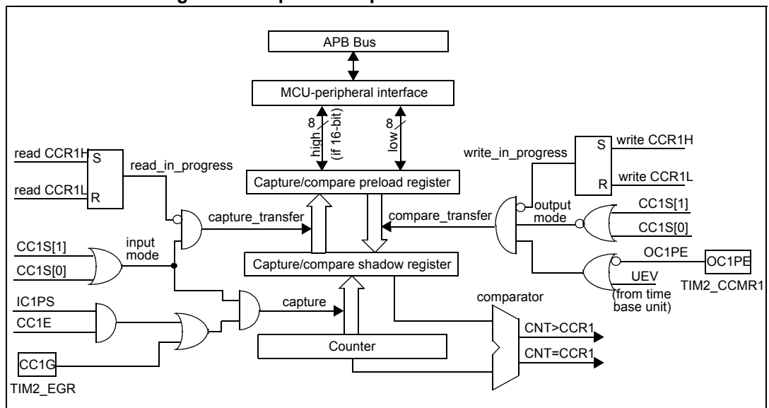
Figure 80. Capture/compare channel 1 main circuit
