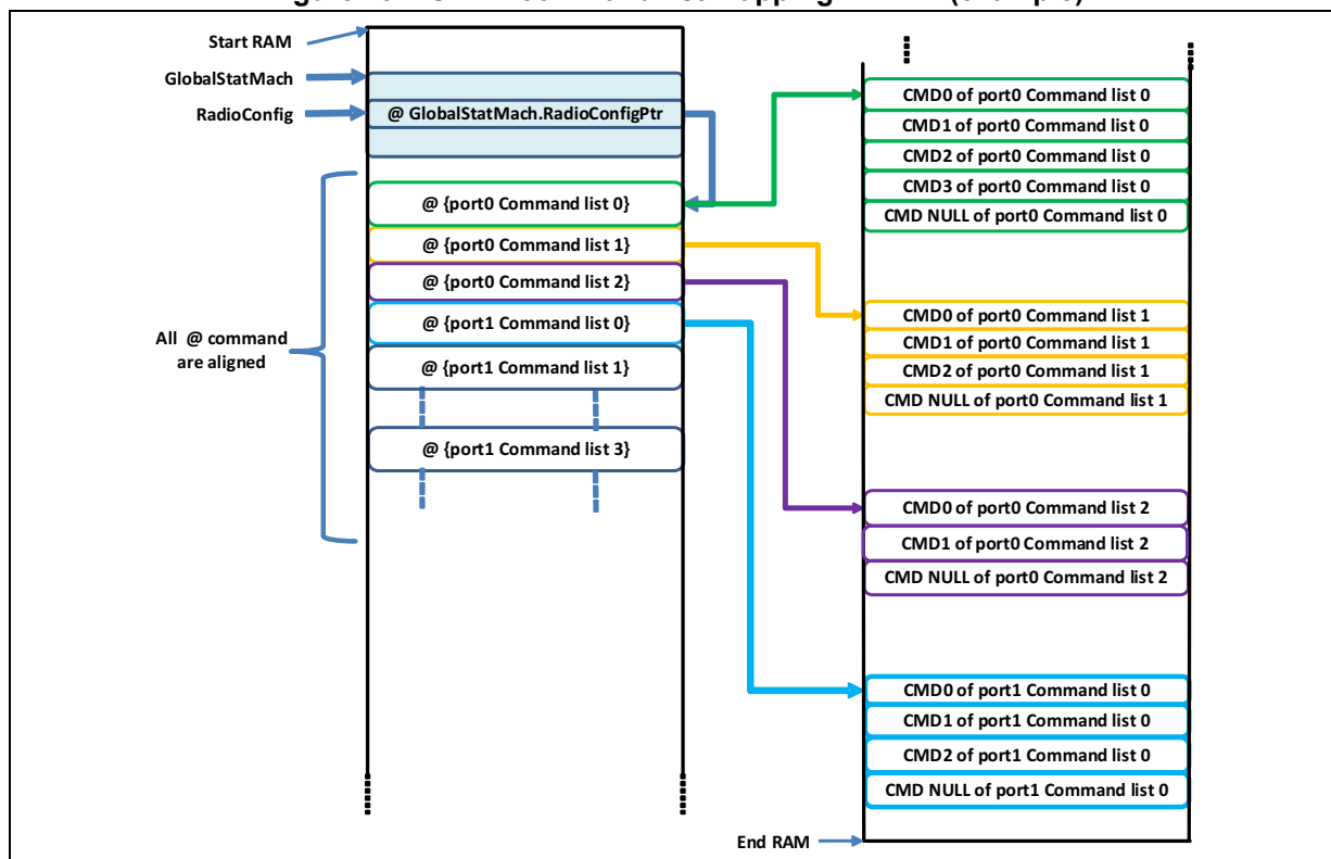
Figure 197. UDRA command list mapping in RAM (example)
