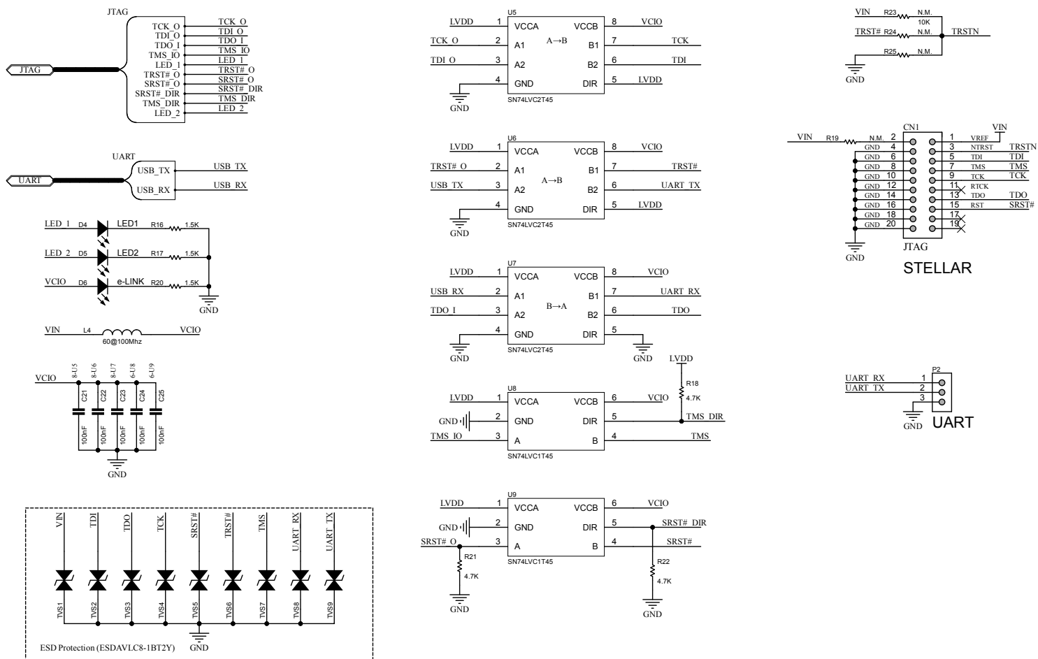
Figure 3. AEK-MCU-SRLNK circuit schematic (3 of 3)
