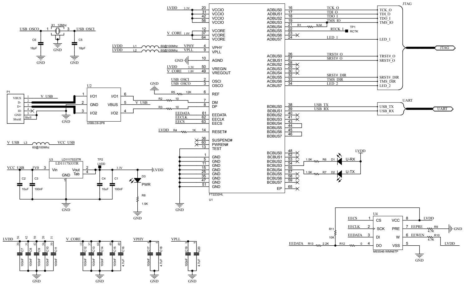
Figure 2. AEK-MCU-SRLNK circuit schematic (2 of 3)
