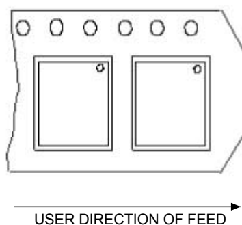
Figure 4. Device orientation on tape
