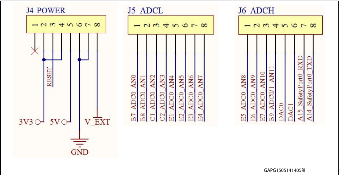
Figure 25. Connectors Arduino-compatible (II)
