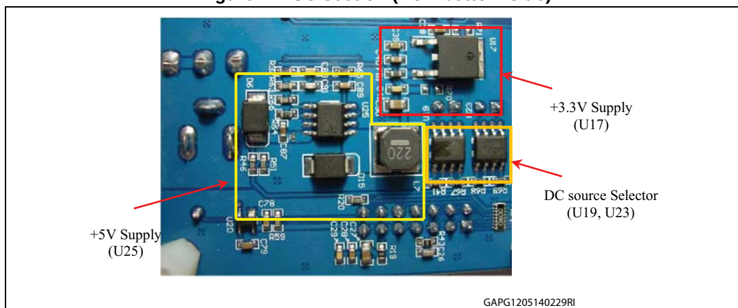
Figure 4. PSU section (PCB bottom side)
