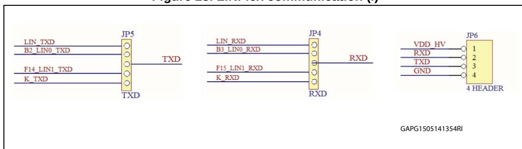
Figure 23. LINFlex communication (I)
