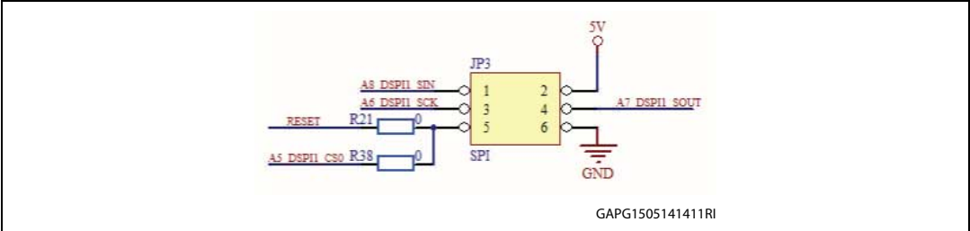
Figure 27. Connectors Arduino-compatible (IV)
