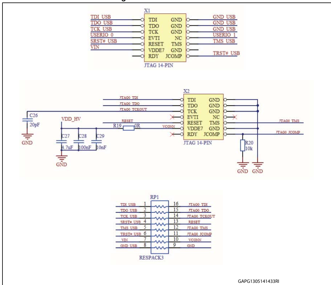
Figure 17. JTAG connectors
