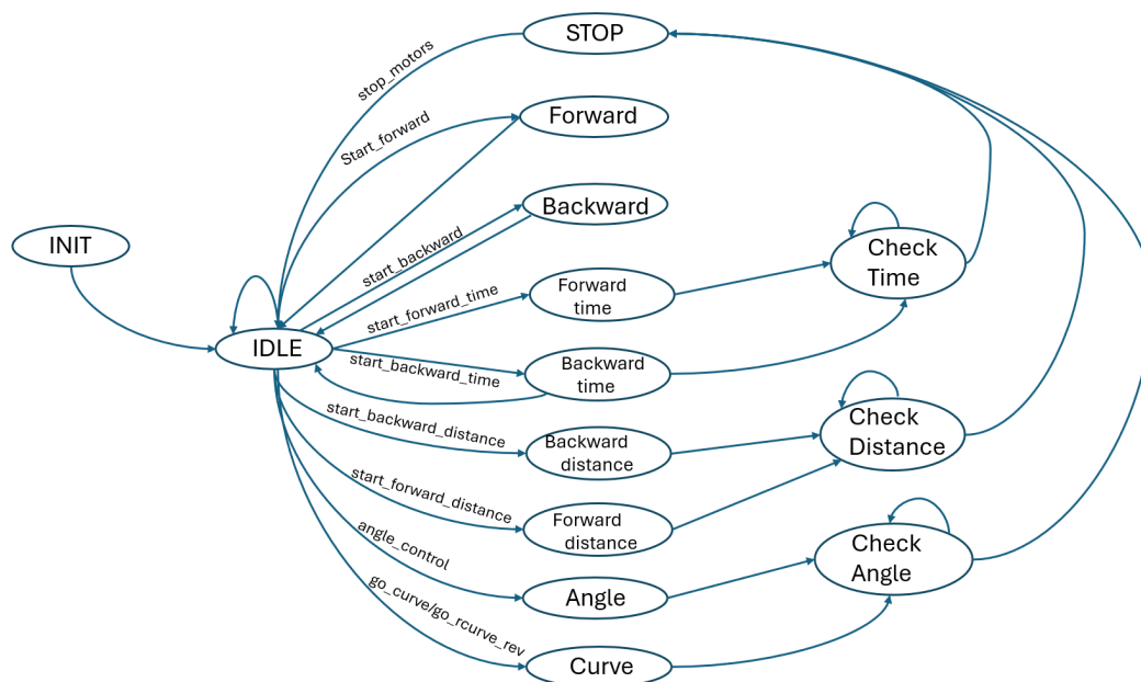
Figure 38. State Machine for STSW-ROBKIT1-2
