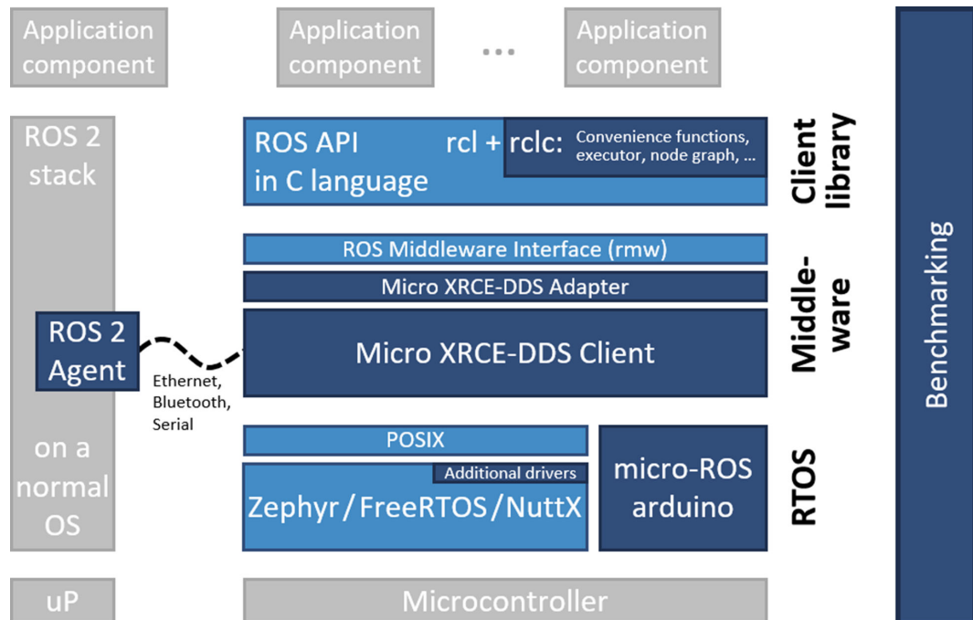
Figure 36. Micro-ROS Software Architecture
