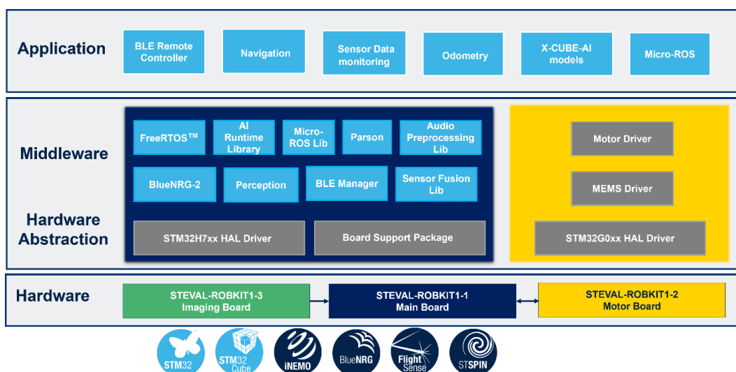
Figure 7. High Level Firmware architecture of Robotics evaluation kit
