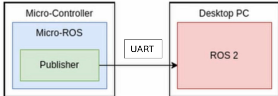
Figure 35. Micro-ROS System Block Diagram
