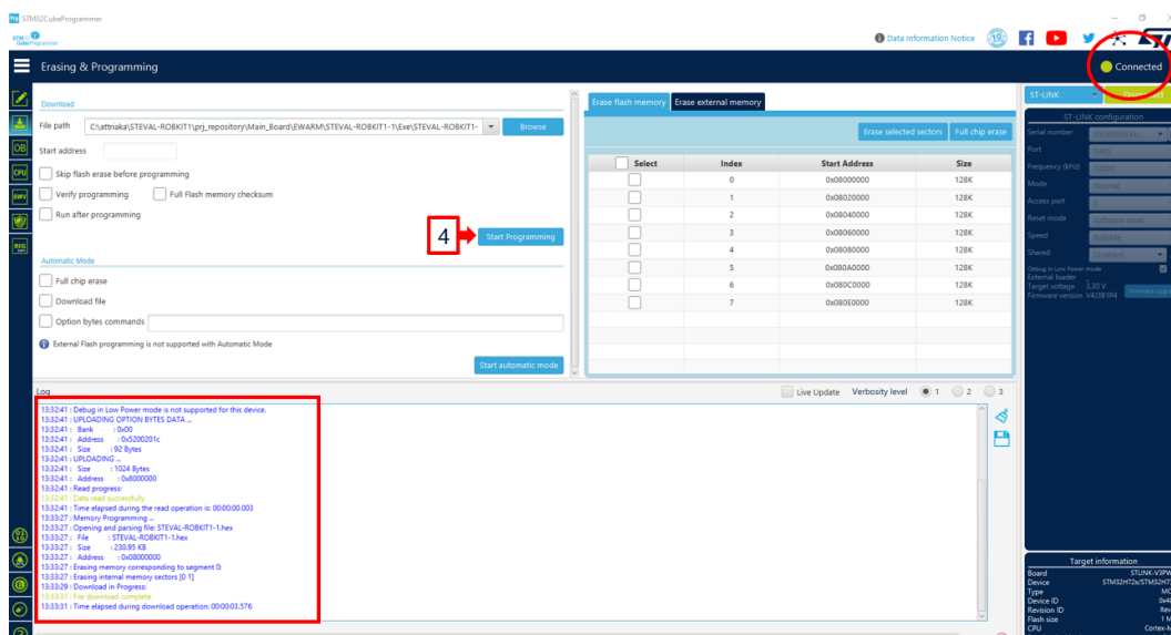
Figure 17. Steps to flash the binary in STEVAL-ROBKIT1-1 using STM32CubeProgrammer
