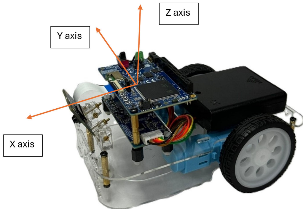
Figure 41. STEVAL-ROBKIT1 X, Y and Z Coordinates for E-Compass
