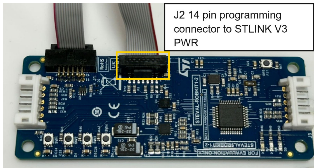
Figure 22. Connection with STLINK Debugger
